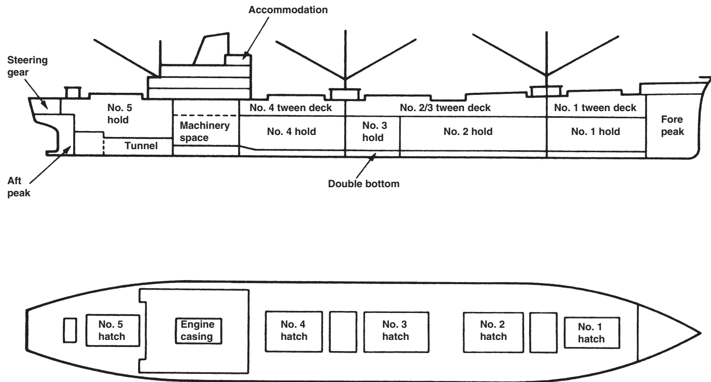
Figure 17.1 General cargo ship
