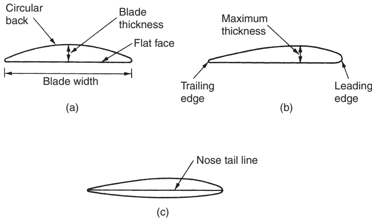
Figure 10.5 (a) Flat face, circular back; (b) Aerofoil; (c) Cambered face
