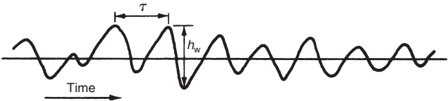
Figure 6.4 Wave record
