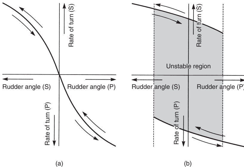
Figure 13.4 Spiral manoeuvre
