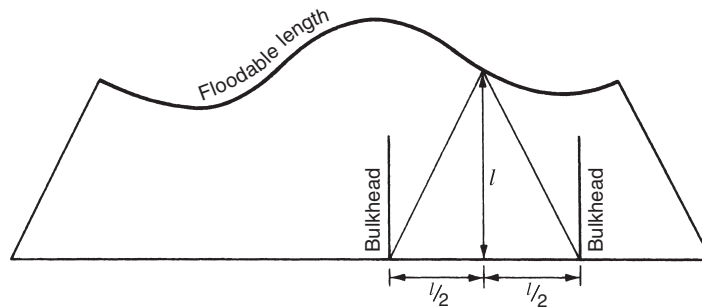
Figure 7.16 Floodable length
