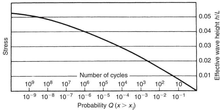
Figure 15.4 Probability curve
