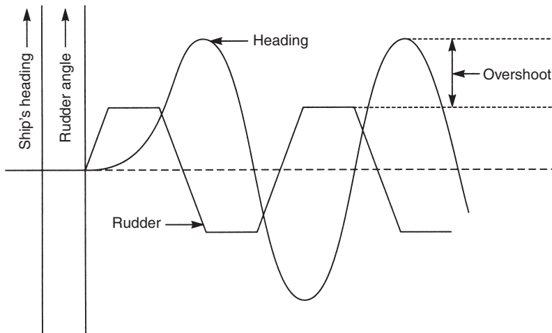
Figure 13.3 Zig-zag manoeuvre
