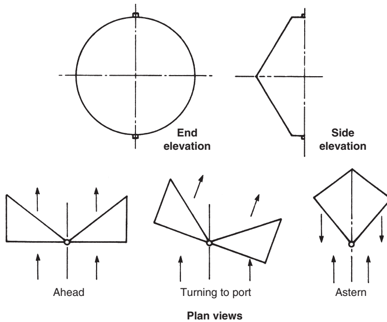
Figure 13.9 Kitchen rudder
