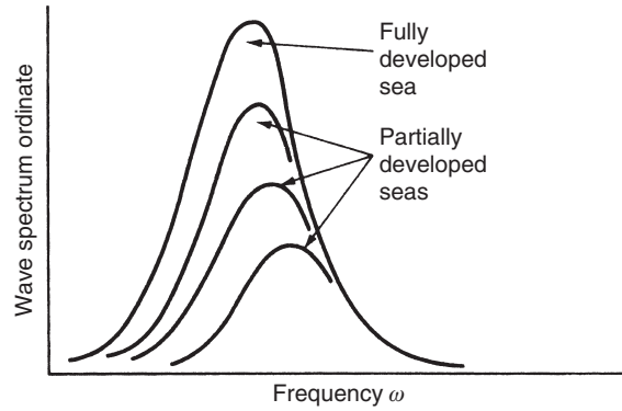
Figure 6.7 Developing spectra
