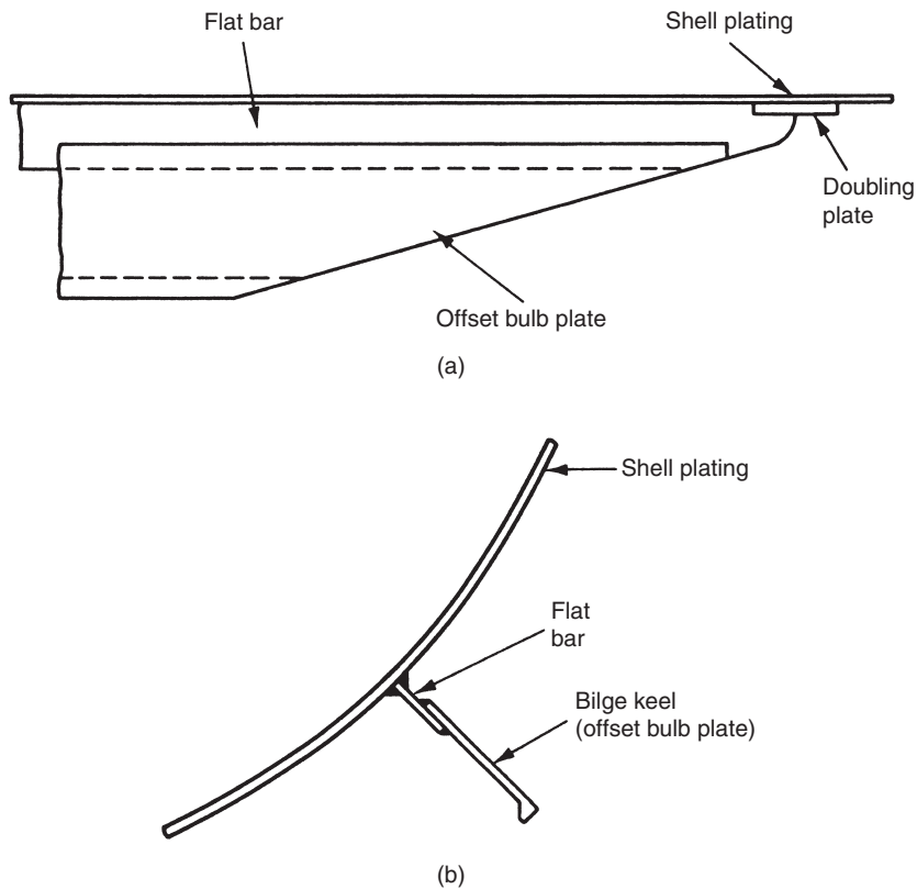
Figure 12.4 Bilge keel
