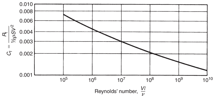
Figure 9.7 Schoenherr line
