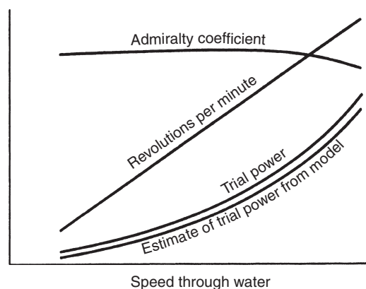
Figure 10.22 Trials data
