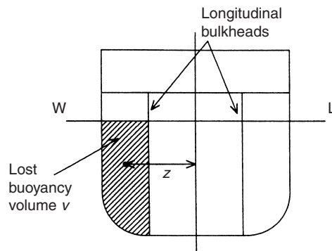
Figure 7.14 Asymmetrical flooding
