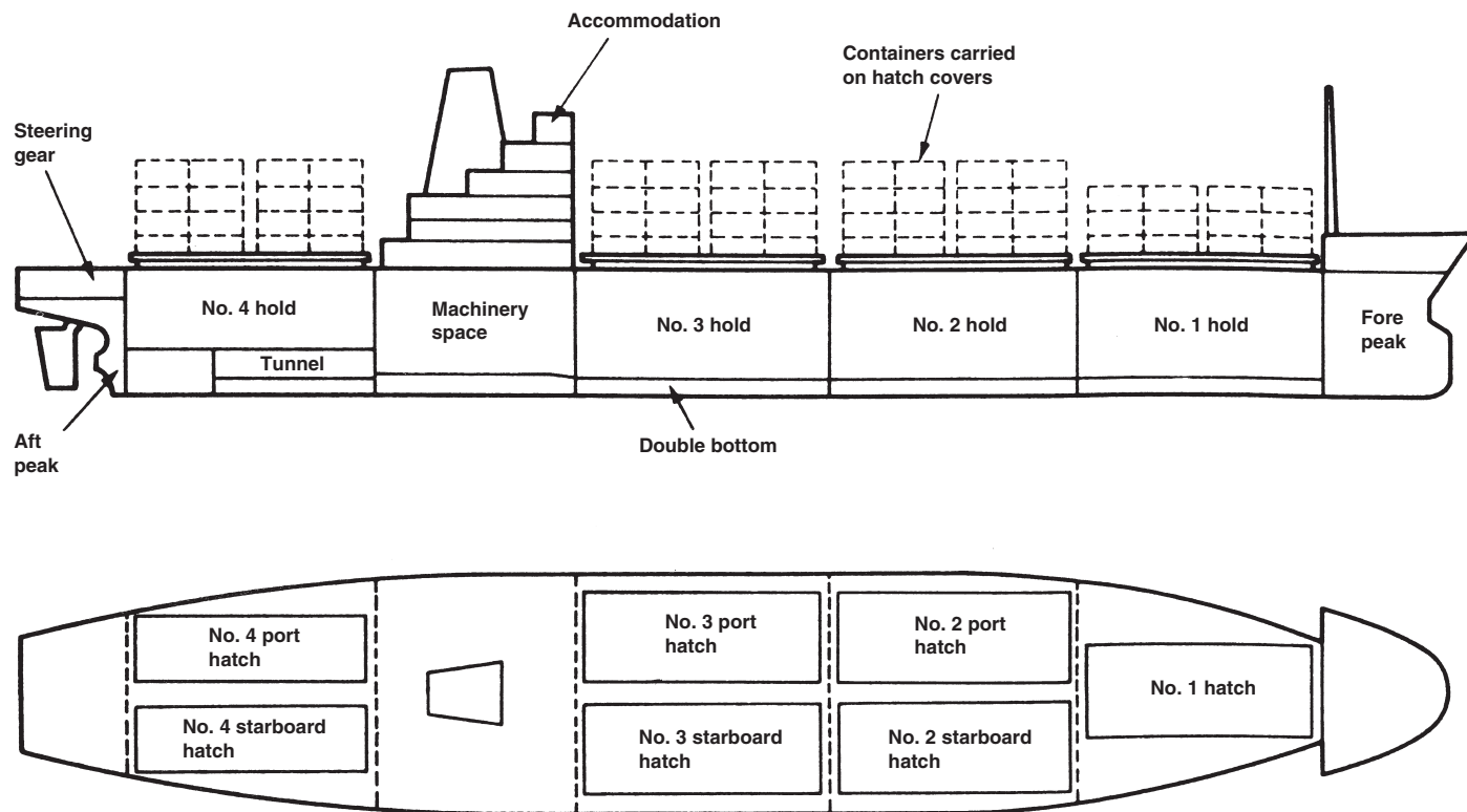
Figure 17.2 Container ship
