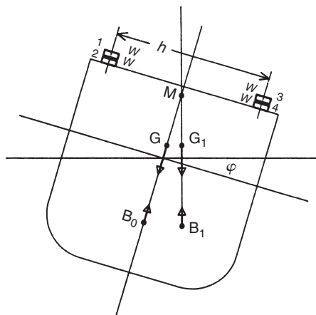
Figure 5.18 Inclining experiment
