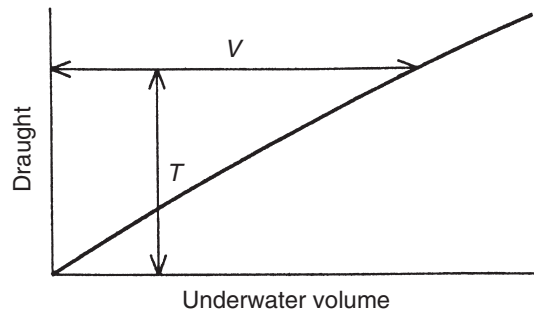
Figure 5.3 Volume curve
