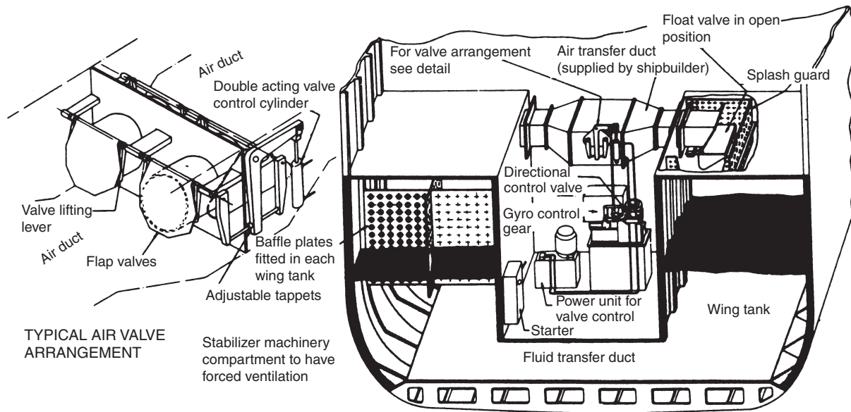
Figure 12.6 Tank stabilizer
