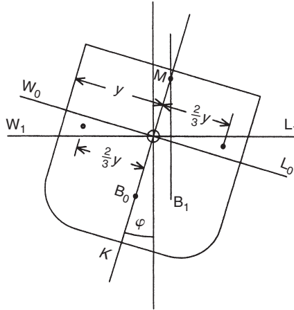
Figure 5.7 Transverse metacentre
