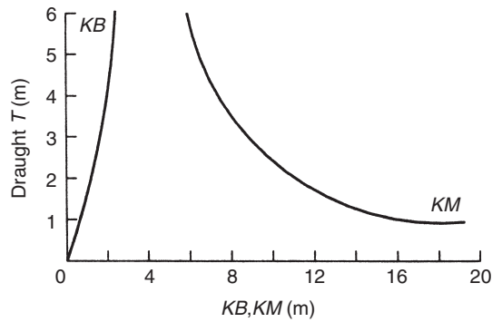
Figure 5.9 Metacentric diagram
