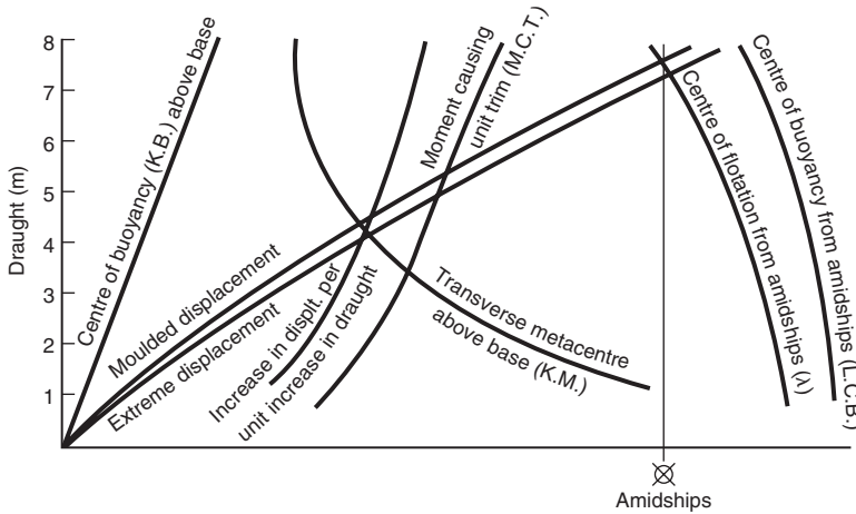
Figure 5.11 Hydrostatic curves
