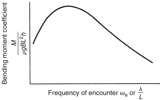
Figure 15.3 Bending moment plot
