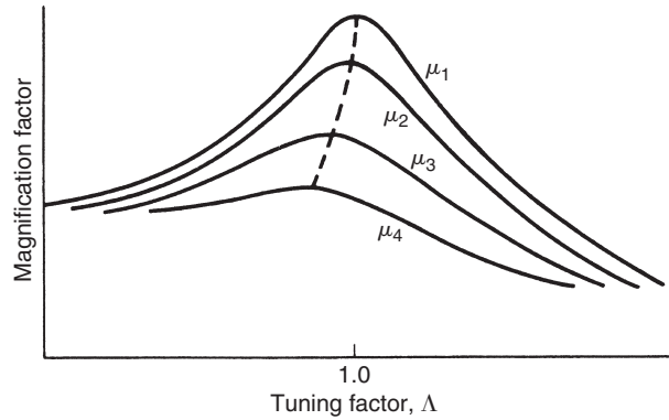
Figure 11.1 Magnification factor
