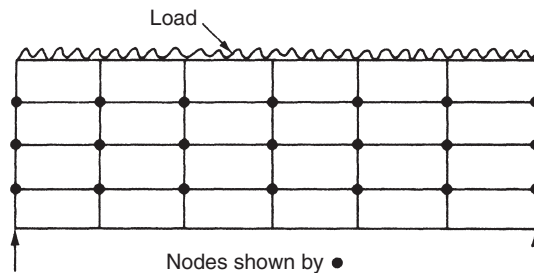
Figure 15.8 Beam finite elements
