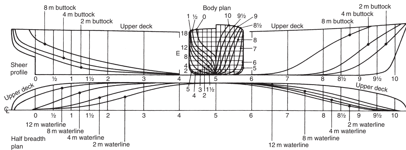
Figure 3.4 Lines plan
