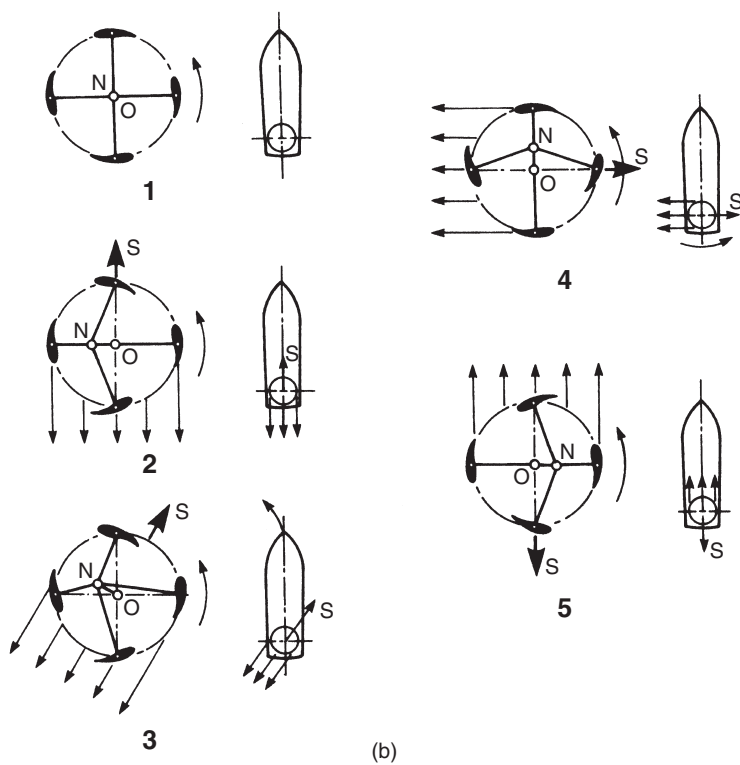
Figure 13.10 Vertical axis rudder: (a) Construction; (b) Operation
