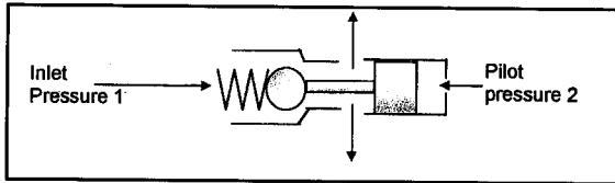
Figure 8. Pilot operated Check Valve
