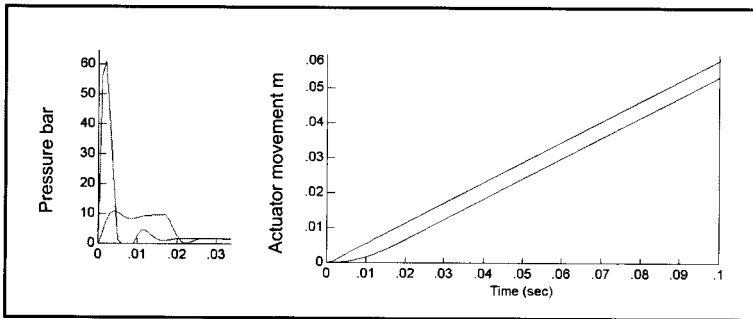
Figure 12. Variation of actuator pressure and displacement
