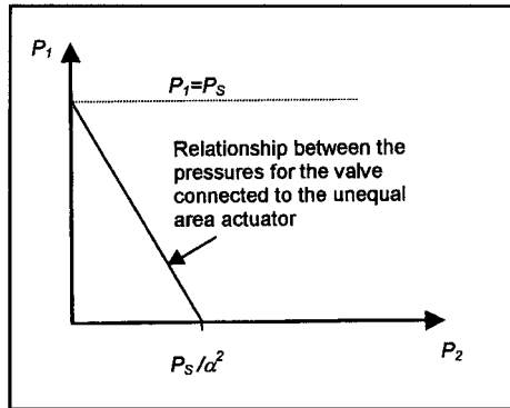
Figure 16. Valve Pressures during Extension
