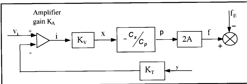
Figure 16. Block Diagram of steady state conditions
