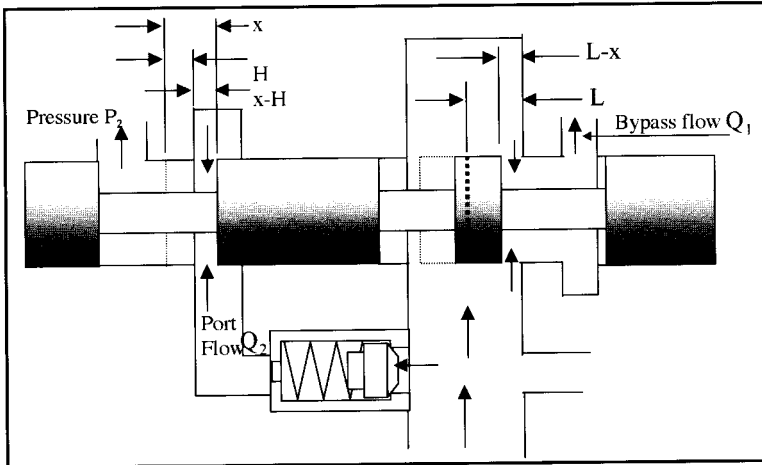
Figure 6. Valve dimensions
