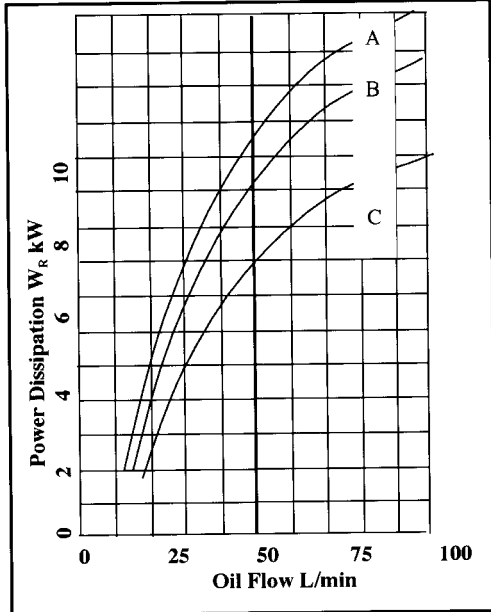
Figure 14. Cooler Performance Characteristics
