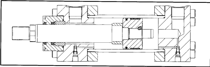
Figure 1. Typical double-acting actuator
