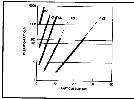
Figure 7. Beta ratio for filters (Pall)
