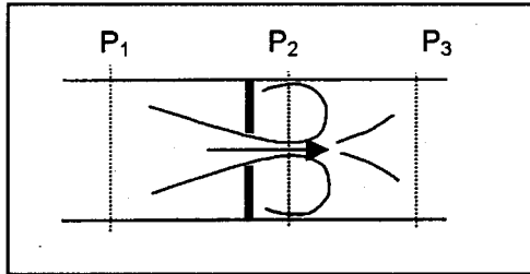
Figure 4. Sharp Edged Orifice
