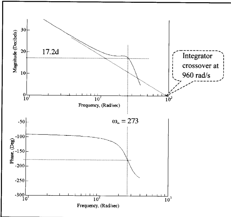
Figure 9. Open Loop Frequency Response
