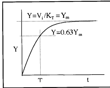
Figure 6 Step response
