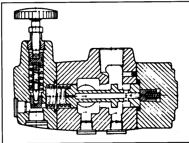
Figure 6. Reducing Valve (Eaton)
