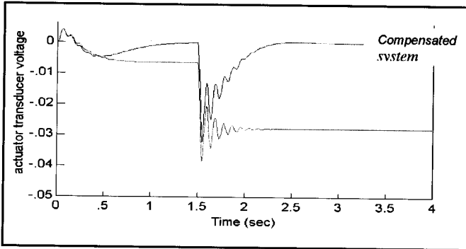
Figure 25. The effect of adding proportional plus integral compensation
