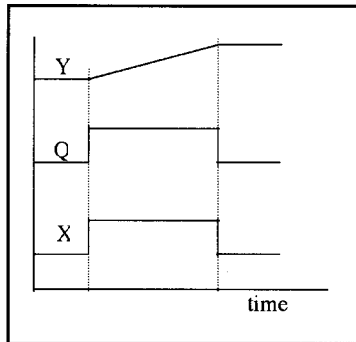
Figure 3. Open loop time response
