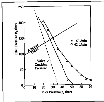
Figure 8 Flow Characteristics for Counterbalance Valve type (b)
