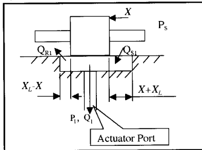
Figure 14. Valve underlap
