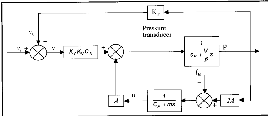
Figure 18. Pressure control
