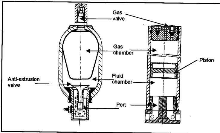
(a) Bladder type (Fawcett Christie) (b) Typical piston type Figure 1. Accumulators
