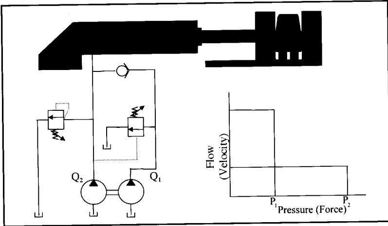
Figure 19. Vehicle Crusher Unloading Pump Circuit
