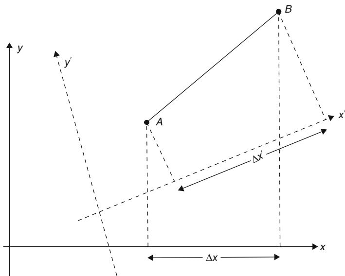
Fig. 3.13 Rotated/translated coordinate systems
