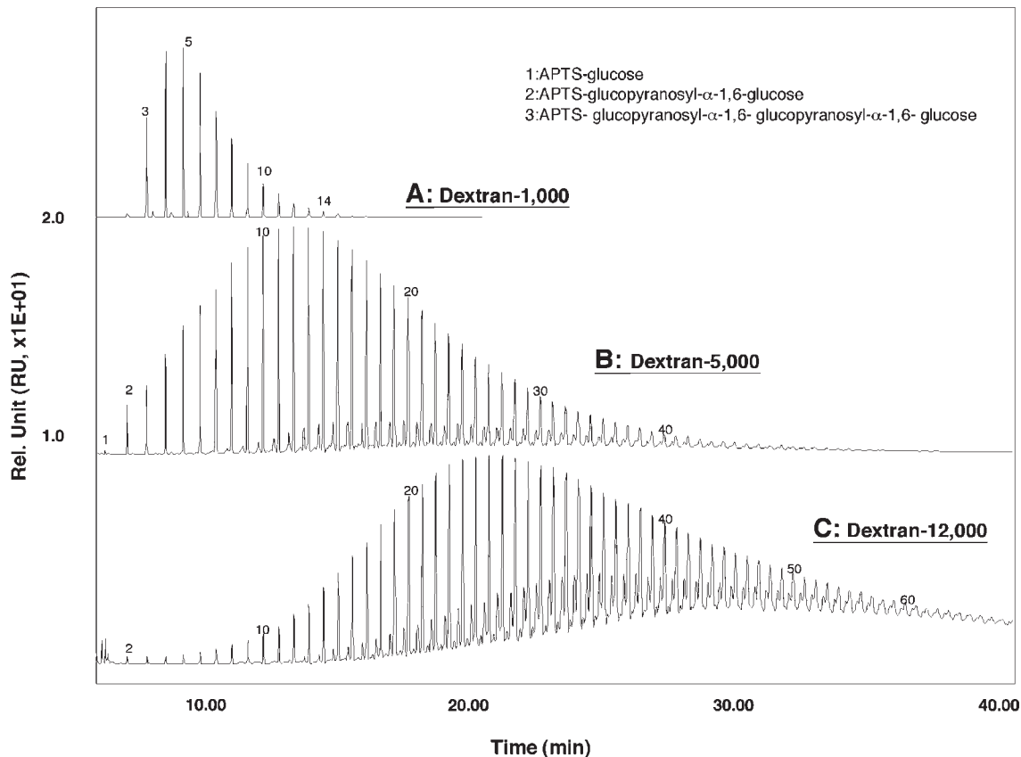
Fig. 2. Electropherograms of APTS-derivatized dextran 1000 (A), dextran 5000 (B), and dextran 12,000 (C). Conditions: 50 \mu m \times 47 cm PVA-coated capillary; buffer: 25 mM acetate, pH 4.75, containing 0.4% PEO; injection: 0.5 psi for 5 s; 23.5 kV/12.6 \mu A; ex: 488 nm/em: 520 nm.
