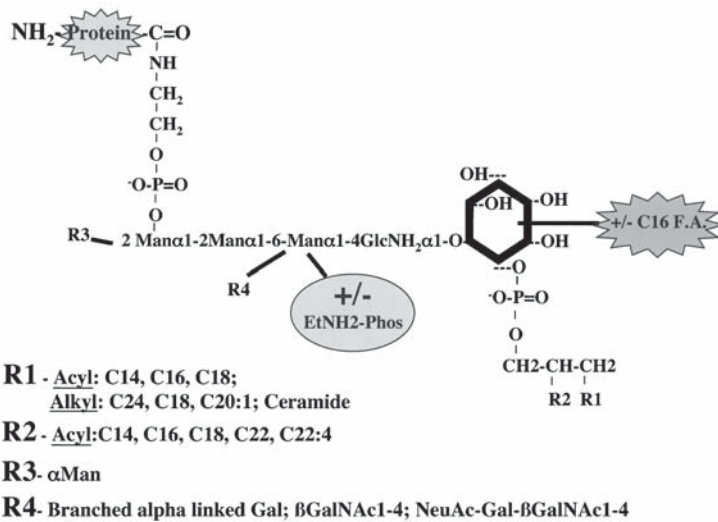
Fig. 5. Illustration of the structural diversity of GPI anchors.
