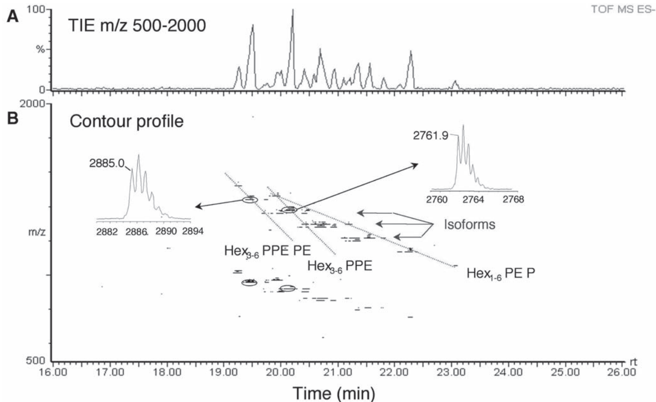
Fig. 3. CE-ESMS analysis of O -deacylated LPS from H. influenzae strain 7004 lic2B . (A) Total ion electropherogram ( m/z 500-2000). (B) Contour profile of m/z vs. time. Dotted lines indicate family of closely related glycoforms generally composed of sequential addition of Hex residues, whereas isoforms are isomeric glycolipids corresponding to substitution of a functional group. Examples of reconstructed molecular mass profiles are shown as insets . Mass spectral acquisition obtained on a Micromass Q-TOF instrument.
