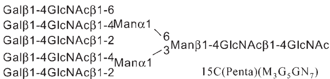
Fig. 5. Basic forms of complex type N -glycans in glycoproteins. Each N -glycan is named according to the Suzuki et al. system.
