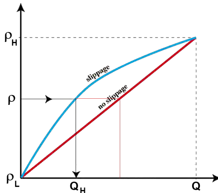
Fig. 14.1.5 – Density vs. heavy phase rate with and without slippage
