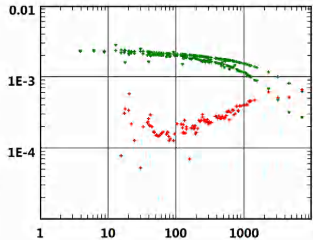
Fig. 4.E.2 – Blasingame plot
