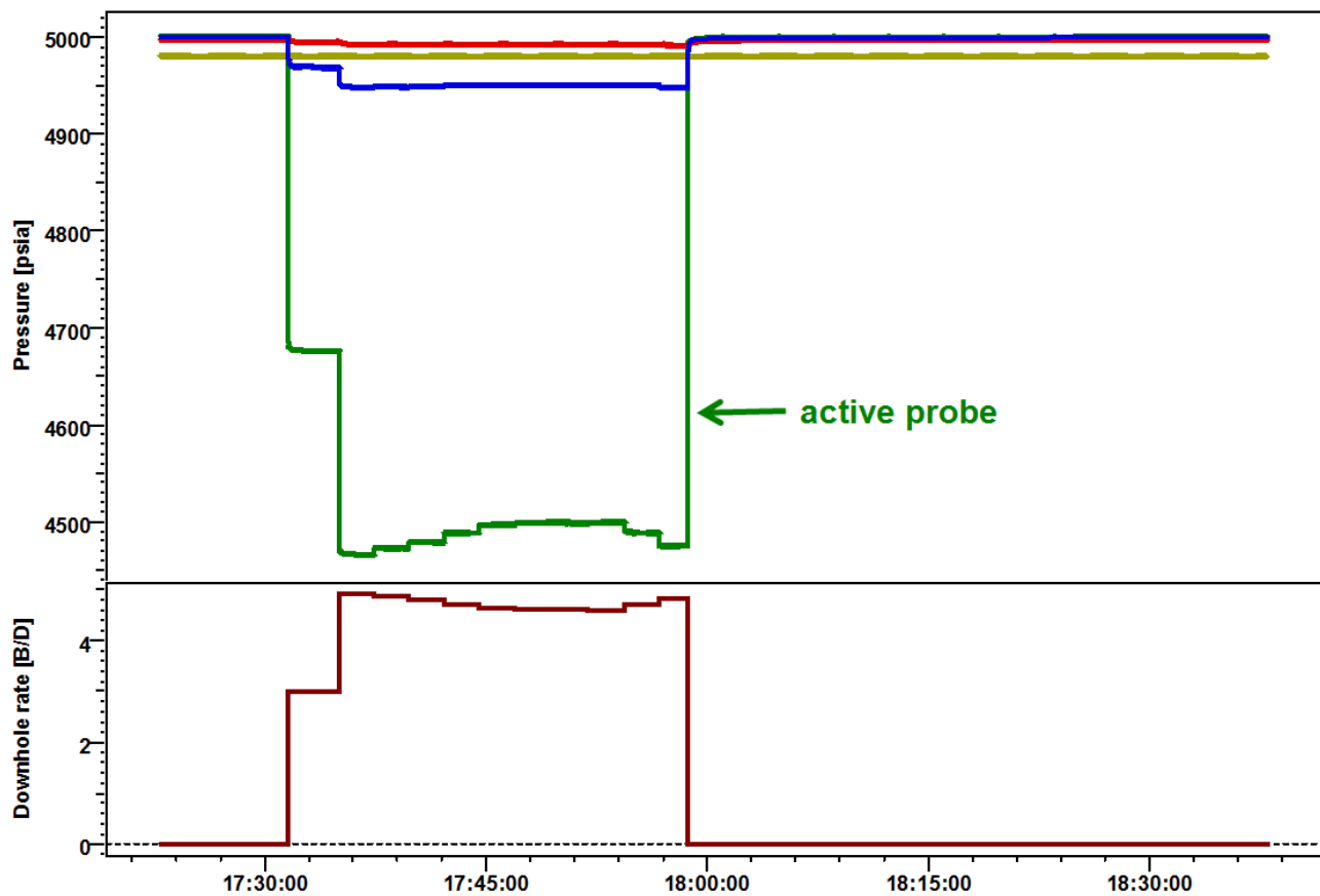
Fig. 11.B.9 – WFT History match
