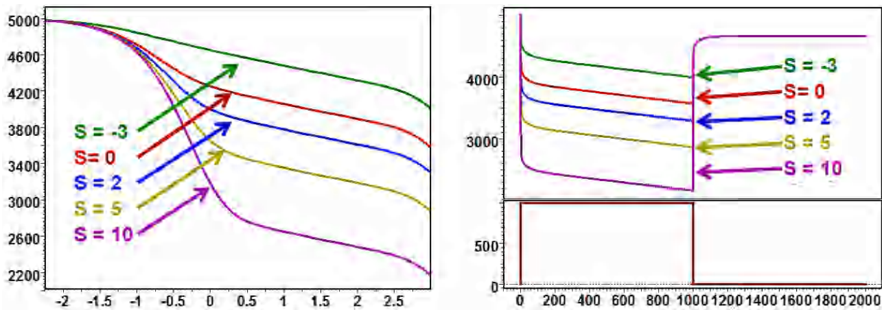
Fig. 6.B.2 – Effect of skin, semilog and history plot
