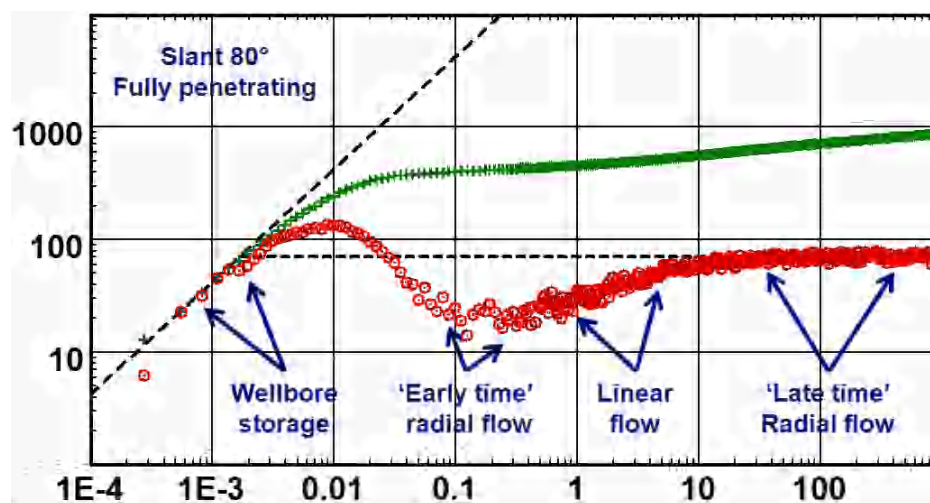
Fig. 6.I.2 – Slanted well response
