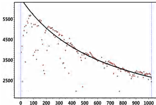
Fig. 1.D.3 – Arps plot
