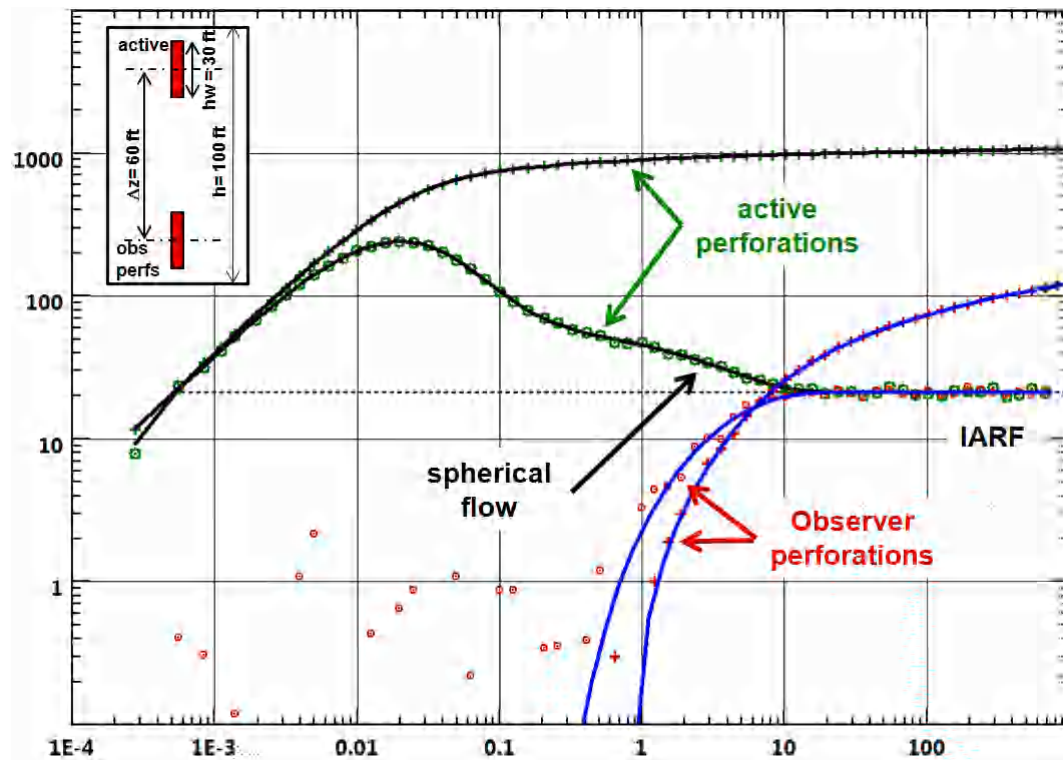
Fig. 11.E.22 – Vertical interference test
