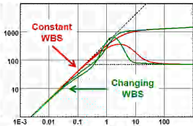
Fig. 5.C.2 – Decreasing storage
