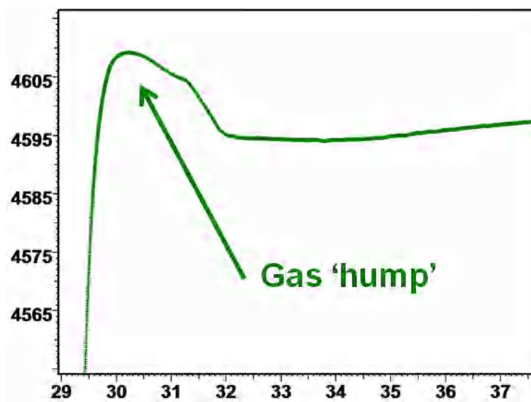
Fig. 3.I.8 – Gas humping
