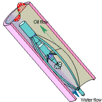
Fig. 14.J.1 – Flow recirculation
