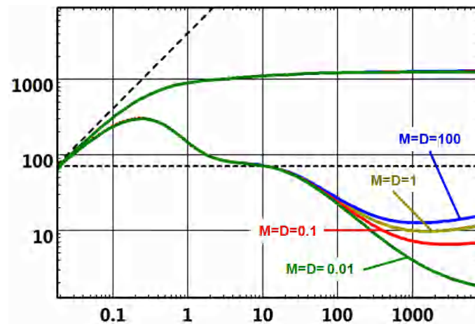
Fig. 8.I.7 – Effects of mobility changes
