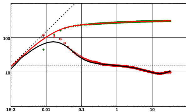
Fig. 3.I.5 – Match non drifting gauge, no fault
