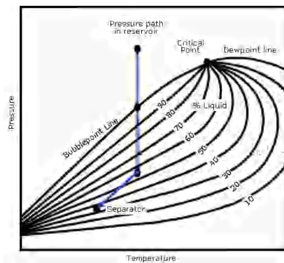
Fig. 9.C.1 – Non-volatile oil
