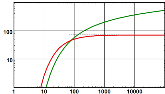
Fig. 7.B.3 – Line source
