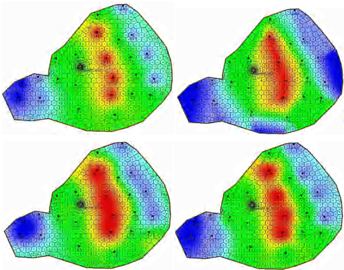
Fig. 10.E.4 – Four different interpolated fields obtained from the same input (porosity) data. From top-left to bottom-right: inverse distance weighting ( n=2 ), linear interpolation, kriging with a range of 1500 ft, kriging with a smaller range of 750 ft.
