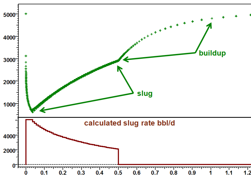
Fig. 11.C.2 – History plot
