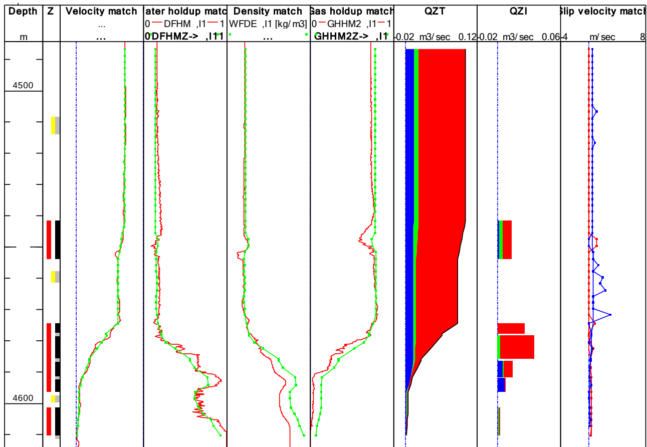
Fig. 14.I.11 – Example of continuous approach result in Emeraude
