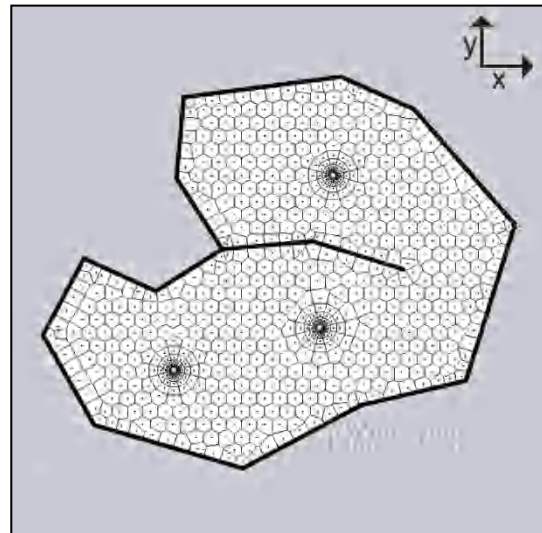
Fig. 2.G.4 – Numerical model
