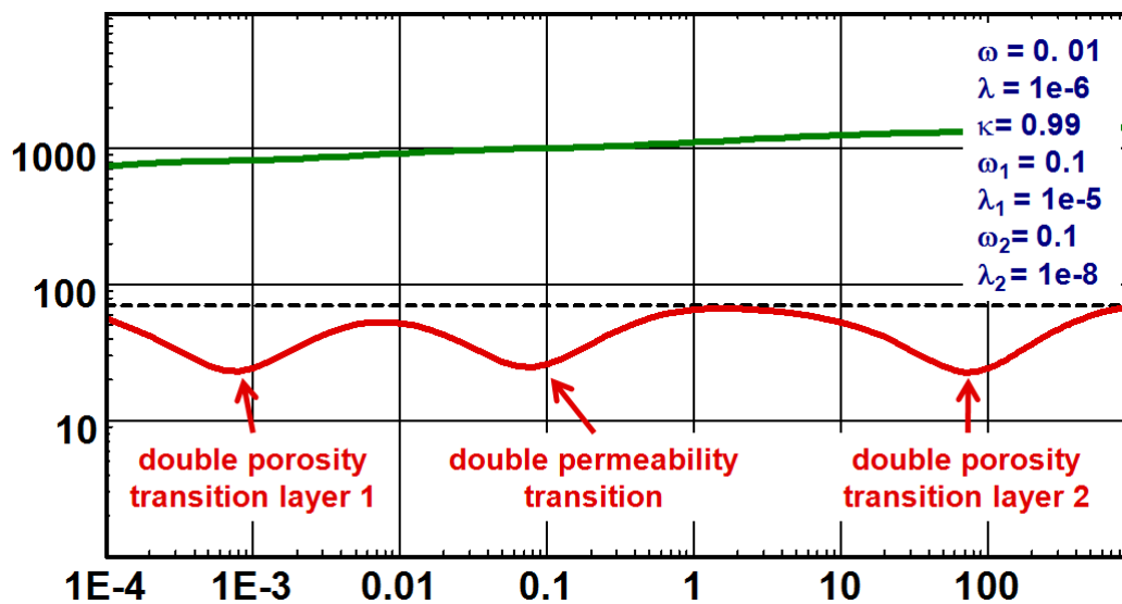
Fig. 7.J.4 – Double-permeability reservoir with double-porosity layers
