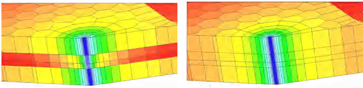
Fig. 10.E.13 – Pressure field around a well producing in a four layer system, without and with vertical crossflow between layers. (left and right respectively). The top and bottom layer have been defined with equal permeability. Middle layers with lower permeability.
