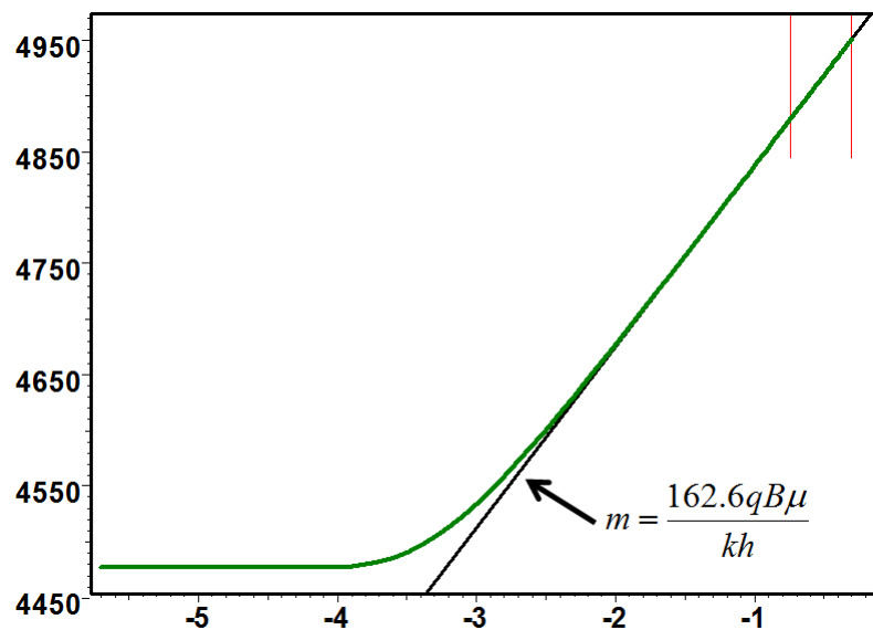
Fig. 2.C.3 – Semilog plot
