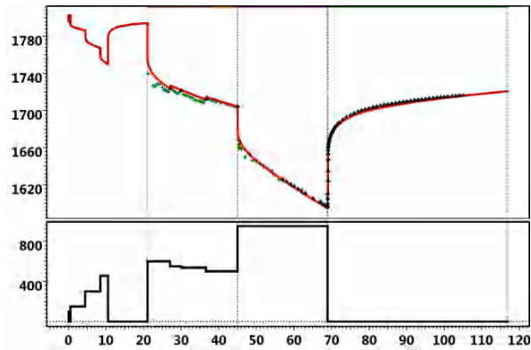
Fig. 1.C.14 – History match
