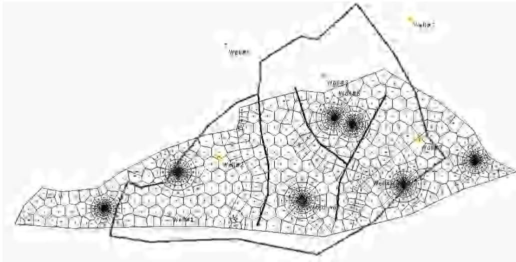
Fig. 10.E.9 – Equivalent Voronoi grid for an anisotropic reservoir ( k_x/k_y=0.2 )
