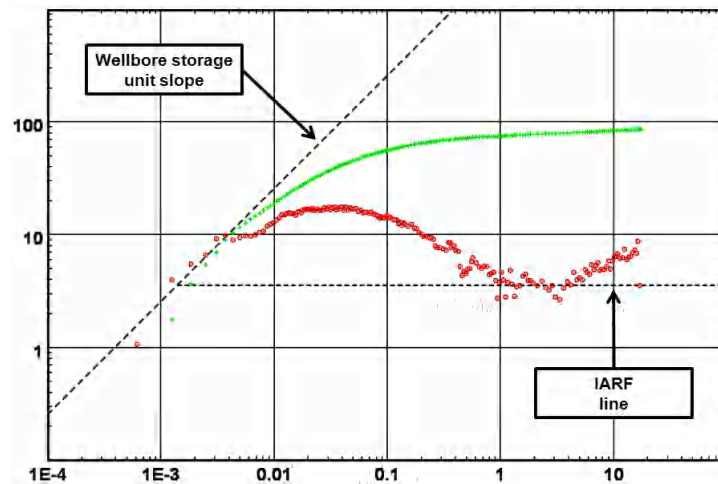
Fig. 3.E.8 – Match lines
