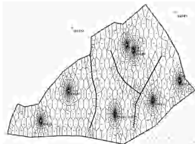
Fig. 10.E.8 – 'Voronoi' grid for an anisotropic reservoir ( k_x/k_y=0.2 )
