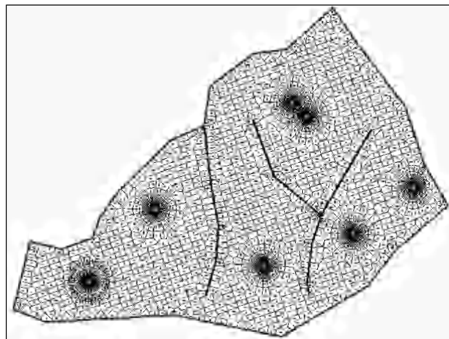
Fig. 10.B.6 – Customized grid
