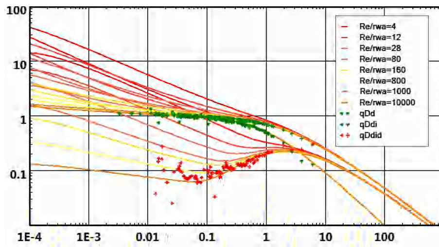
Fig. 4.C.2 – Blasingame type curve
