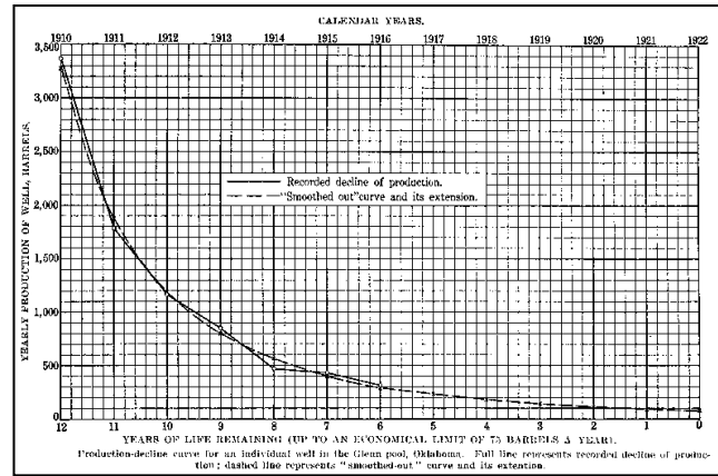
Fig. 1.D.2 – Cutler plot (1924)
