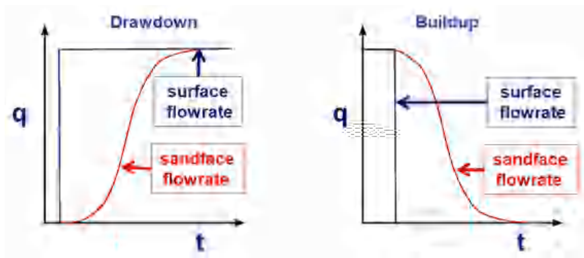
Fig. 5.B.1 – Wellbore storage
