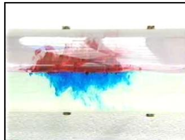
Fig. 14.J.4 – Slippage dependence around horizontal; Courtesy Schlumberger
