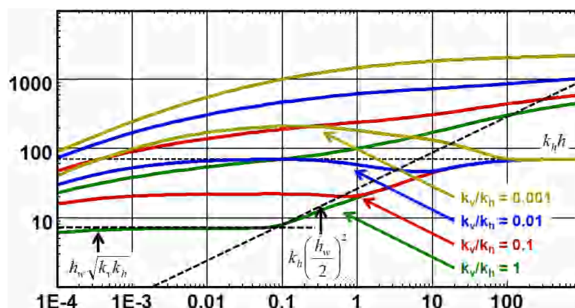
Fig. 7.I.2 – Horizontal well
