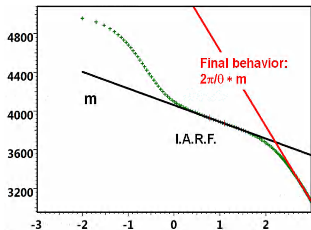
Fig. 3.B.10 – MDH plot for intersecting faults
