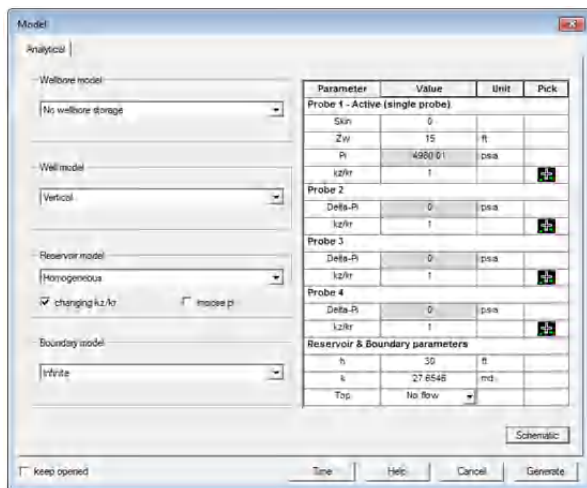
Fig. 11.B.6 – Model dialog probes
