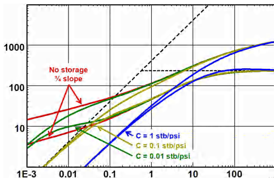
Fig. 6.H.14 – Influence of wellbore storage
