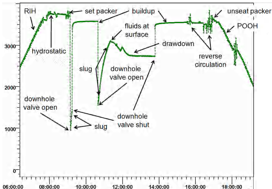
Fig. 11.C.1 – Conventional DST
