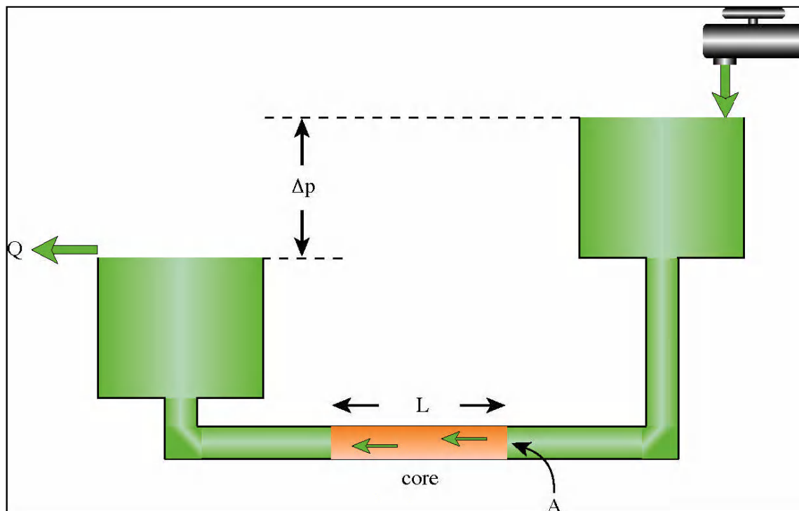
Fig. 2.A.1 – Darcy's experiment
