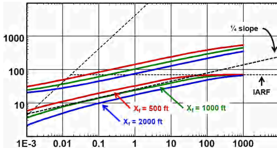
Fig. 6.E.5 – Constant FC_D ; sensitivity to half fracture length, X_f
