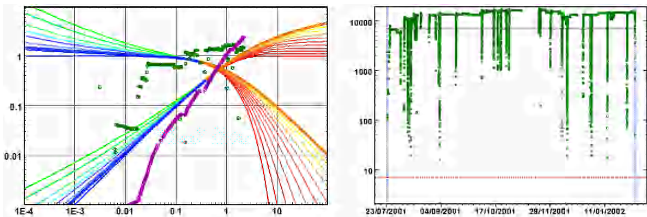
Fig. 13.G.2 – Fetkovich type-curve and Arps plot
