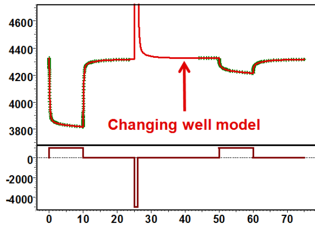
Fig. 6.C.6 – Changing well history match
