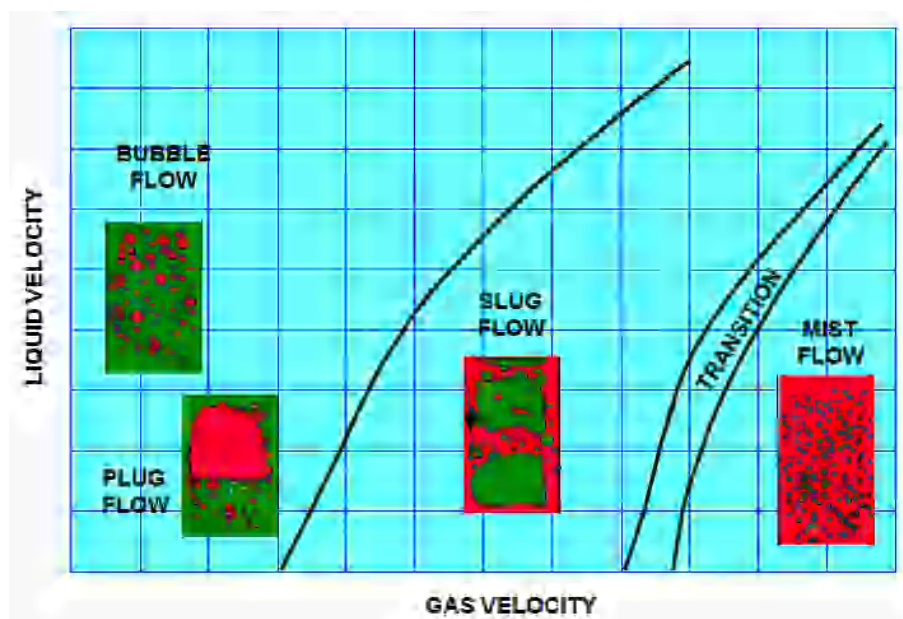
Fig. 14.I.4 – Duns and Ross flow map
