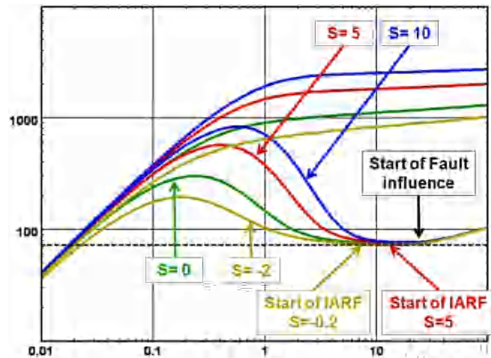
Fig. 3.F.8 – Skin sensitivity
