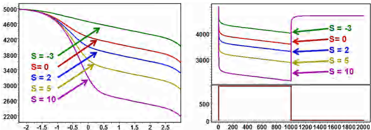
Fig. 7.B.6 – Effect of skin, semilog and history plot
