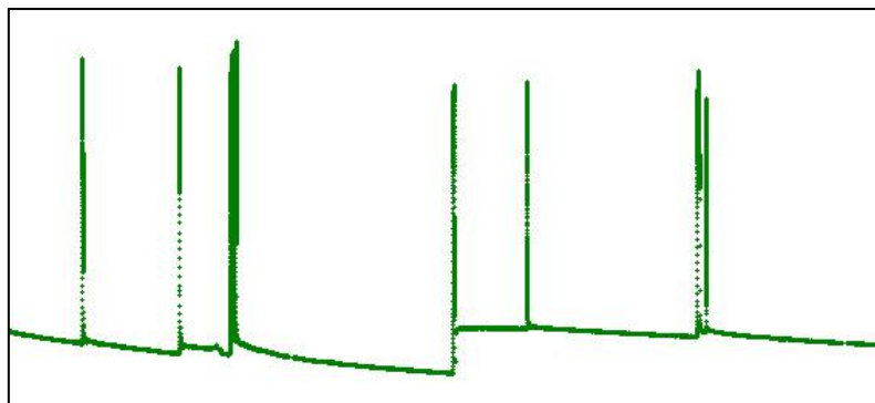
Fig. 13.A.1 – Example of permanent pressure gauge data three months of data - downhole pressure vs. time
