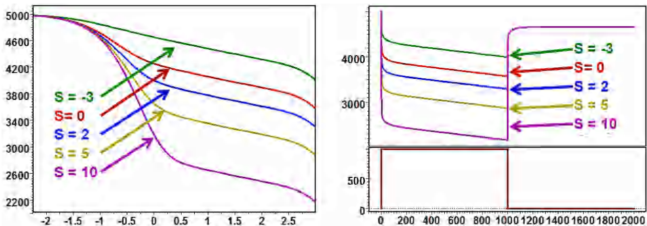
Fig. 2.H.6 – Effect of skin, semilog and history plot
