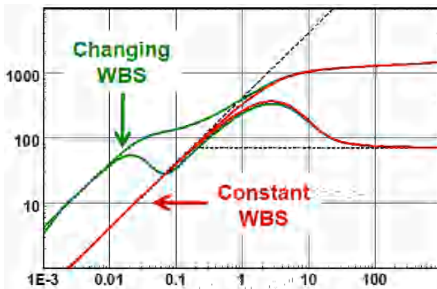
Fig. 5.C.1 – Increasing storage
