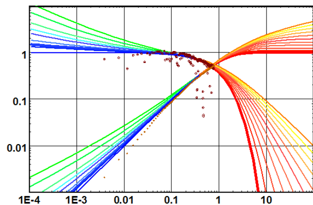
Fig. 4.A.2 – Fetkovich type-curve
