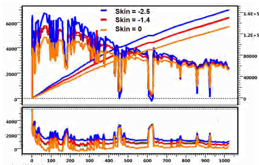
Fig. 4.E.5 – Sensitivity to skin
