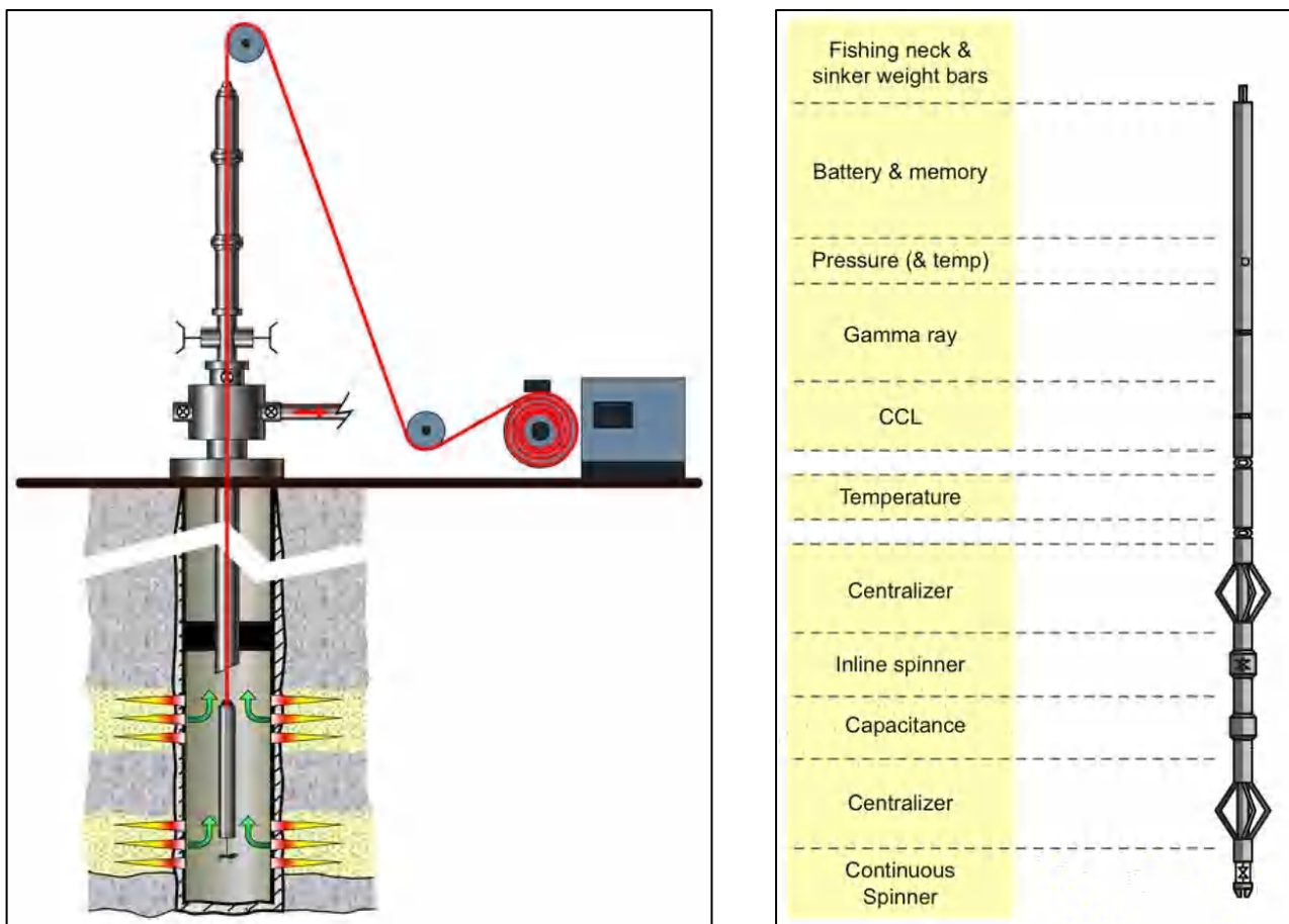
Fig. 14.C.1 – Schematics of PL operations and PL tool string
