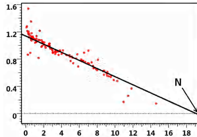
Fig. 4.C.8 – Material balance plot
