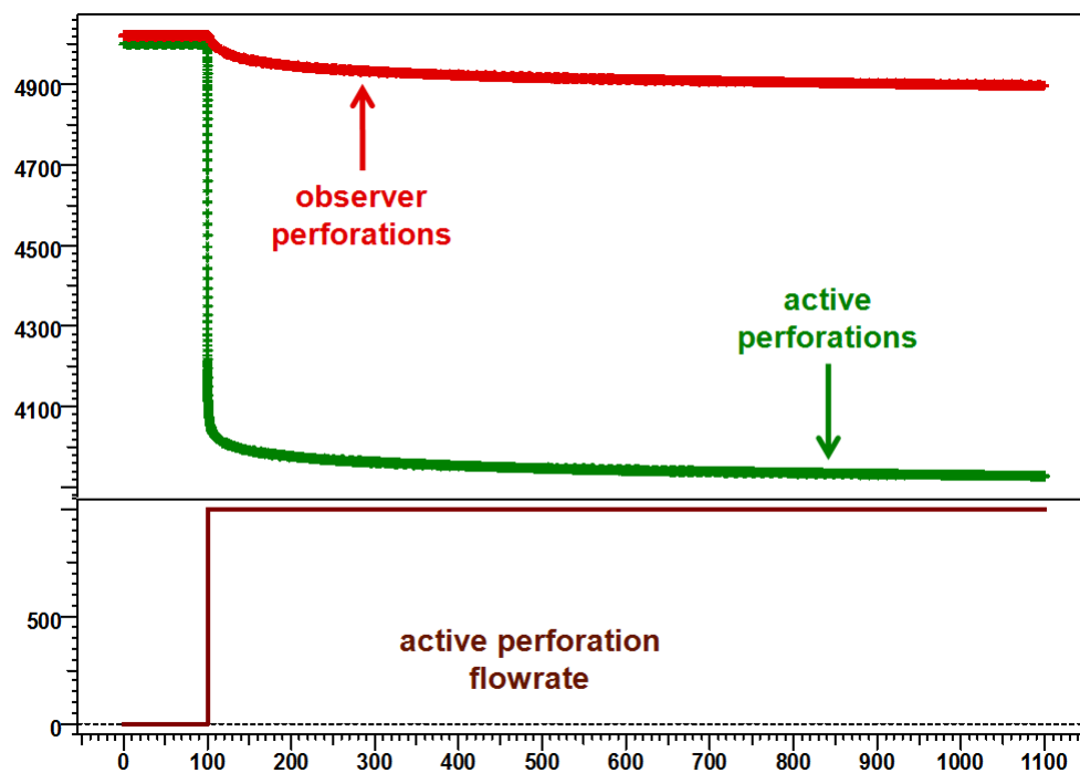
Fig. 11.E.23 – Vertical interference test history plot
