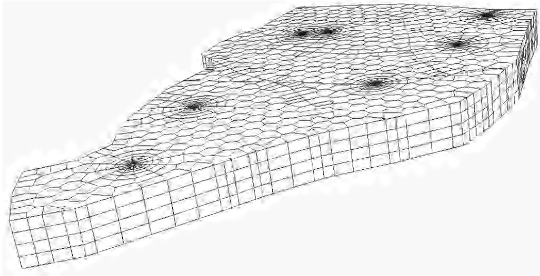
Fig. 10.E.12 – 2D grid piled up to simulate a 4 layer system
