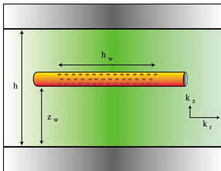
Fig. 6.G.1 – Horizontal well geometry
