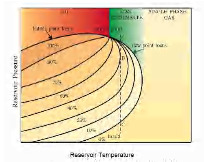
Fig. 9.B.4 – Generalized phase-diagram
