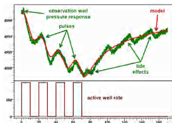
Fig. 11.E.20 – Pulse test
