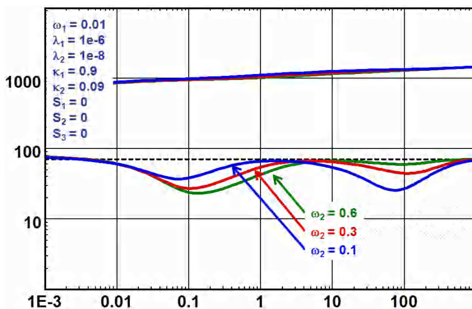
Fig. 7.F.2 – Three layers
