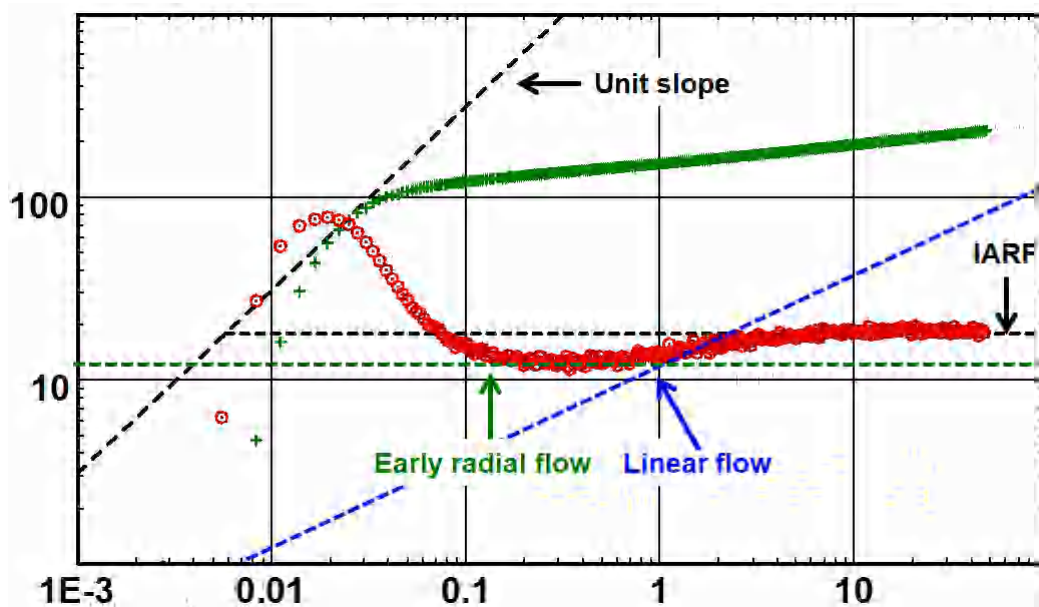
Fig. 6.G.3 – Horizontal well behavior
