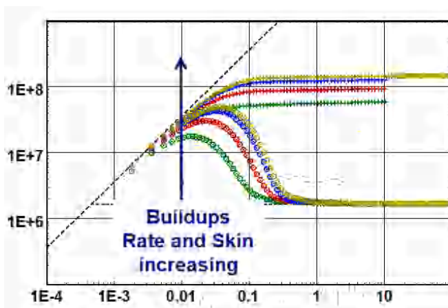
Fig. 6.C.1 – Loglog plot
