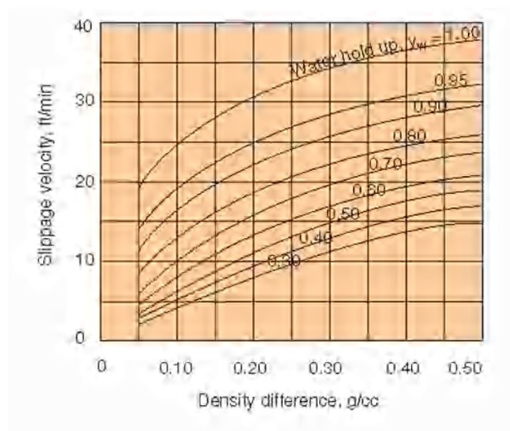
Fig. 14.I.2 – Choquette bubble flow chart
