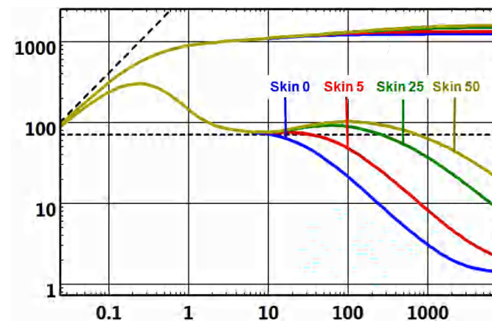
Fig. 8.I.6 – Effects fault skin
