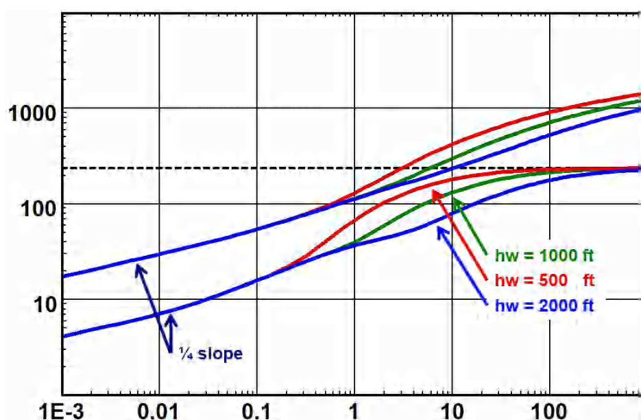
Fig. 6.H.12 – Equal number of identical fracture, sensitivity to horizontal drain length
