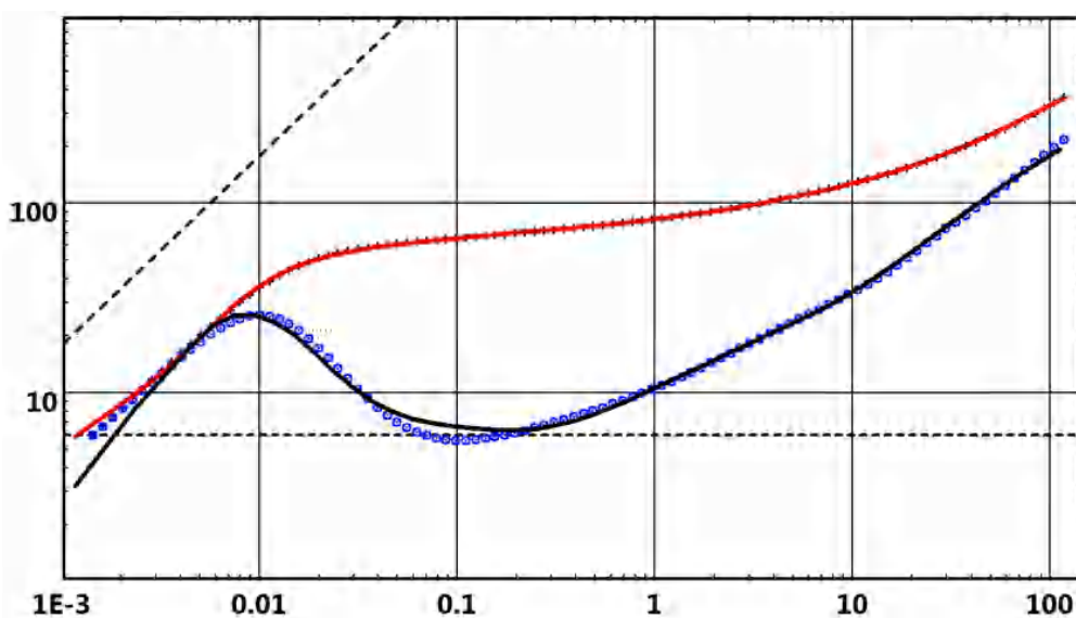
Fig. 1.C.16 – Deconvolution
