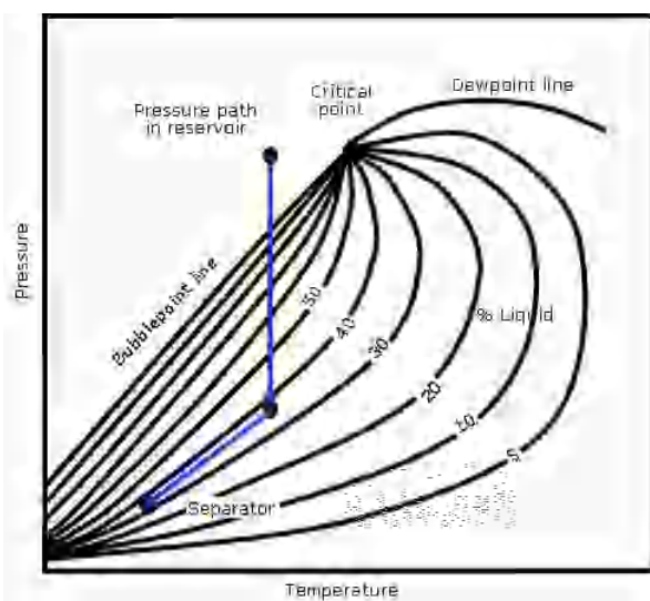
Fig. 9.C.2 – Volatile oil
