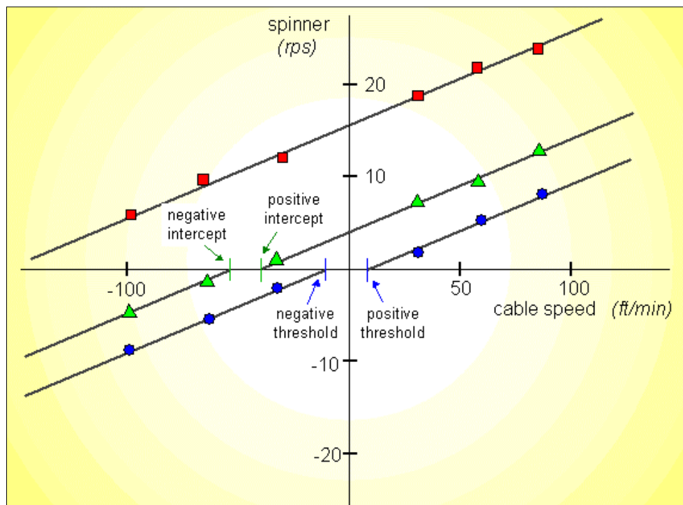
Fig. 14.G.5 – In-situ calibration for the case above
