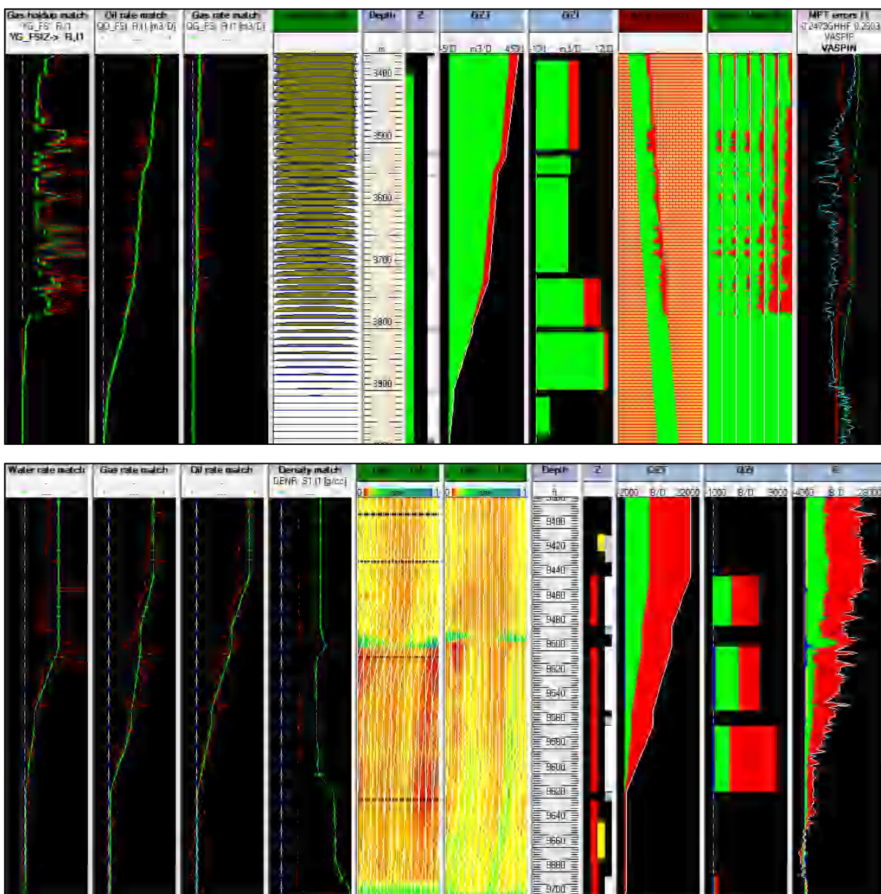
Fig. 14.B.1 – MPT interpretations in Emeraude (FSI top and MAPS bottom)
