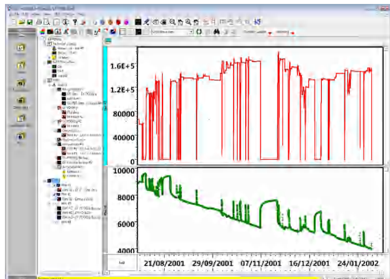
Fig. 1.E.2 – Pressures from PDG and rate data ready for PA and PTA analyses
