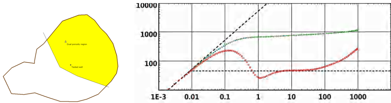
Fig. 10.E.7 – Yellow zone only defined as double porosity.
