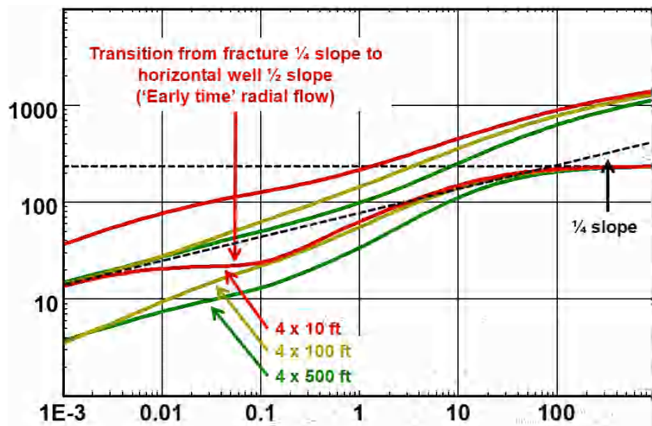
Fig. 6.H.13 – Influence of half fracture length
