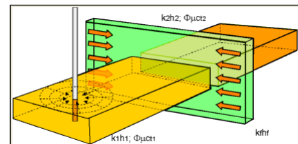
Fig. 1.C.12 Conductive fault
