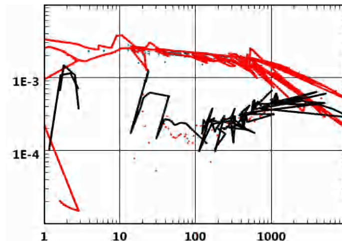
Fig. 4.C.3 – Blasingame plot with 'true' model response
