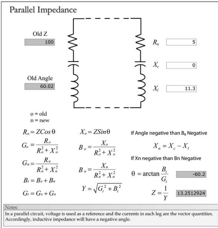
FIGURE 1.31 Parallel impedance.
