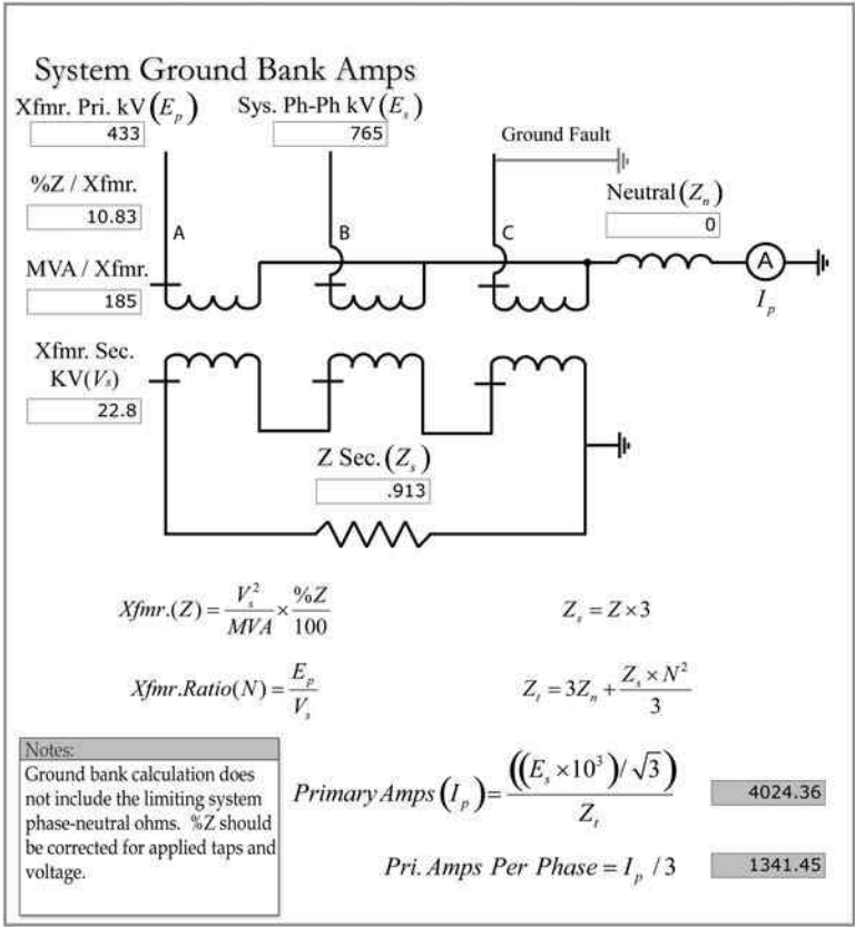
FIGURE 4.40 GSUT ground bank current.
