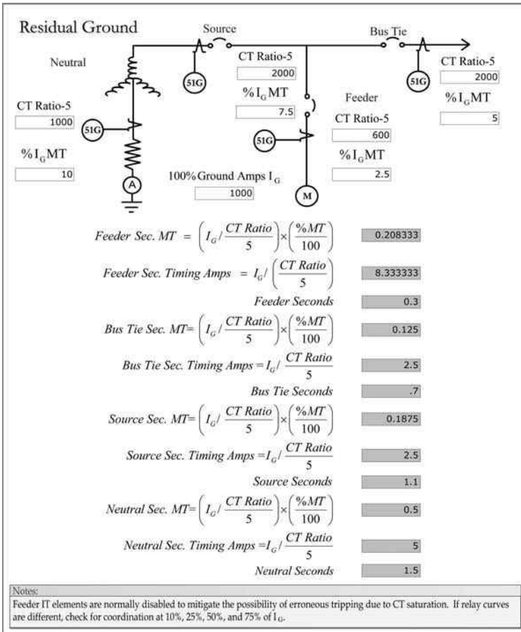
FIGURE 3.19 Residual ground overcurrent settings.
