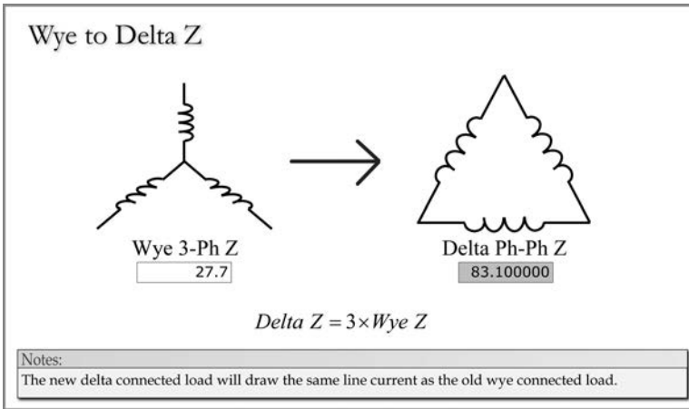
FIGURE 1.48 Wye–delta conversion.
