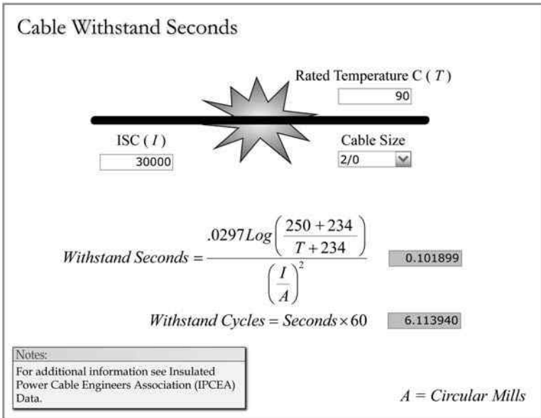
FIGURE 5.2 Cable short circuit withstand seconds.
