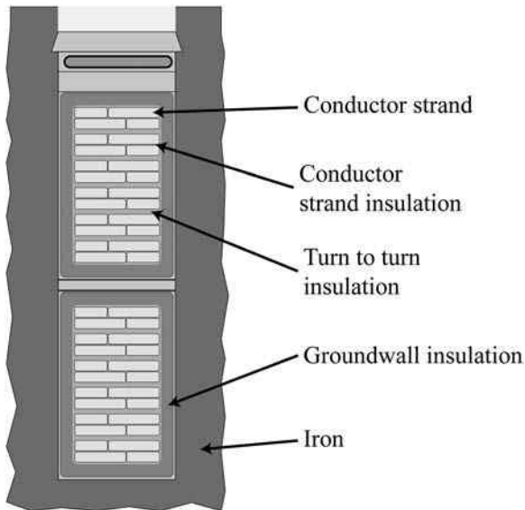
FIGURE 5.27 Motor form wound coils.
