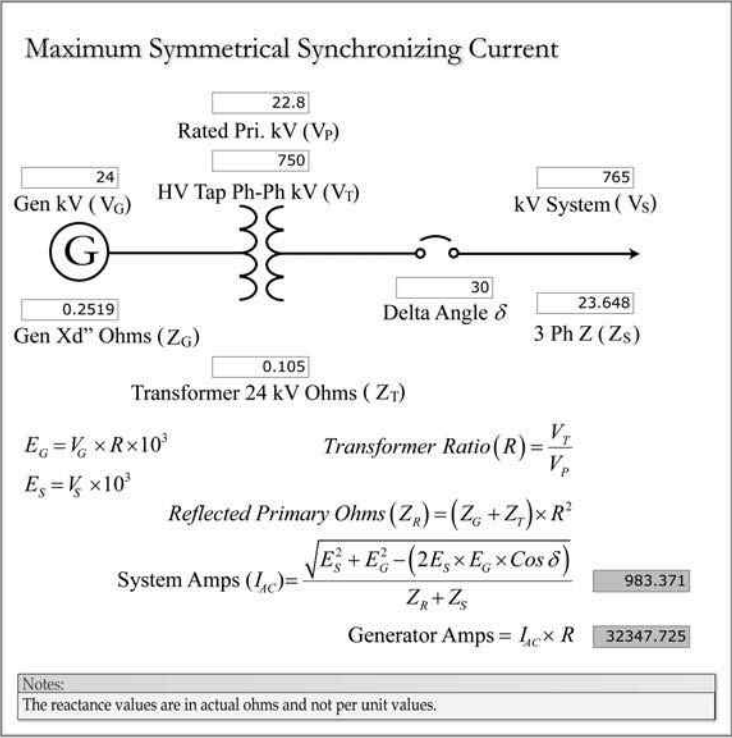
FIGURE 4.22 Maximum symmetrical synchronizing current.
