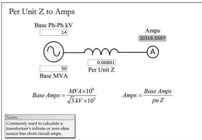
FIGURE 2.34 Per-unit Z to amps.
