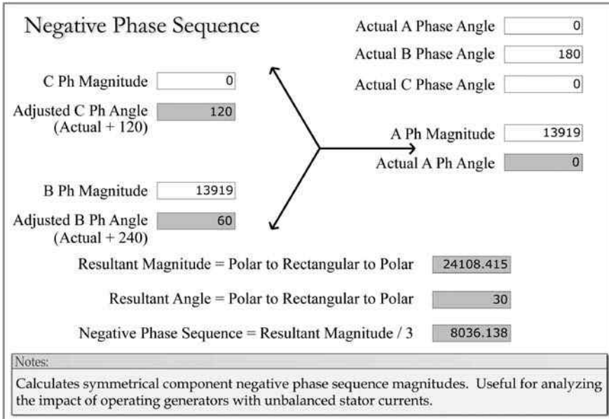
FIGURE 4.31 Negative phase sequence magnitude.
