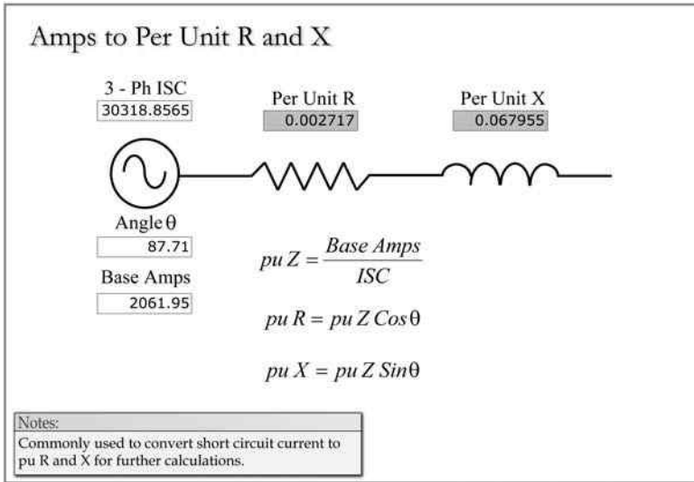
FIGURE 2.35 Amps to per-unit R and X.
