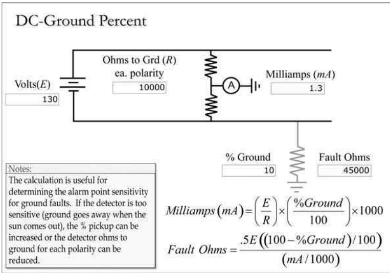
FIGURE 7.12 DC ground fault ohms.
