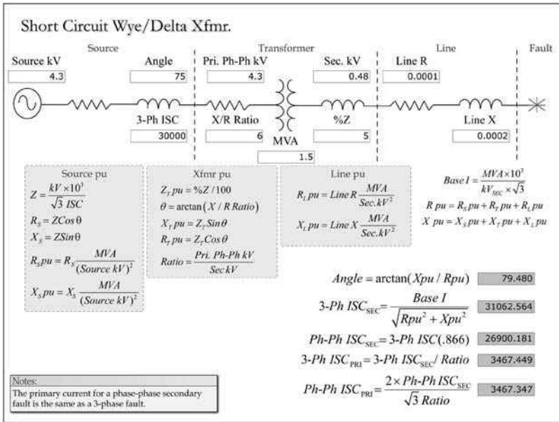
FIGURE 2.42 Wye-delta transformer short circuit.
