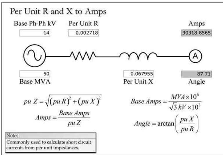
FIGURE 2.36 Per-unit R and X to amps.
