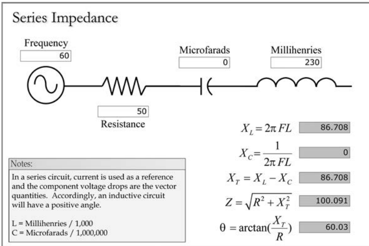
FIGURE 1.25 Series inductive impedance.
