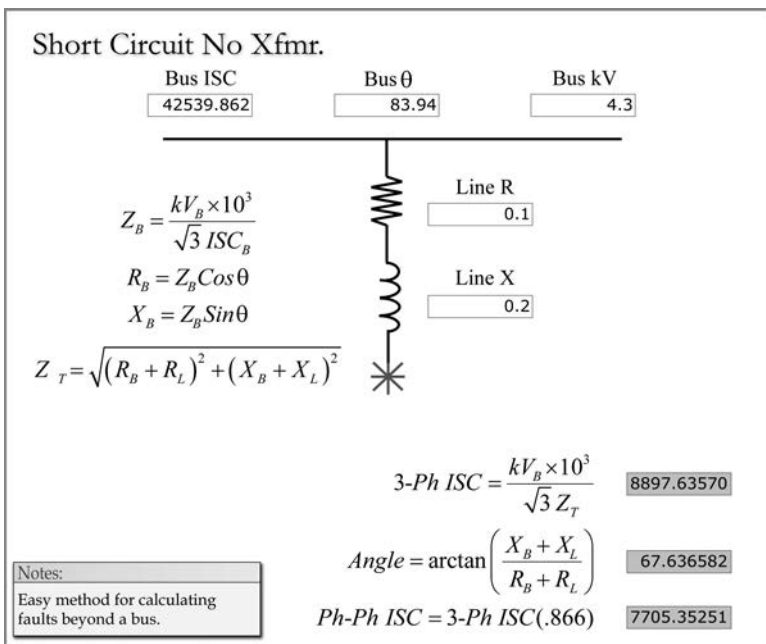
FIGURE 2.28 Short circuit: no transformer.
