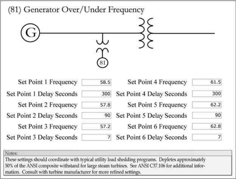
FIGURE 4.54 Overfrequency and underfrequency withstands.
