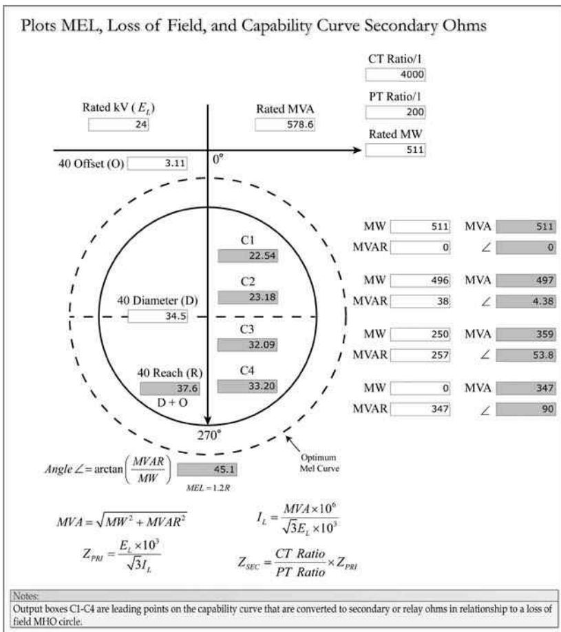
FIGURE 7.15 Loss-of-field, MEL, and capability curve ohmic plots.
