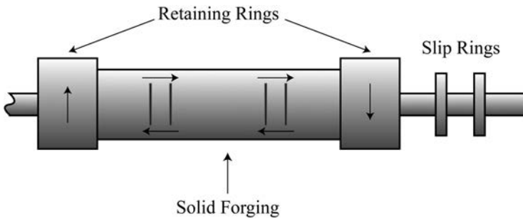
FIGURE 4.24 Cylindrical generator two-pole rotor slip frequency currents.
