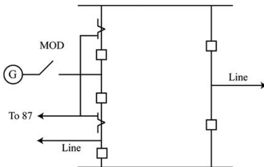
FIGURE 4.7 Breaker-and-a-half configuration.
