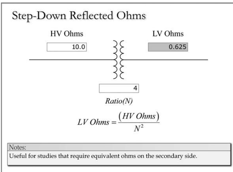
FIGURE 1.35 Reflected ohms HV to LV.
