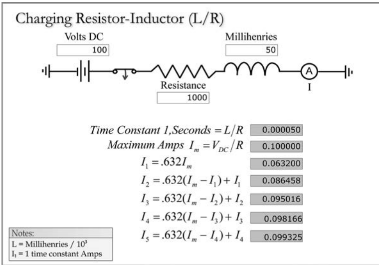
FIGURE 1.15 Charging resistor-inductor (L/R).
