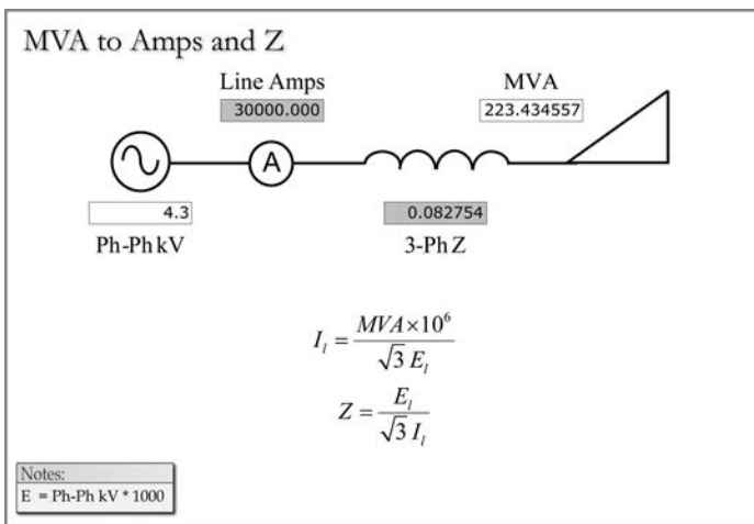
FIGURE 2.4 MVA to amps and Z.
