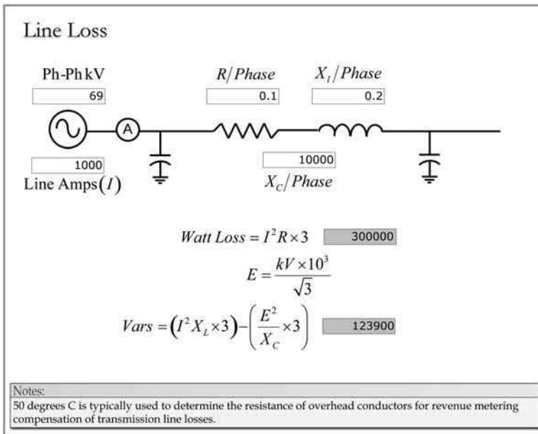
FIGURE 5.4 Cable line loss.
