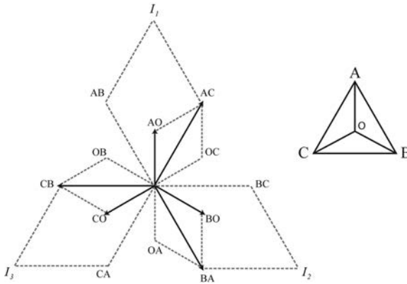
FIGURE 1.47 Delta configurations and relationships.
