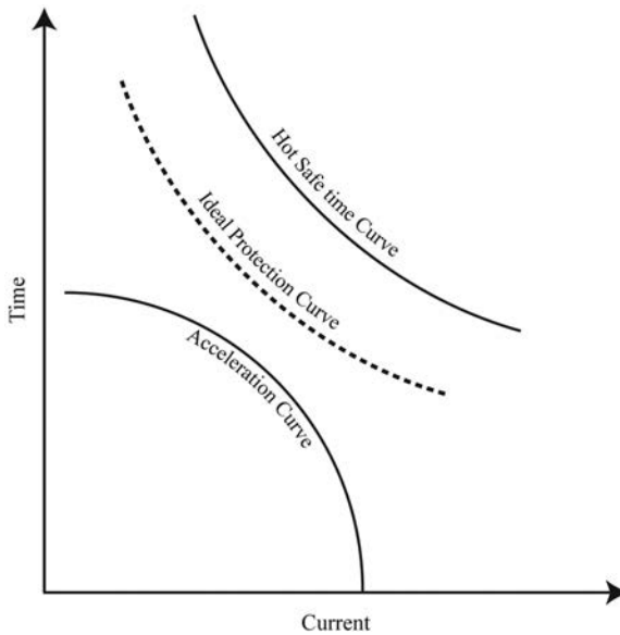
FIGURE 3.9 Motor acceleration, hot safe time, and protection curves.
