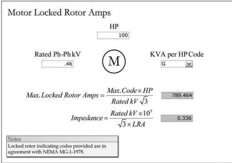
FIGURE 5.24 Motor locked rotor amps.
