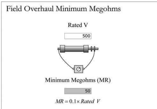
FIGURE 5.11 Generator rotor overhaul insulation testing.
