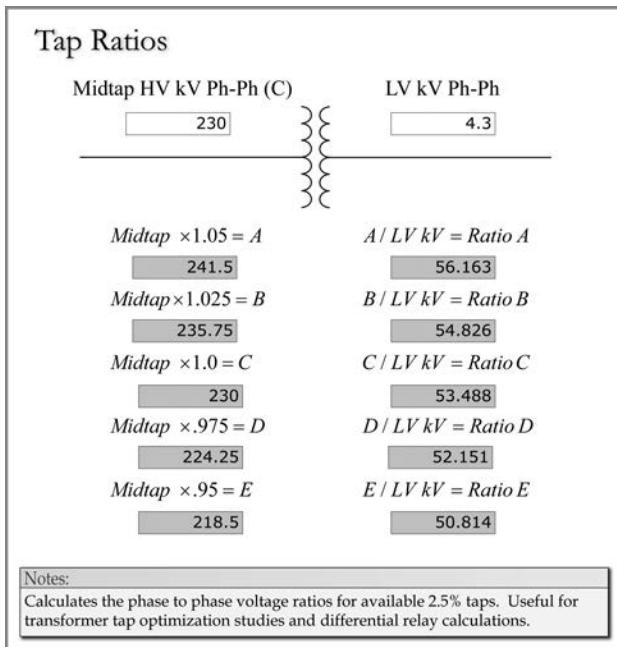
FIGURE 2.7 Transformer winding tap ratios.
