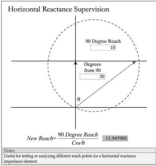
FIGURE 4.53 Horizontal reactance supervision.
