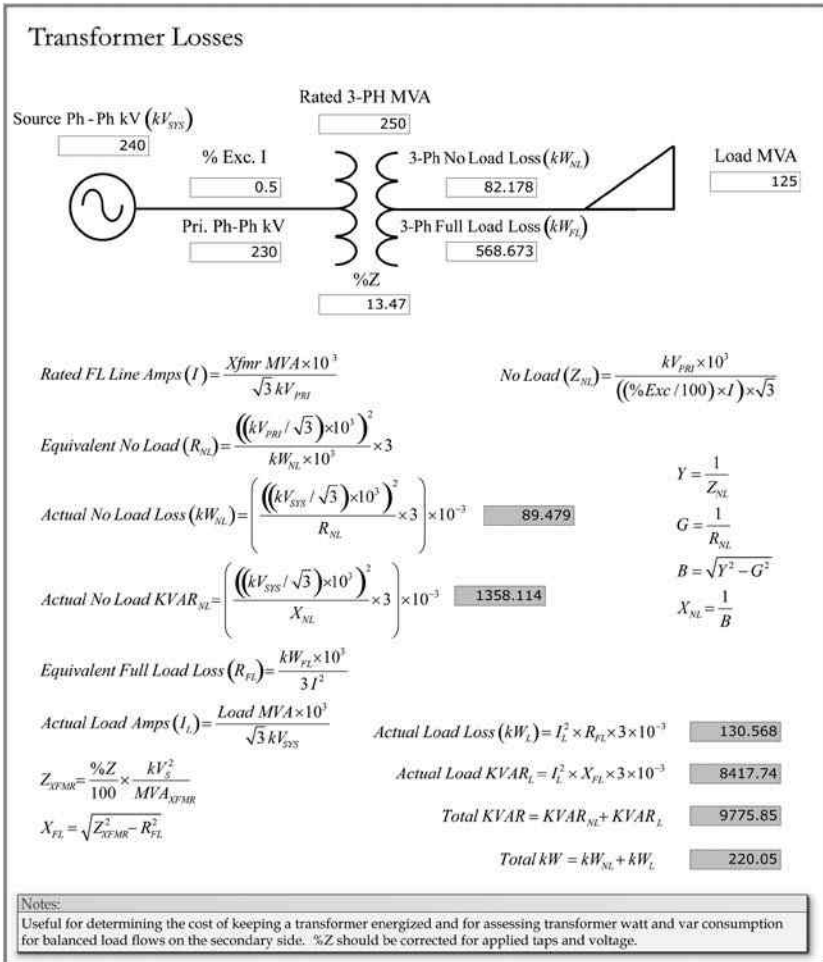
FIGURE 5.32 Transformer losses.
