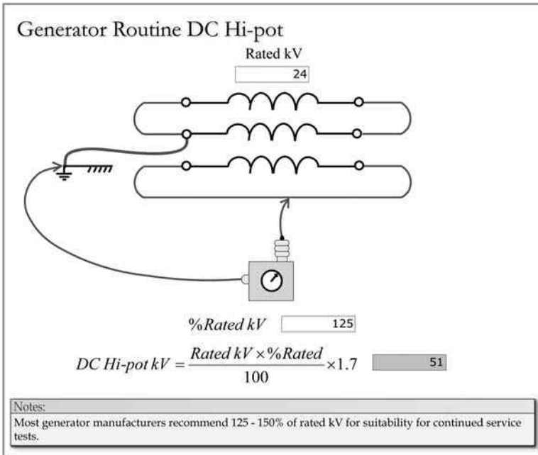
FIGURE 5.8 Generator stator routine DC overvoltage testing.
