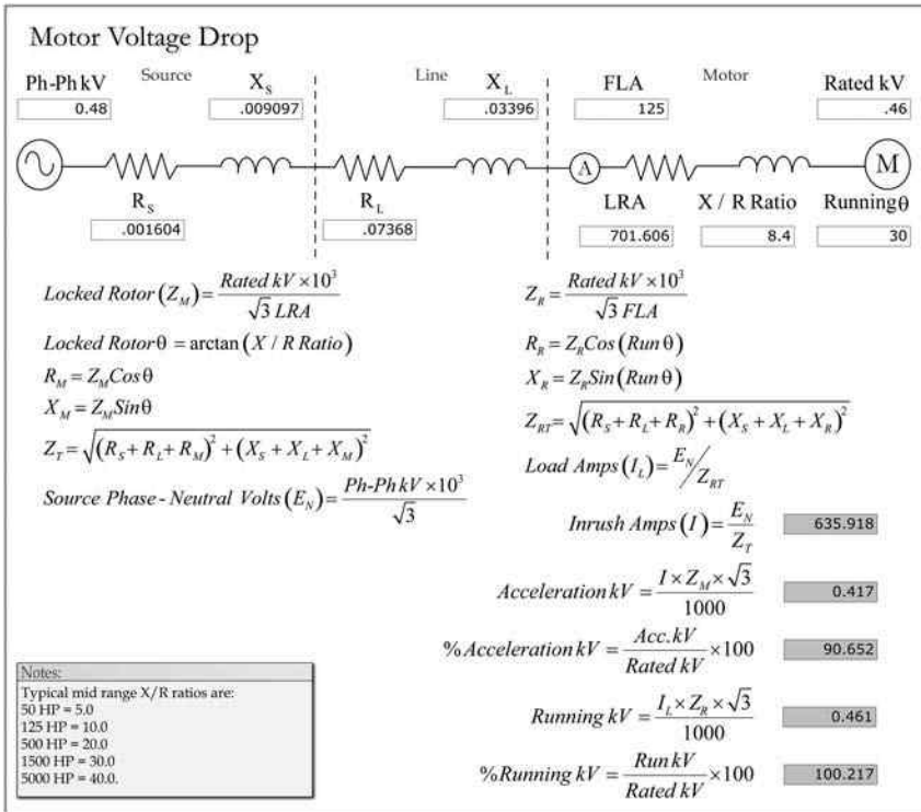
FIGURE 5.29 Motor 4/0 voltage drop.
