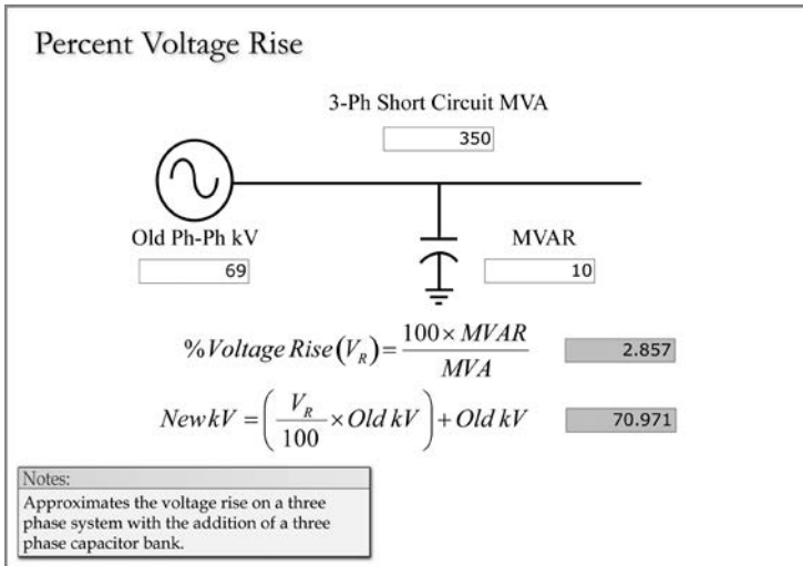
FIGURE 2.24 Capacitive voltage rise.
