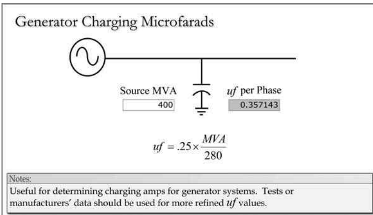
FIGURE 3.25 Typical generator system capacitive microfarads.
