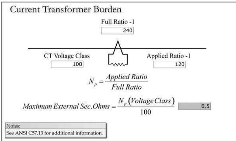
FIGURE 3.4 CT secondary burden.
