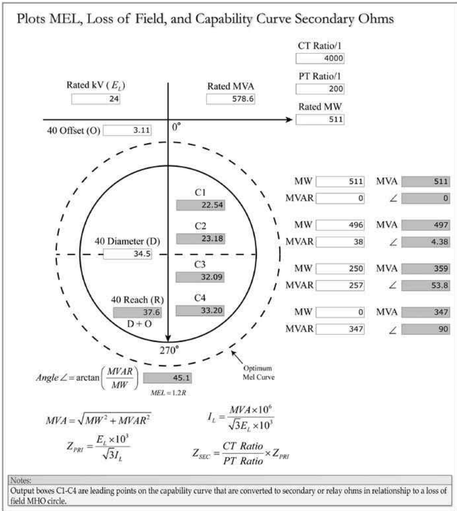
FIGURE 4.29 Generator capability curve, loss-of-field, and Mel plots.
