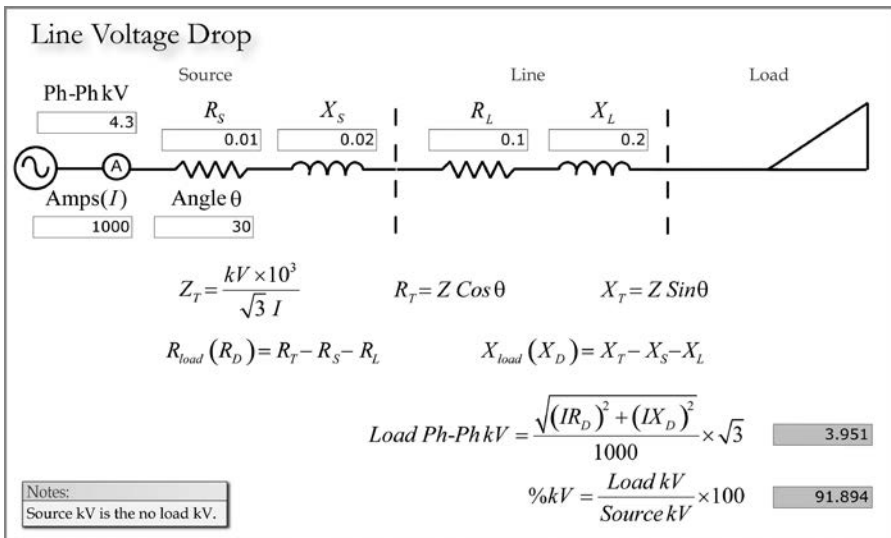
FIGURE 2.23 Line voltage drop.
