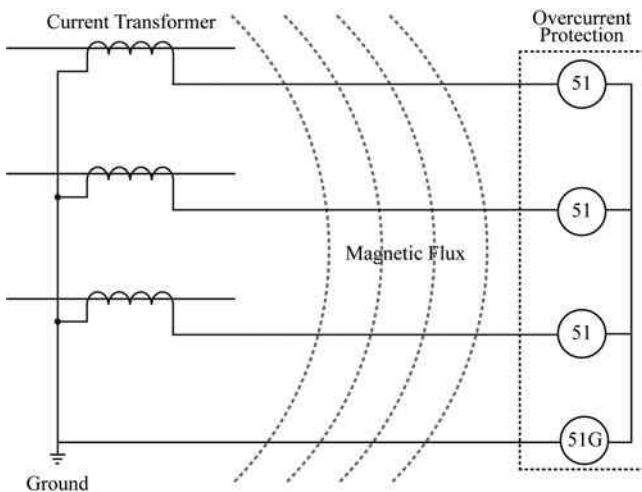
FIGURE 3.2 Typical time overcurrent schematic.
