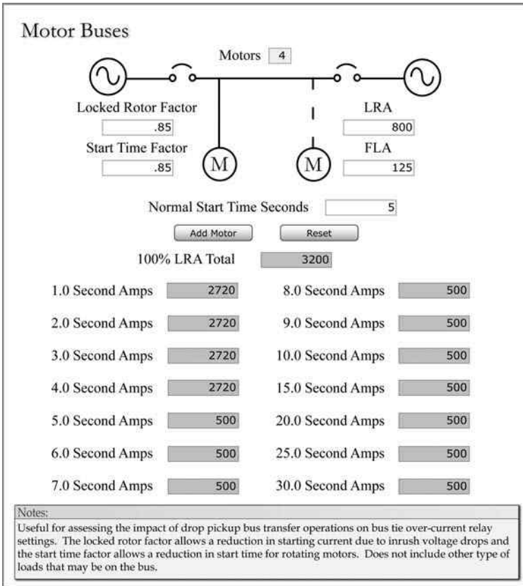
FIGURE 3.13 Motor loads during transfer.
