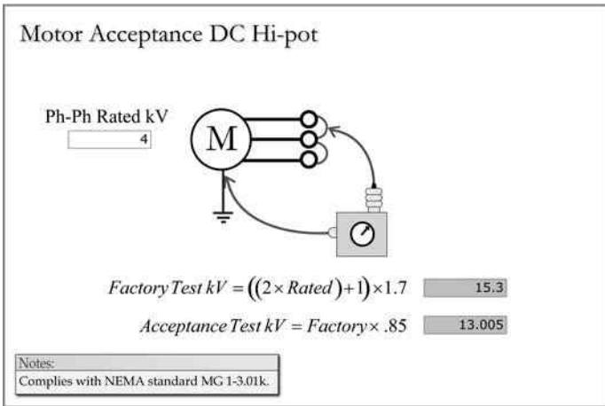
FIGURE 7.7 Motor DC acceptance test.
