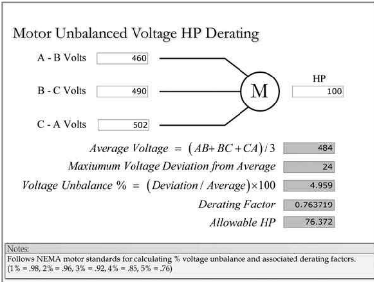
FIGURE 5.25 Motor HP derating for supply voltage unbalances.
