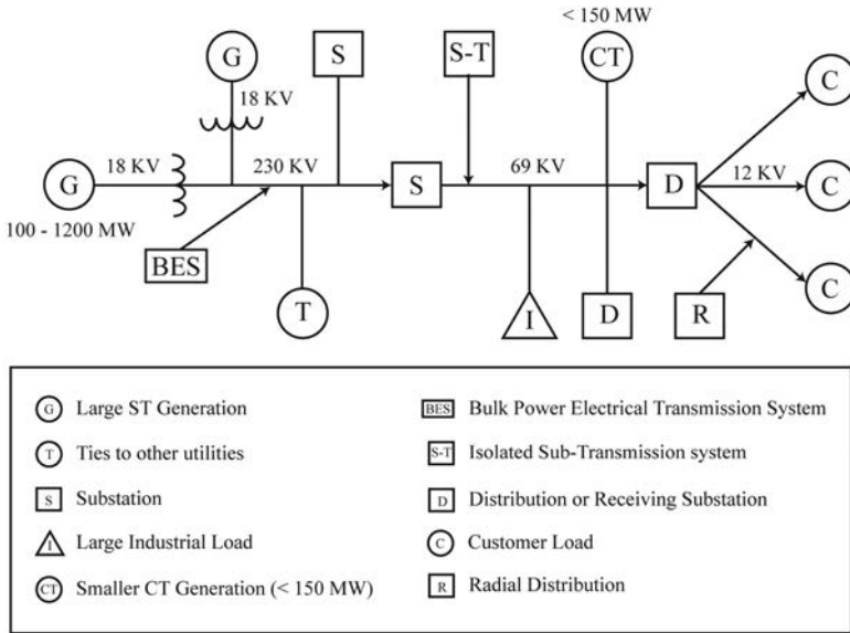
FIGURE 1.37 Typical utility configuration.
