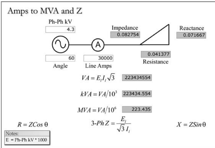
FIGURE 2.5 Amps to MVA and Z.
