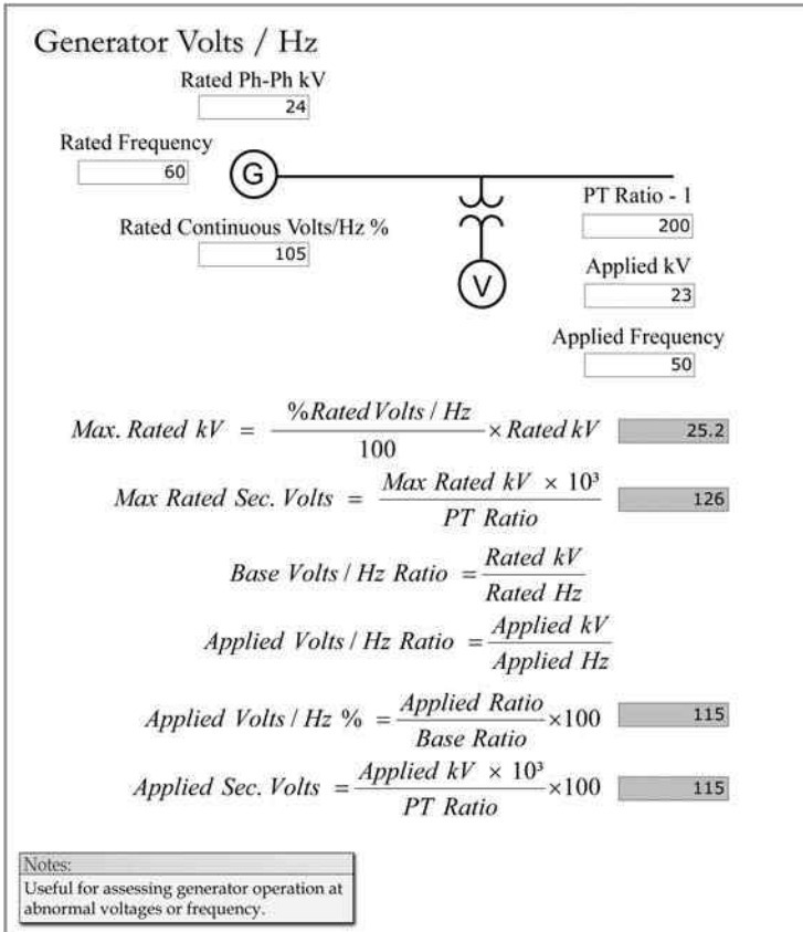
FIGURE 4.15 Generator volts/Hz.
