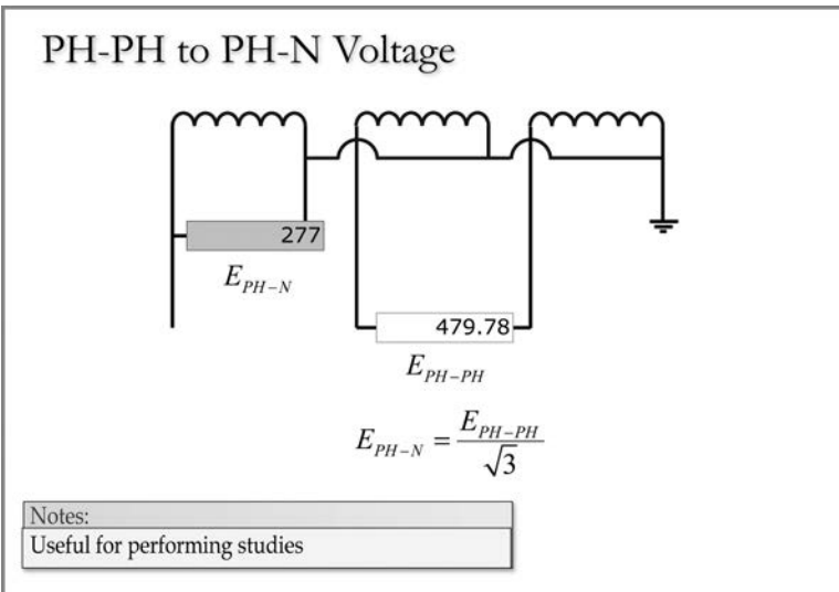
FIGURE 1.42 Phase-phase to phase-neutral.
