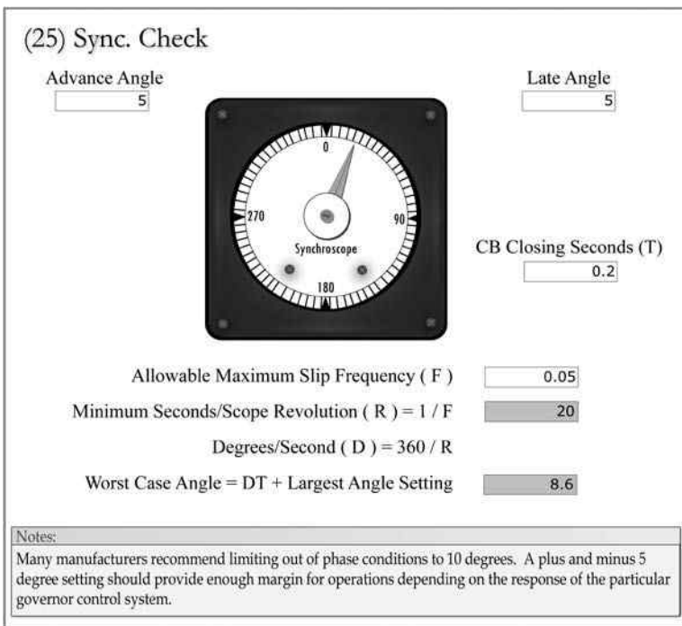
FIGURE 4.21 Synchronizing check relay settings.
