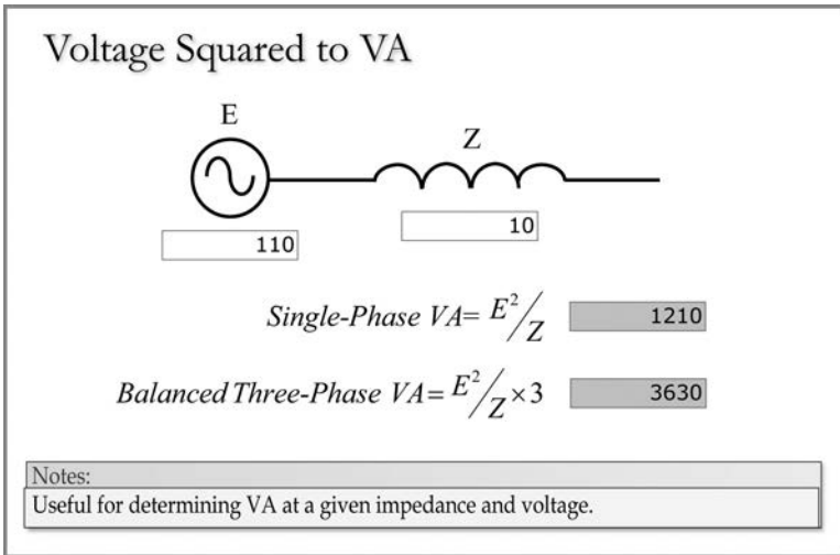
FIGURE 1.43 Voltage squared to VA.
