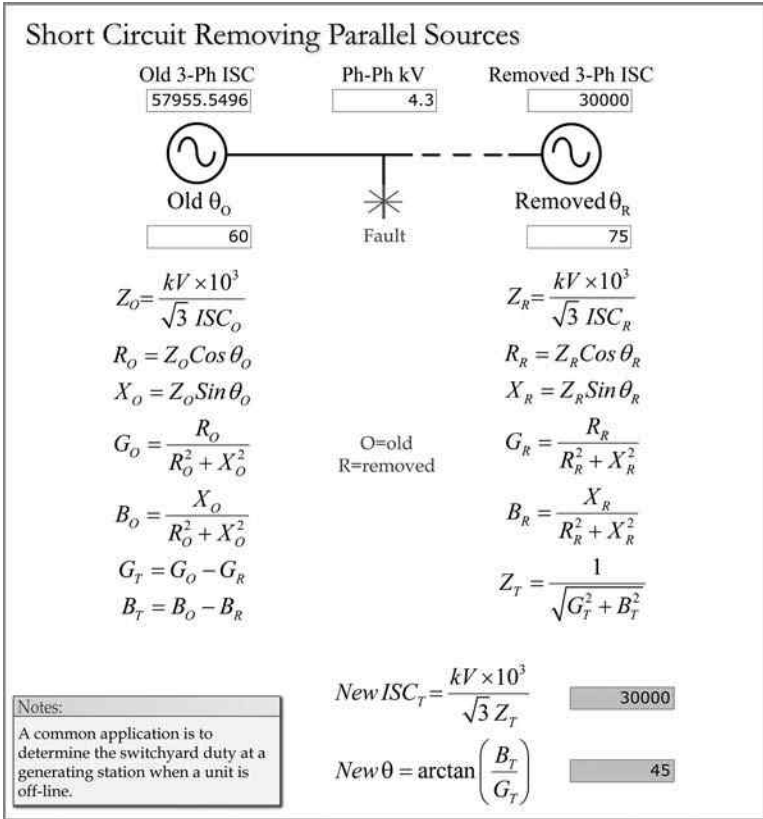
FIGURE 2.30 Short circuit: removing parallel sources.
