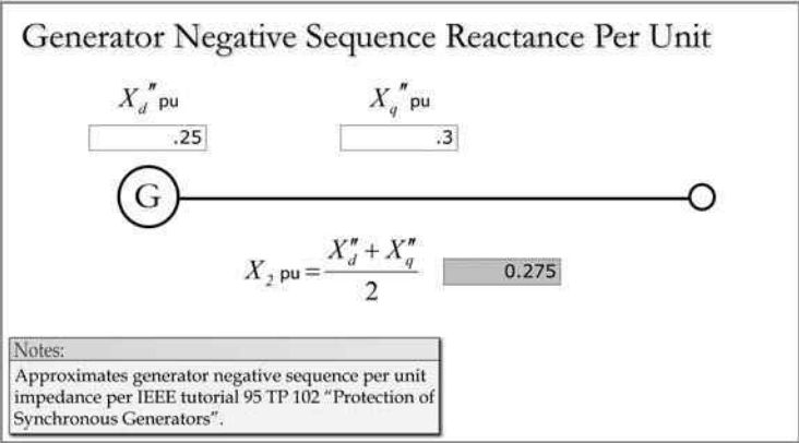
FIGURE 4.37 Negative phase sequence reactance.
