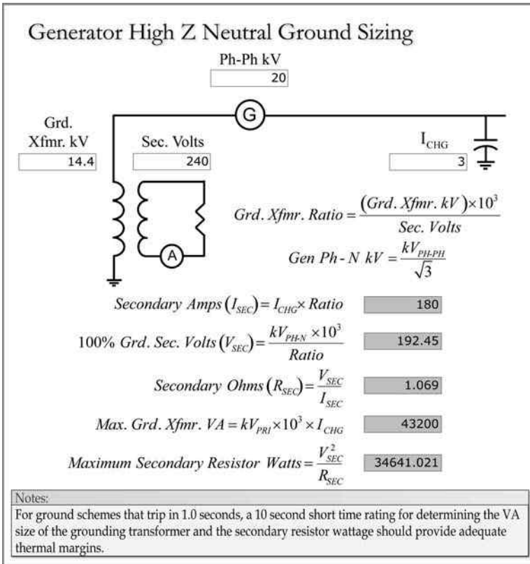
FIGURE 3.28 Generator neutral grounding transformer sizing.
