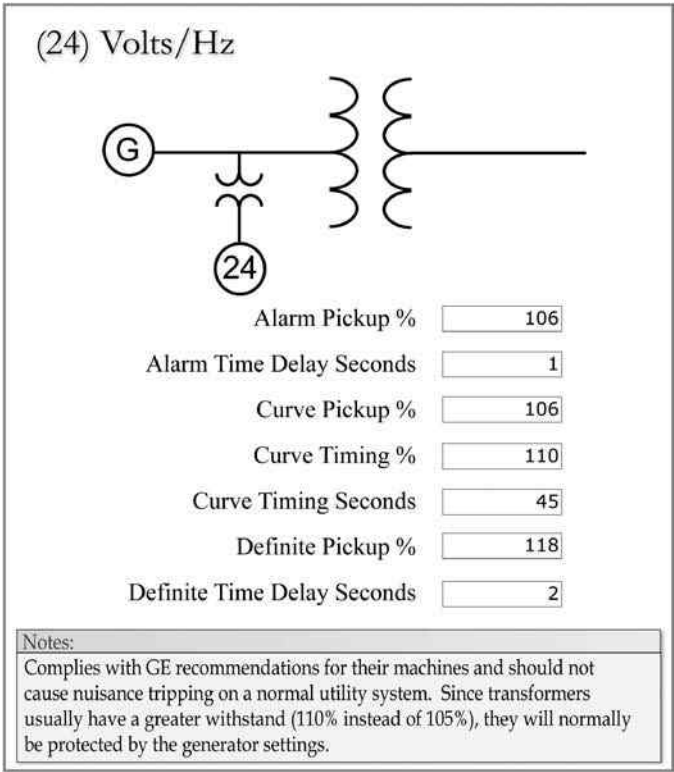
FIGURE 4.19 Volts/Hz settings.
