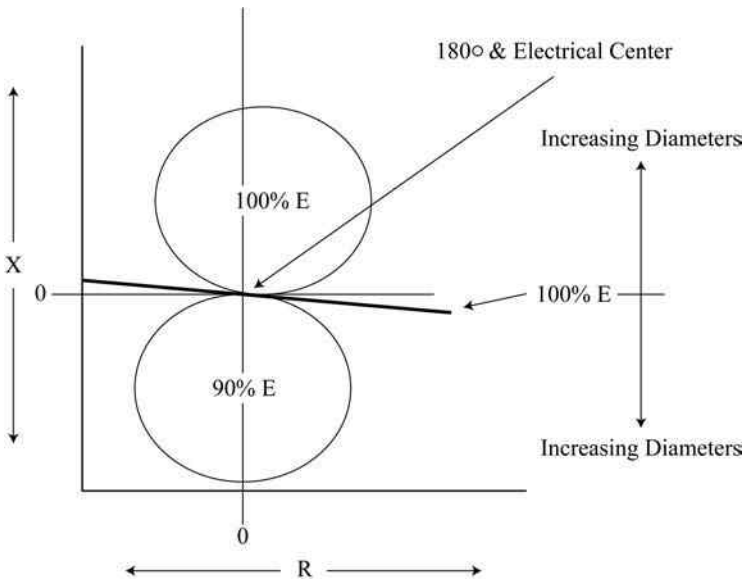
FIGURE 4.49 Out-of-step swing impedance.
