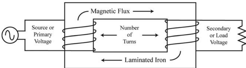
FIGURE 1.33 Simple transformer.
