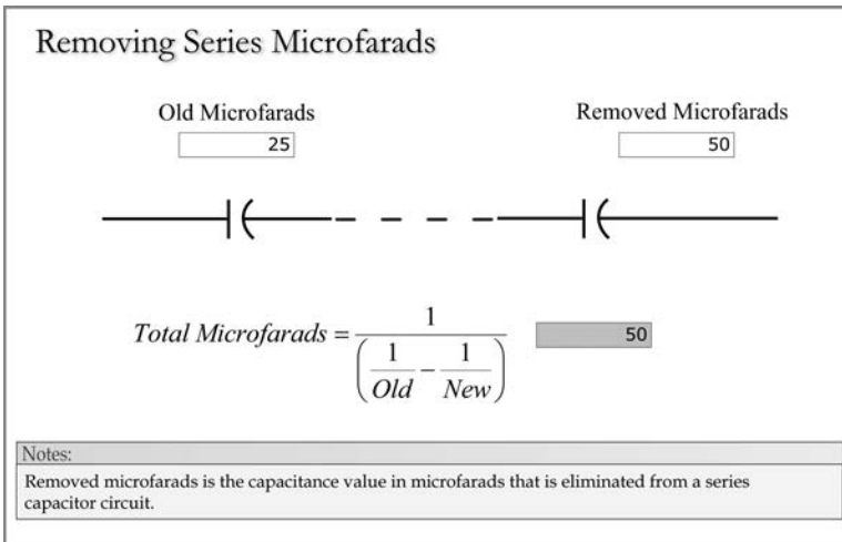
FIGURE 1.12 Removing series microfarads.
