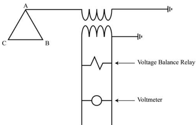
FIGURE 4.41 Single potential transformer ground detection.
