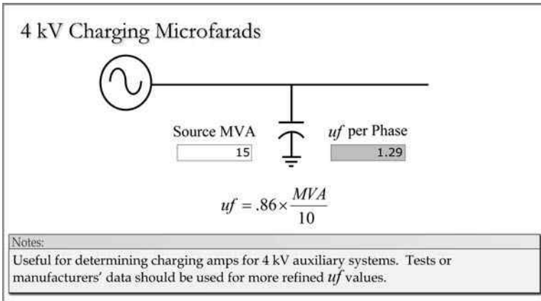
FIGURE 3.24 Typical 4-kV system capacitive microfarads.
