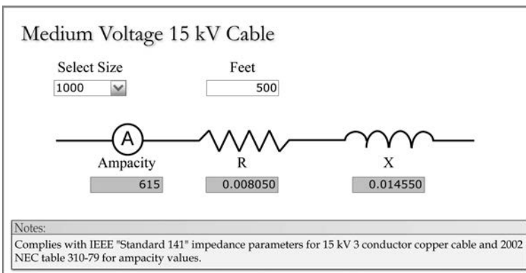
FIGURE 2.16 Medium-voltage 15-kV cable in a nonmagnetic conduit in earth.
