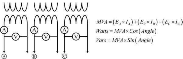
FIGURE 5.17 Three-element metering.
