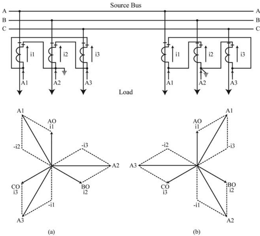
FIGURE 1.65 Current transformer delta lead and lag connections.
