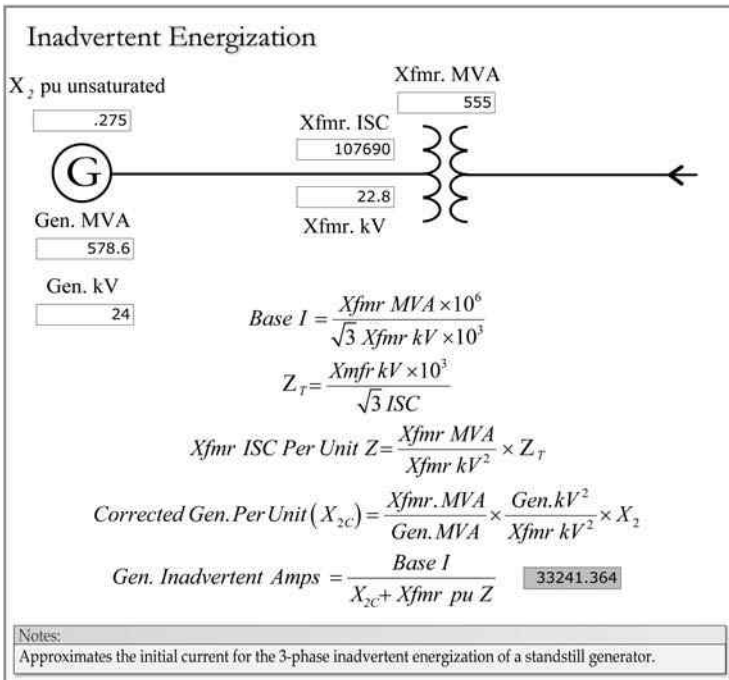
FIGURE 4.36 Inadvertent energization current.
