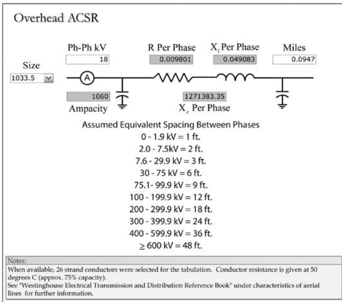
FIGURE 2.19 18-kV 1033.5 ACSR 3-foot spacing.
