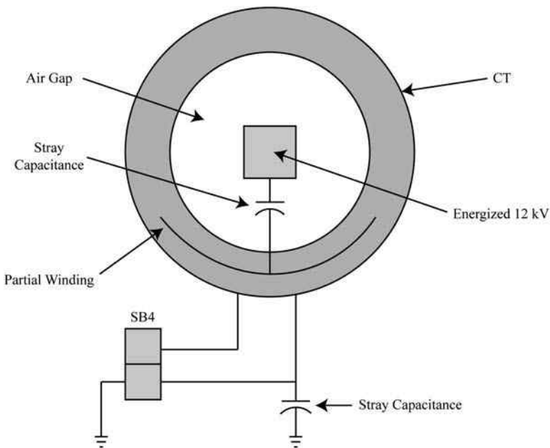
FIGURE 3.3 CT safety ground.
