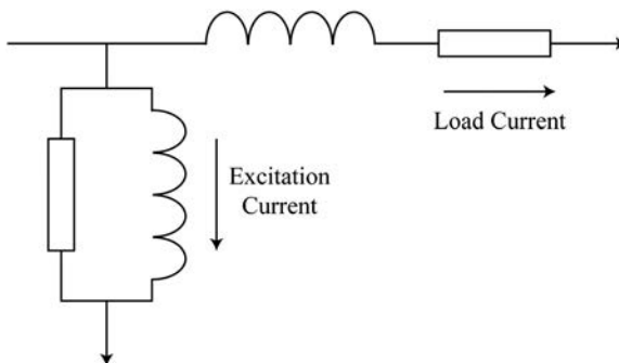
FIGURE 5.31 Transformer loss model.
