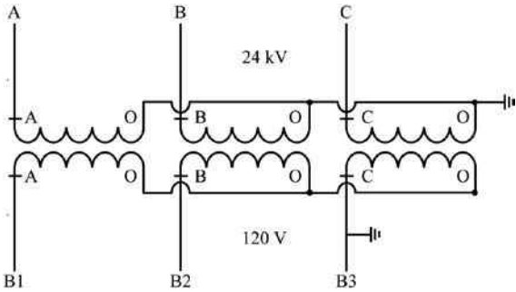
FIGURE 4.44 Modified wye-wye potential transformer grounding.
