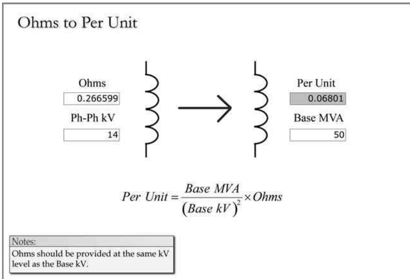
FIGURE 2.39 Ohms to per-unit.
