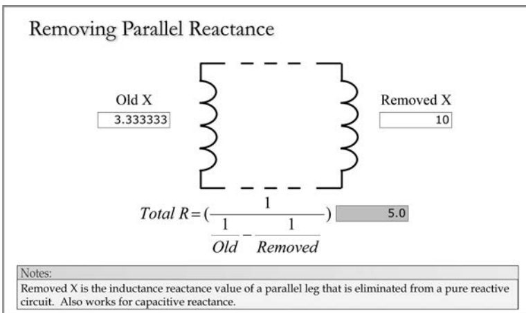
FIGURE 1.10 Removing parallel reactance or impedance.
