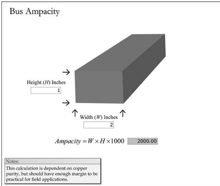
FIGURE 2.11 Copper bus ampacity.
