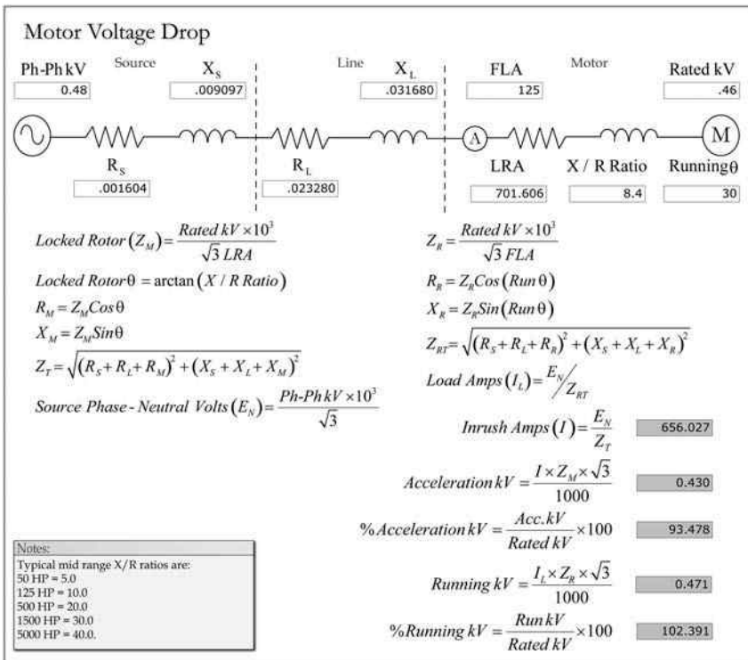
FIGURE 5.30 Motor 750 voltage drop.
