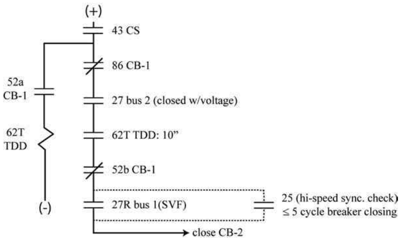
FIGURE 3.41 Bus transfer elementary.
