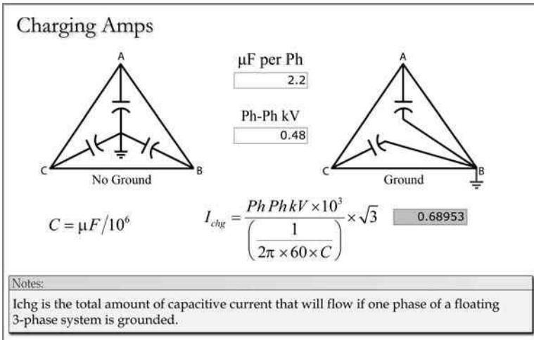
FIGURE 3.22 Capacitive charging amps.
