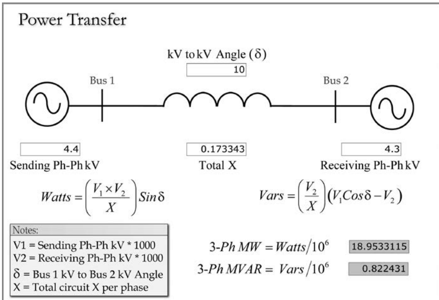
FIGURE 2.26 Power transfer equations.
