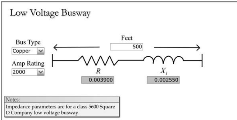
FIGURE 2.12 Low-voltage busway.
