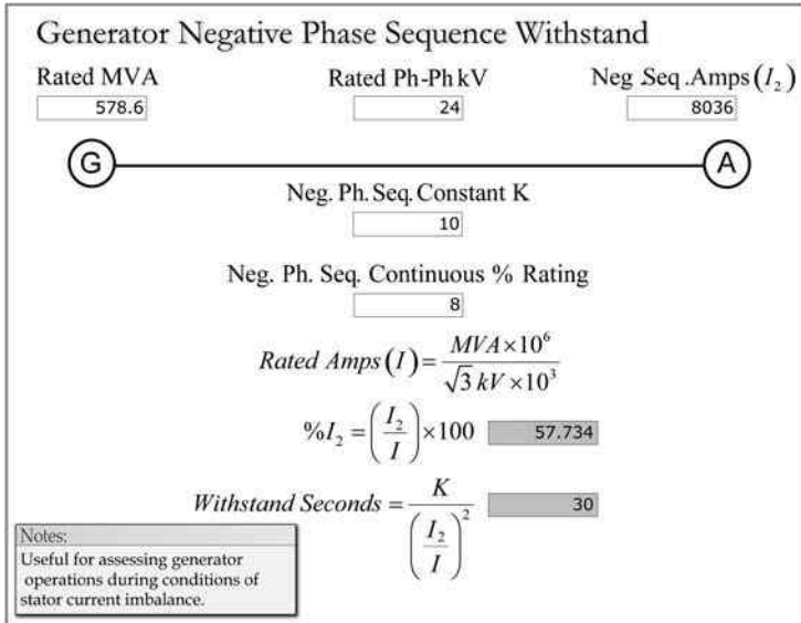
FIGURE 4.34 Negative phase sequence withstand.
