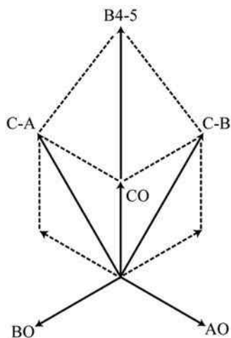
FIGURE 3.32 Grounded wye–broken delta ground detector phasors.
