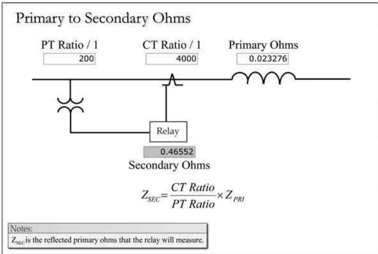
FIGURE 4.4 Primary to relay ohms.
