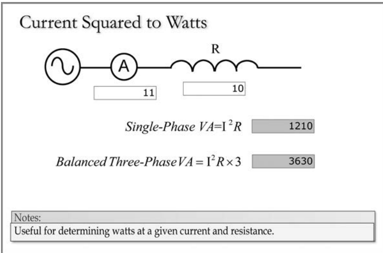
FIGURE 1.45 Current squared to watts.
