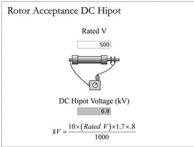
FIGURE 5.9 Generator rotor acceptance DC overvoltage testing.
