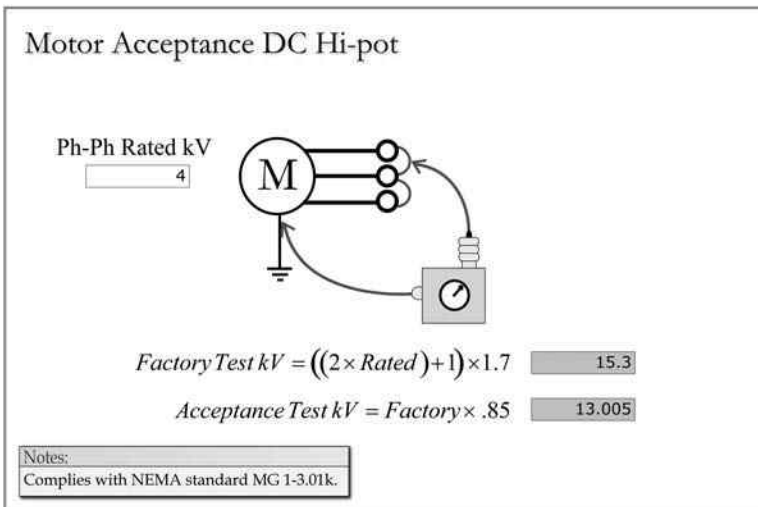
FIGURE 5.22 Motor acceptance DC overvoltage testing.
