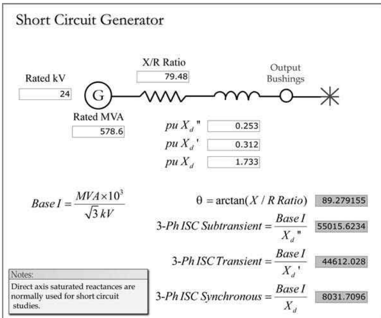
FIGURE 2.54 Generator short circuit.
