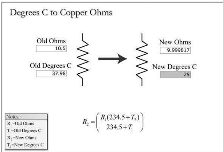
FIGURE 5.13 Degrees Celsius to copper ohms.
