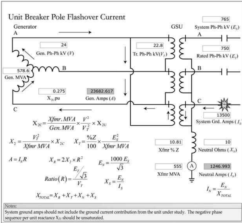
FIGURE 4.39 Pole flashover current.
