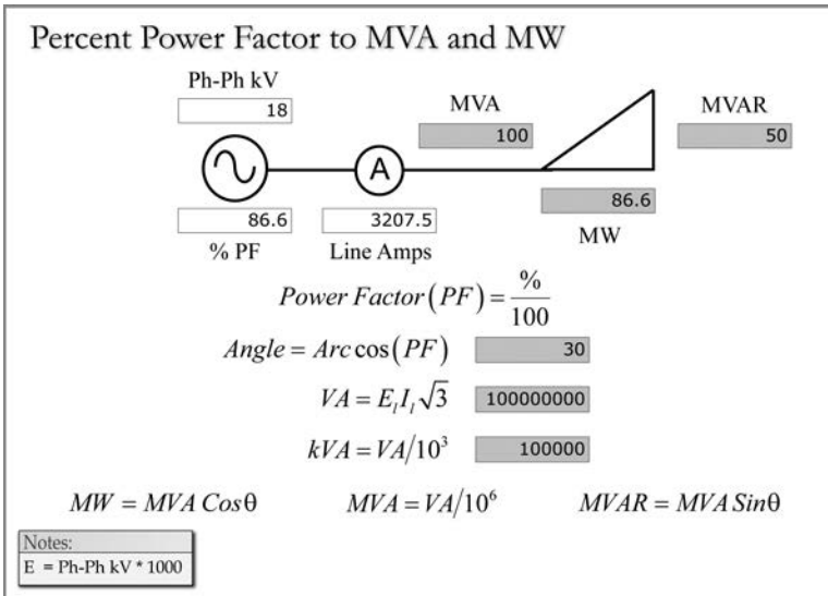
FIGURE 1.52 Percent power factor to MVA and MW.
