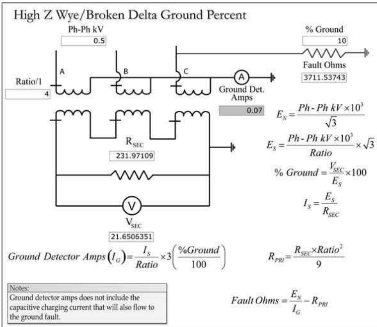
FIGURE 3.34 Grounded wye–broken delta ground detector fault ohms.
