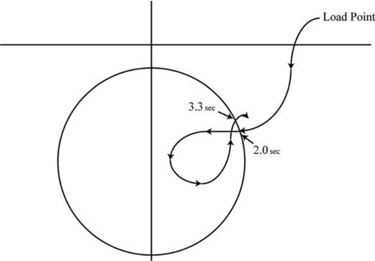
FIGURE 4.27 Loss-of-field impedance swing.
