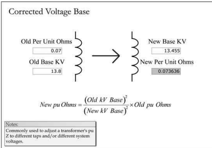
FIGURE 2.31 Transformer winding tap correction.
