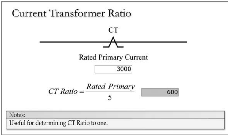
FIGURE 1.64 Current transformer ratio.
