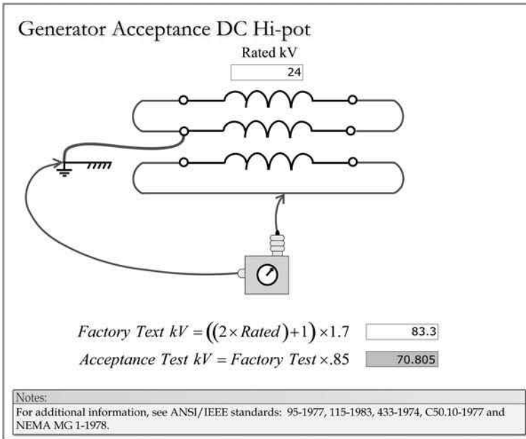
FIGURE 5.7 Generator stator acceptance DC overvoltage testing.
