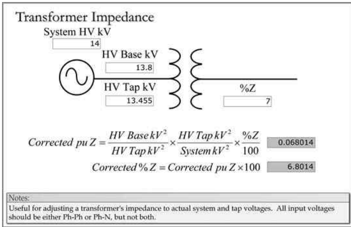
FIGURE 2.33 Transformer tap and applied voltage correction.
