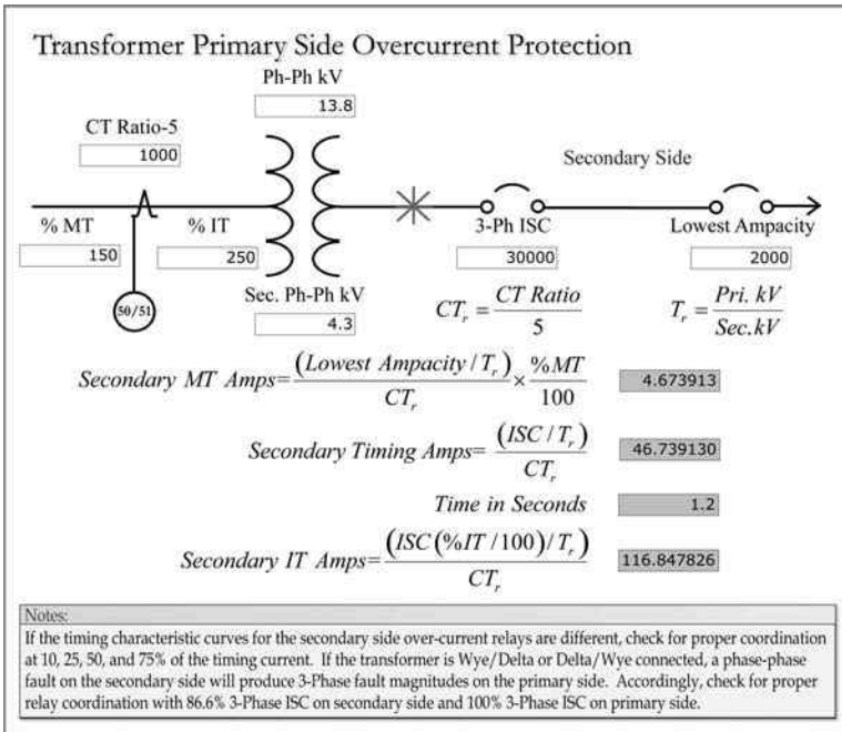
FIGURE 3.17 Transformer primary-side overcurrent settings.
