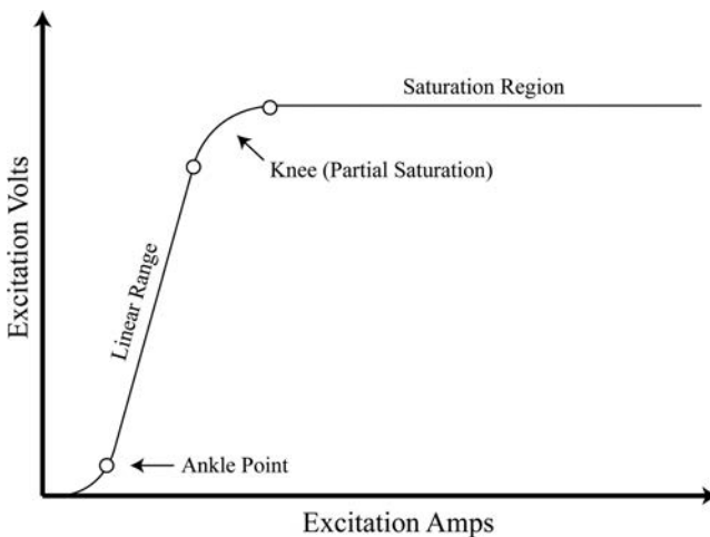
FIGURE 3.6 Typical CT saturation test curve.
