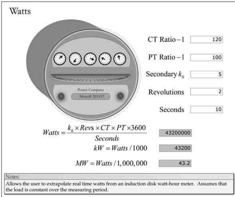
FIGURE 5.20 Watts.
