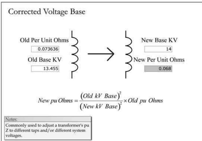
FIGURE 2.32 Transformer applied voltage correction.
