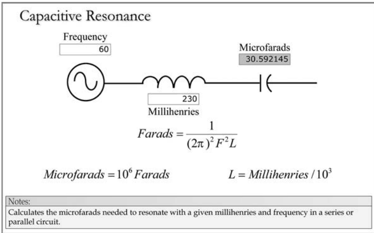
FIGURE 1.29 Capacitive resonance.
