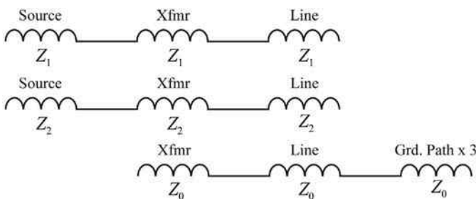
FIGURE 2.49 Normal delta-wye ground fault sequence impedance.
