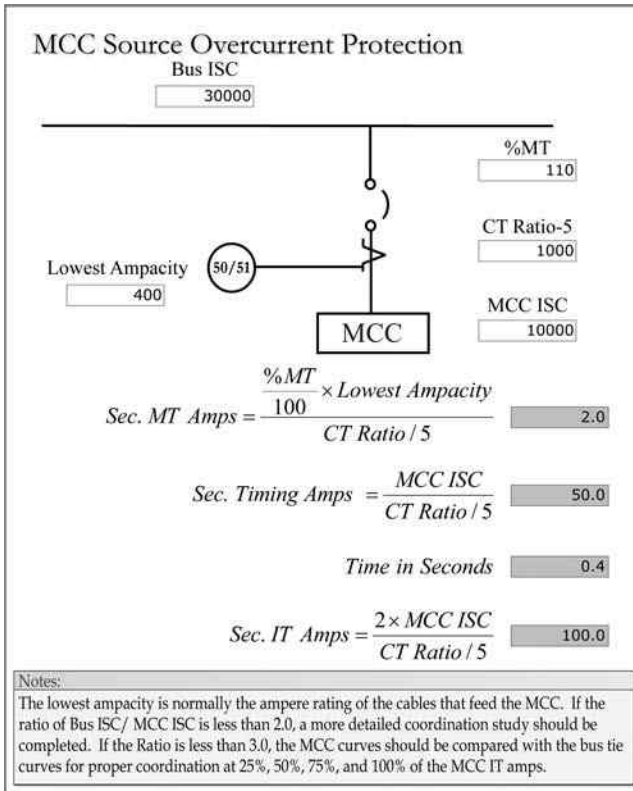
FIGURE 3.11 MCC source feeder overcurrent.
