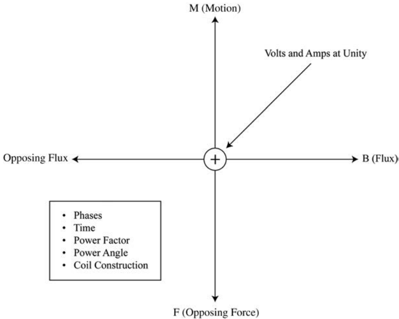
FIGURE 1.1 Magnetic phasors.
