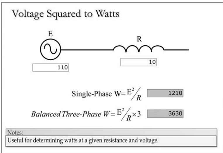
FIGURE 1.46 Voltage squared to watts.
