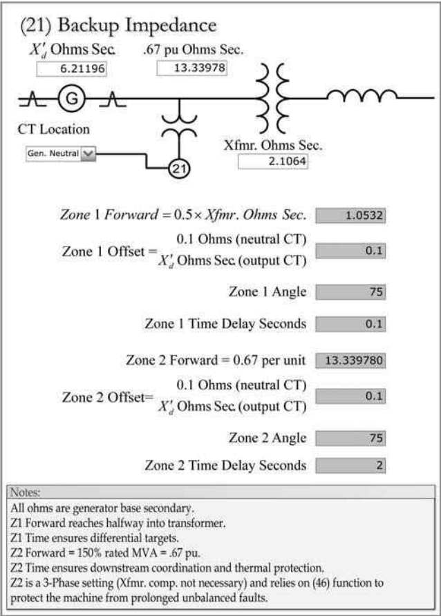
FIGURE 4.12 Generator backup impedance settings.
