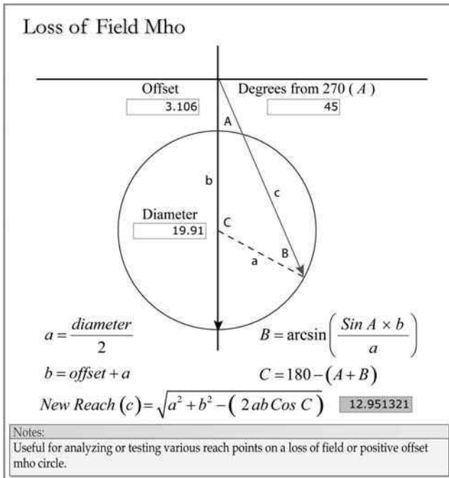
FIGURE 4.26 Loss-of-field mho circle.
