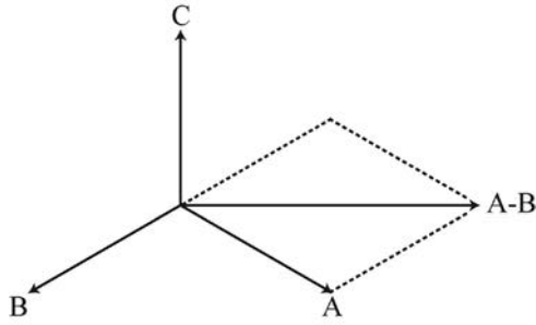
FIGURE 2.45 Delta-wye transformer phase-to-phase vectors.
