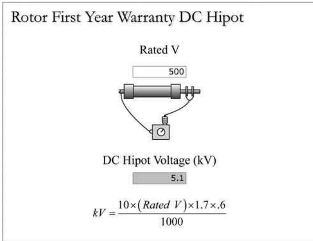
FIGURE 5.10 Generator rotor first-year-warranty DC overvoltage testing.
