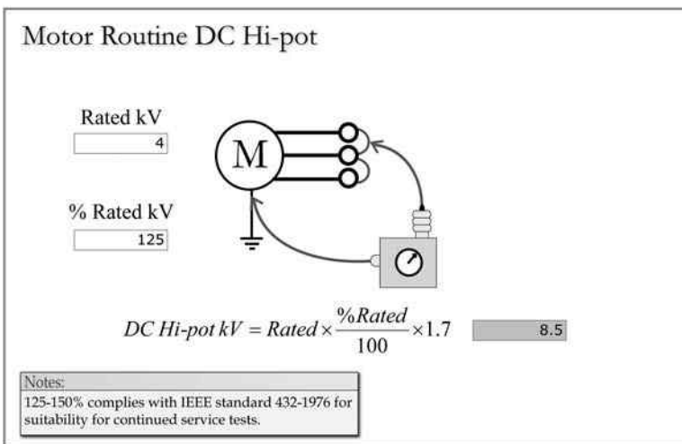
FIGURE 5.23 Motor routine DC overvoltage testing.
