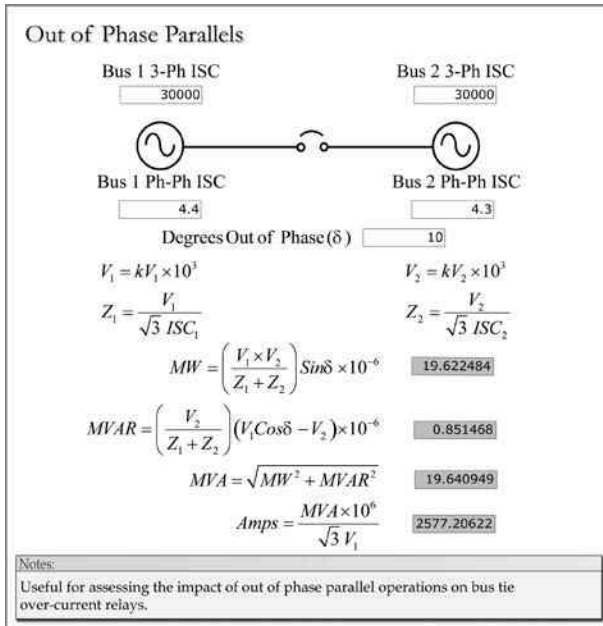
FIGURE 3.14 Bus parallel currents.
