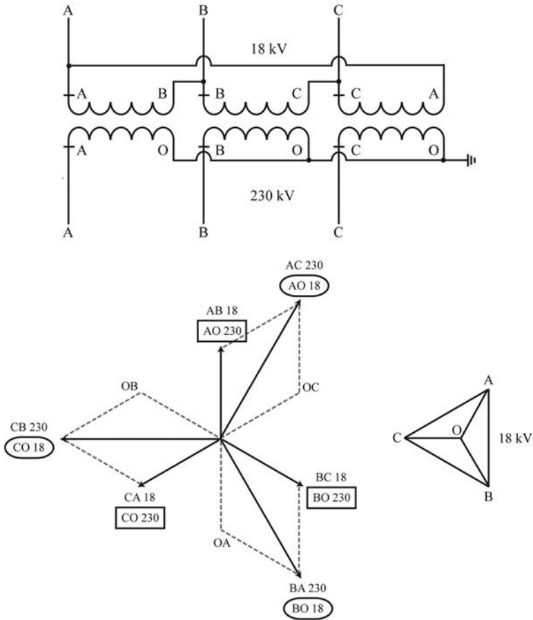
FIGURE 1.57 Delta-wye leading connection.
