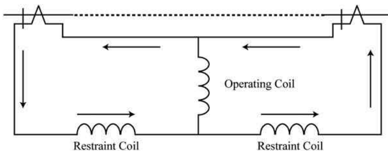
FIGURE 3.36 Current differential protection.
