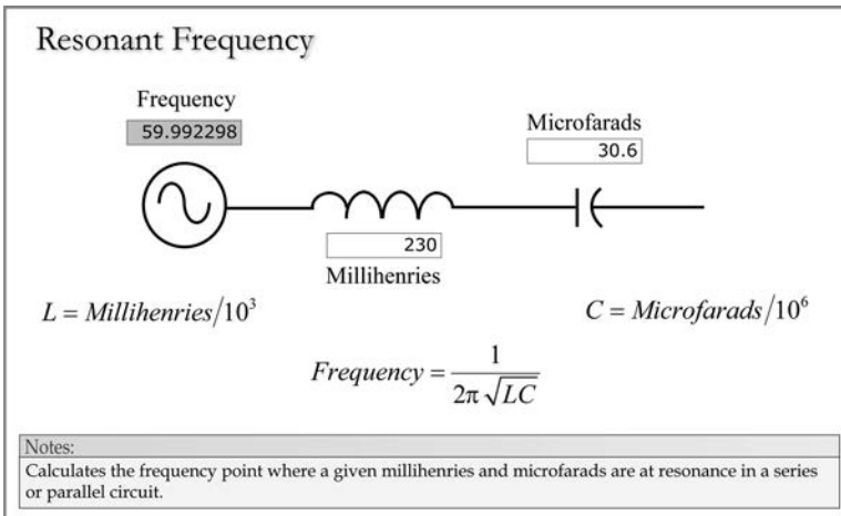
FIGURE 1.28 Resonant frequency.
