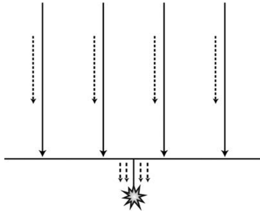
FIGURE 4.10 Fault current distribution and infeed ohms.
