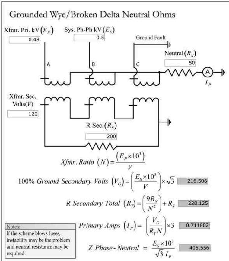
FIGURE 3.35 Grounded wye–broken delta neutral ohms.
