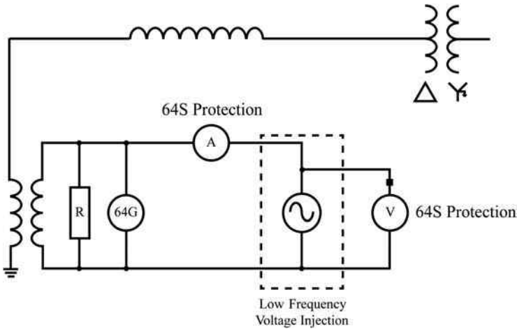
FIGURE 4.46 Typical subharmonic injection circuit.
