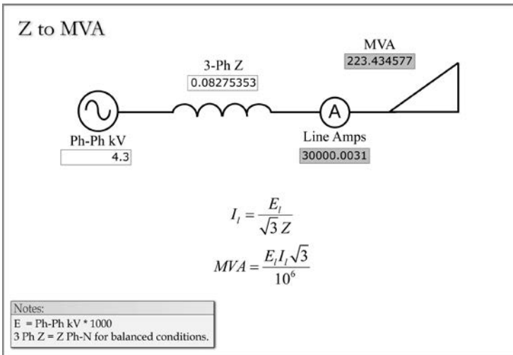
FIGURE 2.6 Z to MVA.
