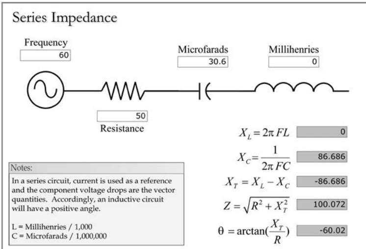
FIGURE 1.23 Series capacitive impedance.
