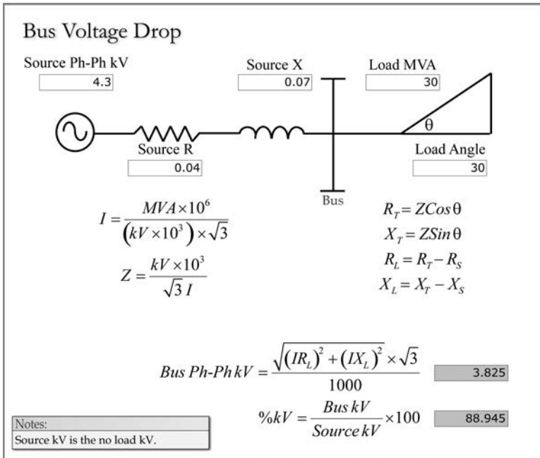
FIGURE 2.22 Bus voltage drop.
