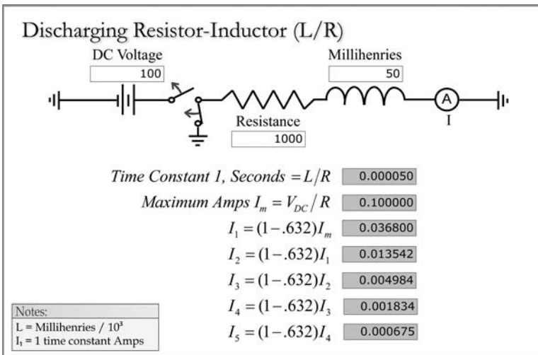
FIGURE 1.16 Discharging resistor-inductor (L/R).
