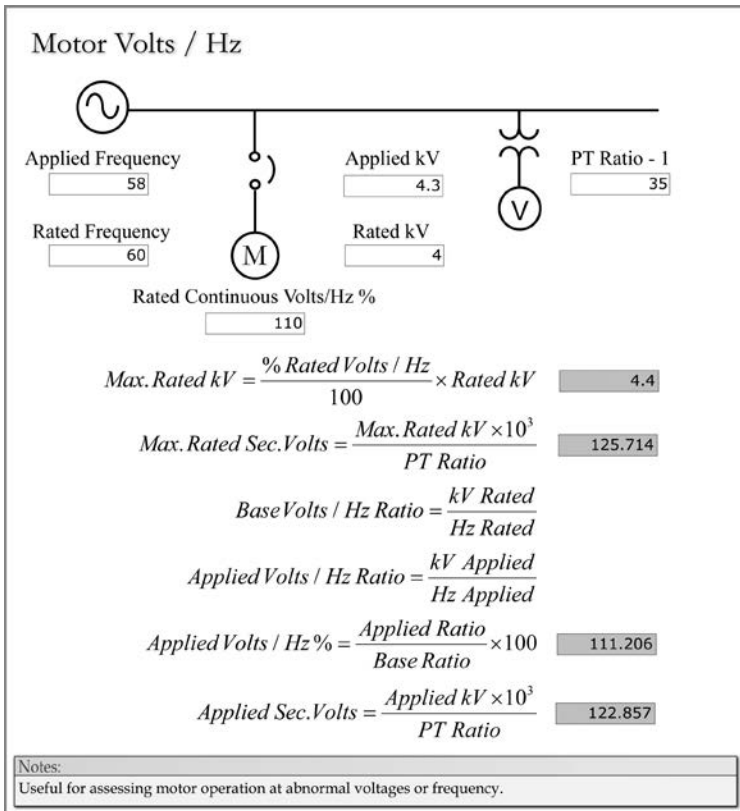
FIGURE 2.9 Motor volts/Hz withstands.
