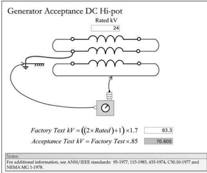
FIGURE 7.5 Generator DC acceptance test.
