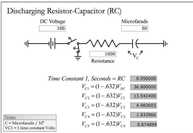
FIGURE 1.14 Discharging resistor–capacitor (RC).
