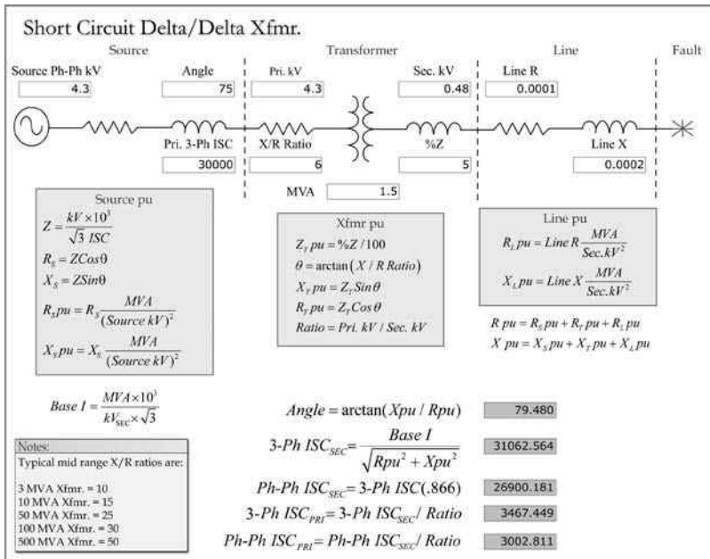
FIGURE 2.41 Delta–delta transformer short circuit.
