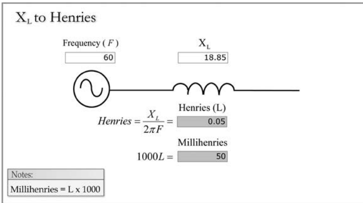
FIGURE 1.21 Inductive reactance to henries.
