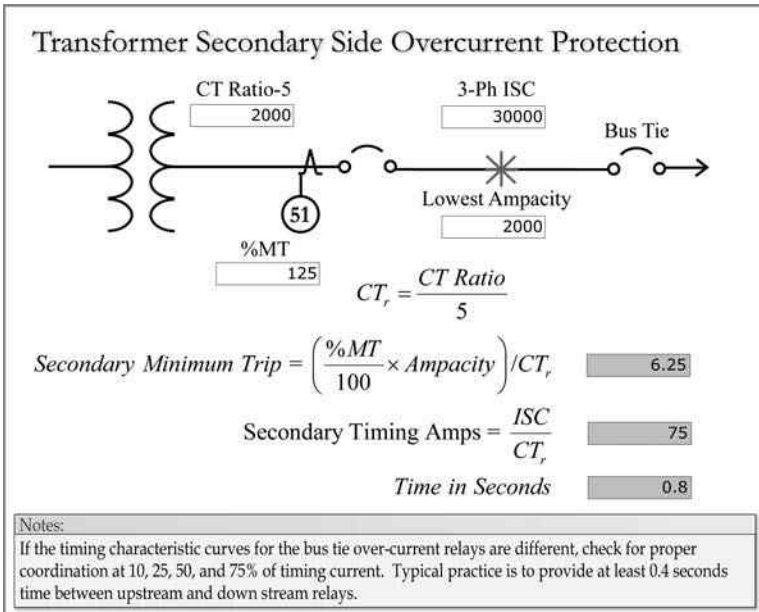
FIGURE 3.16 Transformer secondary-side overcurrent settings.
