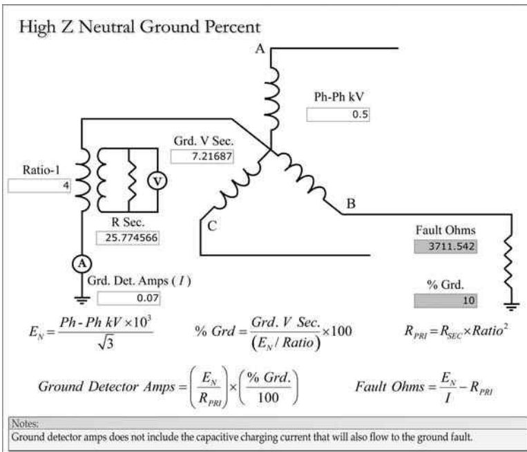
FIGURE 3.30 Neutral ground detector fault ohms.
