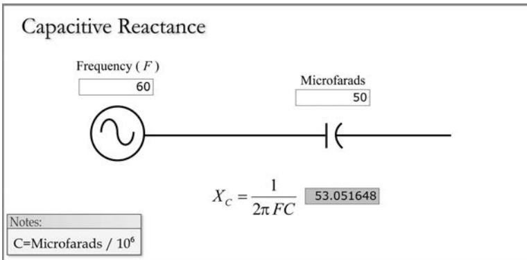
FIGURE 1.19 Capacitive reactance.
