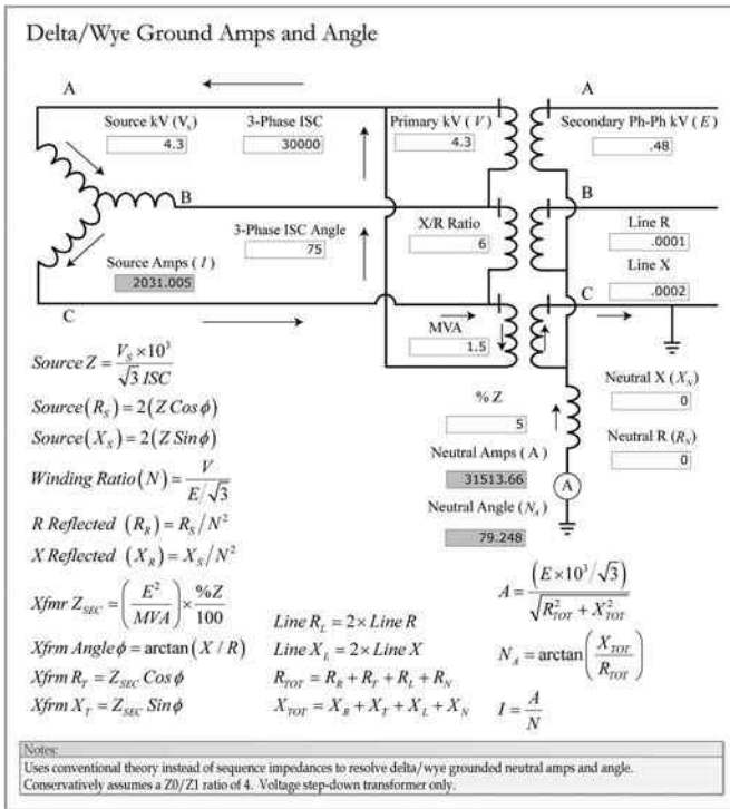
FIGURE 2.53 Step-down transformer ohmic ground fault calculation.
