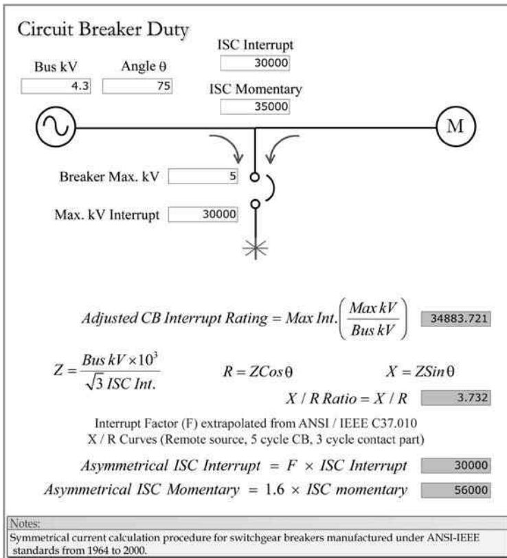
FIGURE 5.6 Circuit breaker duty.
