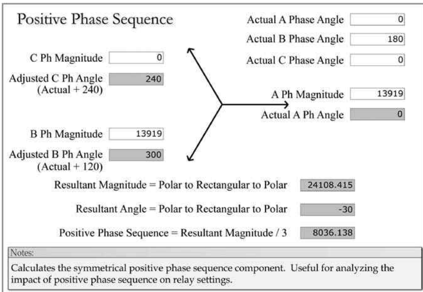
FIGURE 4.32 Positive phase sequence magnitude.
