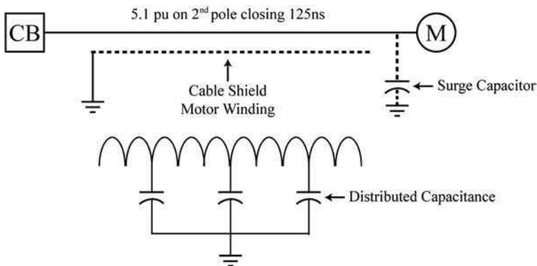
FIGURE 5.28 Motor-switching transients.
