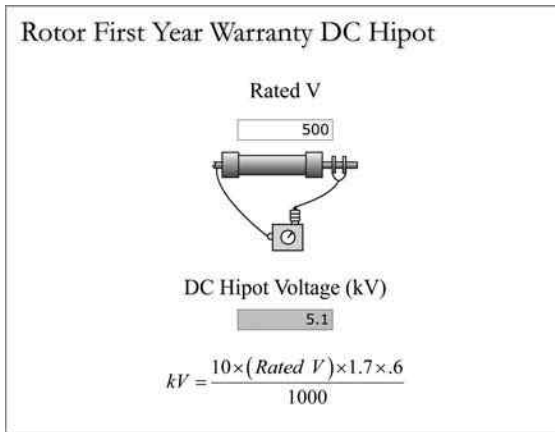
FIGURE 7.10 Generator rotor first-year warranty DC overvoltage testing.
