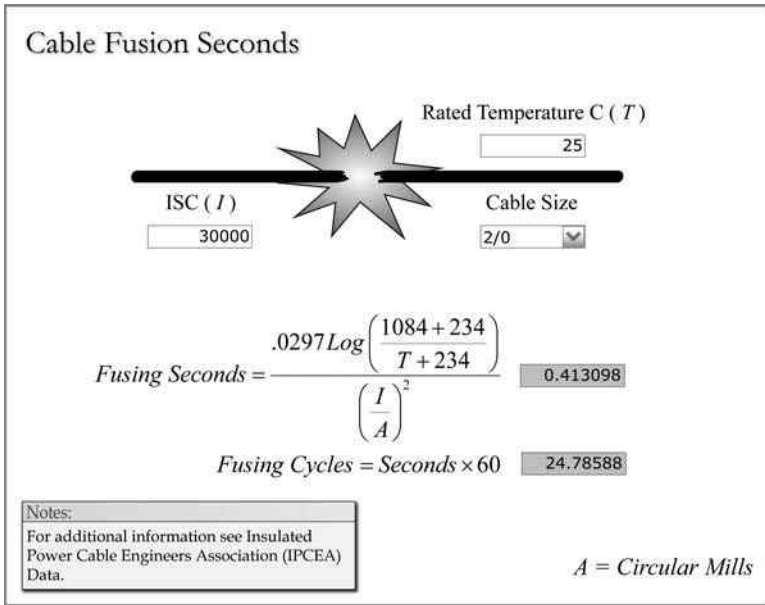
FIGURE 7.13 Cable short circuit fusion.
