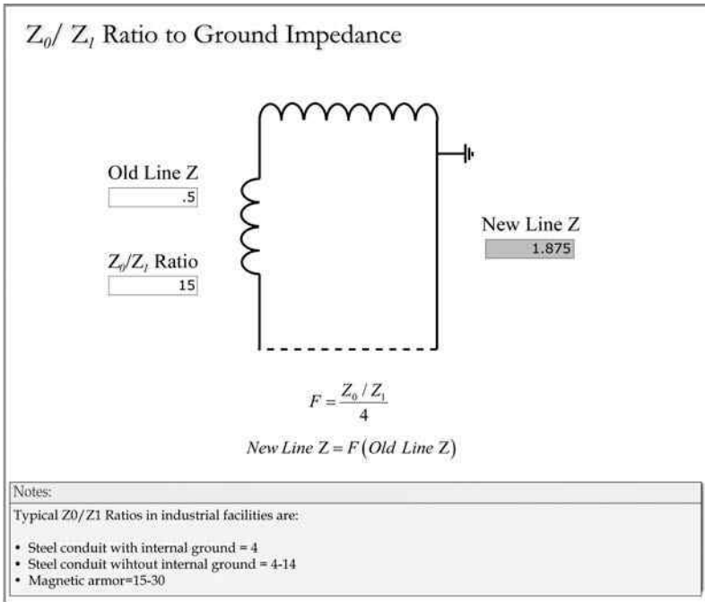
FIGURE 2.52 Z_0 / Z_1 ratio to line impedance increase.
