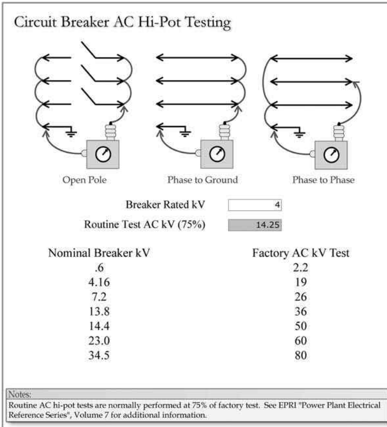
FIGURE 5.5 Circuit breaker AC hipot testing.
