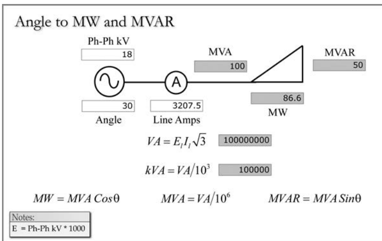
FIGURE 1.49 Angle to MVA and MW.
