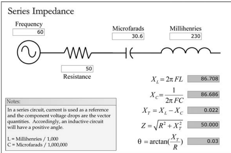
FIGURE 1.27 Series resonant impedance.
