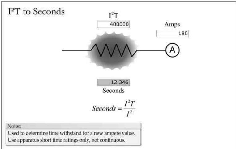
FIGURE 3.29 I 2 T calculation.
