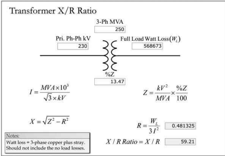
FIGURE 5.33 Transformer X/R ratio.
