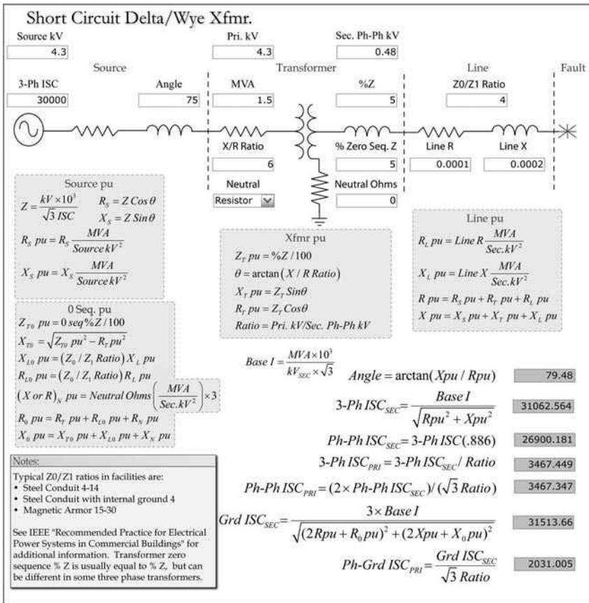
FIGURE 2.43 Delta-wye transformer short circuit.
