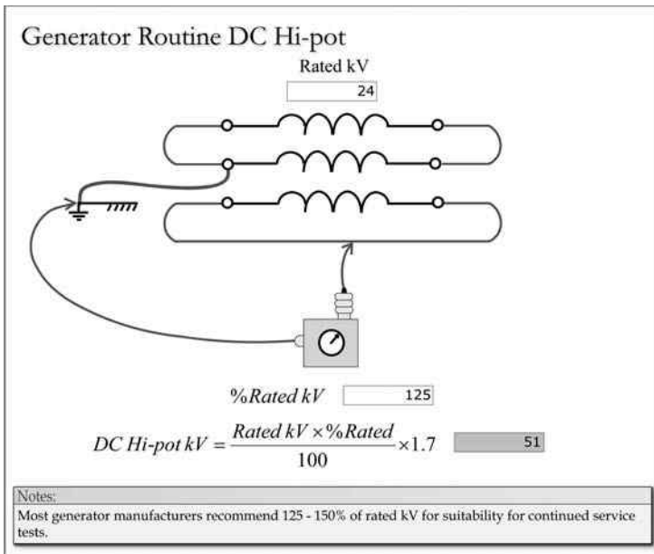
FIGURE 7.6 Generator routine test.
