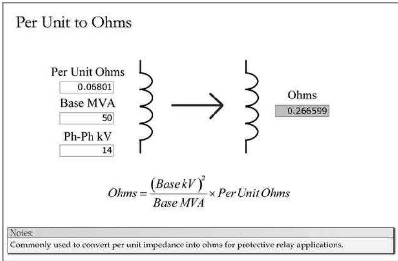
FIGURE 2.38 Per unit to ohms.
