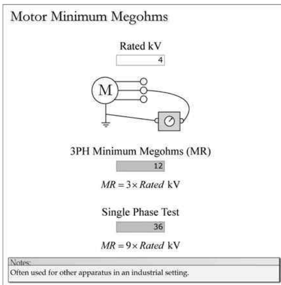
FIGURE 7.4 Motor insulation resistance.
