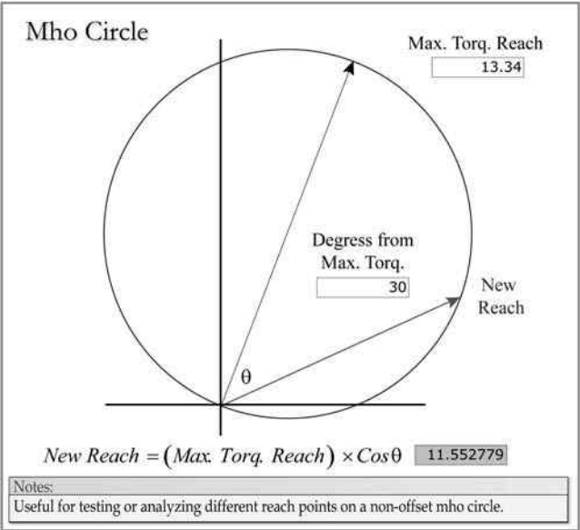
FIGURE 4.13 Mho circle reach points.
