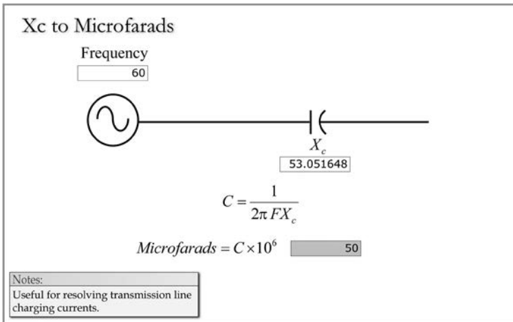
FIGURE 1.22 Capacitive reactance to microfarads.
