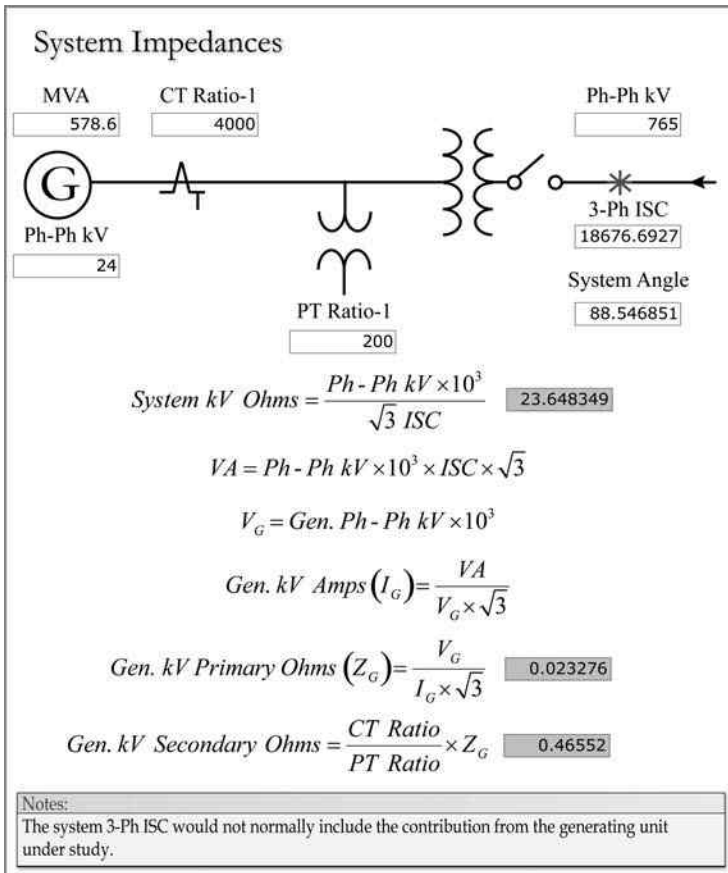
FIGURE 4.3 System data.
