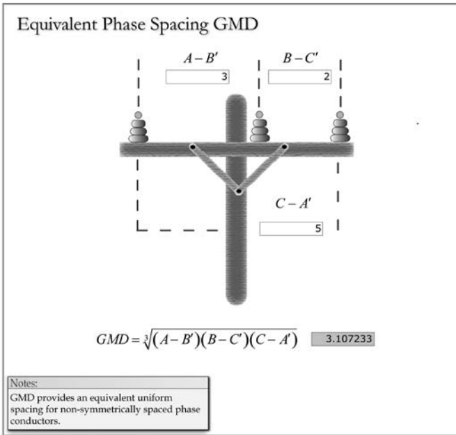
FIGURE 2.18 Equivalent symmetrical conductor spacing.
