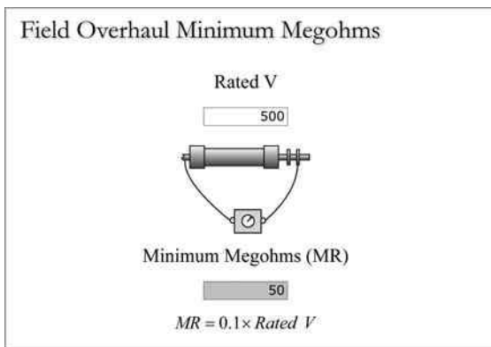
FIGURE 7.11 Generator rotor routine overhaul insulation testing.
