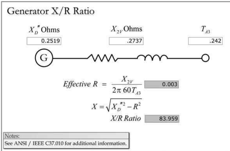
FIGURE 5.16 Generator X/R ratio.
