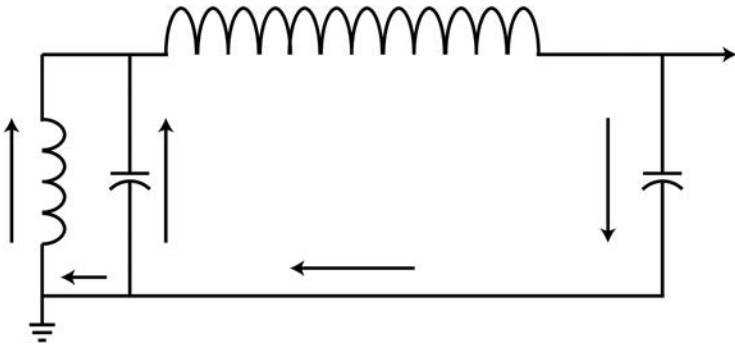
FIGURE 4.47 Generator third harmonic circuit depiction.
