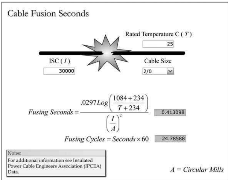
FIGURE 5.3 Cable short circuit fusion seconds.
