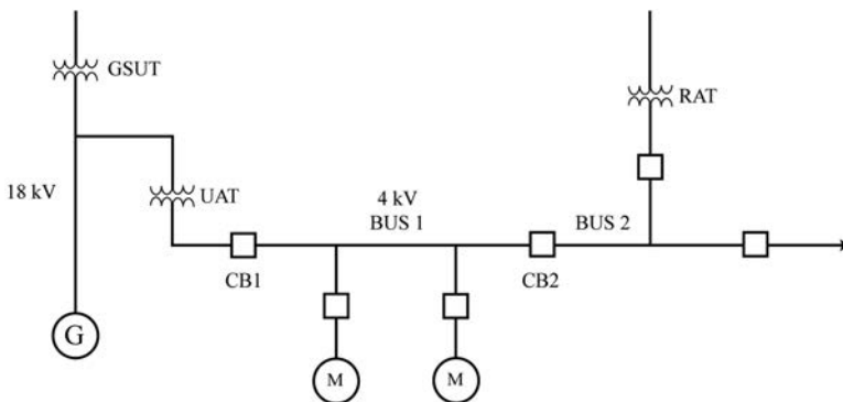
FIGURE 3.39 Typical generating station one-line.
