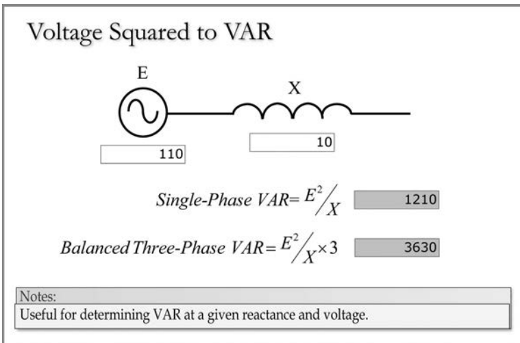
FIGURE 1.51 Volts to VAR.
