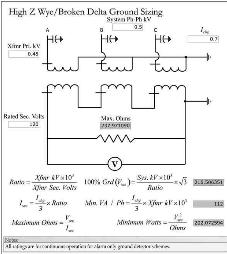
FIGURE 3.33 Grounded wye–broken delta ground detector sizing.
