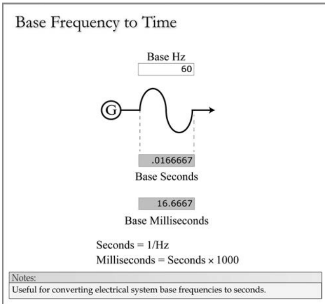
FIGURE 1.4 Base frequency to time.
