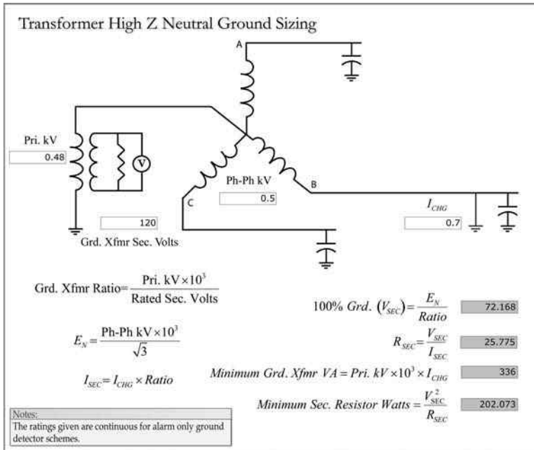
FIGURE 3.27 Neutral grounding transformer sizing.
