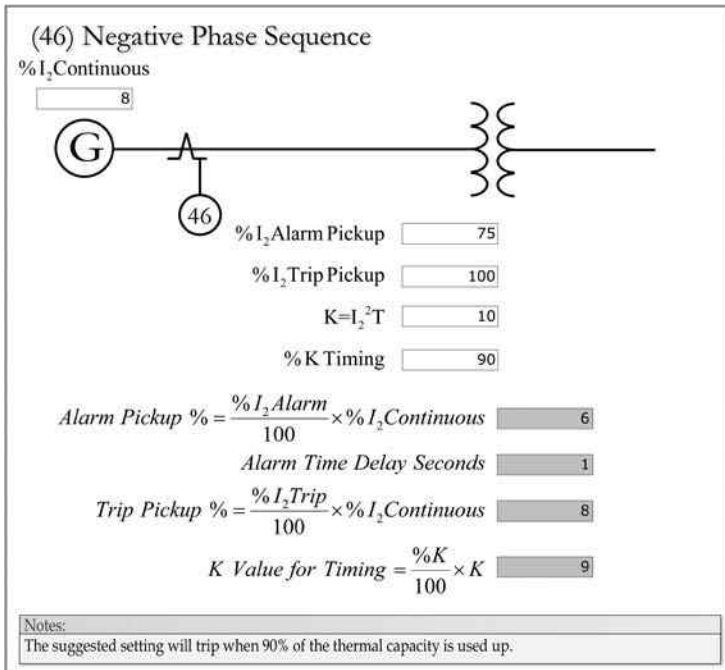
FIGURE 4.35 Negative phase sequence relay settings.
