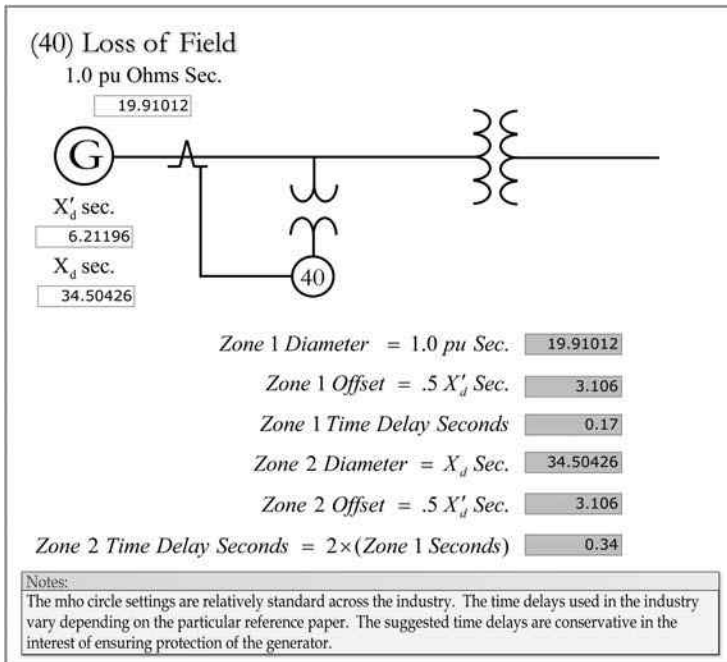
FIGURE 4.28 Loss-of-field relay settings.
