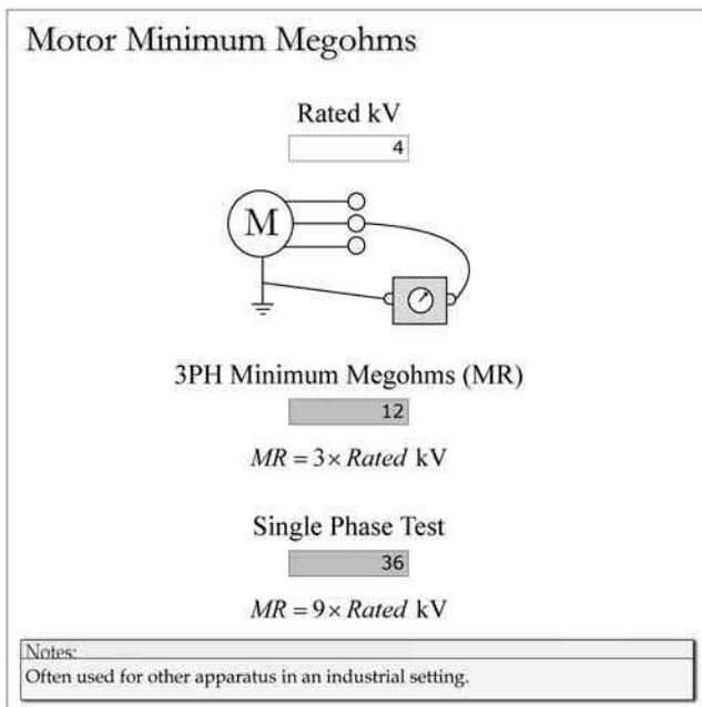
FIGURE 5.21 Motor insulation resistance.
