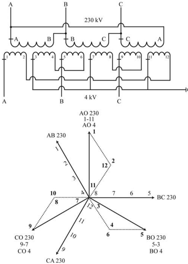
FIGURE 1.61 Delta-wye-zigzag connection.
