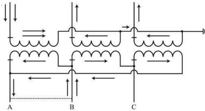
FIGURE 2.46 Wye-delta transformer phase-to-phase faults.
