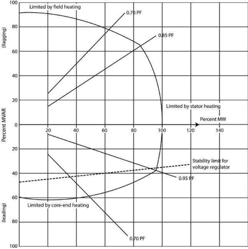
FIGURE 4.25 Generator capability curve.
