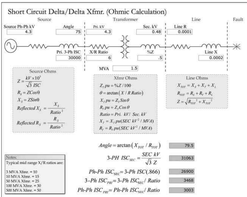
FIGURE 2.48 Comparing per-unit to ohmic short circuit procedures.
