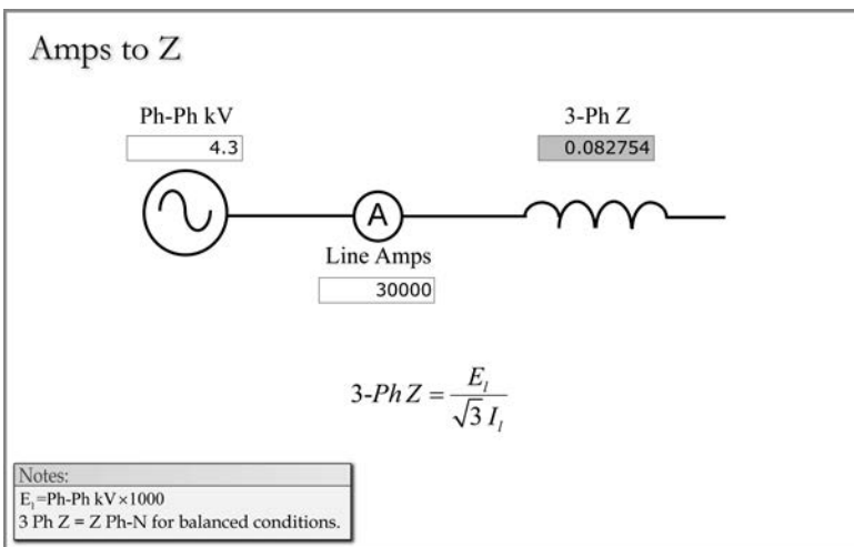
FIGURE 2.2 Amps to Z conversion.
