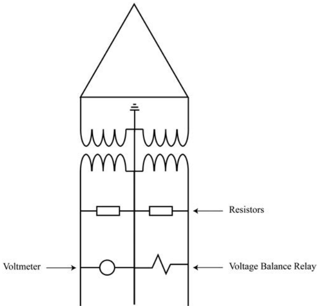
FIGURE 4.42 Two-transformer ground detection scheme.
