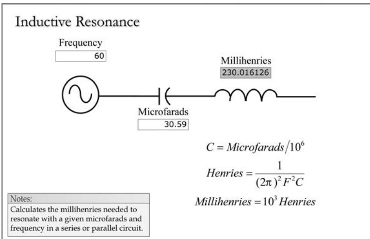
FIGURE 1.30 Inductive resonance.
