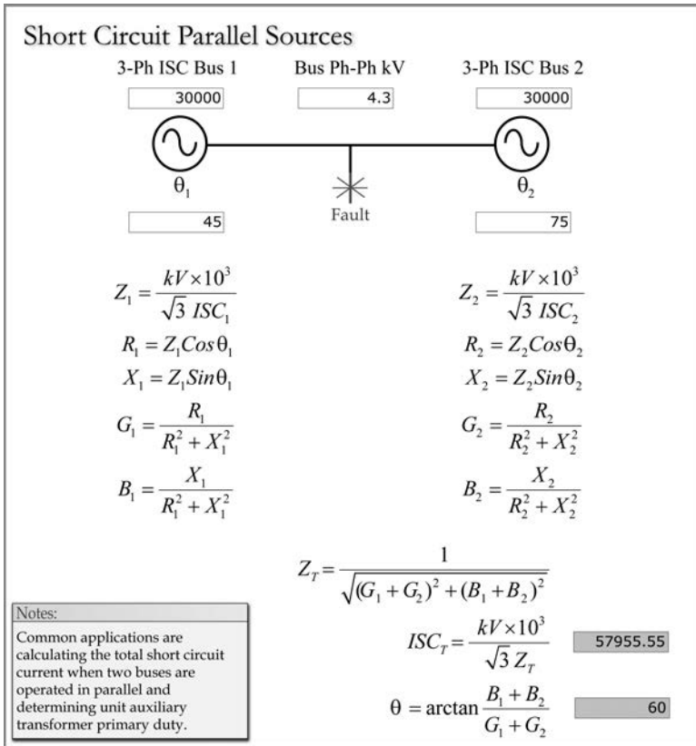
FIGURE 2.29 Short circuit: parallel sources.
