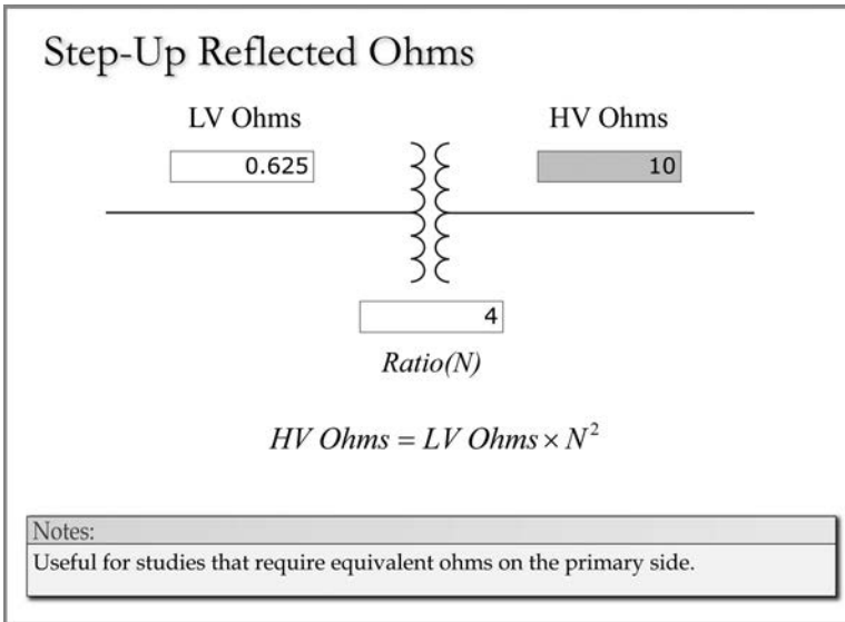
FIGURE 1.36 Reflected ohms LV to HV.
