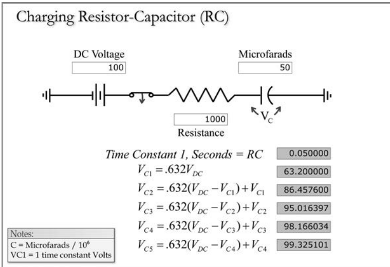
FIGURE 1.13 Charging resistor–capacitor (RC).
