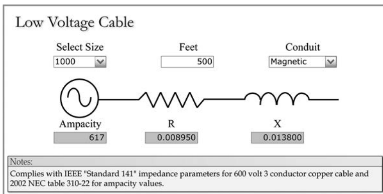
FIGURE 2.13 Low-voltage cable in a magnetic conduit.
