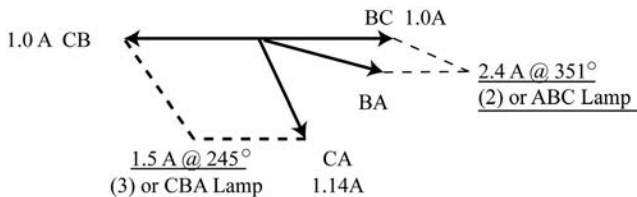
FIGURE 1.55 Vector results for ABC rotation.
