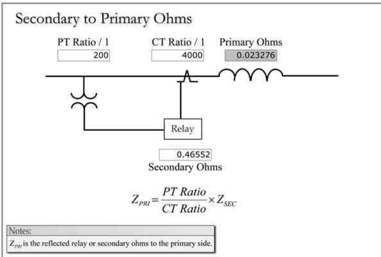
FIGURE 4.5 Relay to primary ohms.
