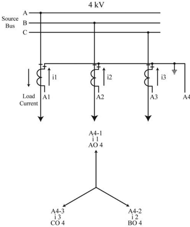
FIGURE 1.63 Current transformer wye connection.
