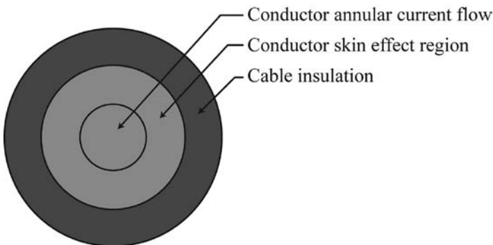
FIGURE 2.10 Conductor radius and inductance.
