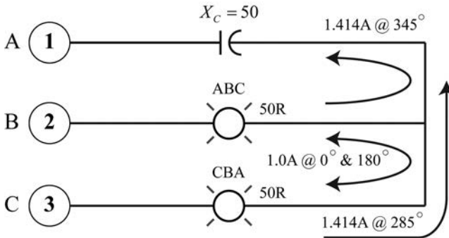
FIGURE 1.54 Two lamp phase rotation sequence indicator.
