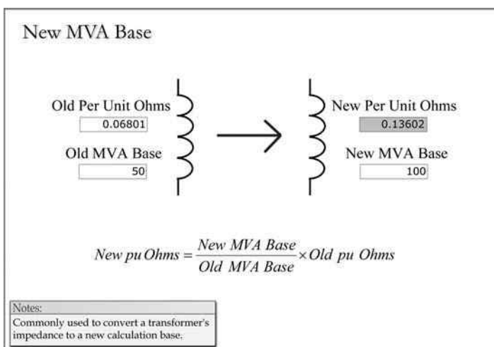
FIGURE 2.37 New MVA base.
