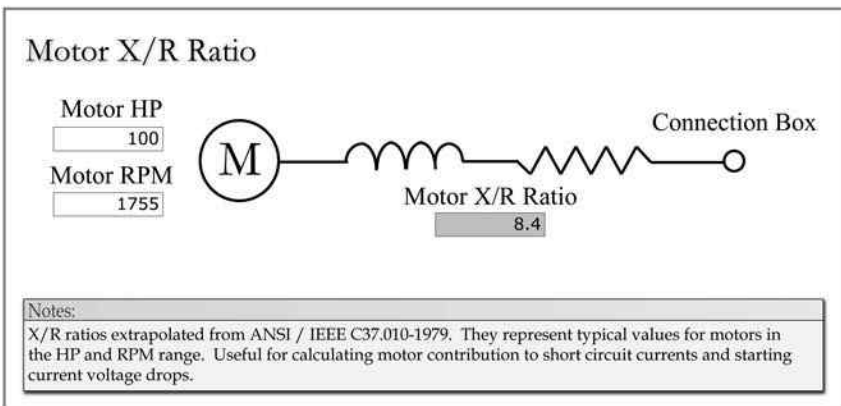
FIGURE 5.26 Motor X/R ratio.
