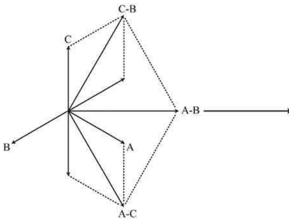
FIGURE 2.47 Wye-delta transformer phase-to-phase vectors.
