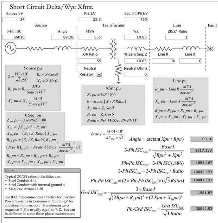
FIGURE 4.38 GSUT short circuit currents.
