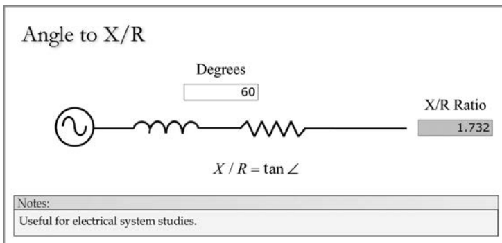
FIGURE 1.18 Angle to X/R.
