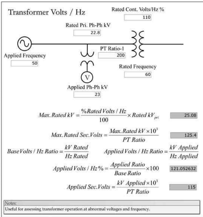
FIGURE 4.16 Transformer volts/Hz.
