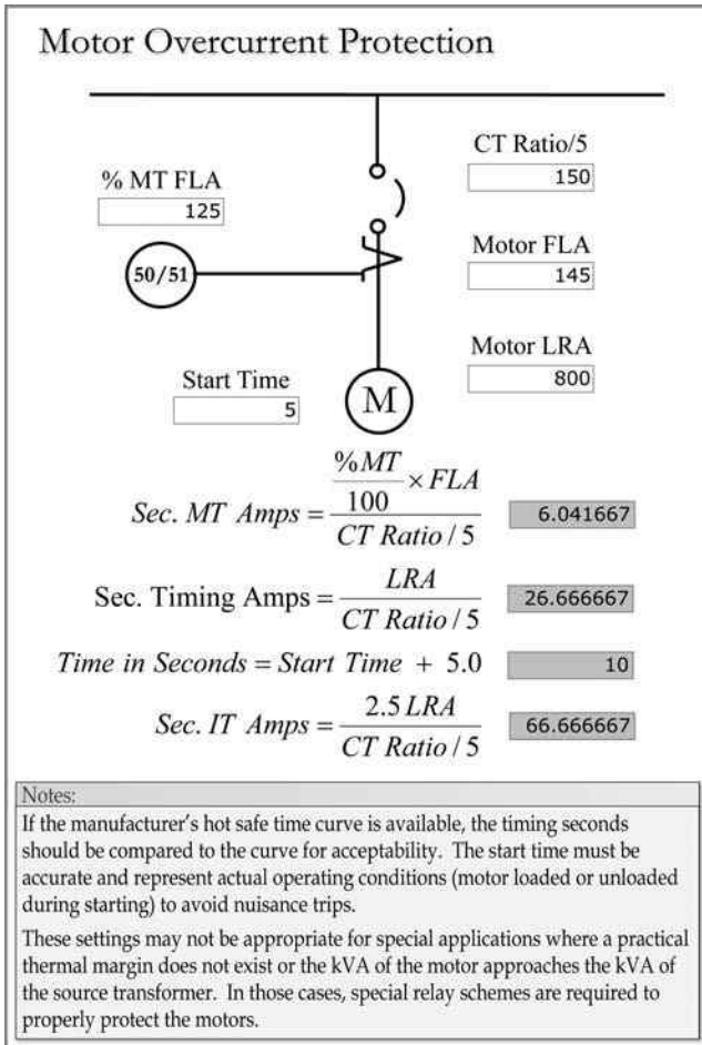
FIGURE 3.8 Motor overcurrent settings.
