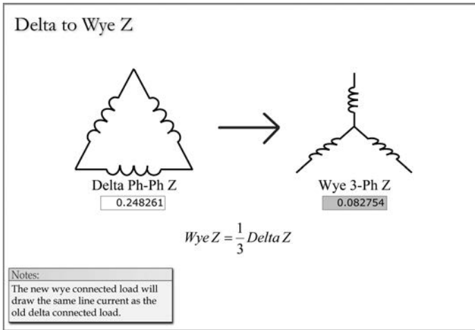
FIGURE 2.3 Delta to wye Z.
