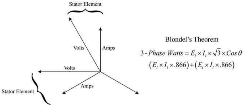
FIGURE 5.18 Two-element metering.
