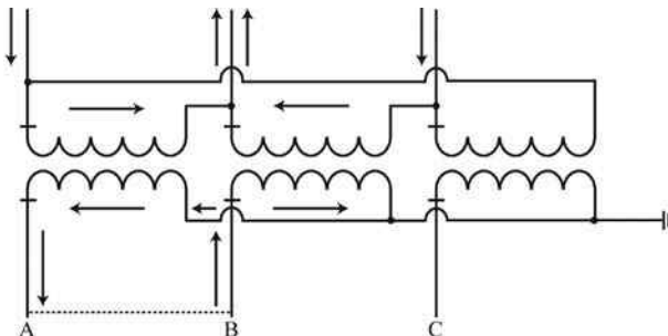
FIGURE 2.44 Delta-wye transformer phase-to-phase faults.
