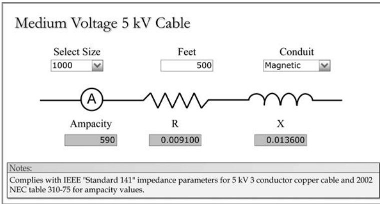
FIGURE 2.15 Medium-voltage 5-kV cable in a magnetic conduit.
