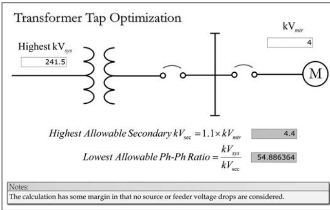
FIGURE 2.8 Transformer winding tap optimization.
