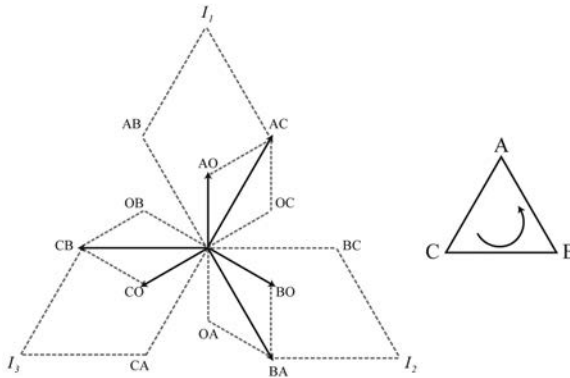
FIGURE 1.40 Wye configurations and relationships.
