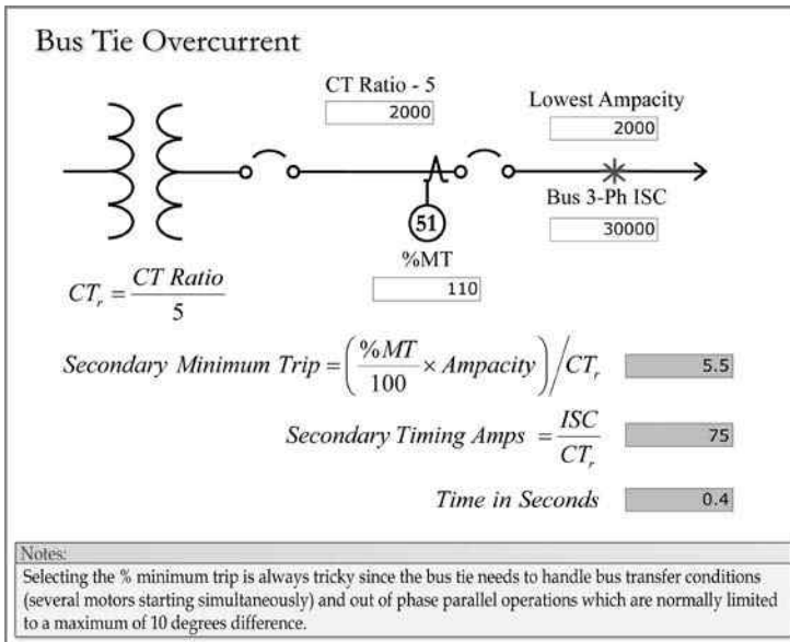
FIGURE 3.15 Bus tie overcurrent settings.
