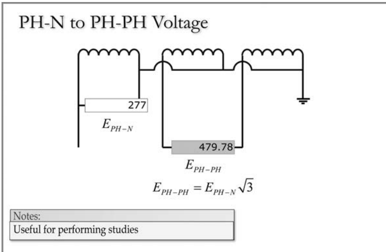
FIGURE 1.41 Phase-neutral to phase-phase.
