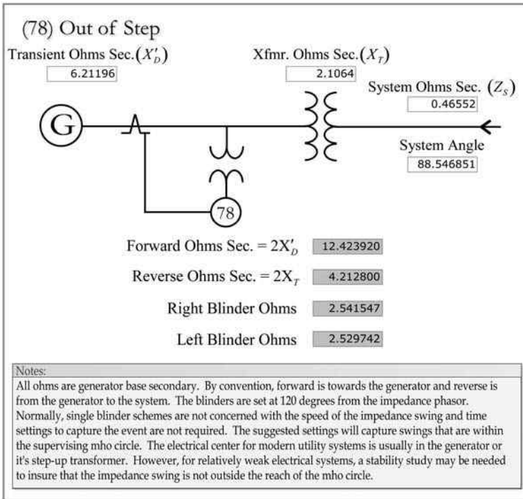
FIGURE 4.50 Out-of-step single blinder relay settings.
