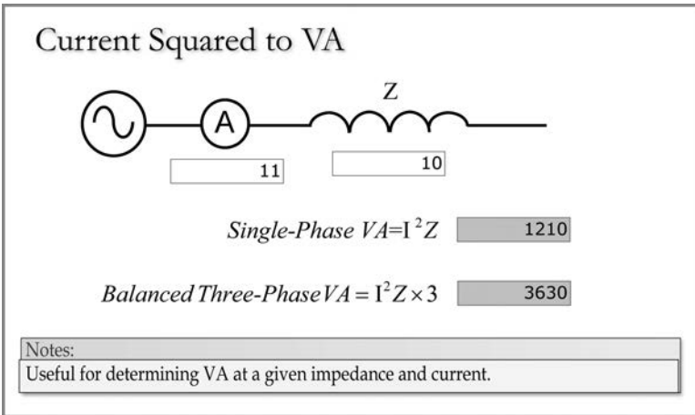
FIGURE 1.44 Current squared to VA.
