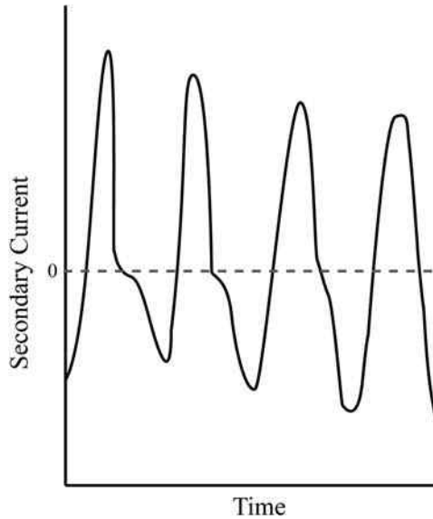
FIGURE 3.7 Saturated CT output waveform.
