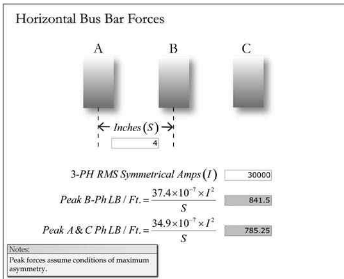
FIGURE 5.1 Horizontal bus bar forces.
