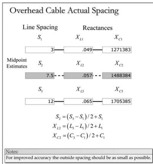
FIGURE 2.21 Roughly extrapolated conductor spacing impedance changes.
