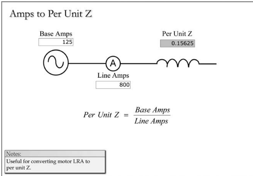
FIGURE 2.40 Amps to per-unit Z.
