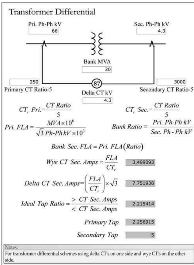
FIGURE 3.38 Transformer differential relay taps.
