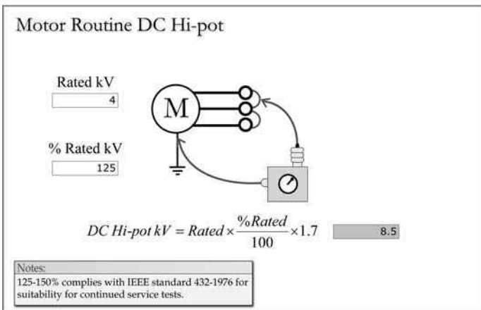
FIGURE 7.8 Motor DC routine test.
