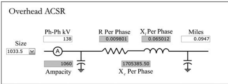
FIGURE 2.20 138-kV 1033.5 ACSR 12-foot spacing.
