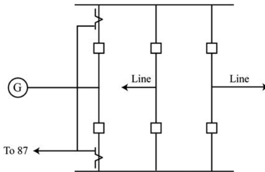
FIGURE 4.8 Double breaker double bus.
