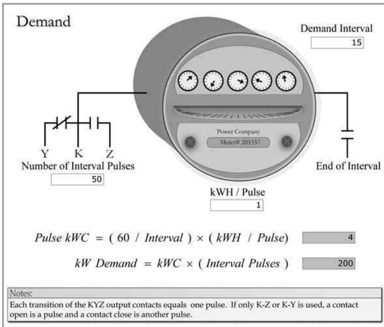
FIGURE 5.19 Watt demand.
