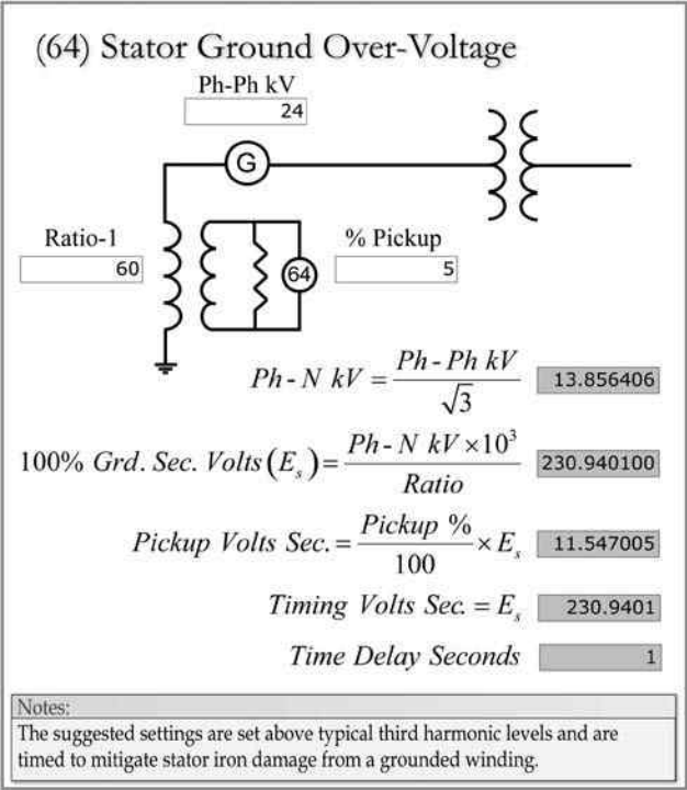
FIGURE 4.43 Conventional generator stator ground scheme protection.
