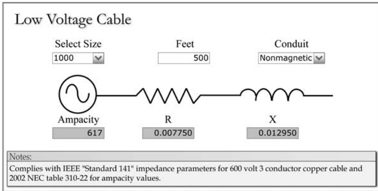
FIGURE 2.14 Low-voltage cable in a nonmagnetic conduit.
