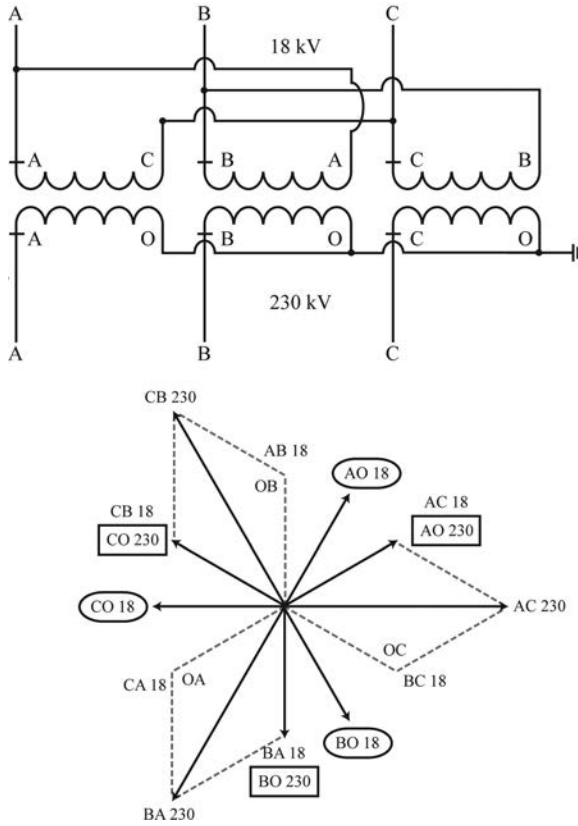
FIGURE 1.58 Delta-wye lagging connection.
