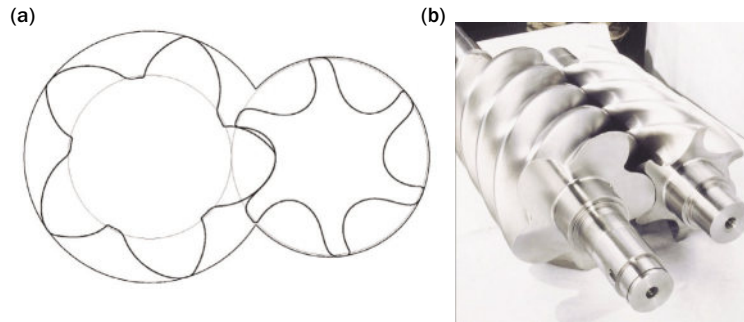
Figure 3.1 A pair of asymmetric rotors. (a) Schematic drawing, (b) finished parts. Left, male; right, female
