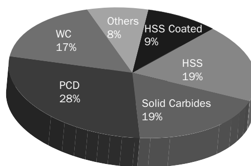
Figure 6.4 Tool materials used for drilling of MMCs
