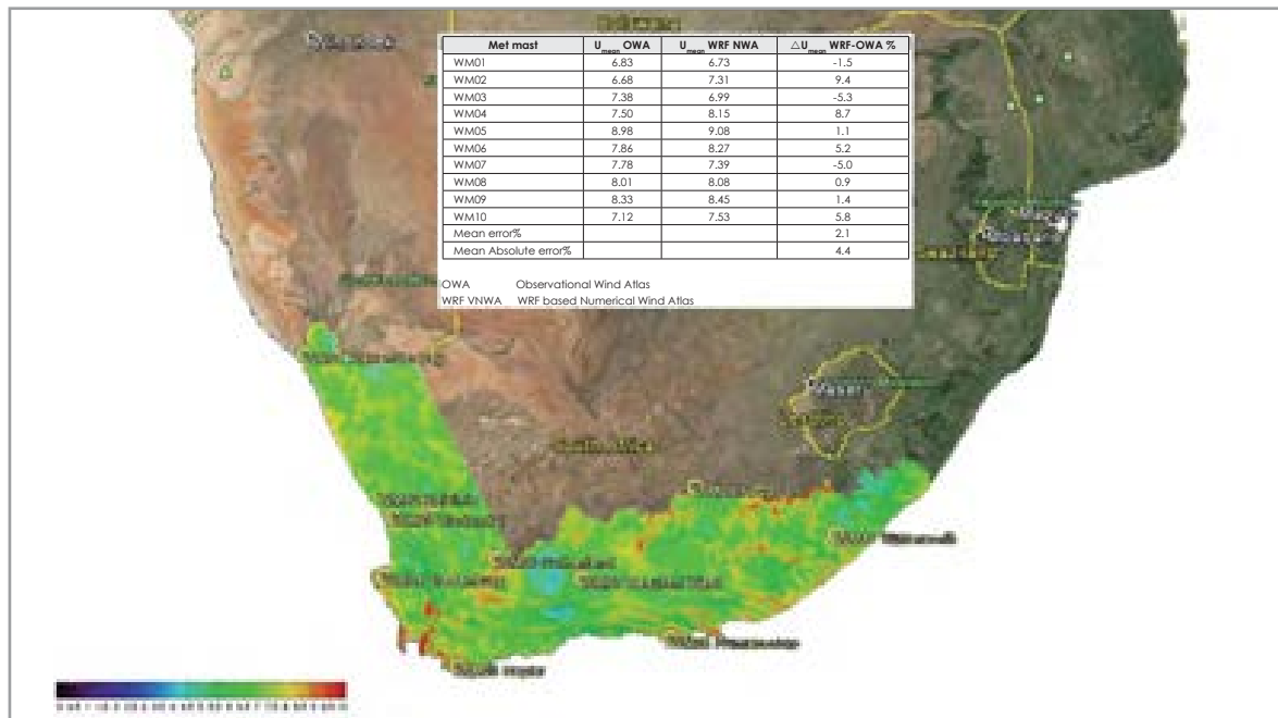
Figure 16: The first verified wind atlas over South Africa showing generalised wind speeds at 100 meters height (in \text{ms}^{-1} ). The location of measurement mast are show as yellow circles and the inset table indicates how closely the wind atlas results match the observational wind atlas developed at each mast
