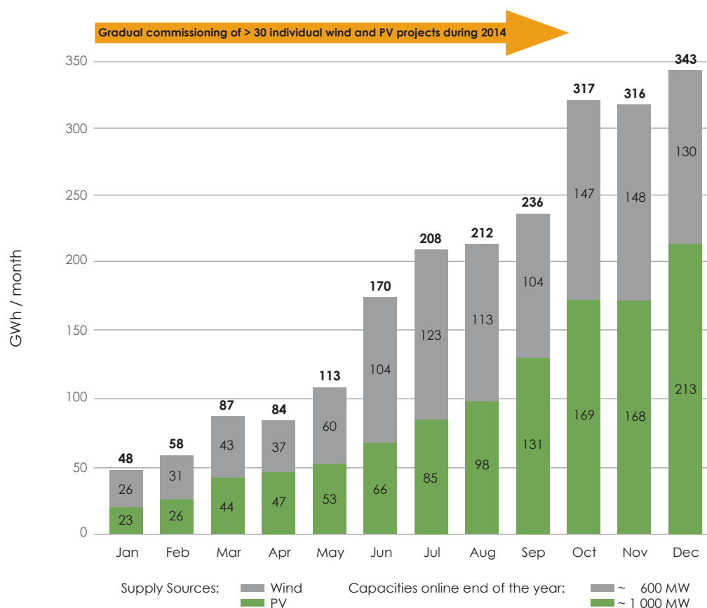
Figure 2: REIPP growth in energy produced during 2014 (Eskom, CSIR Energy Centre analysis)
