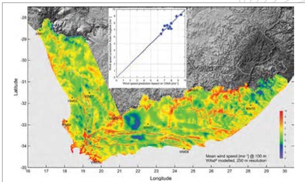
Figure 17: High-resolution wind resource map showing Mean wind speed ( \text{ms}^{-1} ) at 100m. The inserted graph show the accuracy of the NWA (vertical axis) against the observational wind atlas(horizontal axis) at each measurement mast
