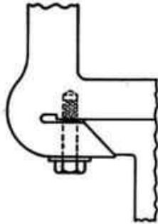
FIG. 211.—Clamping by spring dovetail.
