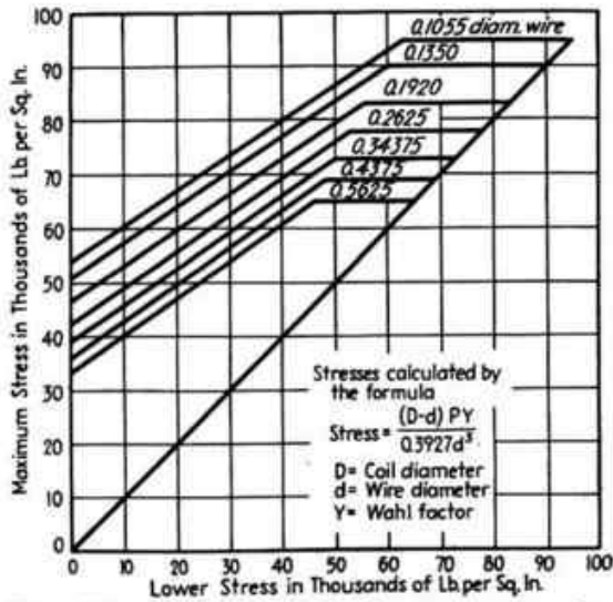
FIG. 249.—Allowable torsional stress range for Swedish steel wire.
