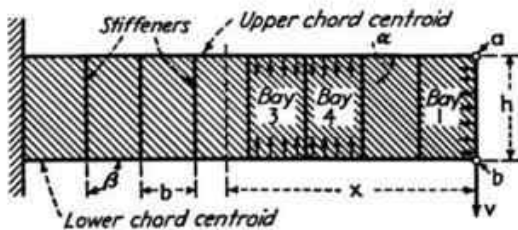
FIG. 8.—Diagonal lines represent the diagonal field tension in a thin web.
