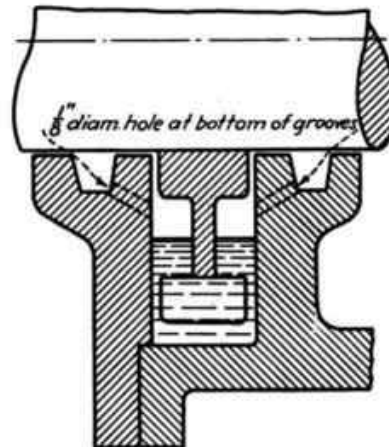
FIG. 317.—Illustrates the principle of the water seal.
