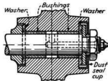
FIG. 347.—The labyrinth seal shown does not rely on nonmetallic materials but on the small clearances with the assembly. A steel washer contacting a bronze thrust washer is clamped against the shaft shoulder after the formed dust seal cup is pressed into the counterbored hole.
