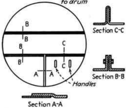
FOUR-SEGMENT DEMOUNTABLE TANK COVER
