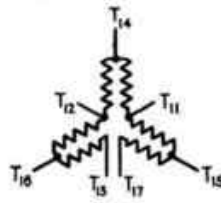
Two winding, four speed N.E.M.A. MG 6-41, Fig. 7, 1930
