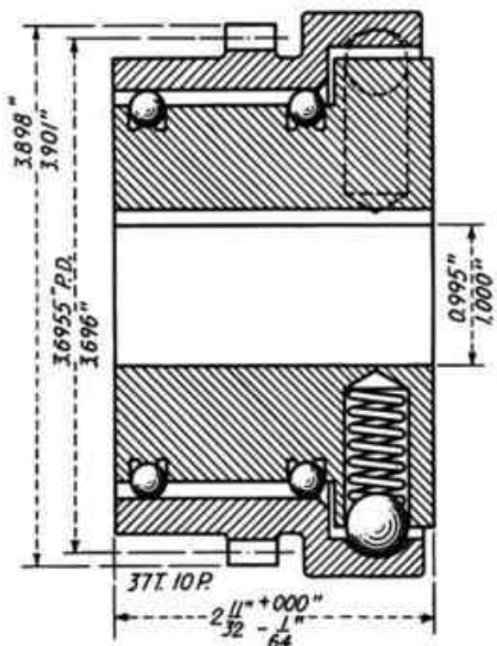
9 springs \frac{31}{64} " outside diameter 0.109" diam. wire Load = 1100 lb. per in. travel per turn Test = load 35 to 40 lb. on 20 in. radius lever FIG. 350.
