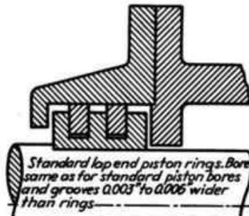
FIG. 312.—The common labyrinth shaft seal.
