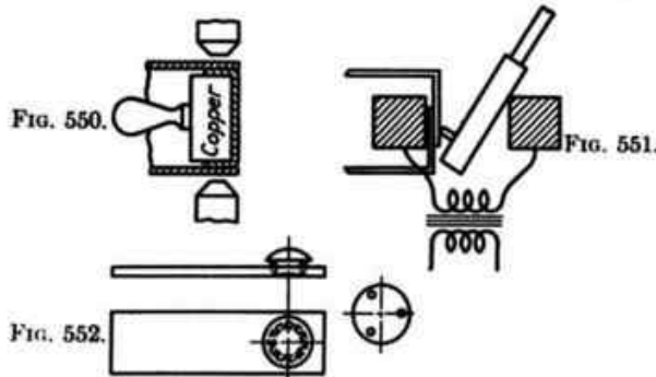
FIG. 550.—Welding both sides of a box form simultaneously, by employing a shunt-block device.
