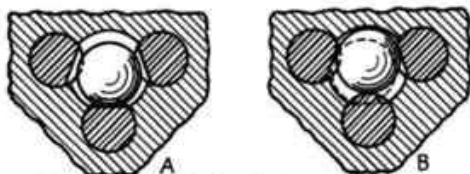
FIG. 81.—Without using a spring of any kind, three gear-shifting rods are locked by a large steel ball. At A , the neutral position is shown. At B , the lower rod has been shifted, forcing the ball upward, thereby locking the other two rods. The dashed circle shows the position of the ball when the right-hand rod has been shifted.
