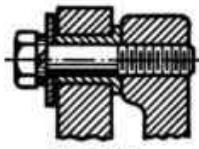
FIG. 135.—Shouldered bushing centered in counterbored hole. FIG. 136.—Bushing centered and held by stud screw.
