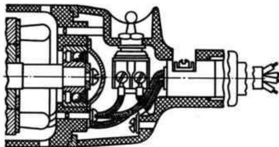
FIG. 499.—Latest design of switch arrangement for small die grinders and sanders. The toggle-operated switch unit is mounted in a dust-tight compartment and a dust seal is provided where the toggle comes through the case. This type of switch does not have a release arrangement that opens it automatically.
