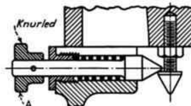
FIG. 74.—An adjustable gear cover lock. If the door is pushed shut, it is automatically latched, whereas pulling out the knurled knob A disengages the latch.
