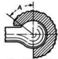
FIG. 154.—Toggle or pawl joint. Angle A should be 30 to 45 deg. to retain the member.
