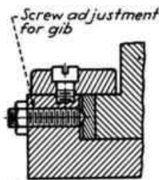
For light loads only FIG. 386.
