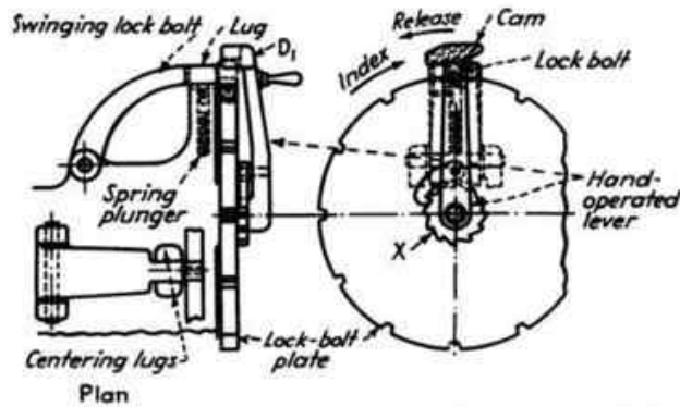
FIG. 207.—By using a lock-bolt plate larger than the work, the indexing error is diminished. The swinging lock bolt is released automatically by the spring plunger, which has a predetermined movement, when the hand-operated lever is moved to the left, as shown by the arrow marked Release, and the cam contacts the rounded top surface of the lock bolt. The ratchet is keyed with the lock-bolt plate to the spindle. As the lock bolt is released and the lever is rotated 30 deg. counterclockwise, the pawl engages the next tooth in the ratchet wheel at X. The lever is then pulled in the direction of the arrow marked Index, the cam moving the lock bolt downward into the next opening in the lock-bolt plate. The plan view of the bolt shows the two centering lugs between which the lock bolt is additionally supported.
