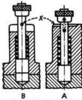
FIG. 69.—Driving plunger, shown in engagement at A , is pulled out and given a 90-deg. turn, pin X slipping into the shallow groove as shown at B , both members being thus disengaged.
