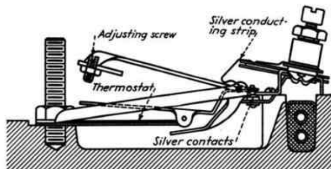
FIG. 515.—Electric irons require a convenient adjustment for the temperature at which the bimetal element opens the circuit. In the mechanism designed by Proctor & Schwartz, a double lever not only permits adjustment of the operating temperature, but also relieves the bimetal strip of any restriction when it cools to room temperature. Since the operating temperature range is high, a heat-resisting bimetal material is used in the form of a short stiff strip. Current is conducted to the bimetal contact through a flexible silver ribbon eliminating the effect of heat caused by current passing through the bimetal strip.
