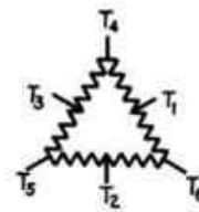
Single winding, two speed A.S.A. C-6 3.720, 1938
