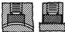
FIG. 174.—When a longer clamping surface is desired, a slot similar to a keyway is cut into the retaining member.
