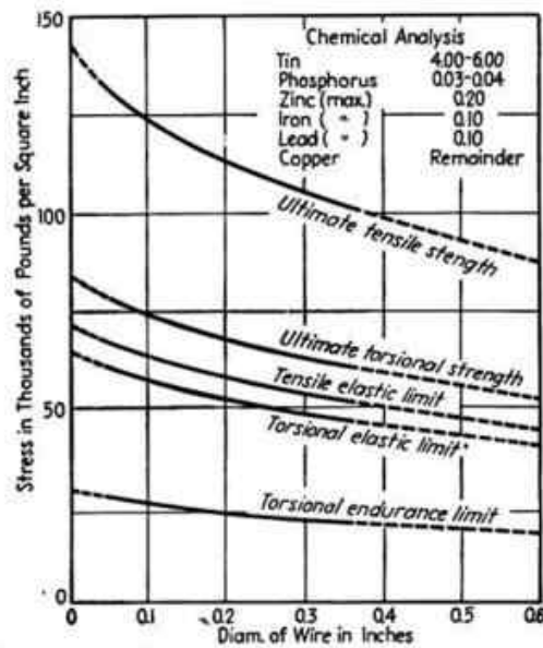
FIG. 247.—Phosphor bronze wire, S.A.E. 81. Relation of wire diameter to physical properties.
