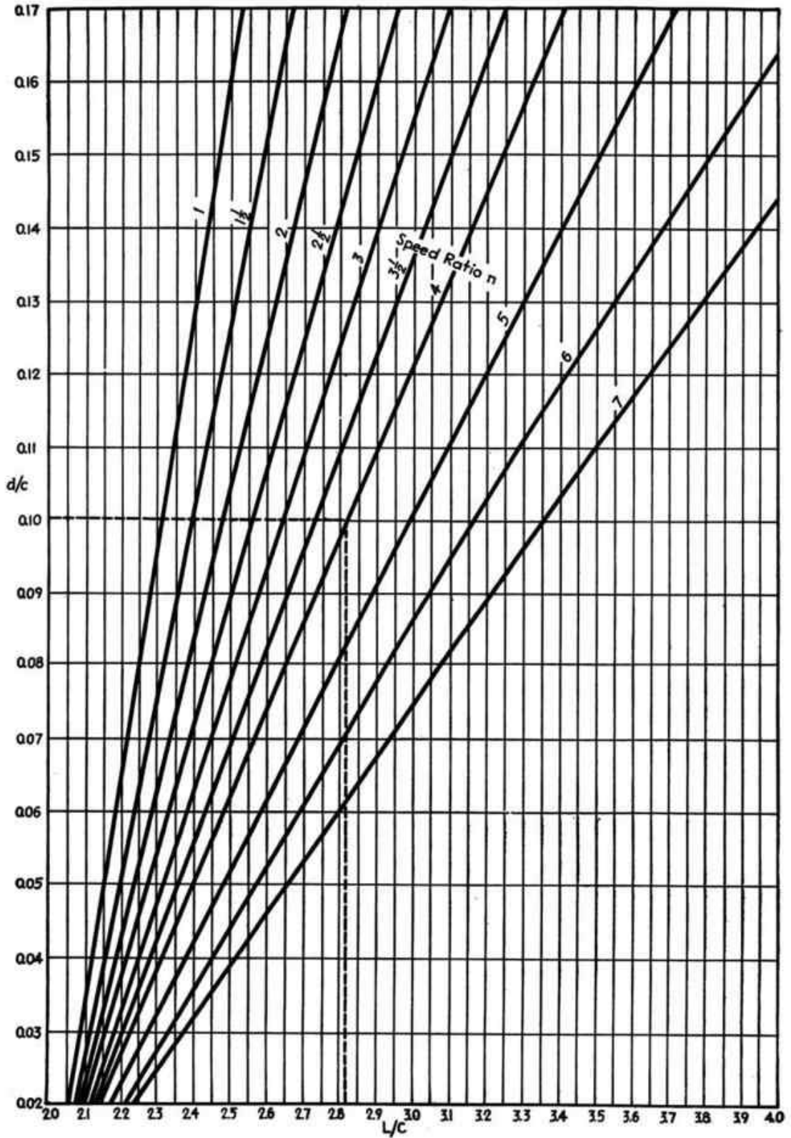
CHART FOR FLAT-BELT LENGTHS AND PULLEY DIAMETERS
