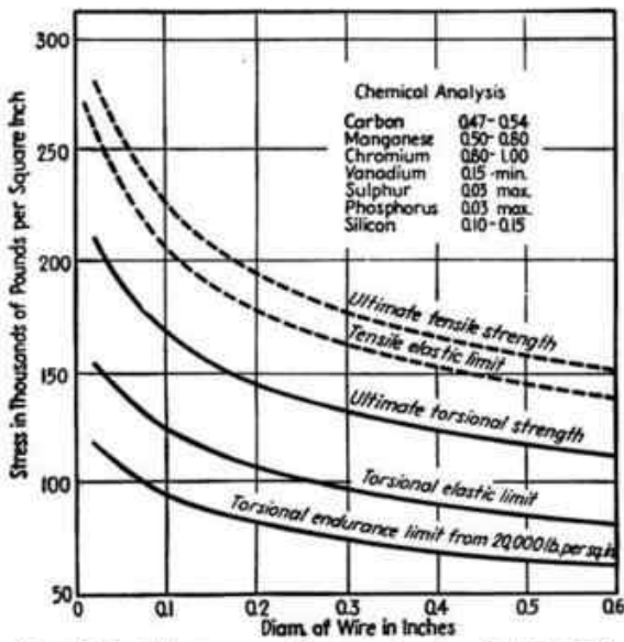
FIG. 245.—Chrome-vanadium-steel wire, S.A.E. 6150. Relation of wire diameter to physical properties.
