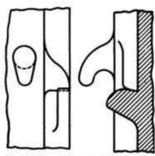
FIG. 241.—Plain gravity latch.
