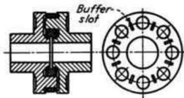
FIG. 267.—In this Brown Engineering Company coupling, flexibility is increased by addition of buffer slots in the laminated leather. These slots also aid in the absorption of shock loads and torsional vibration. Under parallel misalignment or shock loads, buffer slots will close over their entire width, but under angular misalignment, buffer slots will close only on one side.
