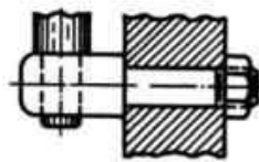
FIG. 146.—Another method of holding the steel lug.
