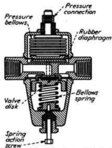
FIG. 517.—In a throttling type of circulating water control valve made by C. J. Tagliabue Manufacturing Company for use in refrigeration plants, the valve opening varies with the pressure on the bellows. This valve controls the rate of flow of the cooling water through the condenser, a greater amount of water being required when the temperature, and therefore the pressure, increases. The pressure in the condenser is transmitted through a pipe to the valve bellows thereby adjusting the flow of cooling water. The bronze bellows is protected from contact with the water by a rubber diaphragm.
