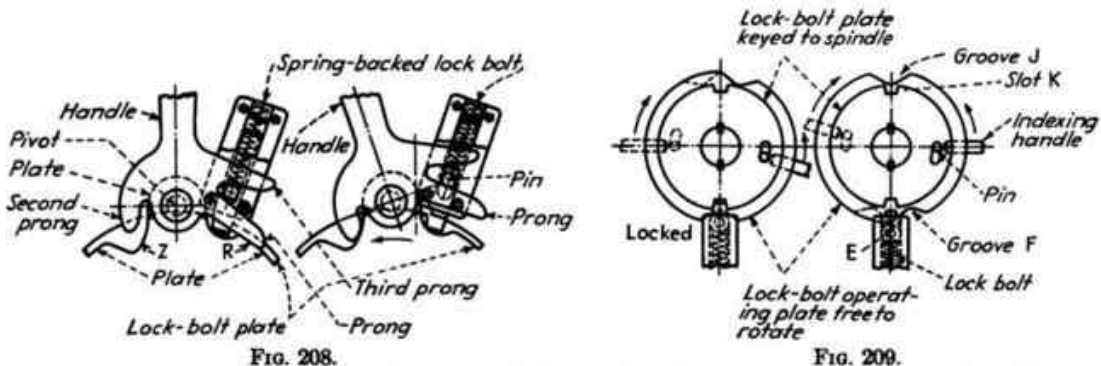
FIG. 208.—The handle is mounted on the plate and is independent of the lock-bolt plate. As the handle is pulled to the left, the prong pushes against the pin driven into the spring-backed lock bolt, thereby disengaging the bolt. At the same time, the second prong contacts the plate at Z. Both plates then move simultaneously, releasing the lock bolt, which rides on the periphery of the lock-bolt plate, and the bolt falls into the next slot. The handle is then pushed back again, clockwise, contacting the plate at R, upon which a third prong pushes against the pin-seating lock bolt in a locked position.
