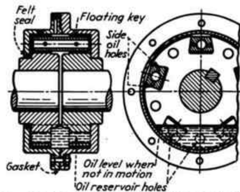
FIG. 292.—In the design of the W. H. Nicholson & Company flexible coupling, a series of floating steel keys slide in dovetail slots cut into each flange. The degree of misalignment compensated for depends on the clearance between the keys and slots. Wear is reduced, and cushioning is provided by operating keys in oil bath. Keys act noiselessly, centrifugal force keeping them against the slot surfaces.
