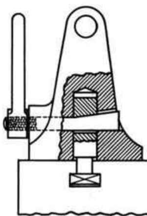
FIG. 216.—Example of wedge clamping.
