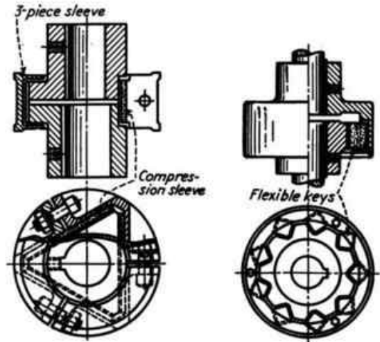
FIG. 290.—In this coupling of Falls Clutch & Machinery Company, two hubs with triangular heads and a three-piece sleeve are used. The sleeve is bolted together when assembling. Three pieces of compression lining provide the necessary flexibility. Misalignment is compensated for in all directions by compression of the linings.
