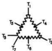
Two winding, four speed N.E.M.A. MG. 6-41, Fig. 8, 1930
