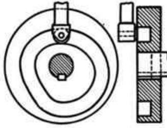
Face Cam
