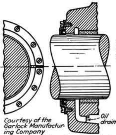
FIG. 347.—The labyrinth seal shown does not rely on nonmetallic materials but on the small clearances with the assembly. A steel washer contacting a bronze thrust washer is clamped against the shaft shoulder after the formed dust seal cup is pressed into the counterbored hole.
