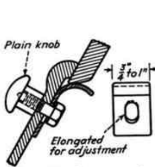
FIG. 224.—Snap-type fastener using a flat formed spring.
