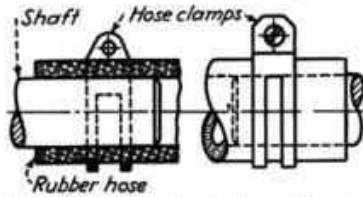
FIG. 255.—For applications where torque is low and slippage unimportant. It is easily assembled and disconnected without disturbing either machine element. It is adaptable to changes in longitudinal distance between machines. This coupling absorbs shocks, is not damaged by overloads, does not set up end thrusts, requires no lubrication, and compensates for both angular and offset misalignment.
