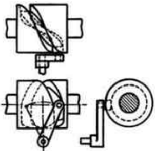
Cylindrical Cam with Swinging Follower
