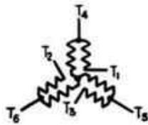
Single winding, two speed N.E.M.A. MG 6-41, Fig. 4, 1930
