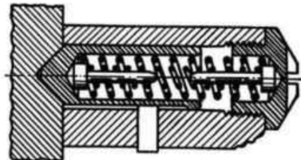
FIG. 94.—This design is similar to Fig. 88. When confined to a small diameter, a smaller spring is placed within the larger. By using a \frac{3}{16} in. outside diameter outer spring, 25 per cent spring tension can be gained by the addition of the inner spring. The larger one has a sliding fit in the plunger and screw plug holes. Two guide pins, the heads fitting closely into the larger spring, keep the inner spring central and free from buckling.
