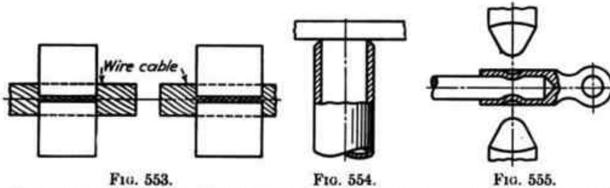
FIG. 553.—When wire cables are "cut" by clamping between the jaws of a welder and burning the cable in two, a globule of metal, formed on the ends, holds the wires together.
