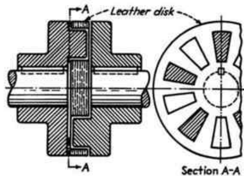
FIG. 273.—The principle of the T. B. Wood & Sons Company coupling is the same as Fig. 272, but the driving lugs are cast integrally with the metal flanges. The laminated leather disk is punched out to accommodate the metal driving lugs of each flange. This coupling has flexibility in all directions and does not require lubrication.
