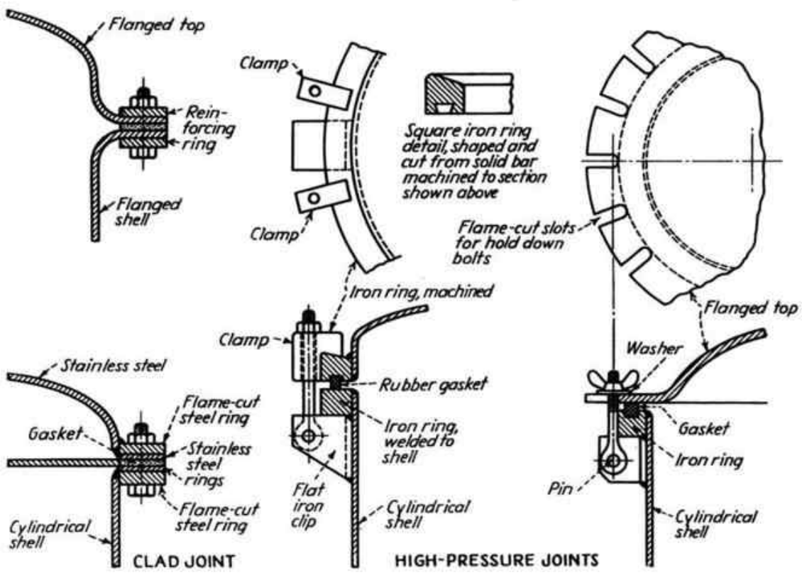
VARIOUS FORMS OF PRESSURE JOINTS
