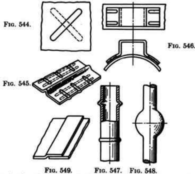
FIG. 544.—Elongated projections that cross each other are for the lightest gages and certain nonferrous combinations and where a good strong weld is imperative.
