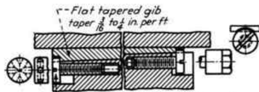
Adjustment and locking through screw engagement in counter-bored segment of gib FIG. 392.
