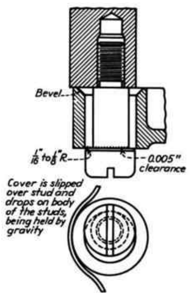
FIG. 242.—Positive type of gravity lock.
