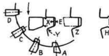
FIG. 197.—More accurate form of lock bolt, which is claimed by many to be the correct method for this type of design. The inclined surface gets the wear as it seats the the bolt, whereas the straight or radial side positions the bolt accurately. Positions A, B, C, and D correspond to those in Fig. 196, and indicate that the corners X and Y should be rounded. At H is shown how the groove is ground. Other notations are the same as given in Fig. 196.
