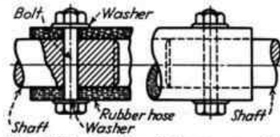
FIG. 256.—Positive drive is assured by bolting hose to shafts. This has the same advantages as the type in Fig. 255, except there is no over load protection other than the rupture of the hose.
