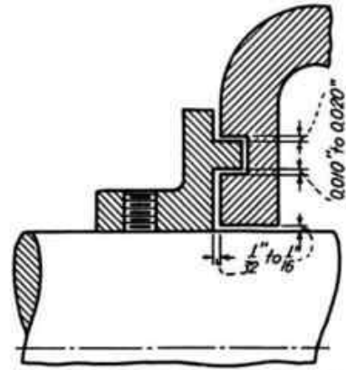
FIG. 307.—A simple design of labyrinth seal. Centrifugal force prevents the entrance of foreign particles while grease or oil lubricant on the shaft is thrown outward, thus filling the labyrinth opening.
