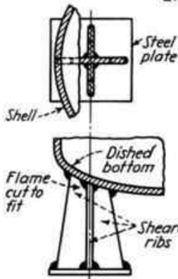
TANK SUPPORT
