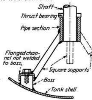
SHAFT SUPPORT
