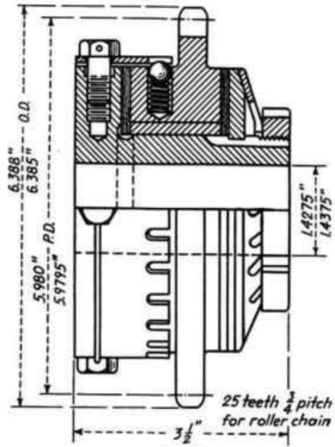
2 springs \frac{11}{32} " outside diameter 0.040" diam. wire Load = 26 lb. per in. travel per turn, for noise maker only Test = load 25 to 28 lb. on a 57 in. radius lever FIG. 351.
