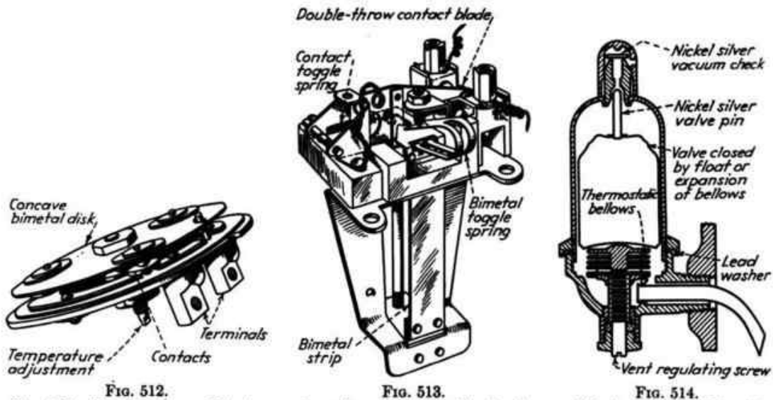
FIG. 512.—Toggle action, without separate springs, is obtained in the Spencer disk thermostat. The disk is a saucer-shaped piece of bimetal sheet which snaps itself from a concave to a convex shape at a predetermined temperature. Both the amount of movement and the temperature differential between opening and closing temperature depend on the design of the disk. For greater sensitivity, smaller differential and a larger movement than can be obtained with the plain disk, the bimetal disk is corrugated. Since the disk is small and stores but little heat, it warms or cools rapidly.
