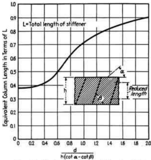
FIG. 7.—Equivalent free buckling length for tension field stiffeners is obtained by multiplying the total actual length by the factors from this curve.
