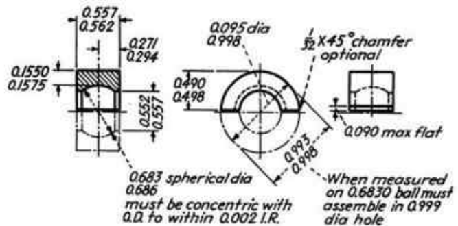
CLUTCH RELEASE SHAFT BEARING
