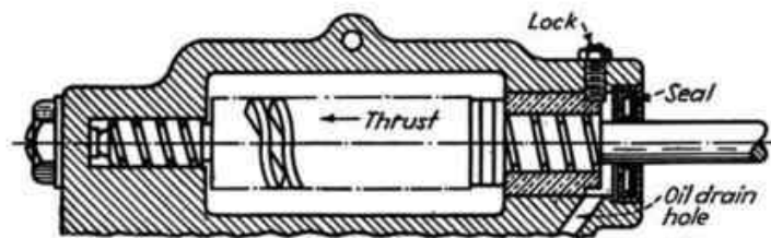
FIG. 349.—Another mounting of small worm-drive shaft for domestic washing machine and domestic stoker. The composition sealing material is held against the shaft by a V-formed spreader spring having serrated edges which nest into the sealing ring. The angle of the V in the spring is greater than the groove in the seal so that the fingers of the spring exert a light pressure on the sealing lip. An oil return hole is drilled outside the bearing to relieve built-up pressure against the seal.
