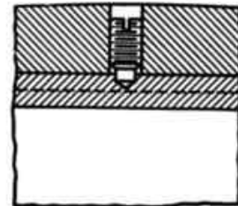
FIG. 185.—In this modified construction, the dog-point setscrew retains the key after the screw is loosened, the dog point fitting in the oversized hole in the key. This, of course, requires a key somewhat wider than the diameter of the dog point of the screw.
