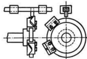
Dog Cam
