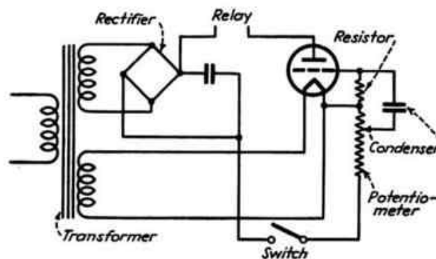
FIG. 485.—In the Westinghouse electronic relay, there is no temperature error, reset is instantaneous, adjustment is easy, and first cost is low. When the switch is closed, the tube passes current. As the current increases, the increasing IR drop from the potentiometer causes a charging current through condenser. The IR drop across the resistor because of this current applies the negative bias to the grid. Plate current cannot build up very rapidly, because the faster it increases, the more negative the grid becomes. After a time period, adjustable through potentiometer, the plate current will operate relay. The time delay is proportional to the product of resistance and capacitance. Long delays require large resistors, and short delays correspondingly small resistors. Maximum time delay with this device is about 3 min. About 0.05 sec. is the minimum.
