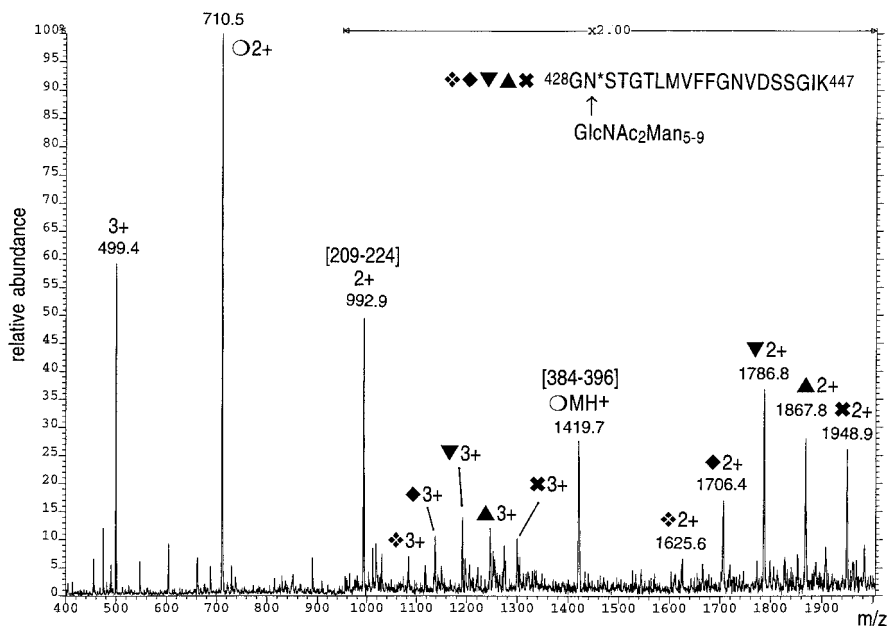
Fig. 3. Electrospray mass spectrum of the third glycopeptide-containing peak from the tryptic digest of the 73 kDa protein of rhFVIIIa ( Fig. 1 ). These data were acquired at normal cone voltage. Reprinted with permission from ref. 25 . Copyright (1997) American Chemical Society.
