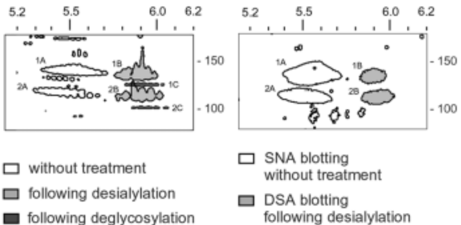
Fig. 2. 2DE analysis of the protein standard mixture following sialidase treatment or deglycosylation monitored by protein staining (silver staining) or lectin blotting. Lectin blotting of deglycosylated proteins is not shown since these do not contain lectin binding sites. The boxes within the figure encircle ceruloplasmin (1A/2A) following desialylation (1B/2B) and deglycosylation (1C/2C).
