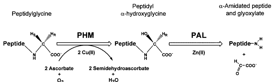
Fig. 2. Chemistry of α-amidation.
