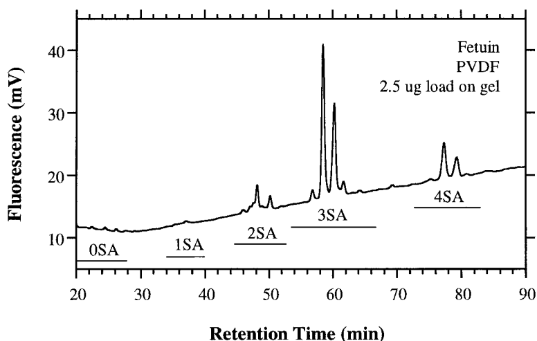
Fig. 2. Oligosaccharide map obtained with 2.5 \mu g of fetuin run on SDS-PAGE and electroblotted onto PVDF membrane. One of the three bands was used for PNGase F digestion (see Note 8 ).
