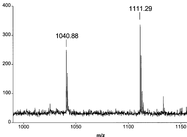
Fig. 4. Mass spectrum of sulfated shark gastrin-8 (see Fig. 3) obtained in the negative reflected mode. The peak at m/z 1111.29 represents the intact peptide (theoretical value 1112.36–1.01) while the peak at 1040.88 represents the in-flight desulfated peptide. The difference between the two is considerably less than the expected 80 (see Note 2). Note that the resolution is higher in the reflected mode than in the linear mode (Fig. 3).
