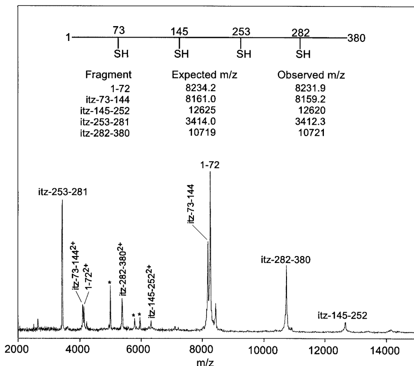
Fig. 2. MALDI spectrum of rabbit muscle creatine phosphokinase (MW. 42977), after cyanylation by CDAP and subsequent cleavage in 1 M \text{NH}_4\text{OH} solution. The peaks marked with asterisk are due to “carry-over” from an impurity in the sample. itz, iminothiazolidine derivative. Reproduced with permission from ref. 9 .
