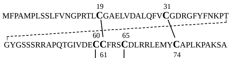
Scheme 2. Amino acid sequence and disulfide bond linkage of LR 3 IGF-I.
