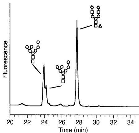
Fig. 6. Rechromatography of N-glycans using RP18-HPLC. The resulted glycan fraction from \text{NH}_2 -HPLC ( Fig. 5 , fraction marked with an asterisk) was rechromatographed on RP-18-HPLC. Mass spectrometry revealed the presence of a biantennary and two isomers of high mannose-sugars (Man7). Glycan key: \circ = mannose, \square = N-acetylglucosamine, \diamond = galactose, \triangle = fucose.
