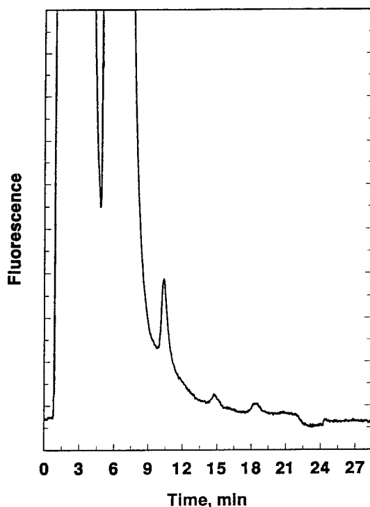
Fig. 3. HPLC chromatogram of an acid hydrolysate of wild-type recombinant protein C after OPA-derivatization. A quantity of 50 \mu g of protein was hydrolyzed with 6 N HCl at 110°C for 20 h, and 5 \mu L, corresponding to 5 \mu g of protein, was applied to the column under the conditions of Fig 1 . The peak at approx 11 min represents Hya.
