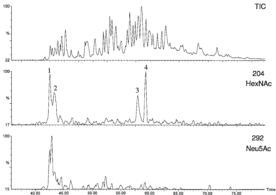
Fig. 1. Total ion chromatogram and selected ion chromatograms of diagnostic carbohydrate ions, m/z 292 (Neu5Ac) and 204 (HexNAc), acquired during high cone voltage LC/ESIMS analysis of a tryptic digest of the 73 kDa protein of rhFVIIIa. Reprinted with permission from ref. 25 . Copyright (1997) American Chemical Society.
