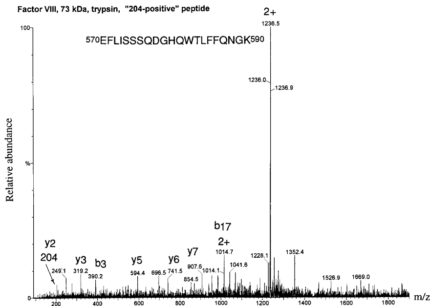
Fig. 4. Electrospray mass spectrum of the last 204-positive peak from the tryptic digest of the 73 kDa protein of rhFVIIIa (peak 4 in Fig. 1 ). These data were acquired at high cone voltage. Peptide fragments are labeled according to Biemann (31). All peptides with Gly-Lys C-terminus may yield a y_2 ion at m/z 204.
