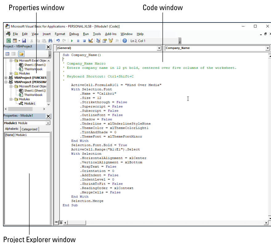
FIGURE 2-1: The Visual Basic Editor window as it normally appears when editing a macro.
