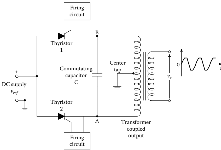
FIGURE 7.34 A single-phase inverter circuit for frequency control.
