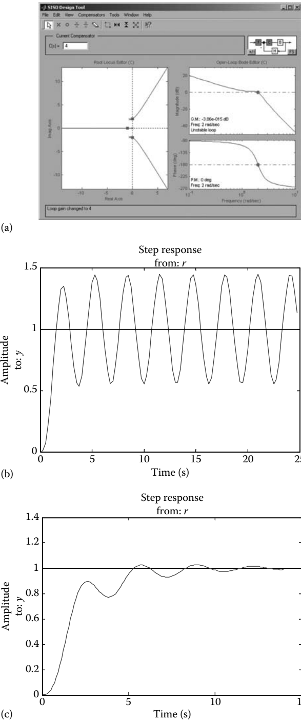
FIGURE D.3 (a) Root locus and Bode plots of the system with proportional gain K_p=4 ; (b) step response of the closed-loop system with K_p=4 ; (c) step response of the closed-loop system with K_p=2 .
