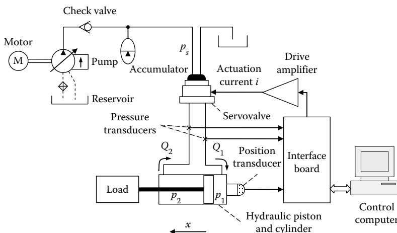
FIGURE 7.53 A computer-controlled hydraulic system.
