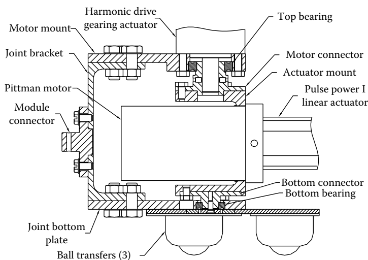
FIGURE 10.7 Details of a revolute joint.
