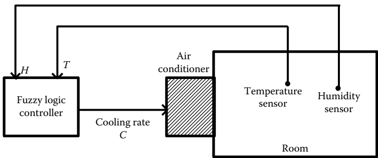
FIGURE 9.24 Comfort control system of a room.
