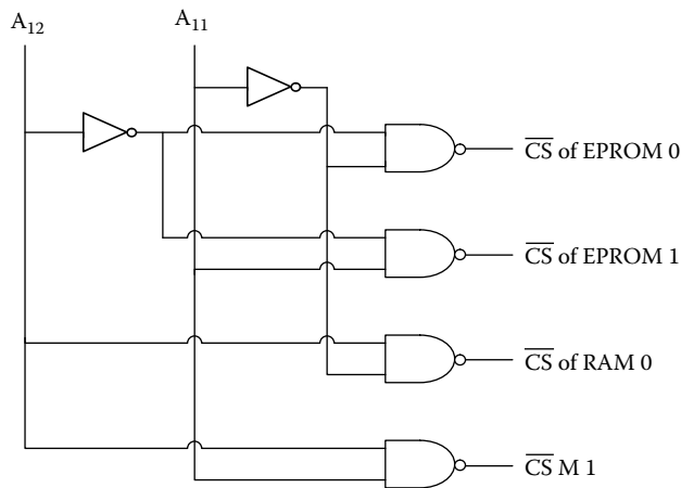
FIGURE 8.27 A 2 to 4 decoder for chip selection.
