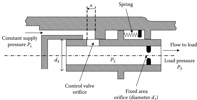
FIGURE P7.56 A flow control valve.
