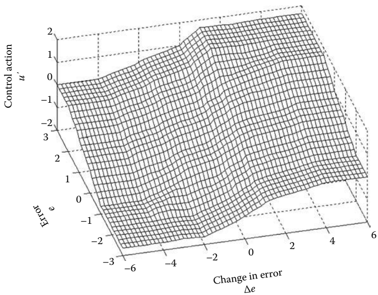
FIGURE 9.28 Control surface with a=1 , b=2 , and c=0.5 .
