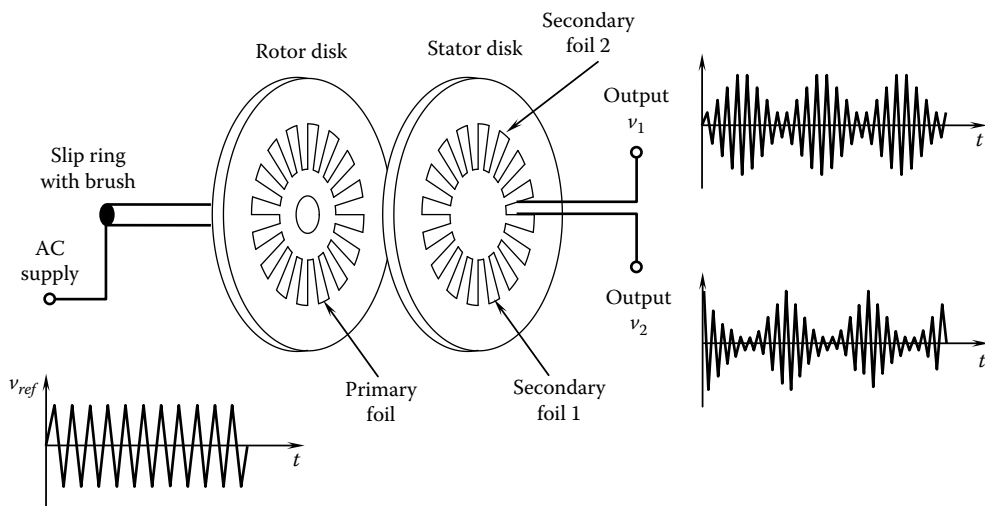
FIGURE 6.53 Schematic diagram of a digital resolver.
