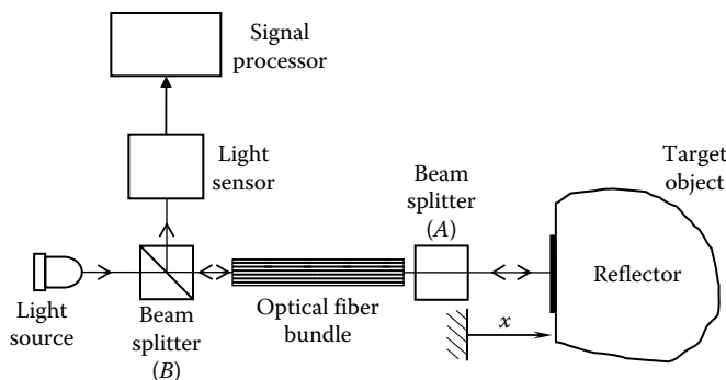
FIGURE 6.38 Laser interferometer position sensor.
