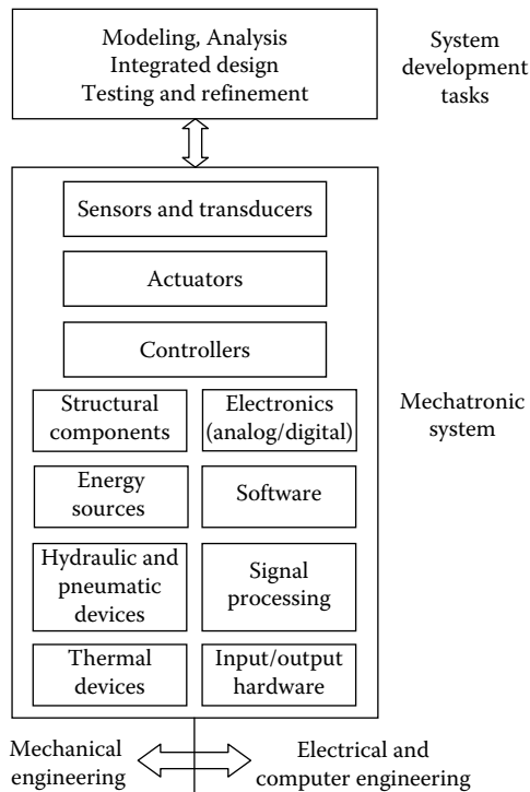
FIGURE 1.4 Concepts and technologies of a mechatronic system.
