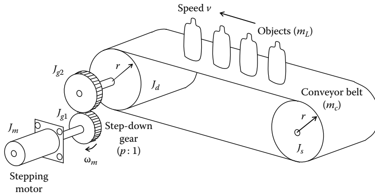
FIGURE 7.12 Conveyor unit with intermittent motion.
