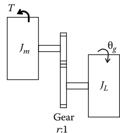
FIGURE P2.8 An inertial load driven by a motor through a gear transmission.
