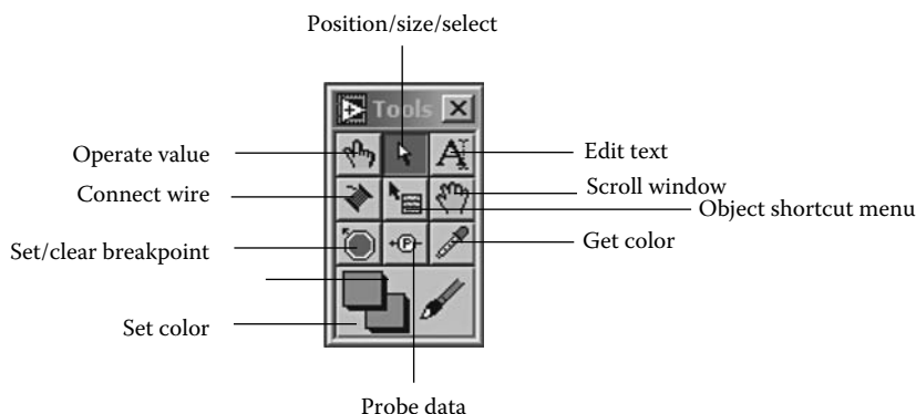
FIGURE D.9 LabVIEW tools palette.
