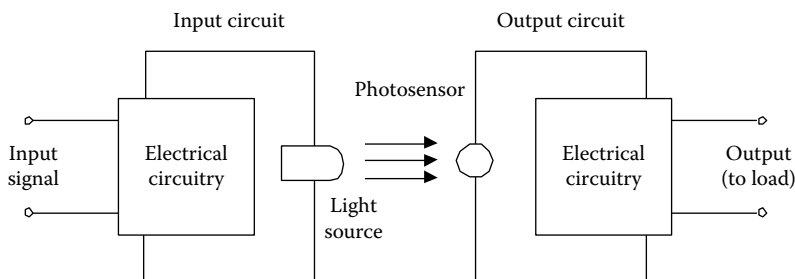
FIGURE 2.35 An optically coupled device.
