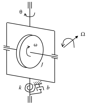
FIGURE P6.32 A rate gyro speed sensor.
