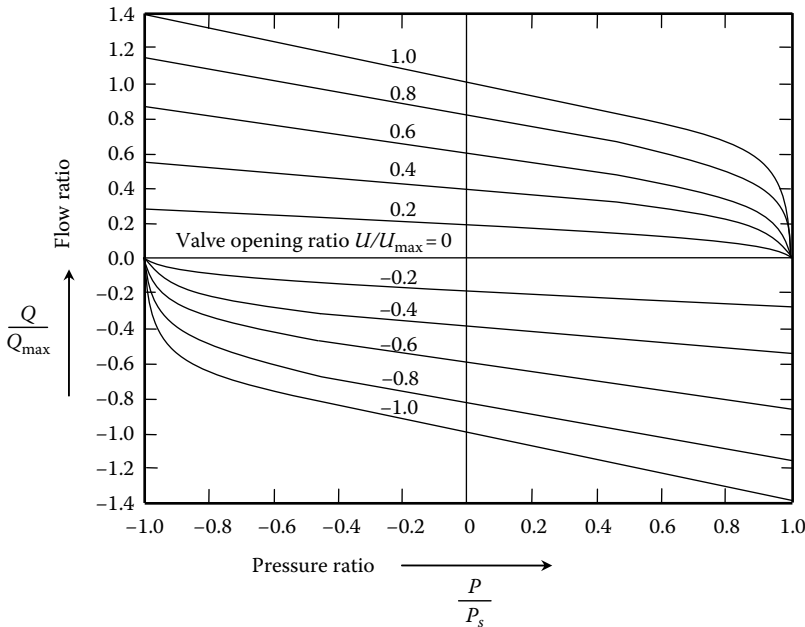
FIGURE 7.46 Steady-state characteristics of a four-way spool valve.
