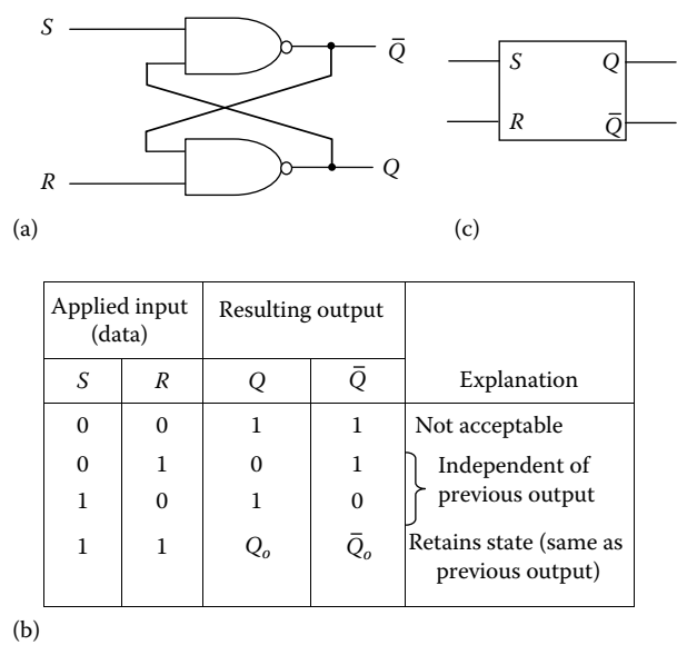
FIGURE 8.13 RS flip-flop formed by using NAND gates: (a) logic circuit, (b) truth table, (c) ANSI symbol.
