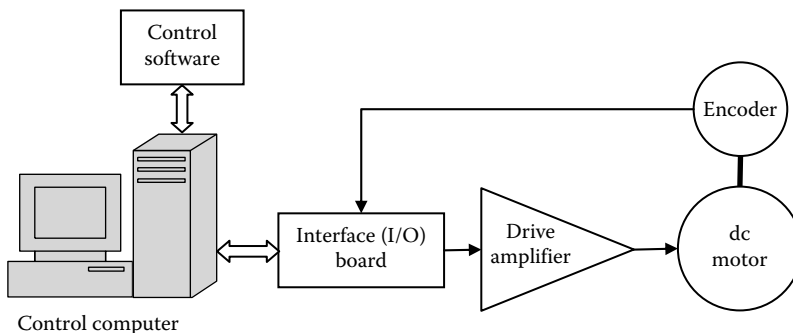
FIGURE 7.23 Components of a dc motor control system.
