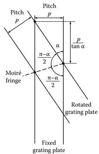
FIGURE 6.60 The orientation of Moiré fringes.
