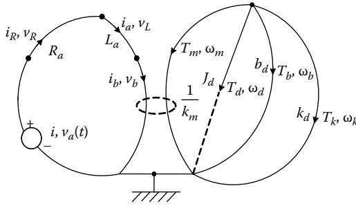
FIGURE 3.25 The complete linear graph of the system.
