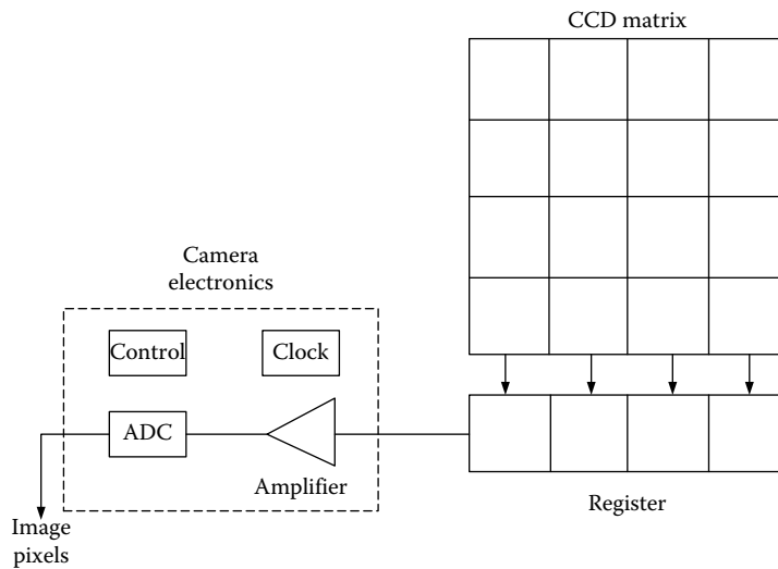
FIGURE 6.63 Digital image generation by a CCD camera.
