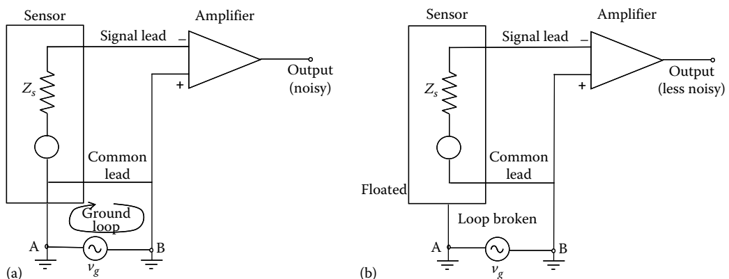
FIGURE 4.11 (a) Illustration of a ground loop. (b) Device isolation to eliminate ground loops (an example of internal isolation).
