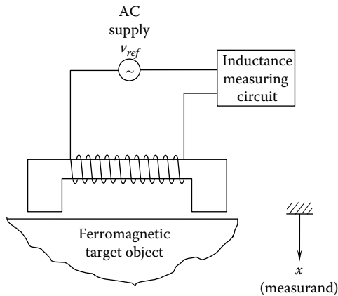
FIGURE 6.11 Schematic diagram of a self-induction proximity sensor.
