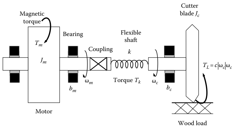
FIGURE P3.16 A wood cutting machine.
