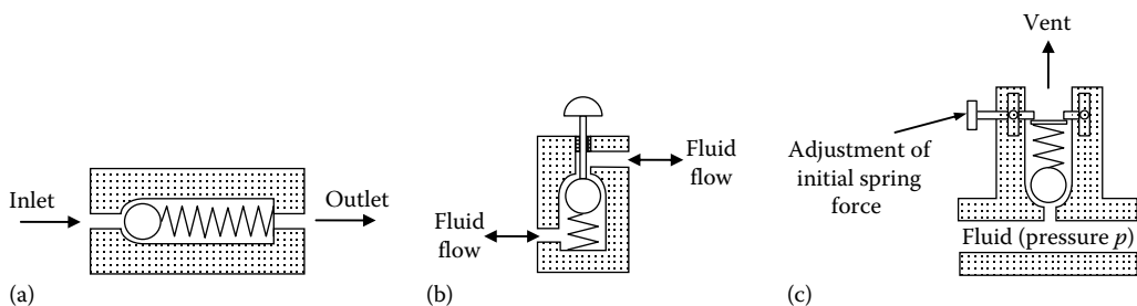
FIGURE 7.44 (a) A check valve (directional valve); (b) a poppet valve (an on/off valve); (c) a relief valve (a pressure regulating valve).
