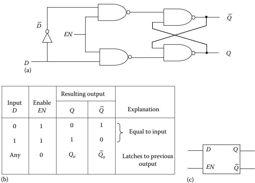
FIGURE 8.14 A latch circuit formed using an RS flip-flop and NAND gates: (a) logic circuit, (b) truth table, (c) symbol.
