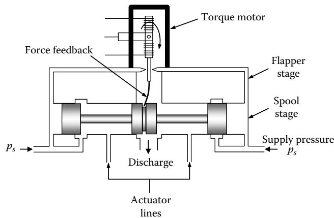
FIGURE 7.58 A two-stage servovalve with pressure feedback.
