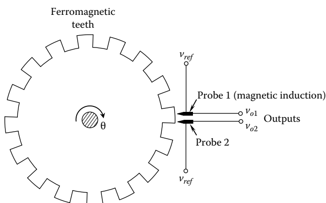
FIGURE 6.54 Schematic diagram of a pulse tachometer.
