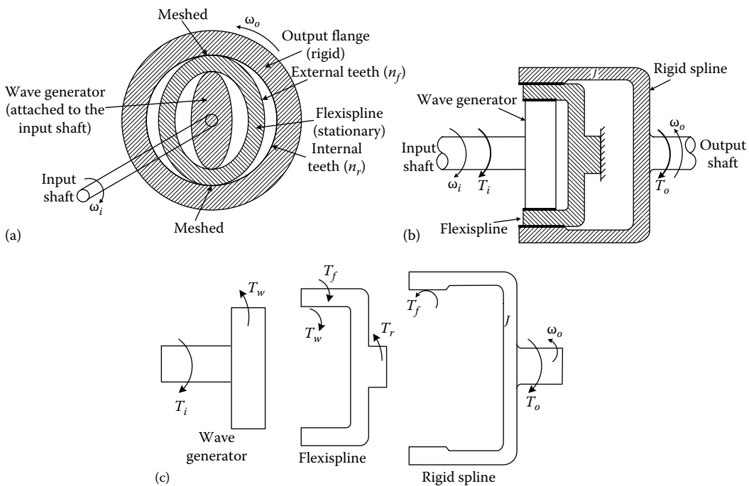
FIGURE 2.14 (a) An alternative design of harmonic drive; (b) torque and speed transmission of the harmonic drive; (c) free-body diagrams.
