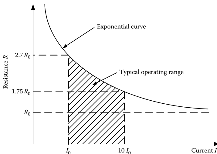
FIGURE 5.11 Characteristic curve of the sensor.
