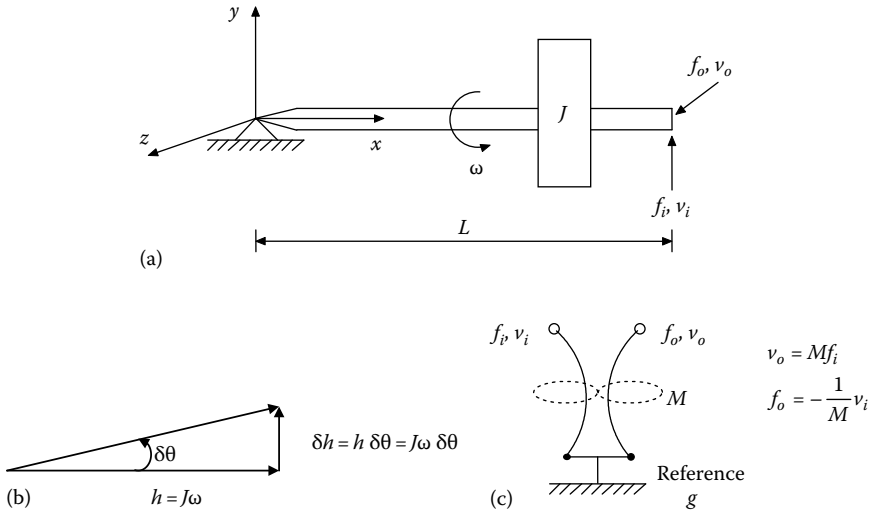
FIGURE 3.19 (a) Gyroscopic (gyroscope or spinning top)—a two-port element; (b) derivation of the constitutive equations; (c) linear graph representation.
