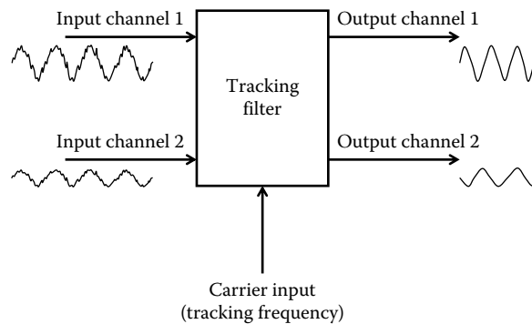
FIGURE 4.13 Schematic representation of a two-channel tracking filter.
