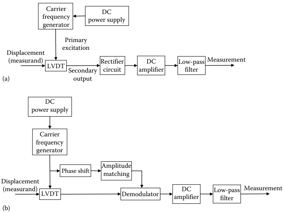
FIGURE 6.7 Signal-conditioning methods for a differential transformer: (a) Rectification; (b) demodulation.
