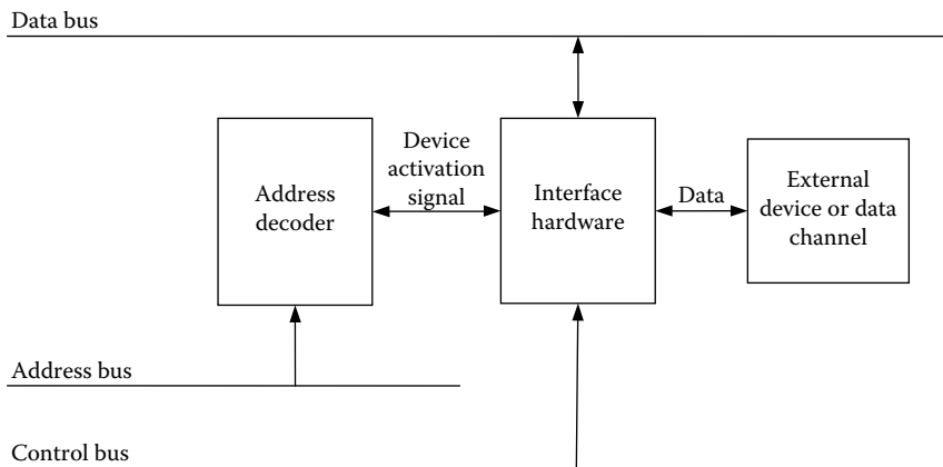
FIGURE 8.29 Memory-mapped I/O.
