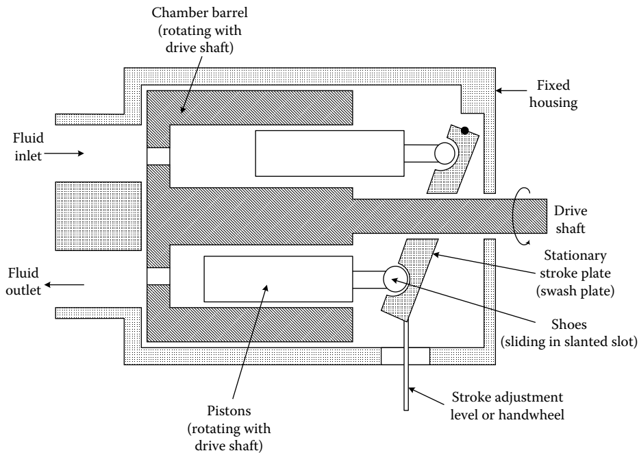
FIGURE 7.43 An axial piston hydraulic pump.
