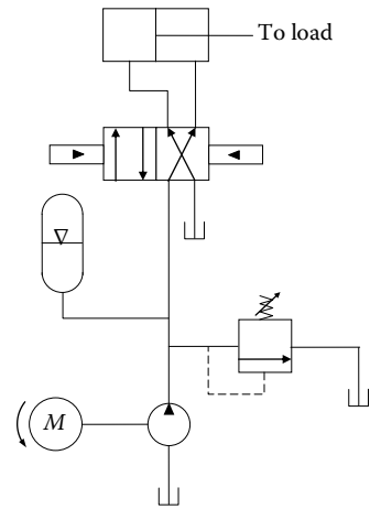
FIGURE P7.55 A hydraulic circuit diagram.
