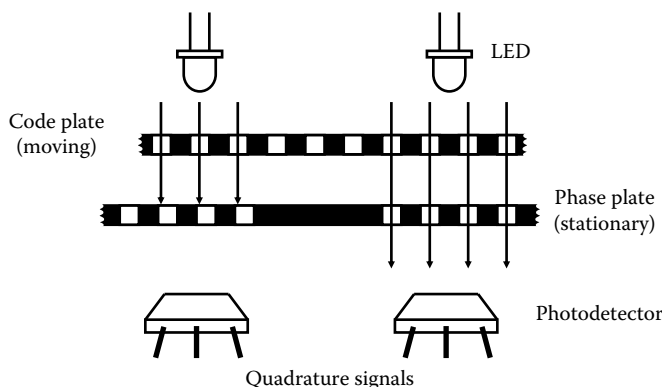
FIGURE 6.57 A rectilinear optical encoder.
