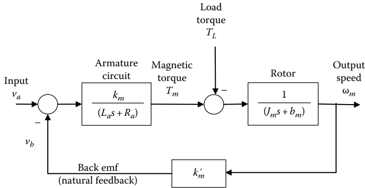
FIGURE 7.19 Open-loop block diagram for an armature-controlled dc motor.
