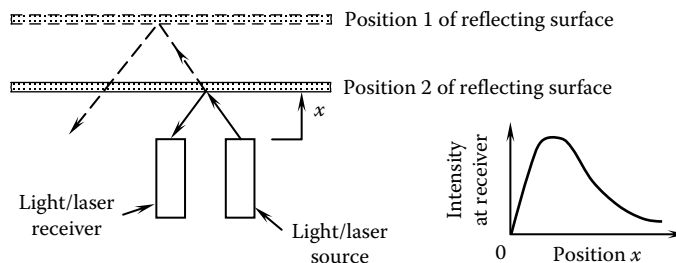
FIGURE 6.37 The principle of a fiber-optic proximity sensor.
