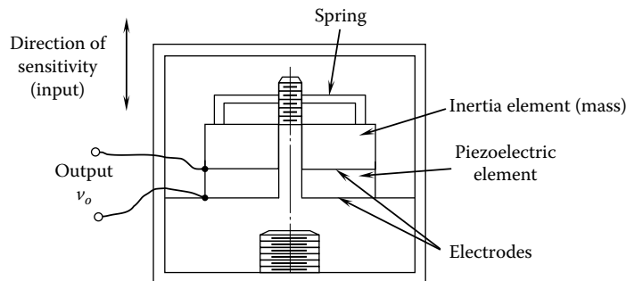
FIGURE 6.19 A compression-type piezoelectric accelerometer.
