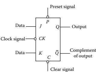
FIGURE 8.15 The symbol of a JK flip-flop.
