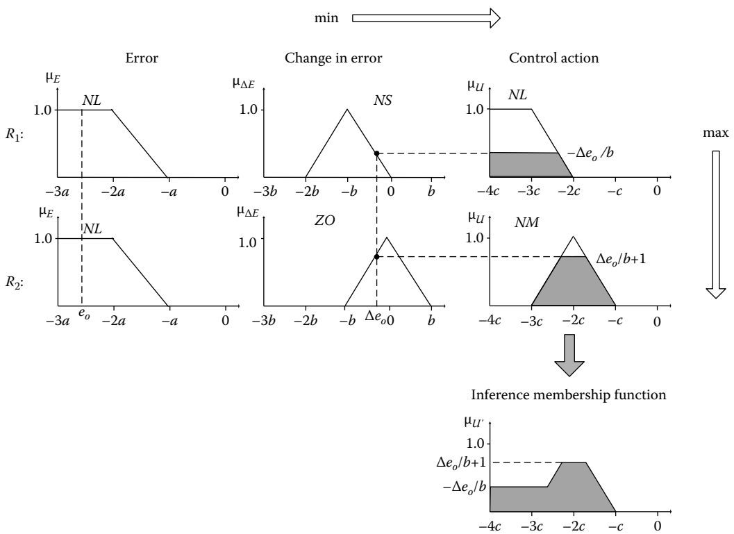
FIGURE 9.27 Individual rule-based inference for e_o[-3a, -2a] and \Delta e_o[-b/2, 0] .
