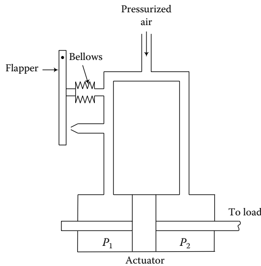
FIGURE 7.59 External pressure feedback for a flapper valve, using a bellows.
