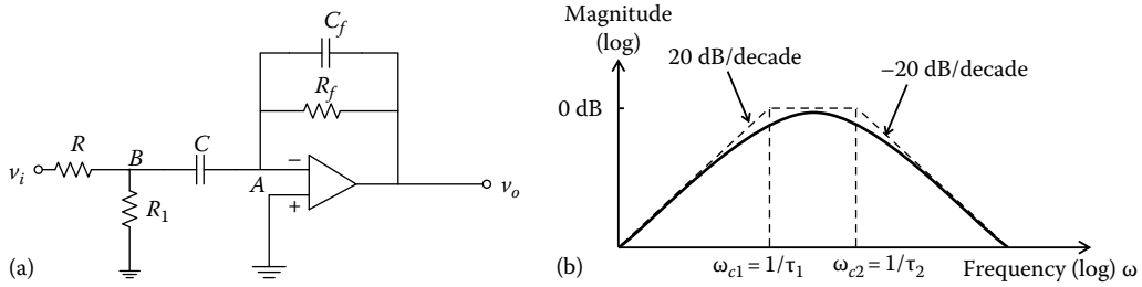
FIGURE 4.17 (a) A band-pass filter. (b) Frequency-response characteristic.
