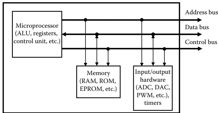
FIGURE 8.21 Typical architecture of a microcontroller.
