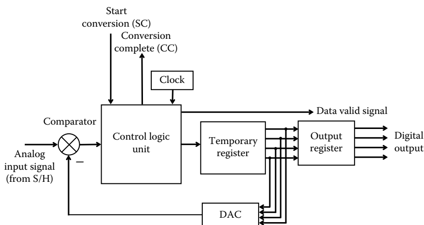
FIGURE 4.27 Successive approximation ADC.
