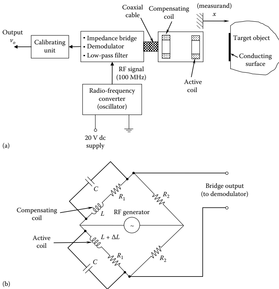
FIGURE 6.12 Eddy current proximity sensor: (a) Schematic diagram; (b) impedance bridge.
