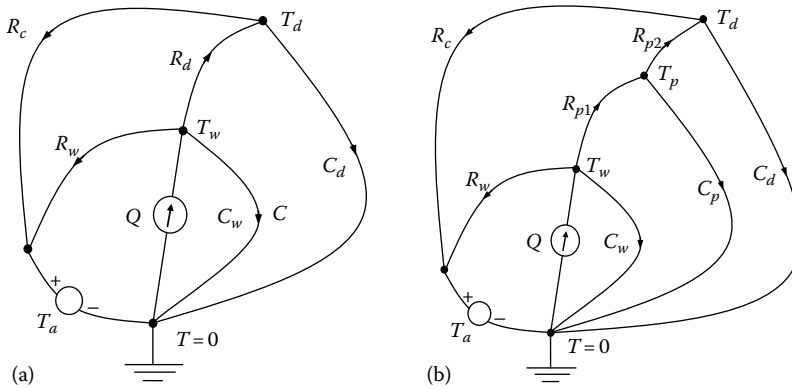
FIGURE 3.27 Linear graph of the: (a) simplified model; (b) improved model.
