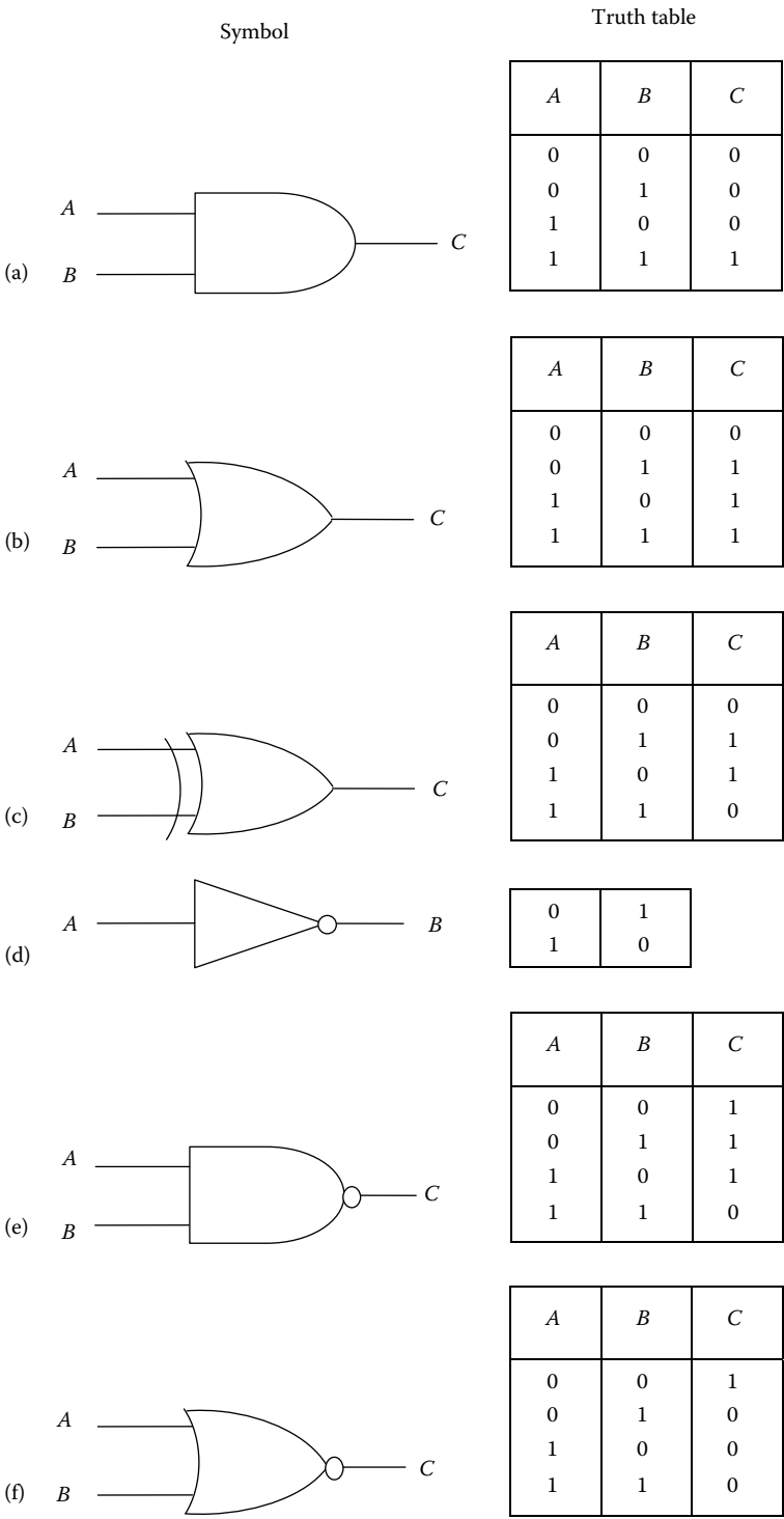
FIGURE 8.3 ANSI symbols and truth tables for the six basic logic gates: (a) AND, (b) OR, (c) XOR, (d) NOT, (e) NAND, (f) NOR.
