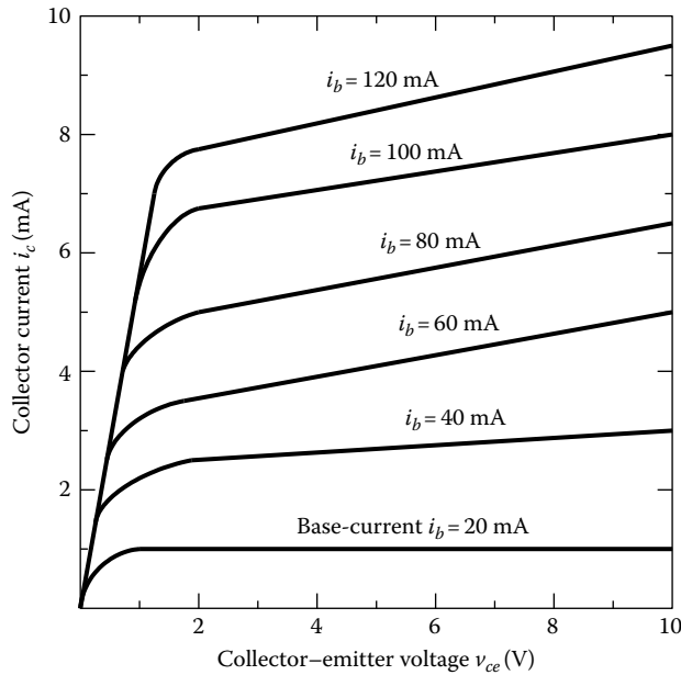
FIGURE 2.24 Characteristic curves of a common emitter BJT.
