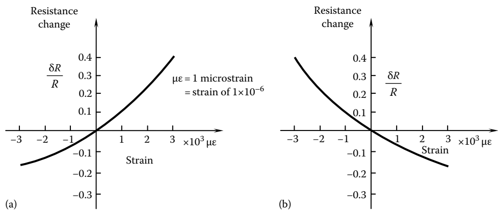
FIGURE 6.26 Nonlinear behavior of a semiconductor (silicon–boron) strain gage: (a) A p -type gage; (b) an n -type gage.
