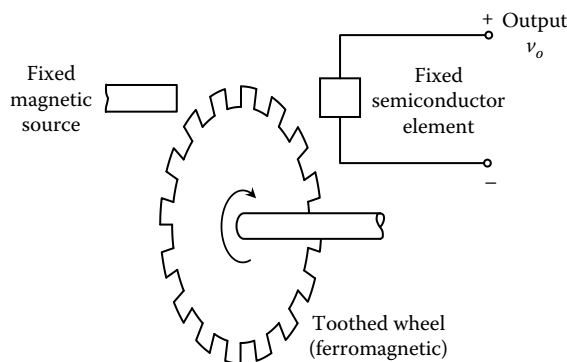
FIGURE 6.56 A Hall effect shaft encoder or digital tachometer.
