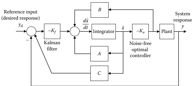
FIGURE 9.20 Linear quadratic Gaussian (LQG) control.
