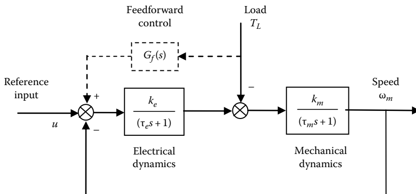
FIGURE P9.8 Control block diagram of a dc motor.
