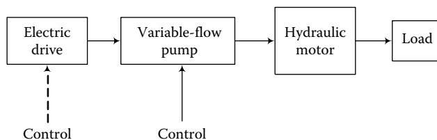
FIGURE 7.56 Configuration of a pump-controlled hydraulic drive system.
