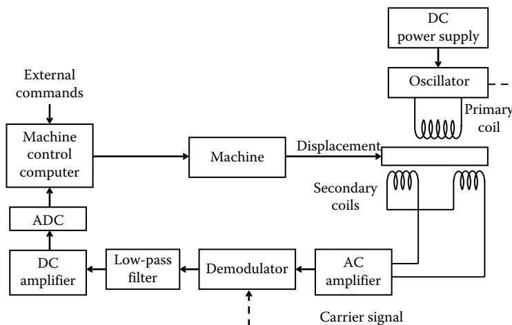
FIGURE P4.19 Components of an LVDT-based machine control loop.
