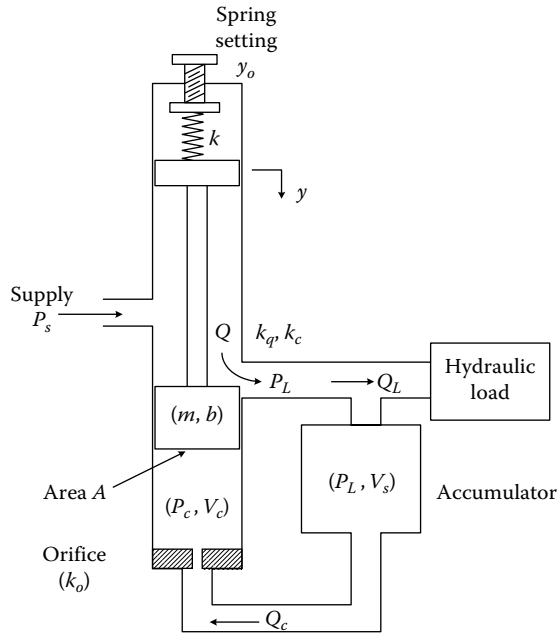
FIGURE 7.51 A single-stage pressure control valve.
