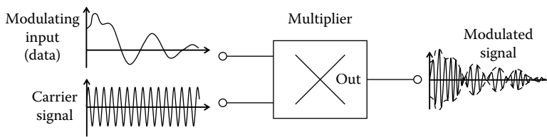
FIGURE 4.21 Representation of an amplitude modulator.
