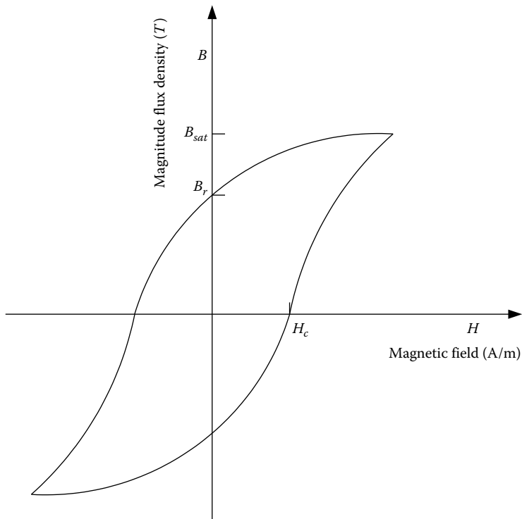
FIGURE 2.17 Hysteresis curve (magnetization curve) of a magnetic material.
