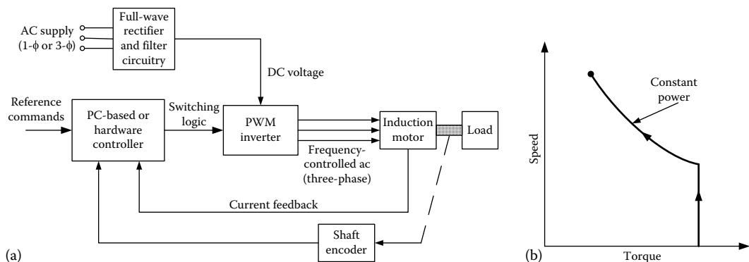
FIGURE 7.35 (a) Variable-frequency control of an induction motor; (b) a typical control strategy.
