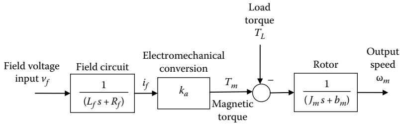
FIGURE 7.20 Open-loop block diagram for a field-controlled dc motor.
