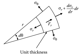
FIGURE A.1 An element of the rotating cylinder.
