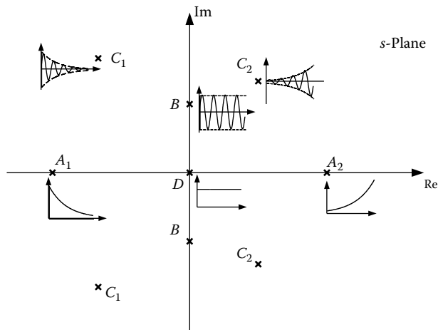
FIGURE 9.11 Pole location on the s-plane and the corresponding response.
