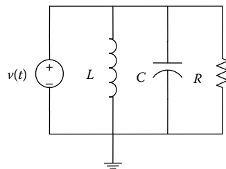
FIGURE P3.18 An L-C-R circuit.
