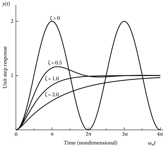
FIGURE 3.37 Step response of a damped oscillator.
