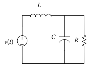
FIGURE P3.21 An electrical circuit.
