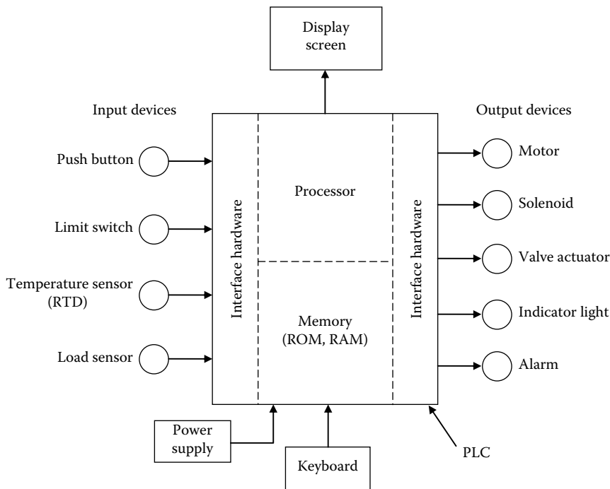
FIGURE 9.3 Schematic representation of a PLC.
