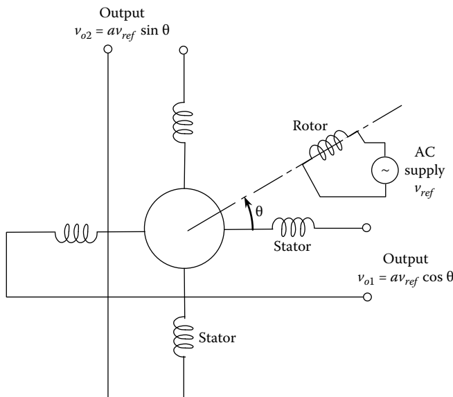
FIGURE 6.10 Schematic diagram of a resolver.
