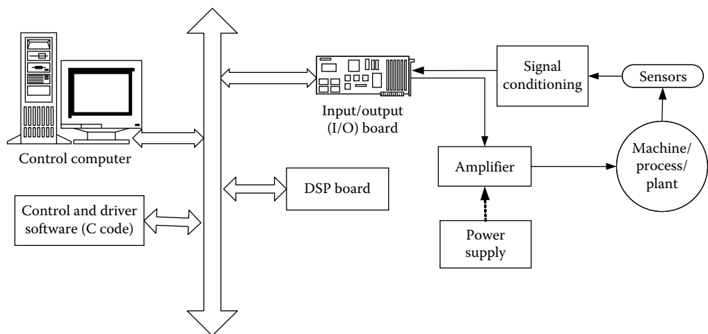
FIGURE 4.23 Components of a data acquisition (DAQ) and control loop.
