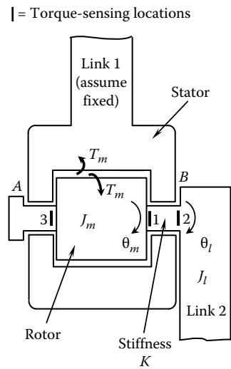
FIGURE P6.24 Torque sensing locations for a manipulator joint.
