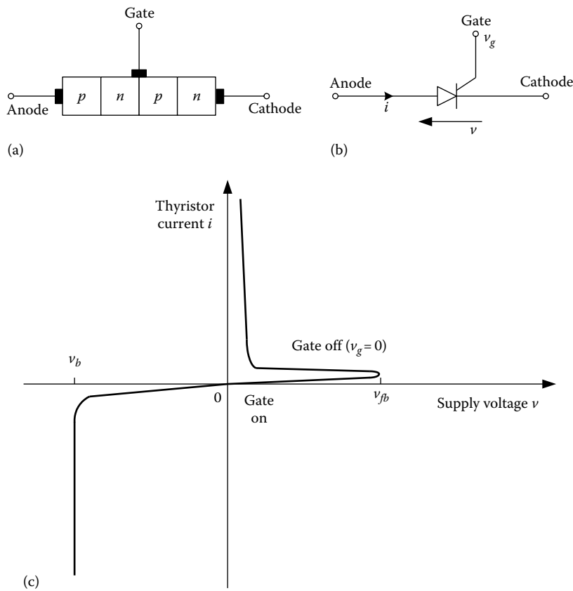
FIGURE 2.22 The thyristor: (a) Schematic representation; (b) circuit symbol; (c) characteristic curve.
