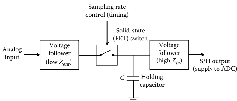
FIGURE 4.30 A sample and hold circuit.
