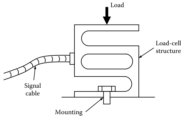
FIGURE 6.31 An industrial force sensor (load cell).
