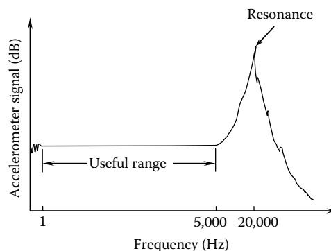
FIGURE 6.20 A typical frequency response curve for a piezoelectric accelerometer.
