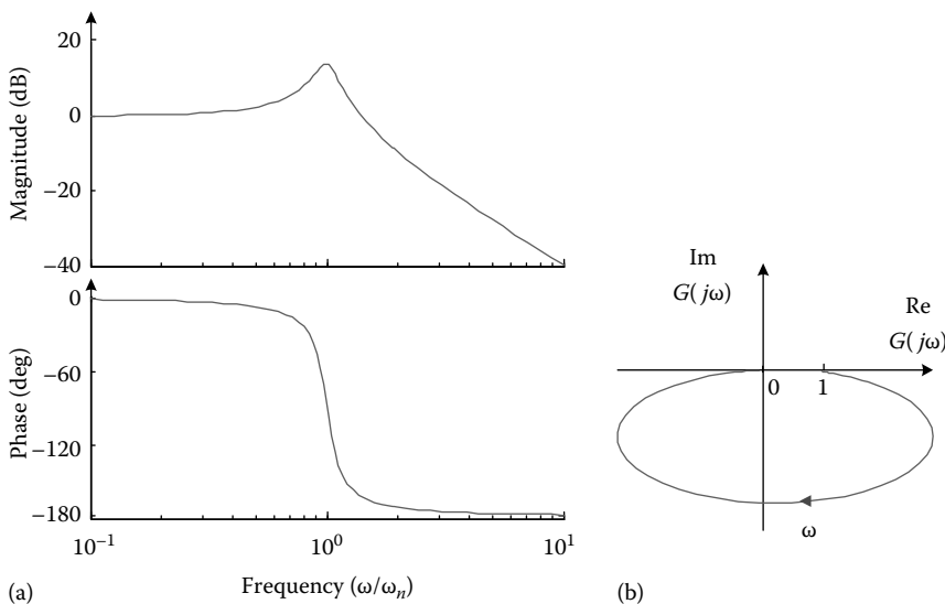
FIGURE 3.29 Frequency-domain model of a simple oscillator: (a) Bode plot; (b) Nyquist plot.
