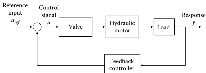
FIGURE 7.54 A closed-loop hydraulic control system.
