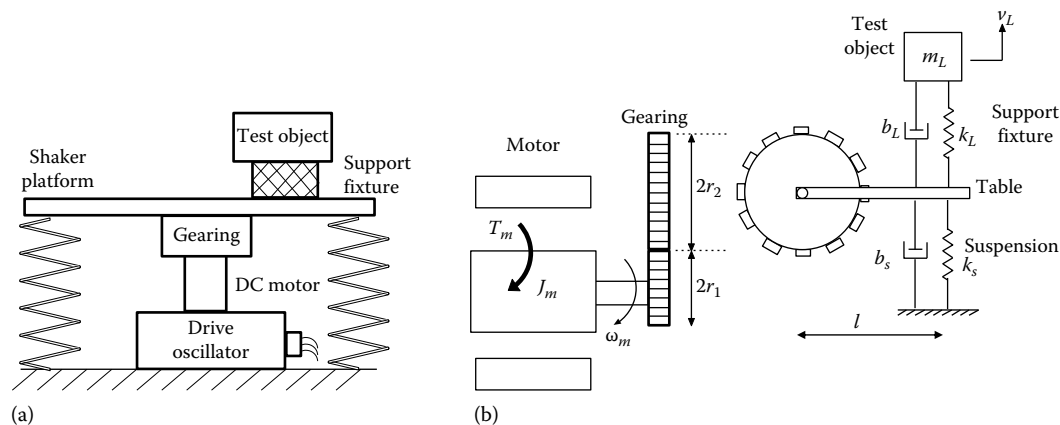
FIGURE P3.20 (a) A dynamic-testing system; (b) a model of the dynamic testing system.
