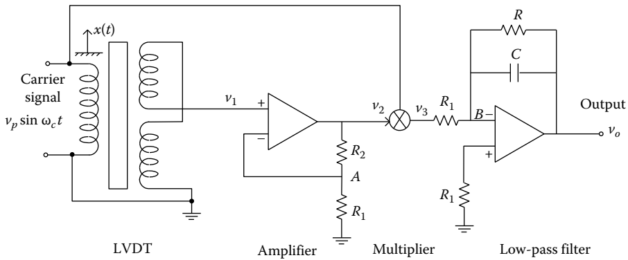
FIGURE 6.8 Signal conditioning system for an LVDT.
