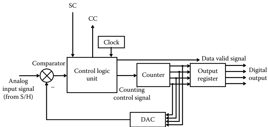
FIGURE 4.29 Counter ADC.
