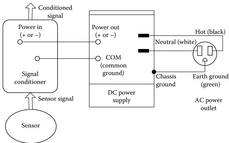
FIGURE 4.10 Instrument grounding—an example.
