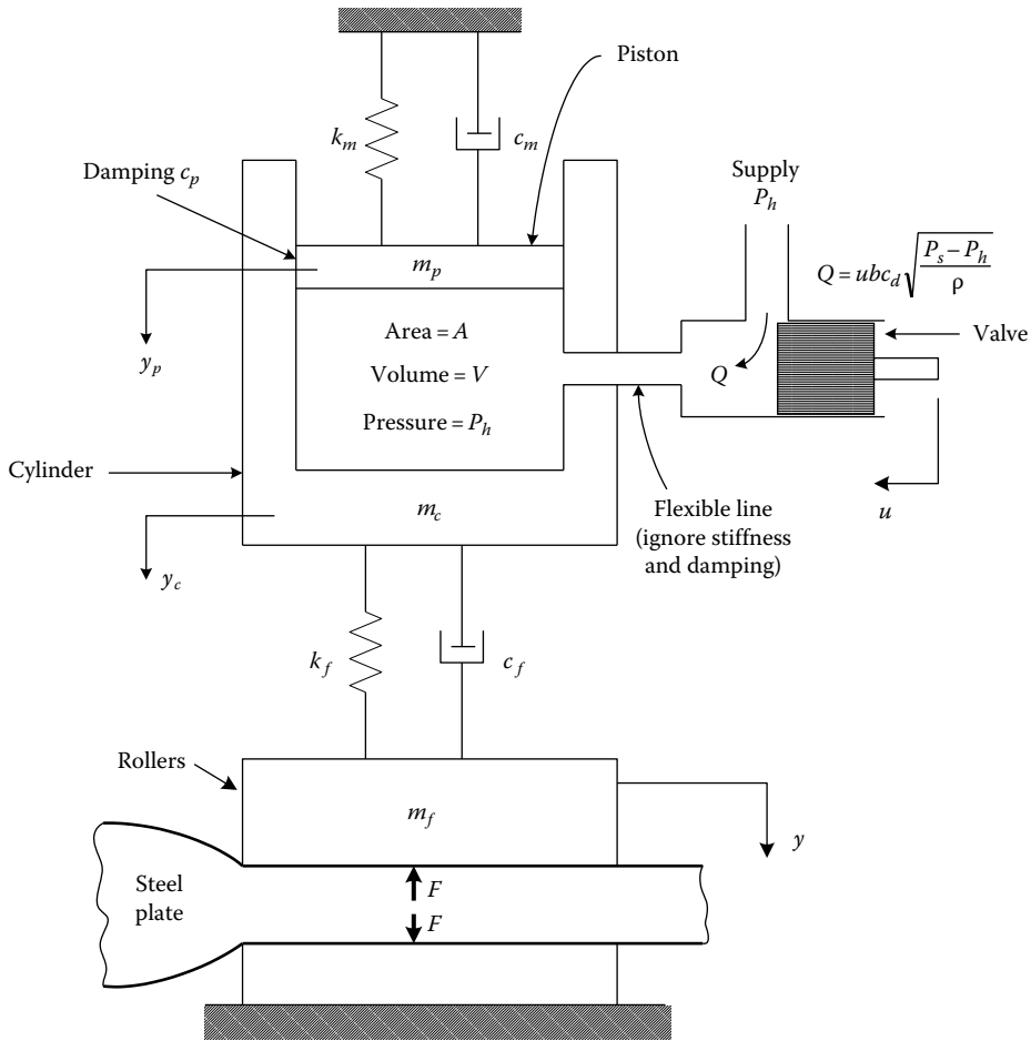
FIGURE 7.49 AGC system of a steel rolling mill.
