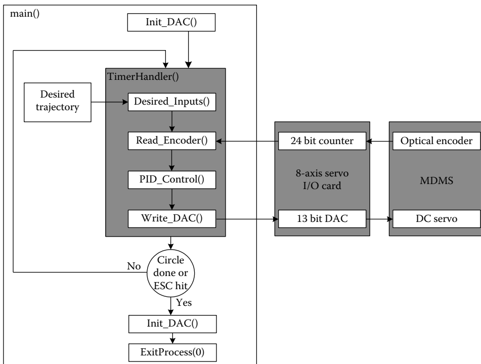
FIGURE 10.9 PID control of the MDMS.
