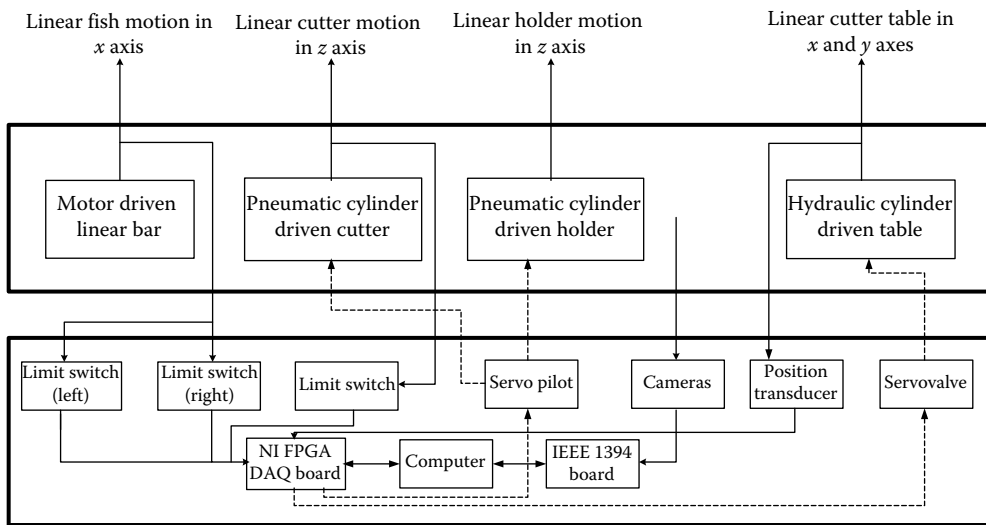
FIGURE 10.11 Control system architecture.
