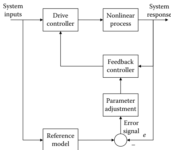
FIGURE 9.18 Model-referenced adaptive controller.
