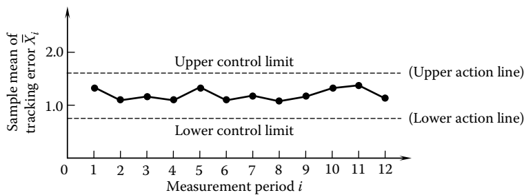
FIGURE 5.12 Control chart for the satellite tracking error example.
