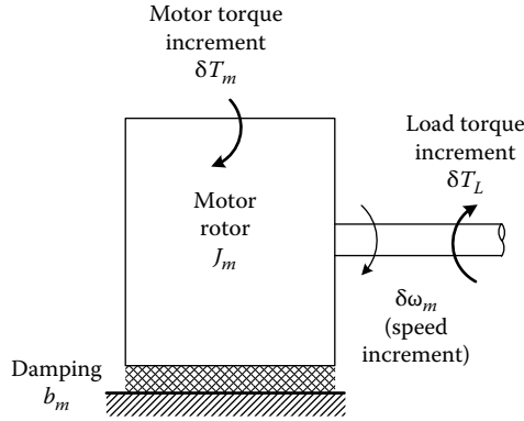
FIGURE 7.37 Incremental load model for an induction motor.
