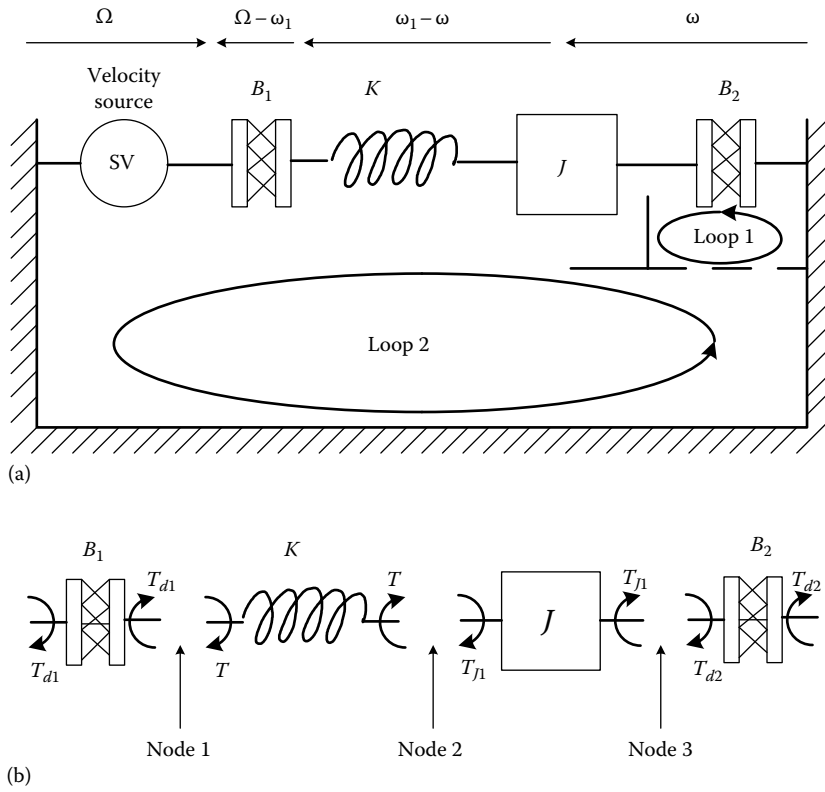
FIGURE 3.7 Model details for writing (a) loop equations; (b) node equations.
