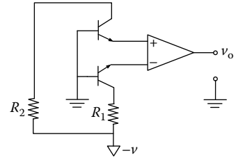
FIGURE 2.29 A circuit for a semiconductor temperature sensor.
