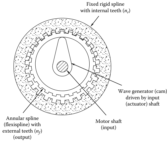
FIGURE 2.12 The principle of operation of a harmonic drive.
