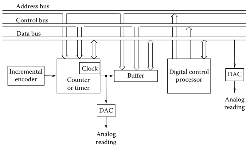
FIGURE 6.51 Computer interface for an incremental encoder.
