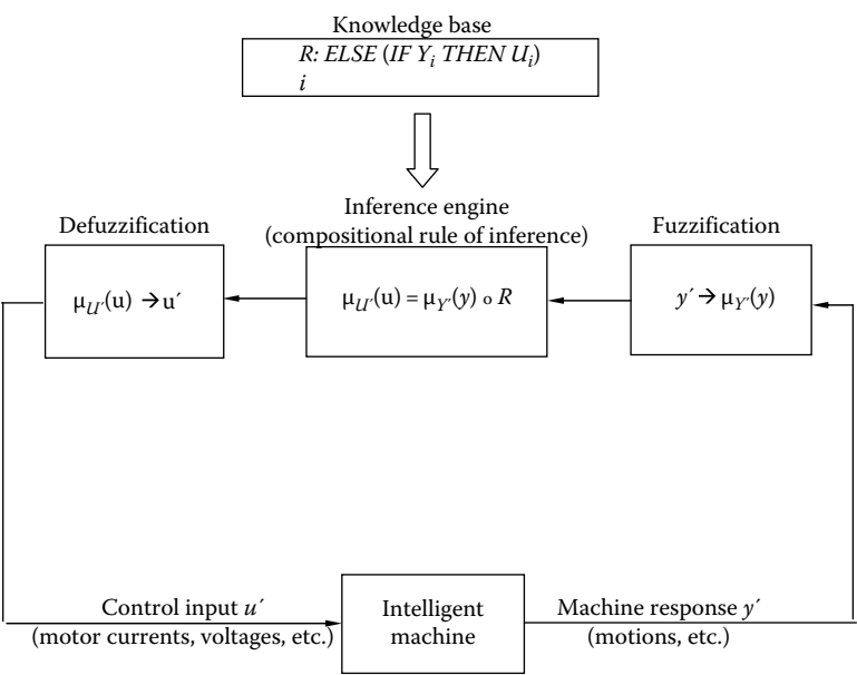
FIGURE 9.23 Structure of a direct fuzzy controller.
