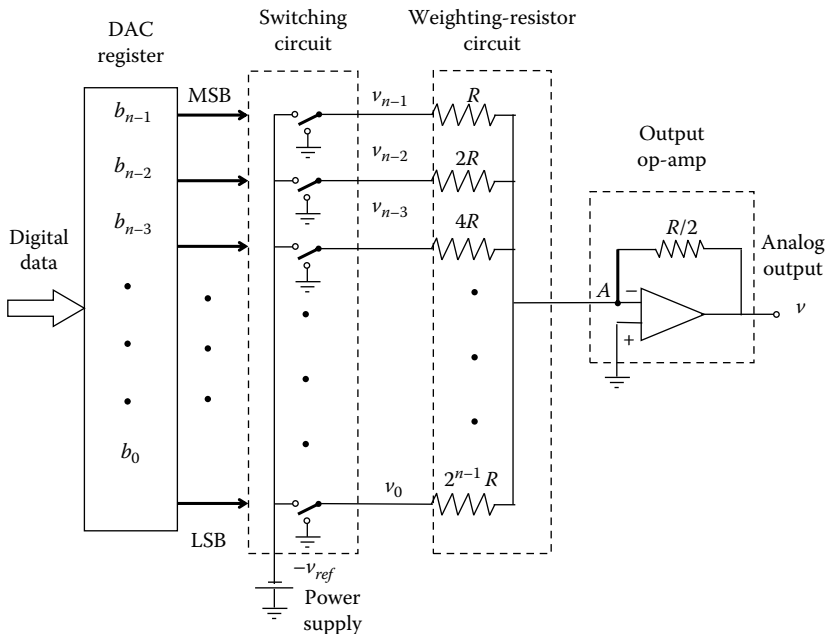
FIGURE 4.25 Weighted-resistor (adder) DAC.
