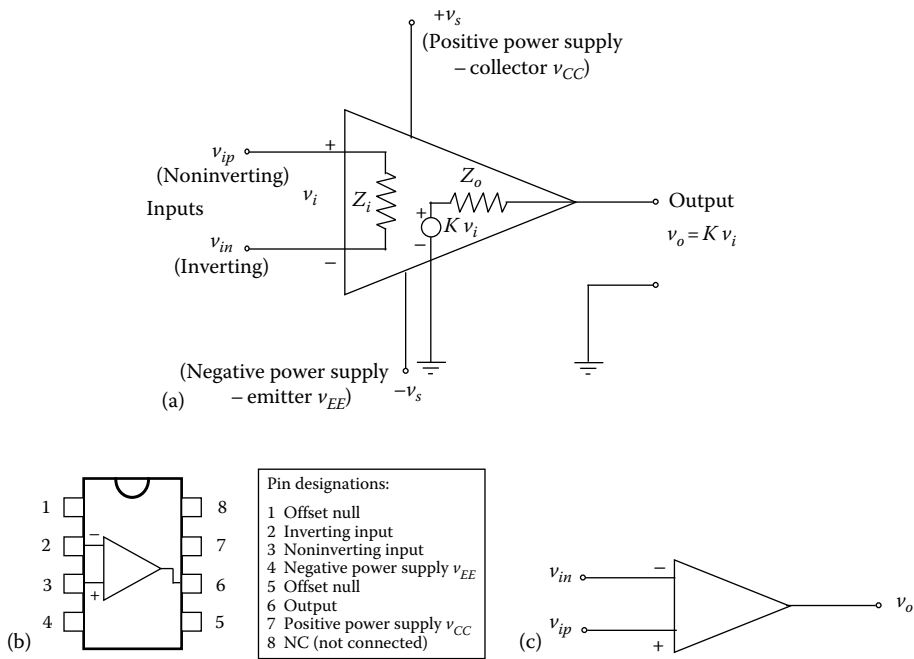
FIGURE 4.7 Operational amplifier. (a) A schematic model. (b) Eight-pin DIP. (c) Conventional circuit symbol.
