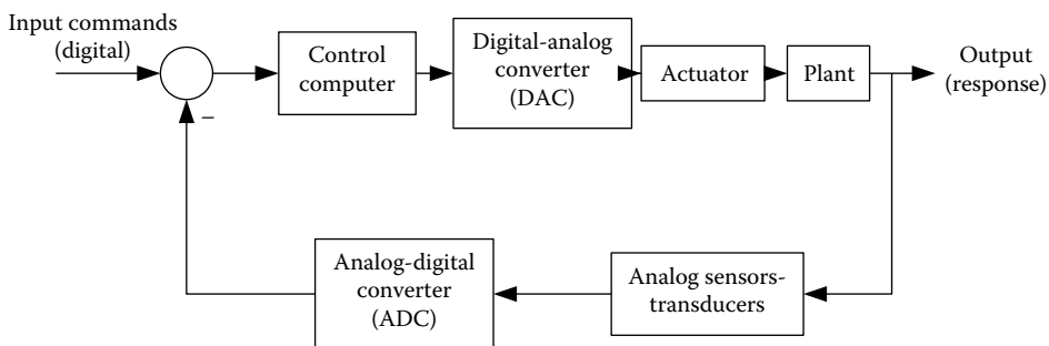
FIGURE 9.29 A digital feedback control system.
