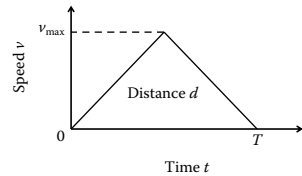
FIGURE 7.13 Speed profile for a motion period of the conveyor.
