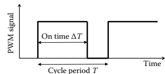
FIGURE 4.19 Duty cycle of a PWM signal.
