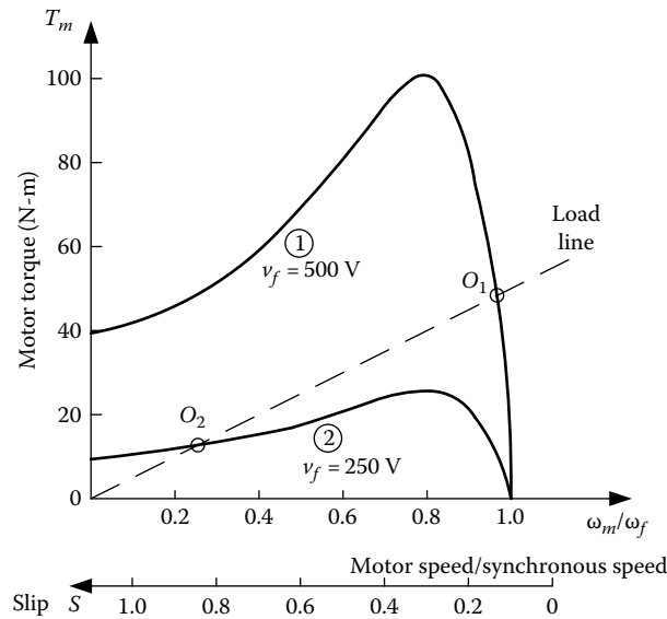
FIGURE 7.36 Speed-torque curves for induction motor voltage control.
