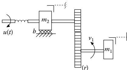
FIGURE P3.19 Rotary-motion system with a gear transmission.
