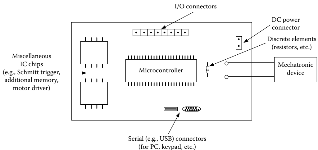
FIGURE 8.31 Microcontroller project breadboard.
