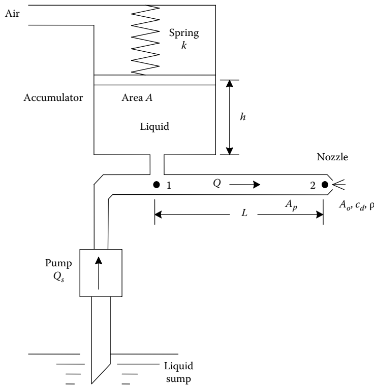
FIGURE P3.7 Pressure regulated liquid jet system.
