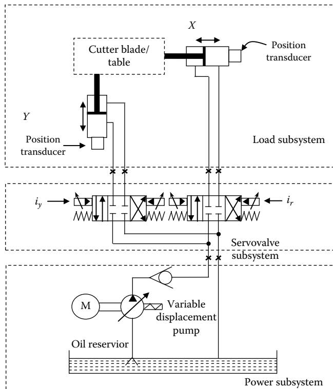
FIGURE 10.15 Schematic diagram of the hydraulic system.
