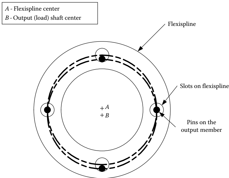
FIGURE 2.13 The principle of a pin-slot transmission.
