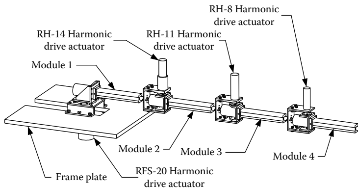
FIGURE 10.6 The CAD model of the MDMS prototype.
