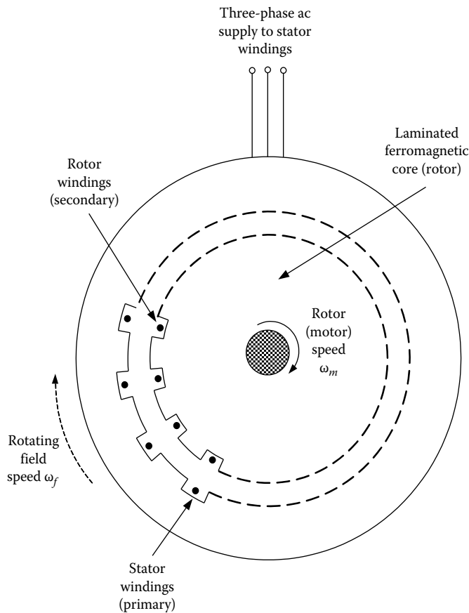
FIGURE 7.31 Schematic diagram of an induction motor.
