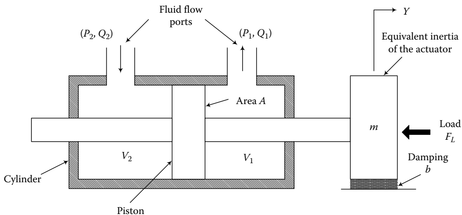
FIGURE 7.47 Double-acting piston-cylinder hydraulic actuator.
