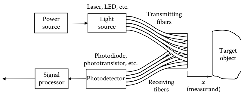
FIGURE 6.36 A fiber-optic position sensor.
