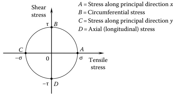
FIGURE A.6 Mohr's circle for pure torsion of a shaft.
