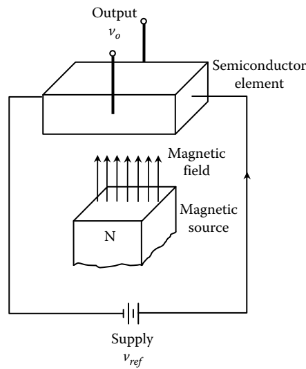
FIGURE 6.55 Schematic representation of a Hall-effect sensor.
