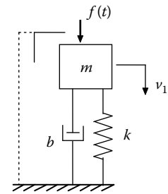
FIGURE 3.28 Damped simple oscillator.
