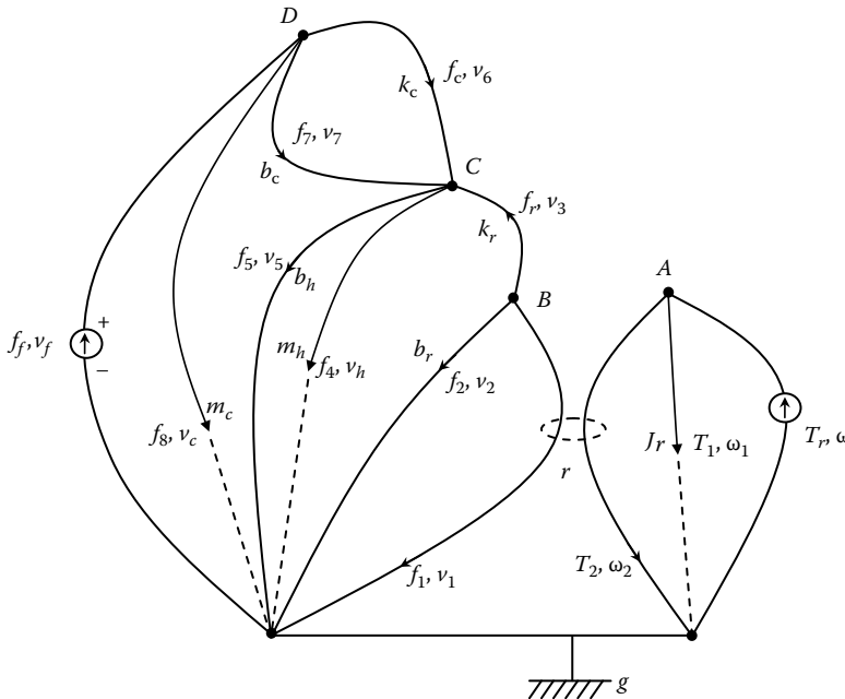
FIGURE 3.21 Linear graph of the robotic sewing system.
