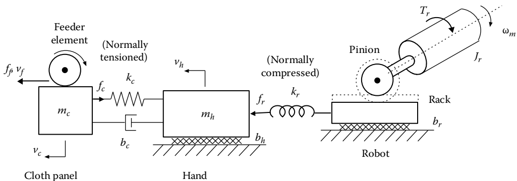
FIGURE 3.20 A robotic sewing system.
