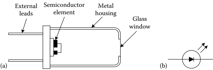
FIGURE 2.30 An LED: (a) Physical construction; (b) circuit symbol.
