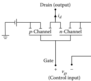
FIGURE 8.23 CMOS (complementary symmetric MOSFET) memory element.
