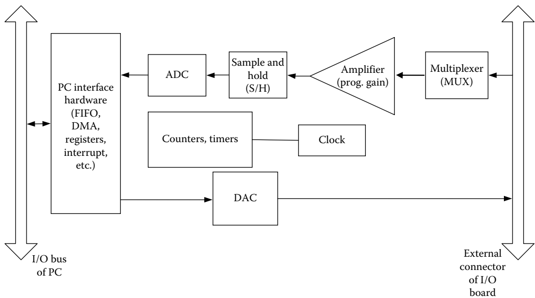
FIGURE 4.24 Main components of an I/O board of a PC.
