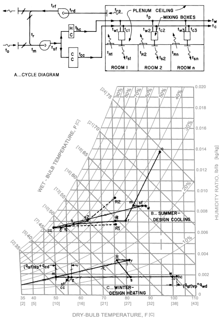
Figure 6-8. Single-fan dual-duct system with blow-through dehumidification—schematic and psychrometric chart.
