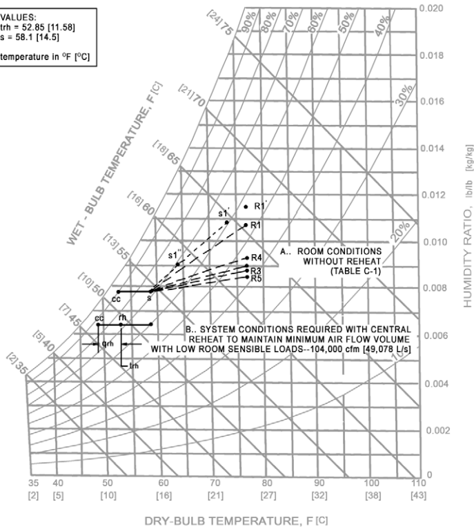
Figure C-2. Psychrometric analysis for single-duct VAV system with separate perimeter radiation at outdoor conditions of 65°F/65°F [18.3°C/18.3°C].
