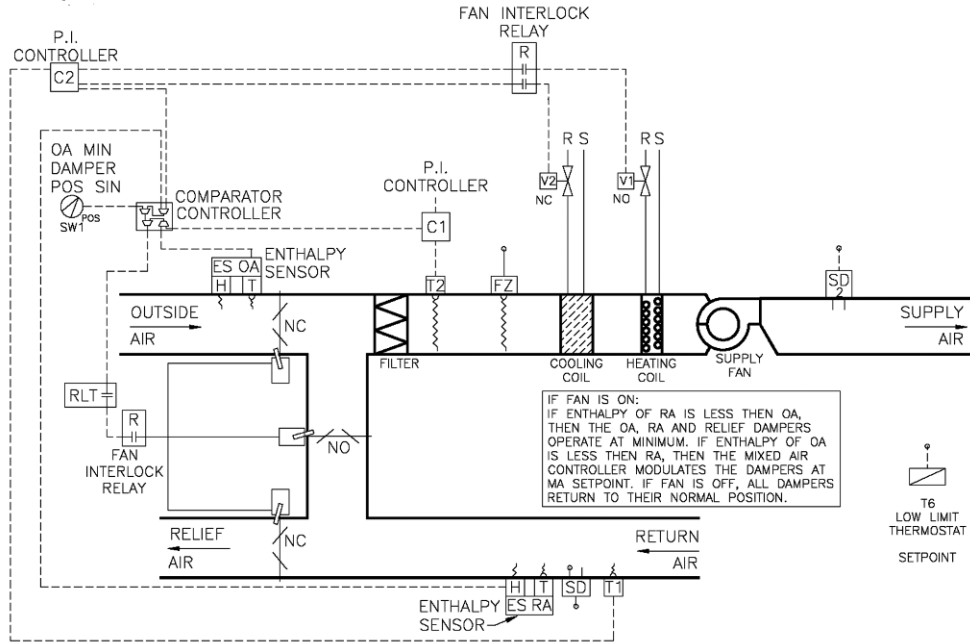
Figure 10-9. Minimum single-zone control system.
