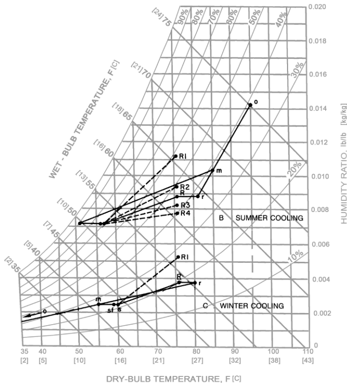
Figure 6-3. VAV system—schematic and psychrometric chart.
