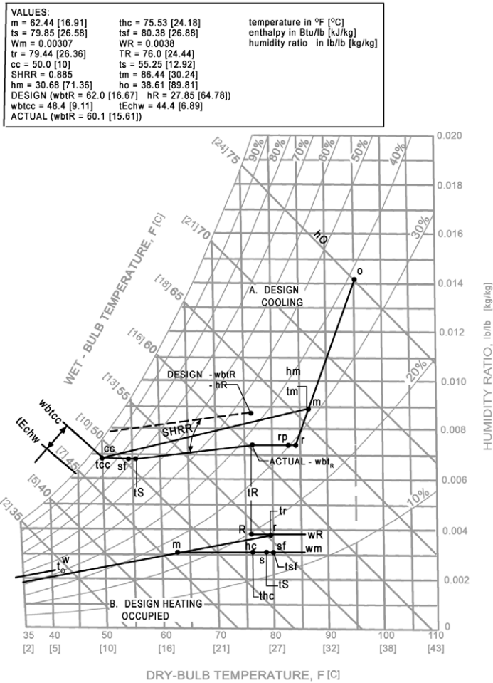
Figure B-1. Psychrometric analysis for single-duct, single-zone system.
