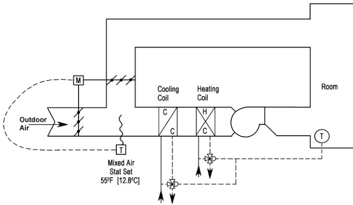
Figure 9-20. Schematic of conventional HVAC system.
