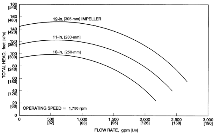
Figure 7-6. Performance of three pumps with different impeller diameters operating at 1750 rpm.
