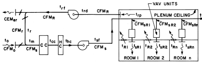
A... TRUE VAV SYSTEM CYCLE DIAGRAM
