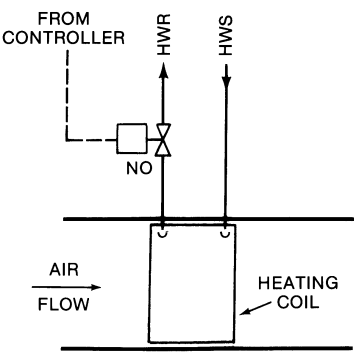
Figure 5-12. Two-way valve controlling hot water circuit.
