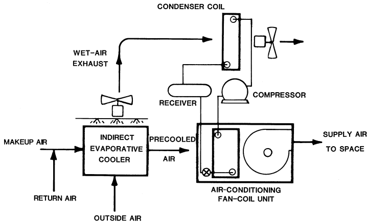
Figure 5-3. Indirect evaporative cooler used as a precooling.
