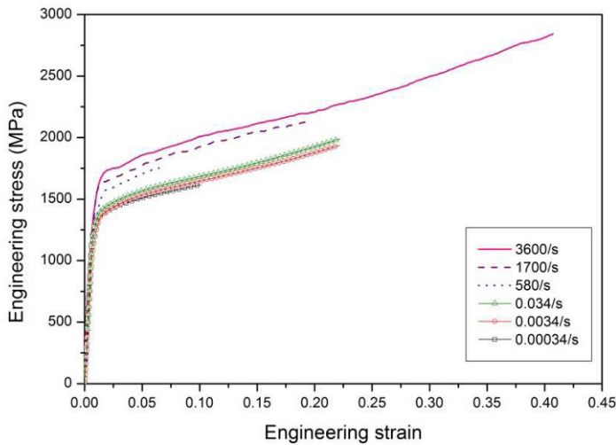
Figure 5.9 Engineering stress-strain curves of 4340 R_c45 steel (Reproduced from Song et al. (2007a) with permission)
