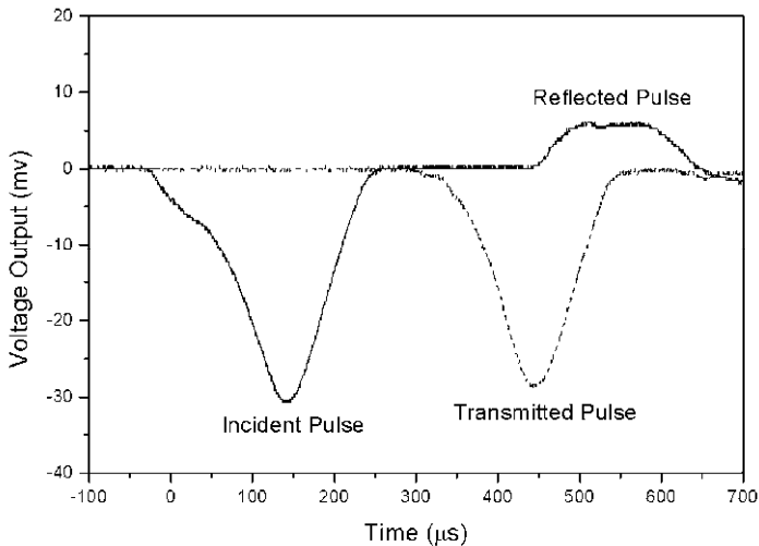
Figure 6.14 Typical incident, reflected, and transmitted signals (Reproduced from Song and Chen (2004a) with permission)
