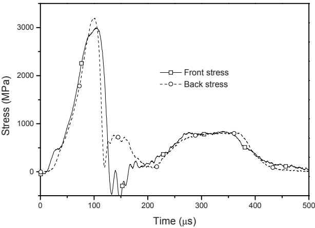
Figure 3.19 Dynamic equilibrium check during loading and reloading (Reproduced from Chen and Luo (2004) with permission)
