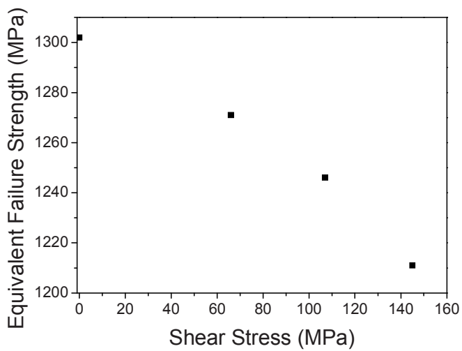
Figure 3.37 Effect of shear stress on the failure initiation in the glass specimen (Reproduced from Nie et al. (2007) with permission)
