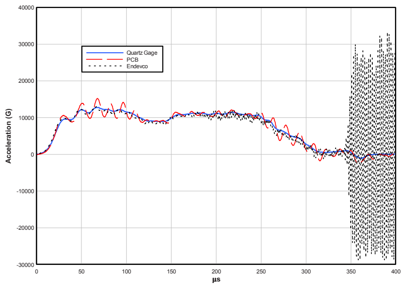
Figure 10.21 The acceleration measured by different devices
