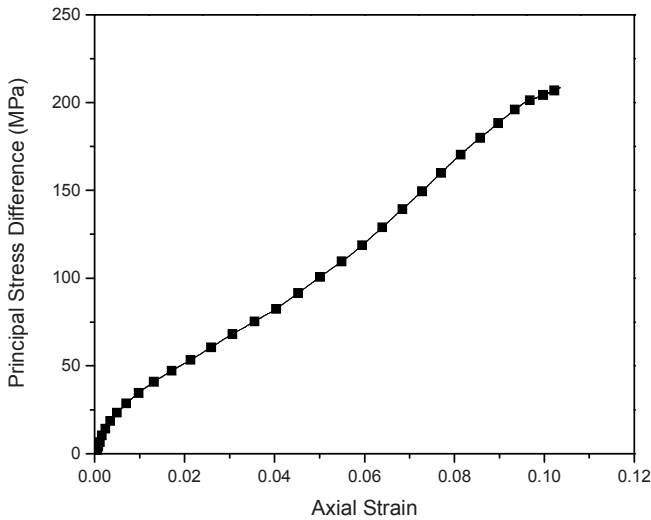
Figure 6.10 An example of dynamic triaxial experimental results on a sand (Reproduced from Kabir et al. (2010) with permission)
