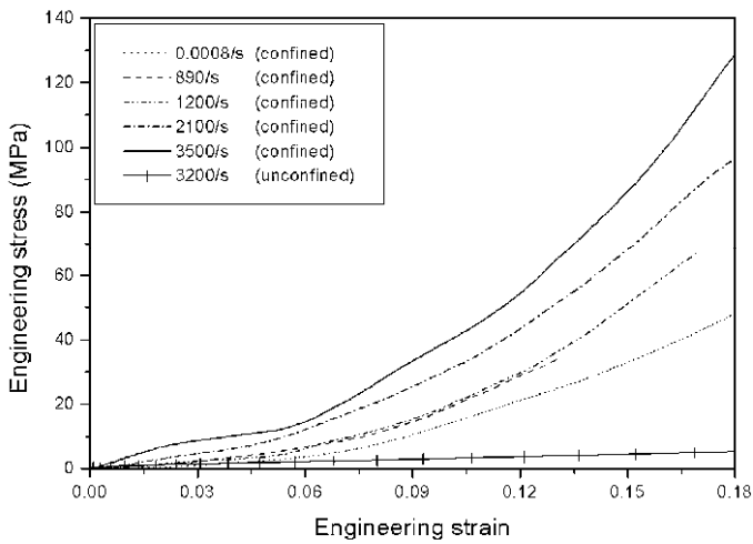
Figure 6.15 Dynamic stress-strain response of the EPDM rubber under confinement (Reproduced from Song and Chen (2004a) with permission)
