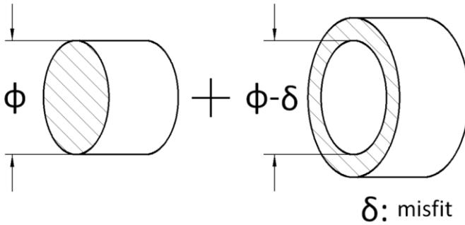
Figure 3.4 Hard platens confined by press-fit ductile rings (Reproduced from Chen and Ravichandran (1997) with permission)
