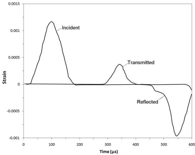
Figure 3.13 Incident, reflected and transmitted pulses in a pulse-shaped Kolsky bar experiment on an Indiana limestone (Reproduced from Frew et al. (2001) with permission)
