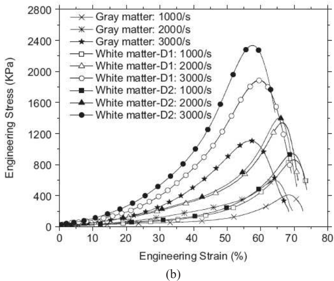
Figure 4.45 Compressive stress-strain curves of bovine brain tissues under (a) quasi-static and (b) dynamic loading conditions (Reproduced from Pervin and Chen (2009) with permission)
