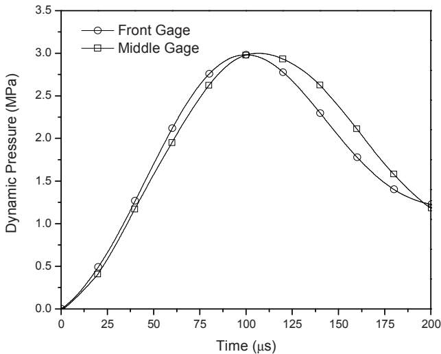
Fig. 6.7 Dynamic pressure variation inside the pressure chamber
