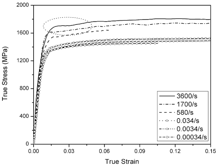
Figure 5.10 True stress-strain curves of 4340 R 45 steel (Reproduced from Song et al. (2007a) with permission)
