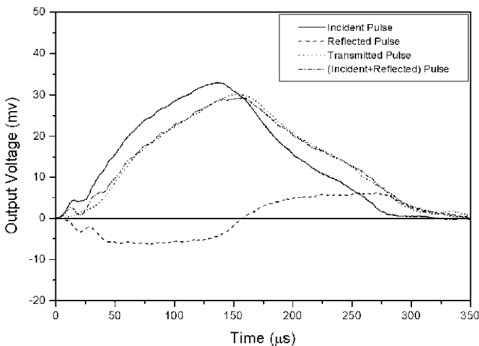
Figure 5.18 Experimental records of the bar signals on the shape memory alloy (Reproduced from Song and Chen (2004c) with permission)
