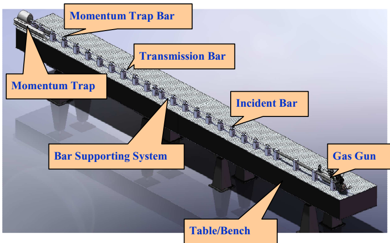
Figure 1.11 A perspective view of the Kolsky compression bar (Reproduced from Song et al. (2009b) with permission)
