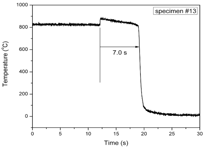
Figure 7.12 Temperature history in the specimen (Reproduced from Song et al. (2010) with permission)
