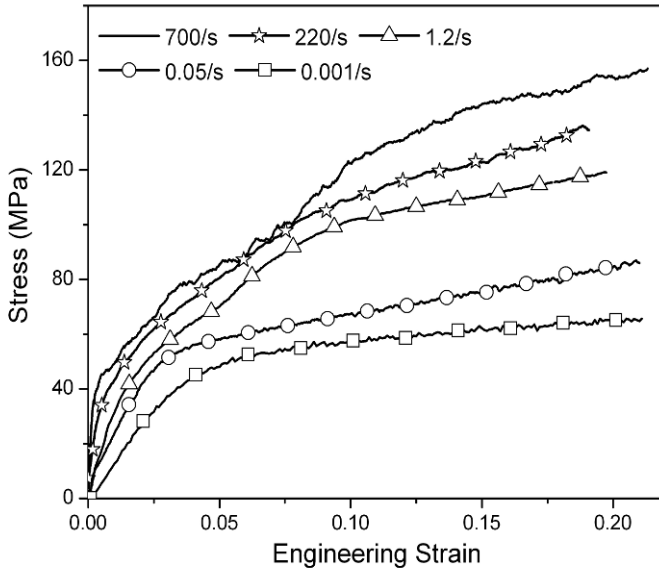
Figure 5.27 Compressive stress-strain curves of Sn3.8Ag0.7Cu solder
