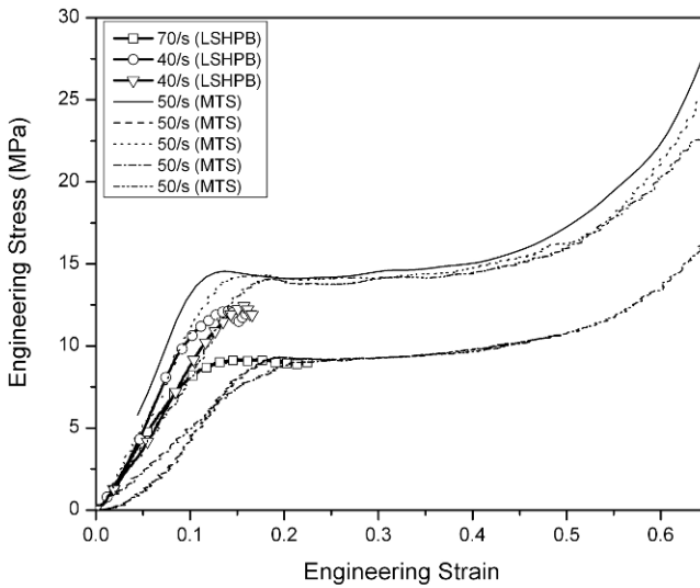
Figure 9.18 Compressive stress-strain curves obtain from MTS and long Kolsky bar at \sim 50 \text{ s}^{-1} (Reproduced from Song et al. (2008) with permission)
