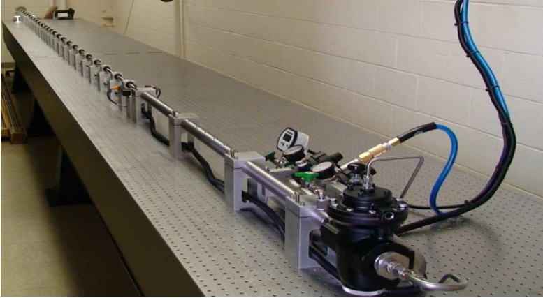
Figure 1.12 Photograph of the Kolsky compression bar (Reproduced from Song et al. (2009b) with permission)
