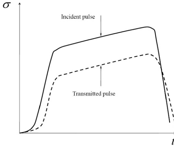
Figure 5.2 Illustration of pulse shaping design for ductile materials
