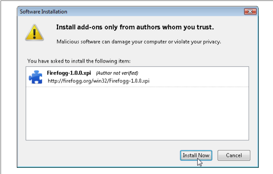
Figure 5-3. Install Firefogg
