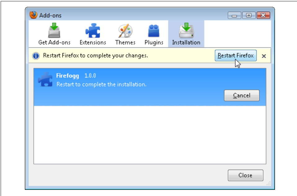
Figure 5-4. Restart Firefox
