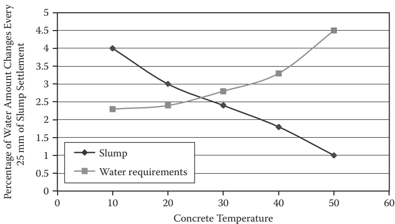
FIGURE 5.40 Effect of concrete temperature on concrete slump and water quantity.
