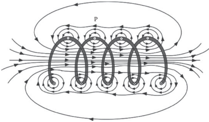
FIGURE 8.56 Direction of magnet flow.
