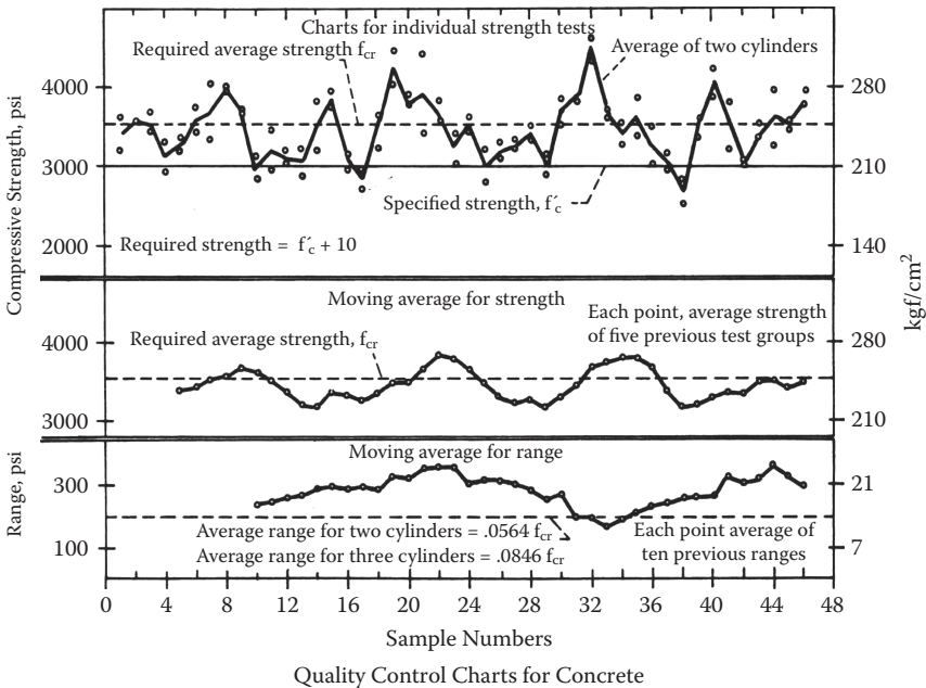
FIGURE 4.21 Concrete quality control chart.
