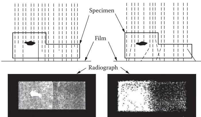
FIGURE 8.11 Internal scatter.
