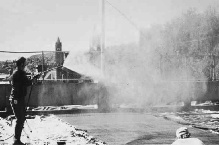
FIGURE 5.48 Curing concrete with silica fume.
