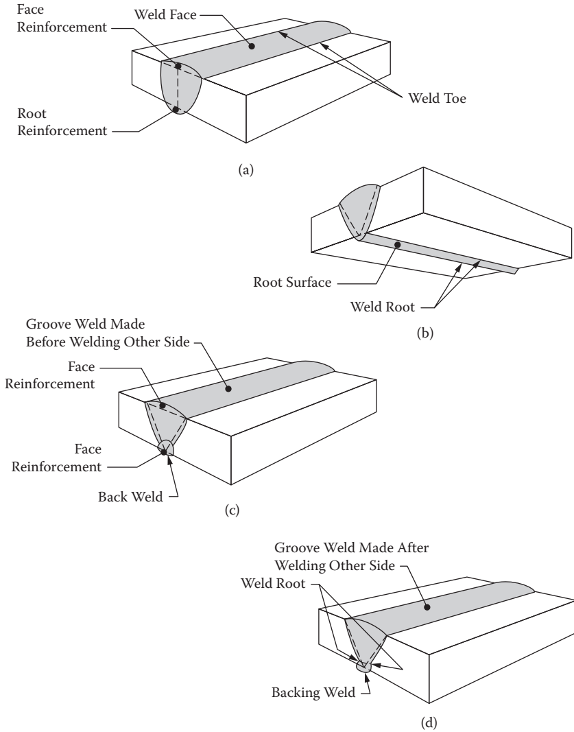
FIGURE 7.8 Butt weld.
