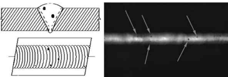
FIGURE 8.24 Porosity.
