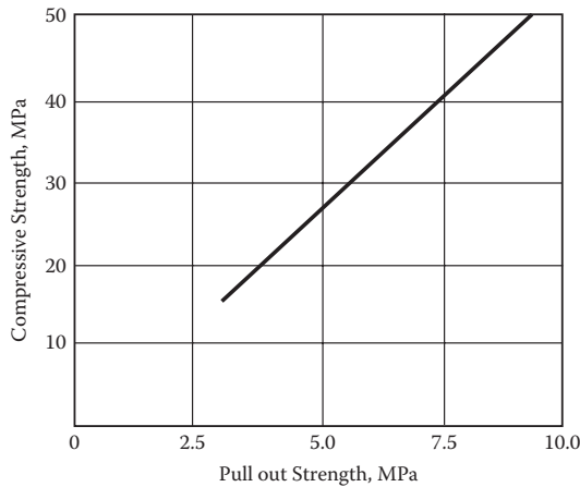
FIGURE 6.16 Sketch of the relation between pullout strength and concrete compressive strength.
