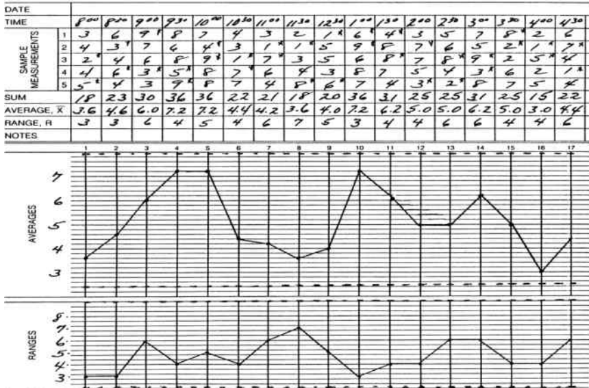
FIGURE 4.20 Process chart.
