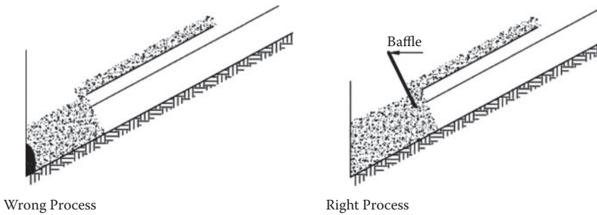
FIGURE 5.21 Pouring inclined concrete slab.
