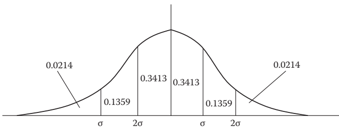
FIGURE 4.5 Dividing the area under the normal distribution curve.
