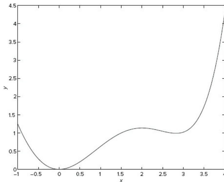
Figure 3.2-4 Plot of the function y = 0.025x^5 - 0.0625x^4 - 0.333x^3 + x^2 .
