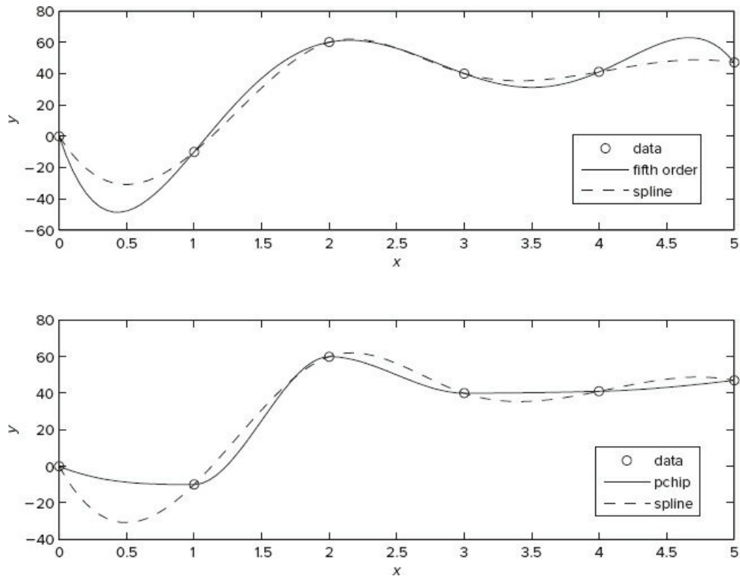
Figure 7.4-5 Top graph: Interpolation with a fifth-order polynomial and a cubic spline. Bottom graph: Interpolation with piecewise continuous Hermite polynomials (pchip) and a cubic spline.
