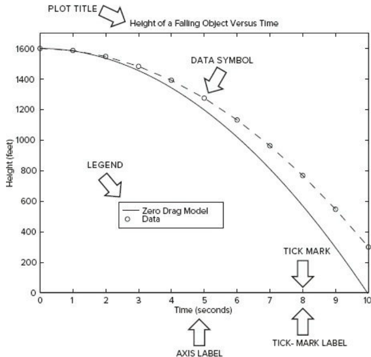
Figure 5.1-1 Nomenclature for a typical xy plot.
