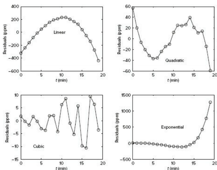
Figure 6.2–3 Residual plots for the four models.
