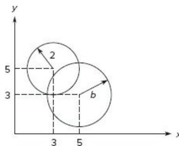
Figure 11.2-1 Intersection points of two circles.
