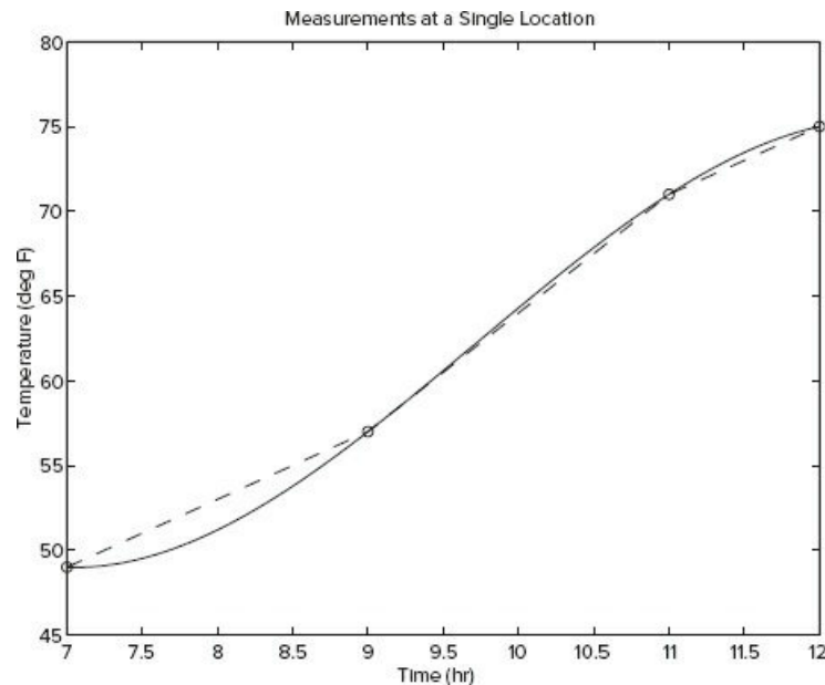
Figure 7.4-3 Linear and cubic spline interpolation of temperature data.
