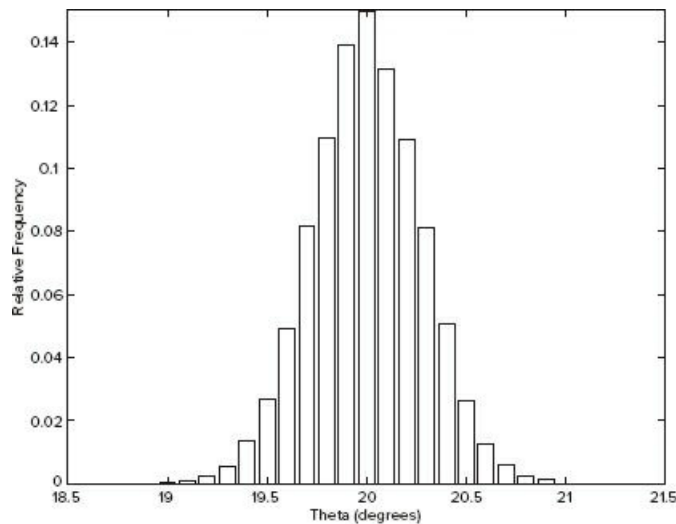
Figure 7.3-2 Scaled histogram of the angle \theta .
