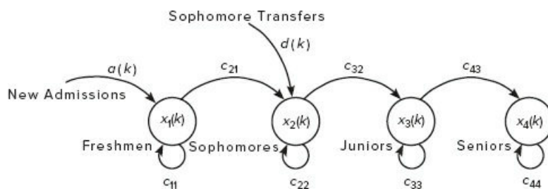
Figure 4.9-1 The state transition diagram for the college enrollment model.
