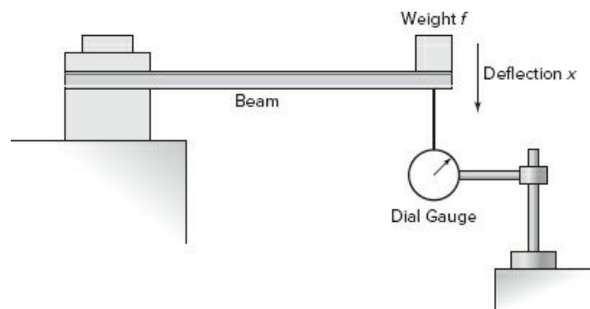
Figure 6.1–7 Measurement of beam deflection.
