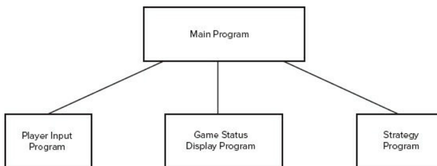
Figure 4.1-1 Structure chart of a game program.
