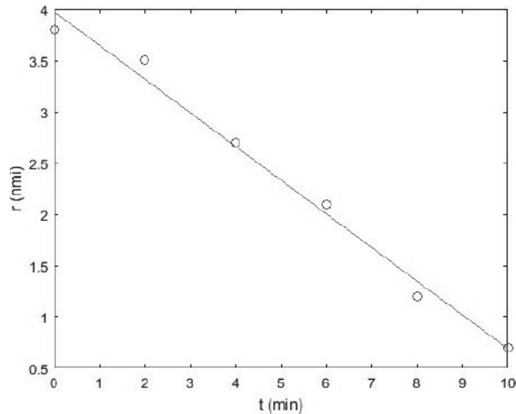
Figure 6.1–3 Range versus time: the sonar data and the fitted line.
