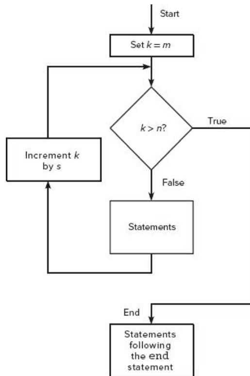
Figure 4.5-1 Flowchart of a for loop.
