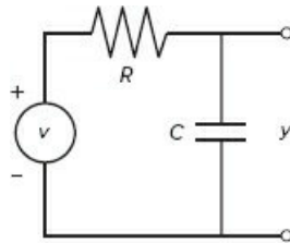
Figure 9.3-1 An RC circuit.
