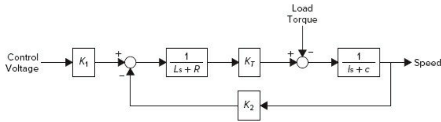
Figure 10.7-9 An armature-controlled dc motor.
