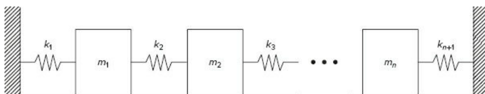
Figure 10.7-8 A vibrating system.
