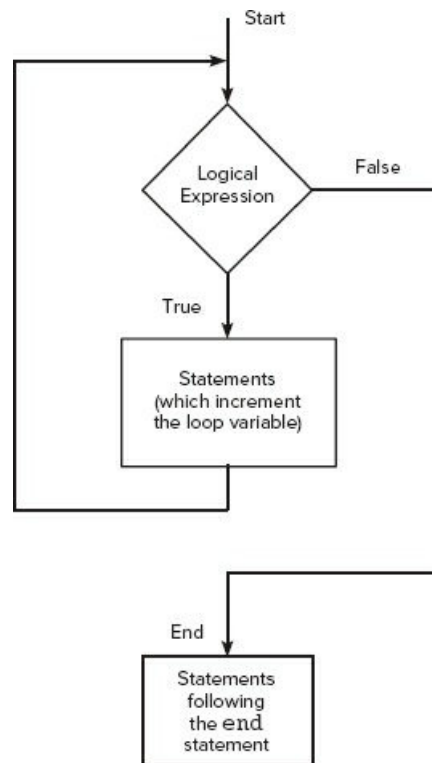
Figure 4.6-1 Flowchart of the while loop.
