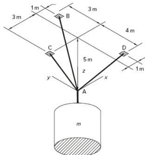
Figure 8.2-1 A mass suspended by three cables.
