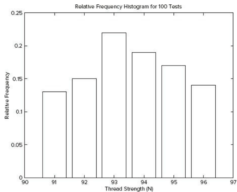
Figure 7.1-3 Relative frequency histogram for 100 thread tests.
