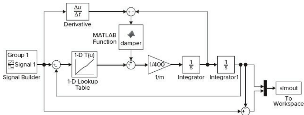
Figure 10.9-6 Simulink model of a vehicle suspension system.
