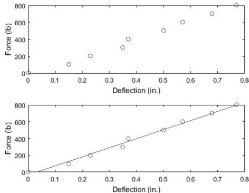
Figure 6.1–8 Plots for the cantilever beam example.
