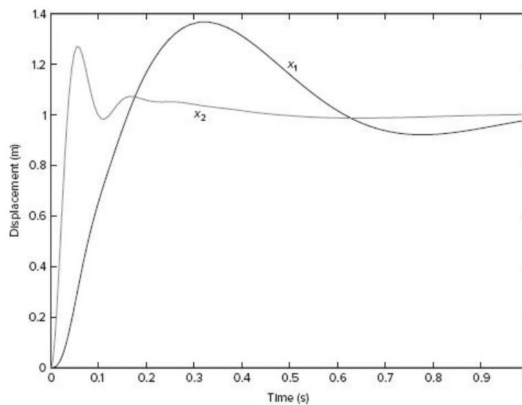
Figure 10.3-3 Unit-step response of the two-mass suspension model.
