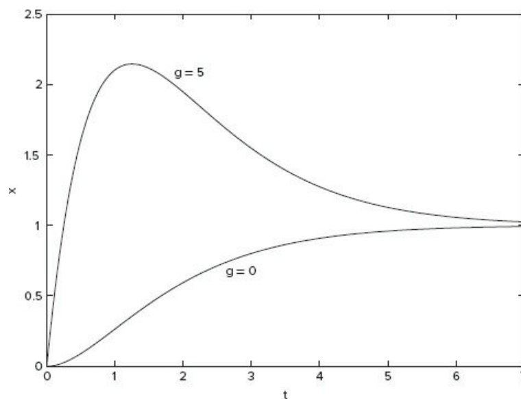
Figure 11.5-3 The step response of the model \ddot{x} + 1.4\dot{x} + x = u + g\dot{u} for g = 0 and g = 5 .
