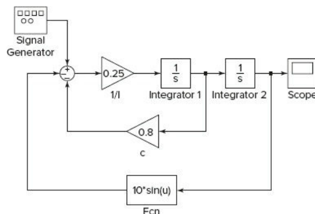
Figure 10.6-2 Simulink model of nonlinear pendulum dynamics.
