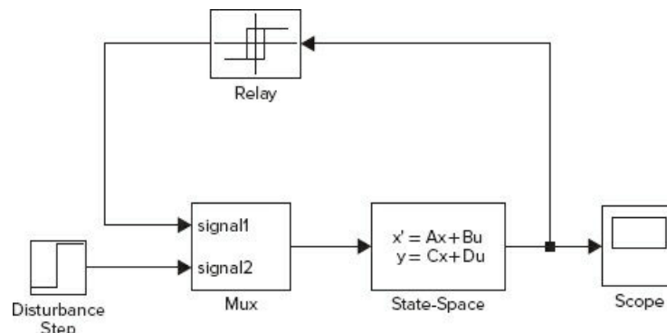
Figure 10.4-9 Simulink model of a relay-controlled motor.
