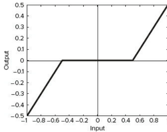
Figure 10.5-1 A dead-zone nonlinearity.
