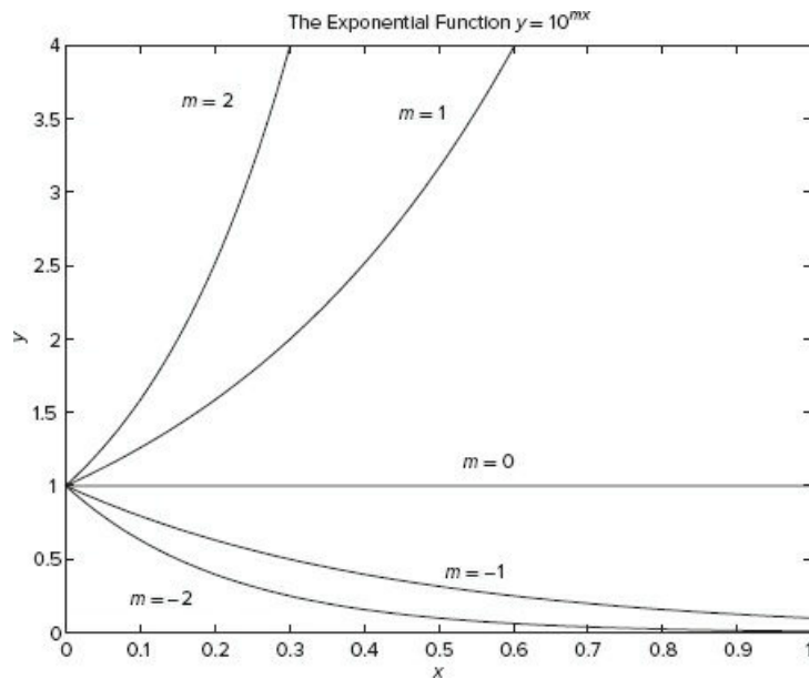
Figure 6.1–1 Examples of exponential functions.
