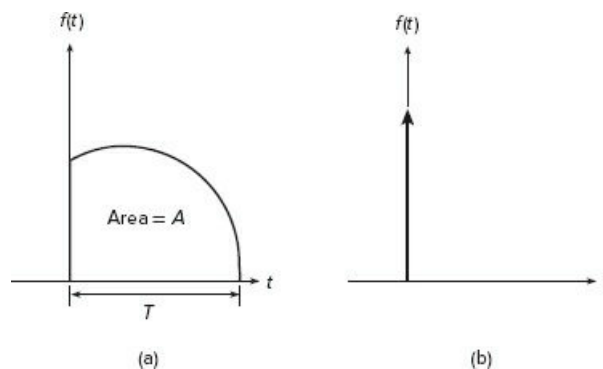
Figure 11.5-4 Pulse and impulse functions.
