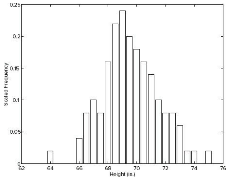
Figure 7.2-1 Scaled histogram of height data.
