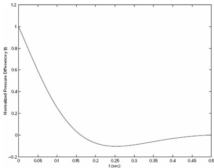
Figure 2.3-1 Aortic pressure response for Example 2.3-2 .
