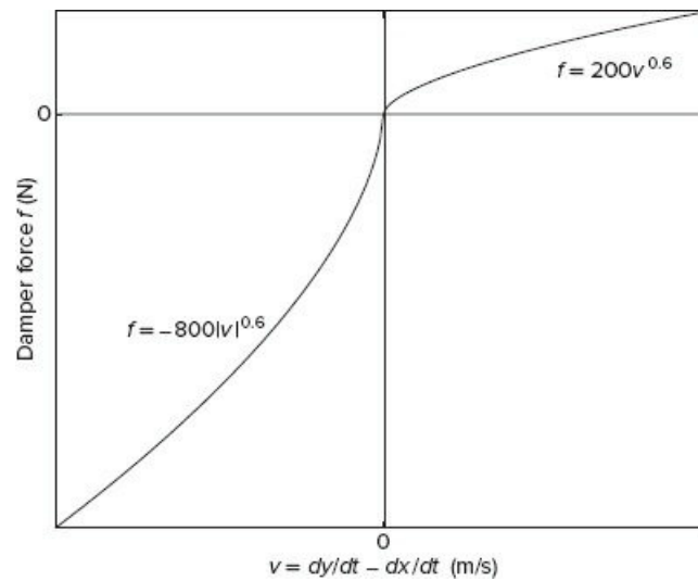
Figure 10.9-3 Nonlinear damping function.
