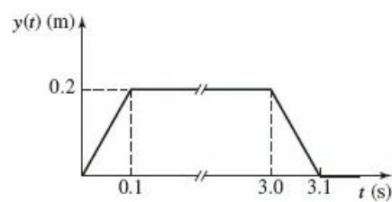
Figure 10.9-4 Road surface profile.
