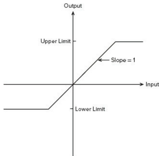
Figure 10.4-1 The saturation nonlinearity.
