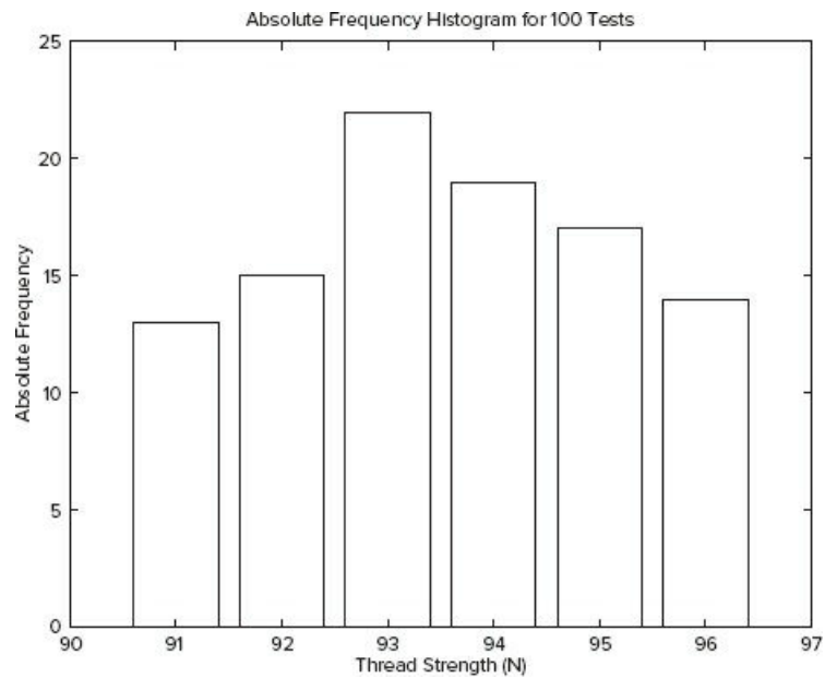
Figure 7.1-2 Absolute frequency histogram for 100 thread tests.
