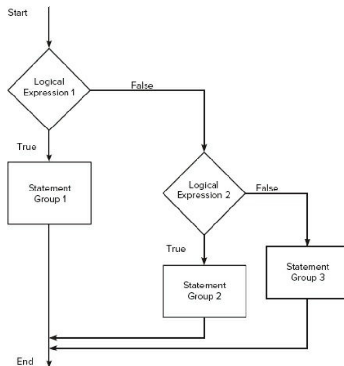
Figure 4.4-3 Flowchart for the general if structure.
