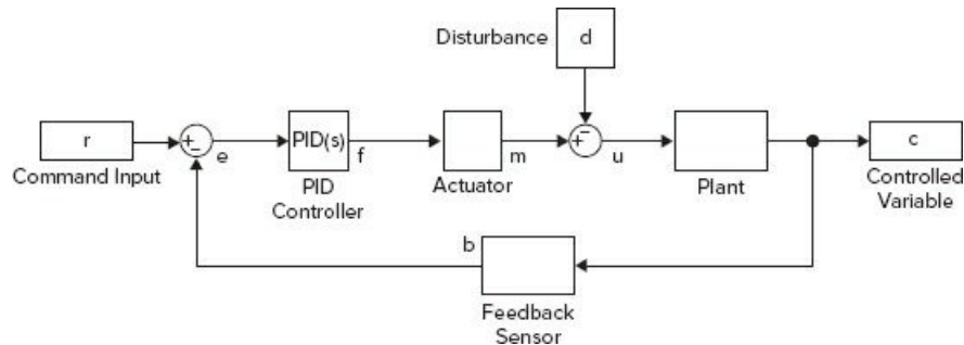
Figure 10.10-1 Structure of a feedback control system.
