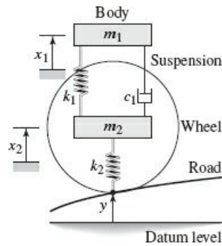
Figure 10.3-1 Two-mass suspension model.
