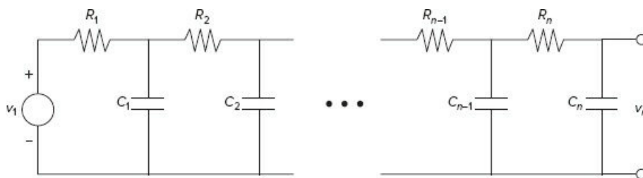
Figure 10.7-7 A network of RC loops.
