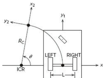
Figure 10.10-8 Turning geometry of a two-wheeled vehicle
