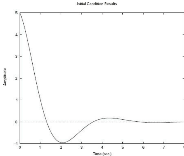
Figure 9.5-2 Free response of the model given by Equations (9.5-5) through (9.5-8) for x_1(0) = 5 and x_2(0) = -2 .
