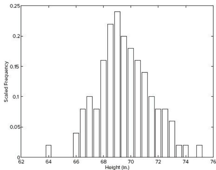
Figure 7.2-1 The basic shape of the normal distribution curve.
