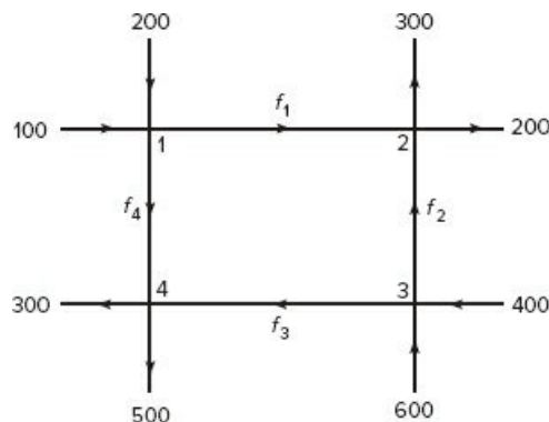
Figure 8.3-2 A network of one-way streets.
