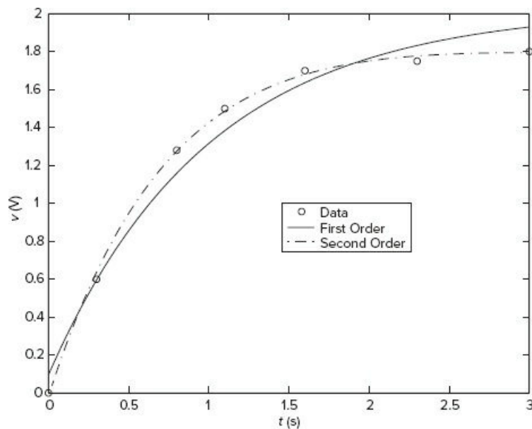
Figure 6.2–4 Comparison of first- and second-order model fits.
