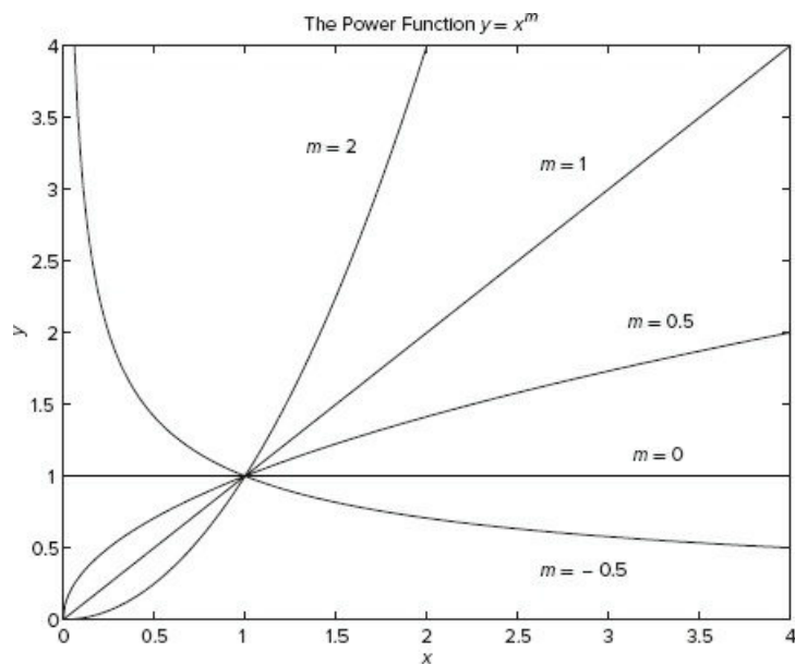
Figure 6.1–2 Examples of power functions.
