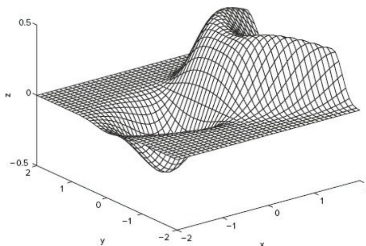
Figure 5.4-2 A plot of the surface z = xe^{-(x-y)^2 - y^2} created with the mesh function.
