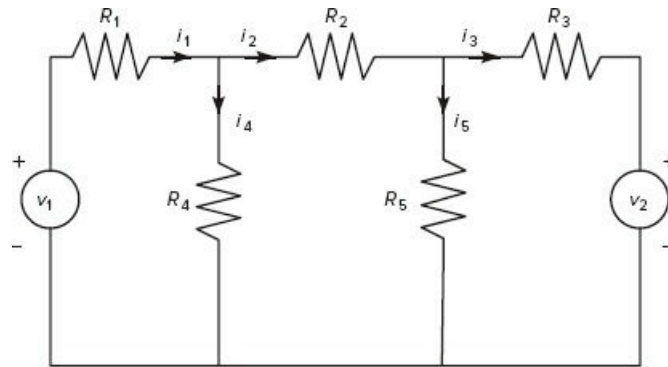
Figure 8.2-2 An electric resistance network.
