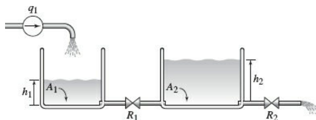
Figure 10.7-5 A hydraulic system with two tanks.
