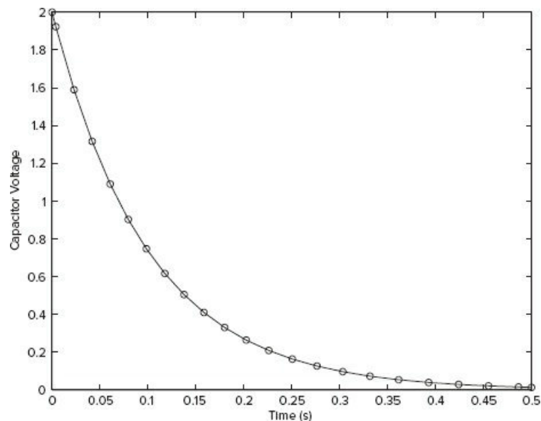
Figure 9.3-2 Free response of an RC circuit.
