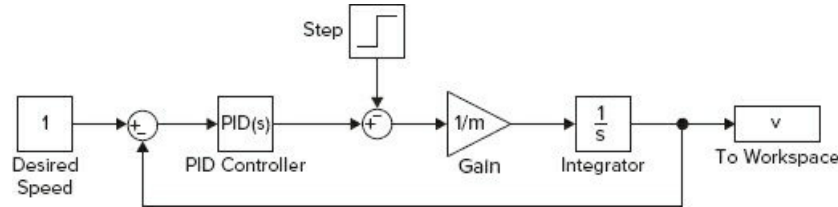
Figure 10.10-3 Simulink model of the simplest speed control system.
