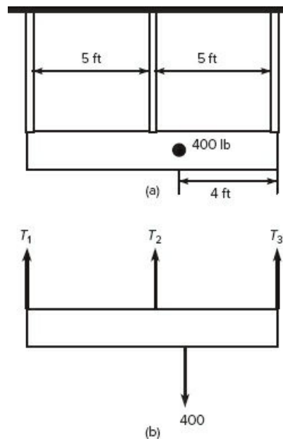
Figure 8.3-1 A light fixture and its freebody diagram.
