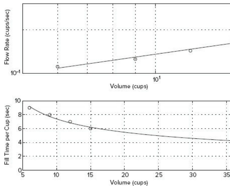
Figure 6.1–6 Flow rate and fill time for a coffee pot.
