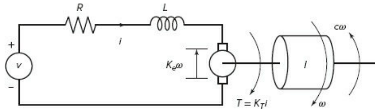
Figure 10.4-8 An armature-controlled dc motor.
