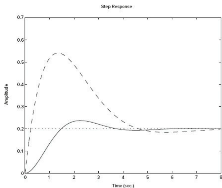
Figure 9.5-3 Step response of the model given by Equations (9.5–6) through (9.5–8) and the model (9.5–10) , for zero initial conditions.
