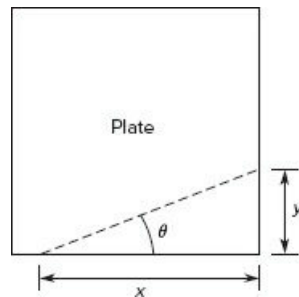
Figure 7.3-1 Dimensions of a triangular cut.
