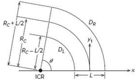
Figure 10.10-9 Wheel paths in a circular turn.
