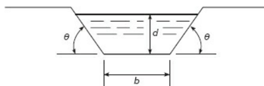
Figure 3.2-5 Cross section of an irrigation channel.
