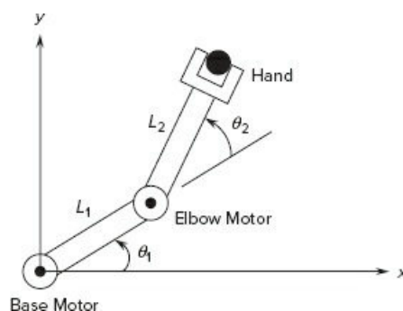
Figure 11.2-2 A robot arm having two joints and two links.
