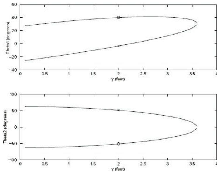
Figure 11.2-3 Plot of the motor angles for the robot hand moving along a vertical line.
