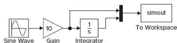
Figure 10.2-5 Simulink model using a Mux and the To Workspace blocks.
