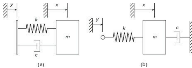
Figure 11.5-2 Two mechanical systems. The model for (a) contains the derivative of the input y(t) ; the model for (b) does not.
