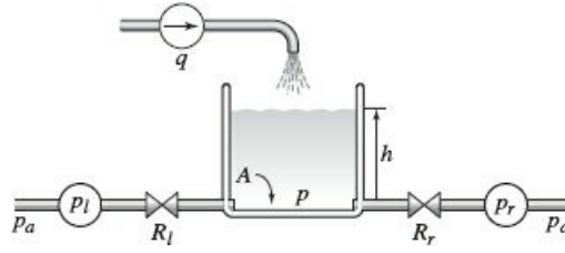
Figure 10.7-2 A hydraulic system with a flow source and two pumps.
