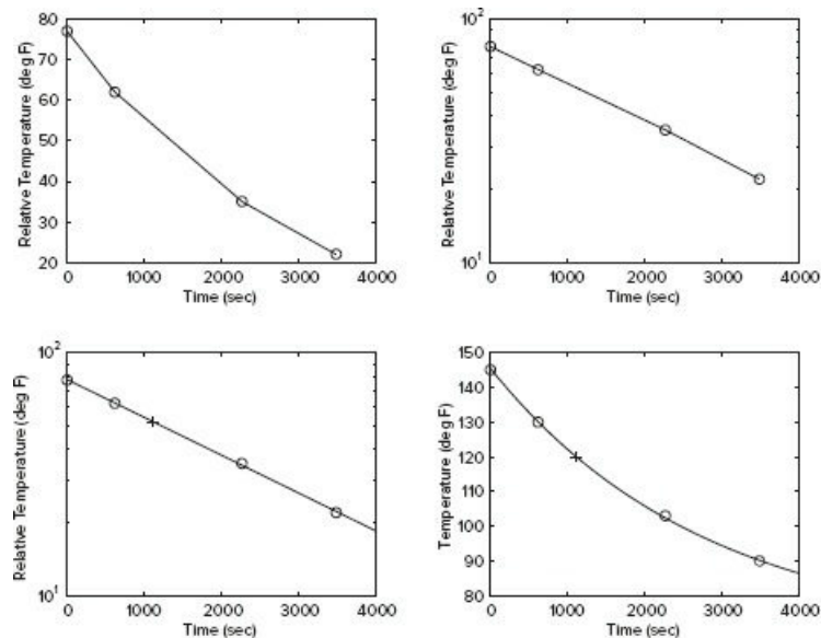
Figure 6.1–4 Temperature of a cooling cup of coffee, plotted on various coordinates.
