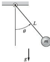
Figure 10.6-1 A pendulum.
