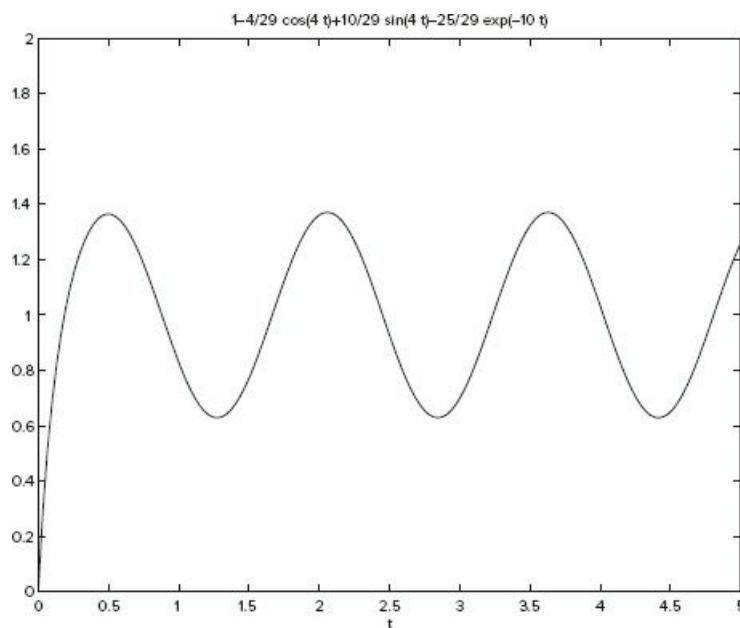
Figure 11.4-1 Plot of the solution of \dot{y} + 10y = 10 + 4 \sin 4t , y(0) = 0 .
