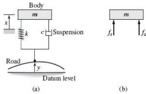
Figure 10.9-1 Single-mass model of a vehicle suspension.
