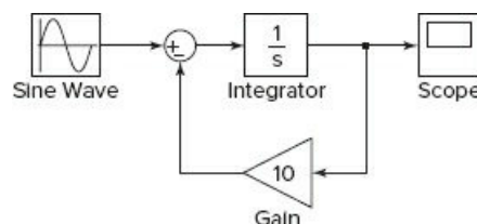
Figure 10.2-6 Simulink model for \dot{y} = -10y + f(t) .
