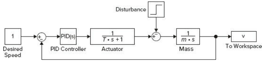
Figure 10.10-5 Simulink model of a speed control system using one block each for actuator and mass.
