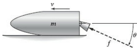
Figure 10.4-2 A rocket-propelled sled.
