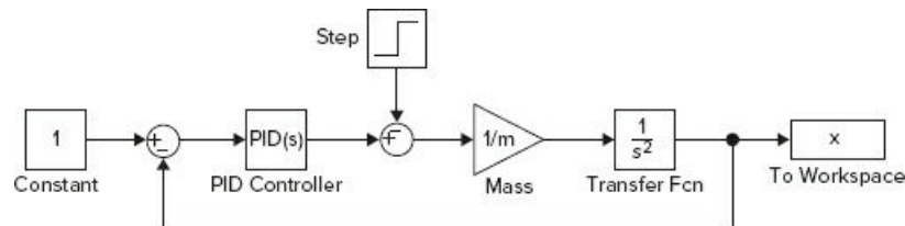
Figure 10.10-6 Simulink model of a simple position control system.
