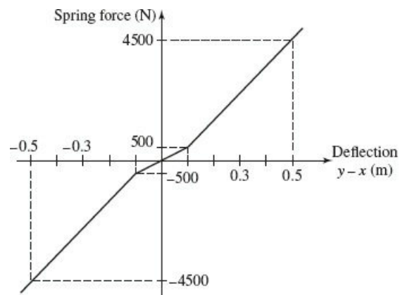
Figure 10.9-2 Nonlinear spring function.
