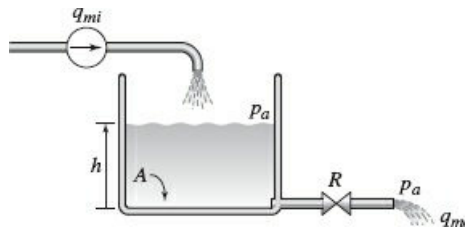
Figure 10.7-1 A hydraulic system with a flow source.
