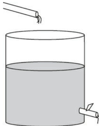
Figure 6.1–5 An experiment to verify Torricelli's principle.
