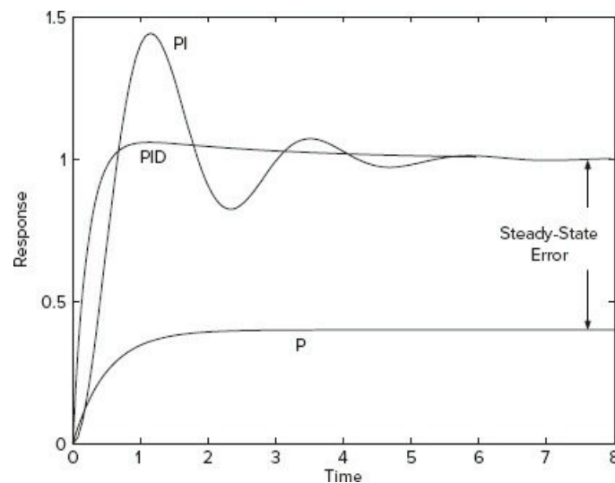
Figure 10.10-2 Typical response of P, PI, and PID control systems when subjected to a unit-step command input.
