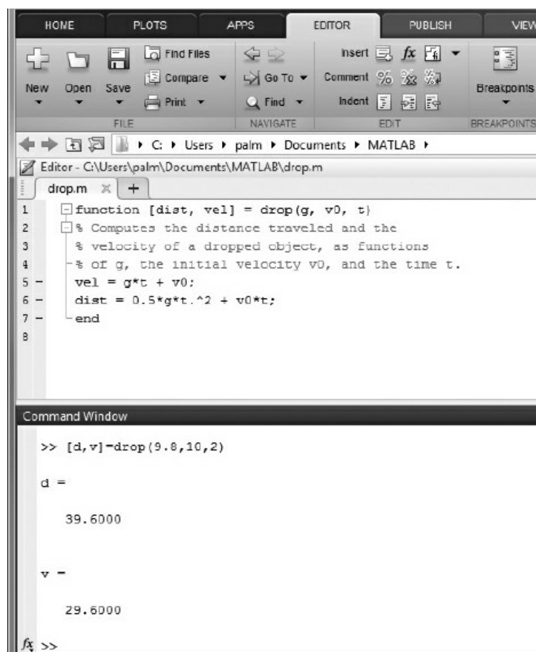
Figure 3.2-2 The Editor after a function has been created. The Command Window shows the results of running
