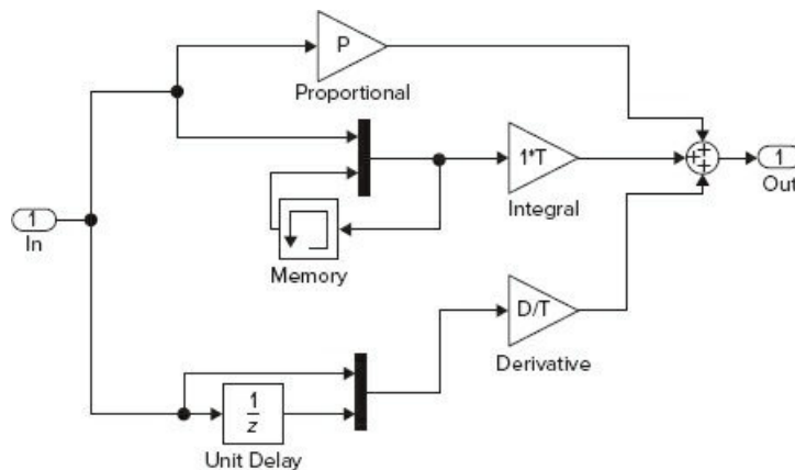
Figure 10.10-7 Simulink diagram of a simplified PID algorithm.
