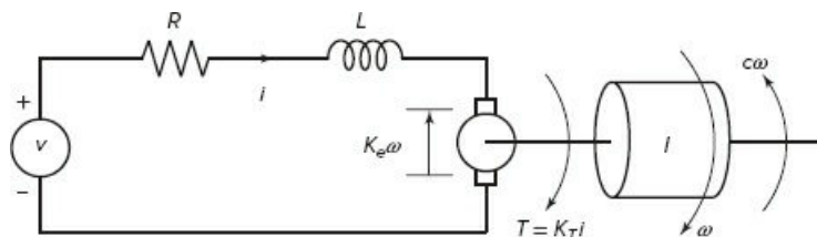
Figure 9.5-4 An armature-controlled dc motor.
