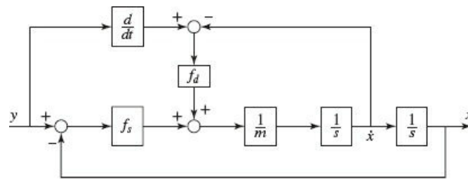
Figure 10.9-5 Simulation diagram of a vehicle suspension model.
