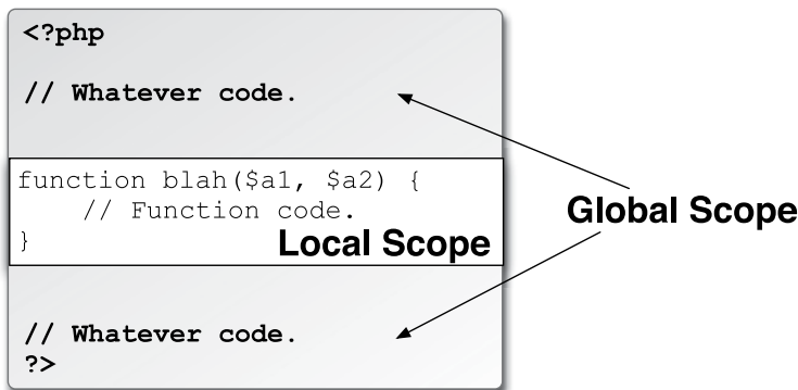
A Adding function definitions to a script adds another area of variable scope.
