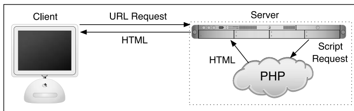
A This graphic demonstrates (albeit in very simplistic terms) how the process works between a client, the server, and a PHP module (an application added to the server to increase its functionality) to send HTML back to the browser.
