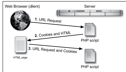
B How cookies are sent back and forth between the server and the client.
