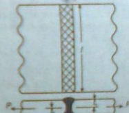
(b) Double V-butt joint.
