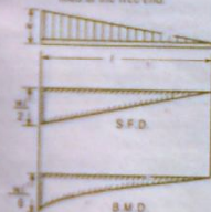
Fig. 2.15. Cantilever beam with gradually varying load.
