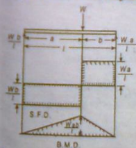
Fig. 2.17. Simply supported beam with an eccentric point load.
