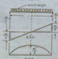
Fig. 2.18. Simply supported beam with a U.D.L.
