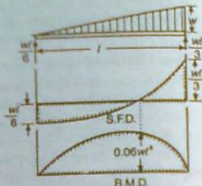
Fig. 2.20 Simply supported beam with a gradually varying load, from zero at one end to w per metre at the other end.
