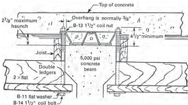
FIGURE 16-4 Hanger for formwork suspended from concrete beams. (Source: Dayton Superior Corporation)
