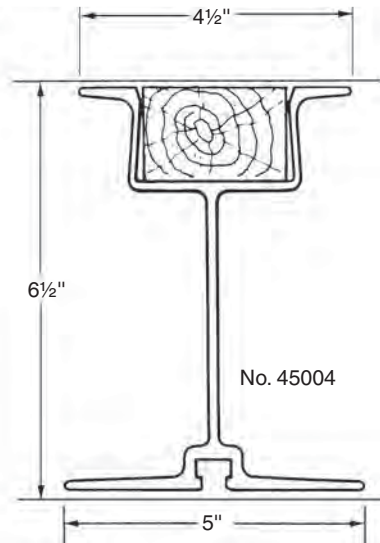
(b) Aluminum joist with wood nailers
