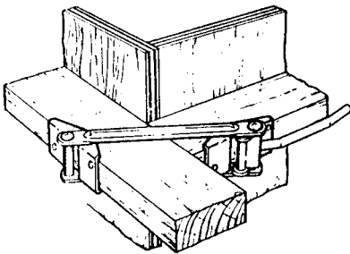
(c) Jahn Cornerlock for securing wales on outside corners of wall forms
