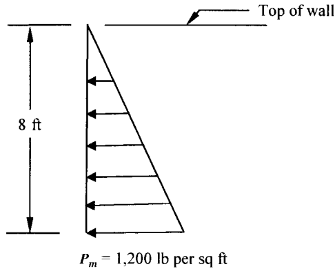
FIGURE 3-3 Distribution of Concrete Pressure for Example 3-2.
