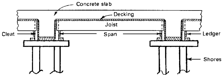
FIGURE 11-2 Forms for concrete beams and slab with single-span joists.
