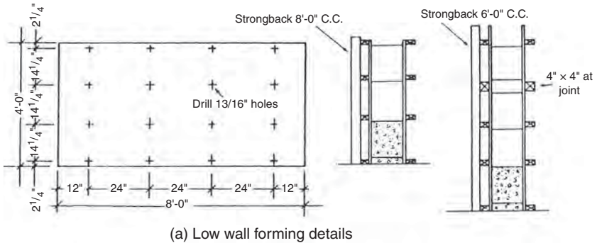
(a) Low wall forming details
