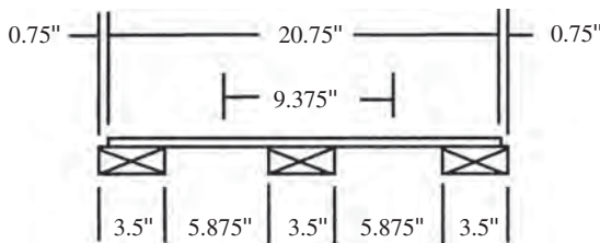
FIGURE 10-3 Plan view of one side of 20-in.-square column form constructed of \frac{3}{4} -in. Plyform with 2 \times 4 vertical battens.
