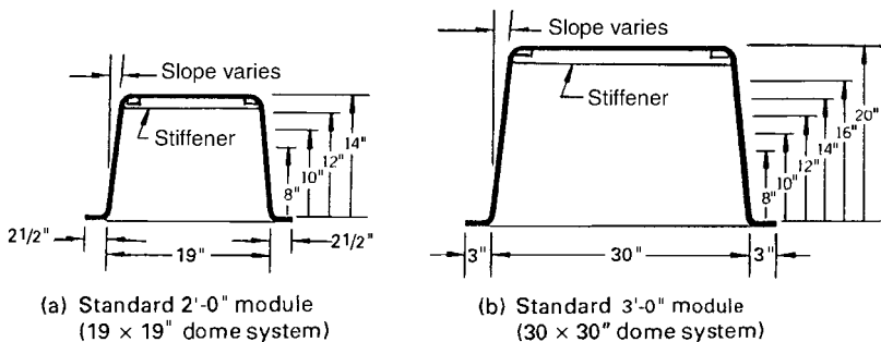
FIGURE 12-7 Ceco Steeldomes. (Source: Ceco Concrete Construction)
