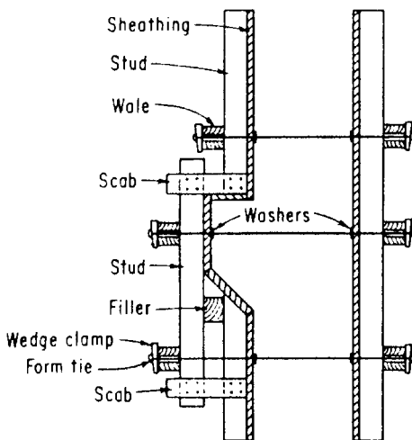
FIGURE 9-8 Forms for walls with corbels.
