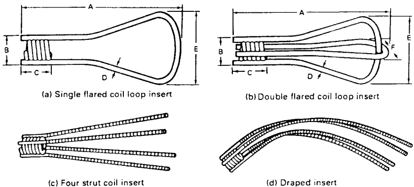
FIGURE 9-17 Coil loop inserts for bolt anchors. (Source: Dayton Superior Corporation)
