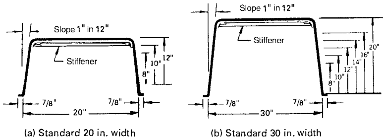
FIGURE 12-1 Typical cross sections of Flangeforms; all dimensions are outside to outside. (Source: Ceco Concrete Construction)
