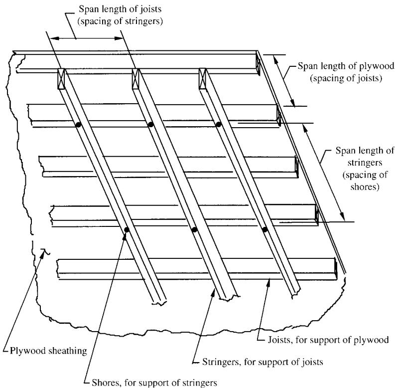
FIGURE 5-18 Allowable span lengths and components of a slab form.
