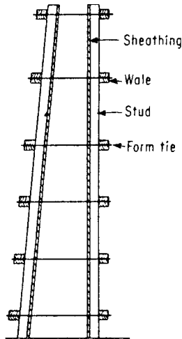
FIGURE 9-6 Forms for walls with batters.
