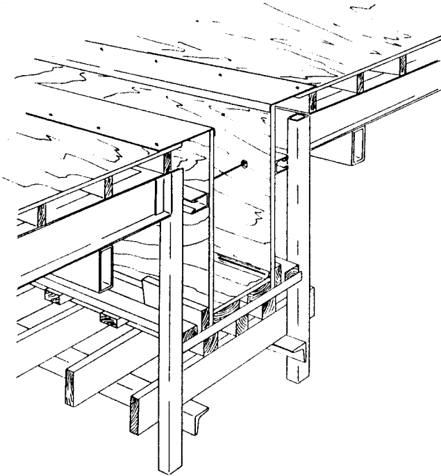
FIGURE 17-9 Representative details for casting a concrete beam in a slab using flying forms. (Source: Form-Eze Systems, Inc.)
