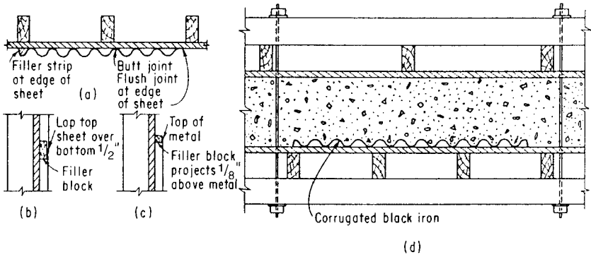
FIGURE 14-8 Fluting formed with corrugated iron. (Source: Portland Cement Association)
