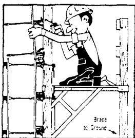
(8) Panels for subsequent lifts are placed by a man on a platform supported by scaffold brackets. These panels can be attached to the strong back with a Strong Back clamp.
