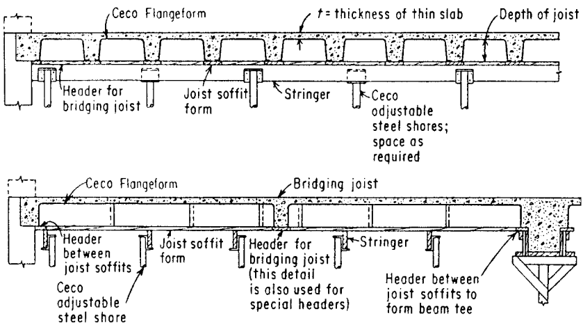
FIGURE 12-2 Installation of concrete floors using Flangeforms; typical arrangement of centering. (Source: Ceco Concrete Construction)
