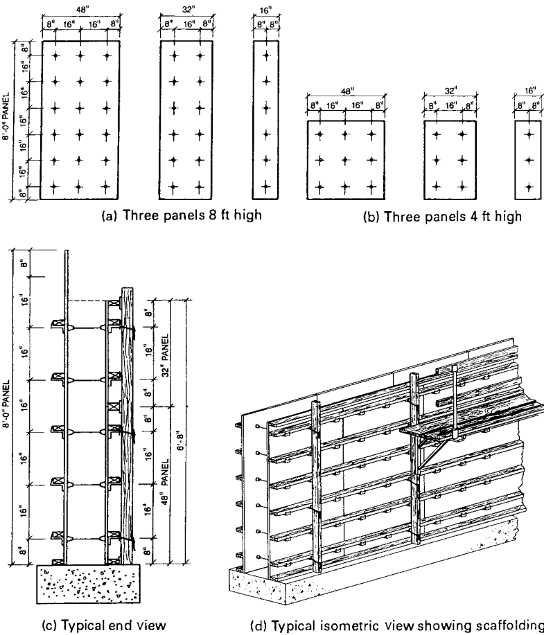
FIGURE 9-21 Suggested form details for 16-in. tie spacing in each direction. (Source: Gates & Sons, Inc.)
