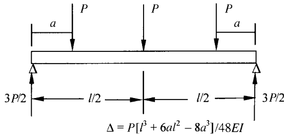
FIGURE 5-5 Single-span beam with three concentrated loads.
