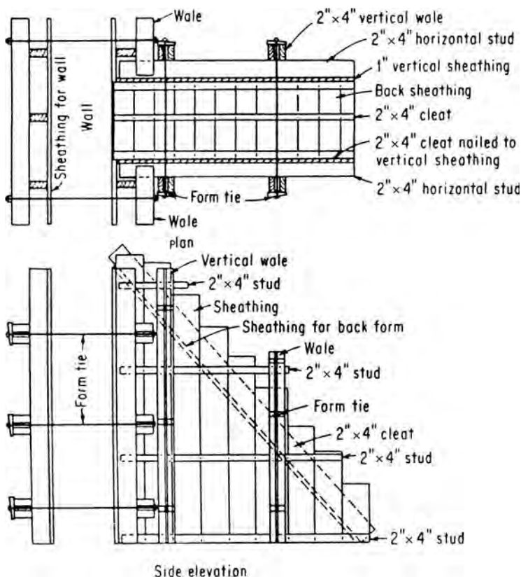
FIGURE 9-10 Forms for wall with counterforts.
