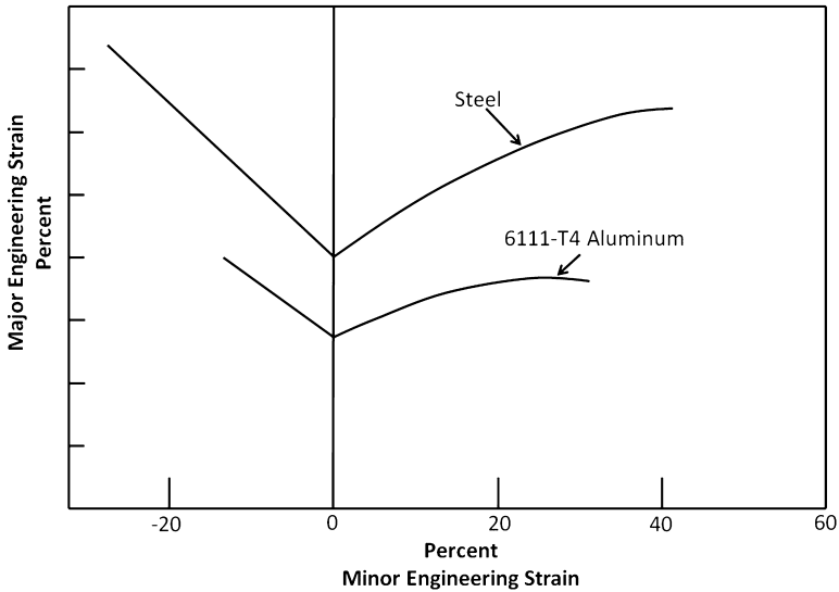
Figure 2.21 The FLD diagrams for steel and aluminum
