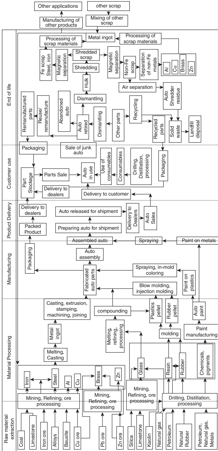
Figure 6.14 The overall material flow within the automotive manufacturing chain
