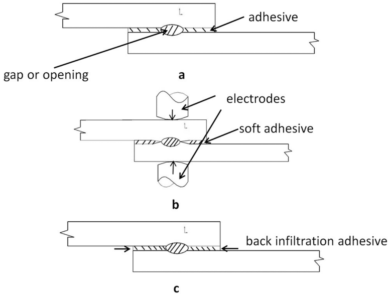
Figure 3.40 A typical example of the weld bonding process
