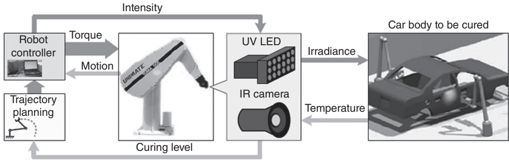
Figure 4.15 The proposed UV curing system
