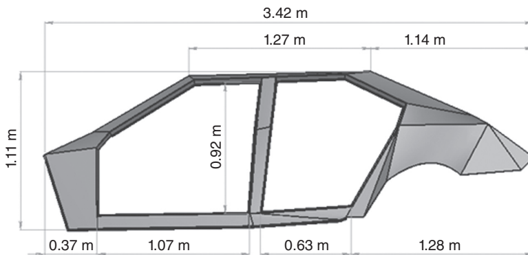
Figure 2.64 Dimensions of the BiW
