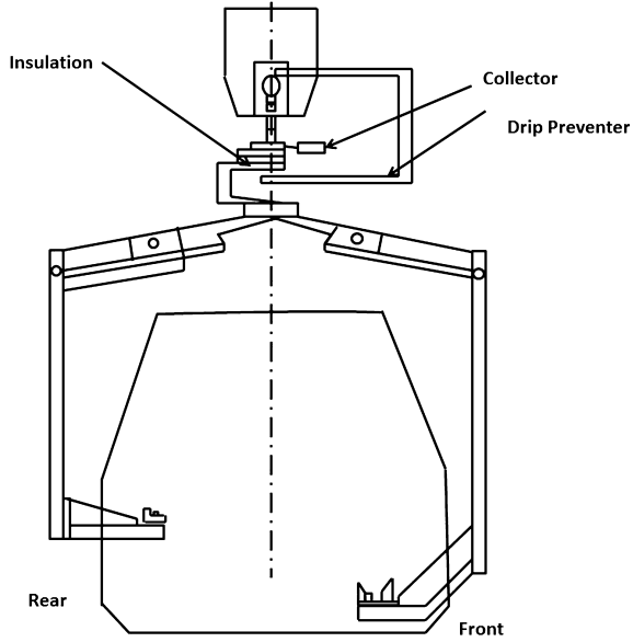
Figure 4.31 The E-coat hanger system
