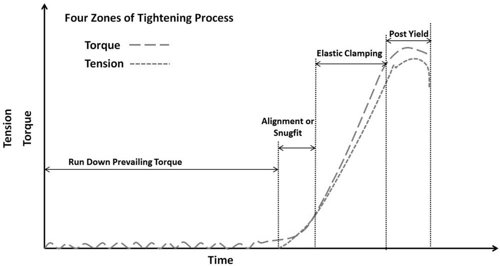
Figure 5.6 The torque-tension evolution with time inside a mechanical joint
