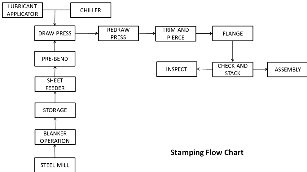
Figure 2.1 The sequence and basic steps in the stamping line
