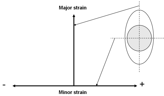
Figure 2.18 The plotting of the FLD strain points from the CGA; major and minor strains
