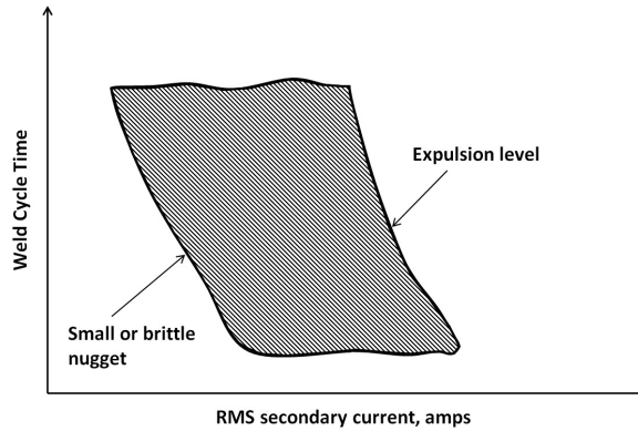
Figure 3.19 The spot welding lobe
