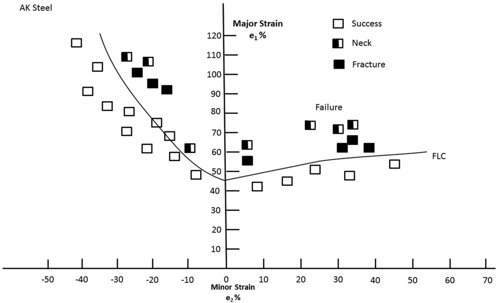
Figure 2.19 A typical FLD diagram for an automotive stamped panel
