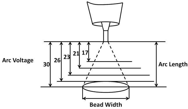
Figure 3.3 The effect of tip distance on the weld bead width
