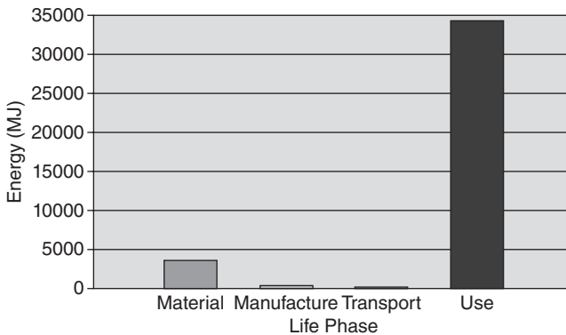
Figure 6.33 The energy consumed for each life phase, lightweight vehicle
