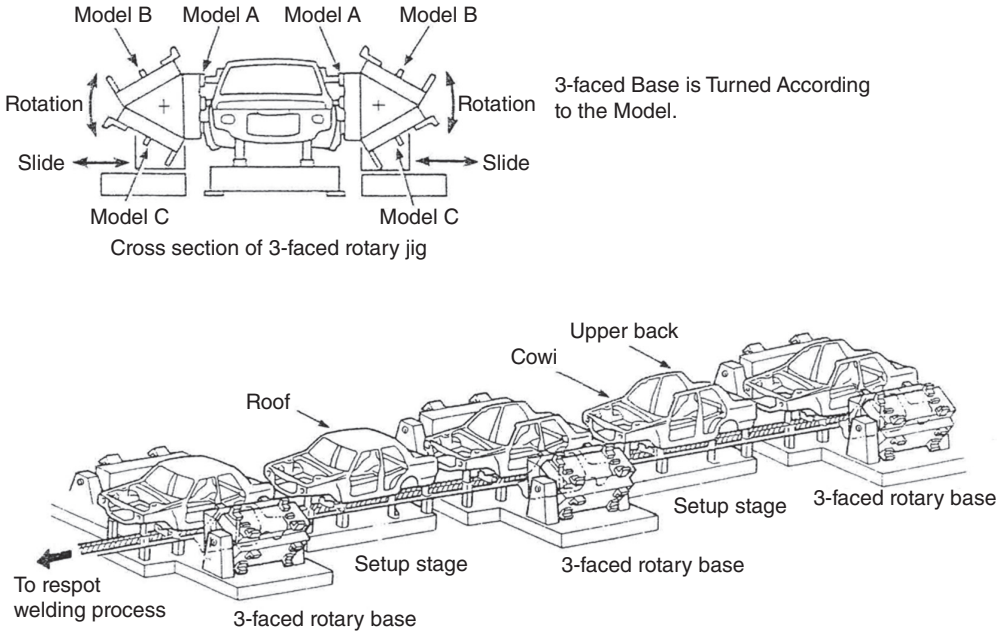
Figure 3.27 The Robotgate fixture systems
