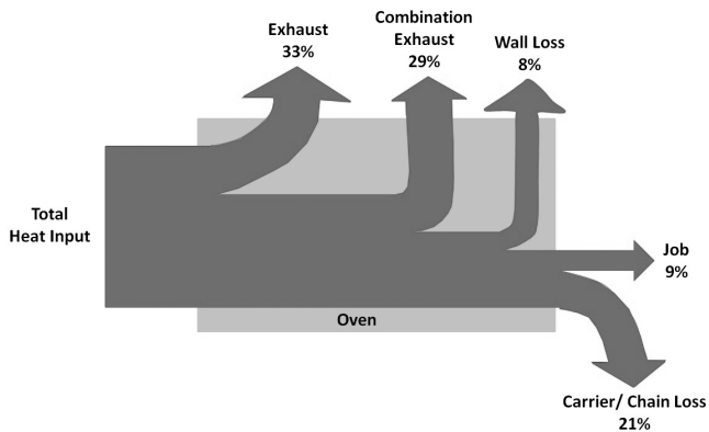
Figure 6.24 Energy distribution for a typical paint curing oven
