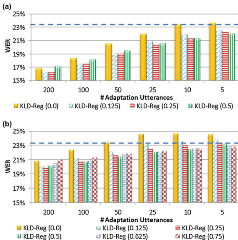
Fig. 11.17 WERs on the SMD dataset using KLD regularized adaptation for different regularization weights \lambda ( numbers in parentheses ). The dashed line is the SI DNN baseline. (Figure from Yu et al. [43]). a Supervised adaptation. b unsupervised adaptation
