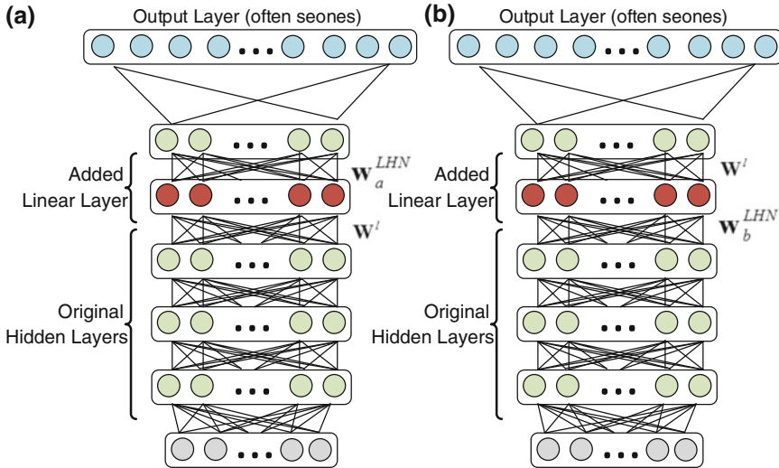
Fig. 11.3 Illustration of the linear hidden network (LHN). The linear transformation can be applied after (a) or before (b) the original weight matrix \mathbf{W}^\ell at hidden layer \ell is applied
