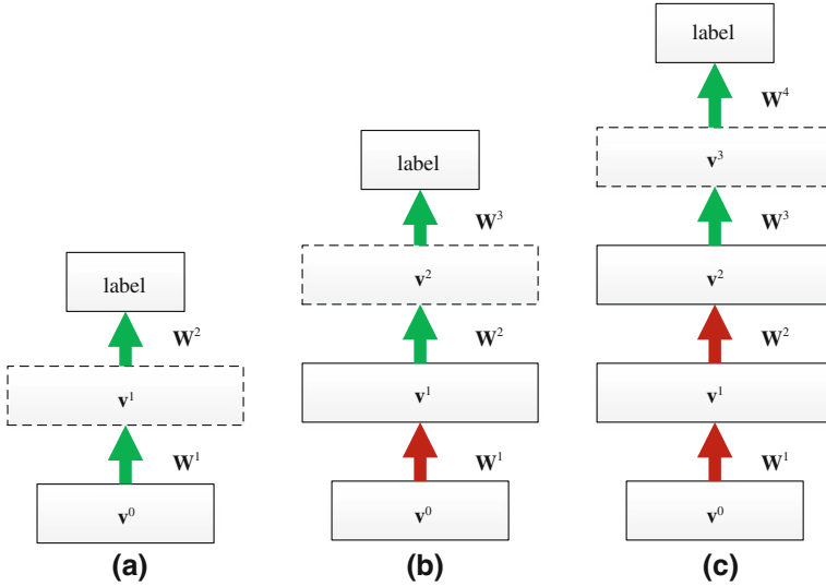
Fig. 5.7 Discriminative pretraining of DNNs
