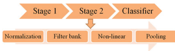
Fig. 9.7 A general framework of feature processing. In the figure, three stages are shown, each of the stage involves four optional steps
