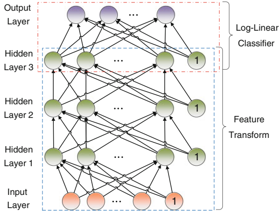
Fig. 9.2 DNN: A joint feature representation and classifier learning view
