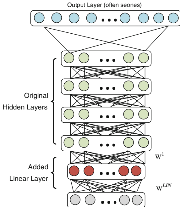
Fig. 11.1 Illustration of the linear input network (LIN) and feature discriminative linear regression (fDLR) adaptation techniques. A linear layer is inserted right above and applied upon the input feature layer
