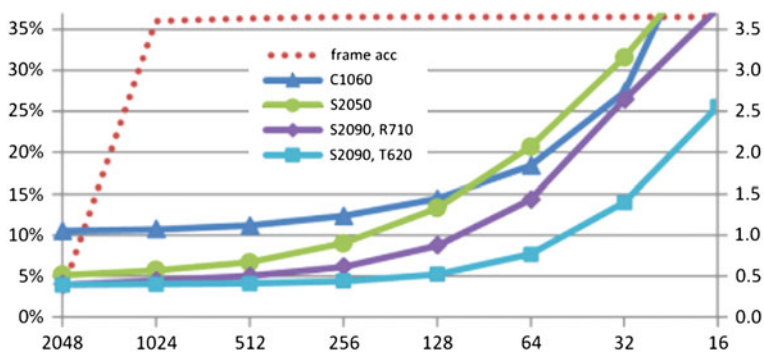
Fig. 7.1 Relative runtime for different minibatch sizes and GPU/CPU model types, and corresponding frame accuracy measured after seeing 12 h of data. Left y-axis frame accuracy; right y-axis runtime relative to C1060 with minibatch size of 2,048 (Figure from Chen et al. [5], permitted to use by ISCA)
