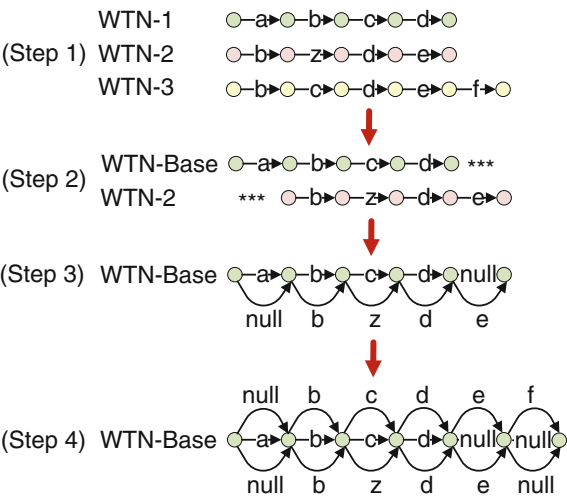
Fig. 10.3 Illustration of the word transition network (WTN) composition procedure. In Step 1 , a linear WTN is generated for each ASR result. In Step 2 , WTN-1 is selected as the base WTN to which WTN-2 is aligned. WTN-2 is merged into the base WTN in Step 3 . In Step 4 , WTN-3 is further merged into the base WTN
