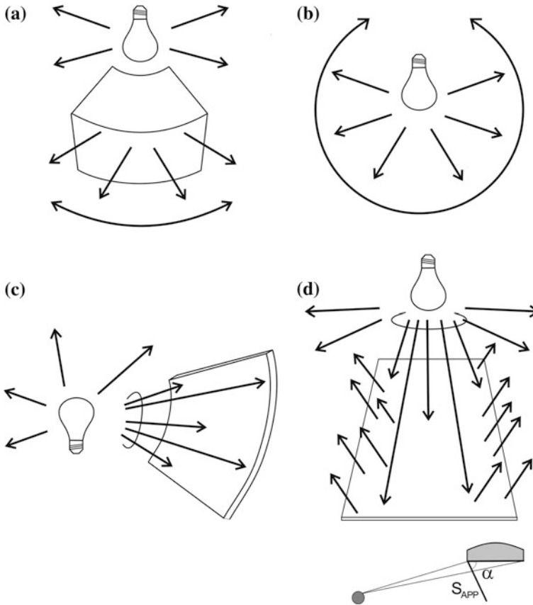
Fig. 12.5 Fotometric quantities: (a) Luminous Intensity, (b) Luminous Flux, (c) Illuminance, (d) Luminance
