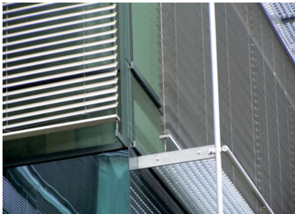
Fig. 13.11 Example of solar shading systems
