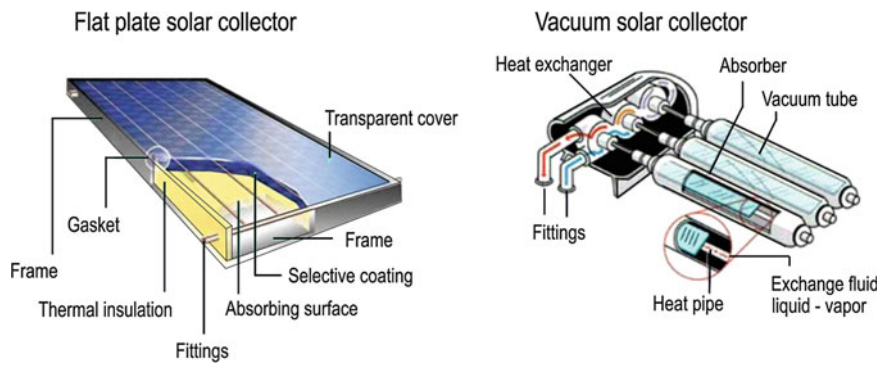
Fig. 13.20 Example of solar collectors: flat plate collector (on the left ), vacuum solar collector (on the right )
