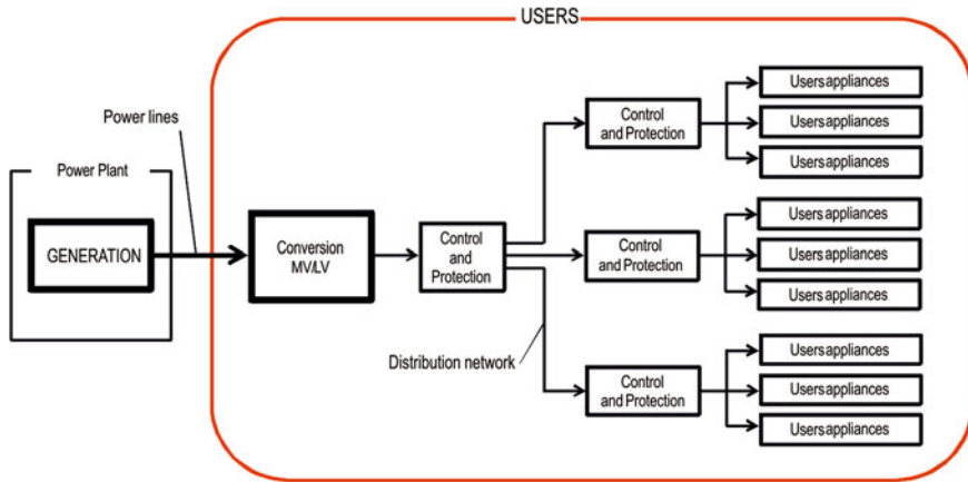
Fig. 8.7 Schematic diagram of an electrical system, from the generation to the user appliances
