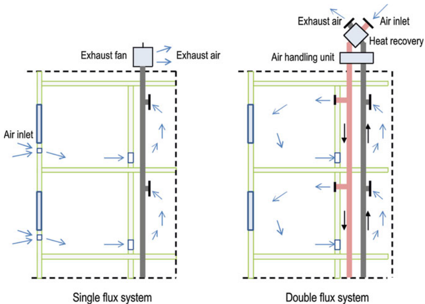
Fig. 13.16 Typical schemes of mechanical ventilation systems
