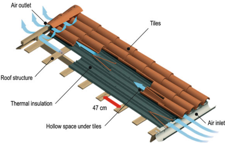
Fig. 13.2 Example of a ventilated roof system (courtesy of Onduline Co.)
