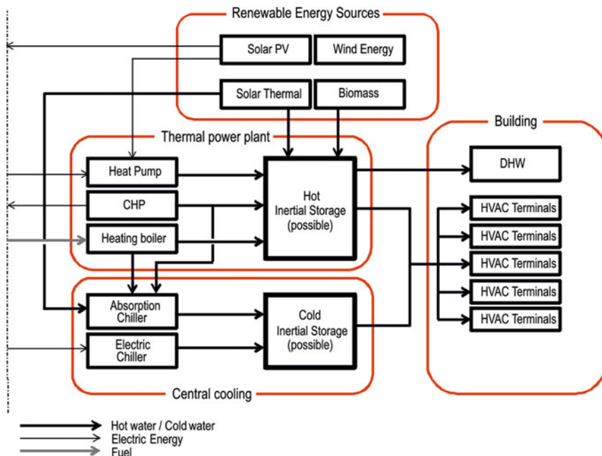
Fig. 8.3 Schematic diagram of a HVAC and DHW integrated system
