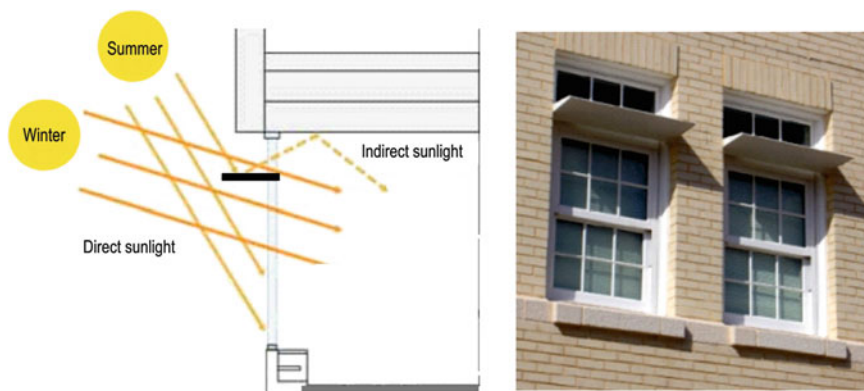
Fig. 13.13 Example of an application of light shelves
