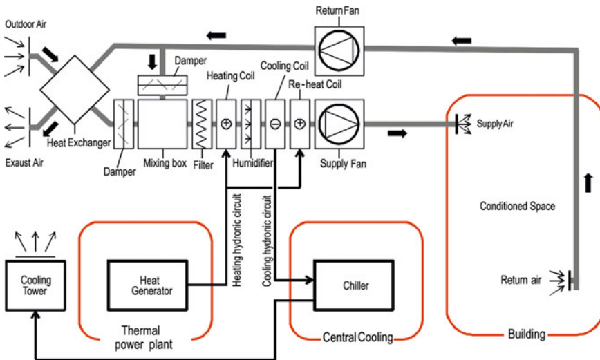
Fig. 8.5 Schematic diagram of a full air HVAC system
