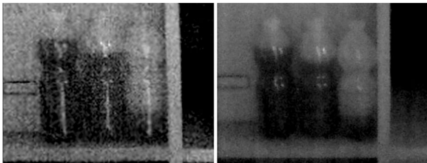
Fig. 6.4 Same scene, different IR camera Thermal Resolution. The coarse-grained thermal image on the left was taken by an IR camera with a NETD value lower than the one on the right . Therefore, the instrument choice directly depends on the objective needs of the professional
