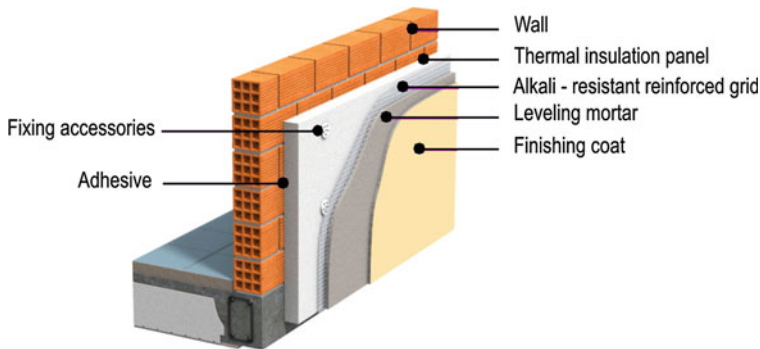
Fig. 13.7 Example of an external thermal insulation composite system (ETICS) (courtesy of Knauf Co.)
