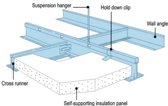
Fig. 13.6 Example of a suspended false ceiling (courtesy of Shakti ceiling Systems Co.)
