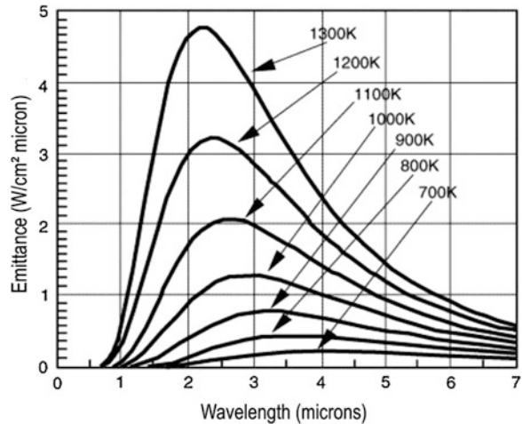
Fig. 6.2 Blackbody spectral radiant emittance
