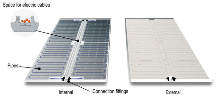
Fig. 13.18 Example of prefabricated radiant panel for ray conditioning applications (courtesy of Messina Co.)
