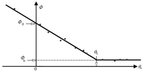
Fig. 5.27 Example of energy signature: the graph constructed on the basis of actual consumption and outside temperature of a heating system (Source EN 15603)
