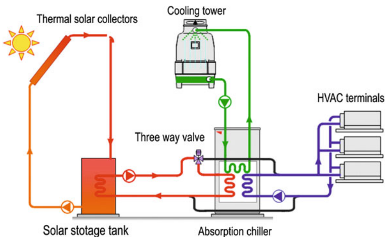
Fig. 13.21 Typical scheme of a solar cooling system (courtesy of Yazaki Co.)
