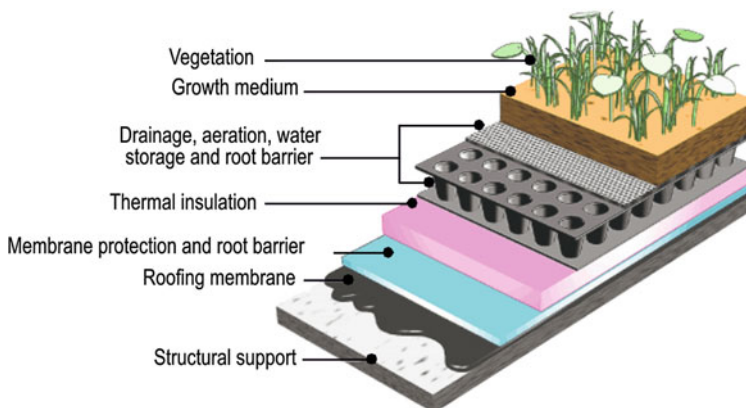
Fig. 13.5 Example of green roof system (courtesy of Heart Pledge Co.)
