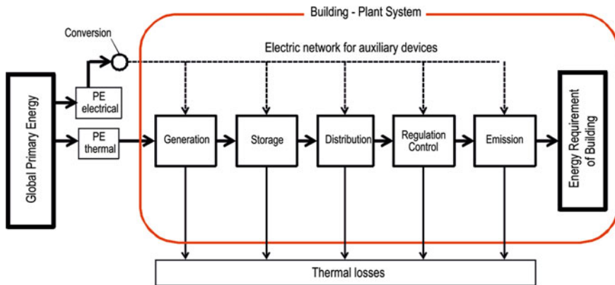
Fig. 8.4 Schematic diagram the subsystem sequence in a HVAC system
