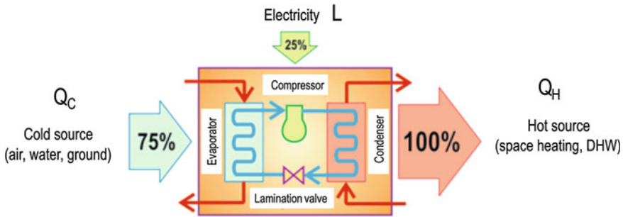
Fig. 13.15 A simple stylised diagram of a heat pump's vapour compression refrigeration cycle
