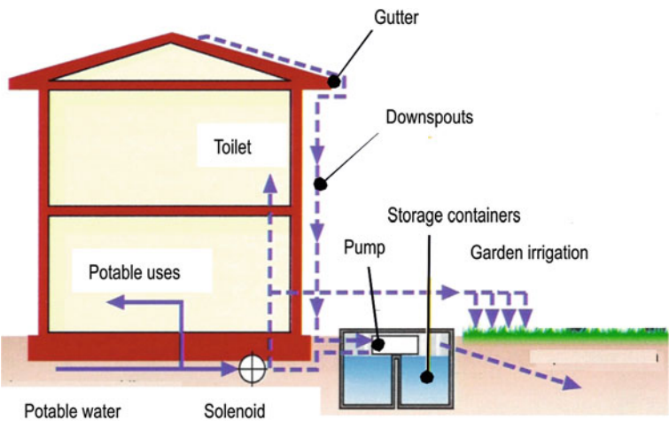
Fig. 13.19 Schematic example of a rainwater harvesting system
