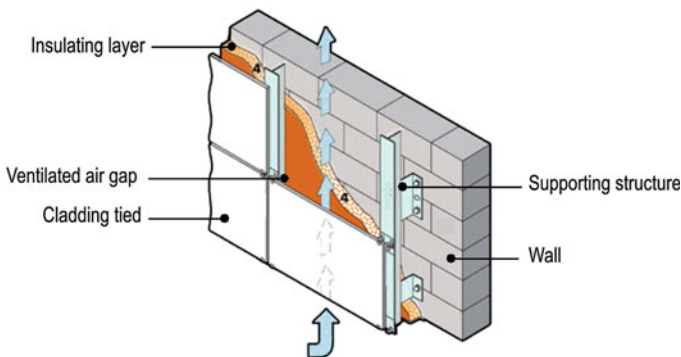
Fig. 13.8 Example of a ventilated façade (courtesy of Grantec Co.)
