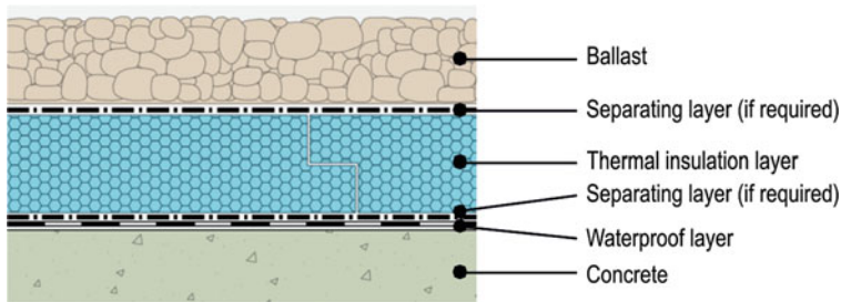
Fig. 13.4 Example of an inverted roof system (courtesy of Dow Corp.)
