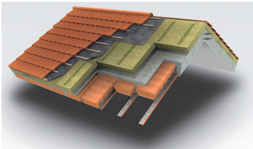
Fig. 13.1 Example of extrados insulation, insulating under the tiles (courtesy of Rockwool Co.)
