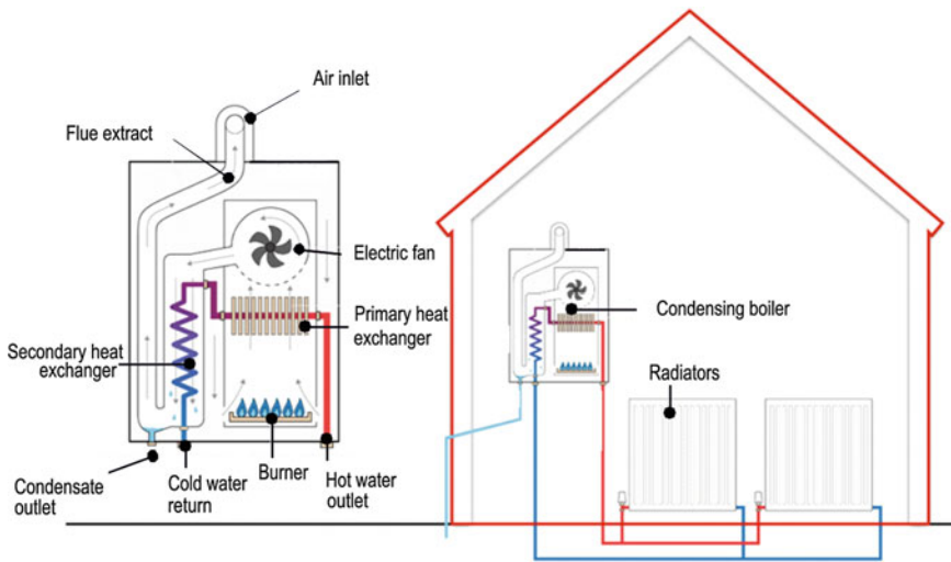
Fig. 13.14 Scheme of a condensing boiler and of a heating system (source: http://www.evoenergy.co.uk )
