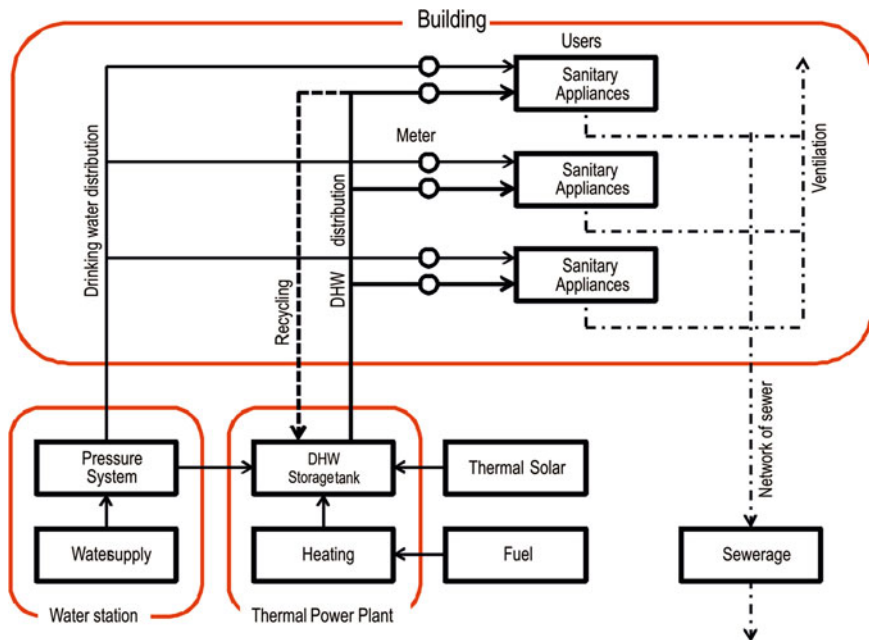
Fig. 8.6 Schematic diagram of a DHW system
