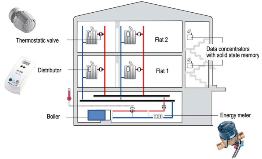
Fig. 13.17 Typical schemes of an individual energy accounting system
