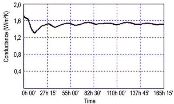
Fig. 5.13 Processing of information acquired by a heat flow meter
