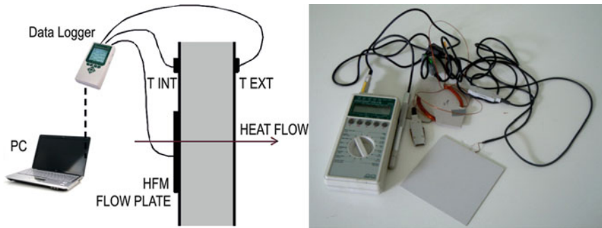
Fig. 5.12 Installation scheme of a heat flow meter and example of a flow meter
