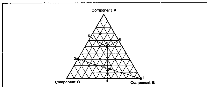
Fig. 2-25. Ternary diagram.
