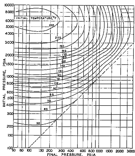
Fig. 17-13. Permissible expansion of 0.9 specific gravity gas without hydrate formation. (Katz, Trans. , AIME, 160, 140. Copyright 1945 SPE-AIME.)
