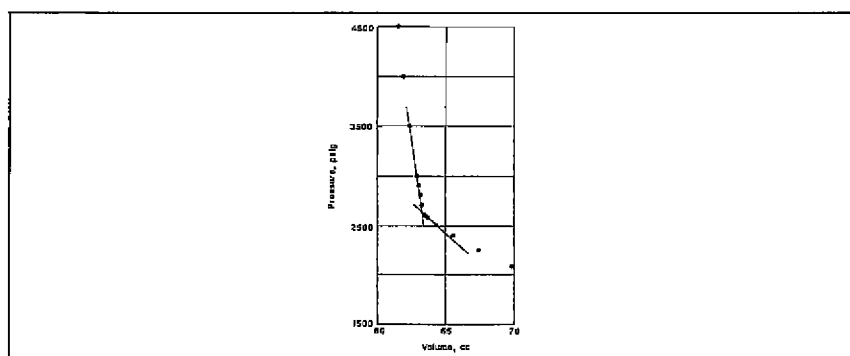
Fig. 10-2. Determination of bubble-point pressure with data from flash vaporization.
