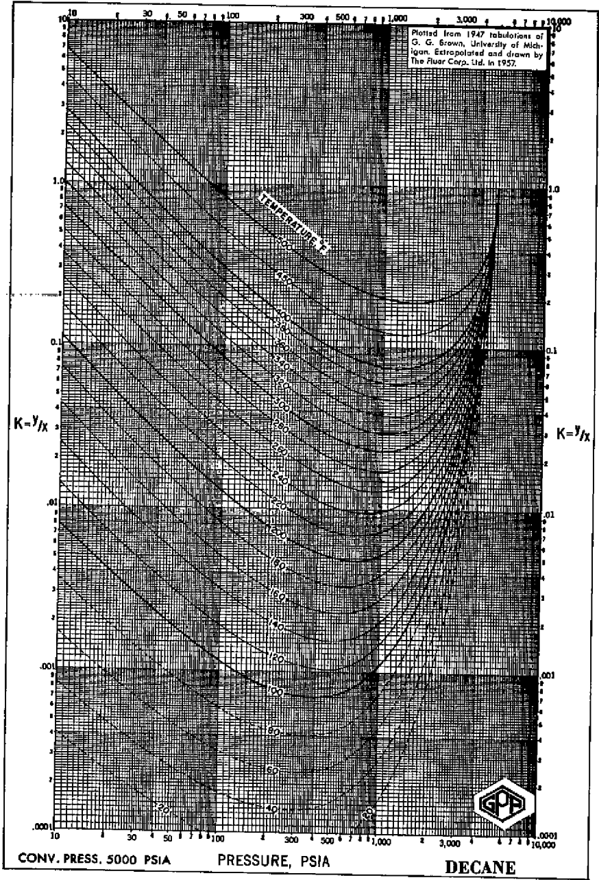
Fig. A-12. Equilibrium ratios for decane in a 5000 psia convergence pressure system. ( Engineering Data Book , 10th Ed., GPSA, Tulsa, 1987, with permission.)
