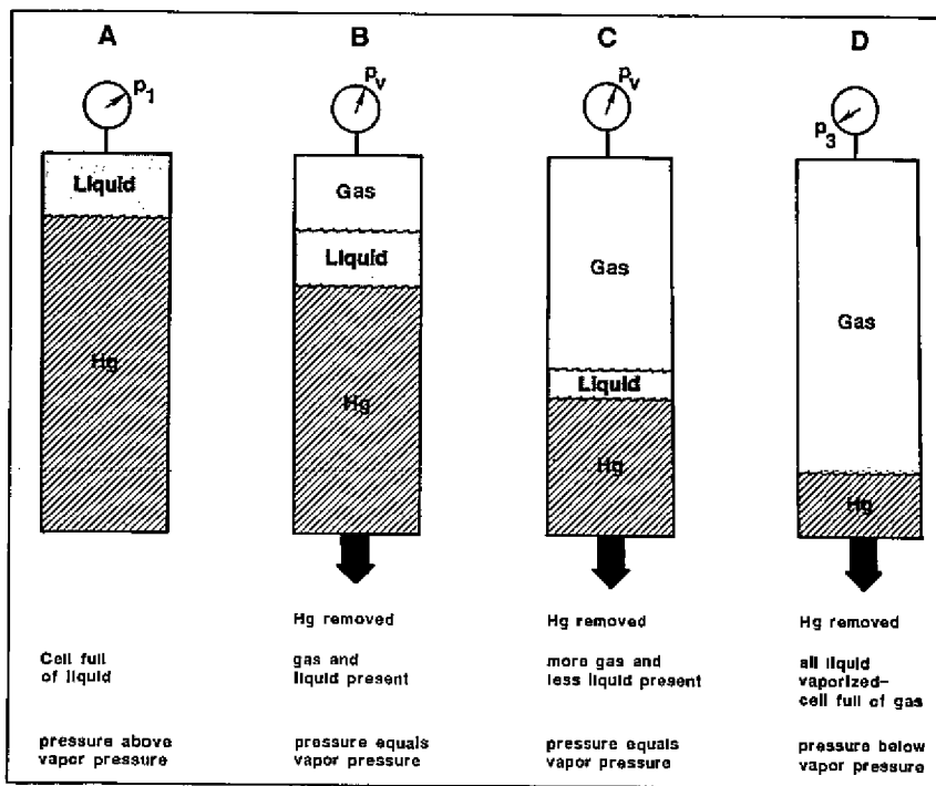
Fig. 2-2. Vaporization of a pure substance at constant temperature.
