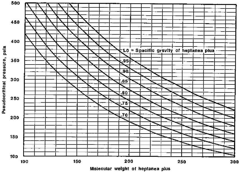
Fig. 3-10. Pseudocritical properties of heptanes plus.
