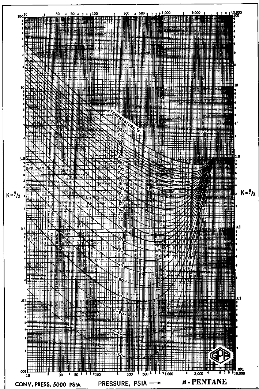
Fig. A-7. Equilibrium ratios for n-pentane in a 5000 psia convergence pressure system. ( Engineering Data Book , 10th Ed., GPA, Tulsa, 1987, with permission.)
