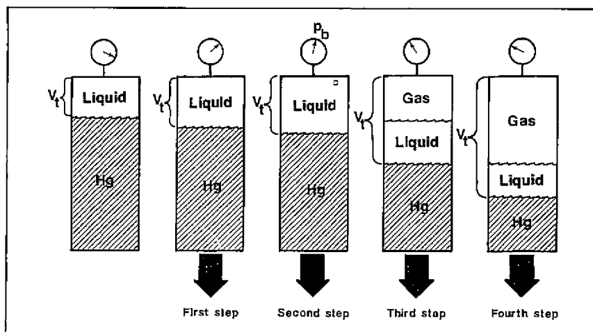
Fig. 10-1. Laboratory flash vaporization procedure.
