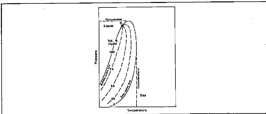
Fig. 2-17. Typical phase diagram of a two-component mixture with definitions of cricondenbar and cricondentherm.
