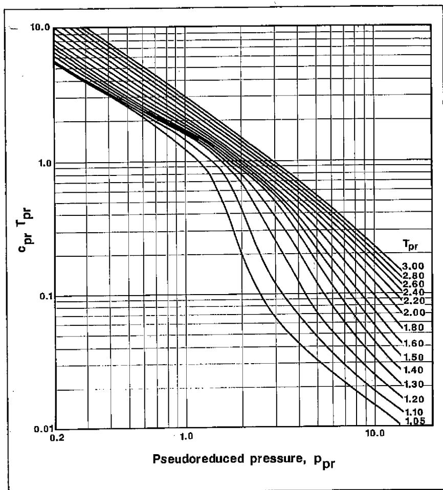
Fig. 6-4. Pseudoreduced compressibilities of natural gases.
