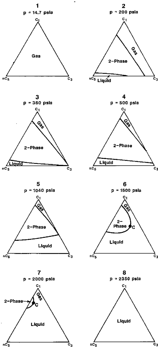
Fig. 2-28. Ternary phase-diagrams of mixtures of methane, propane, and n-pentane at 160°F and various pressures, showing typical changes in shapes of the diagrams as pressure is changed. (Diagram numbers are keyed to the numbered points on Figure 2-29.)
