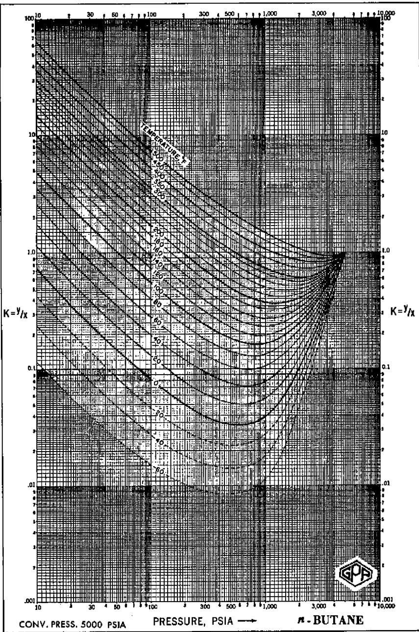
Fig. A-5. Equilibrium ratios for n-butane in a 5000 psia convergence pressure system. ( Engineering Data Book , 10th Ed., GPA, Tulsa, 1987, with permission.)
