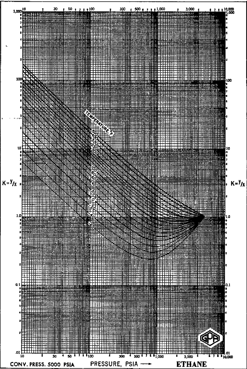
Fig. A-2. Equilibrium ratios for ethane in a 5000 psia convergence pressure system. ( Engineering Data Book , 10th Ed., GPSA, Tulsa, 1987, with permission.)
