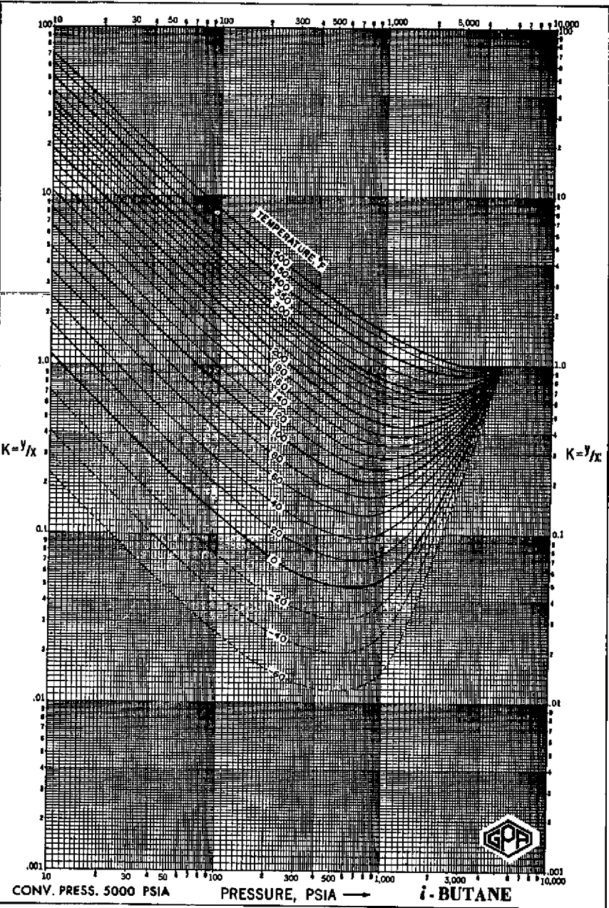
Fig. A-4. Equilibrium ratios for i -butane in a 5000 psia convergence pressure system. ( Engineering Data Book , 10th Ed., GPSA, Tulsa, 1987, with permission.)
