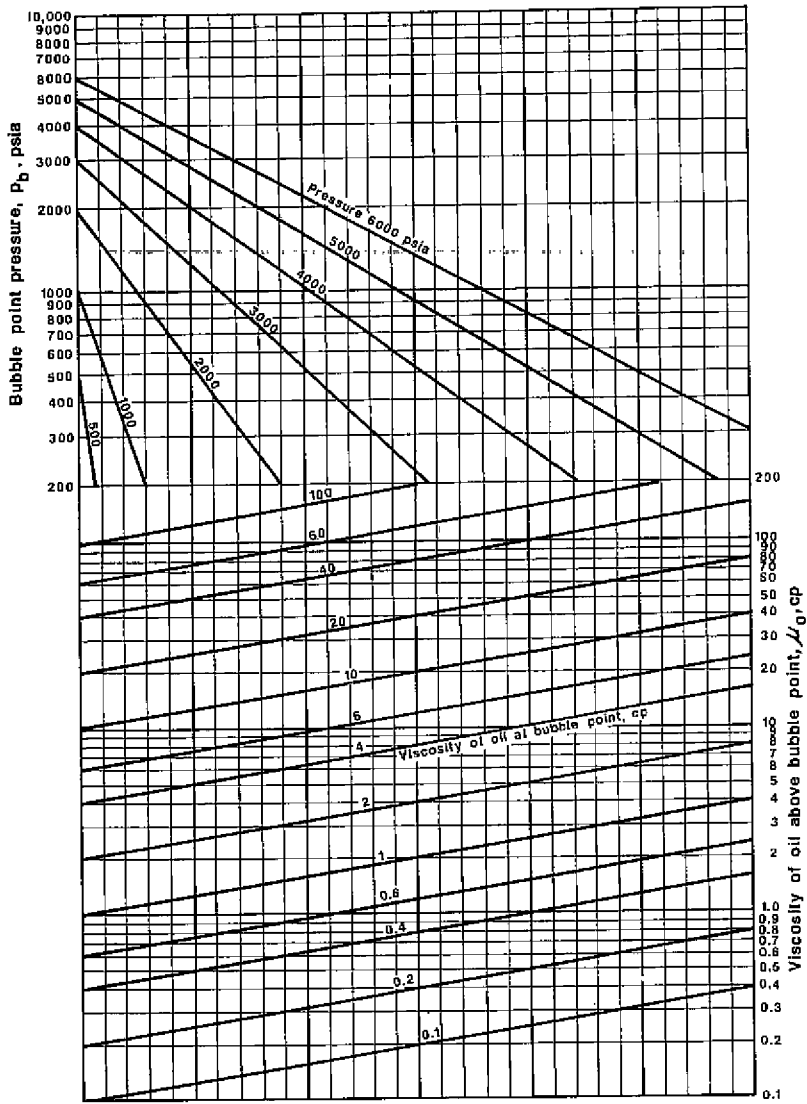
Fig. 11-15. Viscosities of undersaturated black oils.
