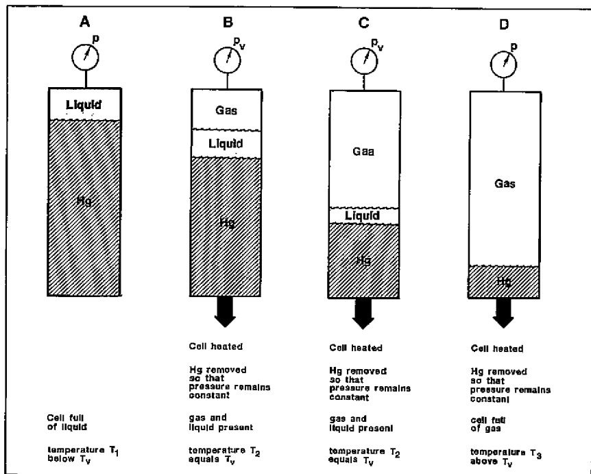
Fig. 2-5. Vaporization of a pure substance at constant pressure.
