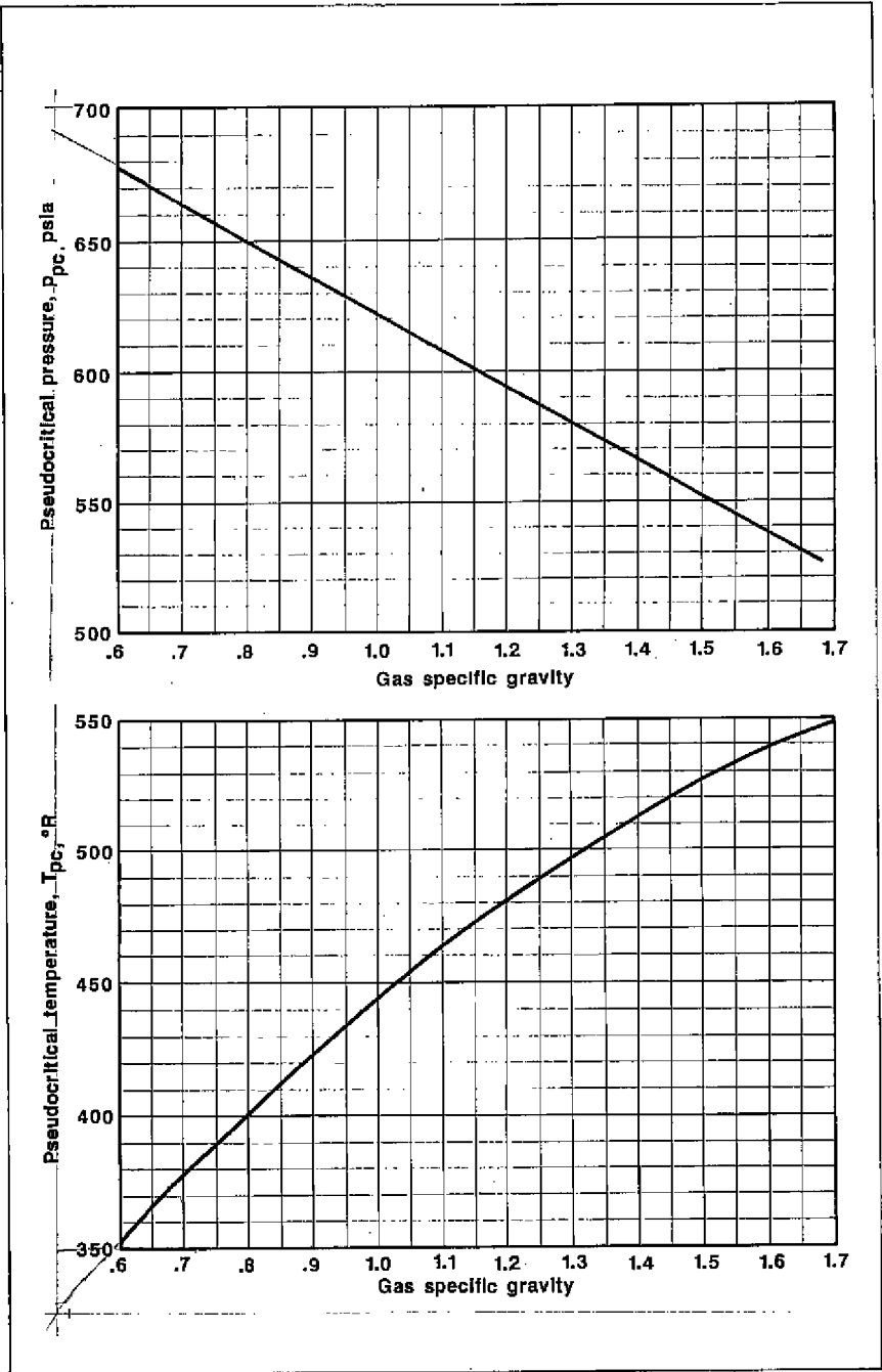
Fig. 3-11. Pseudocritical properties of natural gases.
