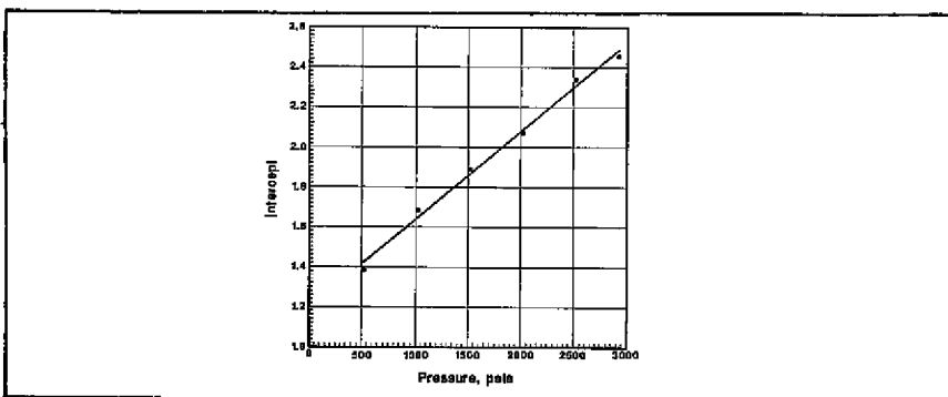
Fig. 14–11. Intercepts of pK plots vs. pressure (part of solution to Example 14–3).
