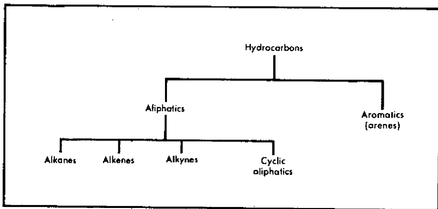
Fig. 1-6. Classes and homologous series of hydrocarbons.
