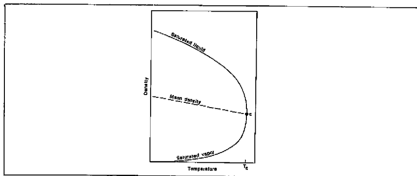
Fig. 2-11. Typical density-temperature diagram of a pure substance.
