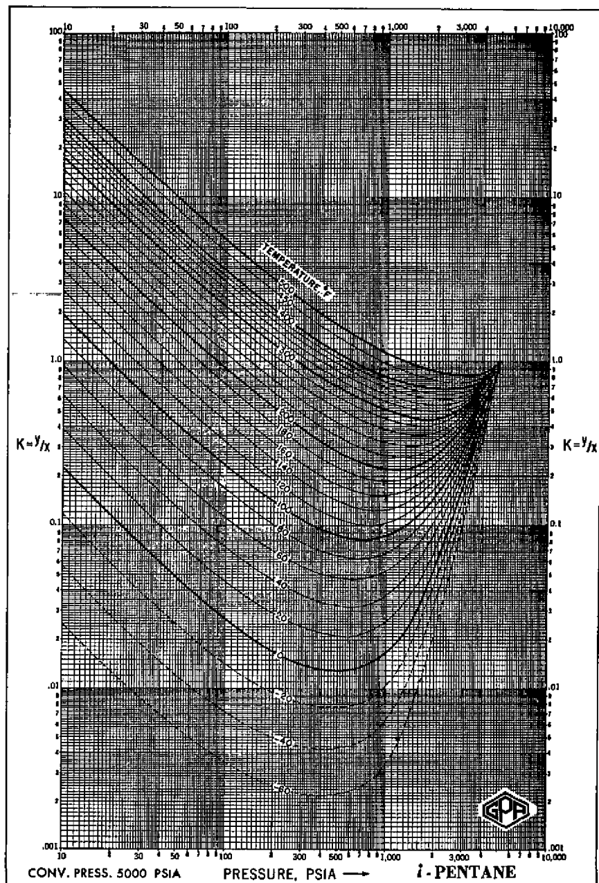
Fig. A-6. Equilibrium ratios for i -pentane in a 5000 psia convergence pressure system. ( Engineering Data Book , 10th Ed., GPSA, Tulsa, 1987, with permission.)
