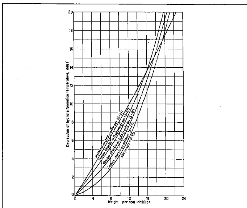
Fig. 17-7. Depression of hydrate-formation temperatures by inhibitors. (From Handbook of Natural Gas Engineering by Katz et al. Copyright 1959 by McGraw-Hill Book Company. Used with permission of McGraw-Hill Book Company.)
