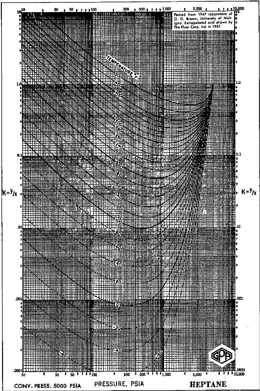
Fig. A-9. Equilibrium ratios for heptane in a 5000 psia convergence pressure system. ( Engineering Data Book , 10th Ed., GPA, Tulsa, 1987, with permission.)
