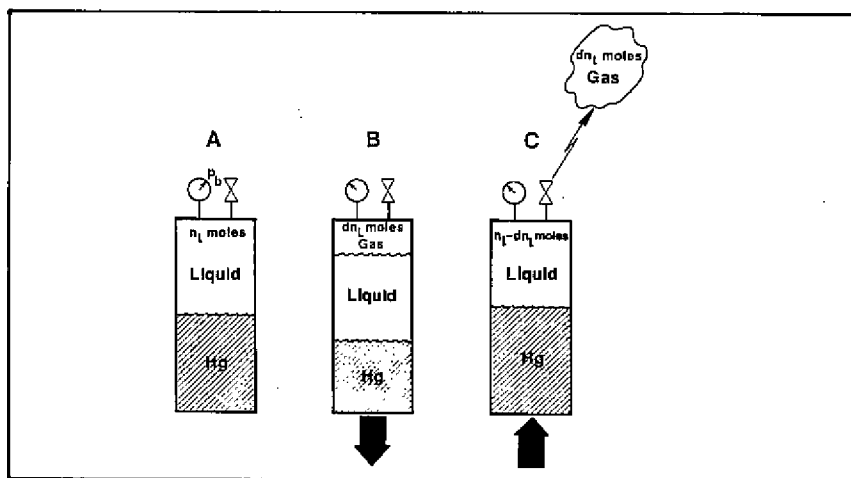
Fig. 12-4. Constant temperature differential vaporization.
