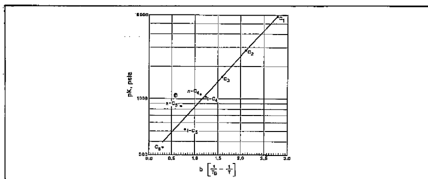
Fig. 14-9. pK_j vs. b(1/T_B - 1/T) (part of solution to Example 14-2).
