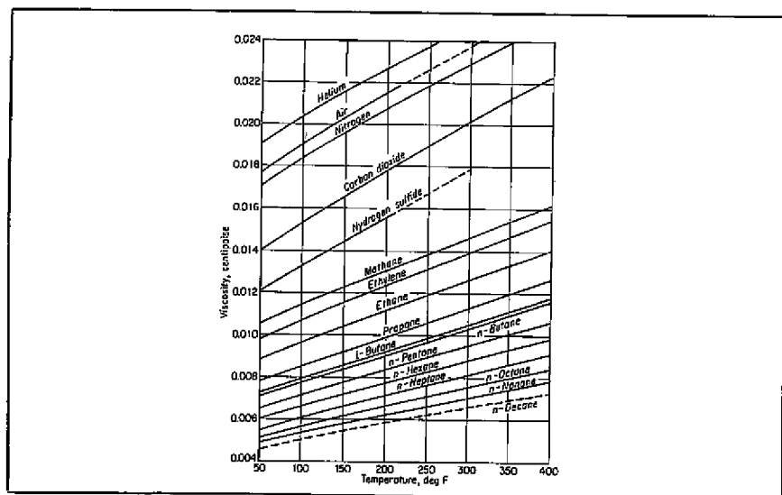
Fig. 6-7. Viscosities of pure gases at atmospheric pressure.
