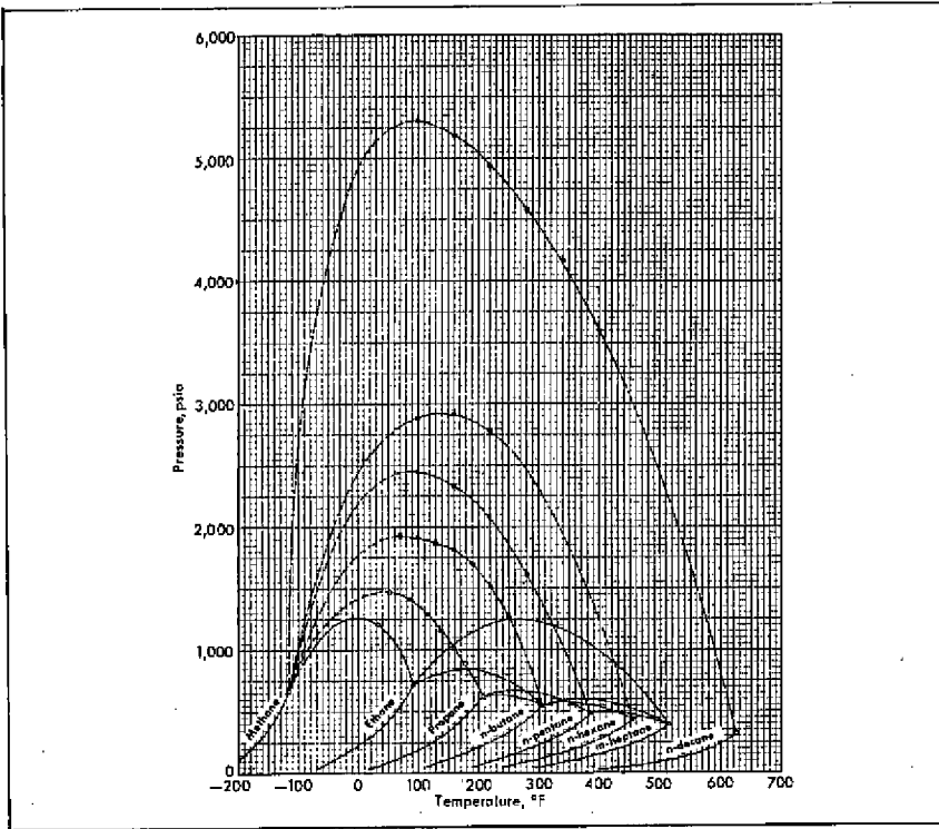
Fig. 2-16. Critical loci of binary n-paraffin mixtures. (Brown et al., Natural Gas and the Volatile Hydrocarbons , NGAA, 1947, 4, with permission.)
