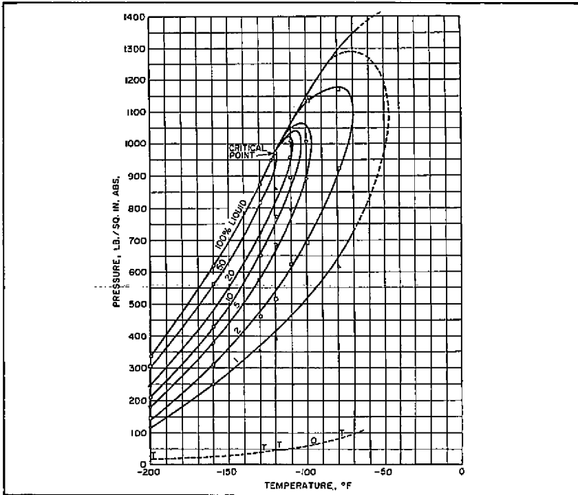
Fig. 2-36. Phase diagram of a reservoir fluid. (Davis et al., Trans. , AIME 201, 245. Copyright 1954 SPE-AIME.)
