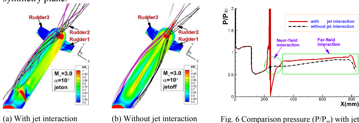
Fig. 5 The surface pressure ( P/P_\infty ) contour and streamlines ( M_\infty=3.0 , P_{0j}=4.0 )
