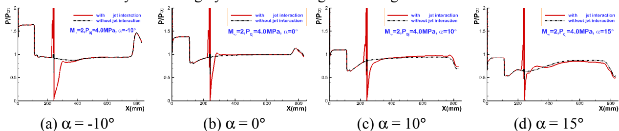
Fig. 8 Comparison with pressure ( P/P_\infty ) with jet interaction and pressure without jet interaction on the nozzle meridian at \alpha is -10^\circ , 0^\circ , 10^\circ , 15^\circ .
