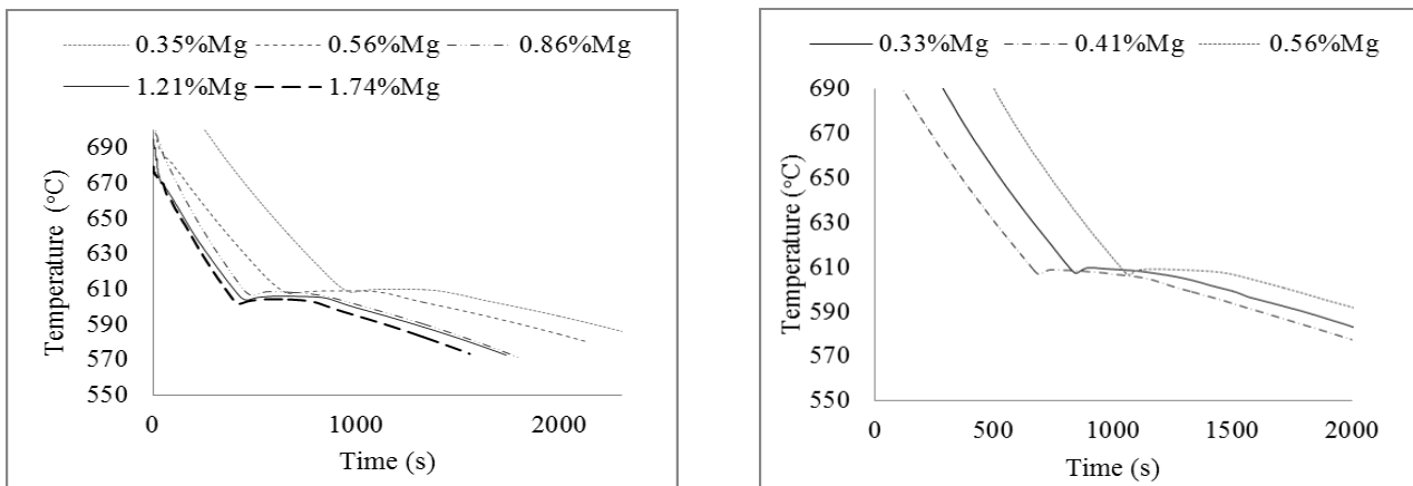
Figure 2 Cooling curves
