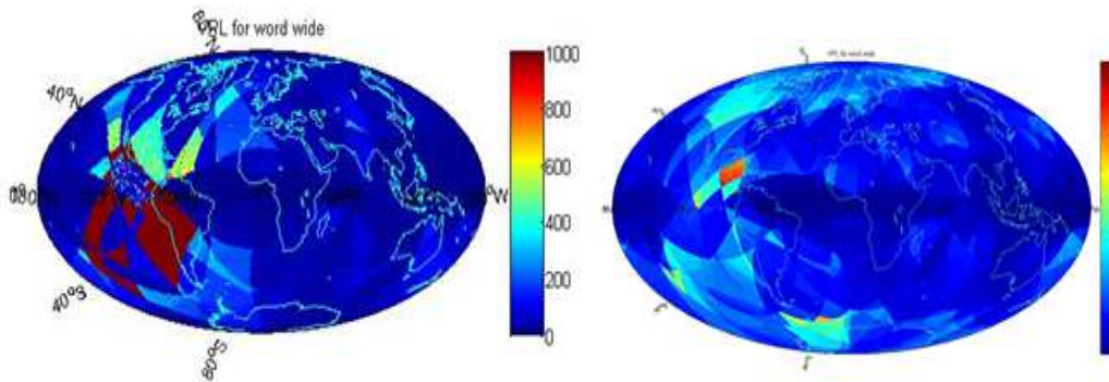
Figure 1 99.5% VPL for RAIM(GPS)
