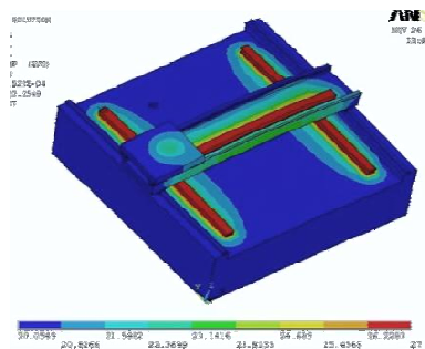
Fig. 3 Temperature distribution
