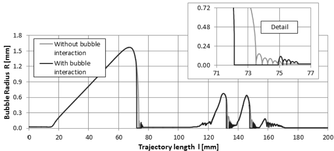
Fig. 4. Dynamics of bubble with initial radius 45 \mu\text{m} . Trajectory from Fig. 3. With bubble breakup.
