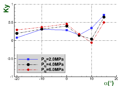
(c) Normal force amplification factor
