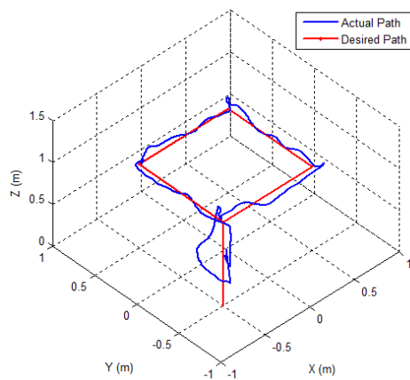
Fig. 4 Position response
