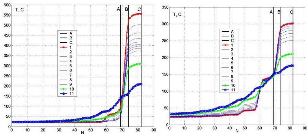
Fig. 4. Temperature distribution at t = 315 s and t = 2200 s ( t > t_{\text{short circuit}} ).
