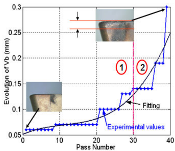
Fig.4 Evolutions of Flank wear V_b
