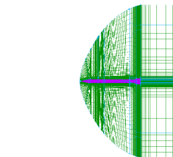
(a) Multi-block grid structure for model
