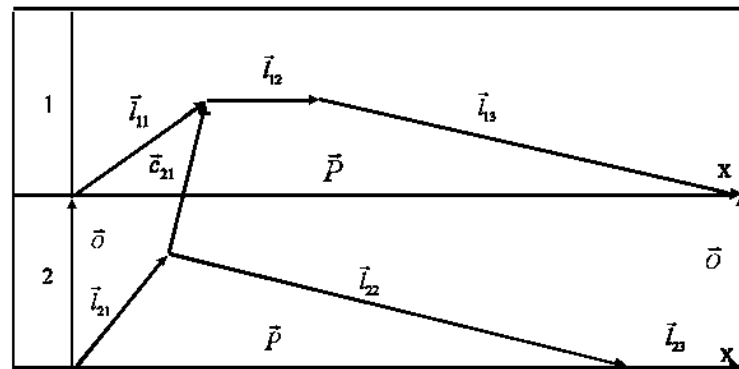
Fig. 3 The vector timing diagram of automatic machine
