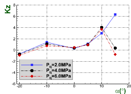
(b) Lateral moment amplification factor
