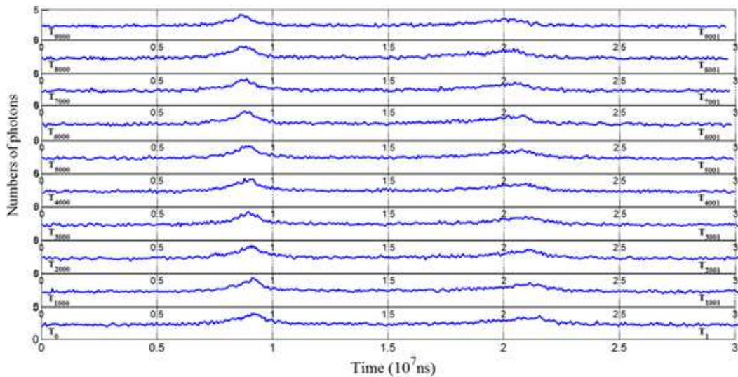
Figure 2 Time series of photons of Crab pulsar separately in ten time cycles.
