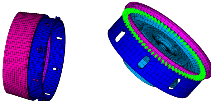
Fig. 4 The bolted joints parameterized model
