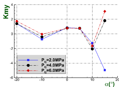
(a) Lateral force amplification factor
