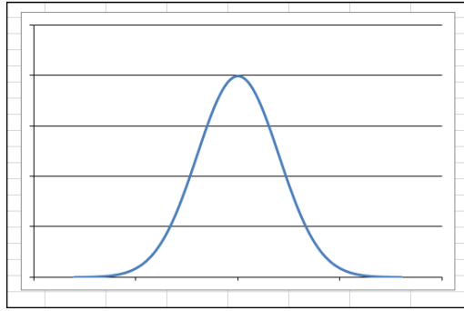
FIGURE 9-7: Displaying a normal distribution in a graph.
