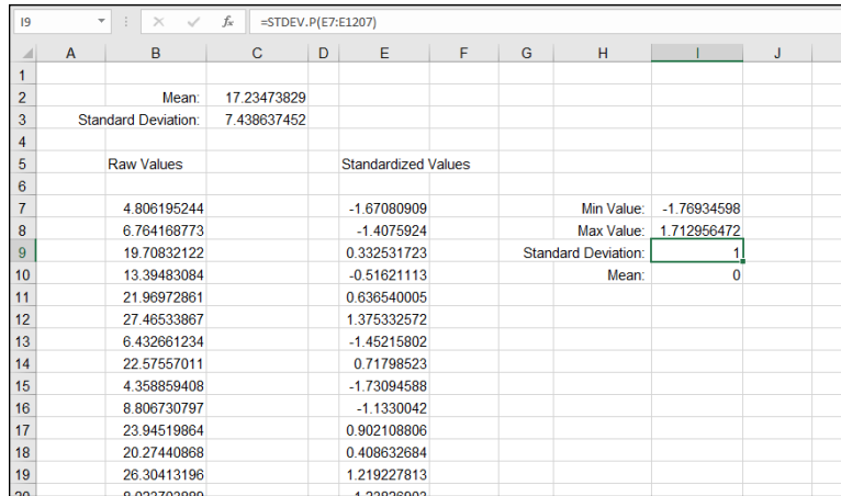
FIGURE 9-9: Standardizing a distribution of data.
