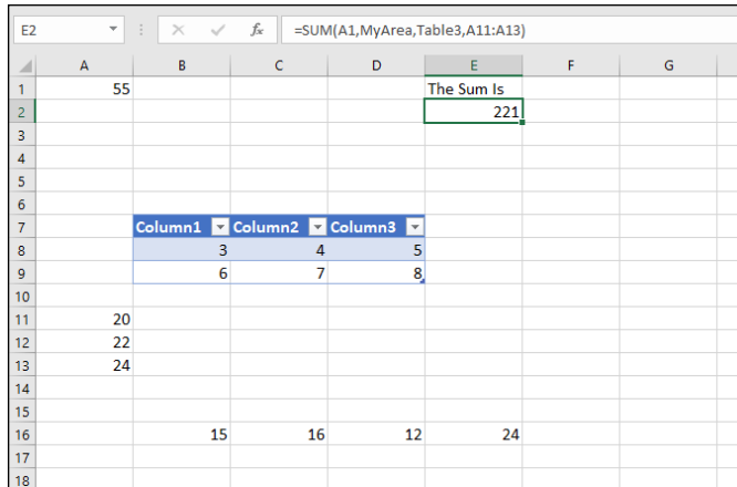
FIGURE 2-12: Calculating a sum based on cell and range references.
