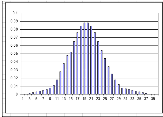
FIGURE 11-9: A Poisson distribution with a mean of 20.
