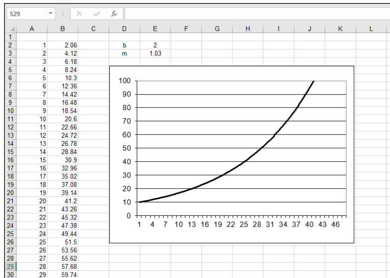
FIGURE 11-1: An exponential curve.
