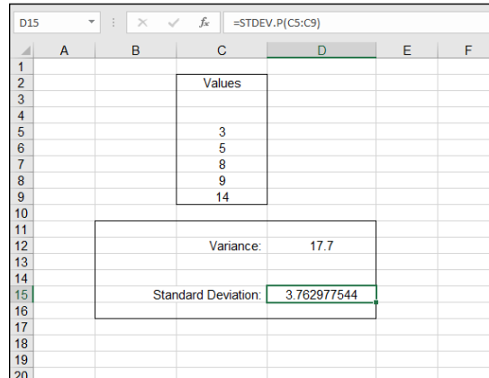
FIGURE 9-6: Calculating the standard deviation.
