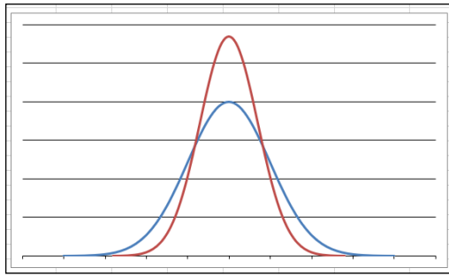
FIGURE 9-8: Normal distributions come in different heights and widths.
