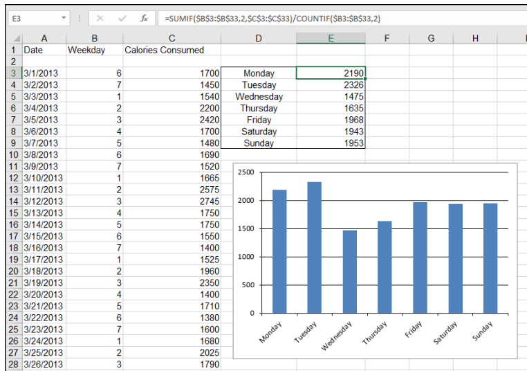
FIGURE 12-8: Using WEEKDAY tells you which day of the week a date falls on.
