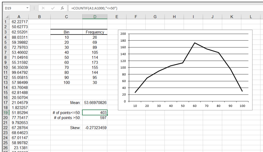
FIGURE 9-10: Working with skewed data.
