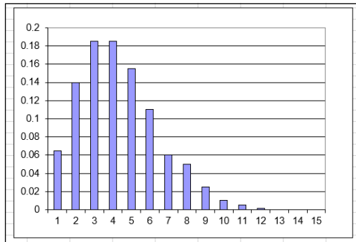
FIGURE 11-10: A Poisson distribution with a mean of 4.
