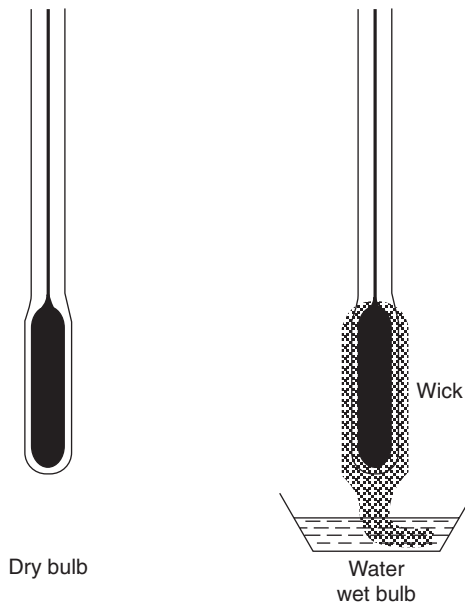
Figure 20.3 Thermometers, dry bulb and wet bulb
