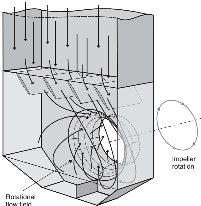
Figure 24.12 Pre-rotation of inlet air by louvred dampers in a fan inlet box prior to entering the impeller for part-load duty (CIBSE/FMA/Howden)
