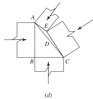
Figure 8.6 Nodal zones [1]. (a) Nodal zone, (b) subdivision of nodal zone, (c) three struts acting on a nodal zone, and (d) struts AE and CE may be replaced by AC .
