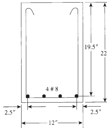
Figure 7.5 Example 7.1.
