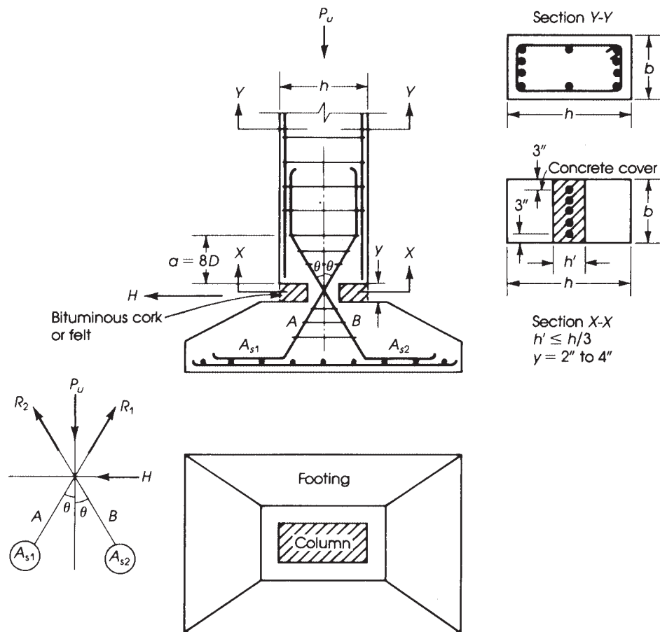
Figure 16.14 Hinge details.
