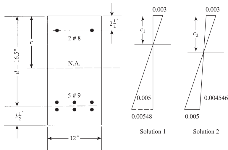
Figure 4.6 Example 4.6.
