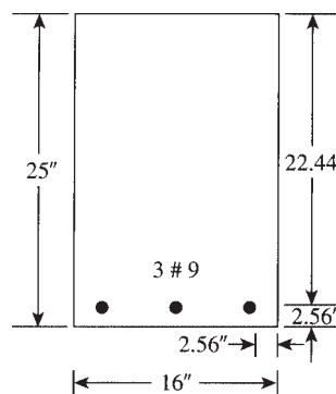
Figure 6.10 Example 6.7.
