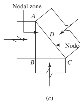
Figure 8.6 Nodal zones [1]. (a) Nodal zone, (b) subdivision of nodal zone, (c) three struts acting on a nodal zone, and (d) struts AE and CE may be replaced by AC .
