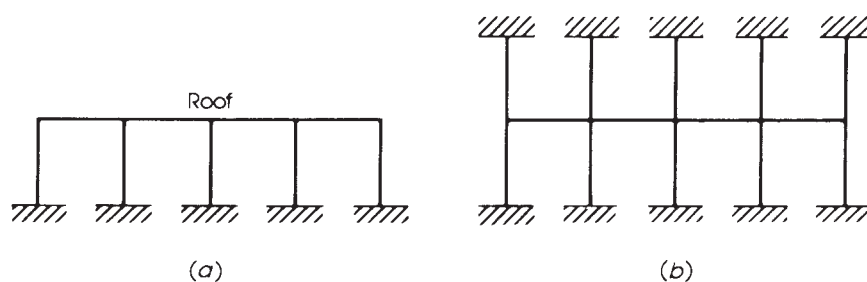
Figure 16.7 Assumption of fixed column ends for frame analysis.
