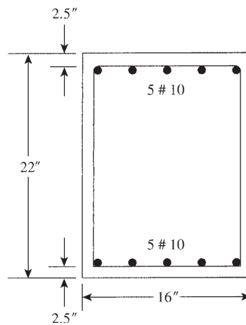
Figure 11.22 Example 11.16.
