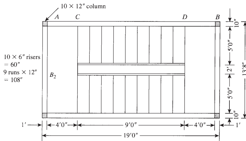
Figure 18.22 Problem 18.1.
