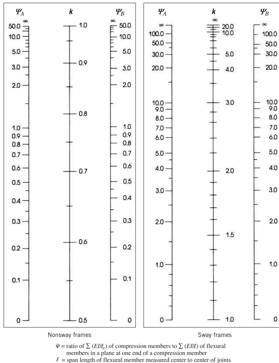
Figure 12.3 Alignment chart to calculate effective length factor, k (courtesy of ACI).
