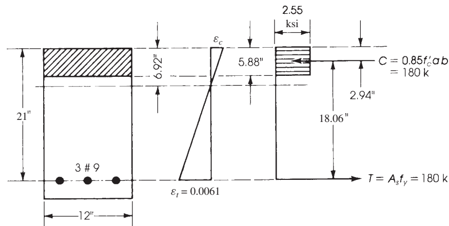
Figure 3.14 Example 3.2.
