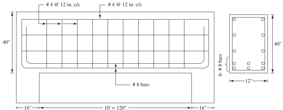
Figure 8.19 Reinforcement details.
