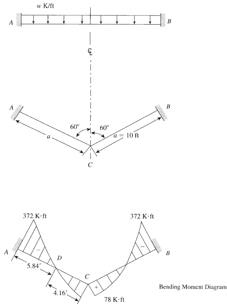
Figure 21.11 Example 21.8.
