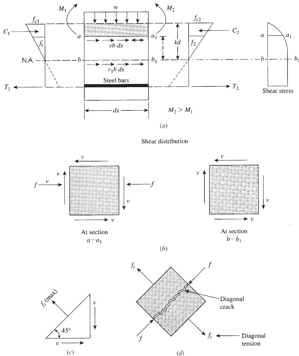
Figure 5.4 (a) Forces and stresses along depth of section, (b) normal and shear stresses, (c) pure shear, and (d) diagonal tension.
