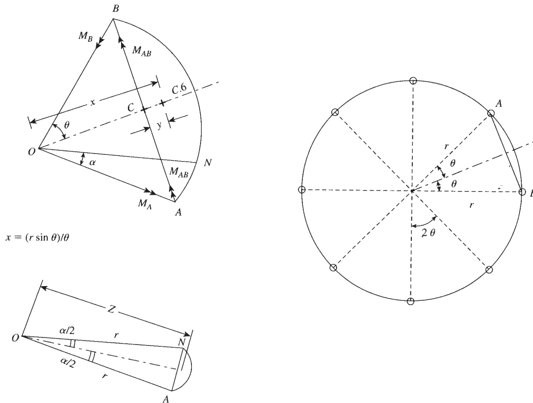
Figure 21.1 Circular beam.
