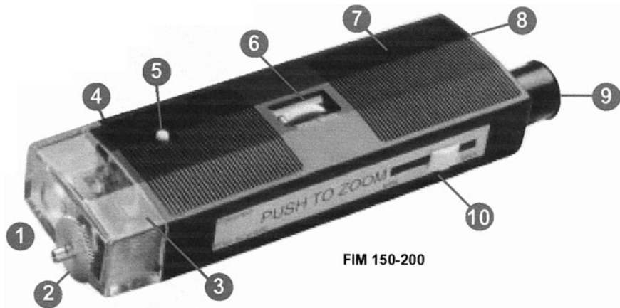
FIGURE 11-14. (M) Fiberoptic inspection microscope.
