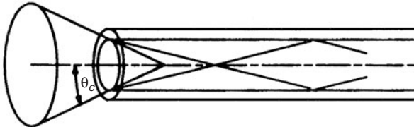
FIGURE 11-9. Cone of acceptance.
