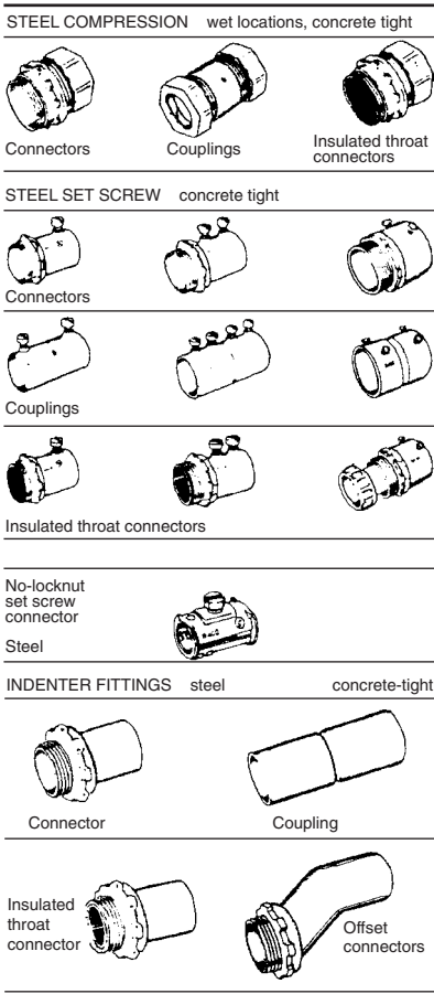
FIGURE 8-13. Variety of fittings used on EMT.
