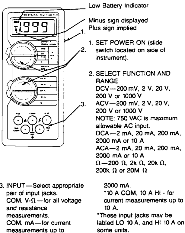
FIGURE 16-6. Digital meter.
