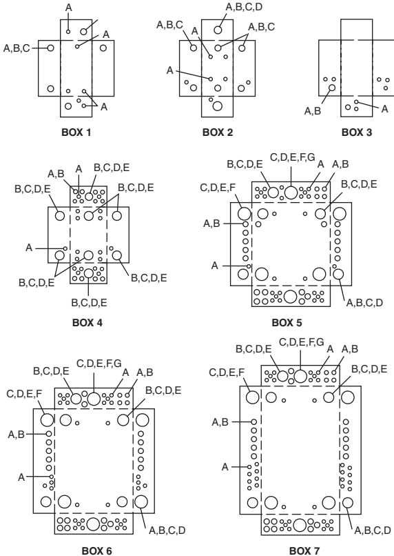
FIGURE 7-15. QO and Homeline Load Centers. Knockout information and enclosure dimensions (Square D).
