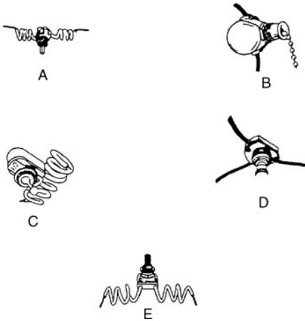
FIGURE 8-33. Canopy switches.
