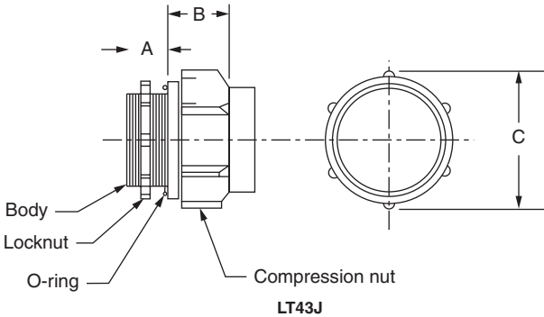
FIGURE 9-9B. Compression nut details (Carlton).
