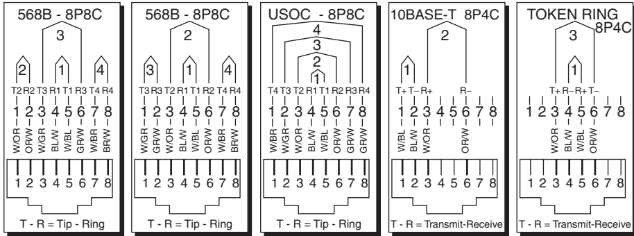
FIGURE 11-4. Modular jack pin/pair assignments.
