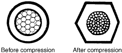
FIGURE 1-6. Cross section of cable.
