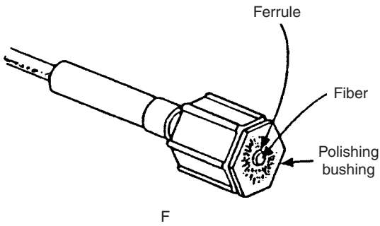
FIGURE 11-11. (E) Polishing bushing on sandpaper (000). (F) Locating the polishing bushing.
