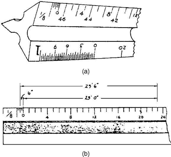
FIGURE 16-1. Architect's scale.
