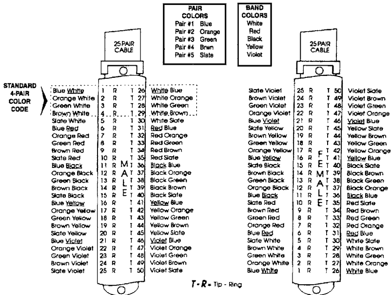
FIGURE 11-7. RJ25 Jelco connector pin/pair assignments. (Greenlee)
