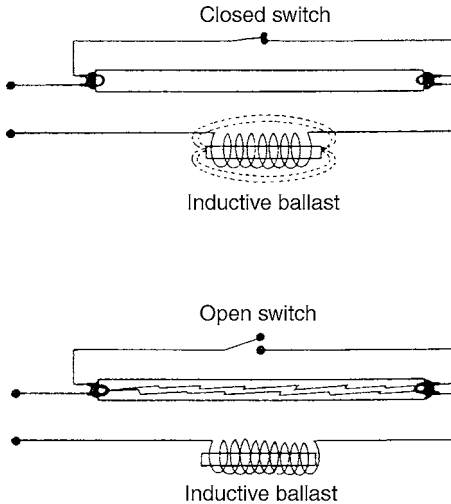
FIGURE 5-5. Simple ballast.
