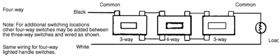
FIGURE 8-34. Four-way switches.
