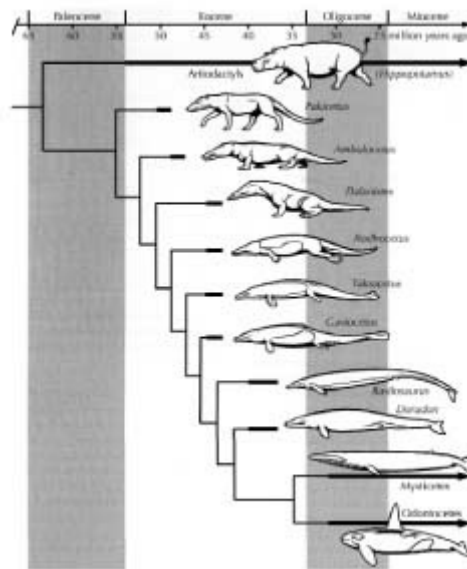
Figure 14.16. Evolution of whales from land creatures, showing the numerous transitional fossils now documented from the Eocene beds of Africa and Pakistan. (Drawing by Carl Buell)
