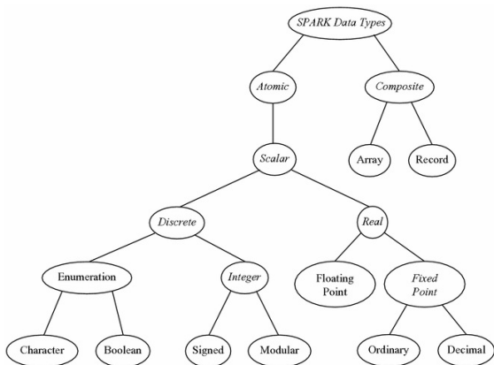
Figure 2.1. The SPARK type hierarchy.
