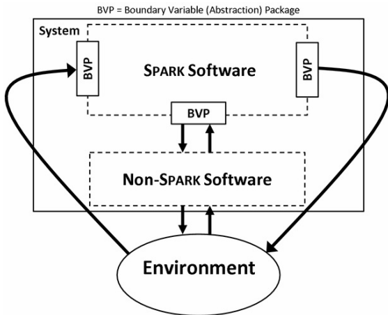
Figure 8.2. Boundary variable packages define the SPARK boundary.
