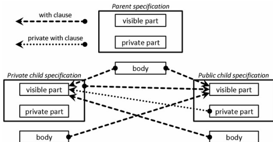
Figure 3.2. Visibility via with clauses in child packages.
