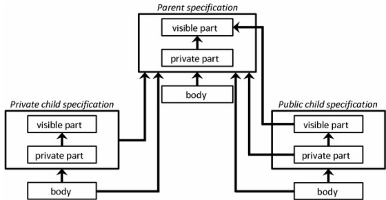
Figure 3.1. Direct visibility with child packages.
