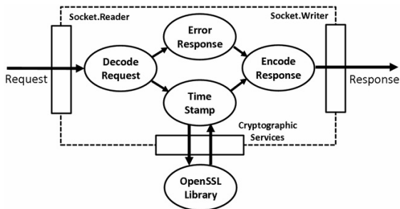
Figure 8.4. Architecture of the SPARK components of Thumper.
