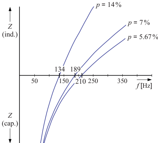
Fig. C12.26 Reactor-connected capacitors in a PFC application
