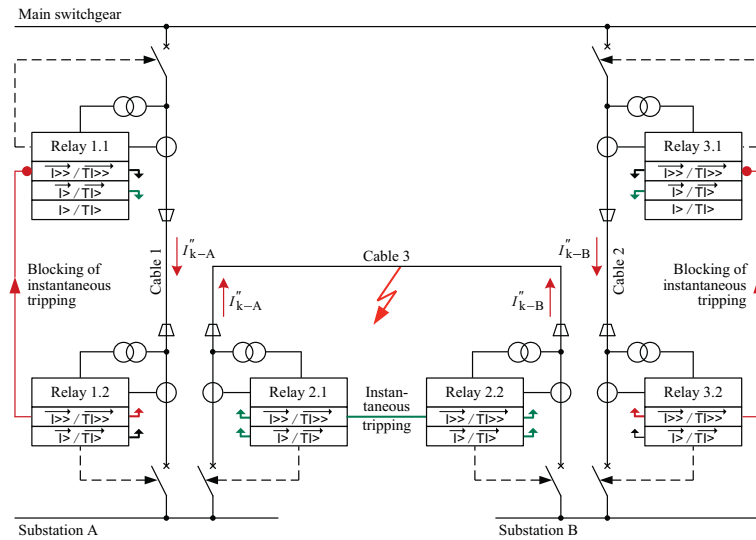
Fig. B7.32 General short-circuit and line-to-earth short-circuit protection in case of loop-in of distribution substations
