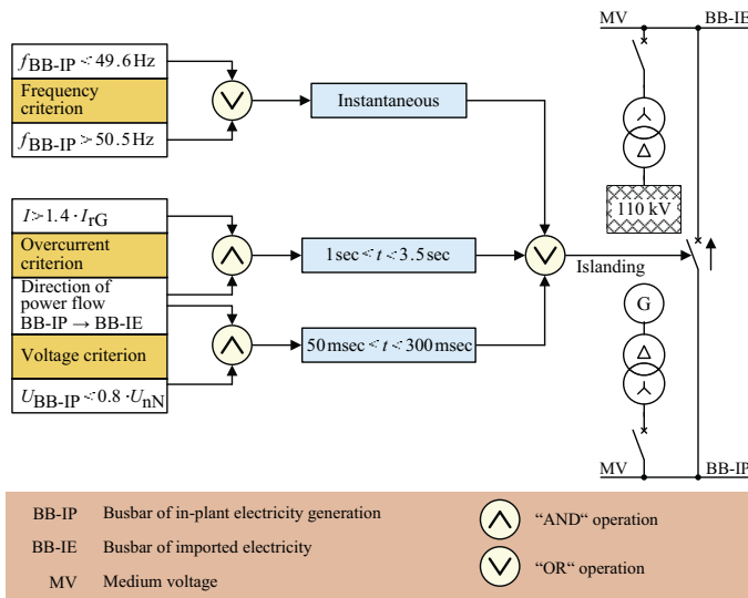
Fig. B5.10 Tripping criteria for islanding for an industrial plant with in-plant generation and imported electricity
