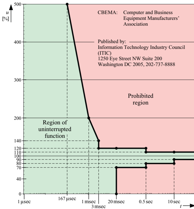
Fig. A2.14 ITIC voltage tolerance envelope for processes in the IT industry (CBEMA curve)
