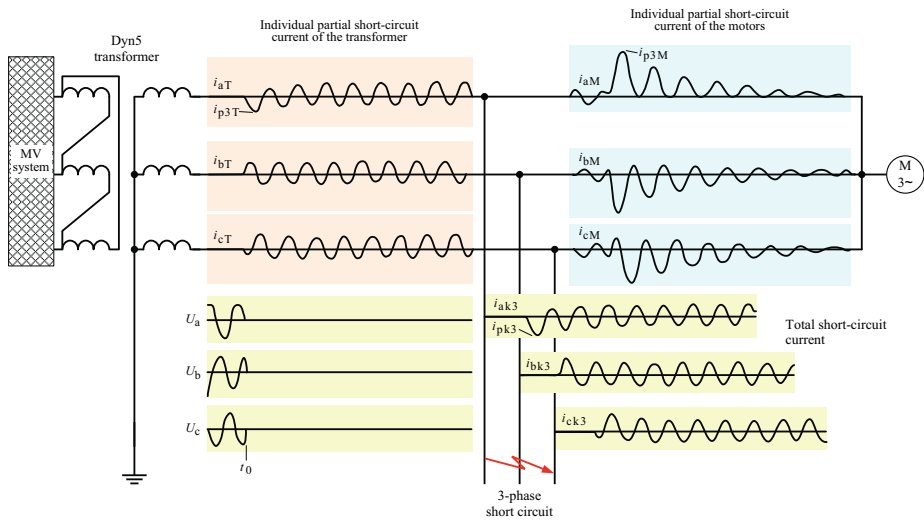
Fig. C9.3 Time characteristic of the currents and voltages on a three-phase short circuit in the central incoming supply of an LV system acc. to [9.2]
