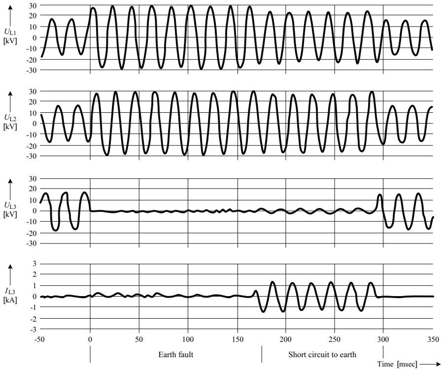
Fig. B6.23 Current and voltages in operation with short-time low-impedance neutral earthing [6.58]
