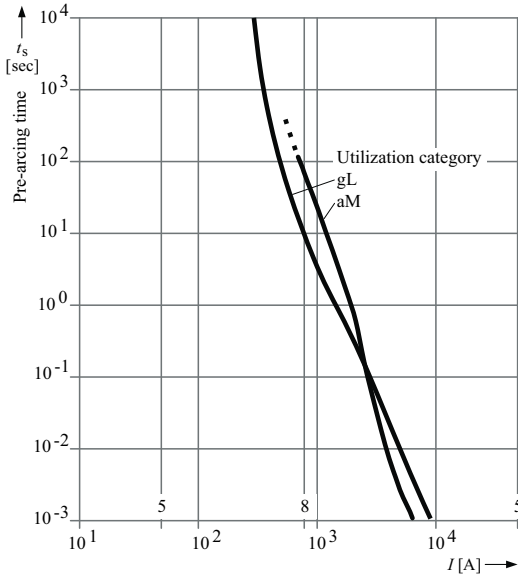
Fig. C13.3 Example of t_s I characteristics of LV HRC fuses of utilization categories gL and aM, I_T = 200\text{ A}
