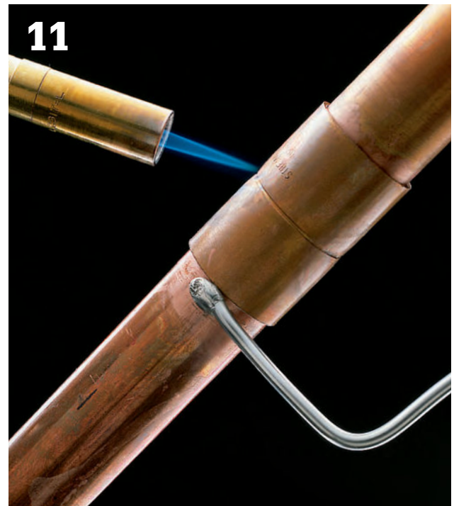
11 Heat the other side of the copper fitting to ensure that heat is distributed evenly. Touch solder to pipe. Solder will melt when the pipe is at the right temperature.
