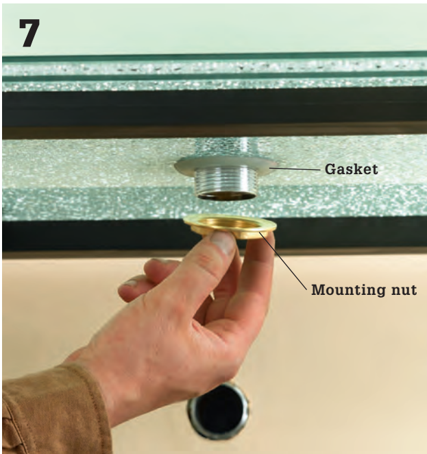
7 From underneath, push the large rubber gasket onto the threaded portion of the pop-up assembly. Thread the nut onto the pop-up assembly and tighten. Use an adjustable wrench or basin wrench to tighten an additional half turn. Thread the tailpiece onto the pop-up assembly.
