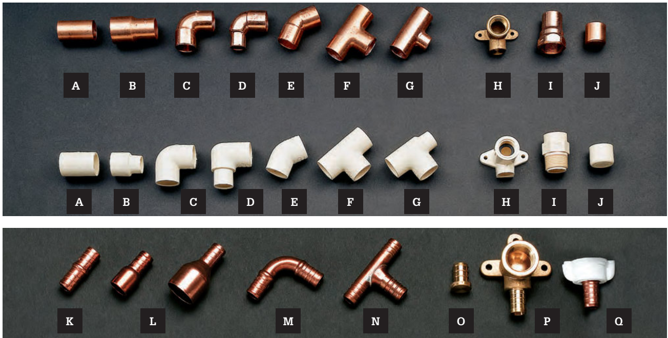
Water supply fittings are available for copper (top), CPVC plastic (center), and PEX (bottom). Fittings for CPVC and copper are available in many shapes, including: unions (A), reducers (B), 90° elbows (C), reducing elbows (D), 45° elbows (E), T-fittings (F), reducing T-fittings (G), drop-ear elbows (H), threaded adapters (I), and caps (J). Common PEX fittings (bottom) include unions (K), PEX-to-copper unions (L), 90° elbows (M), T-fittings (N), plugs (O), drop-ear elbows (P), and threaded adapters (Q).
