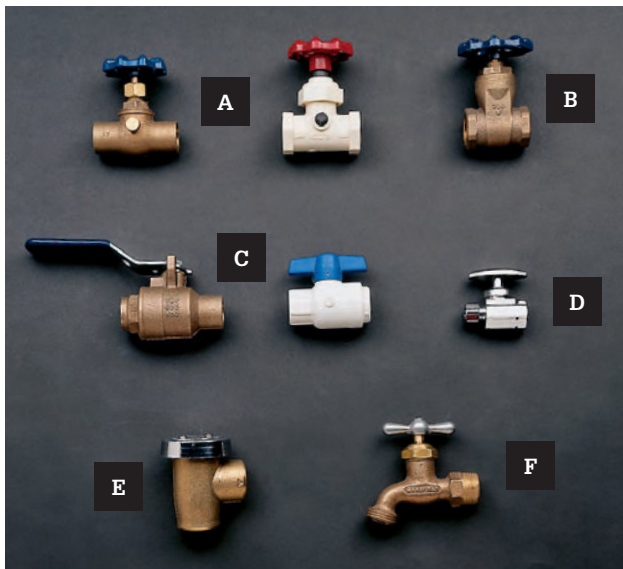
Water supply valves are available in brass or plastic and in a variety of styles, including: drain-and-waste valves (A), gate valve (B), full-bore ball valves (C), fixture shutoff valve (D), vacuum breaker (E), and hose bib (F).
