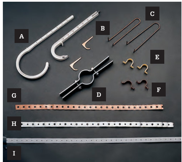
Support materials for pipes include: plastic pipe hangers (A), copper J-hooks (B), copper wire hangers (C), riser clamp (D), plastic pipe straps (E), copper pipe straps (F), flexible copper, steel, and plastic pipe strapping (G, H, I). Do not mix metal types when supporting metal pipes; use copper support materials for copper pipe, and steel for steel and cast-iron pipes.
