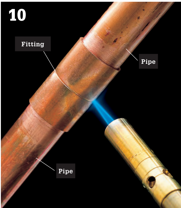
10 Move the torch flame back and forth and around the pipe and the fitting to heat the area evenly.
