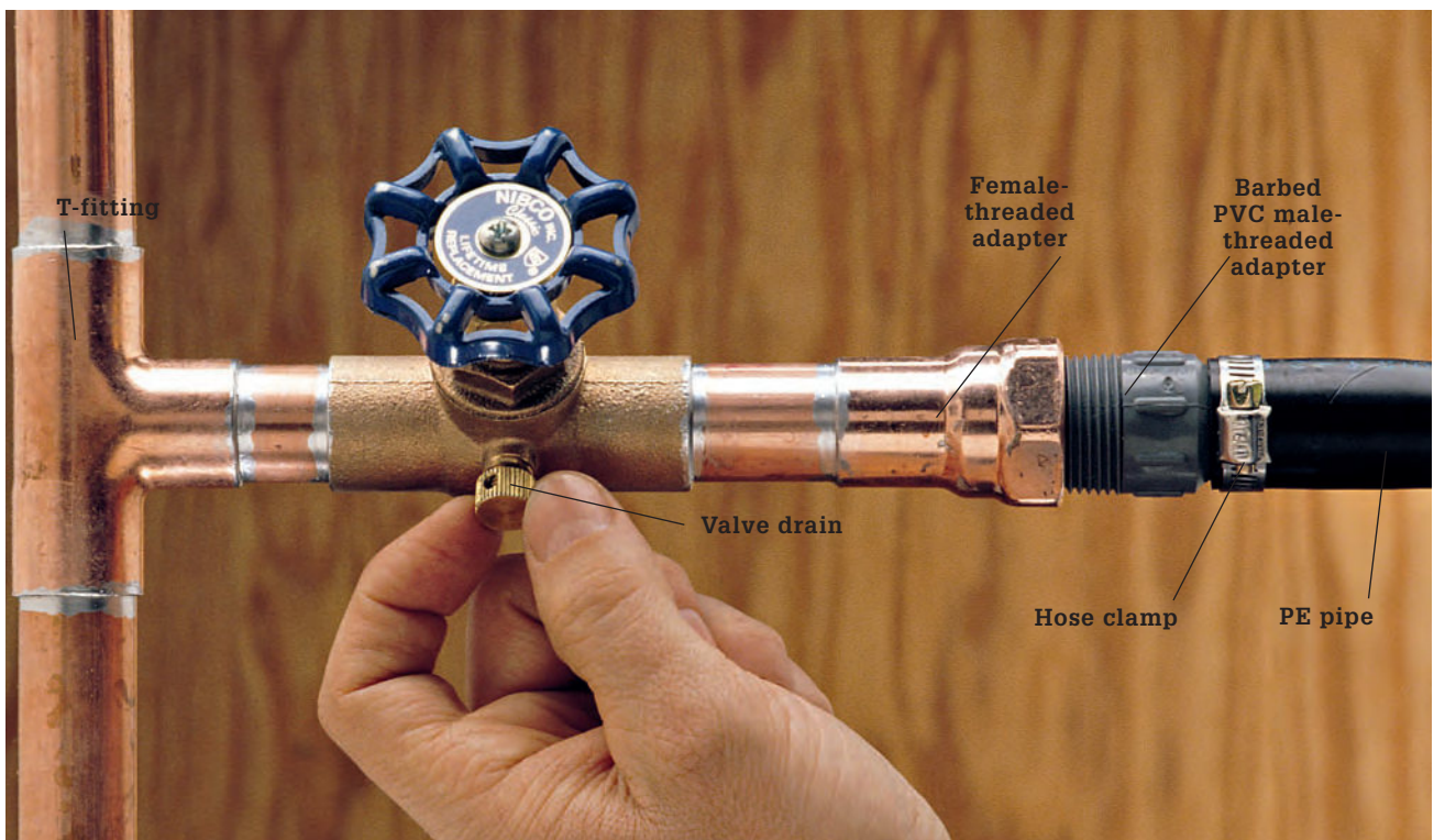
Connect lengths of PE pipe with a barbed PVC fitting. Secure the connection with stainless steel hose clamps.
