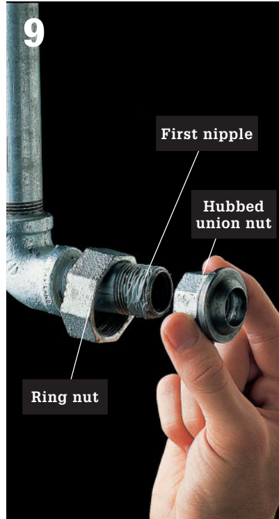
9 Slide a ring nut onto the installed nipple, then screw the hubbed union nut onto the nipple and tighten with a pipe wrench.
