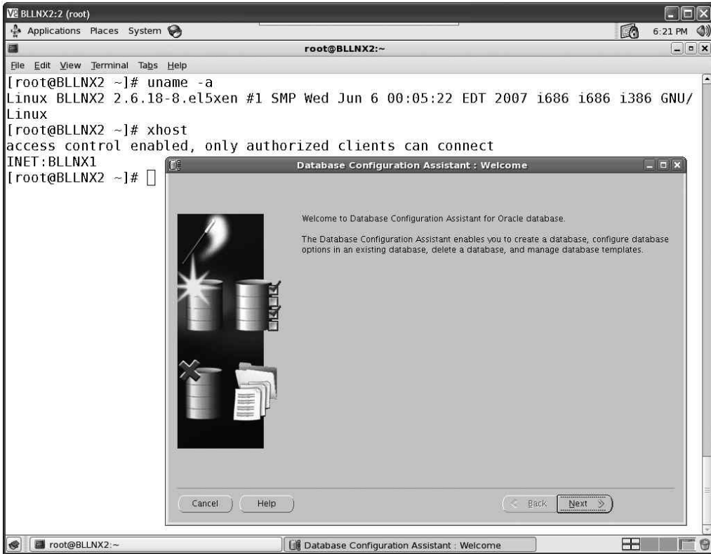
Figure 15-5. Database Configuration Assistant screen
