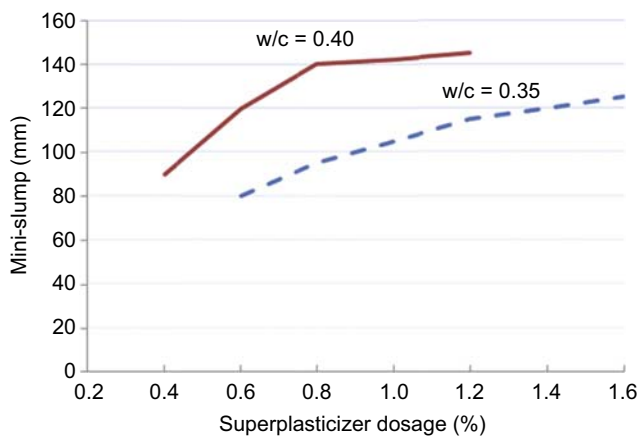
Figure A2.2 Variation of the initial flow of a cement paste as a function of its SP dosage (Yahia and Khayat, 2001).
