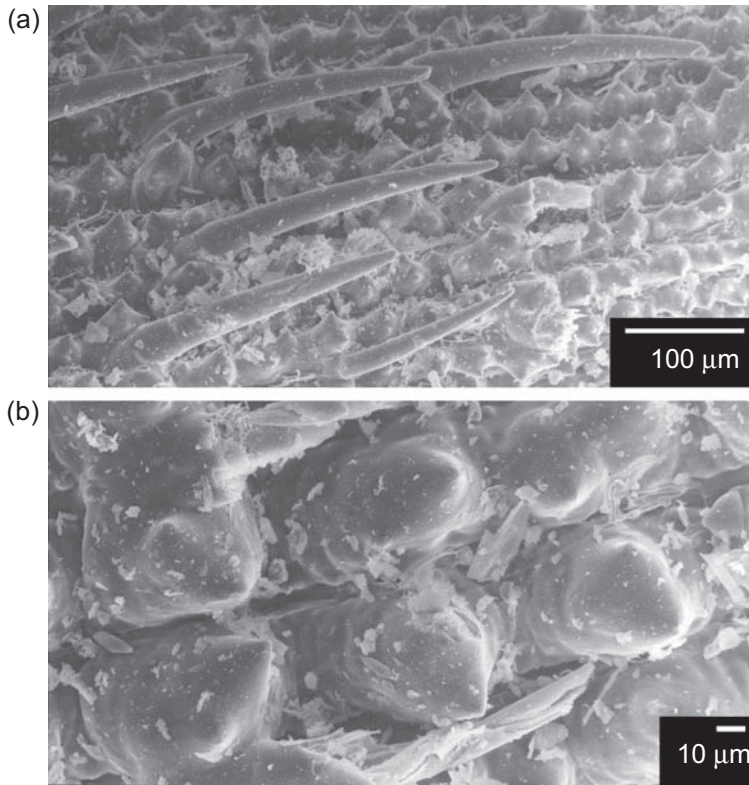
Figure 4.20 (a) Rice husk ash, (b) enlarged view.
