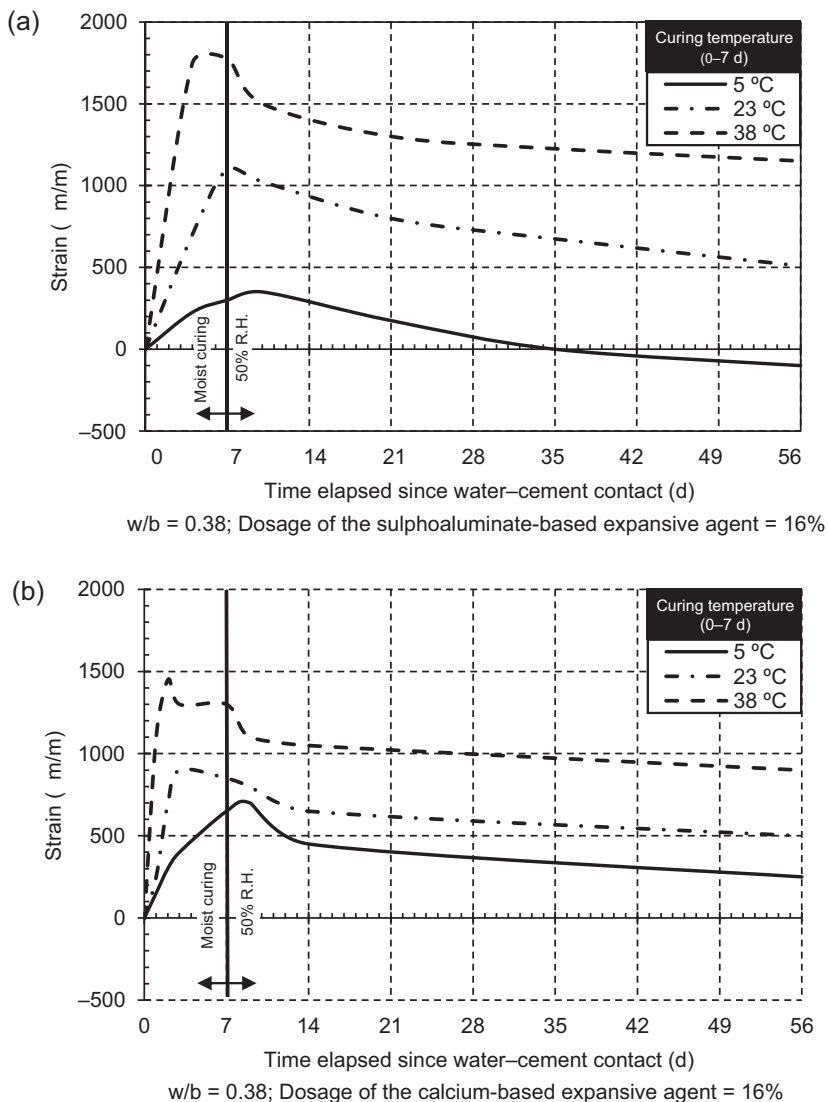
Figure 22.10 Effect of the curing temperature on the restrained expansion of a concrete made with a sulphoaluminate-based expansive agent (a) and a calcium-based expansive agent (b) (Bissonnette et al., 2014).
