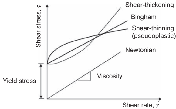
Figure 7.4 Illustration of different rheological behaviours – the cases of shear thinning and shear thickening shown include a yield stress, which is not necessarily always the case.
