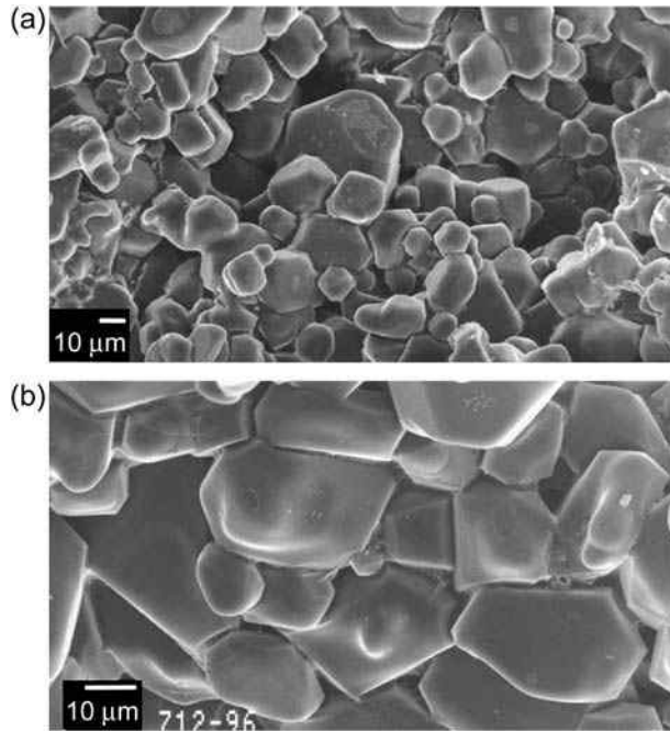
Figure 3.2 Tricalcium silicate crystals in two clinkers: (a) small crystals, smaller than 10\ \mu\text{m} ; (b) coarse crystals, coarser than 10\ \mu\text{m} . Courtesy of Arezki Tagnit-HAMOU ( Aïtcin, 2008 ).
