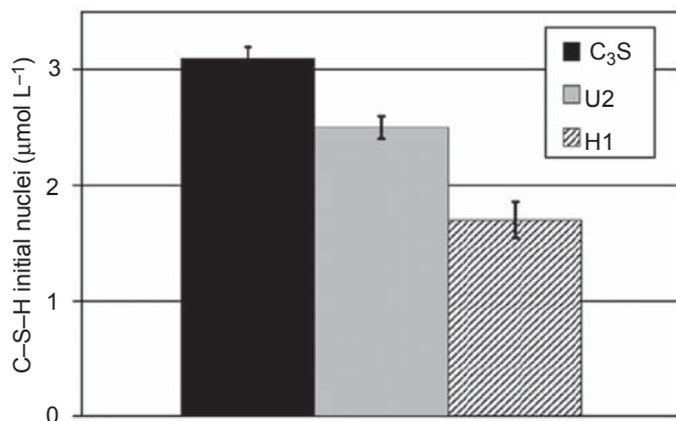
Figure 20.13 The impact of CE on the amount of initial nuclei of C–S–H after 30 min of C 3 S hydration (liquid/solid = 100, polymer/solid = 2%, Ca(OH) 2 = 20 mM).
