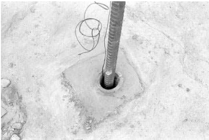
Figure 21.5 The small rectangular base built around each anchor to support the base of the hollow jack used to pull out the anchors. The temperature of each grout was monitored by a thermocouple.
