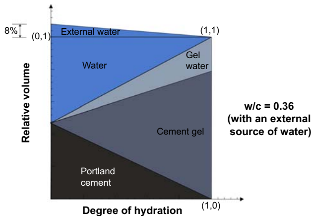
Figure 2.5 Schematic representation of the hydration of a cement paste having a w/c ratio equal to 0.36 benefitting from an external source of water.
