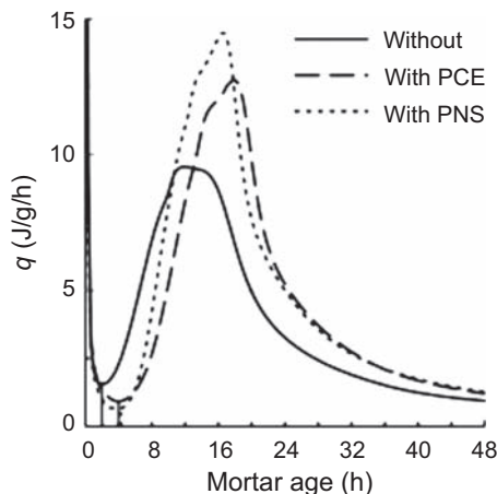
Figure 12.2 Example of isothermal calorimetry showing the effect of a PCE and polynaphtalene sulfonate (PNS) superplasticizer on a mortar with normal Portland cement. The difference in the shapes of the curve is particularly noted.
