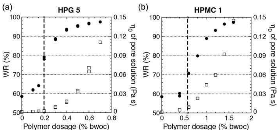
Figure 20.9 Effect of polymer agglomerates formation on water retention for (a) hydroxypropylguar (HPG) and (b) hydroxypropoxy methoxy cellulose (HPMC).
