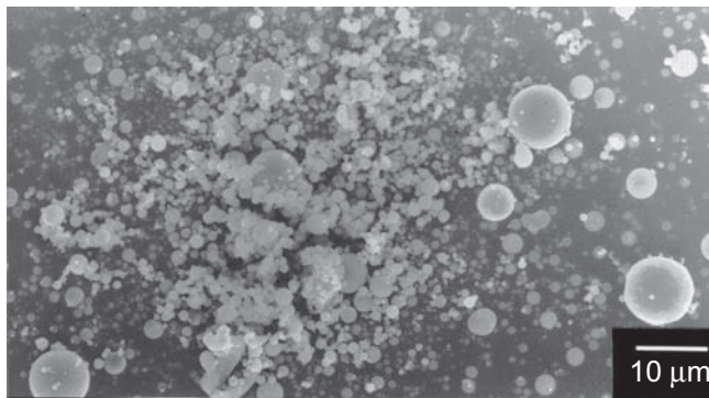
Figure 4.10 Spherical particles of fly ashes.
