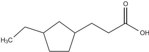
Figure 9.34 Chemical structure of a naphthenic acid.
