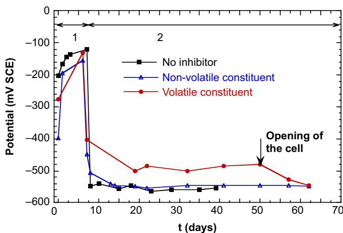
Figure 14.5 Corrosion potentials of rebar samples in solutions containing the two components of the inhibitor: ◼, no inhibitor; ◯, volatile constituent; Δ, nonvolatile constituent (Elsener et al., 1999).
