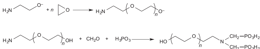
Figure 9.7 Scheme of the two-step synthesis of polyoxyethelene diphosphonate.
