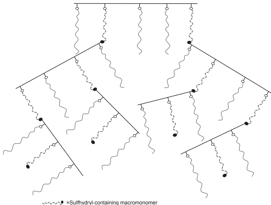
Figure 9.13 Possible structure of a hyperbranched PCE.
