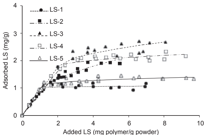
Adsorption data of different lignosulfonate polymers plotted as a function of the added polymer amount.
