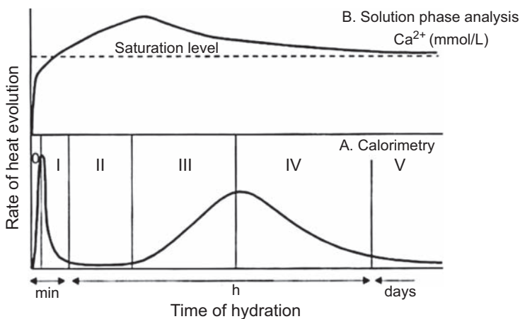
Figure 8.2 Illustration of the different stages of alite hydration following the \text{Ca}^{2+} concentration evolution and the associated heat release.
