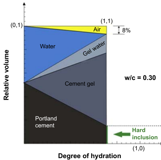
Figure 2.7 Schematic representation of the hydration of a 0.30 cement paste hydrating in a closed system.
