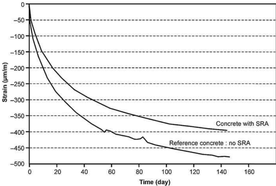
Figure 23.4 Effect of an SRA on the drying shrinkage of a self-compacting air-entrained concrete (Apya, 2011).
