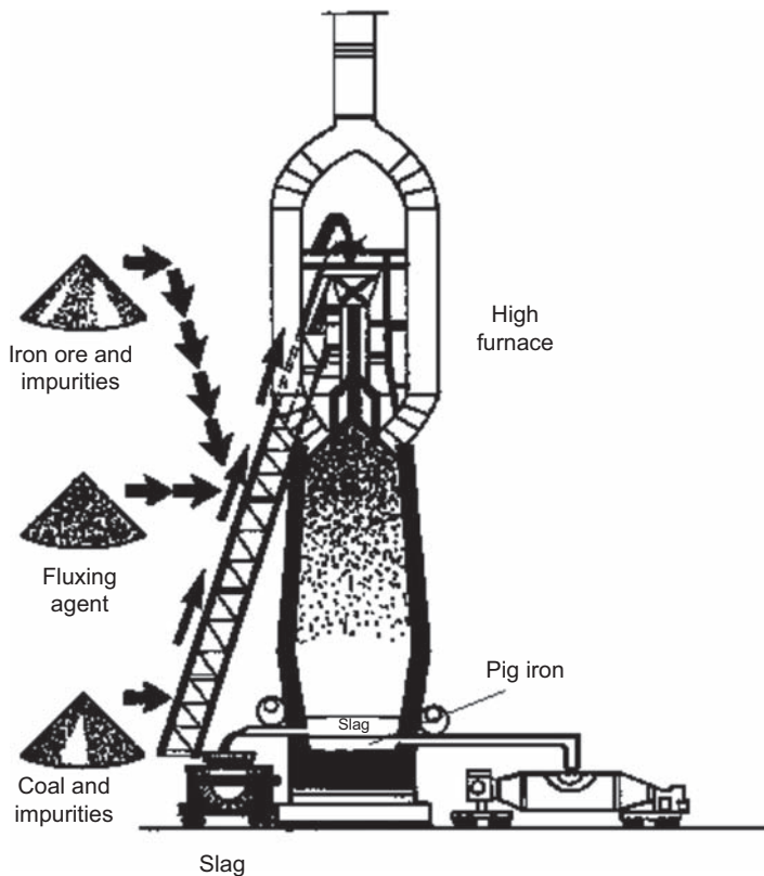
Figure 4.5 Schematic representation of a high furnace.
