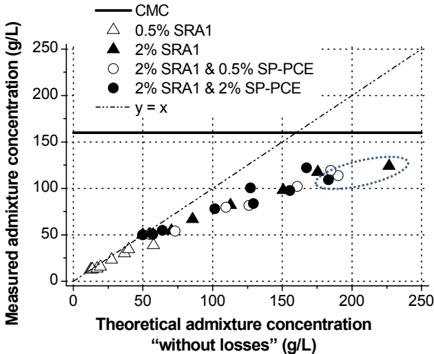
Figure 13.8 Admixture losses for SRA containing cement pastes with different dosages at different hydration stages. Reproduced with permission from Eberhardt (2011).
