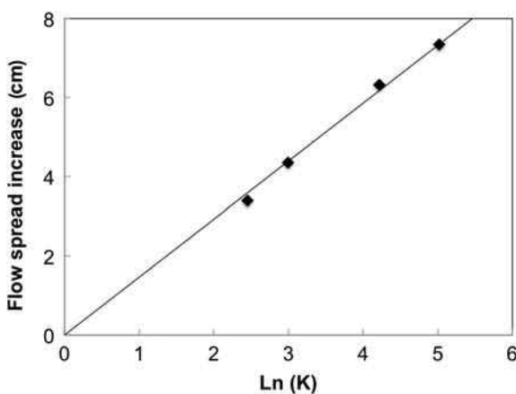
Figure 16.9 Dependence on the flow increase (assume proportional to the amount of scavenged polymer) with respect to the natural logarithm of the adsorption equilibrium constant calculated from molecular structure ( Marchon et al., 2013 ). For this, we use the C/E value of 6 common to all the polymers and the molar mass information given in Plank et al. (2010) .
