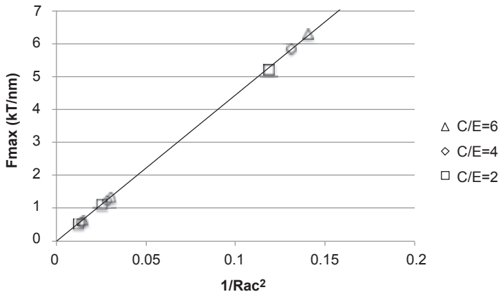
Figure 11.12 Maximum attractive interparticle force plotted versus the inverse square of the adsorbed layer thickness, R_{AC} . The three sets of points represent polymers with side chains of 1000, 3000 and 5000 g/mol with three different values of C/E . The straight line is a linear fit through the origin, demonstrating the scaling of the maximum attractive force with the inverse square of the layer thickness.
