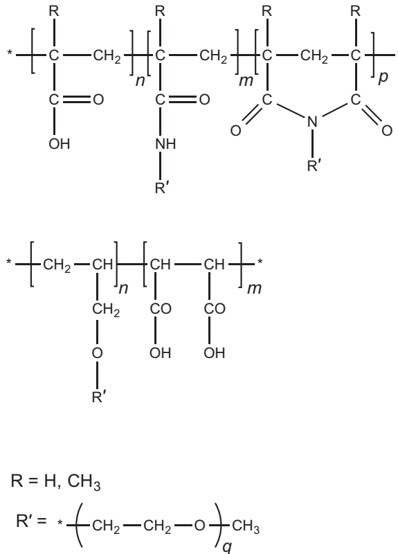
Figure 9.14 Chemical structure of PCEs with imide (top) and ether (bottom) bonds between the backbone and the side chains.
