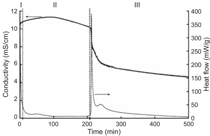
Figure 8.1 Heat release and conductivity measurements during hydration of C_3A with gypsum in saturated solution with respect to portlandite ( L/S = 25 ).
