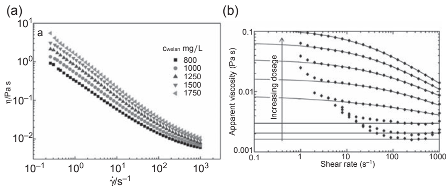
Figure 20.2 Examples of shear thinning behavior induced by (a) welan gum on aqueous solutions and (b) hydroxypropylguar on mortar pore solution.
