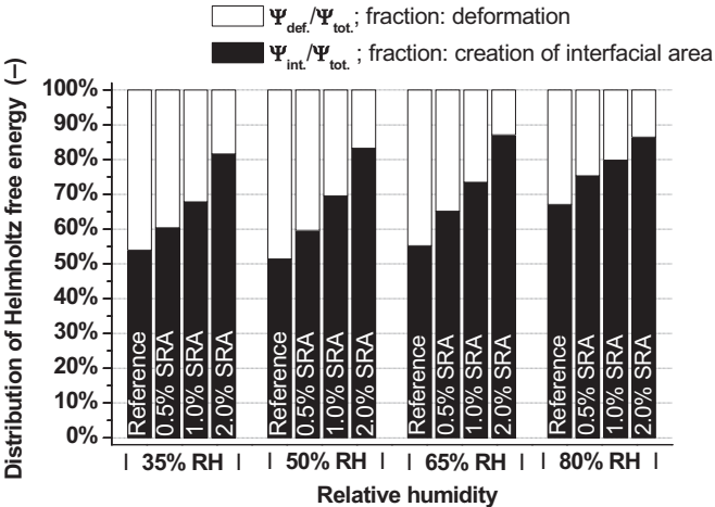
Figure 13.7 Energy fractions for deformation energy and energy utilized at interfaces for cement paste (CP) without SRA and with different dosages of SRA1 at different relative humidities. Reproduced from Eberhardt (2011) with permission.
