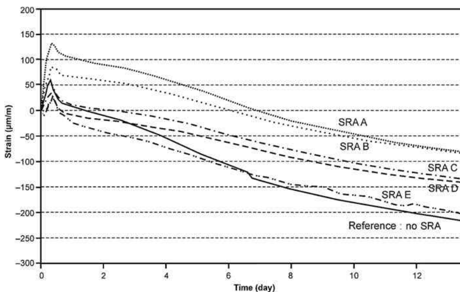
Figure 23.1 Autogenous shrinkage of a reference mortar (no SRA) and of five mortars containing commercial SRAs (A, B, C, D, and E) (Apaya, 2011). Courtesy of Prof. Richard Gagné.
