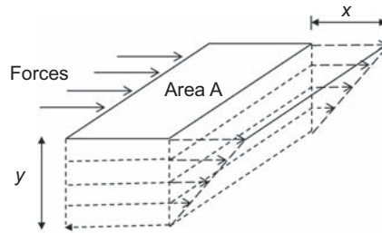
Figure 7.1 Schematic illustration of laminar shear flow.
