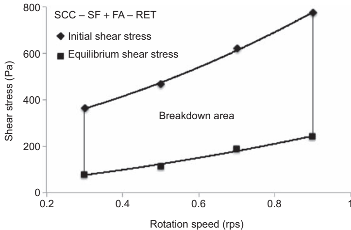
Figure 7.15 Calculation of the structural breakdown area for a ternary SCC system containing fly ash (FA), silica fume (SF), and set-retarding admixture (RET).
