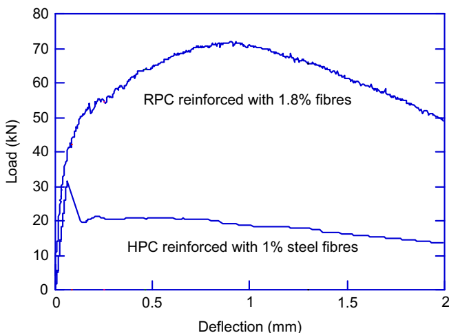
Figure 27.2 Pseudo-ductile behaviour of a fibre-reinforced UHSC.
