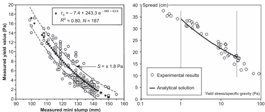
Figure 7.7 Relationship between slump and yield stress.
