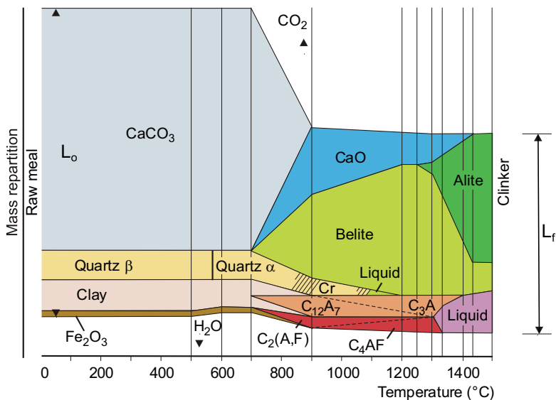
Figure 3.1 Transformation of raw meal into clinker. With the permission of KHD Humboldt Wedag ( Aïtcin, 2008 ).
