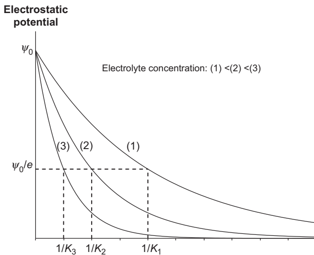
Figure 11.2 Variation in the electrostatic potential as a function of the distance from the surface of a colloidal particle and of the ionic strength (electrolyte concentration) of the continuous phase.
