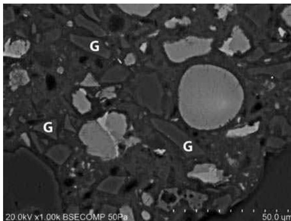
Figure 4.22 Cement paste of an ultra-high-strength concrete containing glass particles (G).
