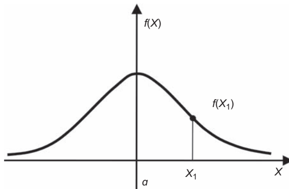
Figure A3.1 Normal frequency distribution curve: the y axis is placed at the average value, a , and f(x_1) represents the number of samples with the value x_1 .
