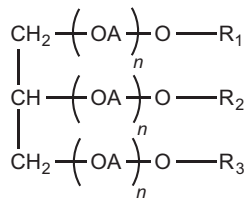
Figure 9.46 Chemical structure of a polymeric surfactant used in SRAs.
