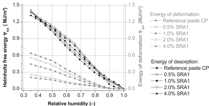
Figure 13.1 Computed changes of Helmholtz and deformation energy for cement paste containing an SRA.
