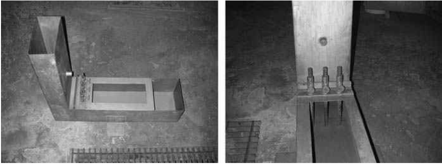
Figure 26.3 Measuring passing ability with an L-box.
