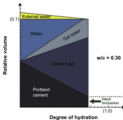
Figure 2.8 Hydration of a cement paste having a w/c ratio equal to 0.30 hydrating under water.
