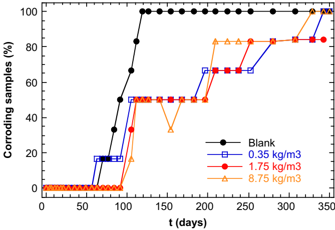
Figure 14.6 Percentage of corroding rebars in mortar versus time of cyclic chloride treatment (Elsener et al., 1999).
