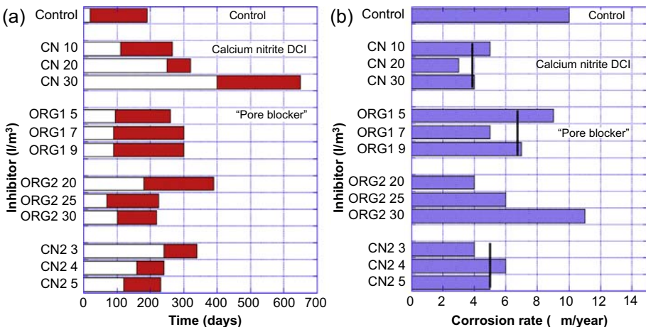
Figure 14.7 Effect of different inhibitors on the initiation of corrosion in mortar (a) and the corrosion rate after initiation (b). Mortar lollipops, w/c = 0.5, at 20 days curing, partially immersed in 3.5% NaCl (steel surface 62.7 cm 2 ) (Trépanier et al., 2001).
