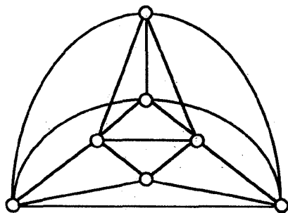
Figure 6.14 A drawing of K_{2,2,3} with two crossings.
