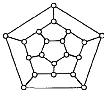
Figure 4.7 The graph of the dodecahedron.
