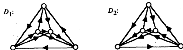
Figure 2.15 Two nonreconstructible digraphs.
