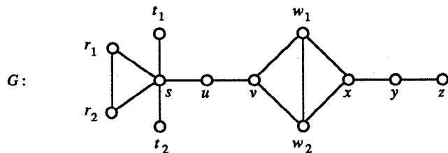
Figure 2.7 Similar vertices in a graph.
