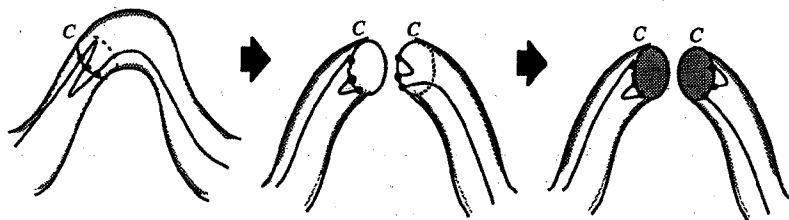
Figure 7.4 Capping a cut handle.
