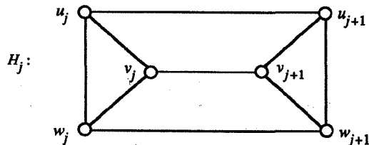
Figure 6.16 The subgraph H_j in the proof of Theorem 4.15.
