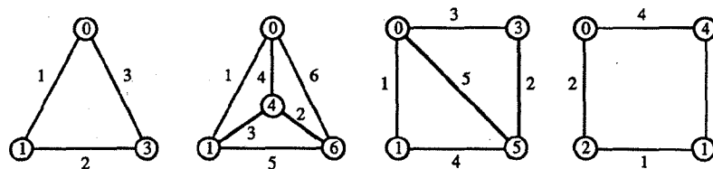
Figure 9.8 Graceful graphs.
