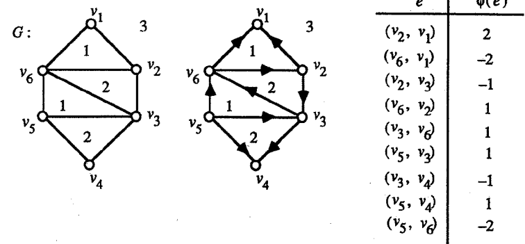
Figure 8.11 Flow construction.
