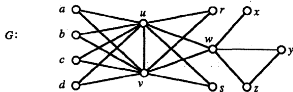
Figure 3.8 A graph of toughness \frac{2}{7} .
