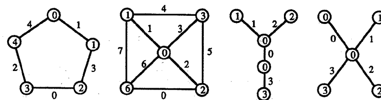
Figure 9.19 Harmonious graphs.
