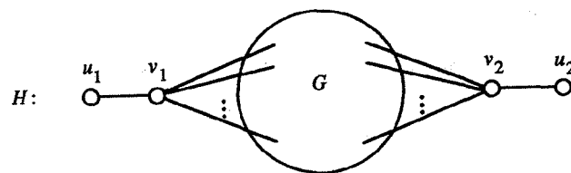
Figure 1.23 A graph with given center.
