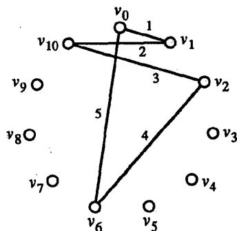
Figure 9.12 A cyclic decomposition of K_{11} into the nongraceful graph C_5 .
