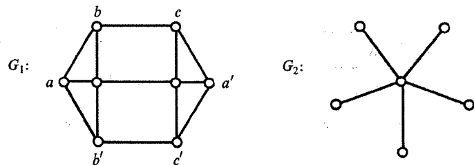
Figure 4.5 Subeulerian graphs.
