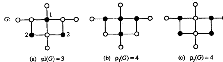
Figure 10.11 A graph with planetary domination number 3.
