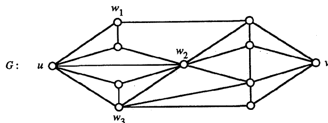
Figure 3.7 A graph illustrating Menger's theorem.
