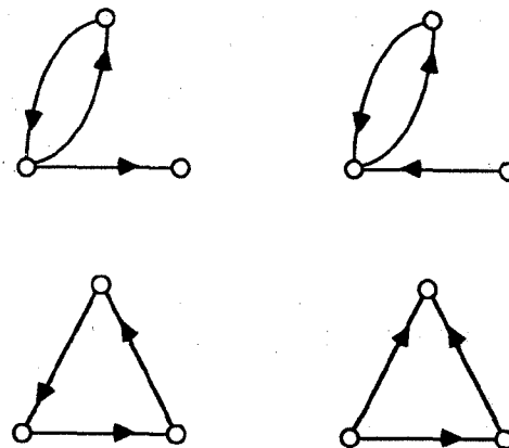
Figure 1.26 The (3, 3) digraphs.
