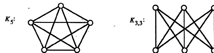
Figure 6.4 The nonplanar graphs K_5 and K_{3,3} .
