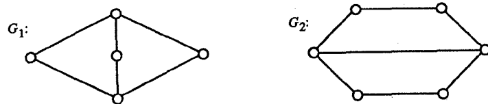
Figure 2.2 Minimal and critical blocks.
