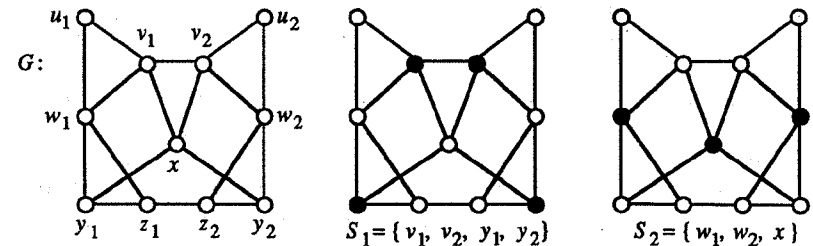
Figure 10.1 Dominating sets.
