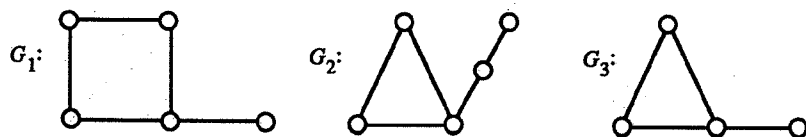
Figure 6.5 Subdivision.
