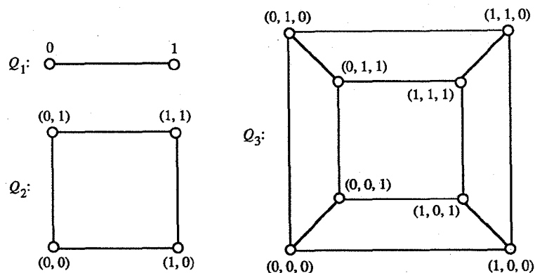
Figure 1.15 Cubes.
