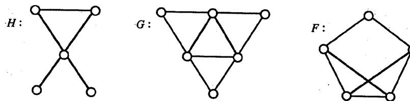
Figure 1.5 Subgraphs.
