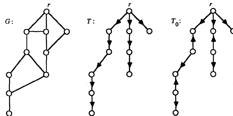
Figure 5.2 An anticonnected orientation of a graph.
