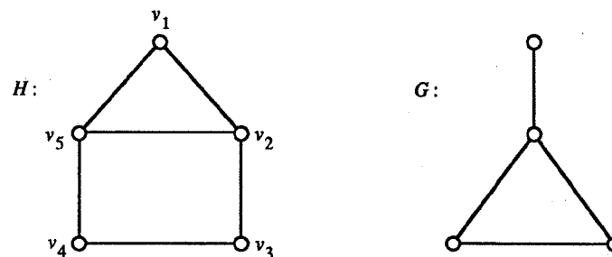
Figure 6.8 Contraction.
