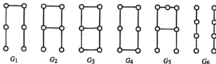
Figure 10.7 Forbidden subgraphs for irredundance perfect graphs.
