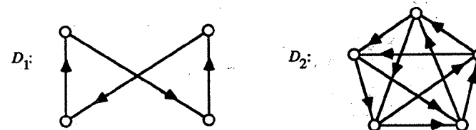
Figure 1.30 Regular digraphs.
