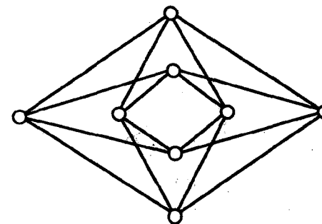
Figure 6.13 A drawing of K_{4,4} with four crossings.
