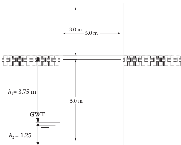
FIGURE 5.3 Sketch for pump room.
