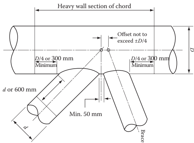
FIGURE 12.23 Details of a tubular joint.
