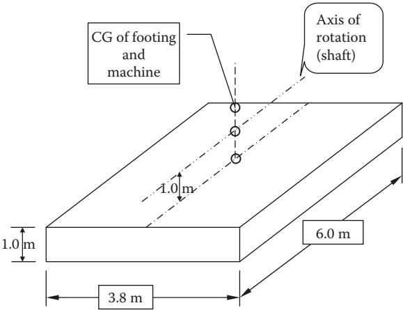
FIGURE 4.4 Sketch for centrifugal machine.
