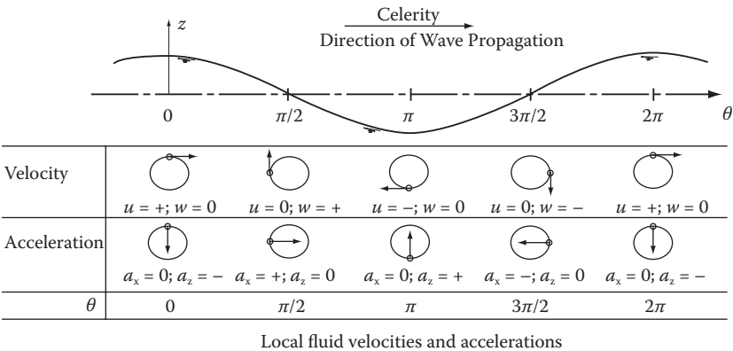
FIGURE 12.9 Local fluid velocities and acceleration.
