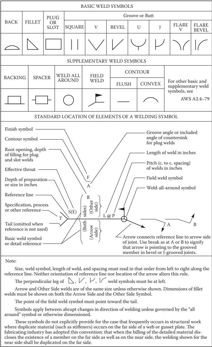
FIGURE 7.22 Welding symbols.
