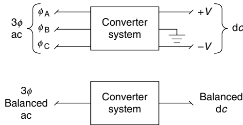
FIGURE 6.13 Single-line diagram.
