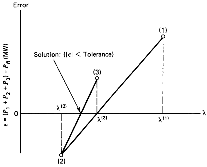
FIGURE 3.7 Lambda projections.
