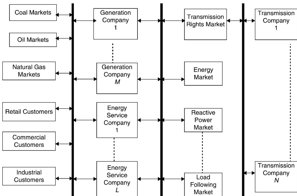
FIGURE 2.10 Leontief model with multiple markets.
