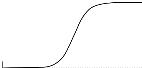
FIGURE 12.3 Sigmoid function.
