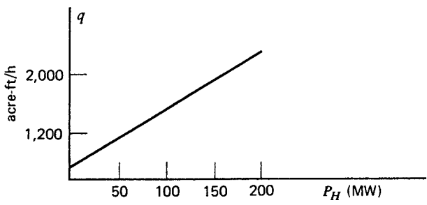
FIGURE 5.23 Hydroplant q versus P_H function.
