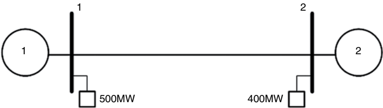
FIGURE 3.14 Two-bus system.
