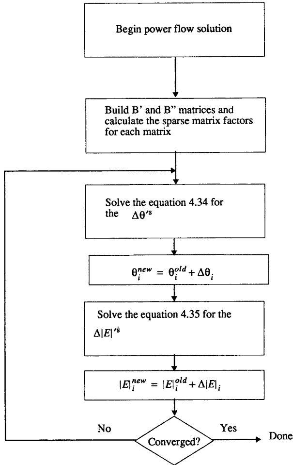
FIGURE 6.19 Decoupled power flow algorithm.
