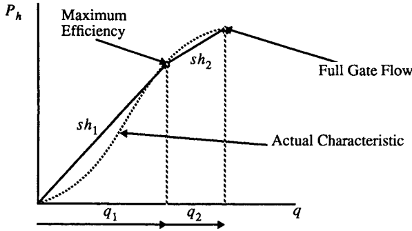
FIGURE 5.18 Hydropower characteristic.
