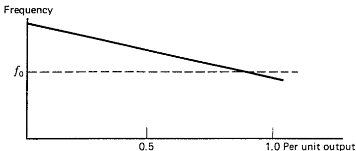
FIGURE 10.12 Speed-droop characteristic.
