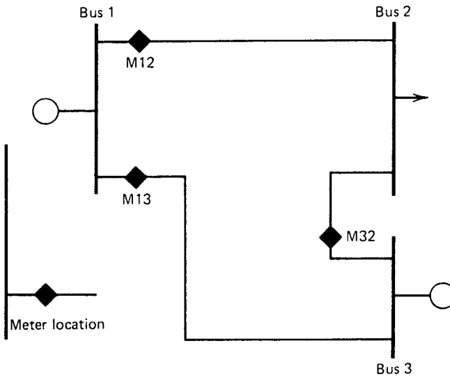
FIGURE 9.2 Meter placement.
