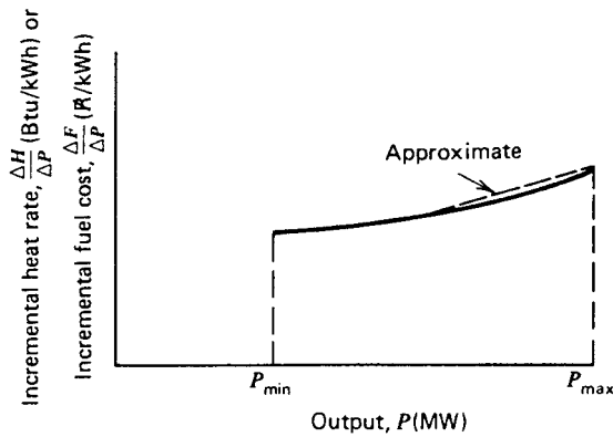
FIGURE 1.3 Incremental heat (cost) rate characteristic.
