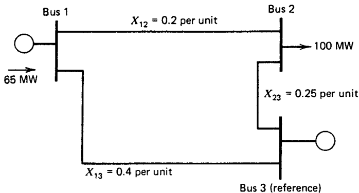
FIGURE 6.21 Three-bus network.
