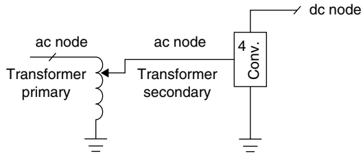
FIGURE 6.16 Monopolar model.
