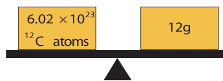
Figure 105 Avogadro's number
