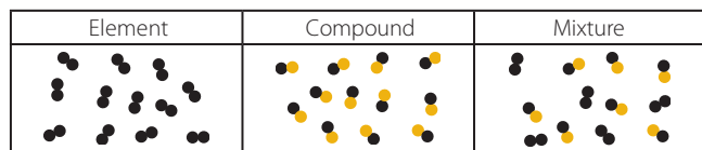
Figure 101 The particles in an element, a compound and a mixture
