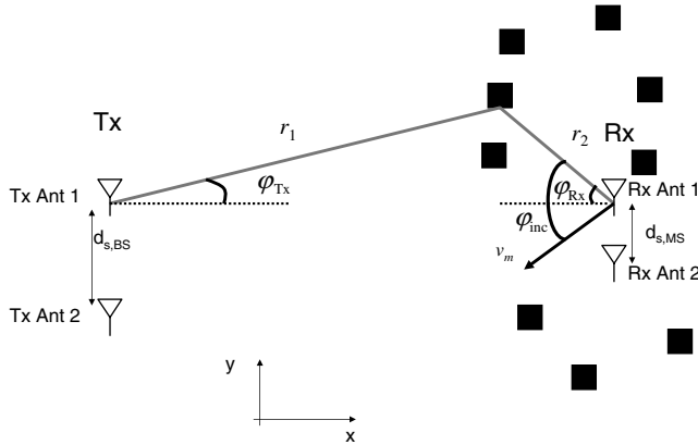
Figure 4.9 2 × 2 system in a single scattering situation.
