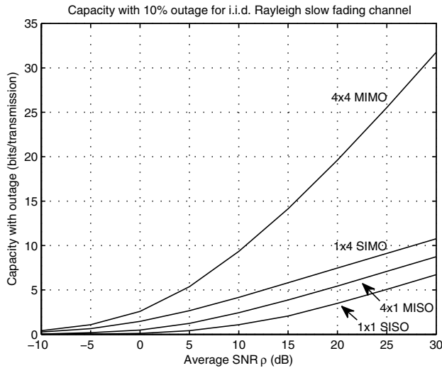
Figure 2.20 Capacity with outage at 10 dB.
