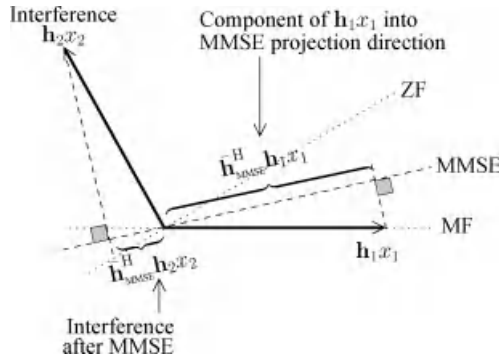
Figure 3.7 MMSE operation for a 2 \times 2 system to estimate stream 1 with channel \mathbf{h}_1 the received signal is projected into a direction that is in-between the MF and the ZF projection direction.
