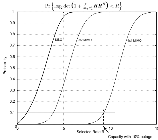
Figure 2.19 Cumulative distribution functions of the maximal achievable rate at 10 dB for a SISO channel, a 2x2 MIMO channel and a 4x4 MIMO channel. The capacity with 10% outage can easily be determined from the CDF.
