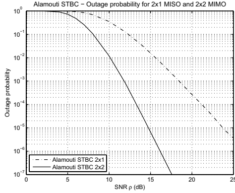
Figure 3.26 Outage probability of the Alamouti STBC for a 2×1 MISO and 2×2 MIMO system and an i.i.d. Rayleigh slow fading channel model (with E|h_{ij}|^2 = 1 ).
