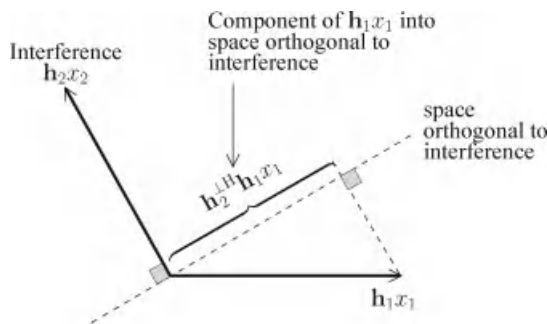
Figure 3.5 ZF operation for a 2 \times 2 system: to estimate stream 1 with channel \mathbf{h}_1 , the received signal is projected into the space orthogonal to the interference.
