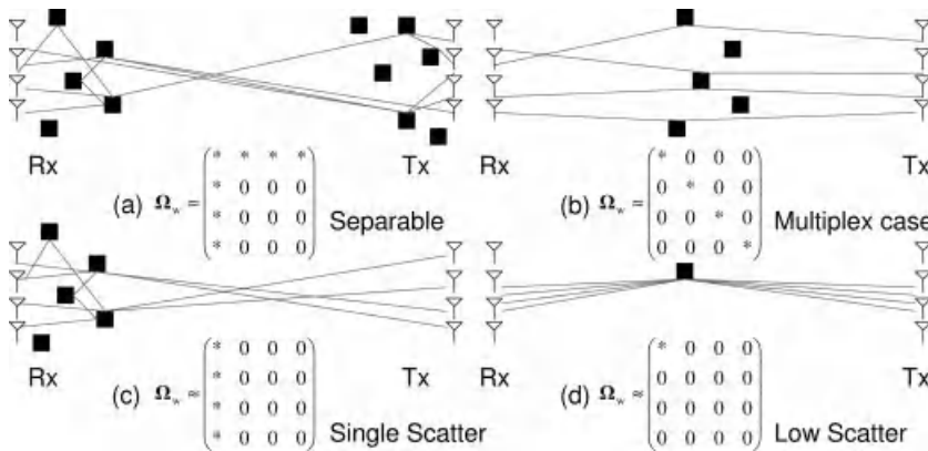
Figure 4.18 Illustration of the parameters applied in the Weichselberger model that can be applied to define physical channel states.
