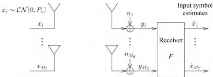
Figure 3.1 General spatial multiplexing structure. M_T packets are sent from M_T transmitting antennas and received at M_R antennas.
