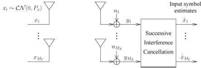
Figure 3.8 V-Blast architecture.
