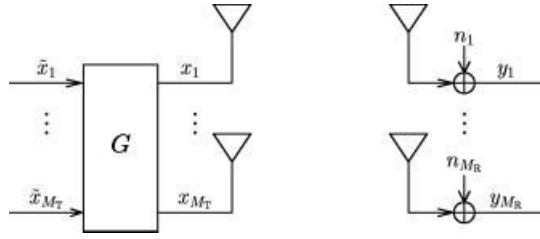
Figure 2.14 MIMO System with fixed input covariance matrix \mathbf{R}_{\mathbf{xx}} = \mathbf{G}\mathbf{G}^H .
