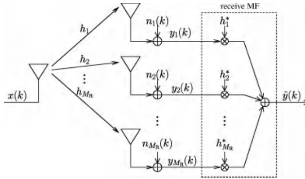
Figure 2.6 SIMO system model with receive beamforming.
