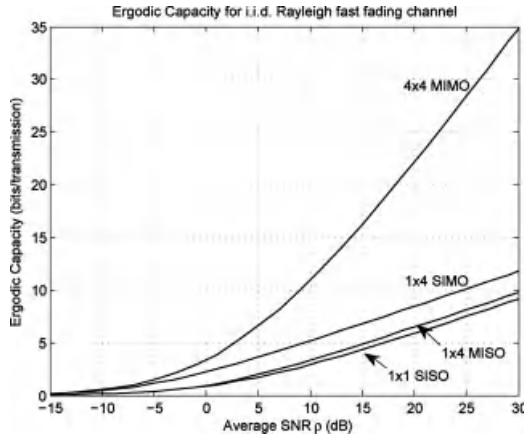
Figure 2.16 Capacity vs SNR \rho .
