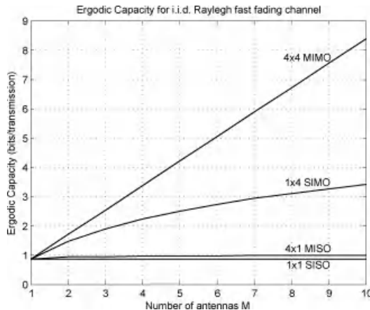
Figure 2.15 Capacity vs number of antennas for a M \times M MIMO system, a 1 \times M SIMO system, a M \times 1 MISO system and a SISO system.
