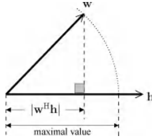
Figure 3.3 SIMO case with two receive antennas and a real channel. The amplitude of the inner product \mathbf{w}^H \mathbf{h} (with \|\mathbf{w}\|^2 = 1 ) is maximised when \mathbf{h} and \mathbf{w} are aligned.
