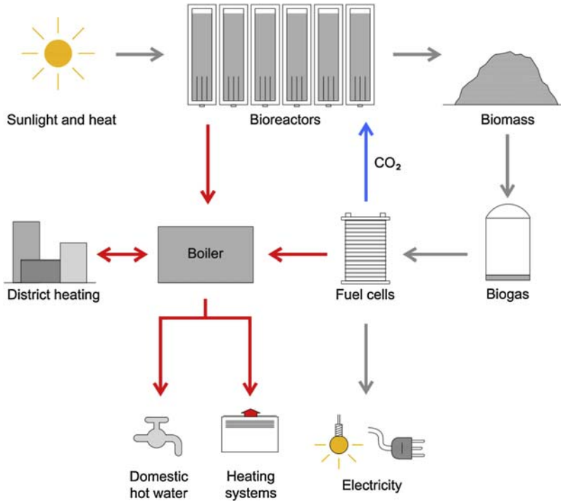
Figure 10.29 Bioadaptive facade operating scheme.
