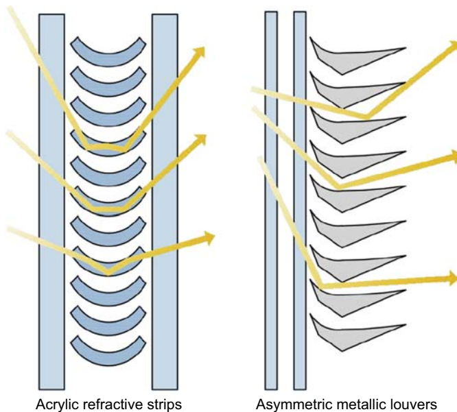
Figure 8.7 Light-redirection louver systems.
