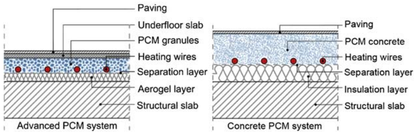
Figure 5.24 Underfloor phase-change material (PCM) application.
