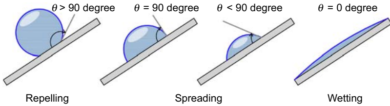
Figure 8.2 Surface wettability and contact angle \theta .
