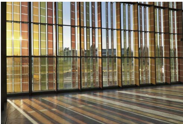
Figure 10.16 SwissTech Congress Center DSSC facade. Courtesy of Solaronix SA.
