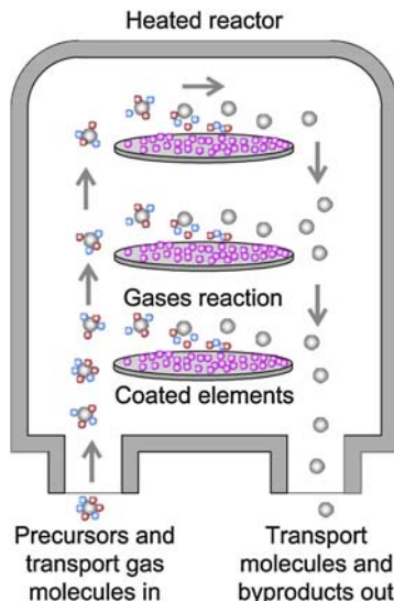
Figure 2.6 Chemical vapor deposition process.
