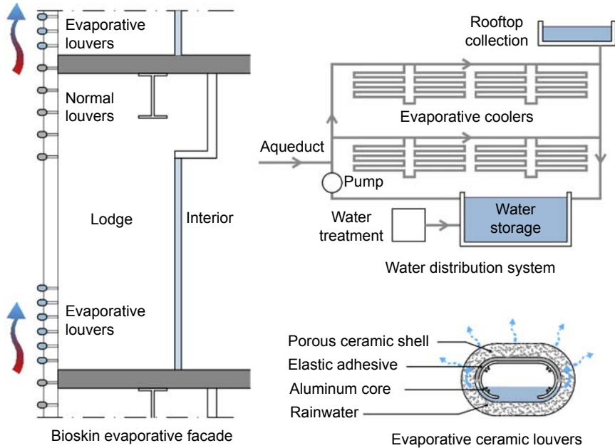
Figure 8.27 Bioskin facade system.
