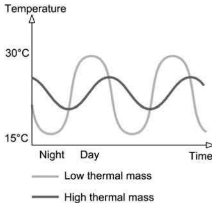
Figure 5.2 Internal temperature fluctuation and thermal mass.
