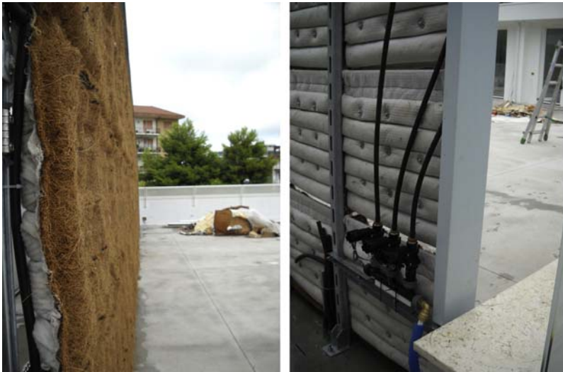
Figure 6.11 Living wall growing felt and irrigation system. Courtesy of Poliflor s.a.s.
