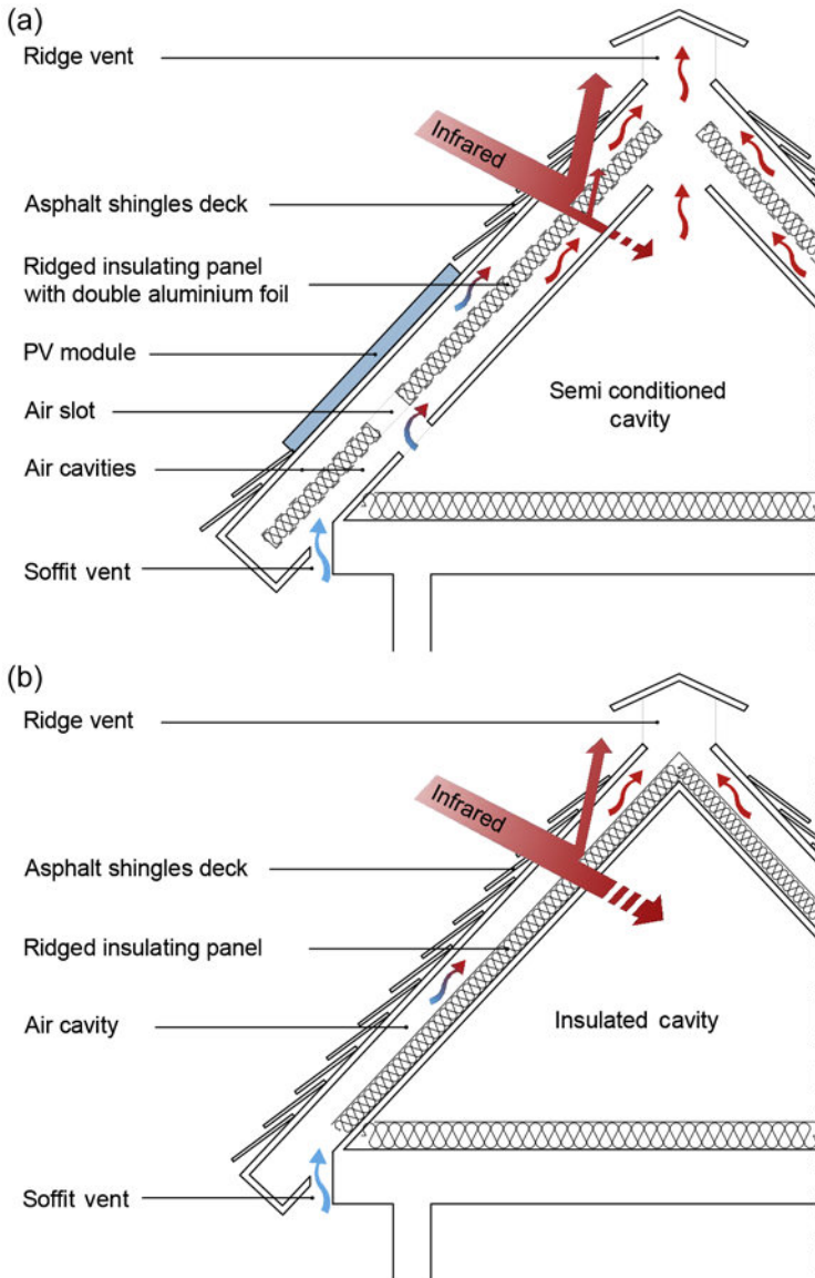
Figure 3.7 (a) Advanced and (b) traditional pitched roofs.
