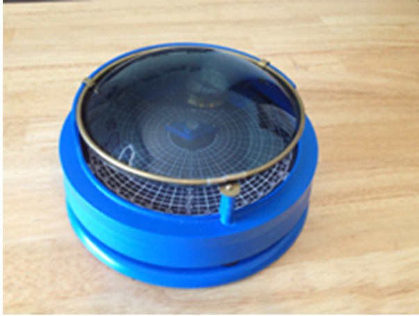
Figure 3.7. Solar pathfinder.
