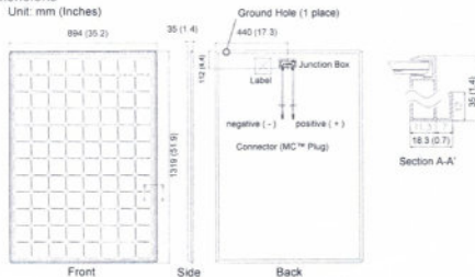
Figure B.1. Sanyo module specifications.
