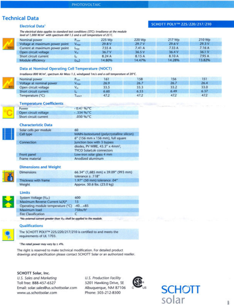
Figure B.4. Schott module specifications.
