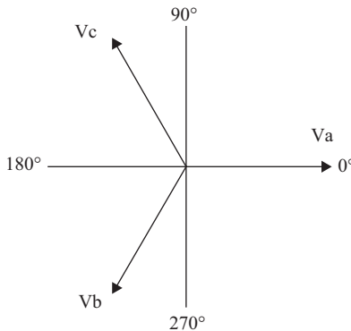
Figure 1.12. Voltage phasor diagram.
