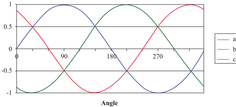
Figure 1.11. Three-phase waveforms.
