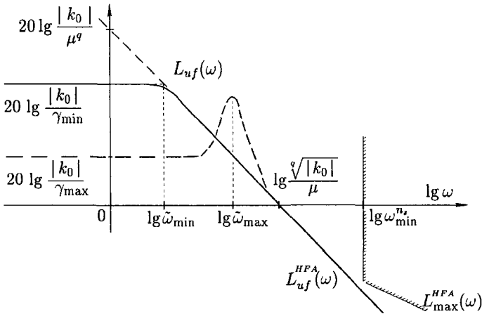
Fig. 5.12 The influence of variations in the parameter g on the bandwidth of the FMS (4.55).
