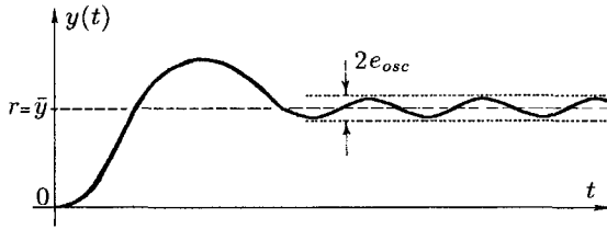
Fig. 6.20 Influence of oscillations in the FMS (6.68) on output behavior.
