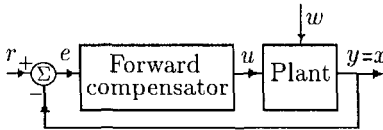
Fig. 5.1 Control law in the form of forward compensator.
