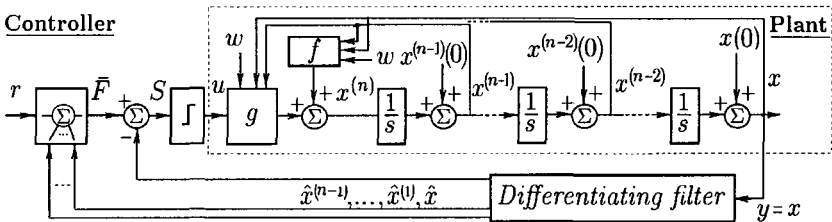
Fig. 3.13 Block diagram of the control system with sliding motions, where a differentiating filter is used.
