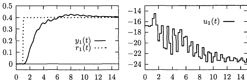
Fig. 10.5 Simulation results for r_1(t), y_1(t), u_1(t) in the system (8.46) and (10.44) given that \gamma_i = 0, \forall i = 1, 2, 3 (without delay compensation).
