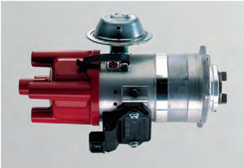
Figure 4.16 Distributors usually contain a Hall effect or inductive pulse generator (Source: Bosch Press)
