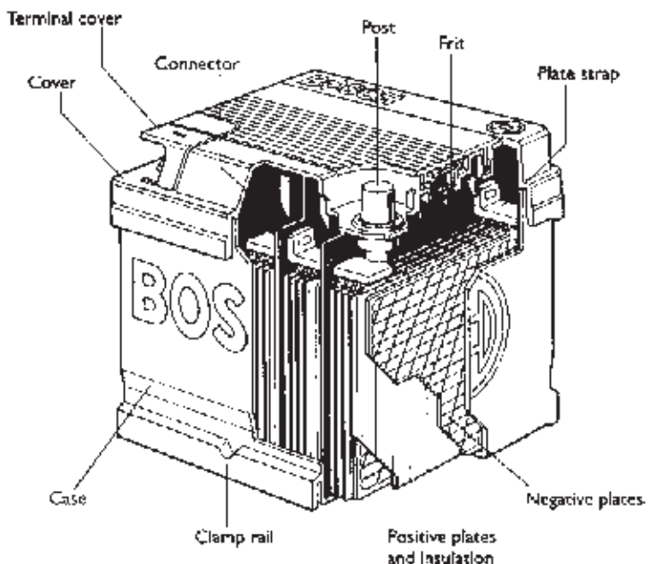
Figure 6.77 Vehicle battery components
