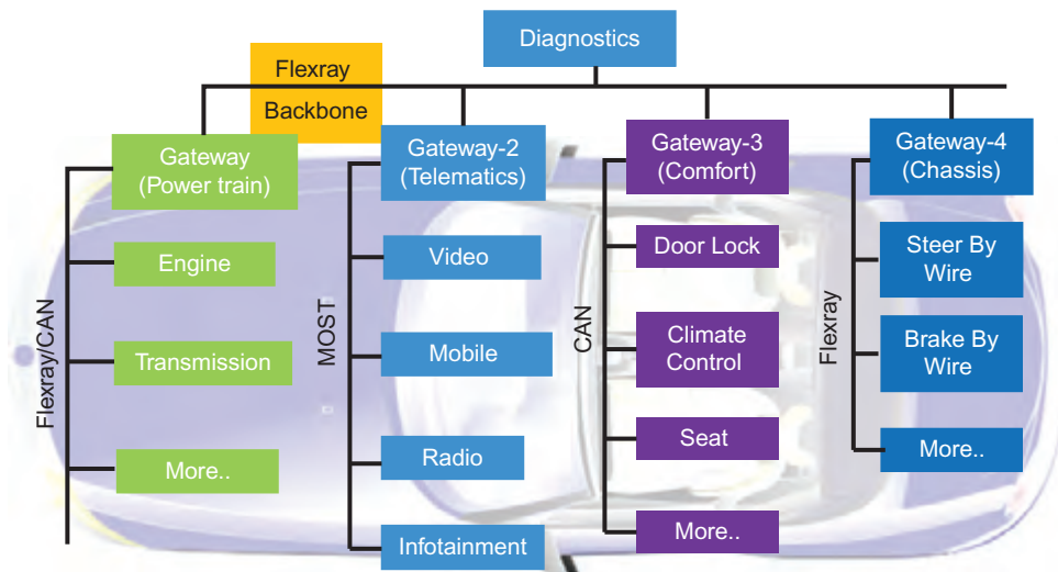
Figure 8.15 FlexRay backbone
