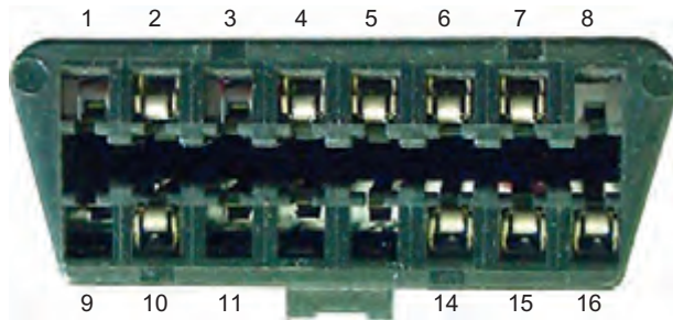
Figure 8.19 16 Pin data link connector
