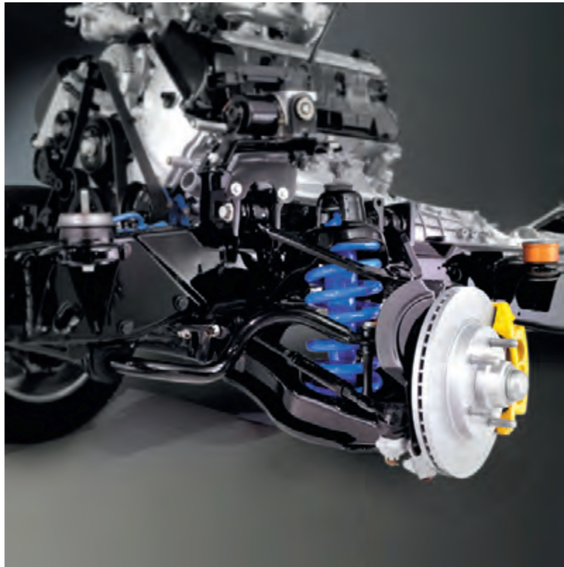
Figure 2.5 Mechanical systems
