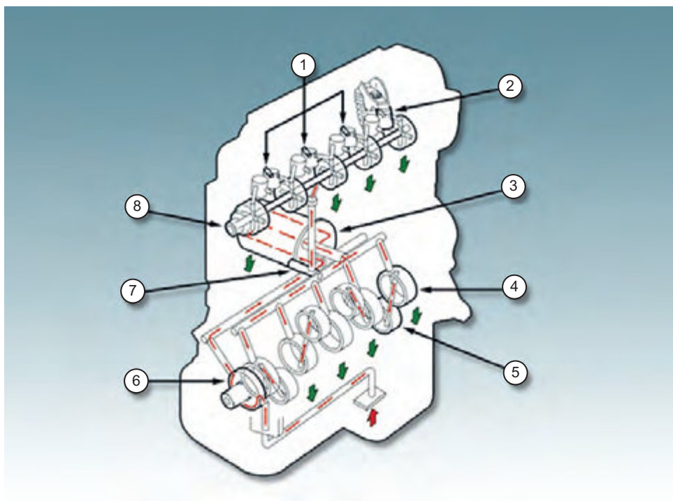
Figure 6.74 Oil flow: 1 – oil to rocker arms; 2 – hydraulic tappets; 3 – oil to crank main bearings; 4 – crank main bearings; 5 – big-end bearings; 6 – crank driven oil pump; 7 – oil under pressure; 8 – camshaft
