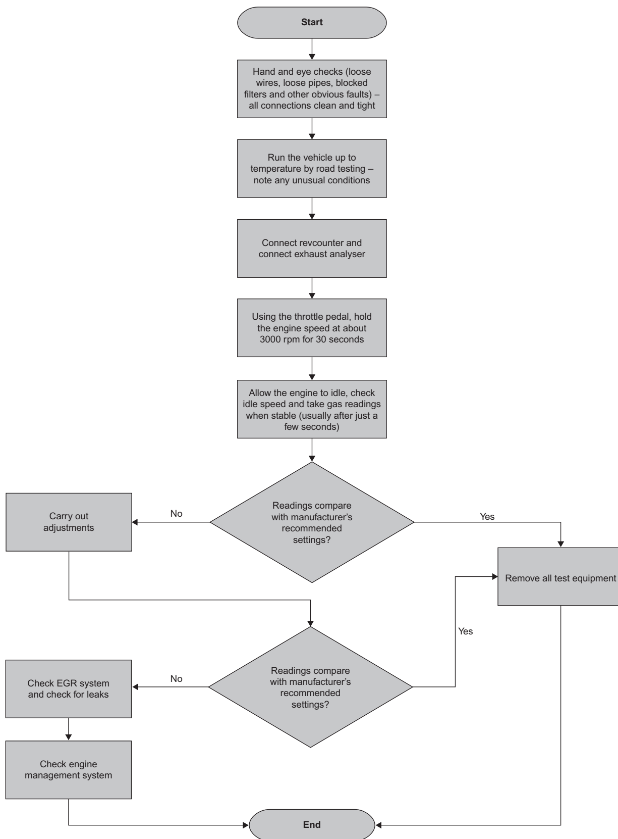
Figure 6.40 Emissions systems diagnosis chart
