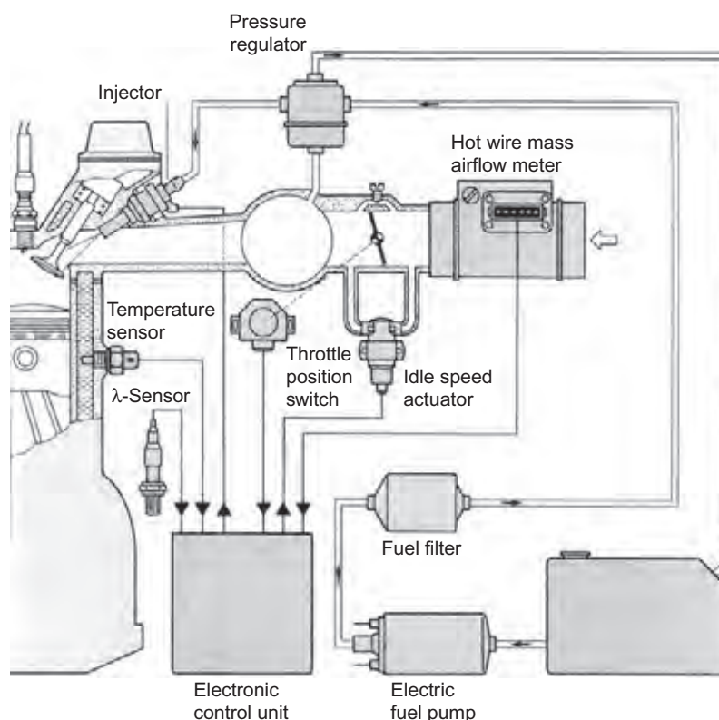
Figure 6.42 Fuel injection system layout
