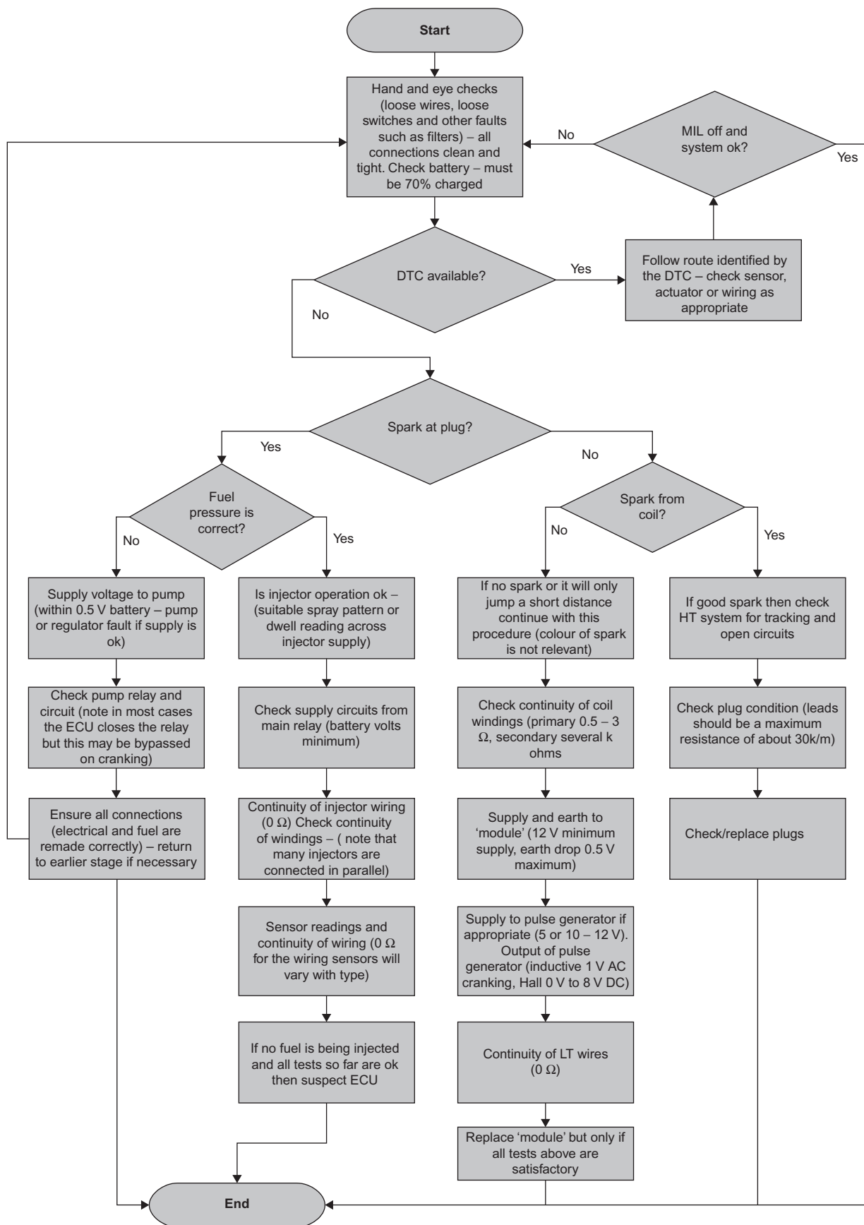
Figure 6.64 Engine management faultfinding chart
