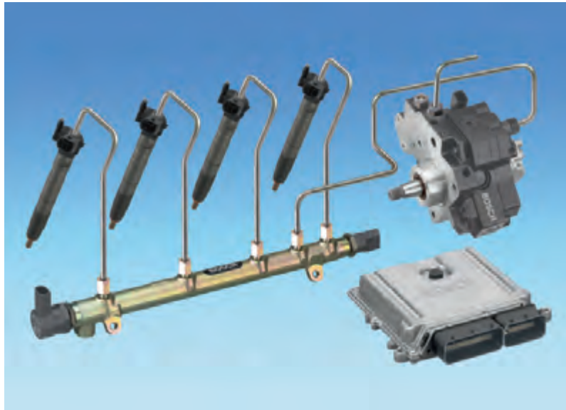
Figure 4.51 Common rail diesel pump, rail, injectors and ECU (Source: Bosch Press)
