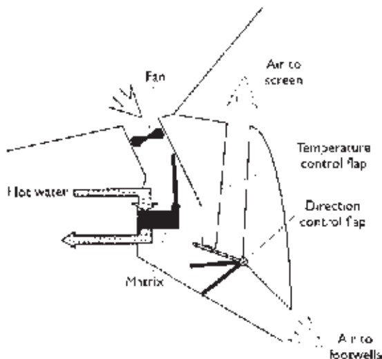
Figure 8.71 Heating and ventilation system
