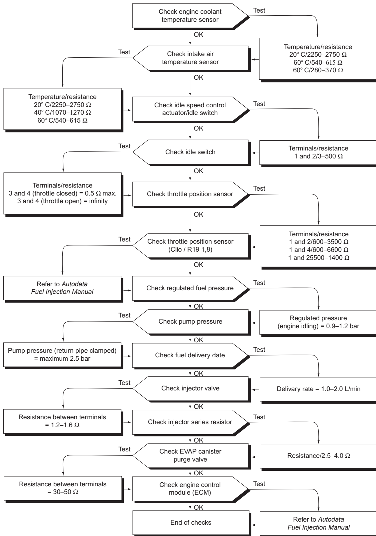
Figure 6.67 Fault finding chart
