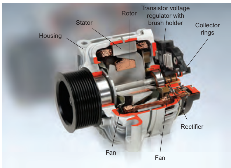
Figure 6.91 Alternator components
