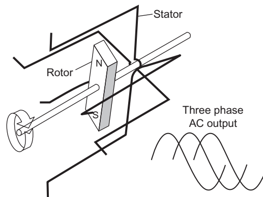
Figure 6.92 Alternator principle
