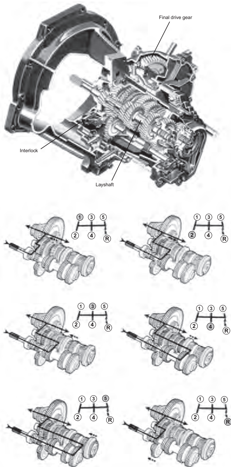
Figure 9.4 Five-speed manual gearbox and powerflw
