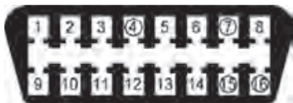
Figure 3.7 Connector pin-out: 4 – battery ground/earth, 7 – K-line, 15 – L-line, 16 – battery positive
