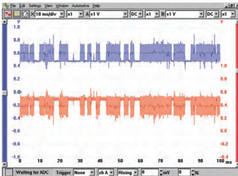
Figure 8.17 CAN signals
