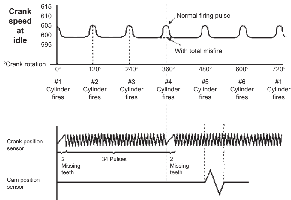
Figure 5.20 Misfire detection via crank sensor
