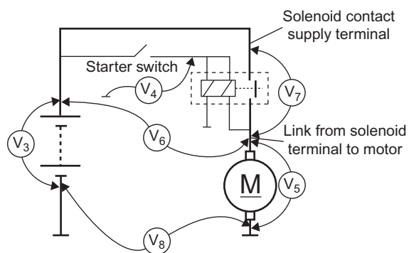
Figure 6.89 Starter circuit testing
