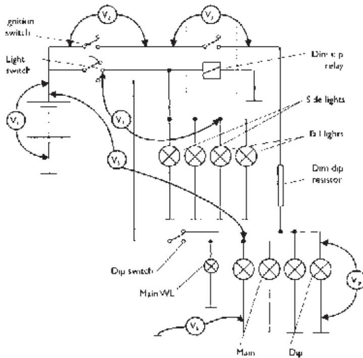
Figure 8.29 Lighting circuit under test
