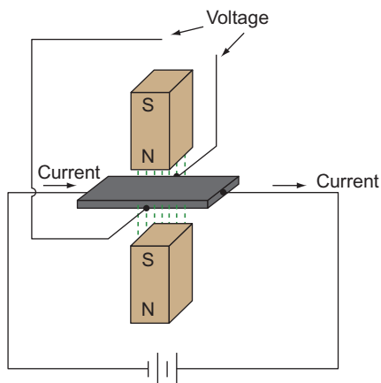
Figure 4.15 Hall effect
