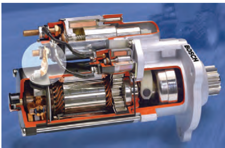
Figure 6.90 The link from the solenoid contacts and the motor is highlighted in this image
