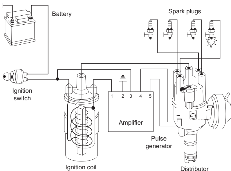
Figure 6.19 Early electronic ignition system
