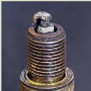
Figure 6.36 Overheating
