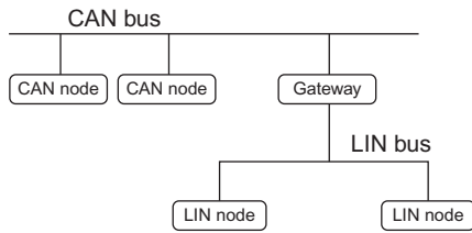
Figure 8.12 Structure using CAN and LIN
