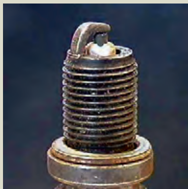
Figure 6.34 Damaged insulation
