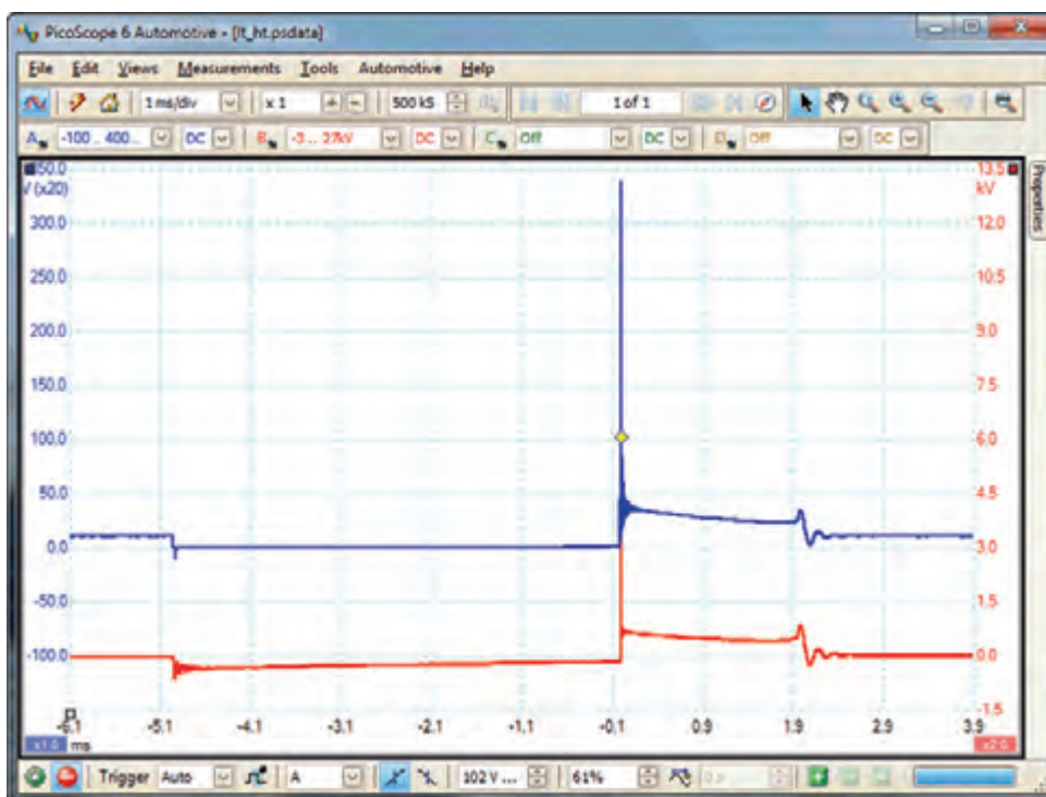
Figure 4.62 Distributorless ignition showing low and high tension (primary and secondary)
