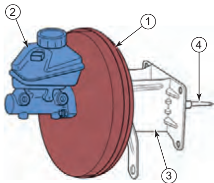
Figure 7.5 Servo unit: 1 – brake servo (booster); 2 – master cylinder and reservoir; 3 – bracket; 4 – diaphragm rod connection to brake pedal
