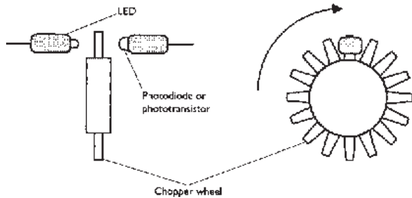
Figure 4.34 Optical sensor
