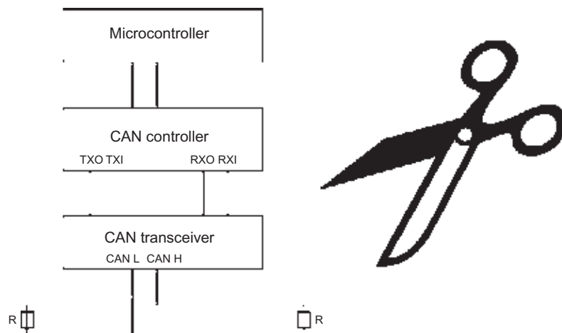
Figure 8.10 CAN nodes can be disconnected by the control program
