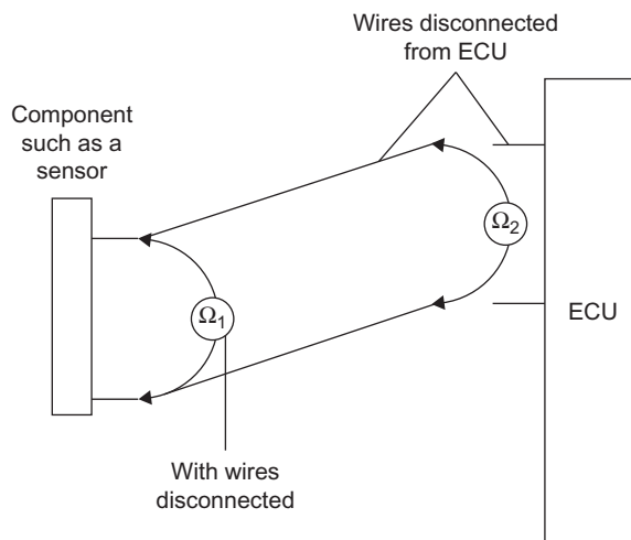
Figure 2.10 Ohmmeter testing
