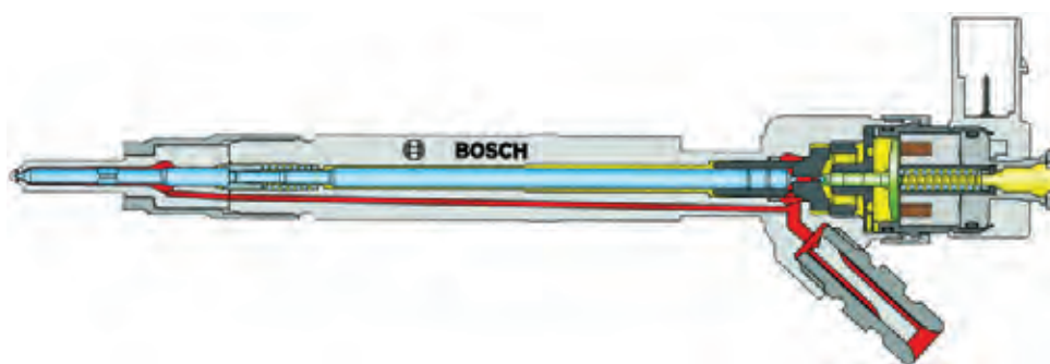
Figure 6.51 Electrically operated diesel fuel injector
