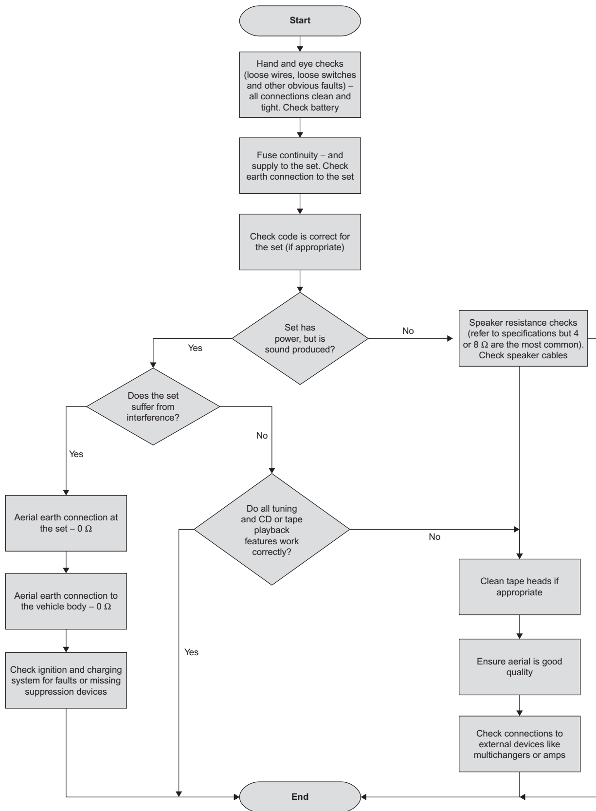
Figure 8.51 ICE system diagnosis chart
