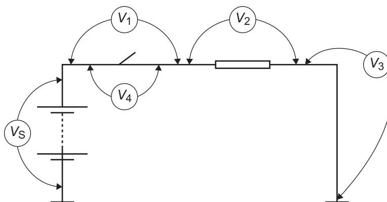
Figure 2.8 Volt drop testing
