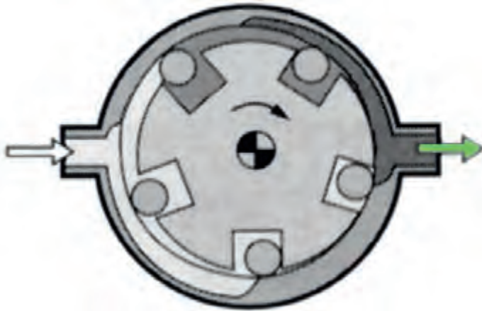
Figure 6.61 Roller cell pump (2)
