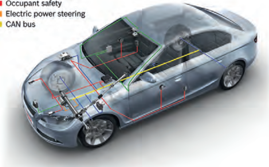
Figure 8.6 A data bus connects all networked components
