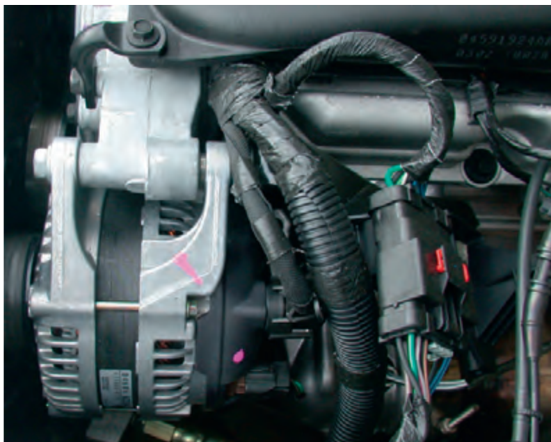
Figure 2.6 Electrical system
