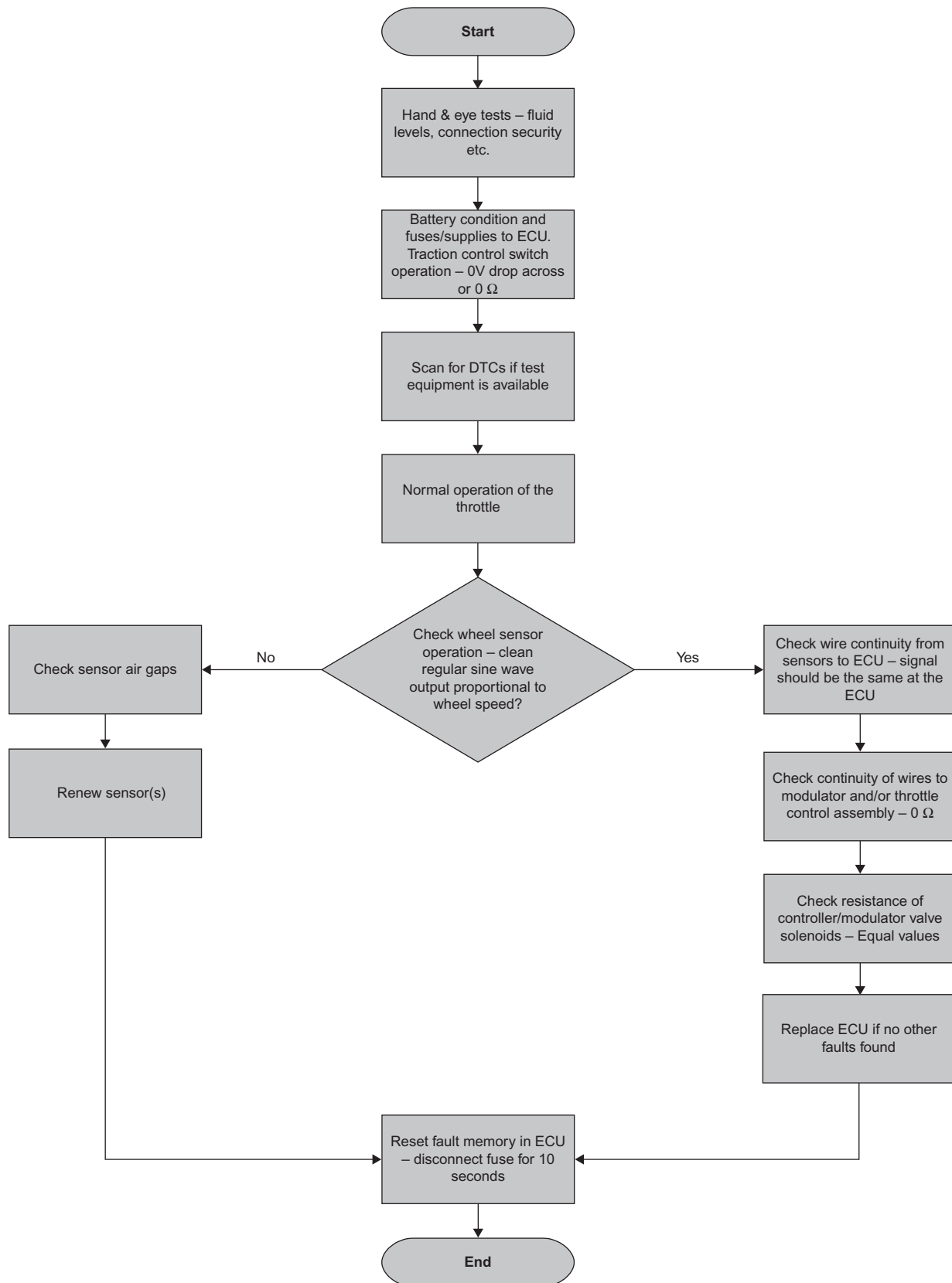
Figure 7.14 Traction control diagnosis chart
