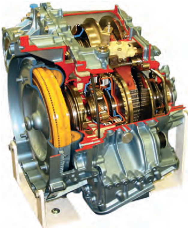
Figure 9.11 Constantly variable transmission (Source: Ford Media)
