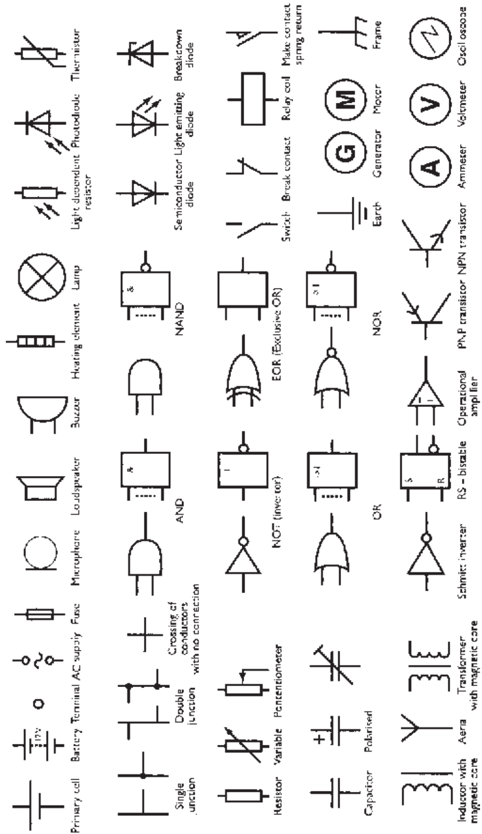
Figure 8.1 Circuit symbols
