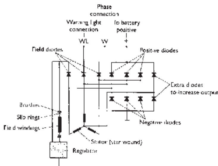
Figure 6.93 Alternator internal circuit
