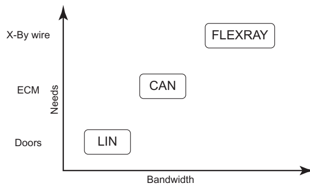
Figure 8.16 Comparing requirements and data rates of the three systems
