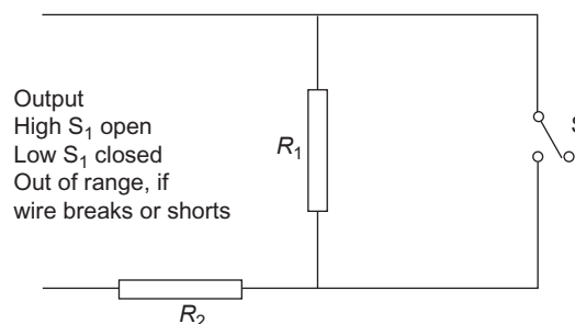
Figure 8.66 Dual-resistance self-testing system
