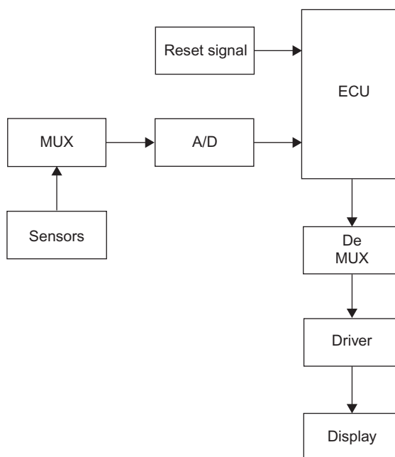
Figure 8.63 Digital instrumentation block diagram
