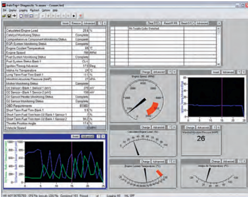
Figure 3.9 Screen grab from the Autap software showing tables, gauges and graphs
