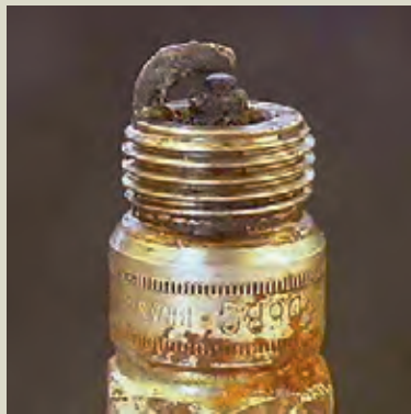
Figure 6.33 Deposits
