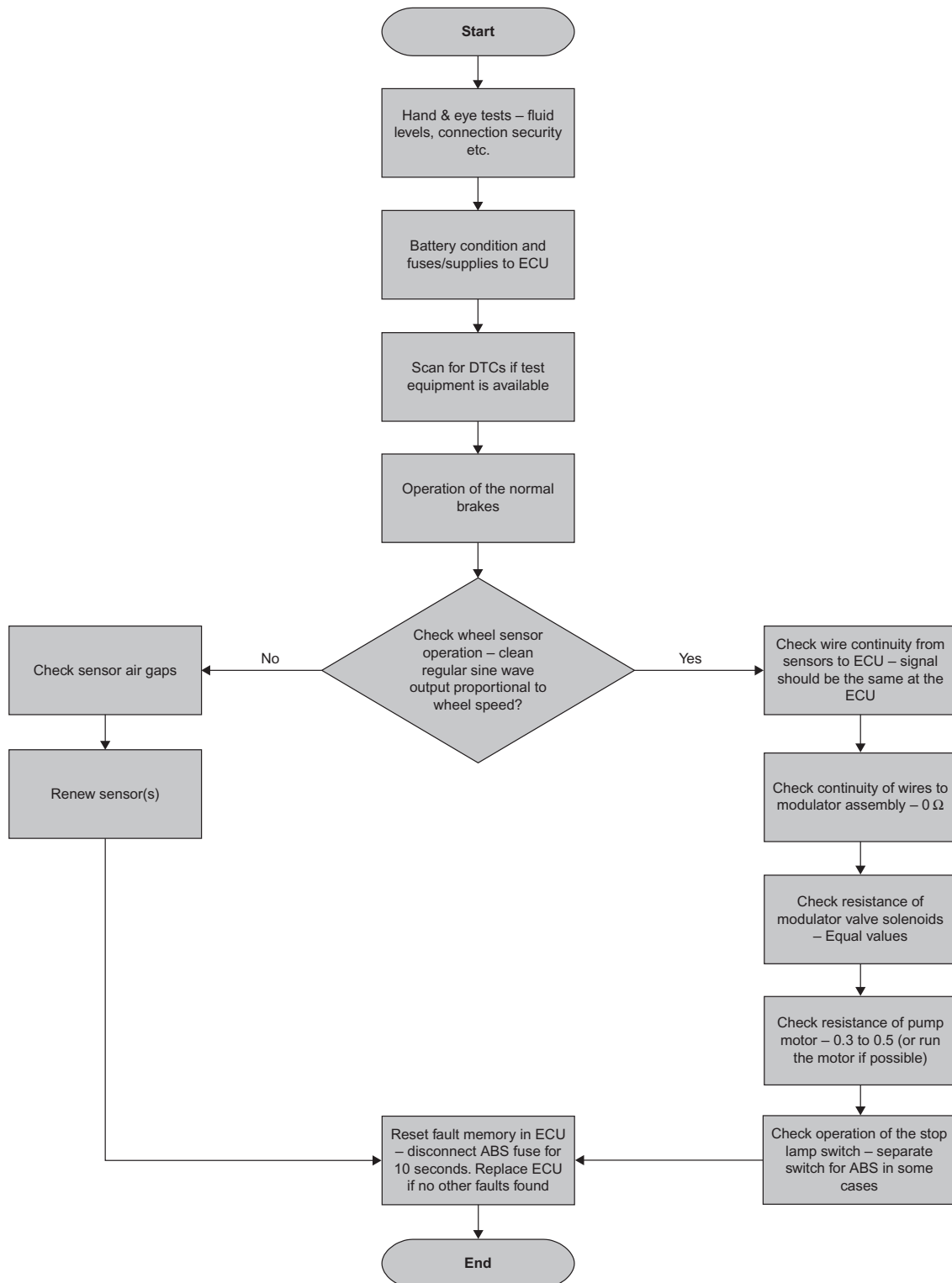
Figure 7.11 ABS diagnosis chart
