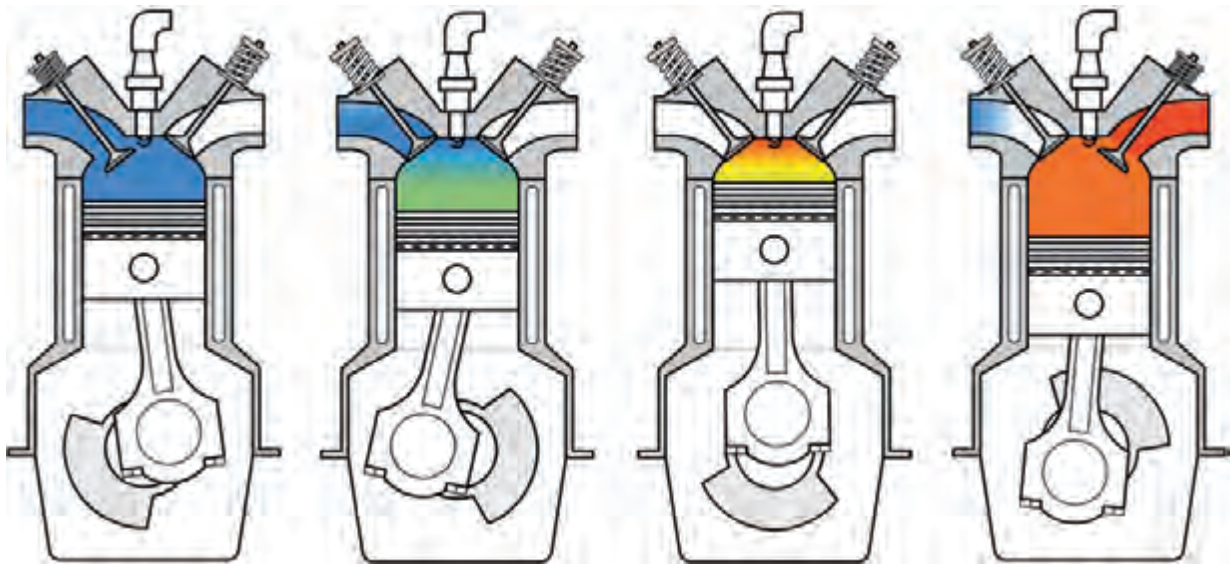
Figure 6.2 Four-stroke cycle: induction, compression, power and exhaust
