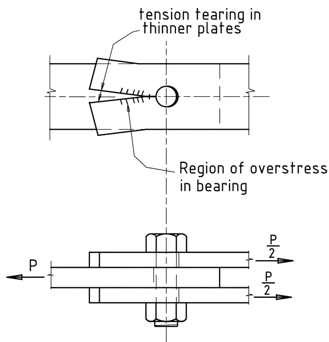
Figure 3-3. Tension tear-out failure.
