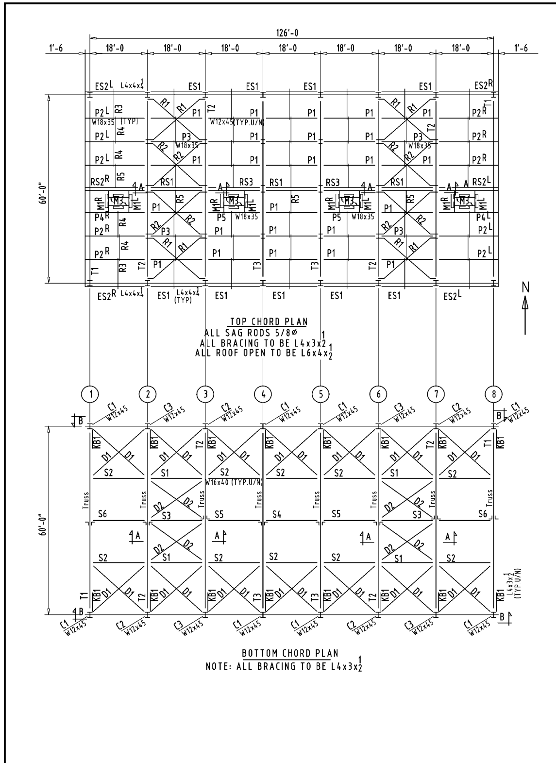
Figure 6-1a. Erection drawing.
