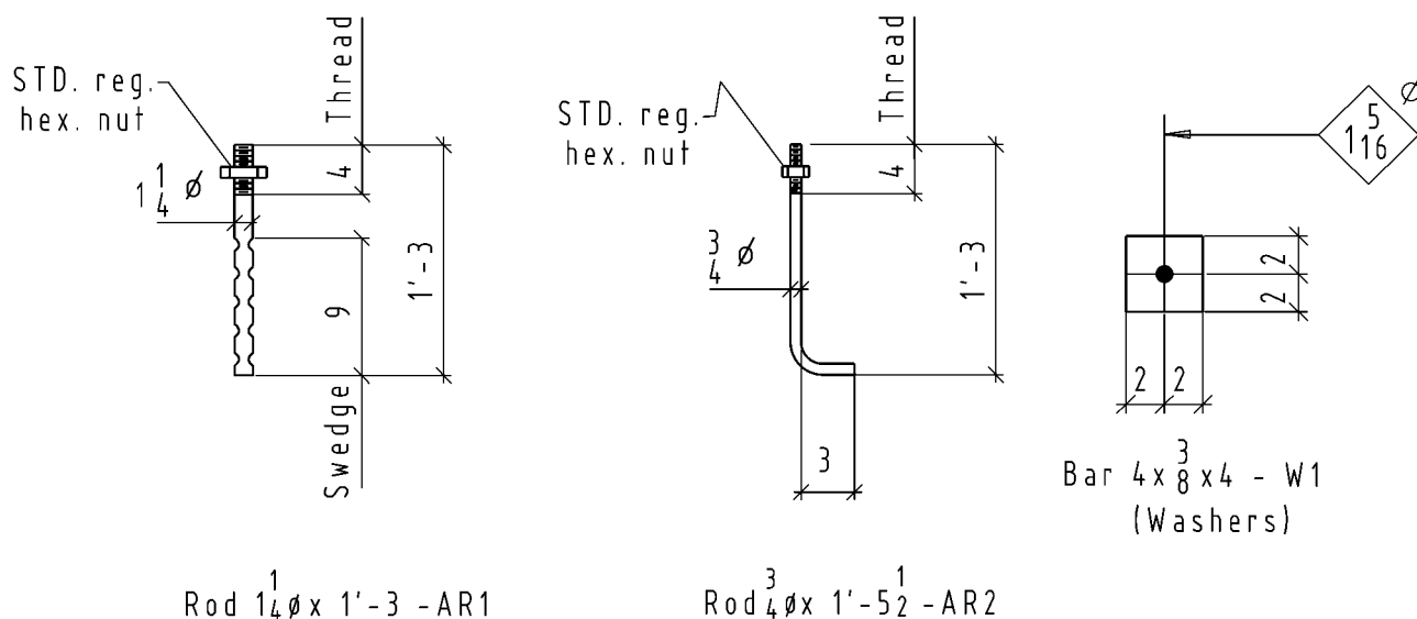
Figure 7-7. Typical anchor rod details.
