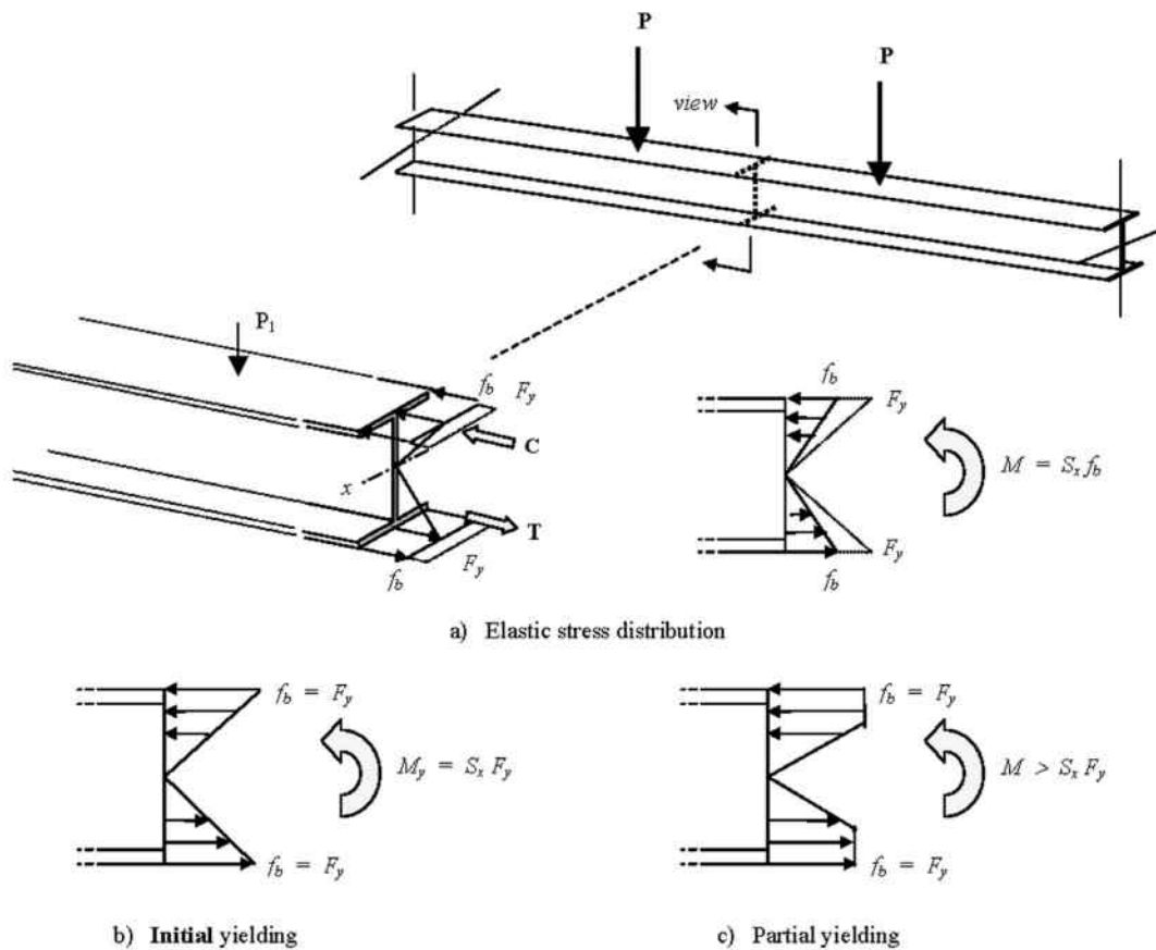
Figure B-19. Yielding failure of a steel beam.
