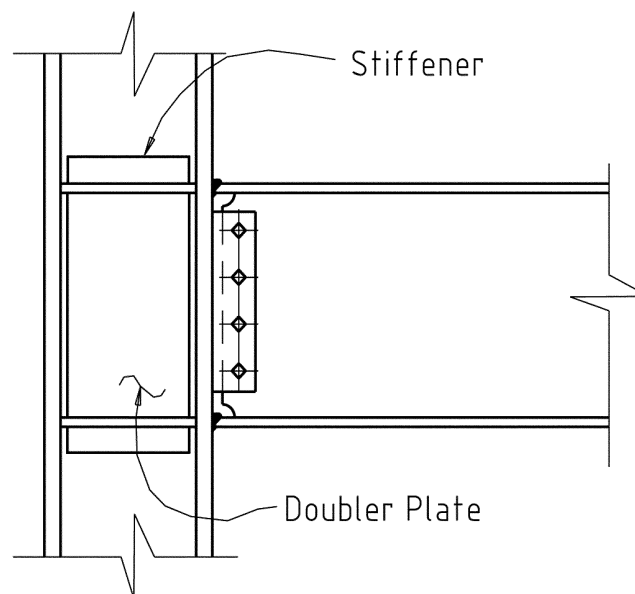
Figure 2-5. Typical moment connection.
