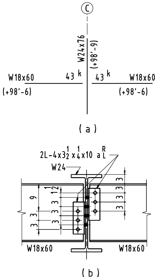
Figure 7-30. Staggered shop and field bolts.
