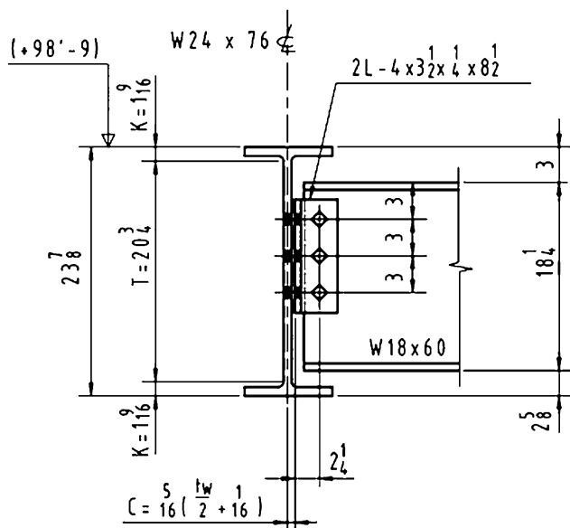
Figure 3-6. Bolted double-angle connection.
