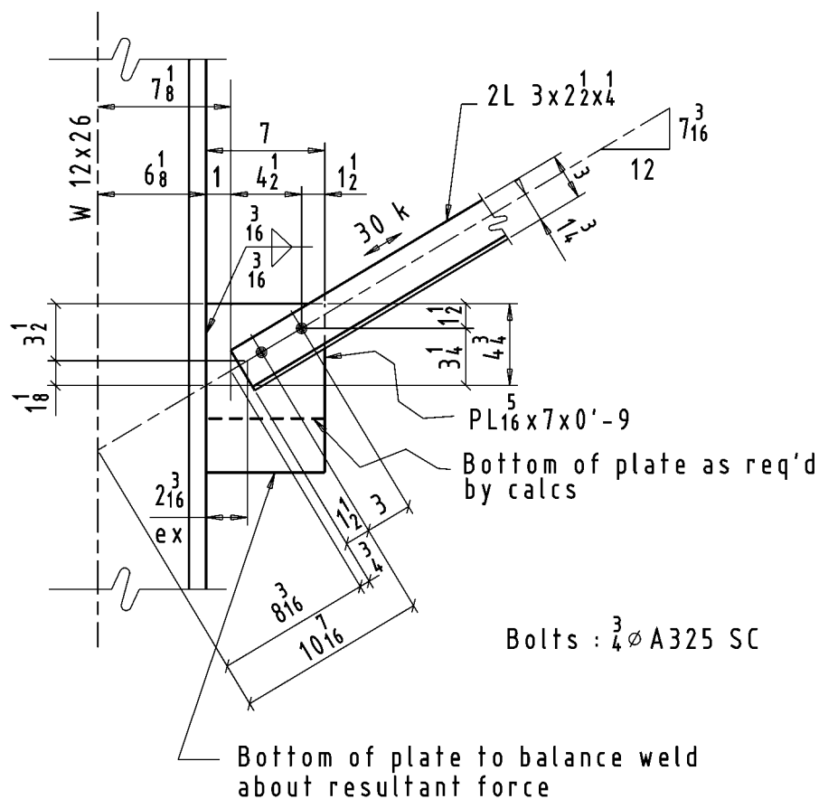
Figure 7-64. Knee brace detail.
