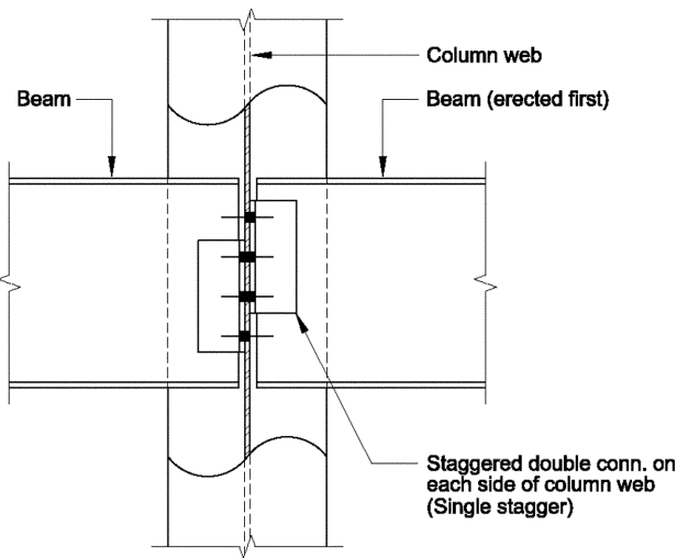
Figure 2-13. Single-staggered stabilization of beam's top flange.
