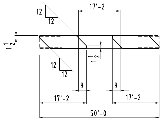
Figure 7-27. Nested or multiplied pieces.
