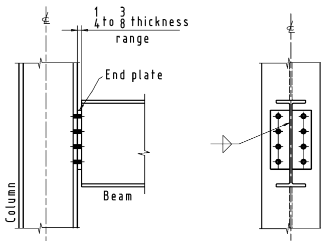
Figure 3-8. Typical end-plate connection to a column flange.
