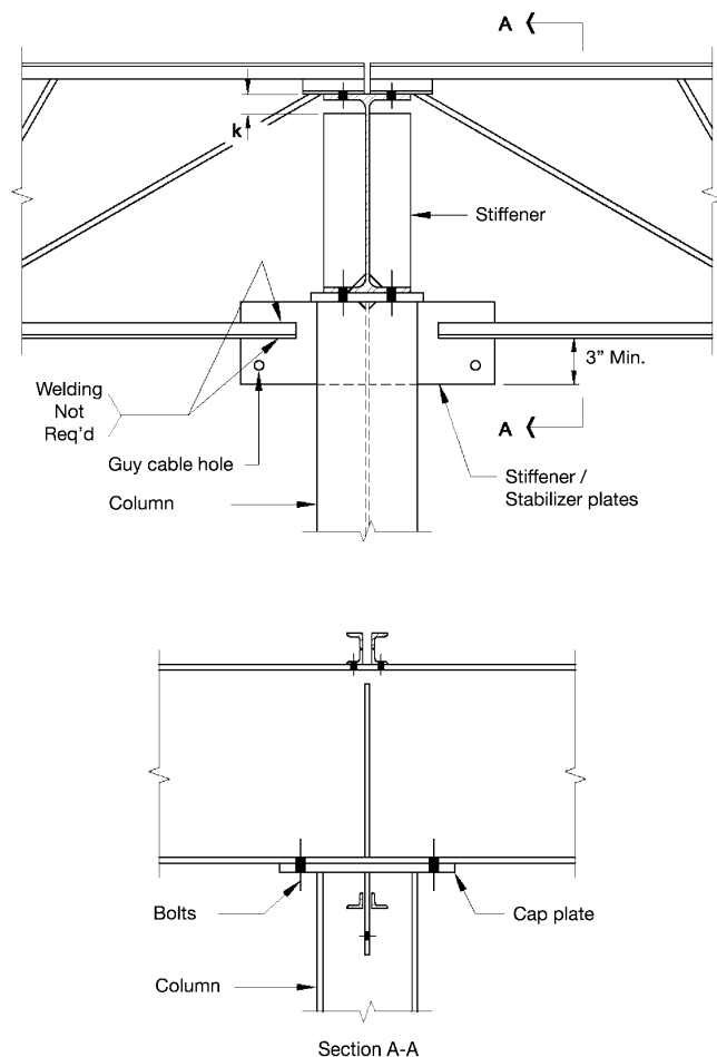
Figure 2-18. Strut joist with stiffener and stabilizer plate.
