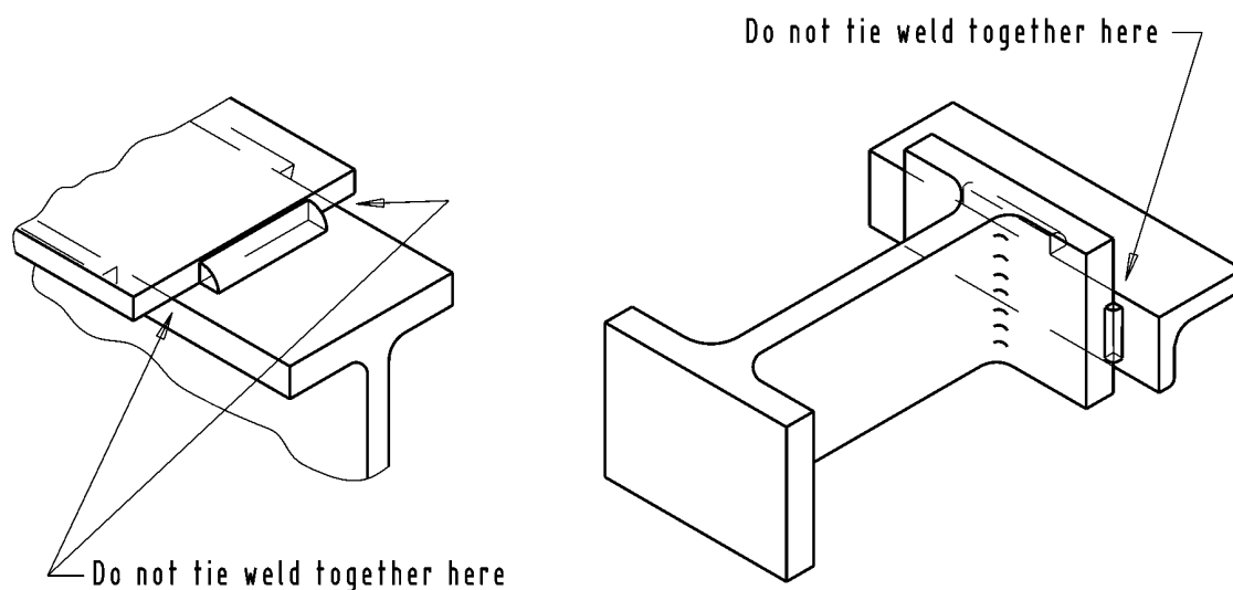
Figure 3-25. Seat angle weld arrangement.
