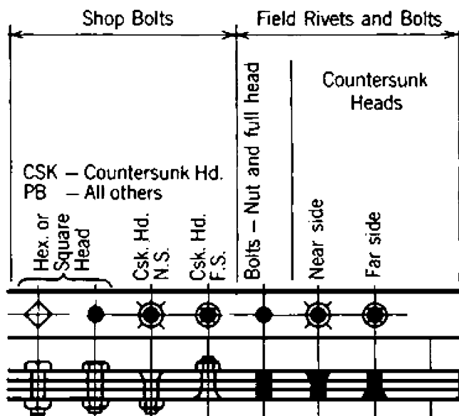
Figure 4-8. Conventional signs or symbols for bolts.
