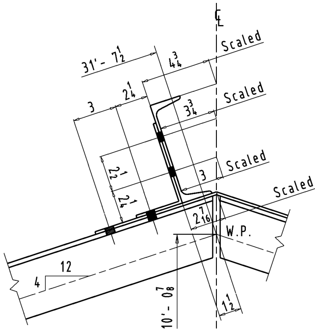
Figure 7-72. Scaled layout.
