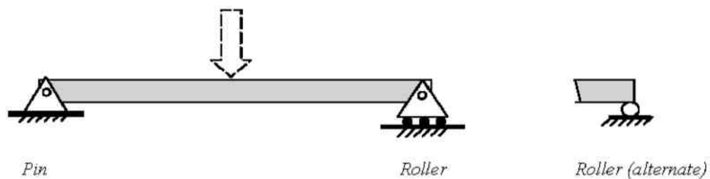
a) Idealized beam and support details
