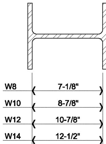
Figure 2-12. Approximate clear distance between column flanges.
