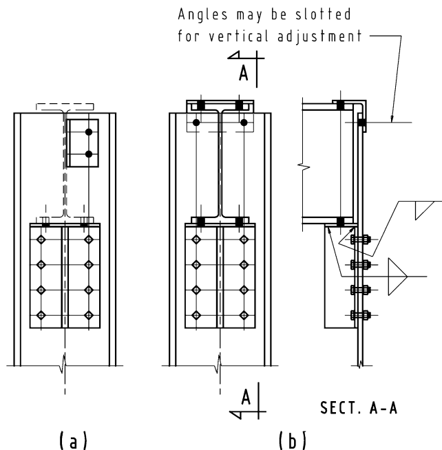
Figure 7-26. Methods of providing lateral support.
