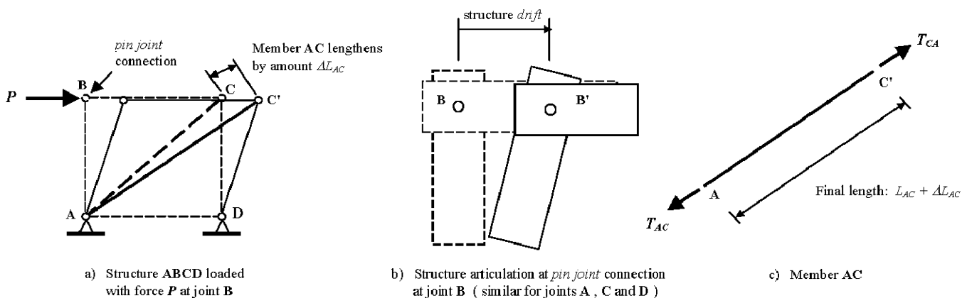
Figure B-1. Tension member—diagonal bracing.
