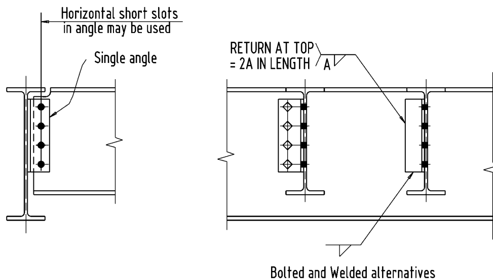
Figure 3-14. Single-angle connection.
