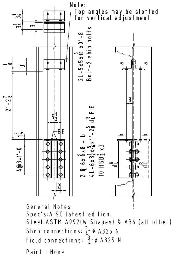
Figure 7-25. Detailed stiffened seat.
