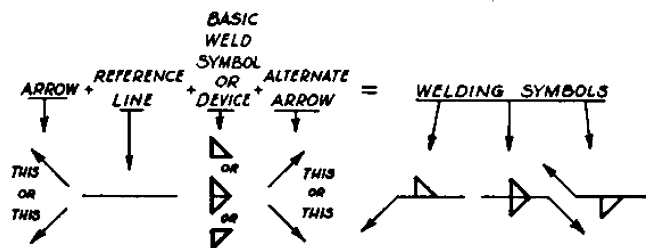
Figure 4-21. Fillet weld symbol.
