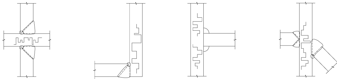
Figure 4-9. Weld configurations that can cause weld distress from shrinkage.
