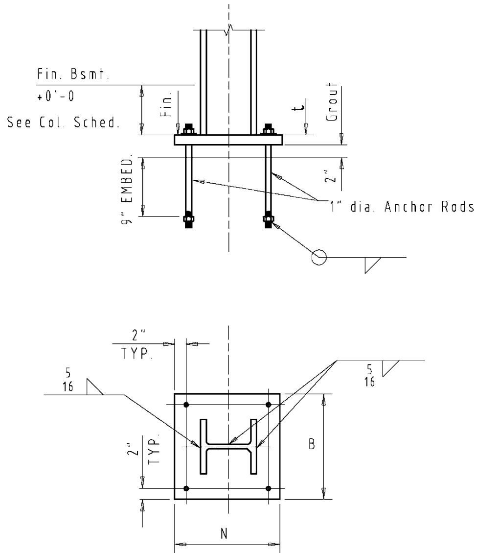
TYPICAL COLUMN BASE PLATE
