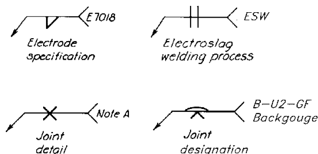
Figure 4-22. Weld symbols.
