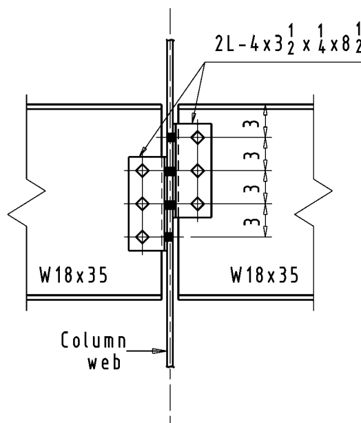
Figure 6-10. Staggered connections.
