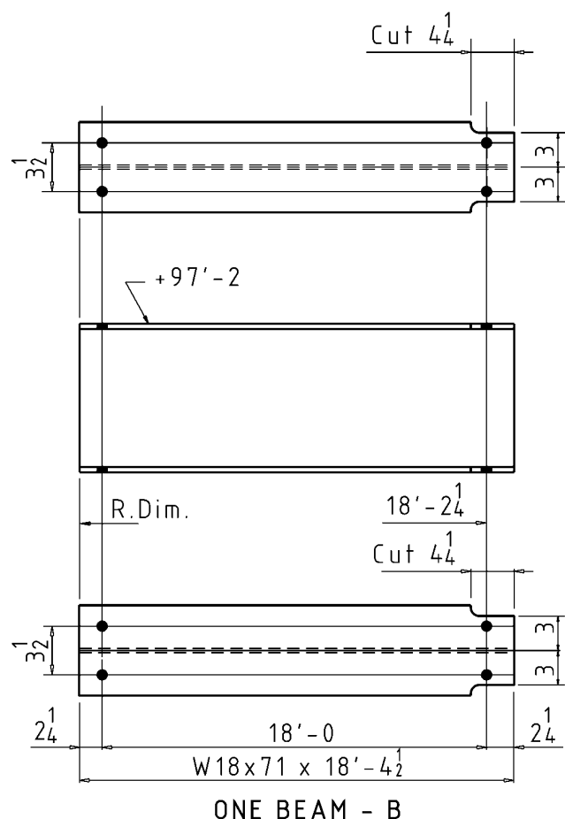
Figure 7-38. Completely developed shop detail of beam B with top and bottom views.
