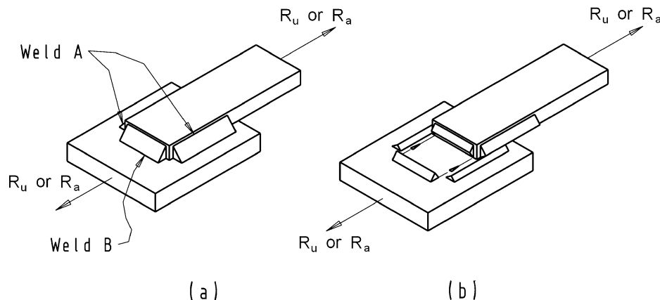
Figure 3-17. Fillet weld shear failure.
