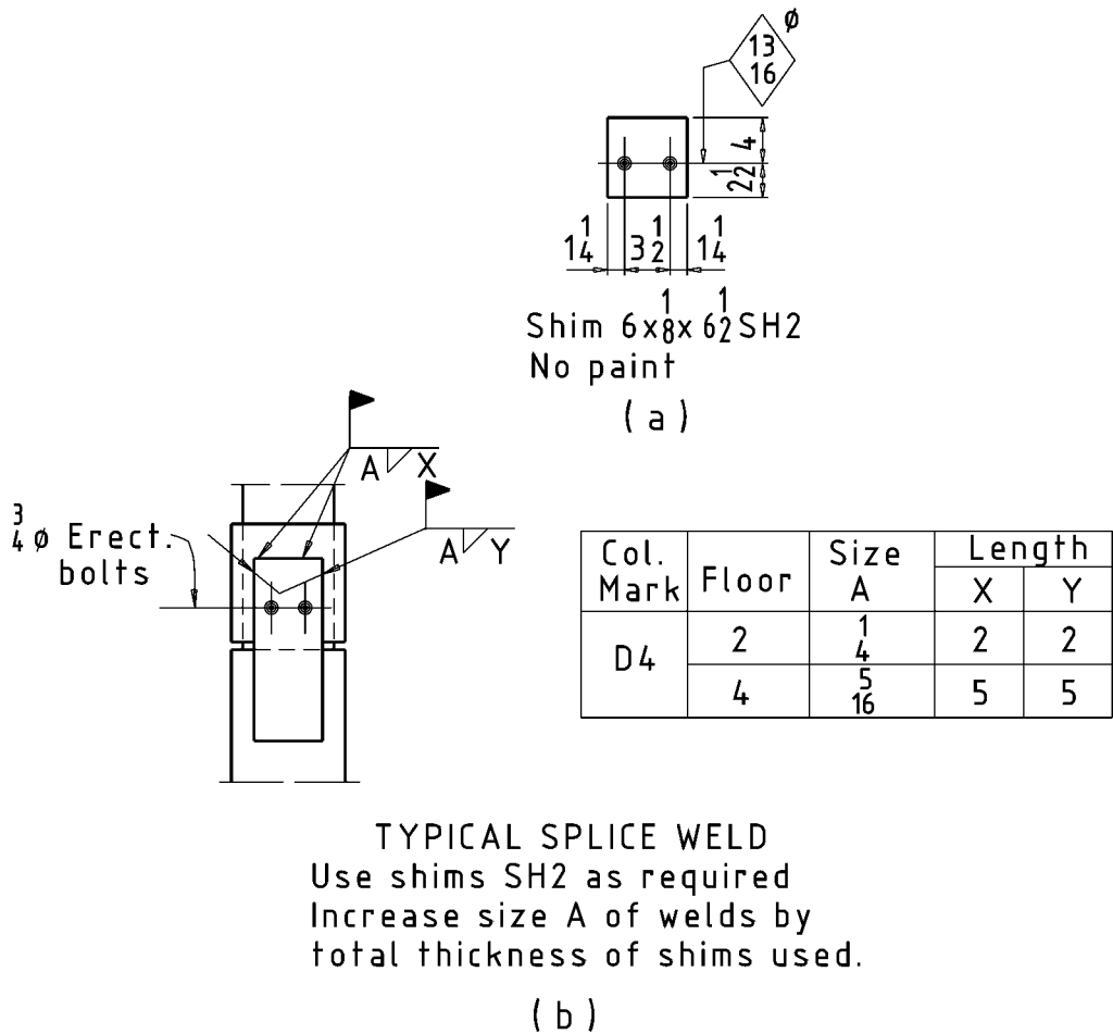
Figure 7-41. Typical splice weld.
