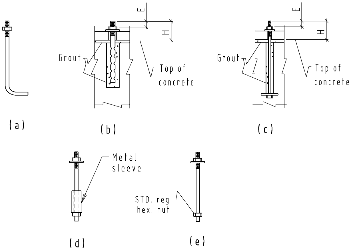
Figure 7-6. Anchor rods.
