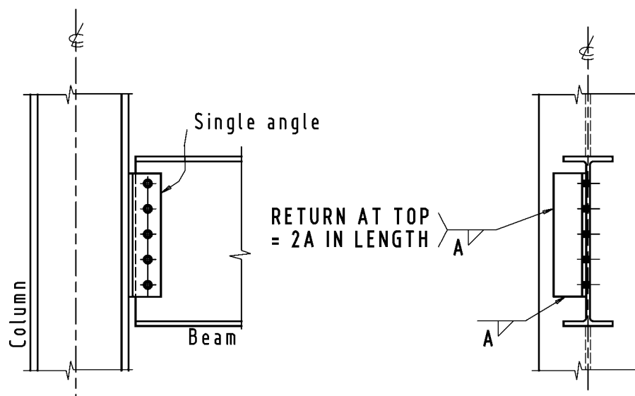
Figure 3-34. Single-angle connection shop attached to the column.
