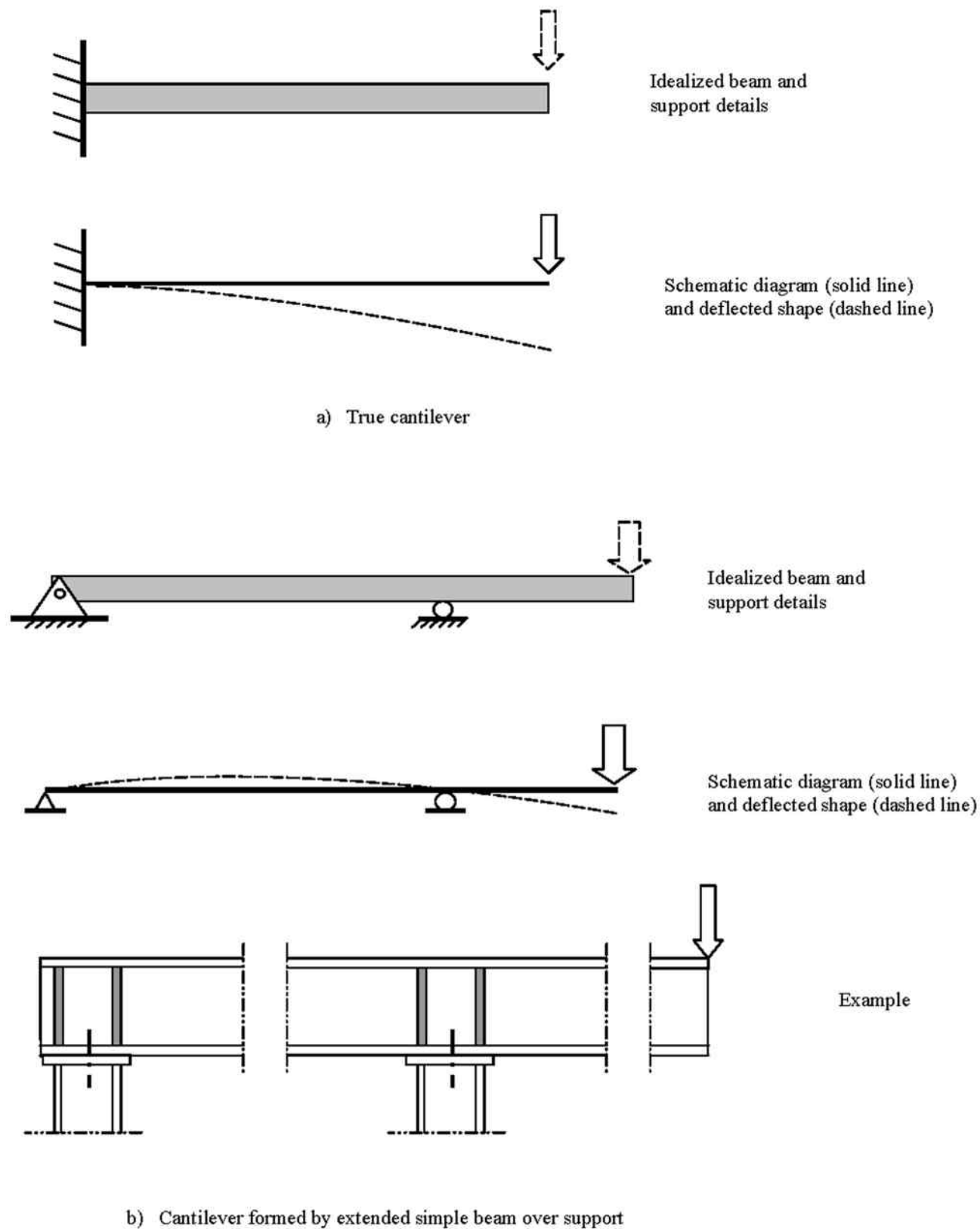
Figure B-5. Cantilevered beam.
