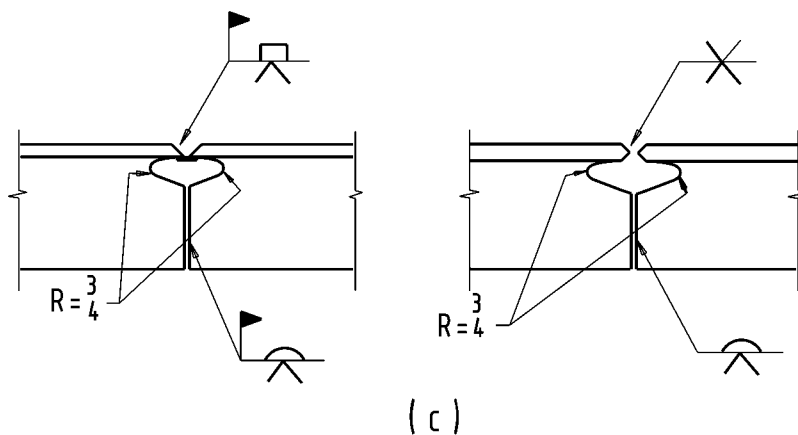
Figure 3-47. Welded truss-chord splices.
