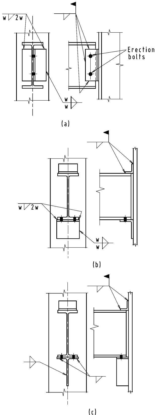
Figure 3-30. All-welded framed connections.
