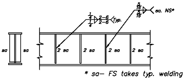
Figure 4-27. Typical welded joint.
