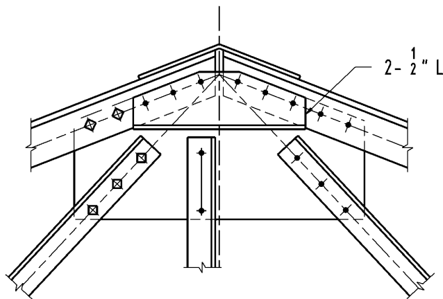
Figure 7-50. Stiffening angles at truss peak.
