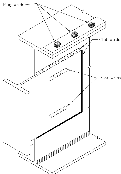
Figure 4-16. Slot welds used in conjunction with fillet welds to stitch a wide area of tee stem to a beam web.
