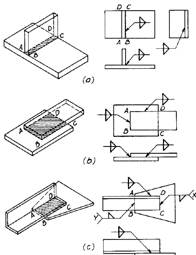
Figure 4-23. Fillet welds.
