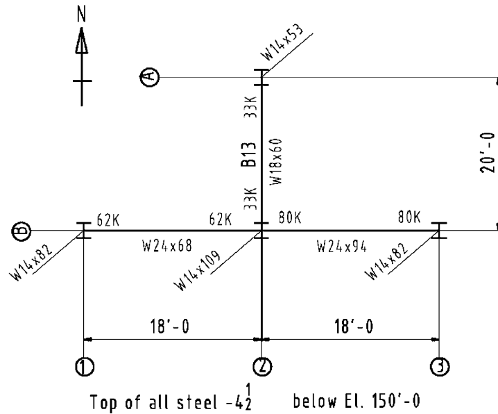
PART PLAN
