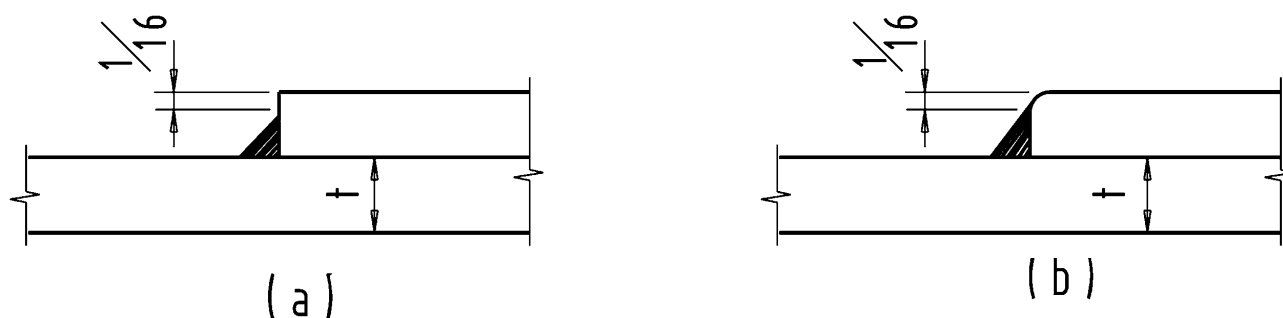
Figure 3-18. Resultant fillet weld dimensions.
