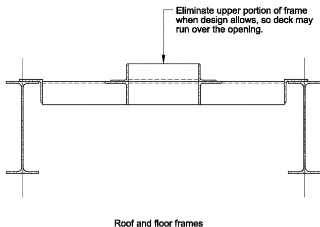
Figure 2-8. Continuous structural supports for deck openings.
