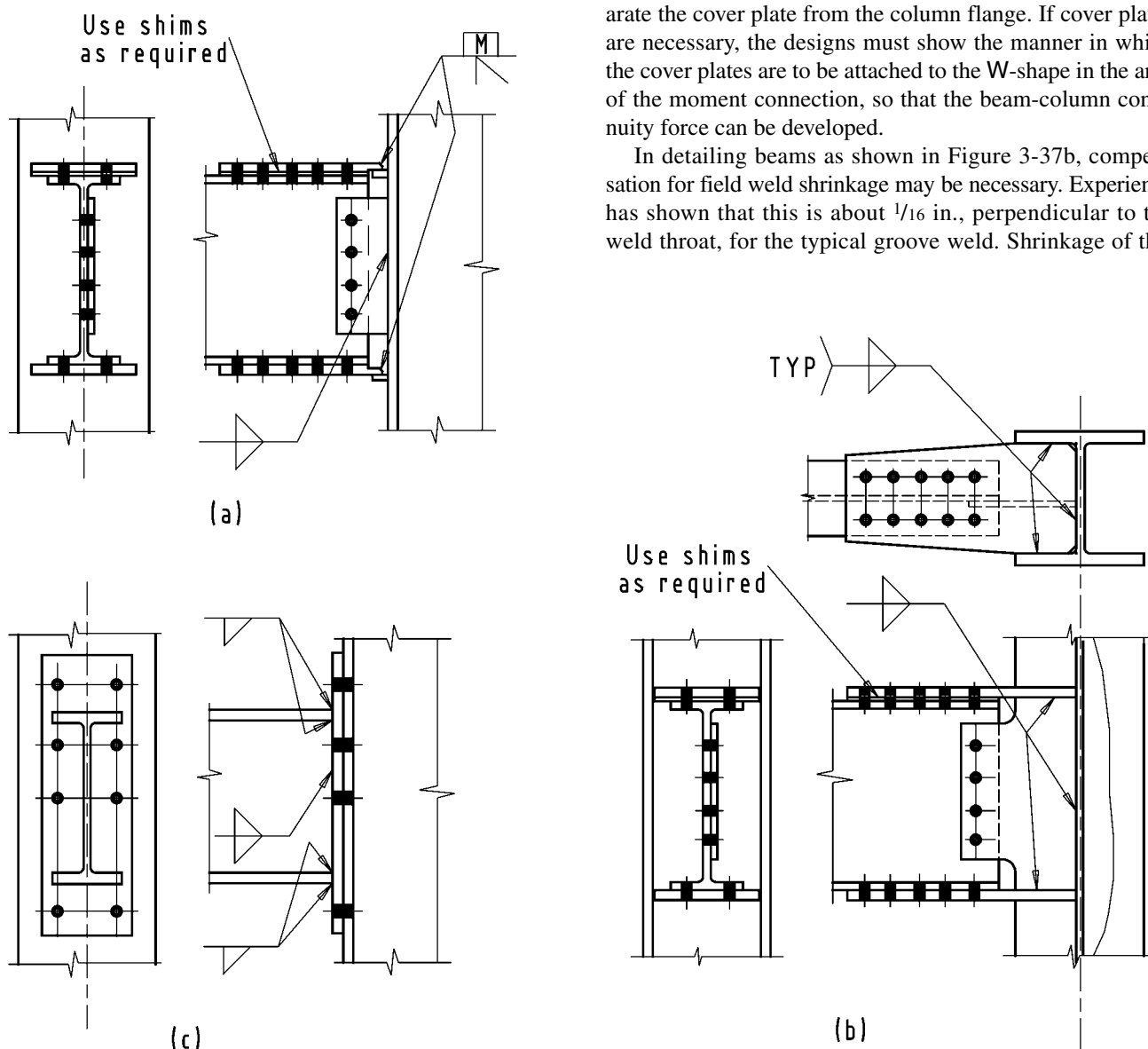
Figure 3-36. Shop-welded, field-bolted moment connections.
