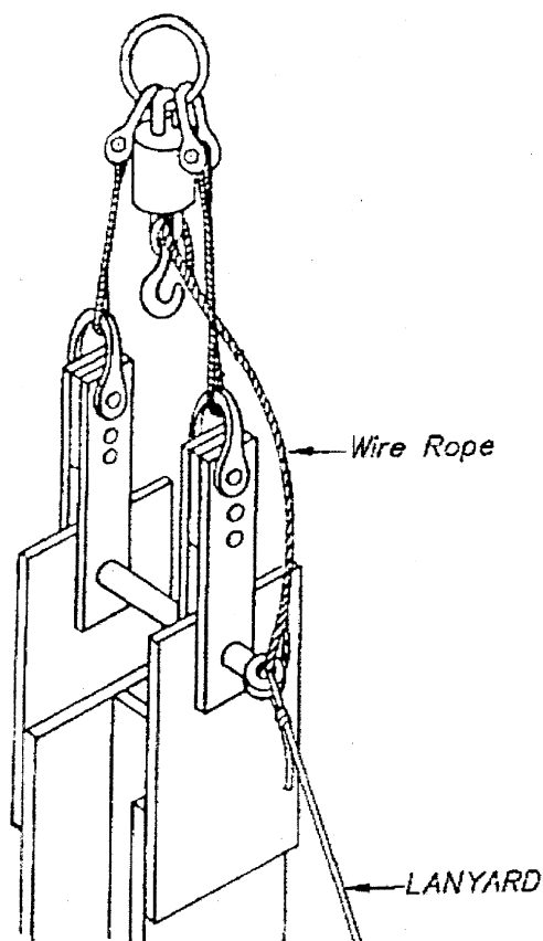
Figure 6-12. Lifting hook and lanyard.
