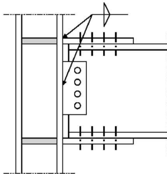
c) Fully restrained (FR) flange plate moment-resisting connection
