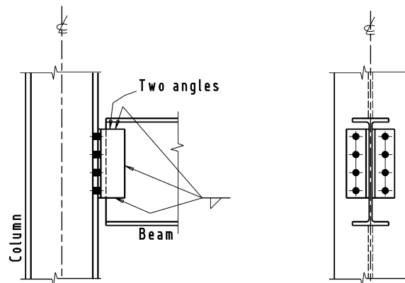
Figure 3-33b. Shop-bolted or shop-welded connection angles to the beam web.
