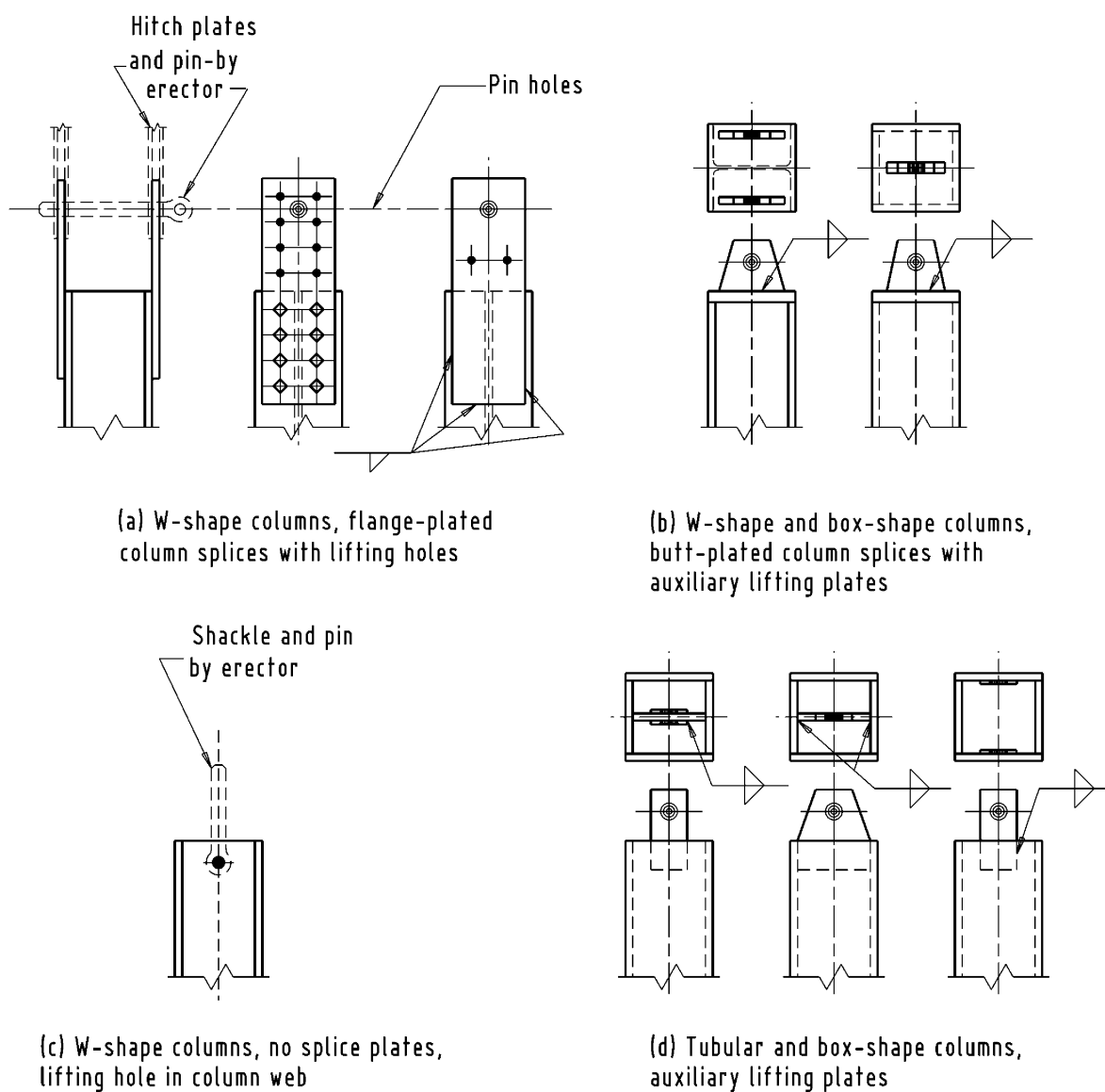
Figure 6-11. Column lifting devices.
