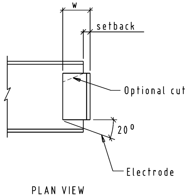
Figure 7-83. Welding clearance.
