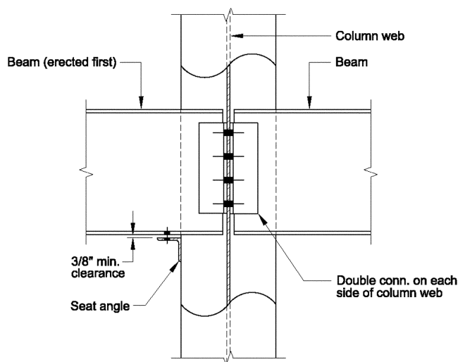
Figure 2-16. Double connection with shop-welded erection seat.
