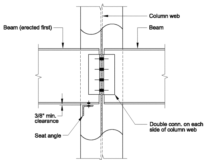
Figure 2-17. Double connection with shop-welded erection seat (alternative location).
