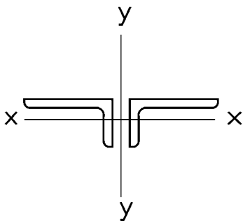
Figure 3-44. Double angles, long legs outstanding.
