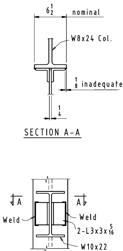
Figure 7-85. Improper connection detail.
