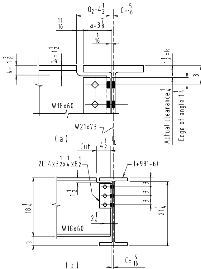
Figure 7-32. Cope, block or cut.
