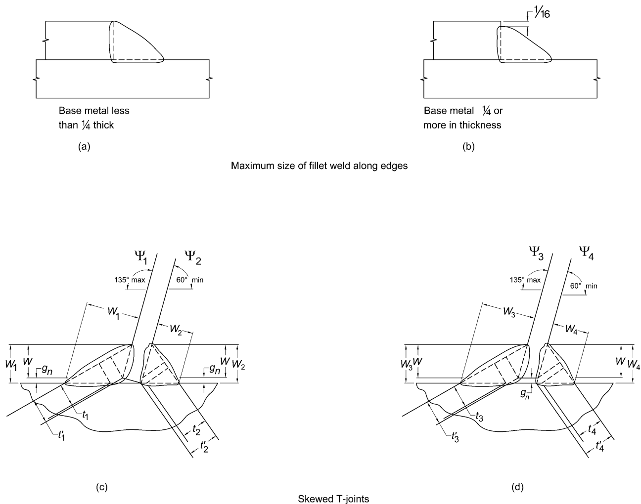
Figure 4-12. Limitations of angle and edge preparations for prequalified skewed tee-joint fillet weld.
