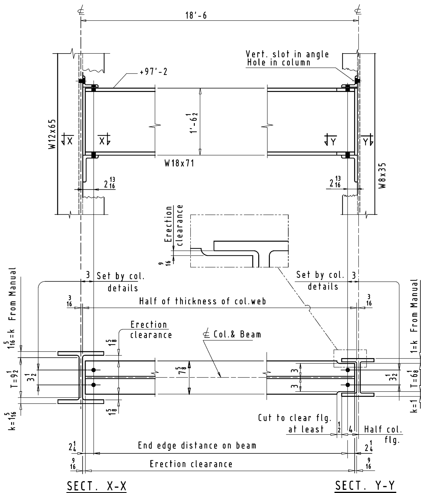
Figure 3 -9. Erection clearances.
