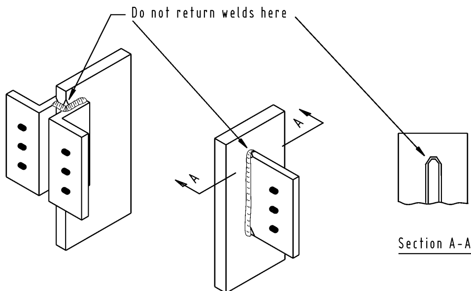
Figure 3-26. Reduction in thickness from wrapping or returning a weld around the end of a material.
