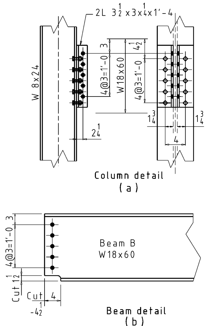
Figure 7-37. A pair of connection angles (or framing angles) shop bolted to the column flange.
