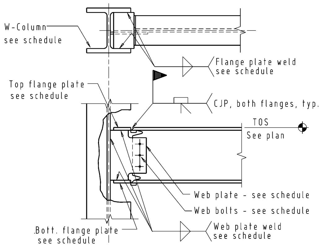
(b) Column web support, welded flanges
