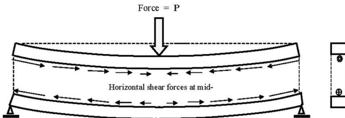
c) Horizontal shear forces ( maximum at mid-depth )
