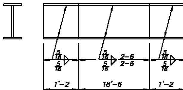
Figure 4-25. Welded joint.
