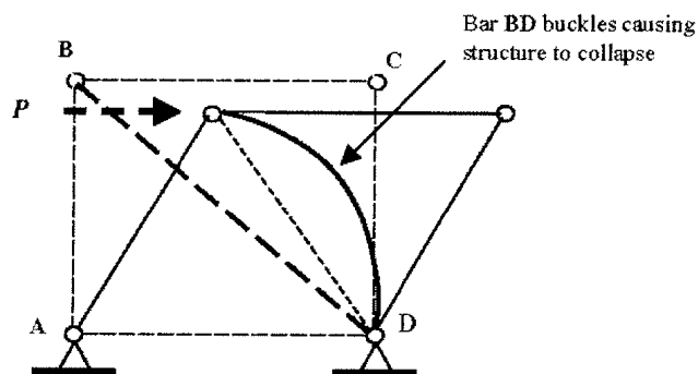
c) Compression member buckling failure
