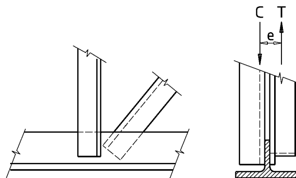
Figure 3-46. Torque on the chord caused by staggered web members.
