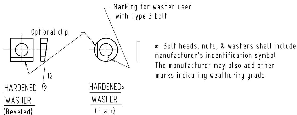
Figure 4-7. Bolt markings.
