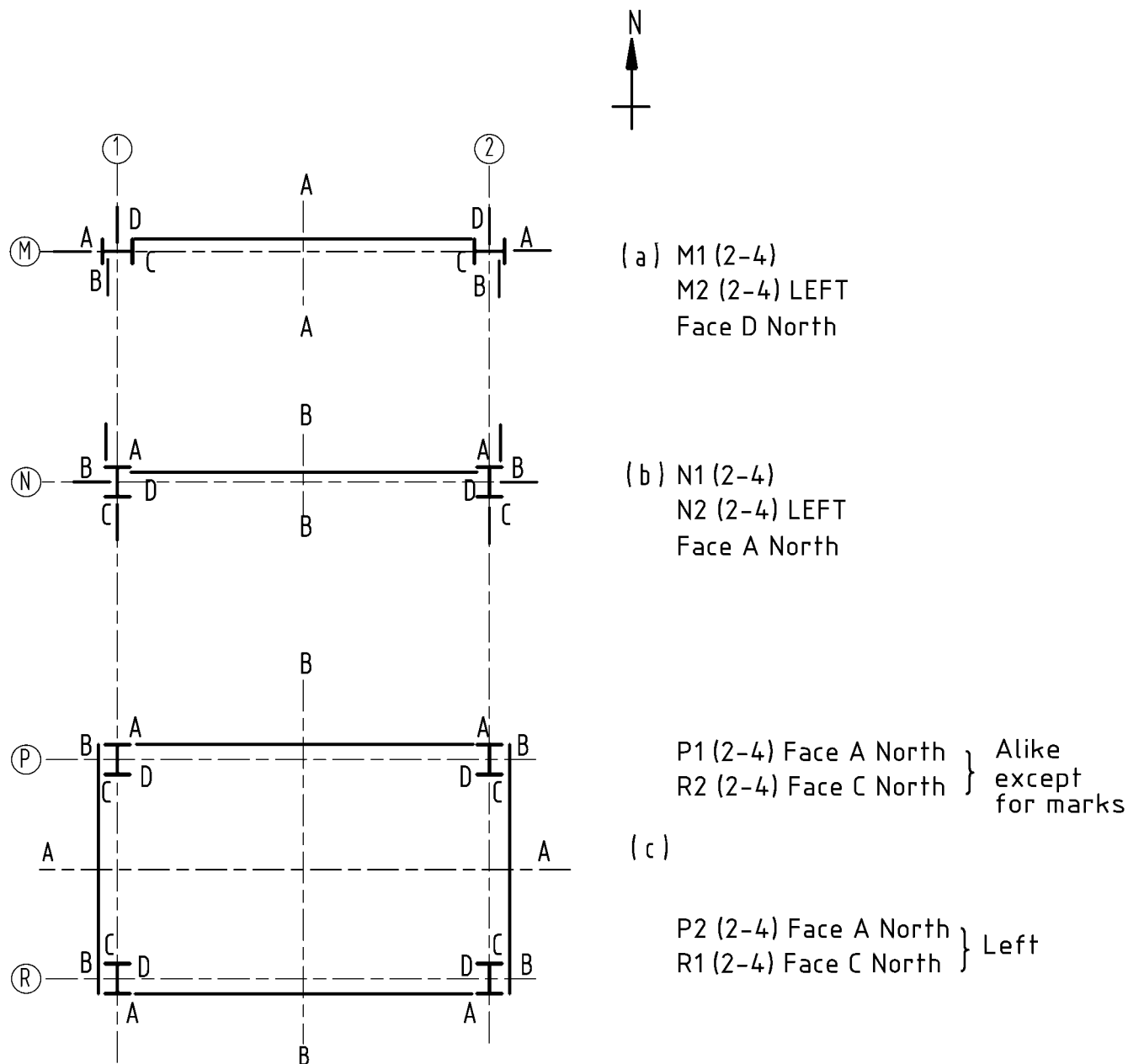
Figure 4-4. Typical framing details.
