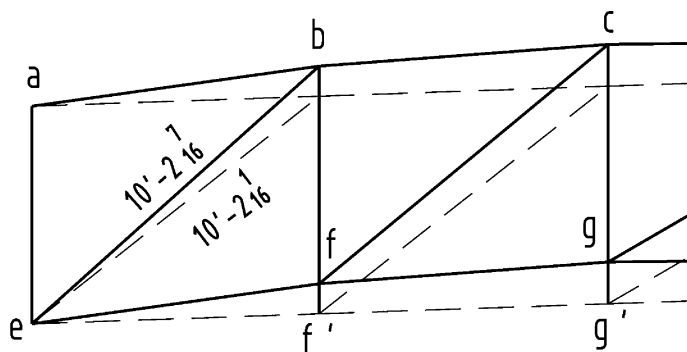
Figure 7-53. Truss camber.
