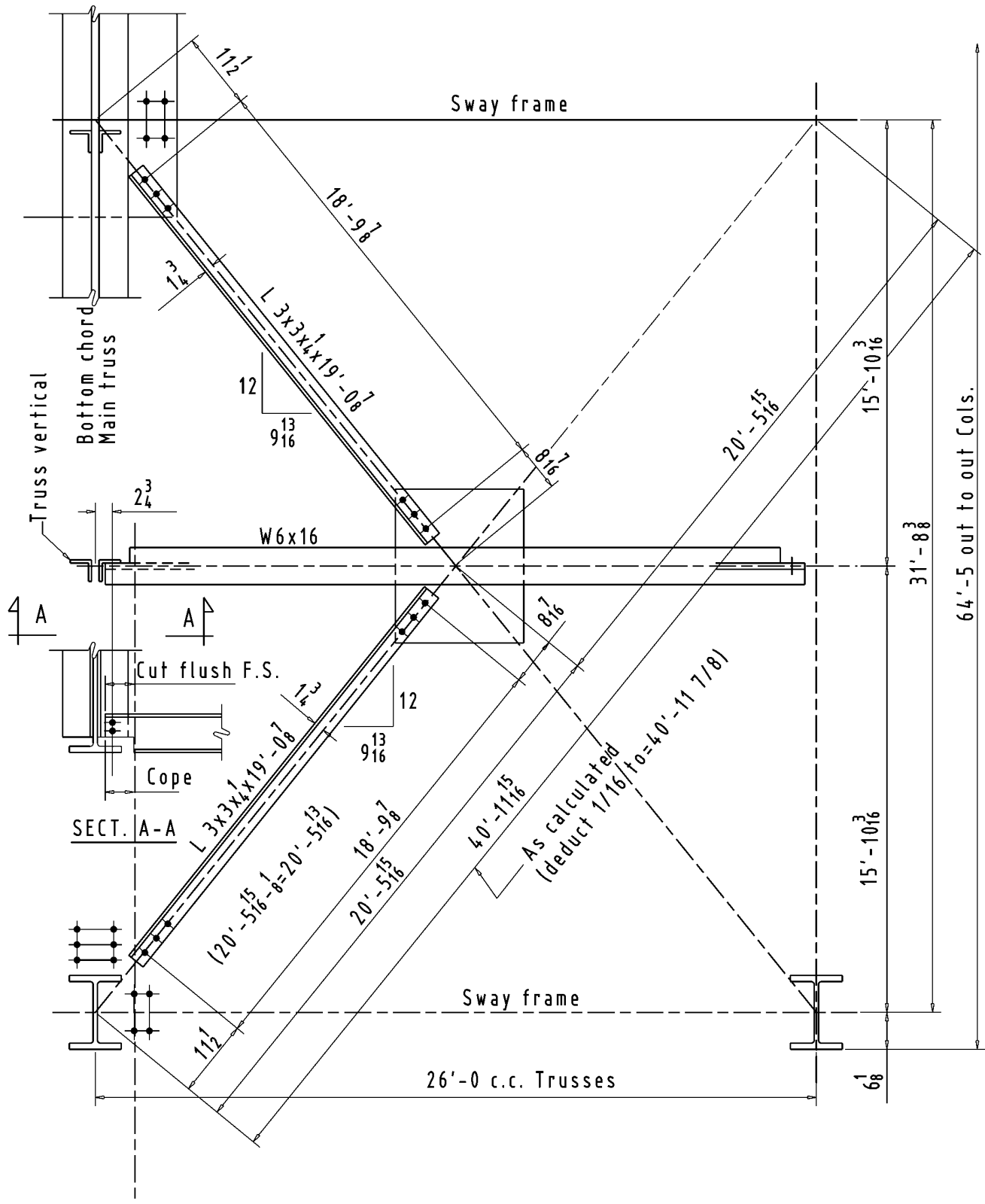
Figure 7-56. Diagram showing the relationship of all parts of the bottom lateral bracing system.
