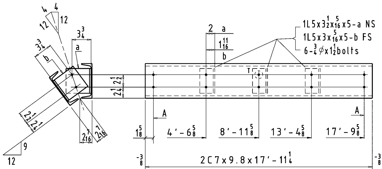
Figure 7-72. Scaled layout.
