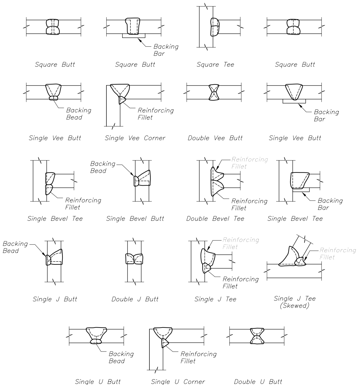
Figure 4-14. Typical complete-joint-penetration groove welds.
