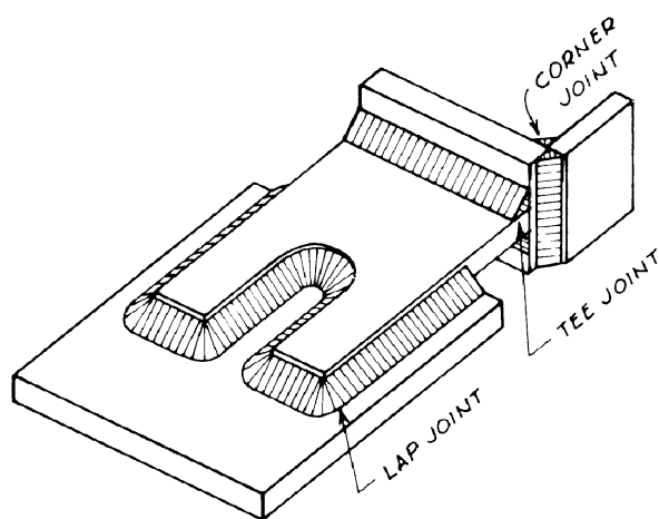
Figure 4-11. Fillet welds.
