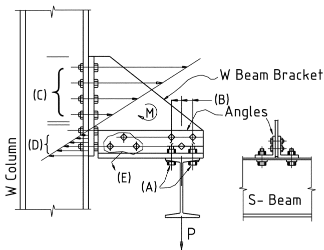
Figure 3-1. Basic functions of fasteners in a connection.
