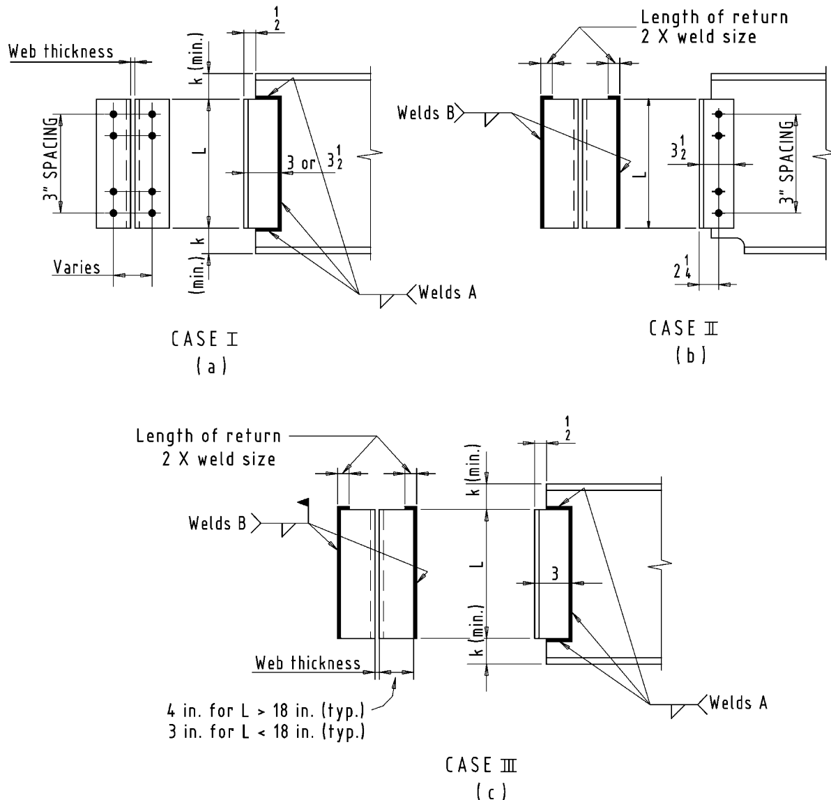
Figure 3-23. Typical welded framed beam connections.
