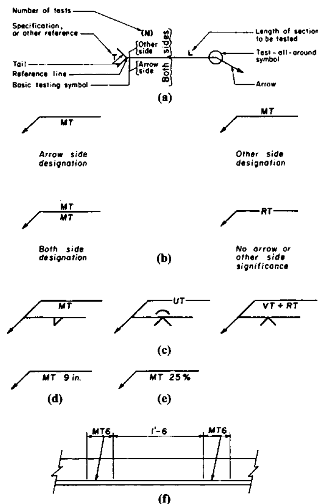
Figure 4-30. Nondestructive testing symbols combined with welding symbols.
