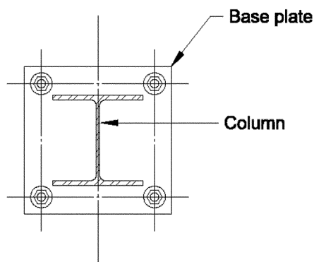
Figure 2-9. Minimum anchor rod requirement.
