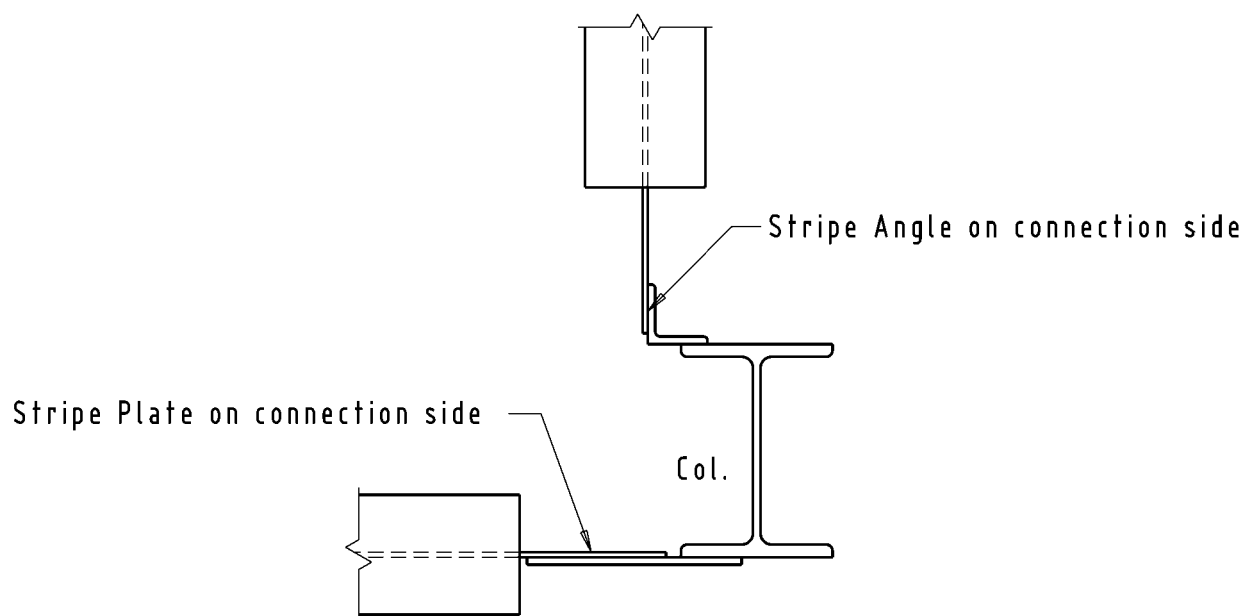
Figure 6-15. Striping or spotting.
