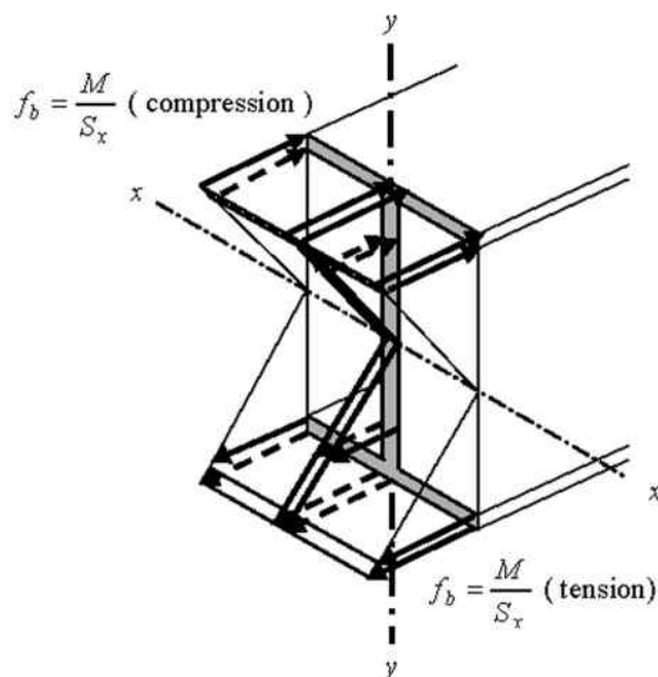
Figure B-16. Bending (flexural) stress distribution in a W-shape steel beam.
