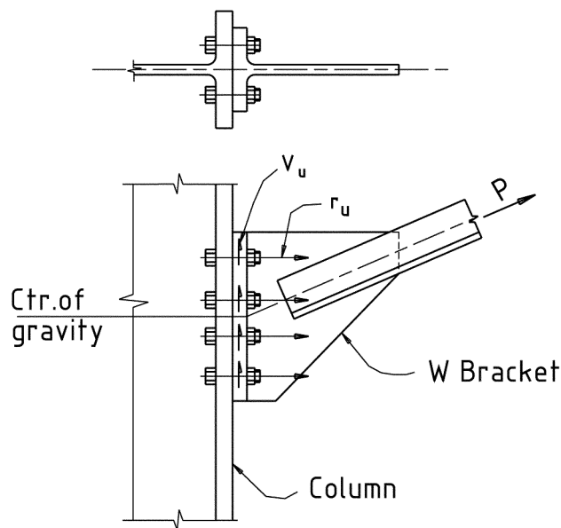
Figure 3-5. Typical end connection of a diagonal bracing member.
