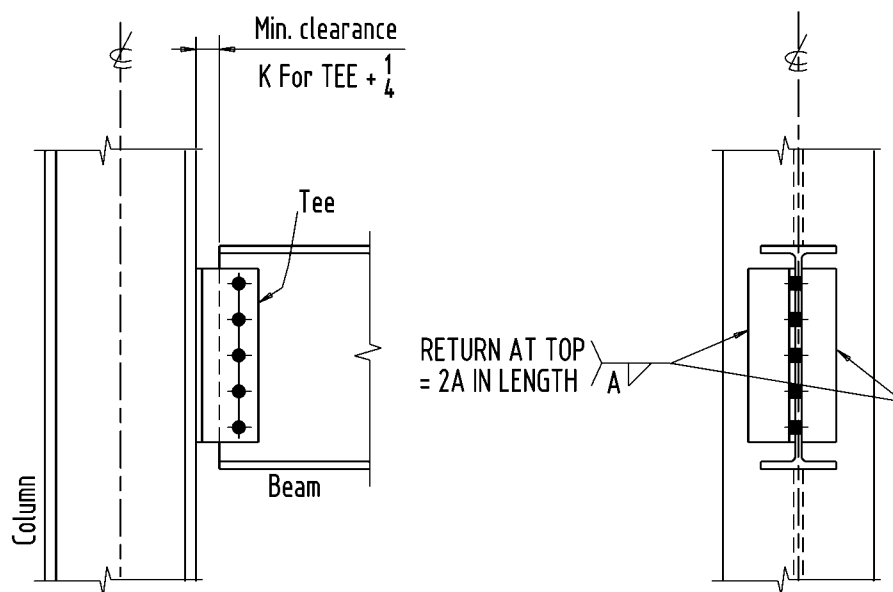
Figure 3-15. Tee connection.
