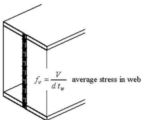
Figure B-15. Shear stress distribution in a W-shape steel beam.
