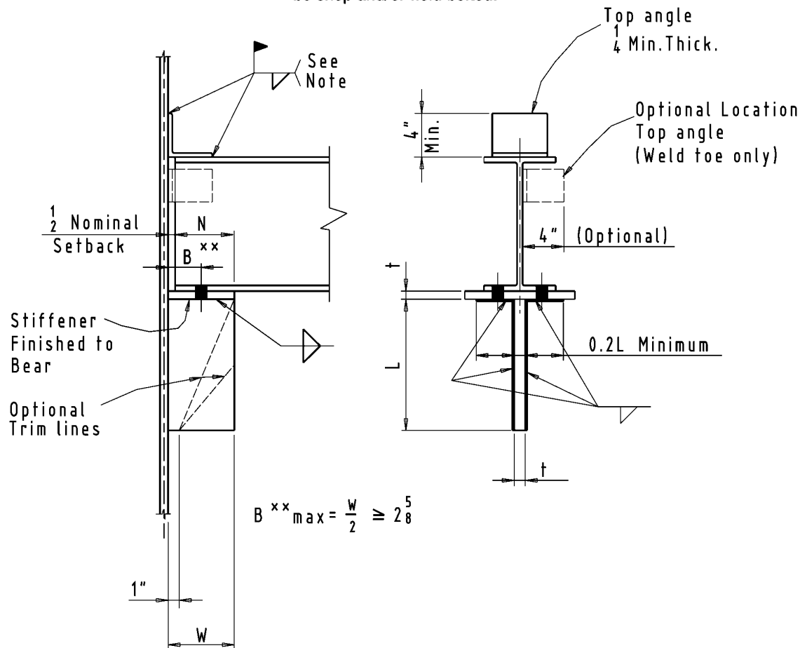
Figure 3-27. Stiffened seated connection.
