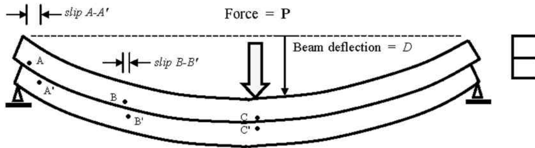
a) Effect of horizontal slip at mid-depth
