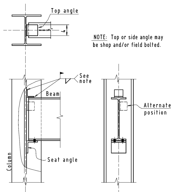
Figure 3-24. Unstiffened seated connection.
