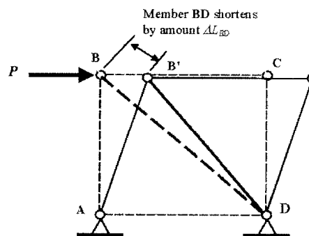
a) Structure ABCD loaded with force P at joint B.
