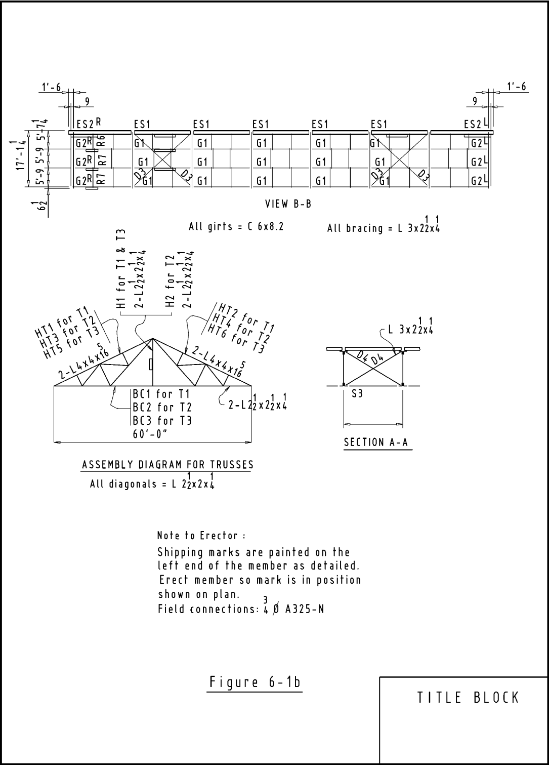
Figure 6-1b. Erection drawing.
