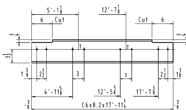
Figure 7-78. Detailed layout for the connection of a girt to a column flange.
