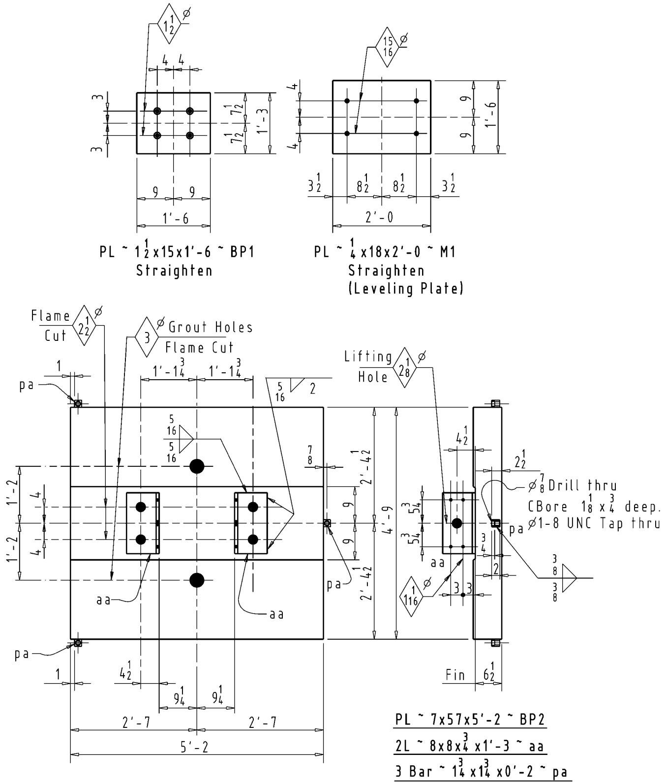
Figure 7-4. Base plate details.
