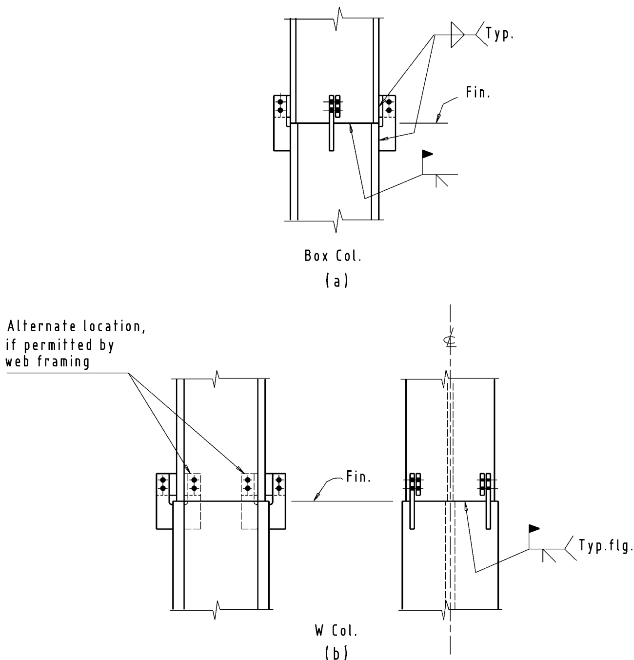
Figure 3-40. Column splices.
