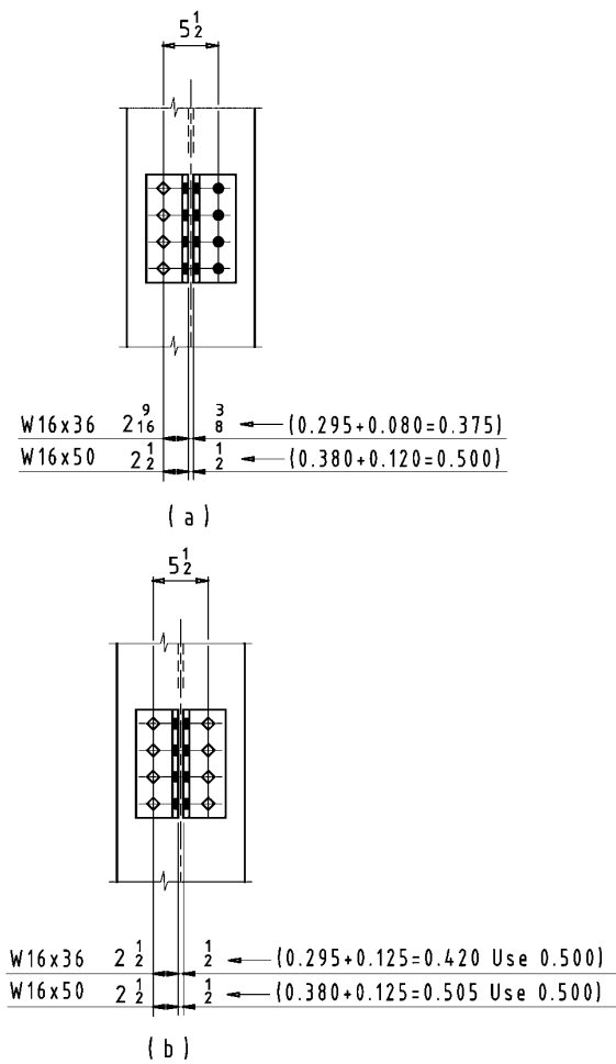
Figure 3-32. Beam web connections placed on column flanges.
