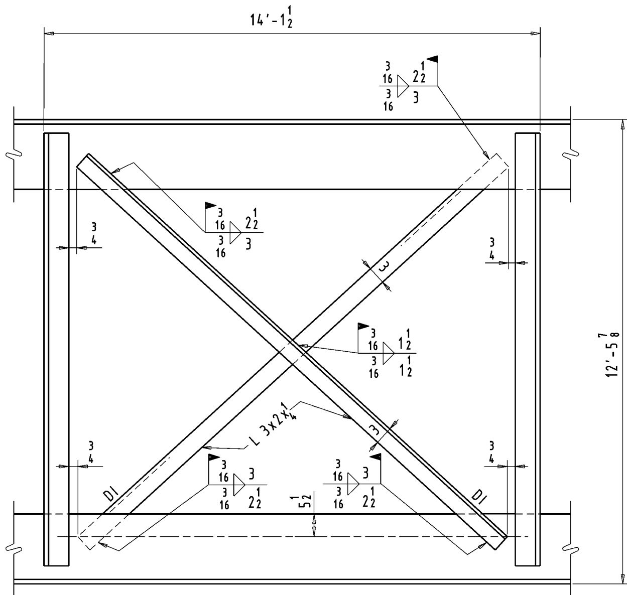
Figure 7-65. Field assembly diagram for a bracing panel.
