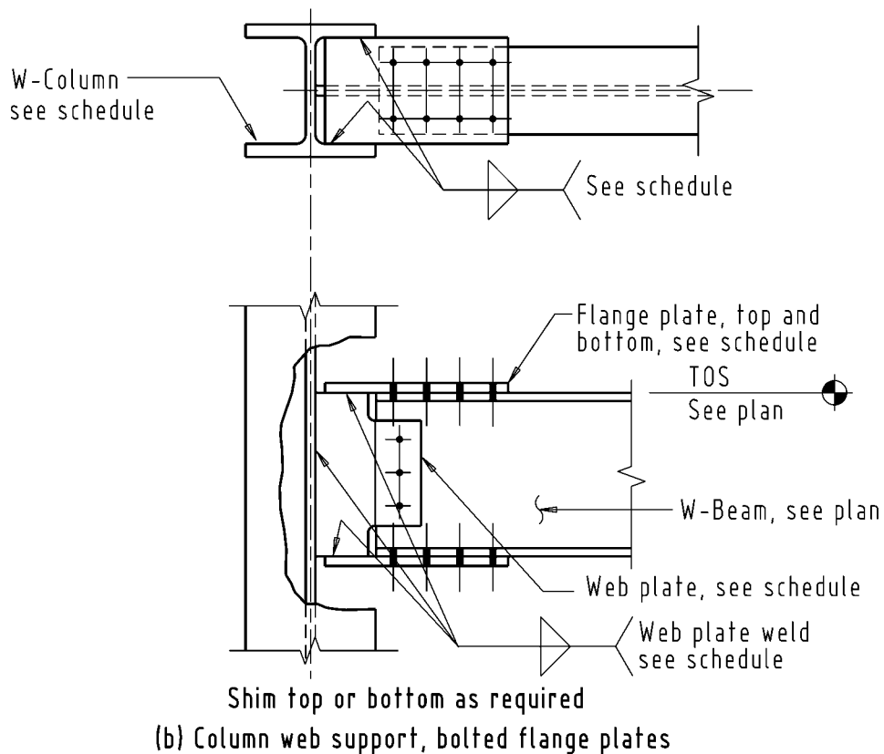
Figure 7-1d. Structural design drawing—bolted moment connection detail.
