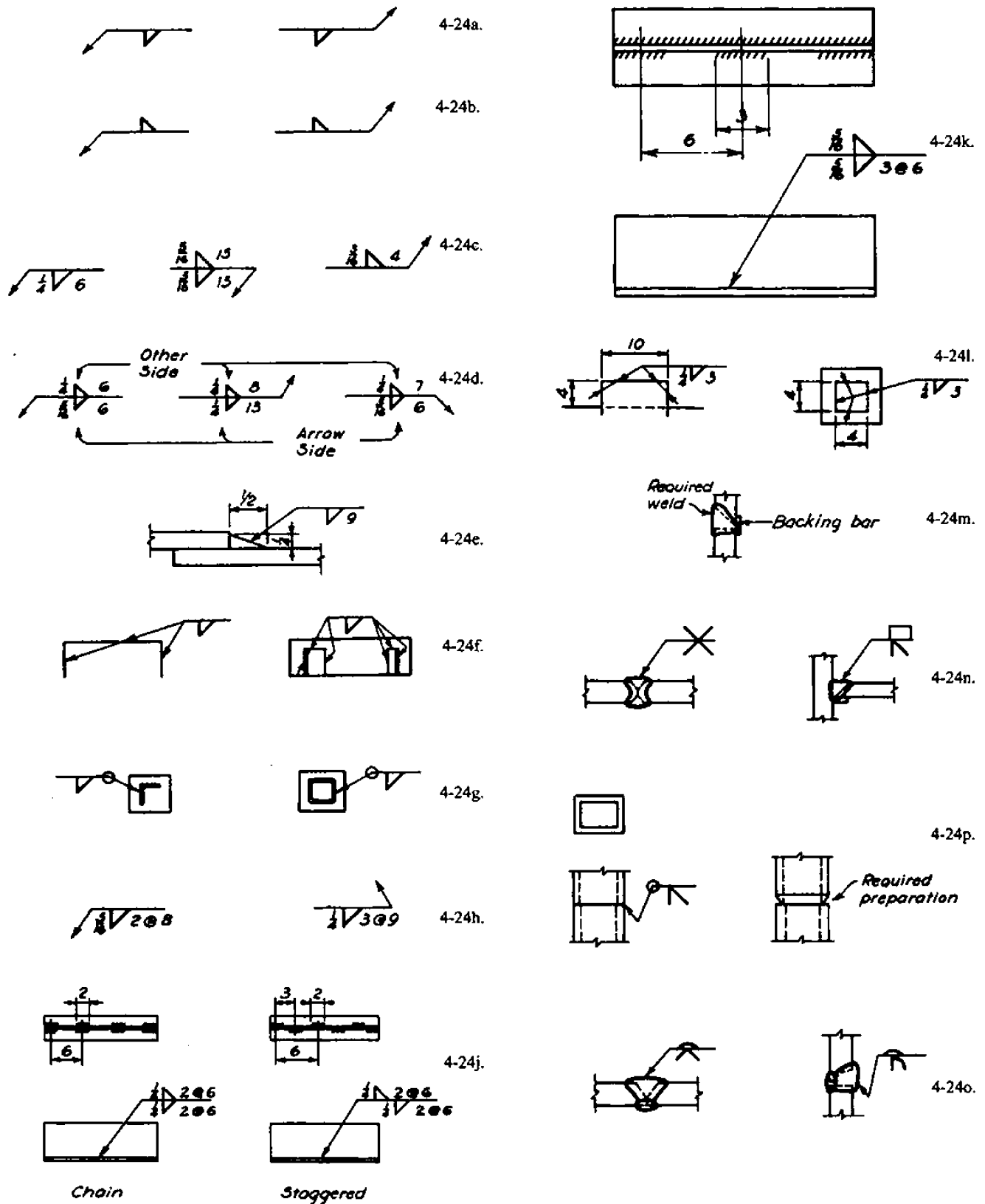
Figure 4-24. Miscellaneous weld symbols and details.
