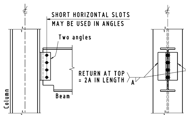
Figure 3-33a. Knife connection.
