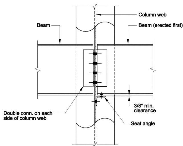
Figure 2-15. Double connection with temporary bolted erection seat.
