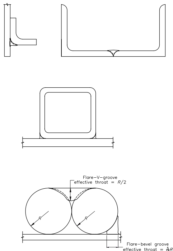
Figure 4-15. Several types of flare welded joints.
