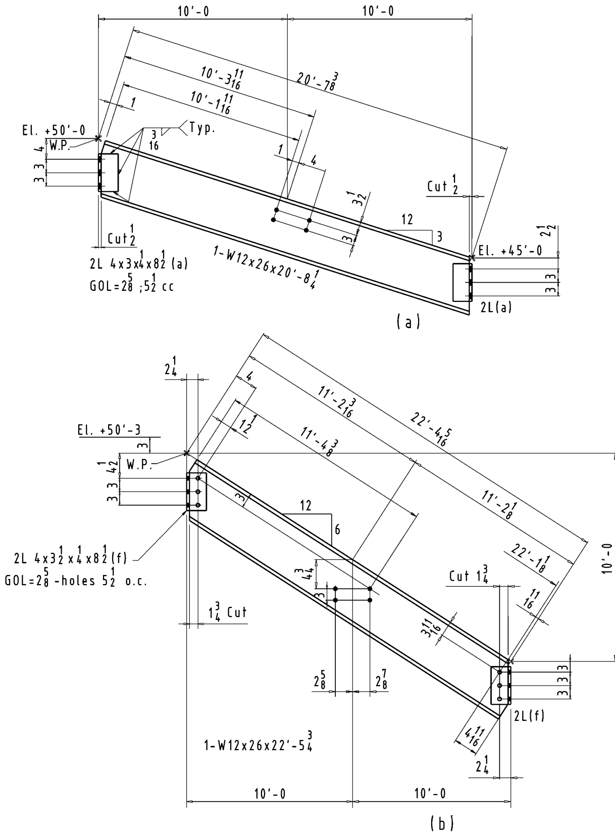
Figure 7-36. Beams cut on a vertical bevel.
