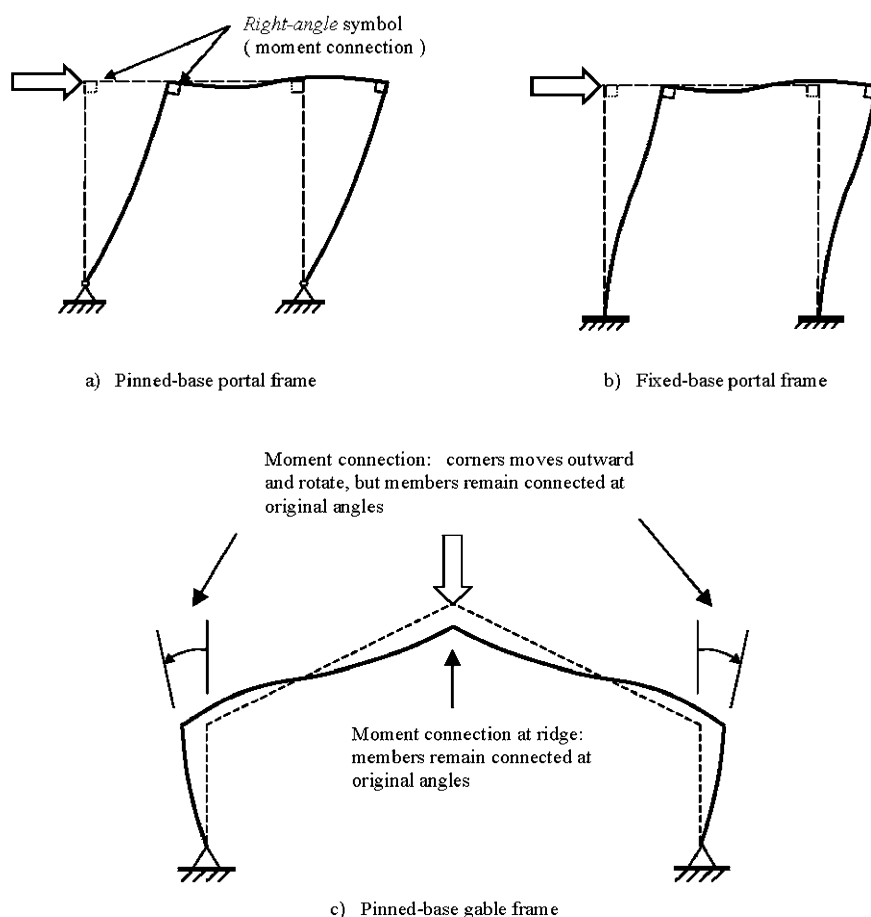
Figure B-6. Rigid frames.
