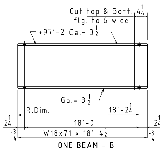
Figure 7-39. “Short cut” shop detail.
