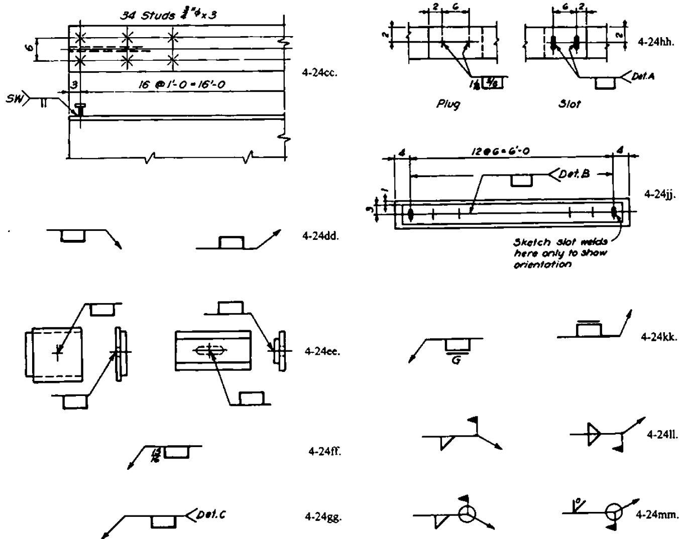
Figure 4-24 (continued). Miscellaneous weld symbols and details.
