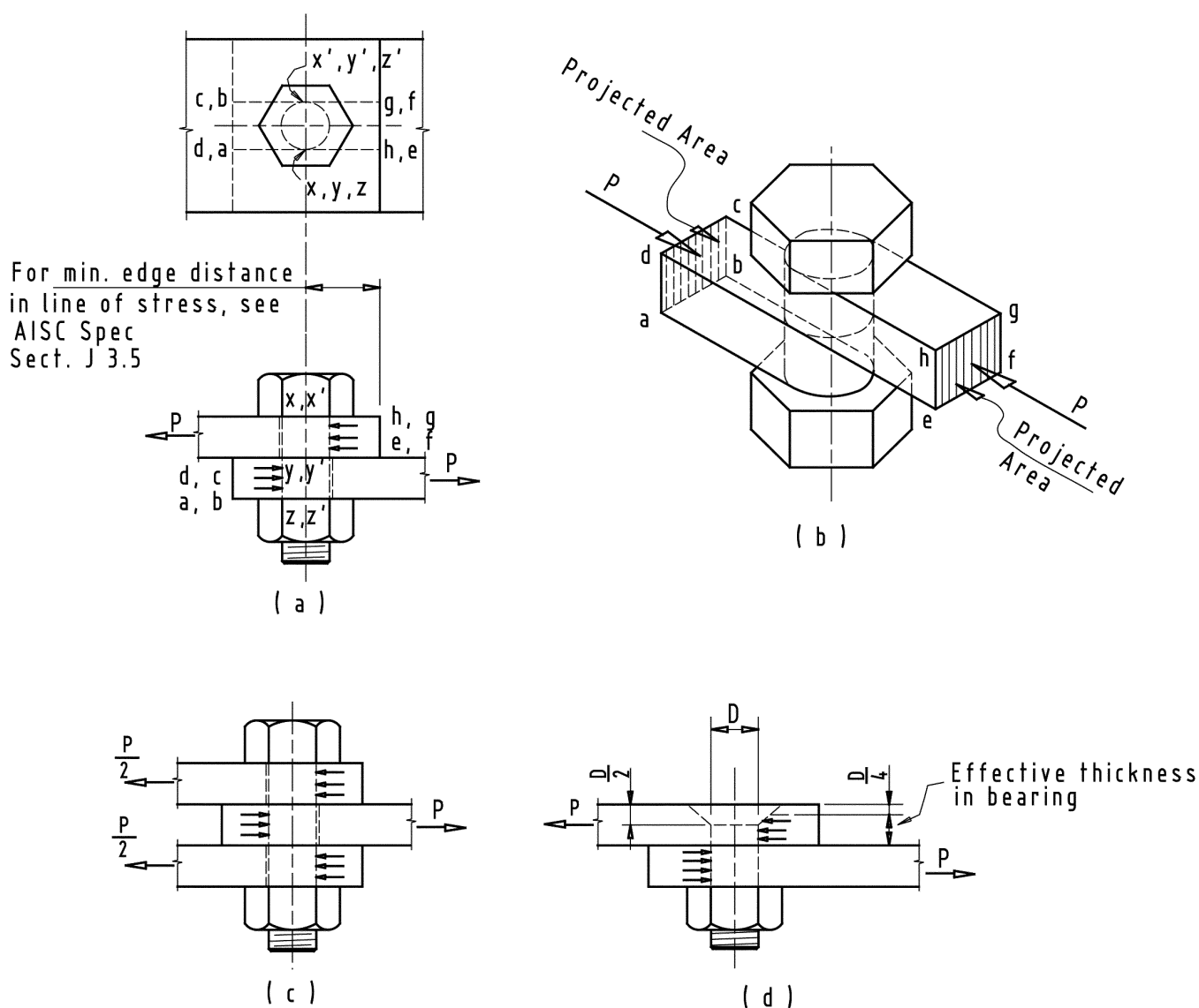
Figure 3-4. Bolt bearing.
