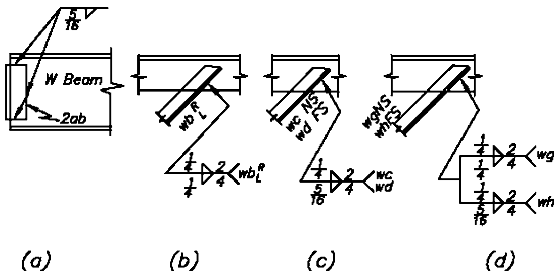
Figure 4-26. Welded joint combinations.
