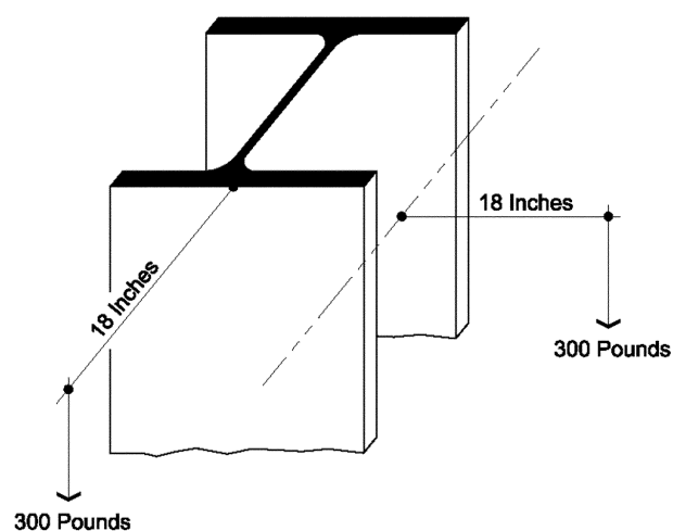
Figure 2-10. Loads required at column tops for erection.
