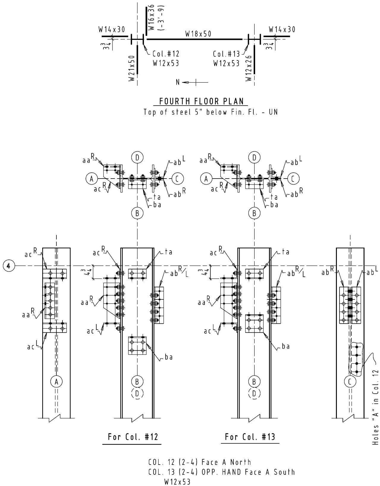
Figure 4-5. Partial details: the opposite-hand relationship of columns.
