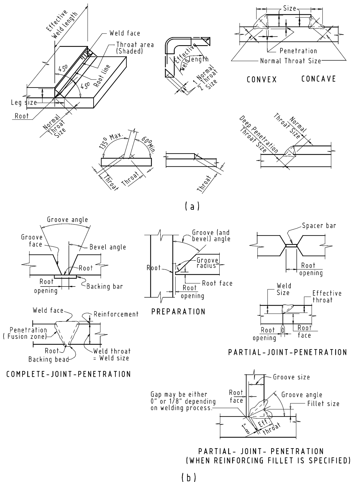
Figure 3-16. Common fillet and groove weld nomenclature.
