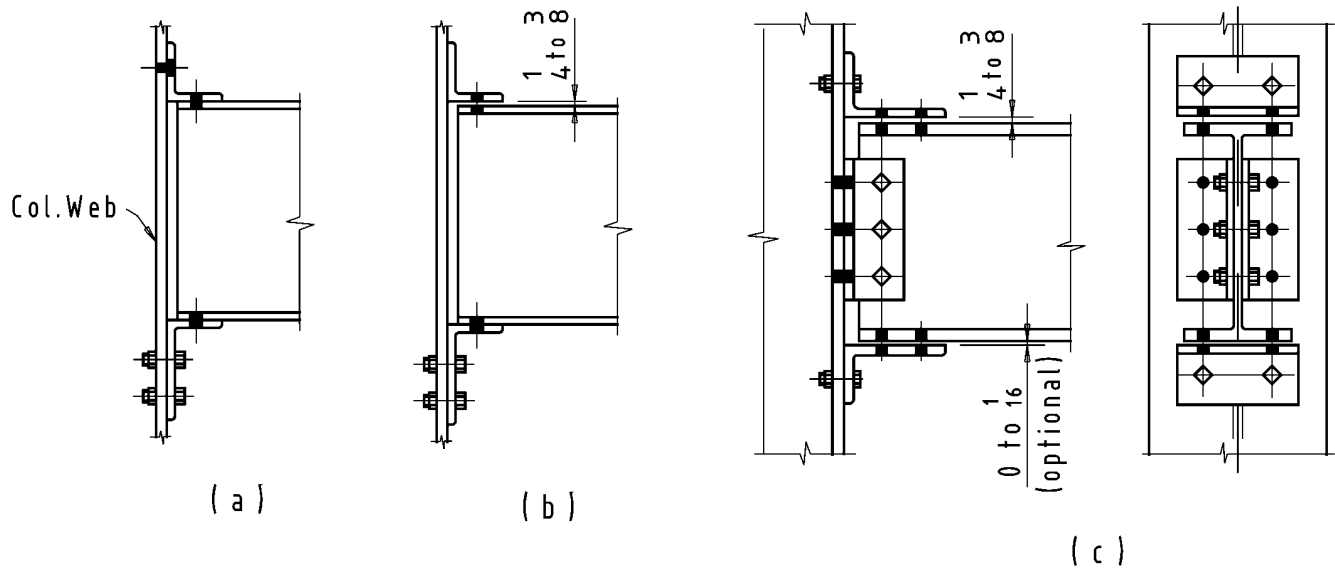
Figure 3-31. Typical seated connections and the clearances provided.
