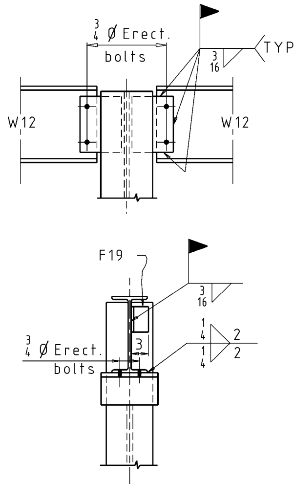
Figure 7-22. Part plan taken from a design plan and connection details.
