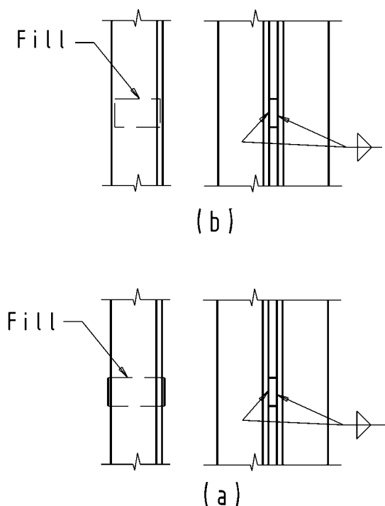
Figure 7-54. Fills.
