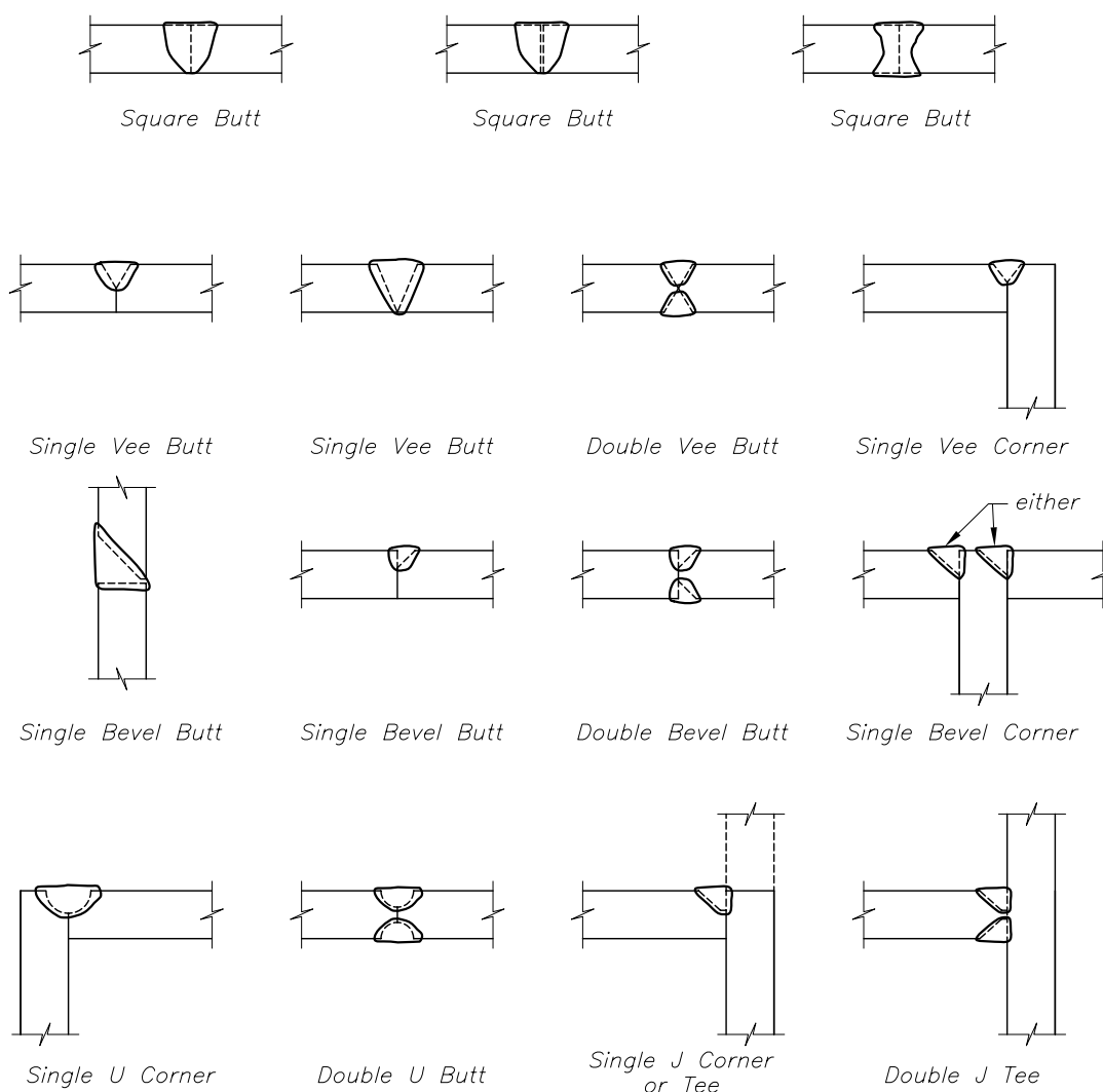
Figure 4-13. Typical partial-joint-penetration groove welds.
