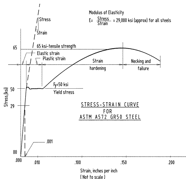
Figure 1-2. Stress-strain diagram for ASTM A572 Grade 50 steel.
