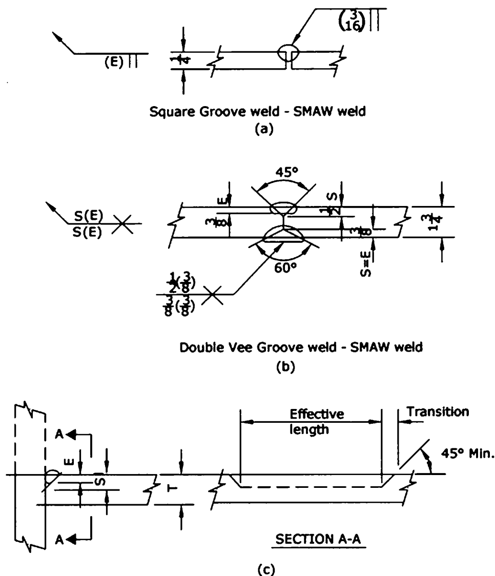
Figure 4-29. Groove welds.
