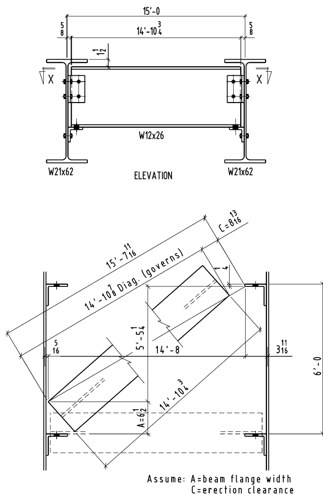
Figure 7-86. Clearance available for erecting seated filler beams where the side-angle connections are to be shop fastened to the supporting girder beams.
