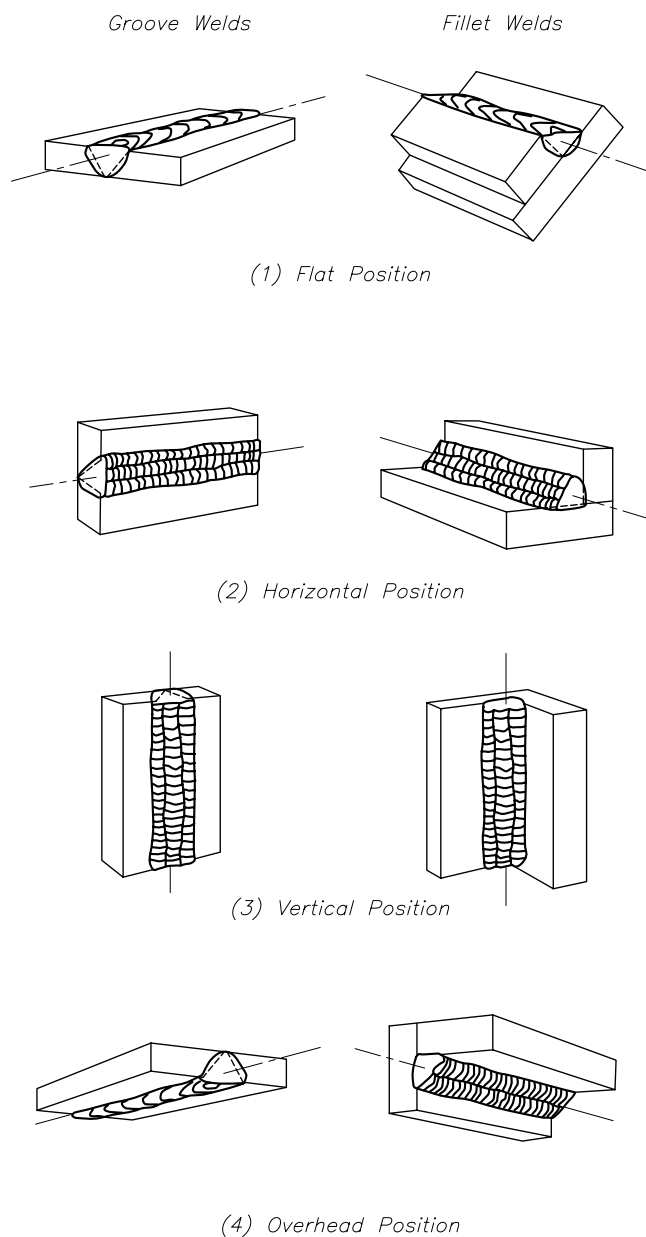
Figure 4-18. Basic weld positions.
