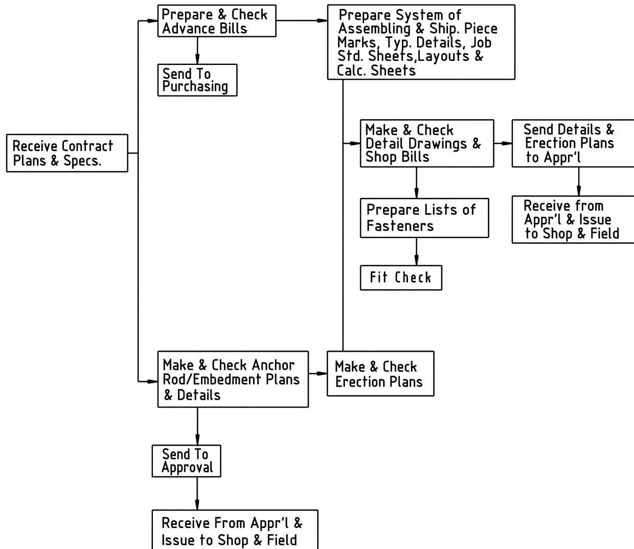
Figure 2-4. Detailing process sequence of operations diagram.
