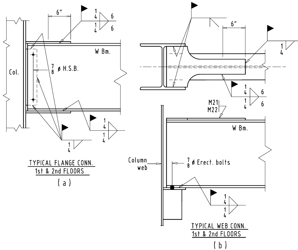
Figure 6-4. Field-welded moment connection.
