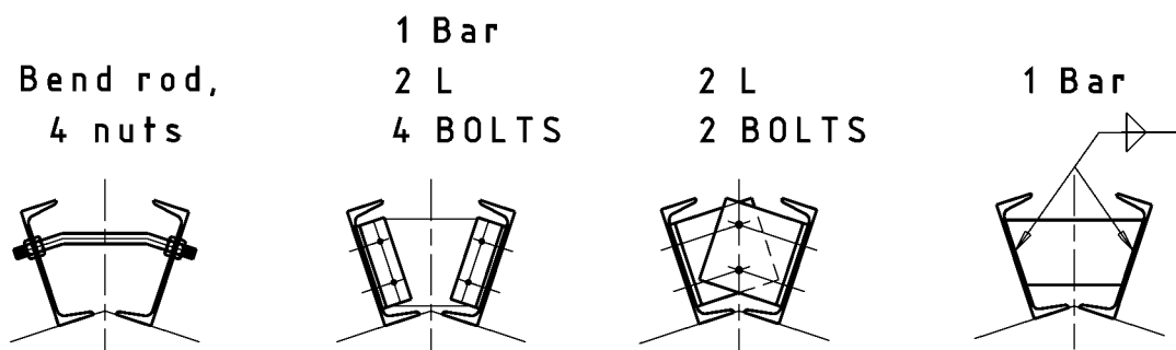
Figure 7-71. Roof ridge connections.
