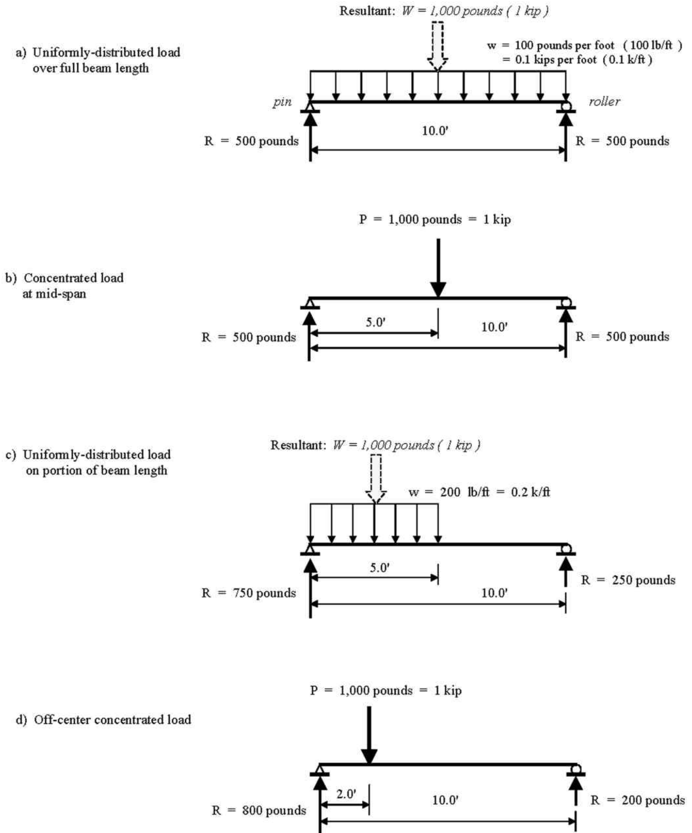
Figure B-7. The effect of load placement on beam reactions.
