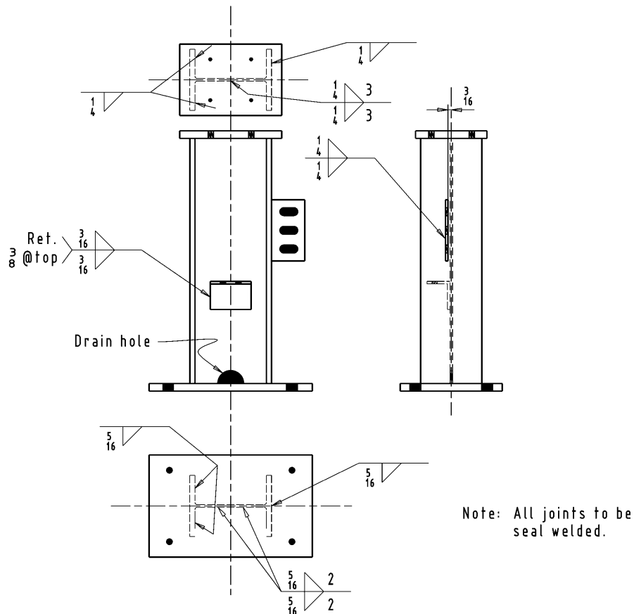
Figure 4-35. Weld access holes.
