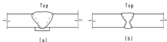
Figure 4-19. Vee and double-vee groove weld placement.
