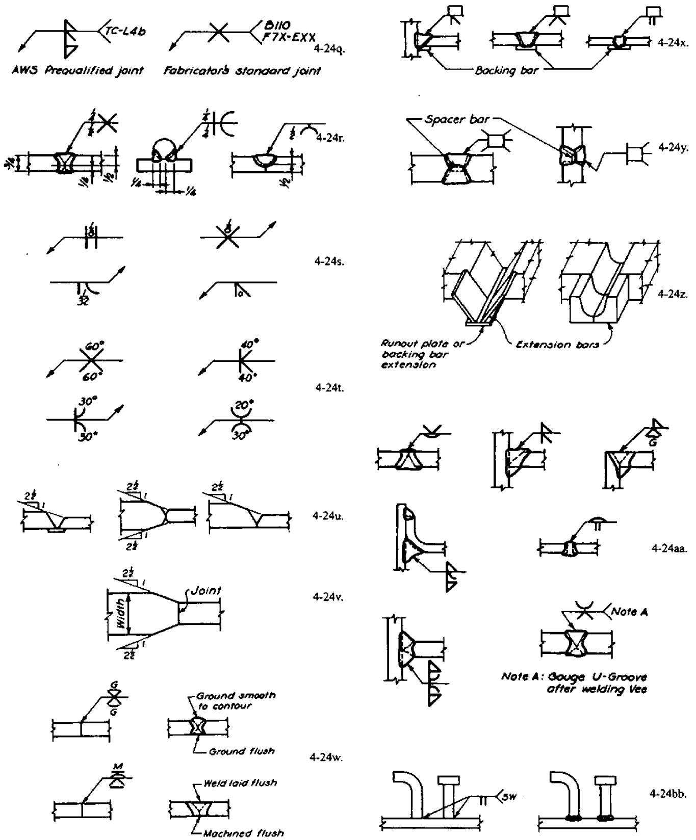
Figure 4-24 (continued). Miscellaneous weld symbols and details.
