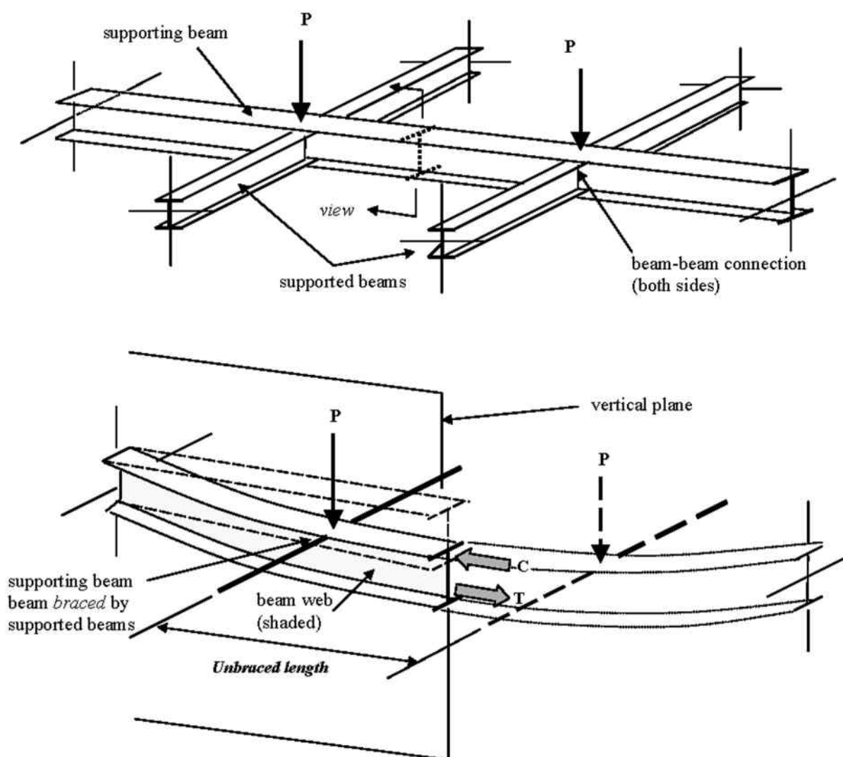
Figure B-20. Beam bracing to prevent out-of-plane buckling (lateral-torsional buckling).
