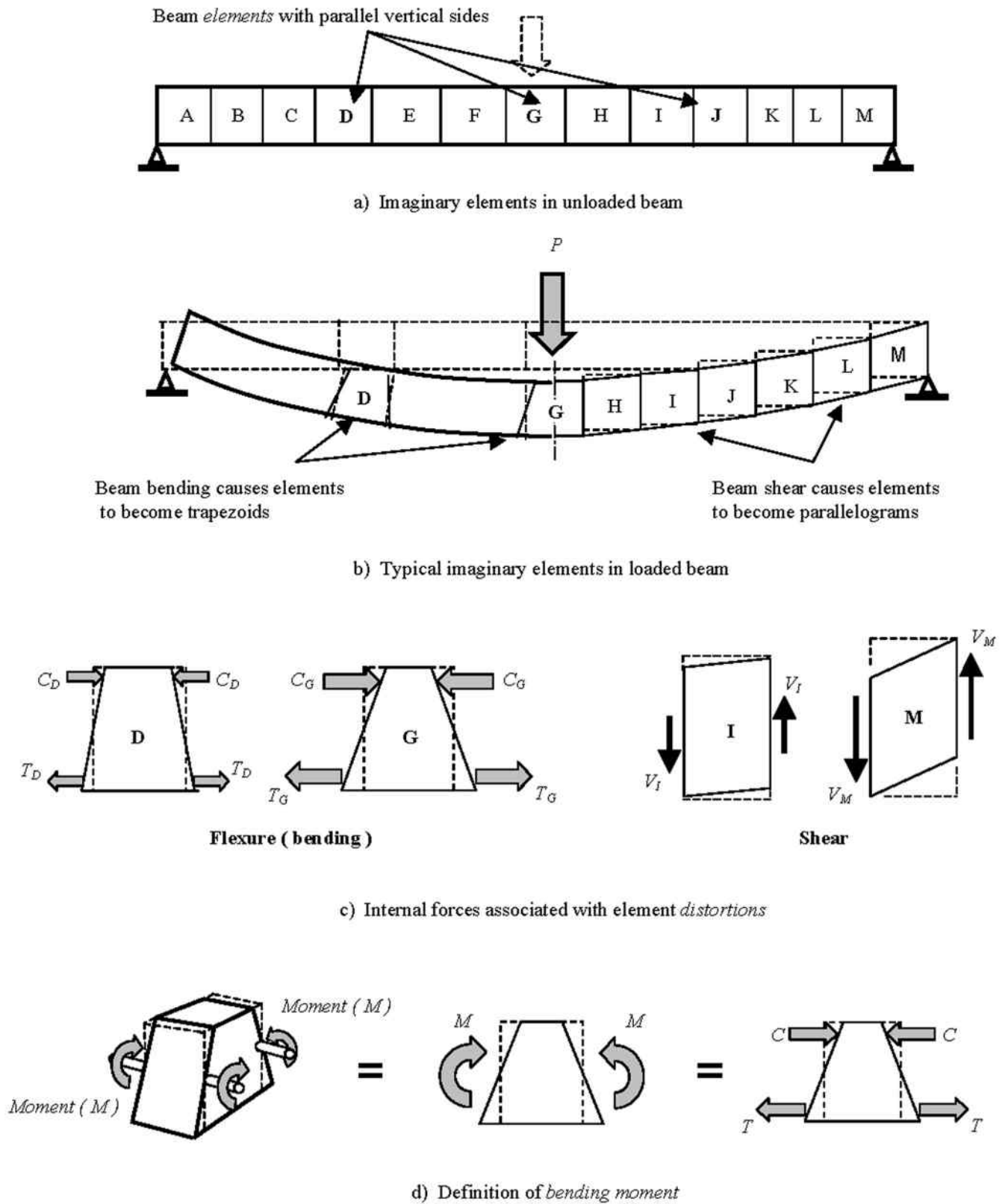
Figure B-10. Moment and vertical shear in beams.
