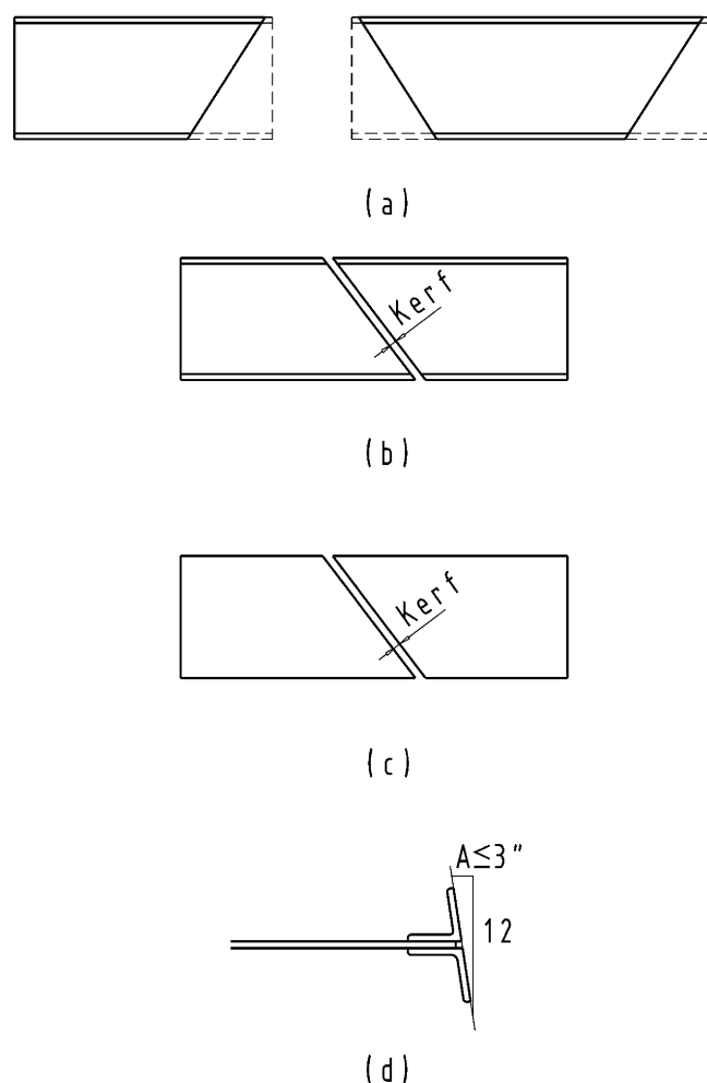
Figure 5-3. Kerf, diagonal and skew.
