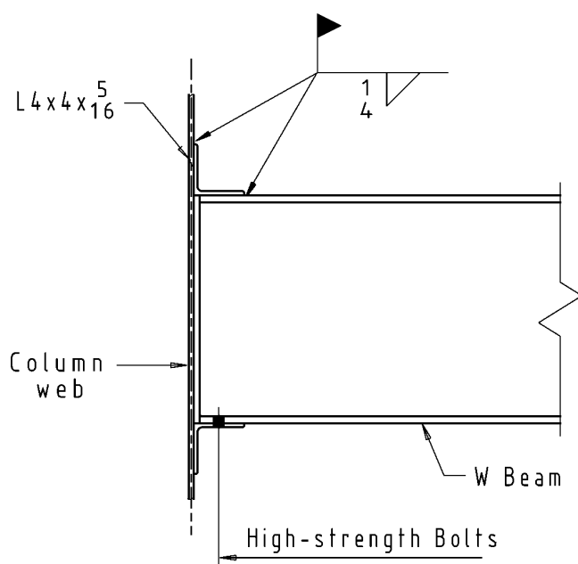
Figure 6-2. Seated connection.
