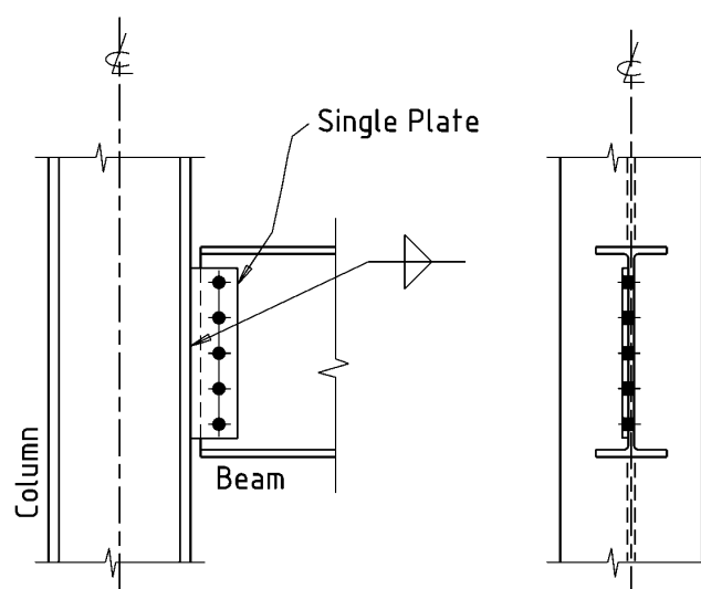
Figure 3-13. Single-plate connection to a column flange.
