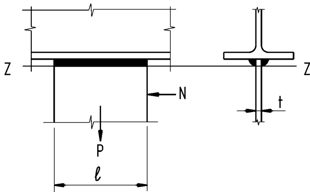
Figure 3-19. Plate loaded in tension.
