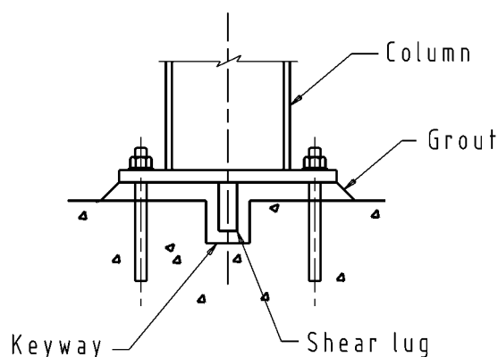
Figure 7-5. Keyway in concrete foundation.
