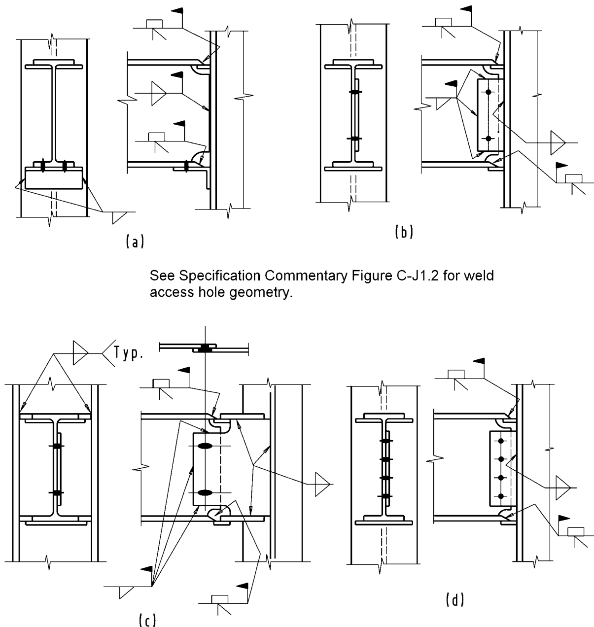
Figure 3-37. All-welded moment connections to column flanges.
