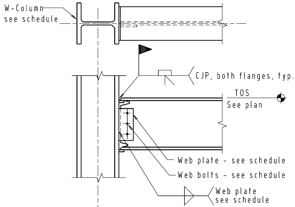
(a) Column flange support, welded flanges
