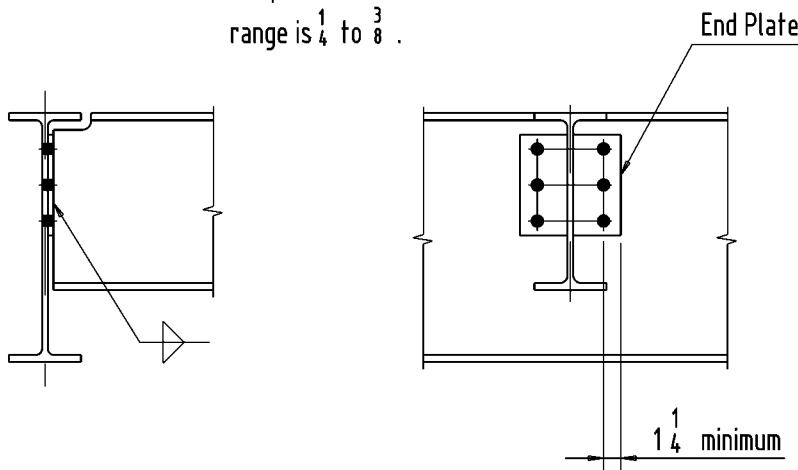
Figure 3-7. Typical end-plate connection to the web of a beam.
