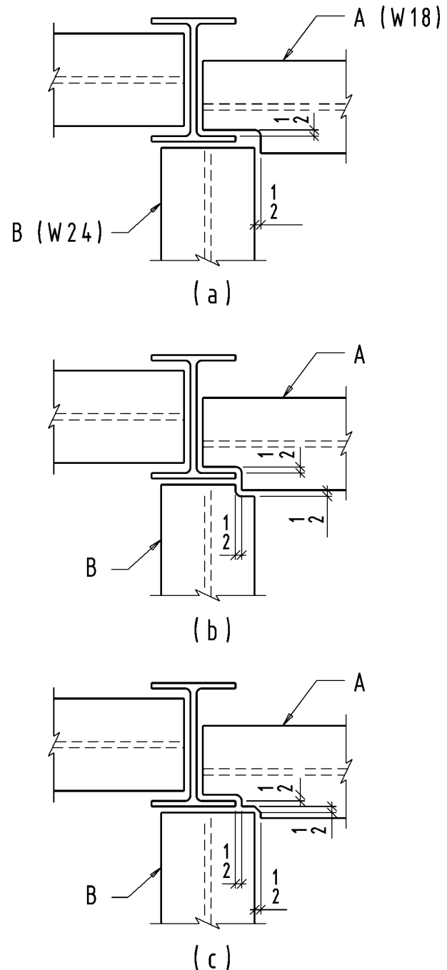
Figure 7-90. Flush-top beams A and B.
