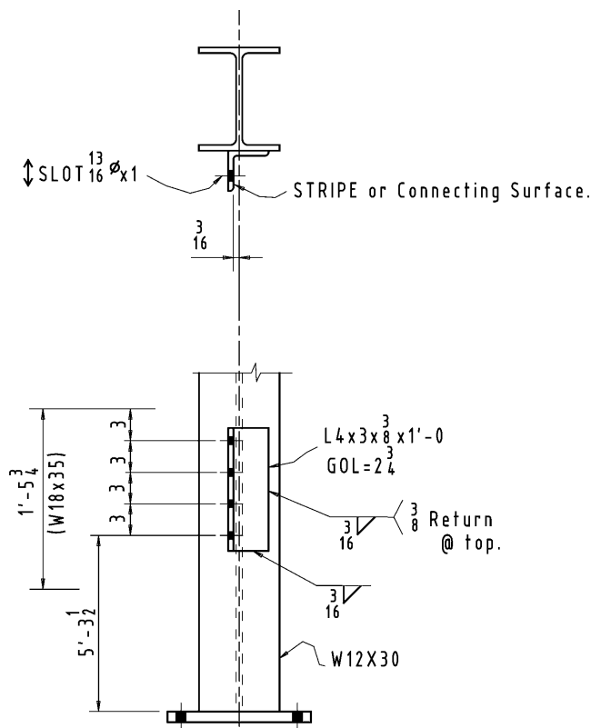
Figure 4-2. Wrap-around connection use.
