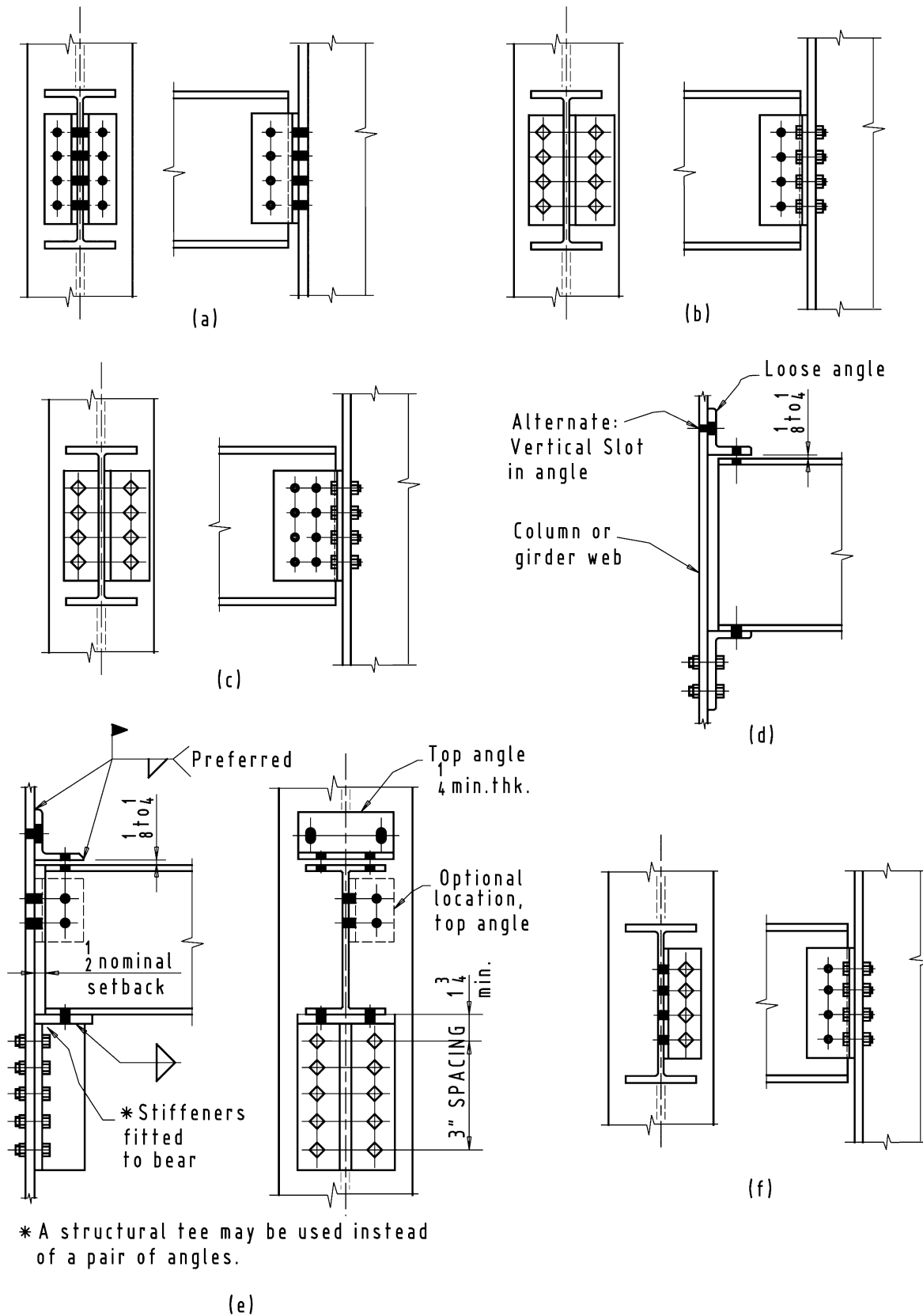
Figure 3-28. Framed and seated connections for shop-bolted construction.
