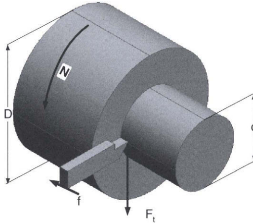
Figure 1.2. The turning process, where a workpiece of initial diameter D is being reduced to d ; F_t is the tangential cutting force, N is the spindle speed, and f the feed rate. In the diagram the depth of the cut is exaggerated.
