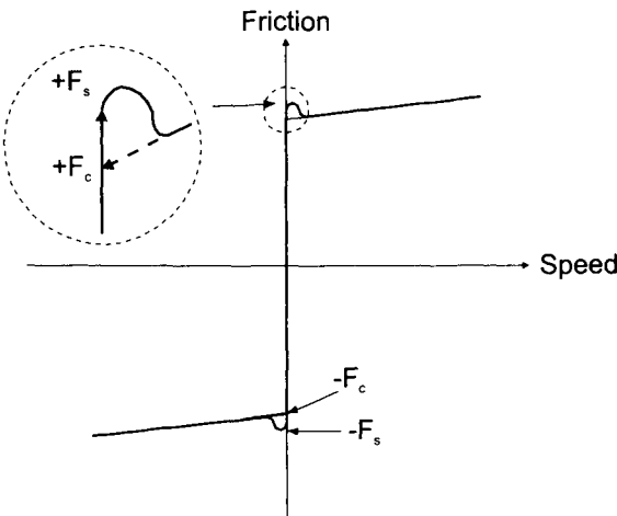
(b) The general kinetic friction model
