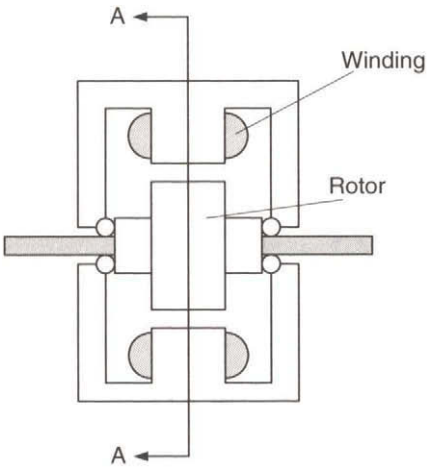
(a) Axial cross section.
