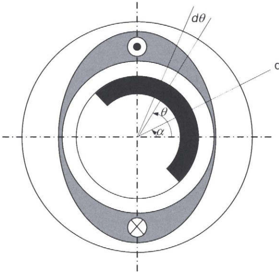
Figure 6.9. Cross section of an ideal sinewave-wound permanent magnet machine.
