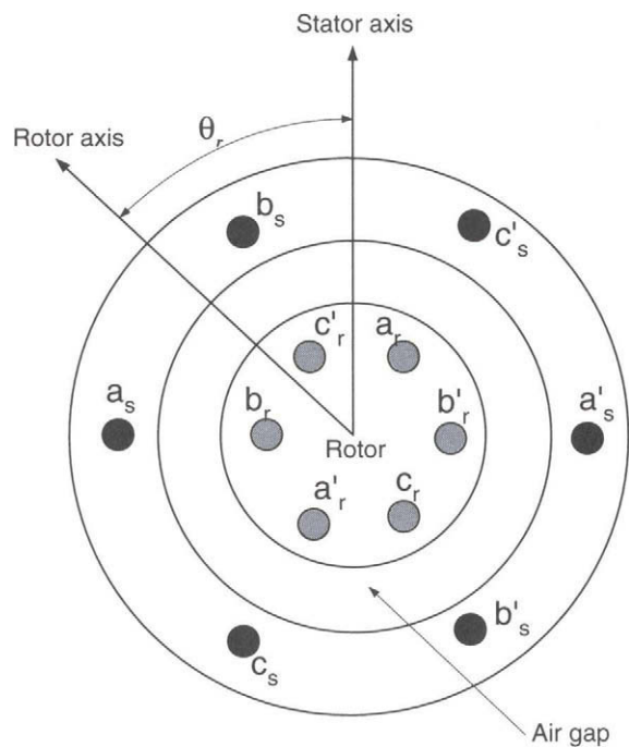
Figure 7.1. Cross section of an idealised three-phase, two-pole induction motor. The rotor and stator windings are represented as concentrated coils. The rotor’s speed is \omega_r , and the lag between the rotor and stator axes is \theta_r .
