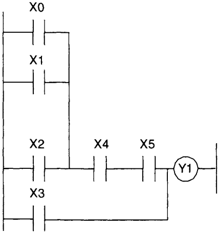
Figure 10.13. Combinational logic extended through nesting.
