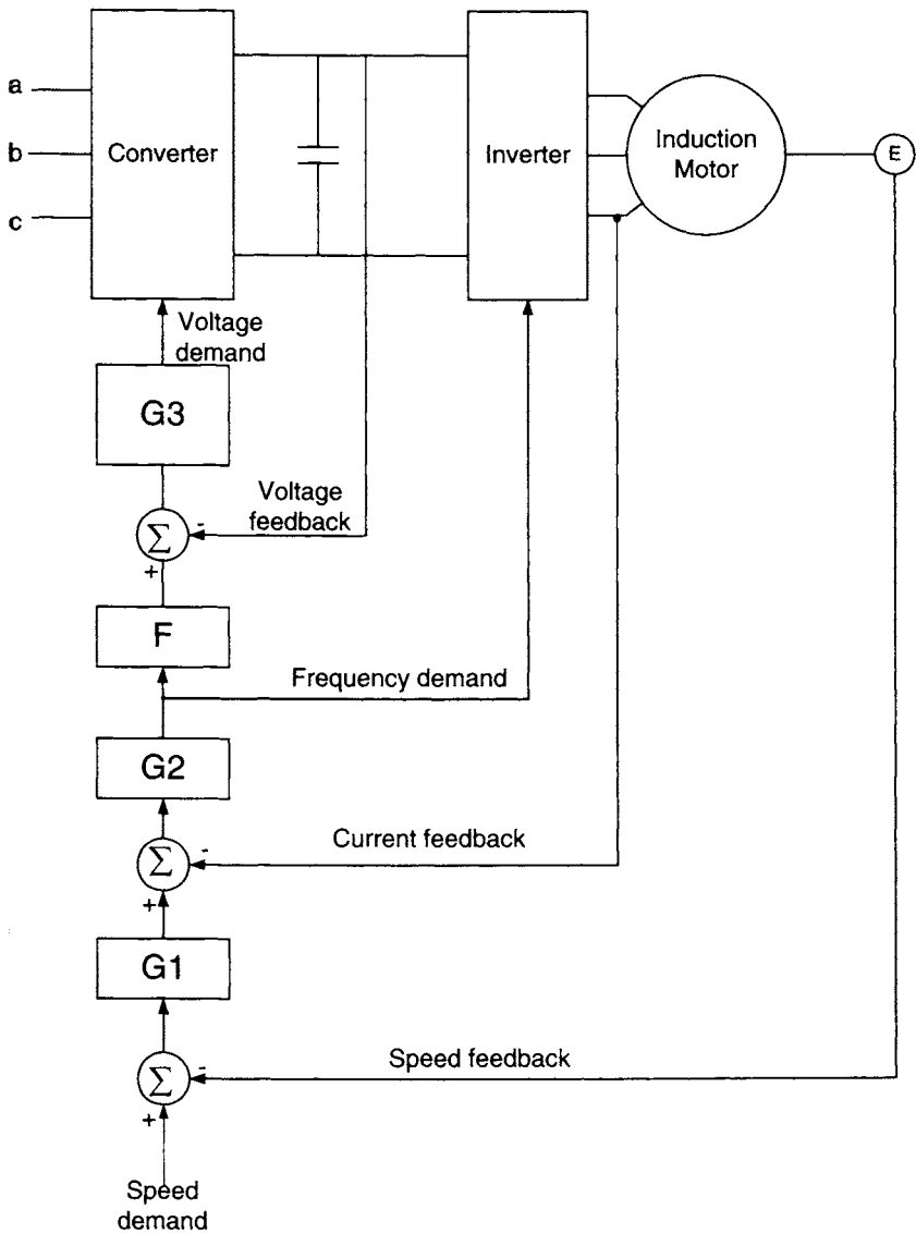
Figure 7.6. Block diagram of the variable-voltage, variable-frequency inverter: F is a function generator that defines the link voltage demand as a function of the inverter frequency; G1 , G2 and G3 are gain blocks within the control loops.
