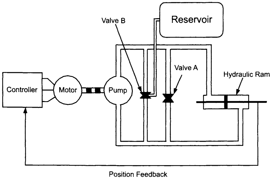
Figure 1.17. Concept of an electrohydraulic Actuator for use in an aircraft. Valve A is a bypass valve that can allow the ram to move under external forces in the case of a failure, while valve B ensures that the pressure of the input side of the pump does not go below that of the reservoir.
