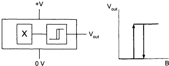
(b) A digital Hall-effect device, a Schmitt trigger is applied to the output of the Hall device to give a clean waveform.
