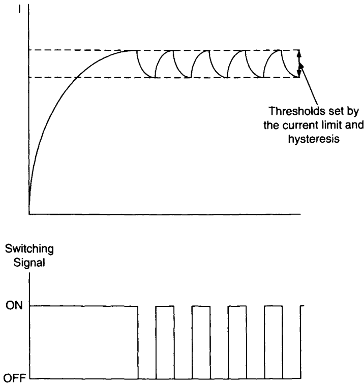
(b) Switching waveforms.
