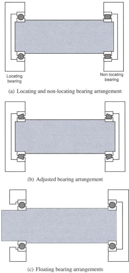
Figure 3.9. Three approaches to supporting a rotating shaft.
