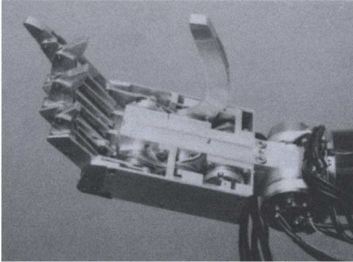
Figure 1.10. The Whole Arm Manipulator's anthropomorphic hand.
