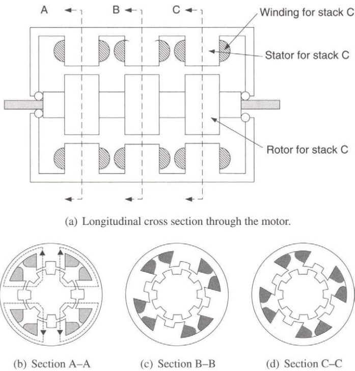
Figure 8.1. A three-stack variable reluctance stepper motor; the flux path is shown for phase A.
