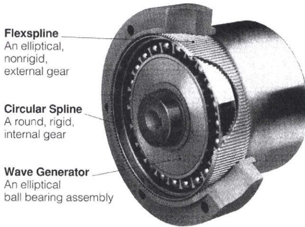
(a) Components of a harmonic gearbox
