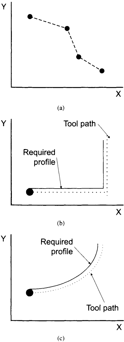
Figure 2.7. Tool paths: (a) point to point, (b) straight cut and (c) contouring. In cases (b) and (c) the tool path is offset by the radius of the cutter or, in the case of a robot application the size of the robot's end effector.
