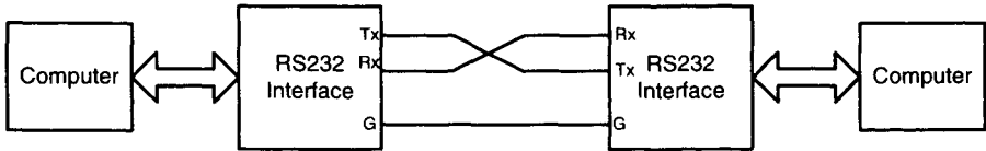
Figure 10.18. The key features of a RS 232 communication link. G is ground, Tx is data transmission, and RX is data receive.
