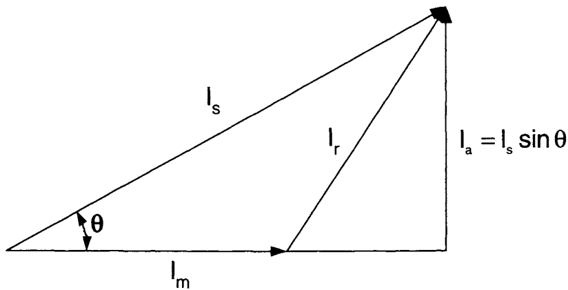
Figure 7.8. The relationship between I_a and I_s as applied to vector control.
