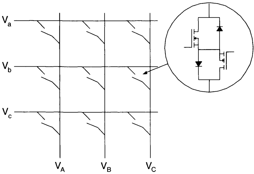
Figure 7.16. Switch layout of a matrix converter. V_a , V_b , V_c are the supply, V_A , V_B , V_C are connected to the load. The load's voltage and frequency is determined by controlling the individual switches.
