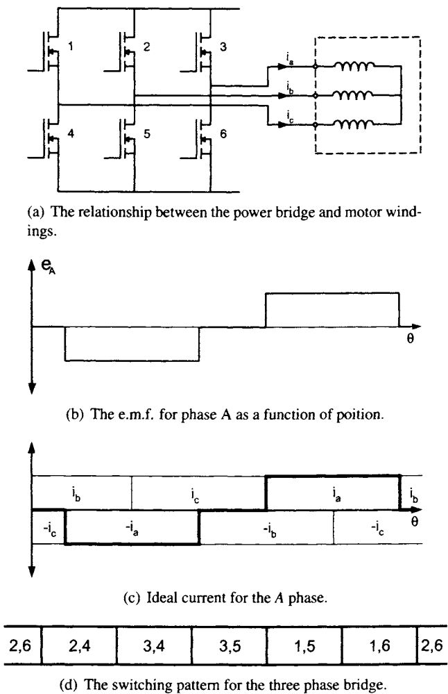
Figure 6.5. The switching requirements for an ideal brushless motor, adapted from Miller (1989).
