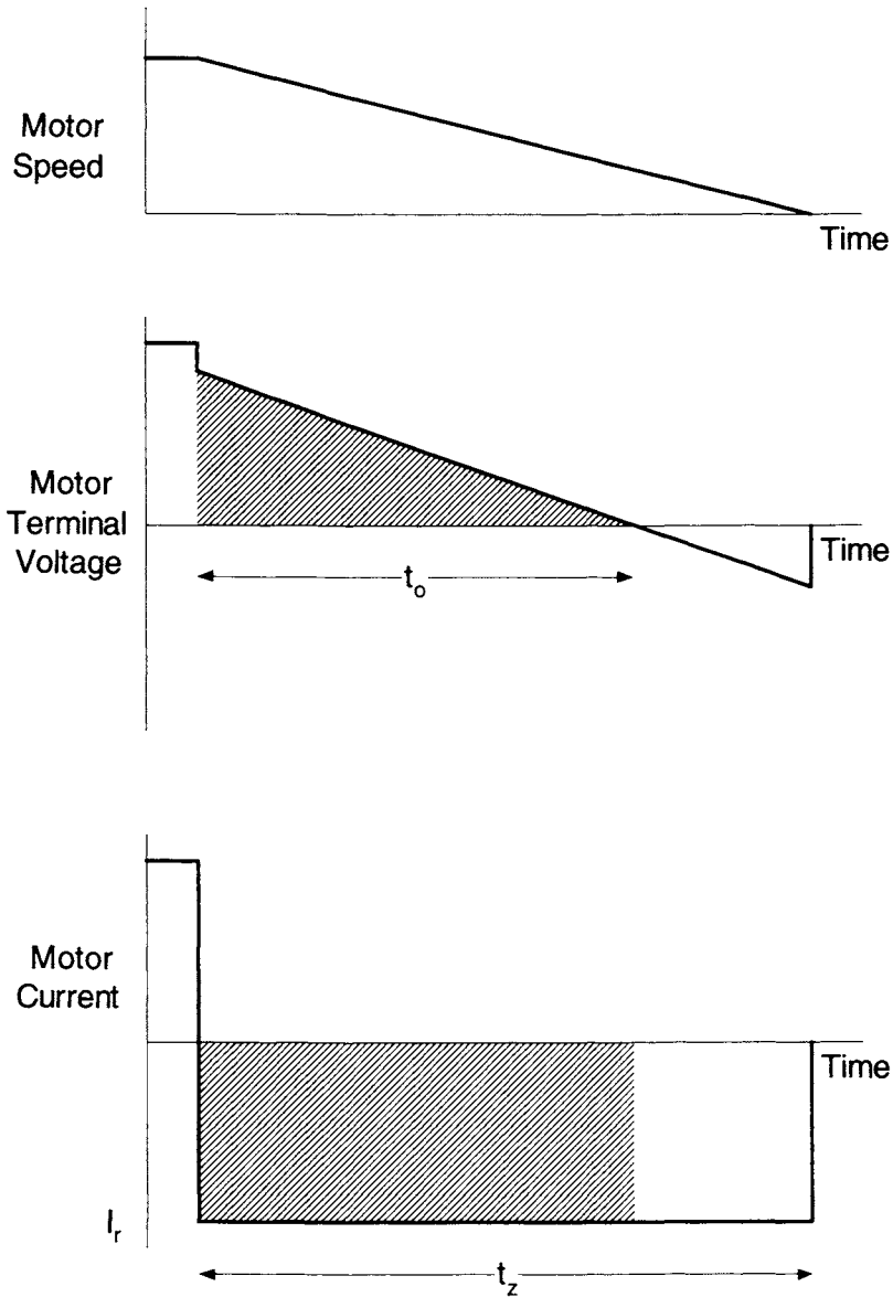
Figure 5.19. A motor's speed, terminal voltage, and armature current during high-speed regeneration. The shaded areas indicates when energy is being returned to the supply from the motor.
