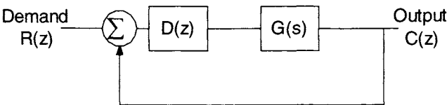
Figure 10.5. An elemental digital-control loop.
