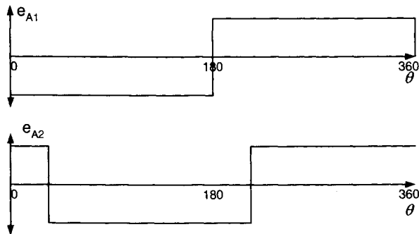
(c) The e.m.f. of the individual coils.
