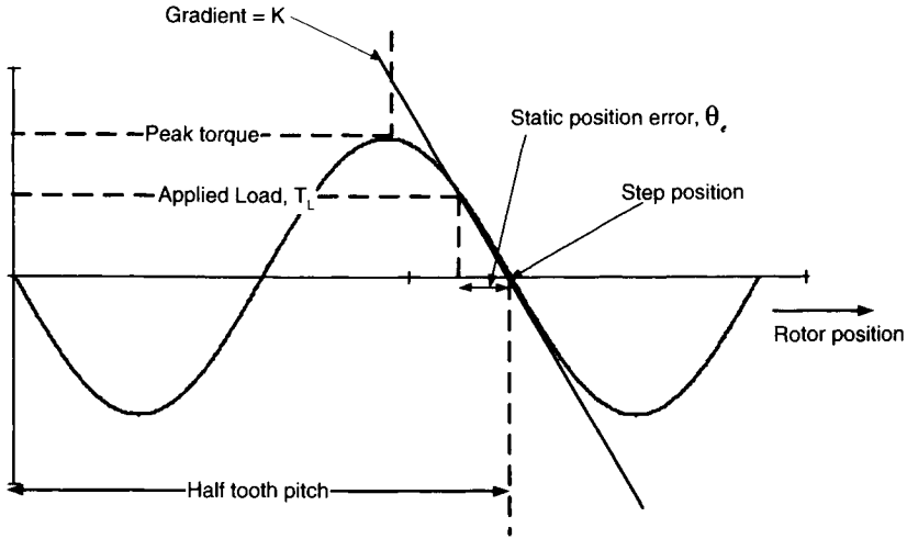
Figure 8.5. Static-torque rotor-position characteristics showing the static position error, \theta_e due to the applied load T_L and the motor stiffness, K .
