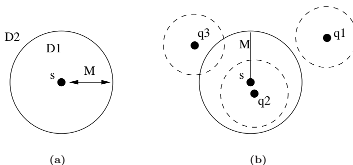
FIGURE 36.7: (a) The vantage sequence s and partitioning of the database into two subsets D_1 and D_2 . M is the median distance to s . (b) An illustration of the three cases for querying the VP-tree: Prune left sub-tree for q_1 , and right sub-tree for q_2 . Search both left and right sub-trees for q_3 .
