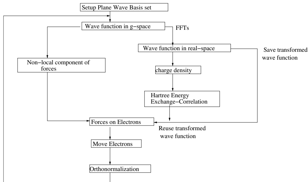
FIGURE 34.6: Schematic flowchart of the implementation of the CP algorithm
