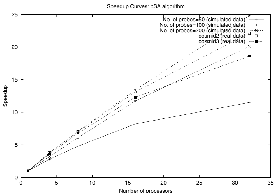
FIGURE 11.8: Speedup curves for the PILM pSA algorithm on an SMP cluster.
