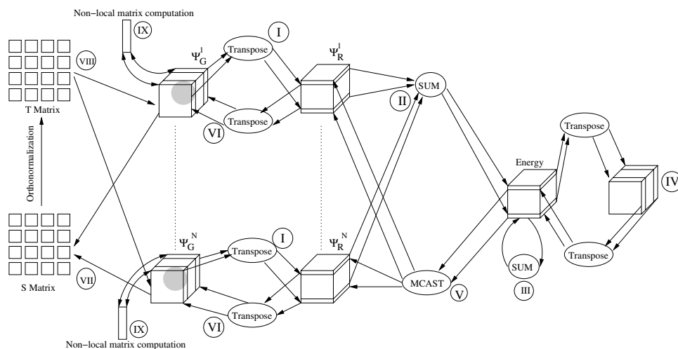
FIGURE 34.7: Parallel structure of our implementation. Roman numbers indicate phases
