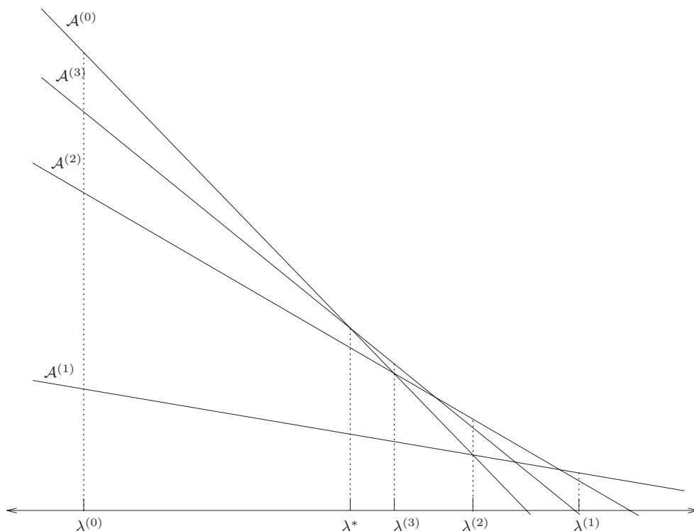
FIGURE 4.5: Newton's method for ray shooting.
