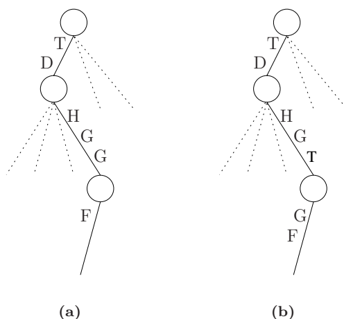
FIGURE 6.14: Suppose the NC-spectrum graph in Figure 6.13 (b) is used in our search. (a) A path that matches the peptide TDHGGF completely, when F is encountered in the search. The peptide TDHGGF is returned as a candidate peptide. (b) A path with an insertion T in the middle (between the two G's), the peptide is also returned as a candidate.
