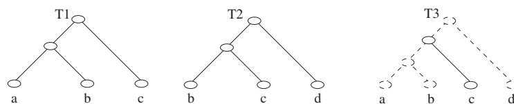
FIGURE 20.1: The supertree T3 contains the branching information of the input trees T1 and T2 . The branching information of the dashed subtree tree in T3 is not contained in either tree T1 or tree T2 , but derives from the branching information of tree T1 and T2 together.
