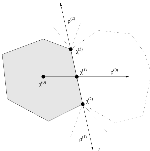
FIGURE 4.6: Ray shooting to determine an edge of the region of optimality of alignment \mathcal{A}^{(0)} .
