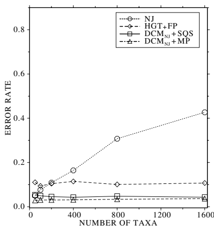
FIGURE 21.2: The performance of DCM1_{NJ} with different techniques used in Phase II, compared to NJ and to another afc method, HGT+FP, as a function of the number of taxa. In this experiment we simulated evolution of sequences with 1000 sites down uniform distribution random trees with branch lengths drawn from the same distribution under the Kimura 2-parameter model [23] of evolution. K2P distances were used as inputs to each method.
