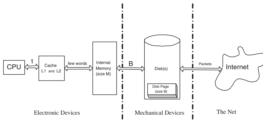
FIGURE 35.1: An example of memory hierarchy of a modern computer.
