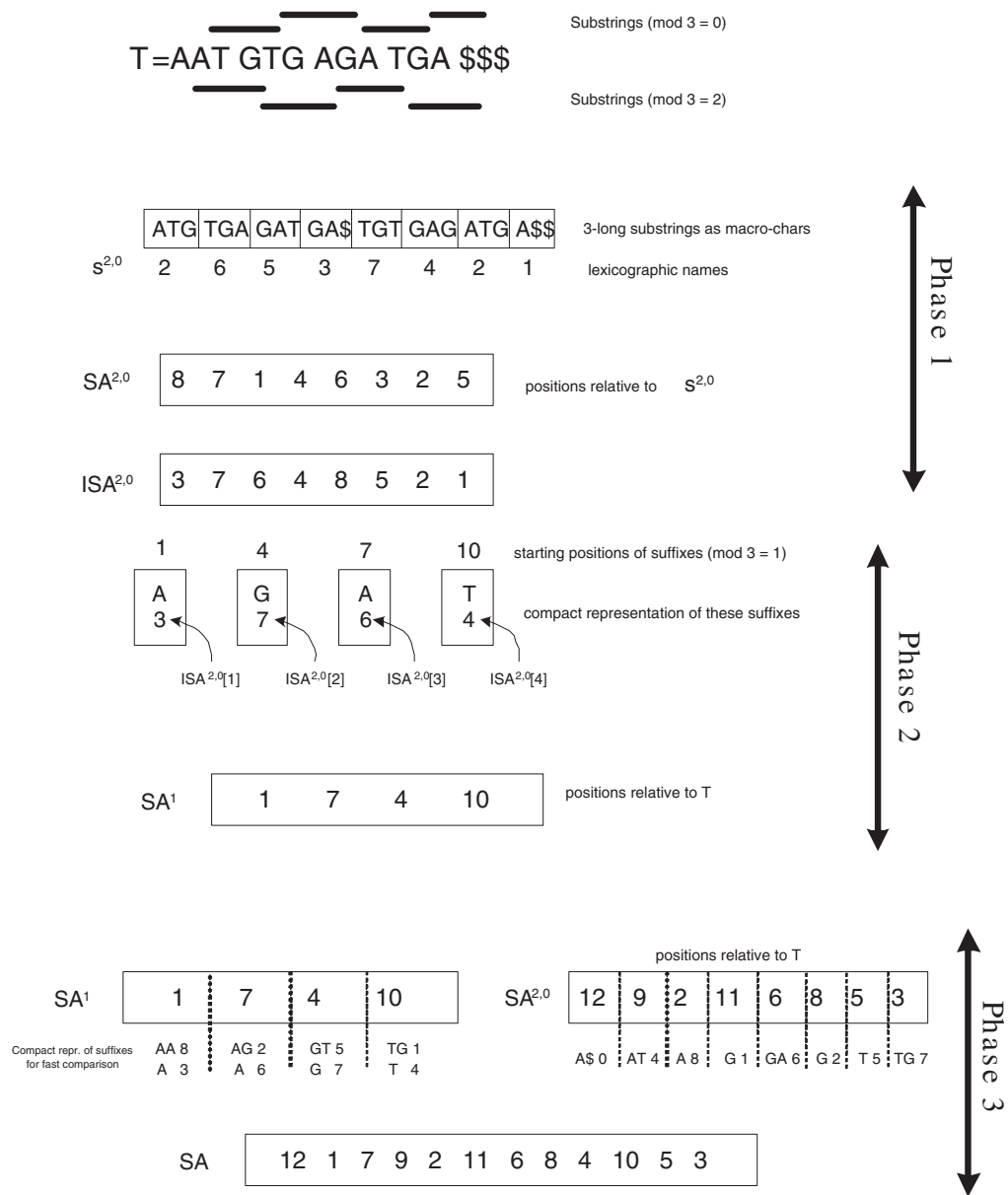
FIGURE 35.4: A running example of the Skew algorithm on T = \text{AATGTGAGATGA} .
