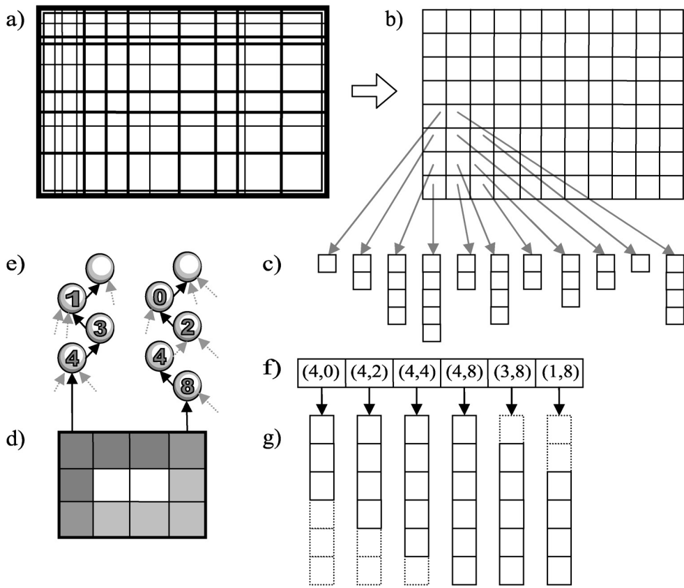
FIGURE 1.8: From the block decomposition of the dynamic programming table (a), we create an index (b) of size O((\frac{hn}{\log n})^2) that points to the score column stored for each block (c). Each block (d) points to its corresponding node in the two trie indexes (e). Travelling up the path of these two trees, we can create a temporary array (f) that collects the rows needed to access the path matrix for this block (g) in constant time. Refer to Figure 1.7 for a description of the path matrix.
