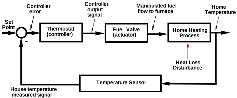
FIGURE 28.4: Diagram showing components of a typical feedback system.
