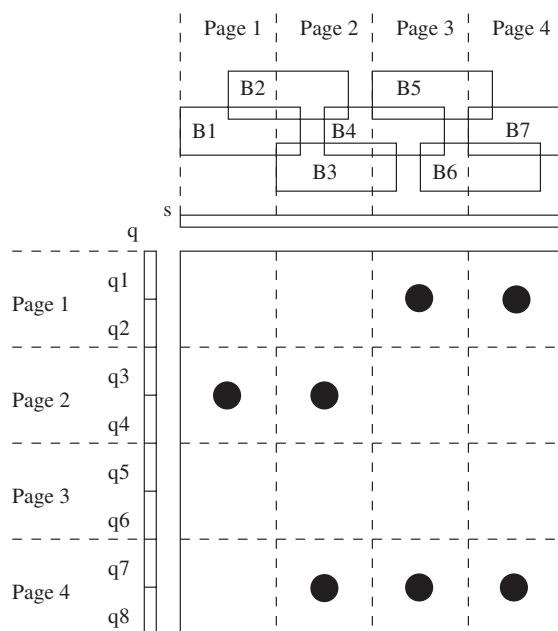
FIGURE 36.14: The match table created on sequences q and s . q is partitioned into 8 subsequences q_1, \dots, q_8 . The MRS index structure built on s contains 7 MBRs B_1, \dots, B_7 . Both q and s fit into 4 pages. The black dots represent the marked entries of the match table.
