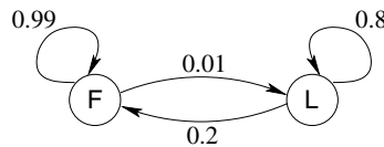
FIGURE 4.9: State transition diagram for a simple Markov model.
