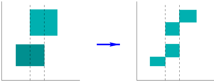
FIGURE 15.14: Two fragments overlapping on the x -axis but not on the y -axis are subdivided into four refined fragments.
