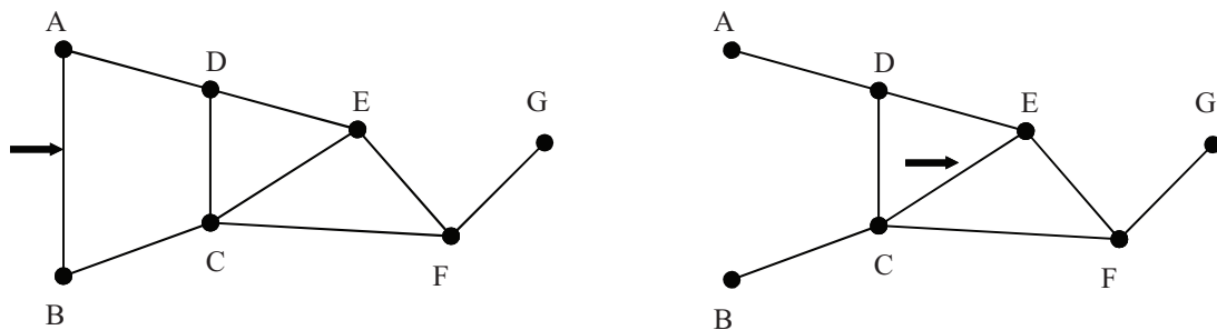
FIGURE 9.5: Deleting an edge from a chordless cycle resulting in an asteroidal triple and vice versa
