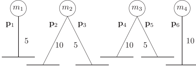
FIGURE 10.11: A 1-CSR problem instance with 3 overlap components C_1 = \{\mathbf{p}_1, \mathbf{p}_2\} , C_2 = \{\mathbf{p}_3, \mathbf{p}_4\} and C_3 = \{\mathbf{p}_5, \mathbf{p}_6\} .
