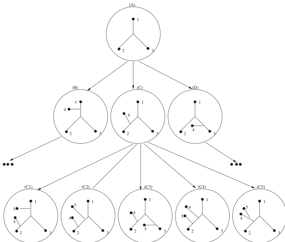
FIGURE 22.1: An example of taxon addition tree generation. At top, tree A is the base three taxa tree. Trees B , C , and D , represent the three four-taxa trees by adding taxon 4 to each of three branches of tree A .
