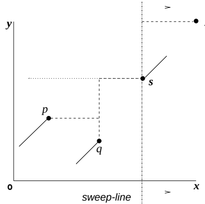
FIGURE 15.8: Points p and q are active end points of the fragments f and \tilde{f} . The start point s of fragment f' is currently scanned by the sweeping line and t is the terminus point.
