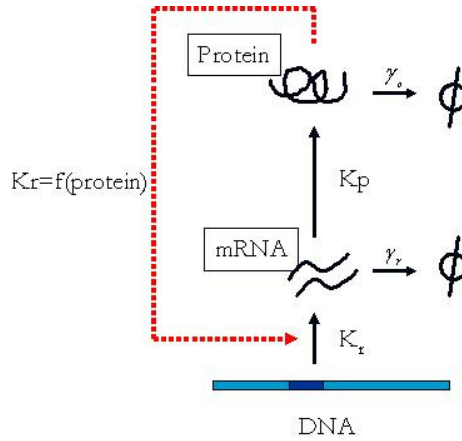
FIGURE 28.9: Simple transcription/translation module. Adapted from [70]
