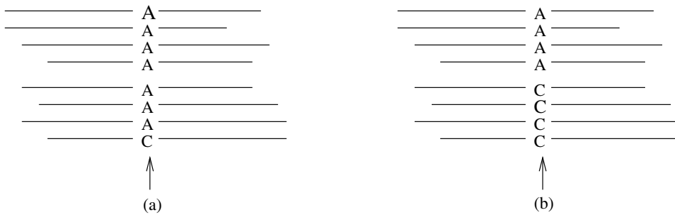
FIGURE 12.5: Overlap layout suggesting a case of a (a) sequencing error, and (b) natural variation.
