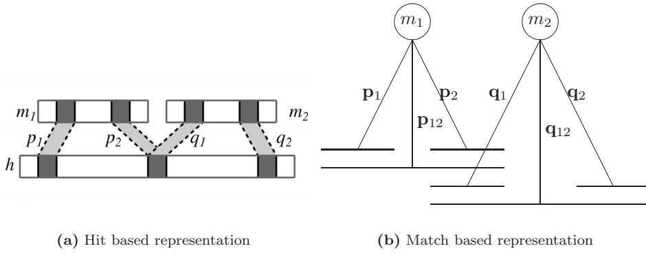
FIGURE 10.8: The match based representation shown on the right displays owners of matches (as circles) and the h -intervals of matches as horizontal lines. \mathbf{p}_1 = \text{match}(p_1) , \mathbf{p}_{12} = \text{match}(p_1, p_2) etc.
