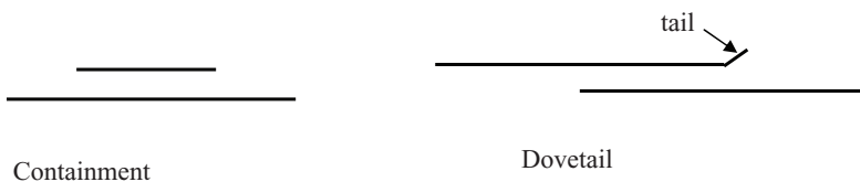
FIGURE 9.3: Consistent overlaps showing containment or dovetail
