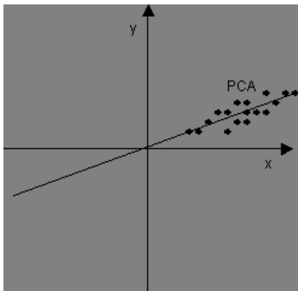
FIGURE 25.1: A two-dimensional set of points with its principal component axis.
