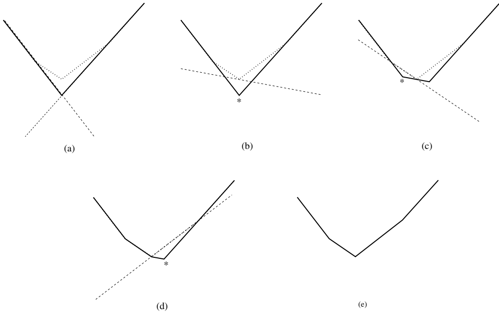
FIGURE 4.8: Executing 1PARAMCONSTRUCT: (a) Initial configuration. The solid curve is the upper envelope of \text{score}(\mathcal{A}^{(l)}, \lambda) and \text{score}(\mathcal{A}^{(r)}, \lambda) ; the dotted curve is Z(\lambda) . (b–d) A series of evaluations and updates. An asterisk is shown next to the breakpoint being verified; the corresponding score function is shown as a dashed line. (e) The final result. Not shown is the verification of the three intermediate breakpoints of W .
