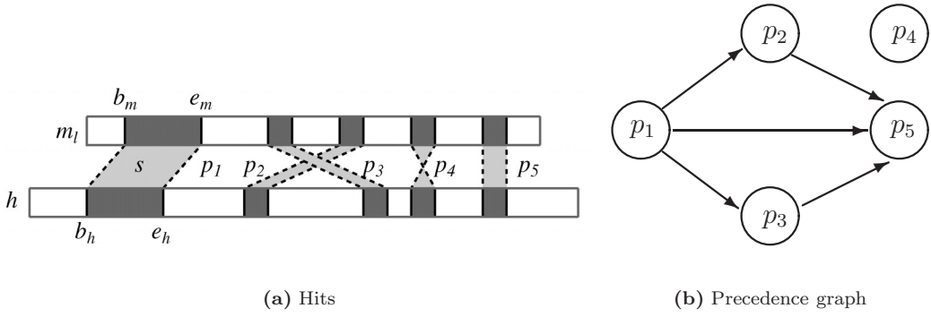
FIGURE 10.7: The hit precedence graph restricted to hits owned by m_l is shown on the right. Hit p_4 is inconsistent with all other hits and appears as an isolated vertex.
