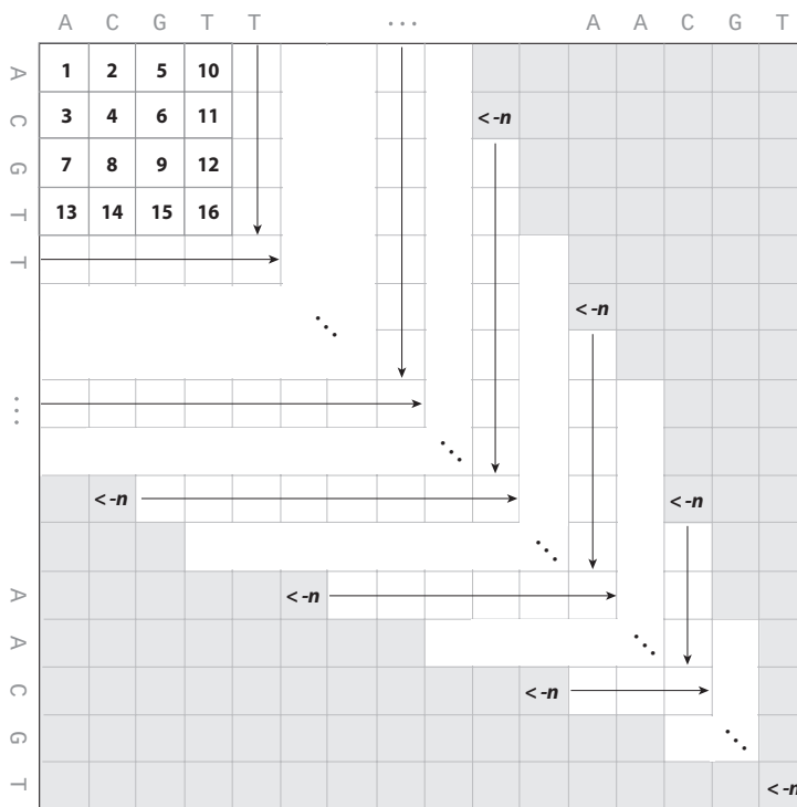
FIGURE 24.6: Linear-time local alignment algorithm. To determine a local alignment in linear-time, one can interleave the row and column construction steps of an alignment matrix in the order indicated by the numbers. The starting boundary of the construction of each row or column is limited by the accumulated negative alignment score boundary, such that when the score is below a certain threshold value -n , one can skip those cells above (in column construction) or to the left (in row construction) during the construction process. This maintains a narrow alignment white band that grows in linear-time. The alignment stops when the row and column boundaries converge.
