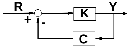
FIGURE 28.8: Elementary feedback system with atuator/system K and controller/sensor C . The goal is for response Y to track reference R , independent of uncertainty and variation in K .
