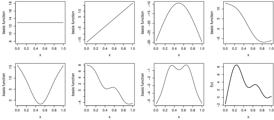
Figure 4.5 Illustration of a rank 7 thin plate regression spline basis for representing a smooth function of one variable, with penalty order m = 2 . The first 7 panels (starting at top left) show the basis functions, multiplied by coefficients, that are summed to give the smooth curve in the lower right panel. The first two basis functions span the space of functions that are completely smooth, according to the wiggleness measure. The remaining basis functions represent the wiggly component of the smooth curve: notice how these functions become successively more wiggly while generally tending to contribute less and less to the overall fit.
