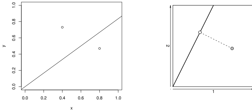
Figure 4.20 The simple, one parameter, linear regression used to illustrate the geometry of penalized regression in section 4.10.3. The left panel shows the least square fit to two response data of a straight line through the origin. The right panel shows the corresponding un-penalized fitting geometry in a space in which there is an axis for each response datum, and the response data are therefore represented by a single point (the grey circle). The thick line shows the model-subspace: the model fitted values must lie on this line. The open circle is the orthogonal projection of the response data onto the model space: i.e. the fitted values.
