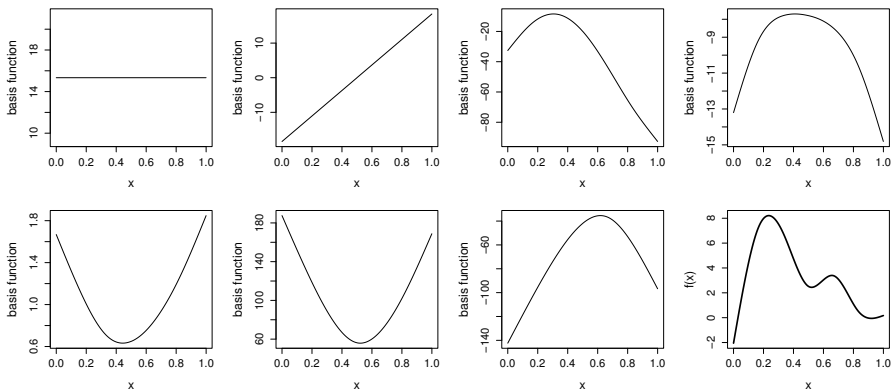
Figure 4.4 Illustration of a thin plate spline basis for representing a smooth function of one variable fitted to 7 data with penalty order m = 2 . The first 7 panels (starting at top left) show the basis functions, multiplied by coefficients, that are summed to give the smooth curve in the lower right panel. The first two basis functions span the space of functions that are completely smooth, according to the wiggleness measure. The remaining basis functions represent the wiggly component of the smooth curve: these latter functions are shown after absorption of the thin plate spline constraints \mathbf{T}^T \boldsymbol{\delta} = \mathbf{0} into the basis.
