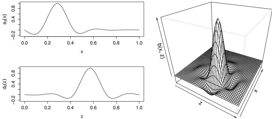
Figure 4.7 How the product of two marginal basis functions for smooth functions of x and z , separately, results in a basis function for a smooth function of x and z together. The two left panels show the 3rd and 5th basis functions for rank 8 cubic regression spline smooths of x and z respectively. The right hand plot shows a_3(x)b_5(z) , one of 64 similar basis functions of the tensor product smooth derived from these two marginal smooths.
