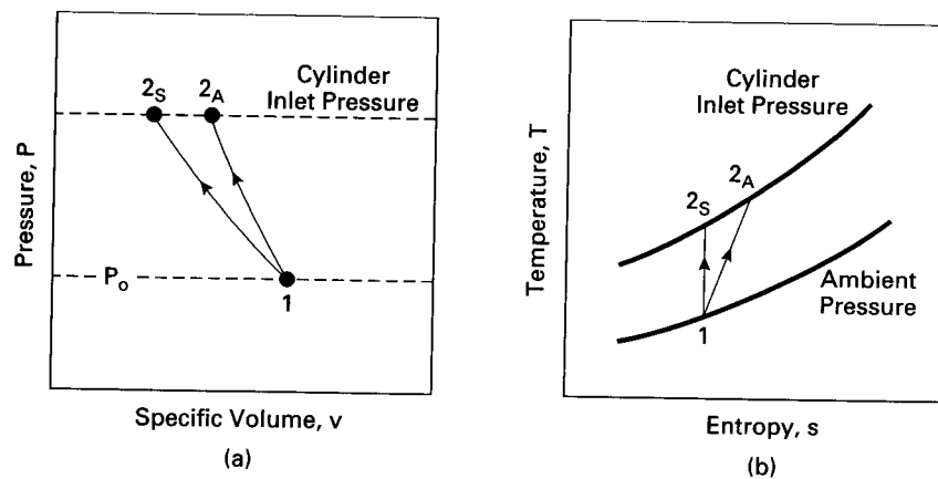
Figure 5-7 Ideal flow process (1-2 s ) and actual flow process (1-2 A ) through a supercharger or a turbocharger compressor in (a) pressure-volume coordinates, and (b) temperature-entropy coordinates.
