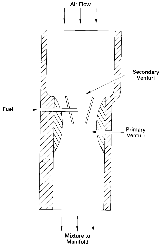
Figure 5-6 Throat of carburetor with secondary venturi. The small secondary venturi gives a large pressure drop and good fuel flow control, while the larger primary throat offers less resistance to the main air flow.
