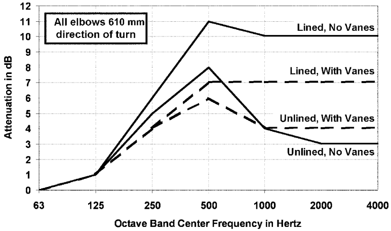
Figure 2-35 Attenuation of rectangular elbows with and without turning vanes (lined and unlined).
