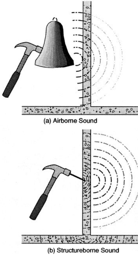
Figure A-1 Airborne and structure-borne sound transmission.
