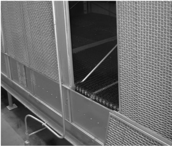
Figure 3-9 Honeycomb water basin silencers installed several centimeters above the water surface to reduce the velocity of the falling water before it hits the basin.
