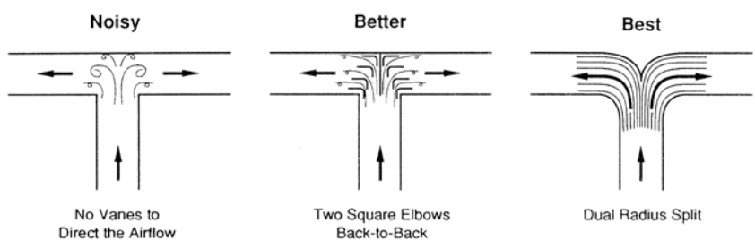
Figure 2-32 Guidelines for minimizing regenerated noise in duct tees.
