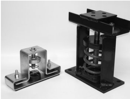
Figure 5-6 Two types of spring floor mounts with seismic/wind-loading standby restraints. The mount on the left is for low loads and static deflections under 25 mm. The mount on the right is for larger loads and static deflections greater than 25 mm.
