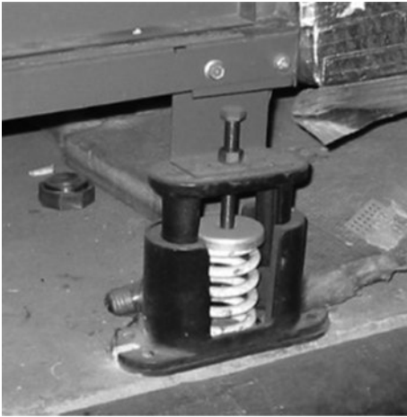
Figure 8-4 Restrained spring isolator with a “short circuit” between its baseplate and equipment mounting plate. This type of isolator has become obsolete and is not recommended for any type of HVAC equipment.
