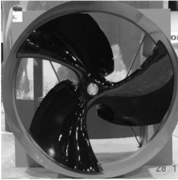
Figure 2-15 Ultra-low-noise propeller fan with backsweppt airfoil blades. Versions of this fan are available with 2, 3, or 4 blades of adjustable blade twist and diameters up to 12.3 m for very large capacities.
