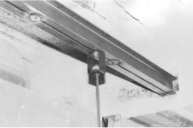
Figure 7-5 Overloaded spring hanger.
