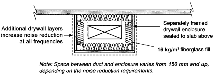
Figure I-22 Noise control duct enclosure.
